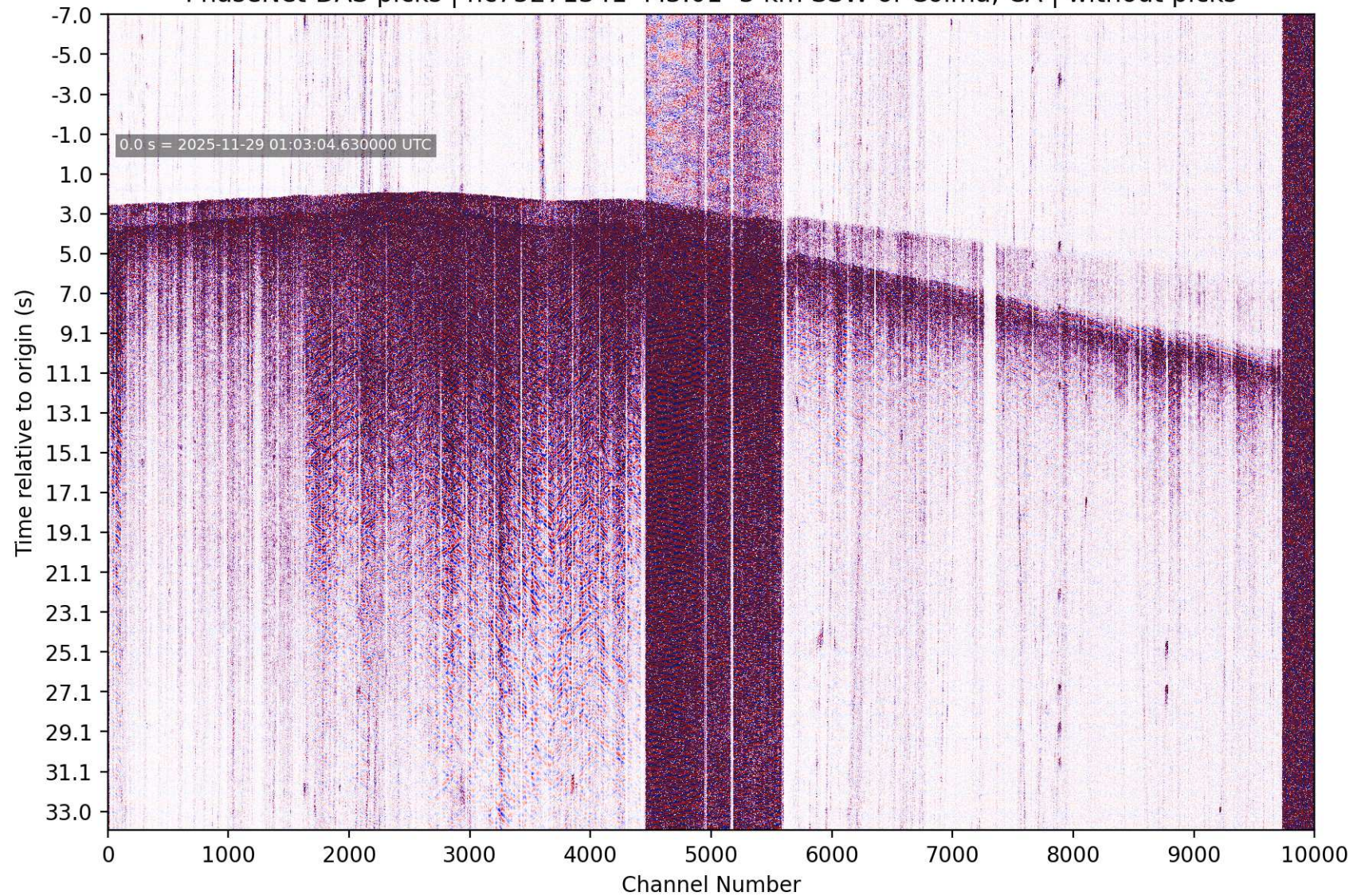
PhaseNet-DAS picks | nc75271341 M3.01 3 km SSW of Colma, CA | without picks
