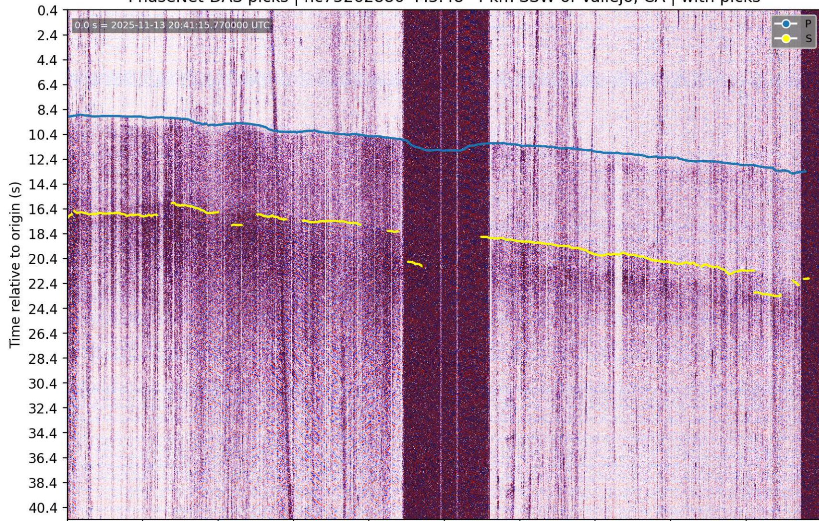
PhaseNet-DAS picks | nc75262886 M3.48 4 km SSW of Vallejo, CA | without picks
