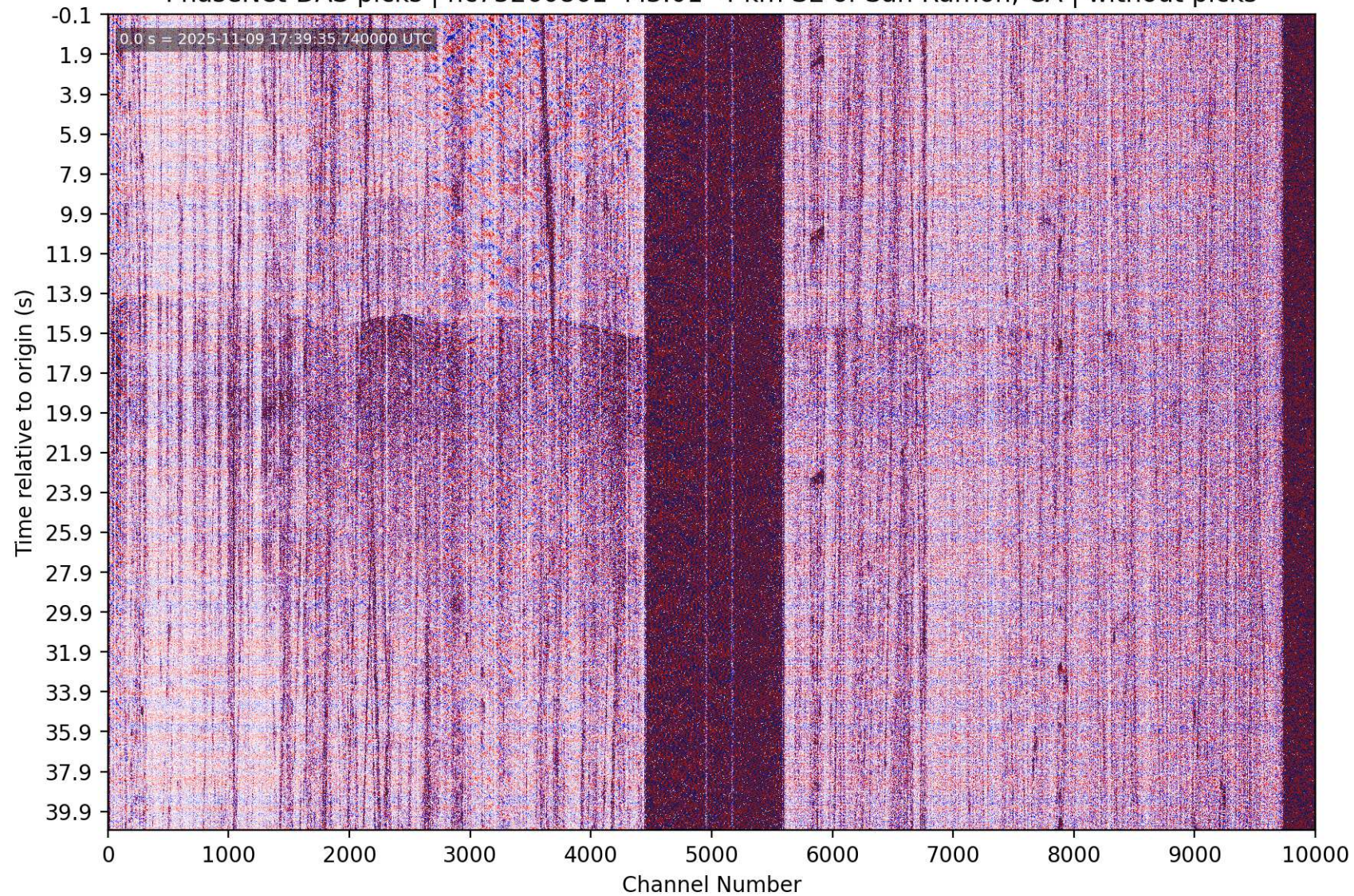
PhaseNet-DAS picks | nc75260861 M3.01 4 km SE of San Ramon, CA | without picks
