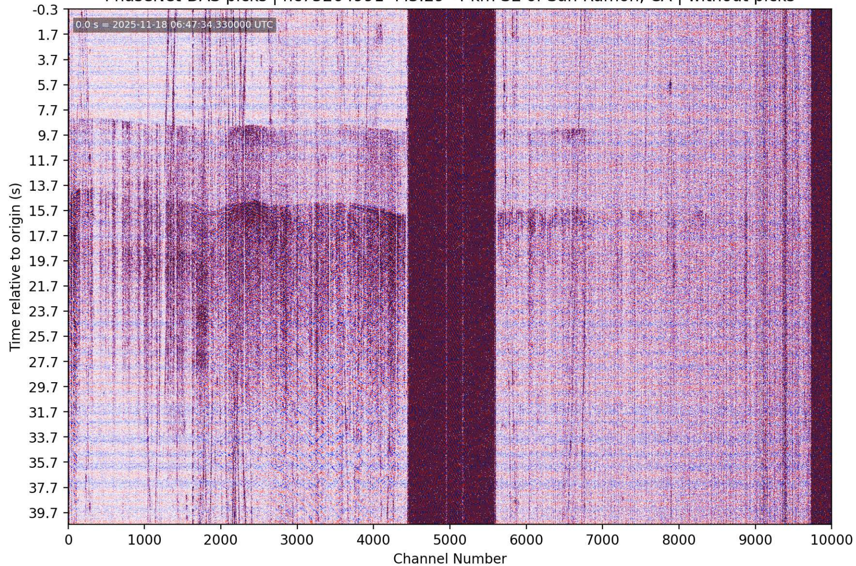
PhaseNet-DAS picks | nc75264991 M3.29 4 km SE of San Ramon, CA | without picks
