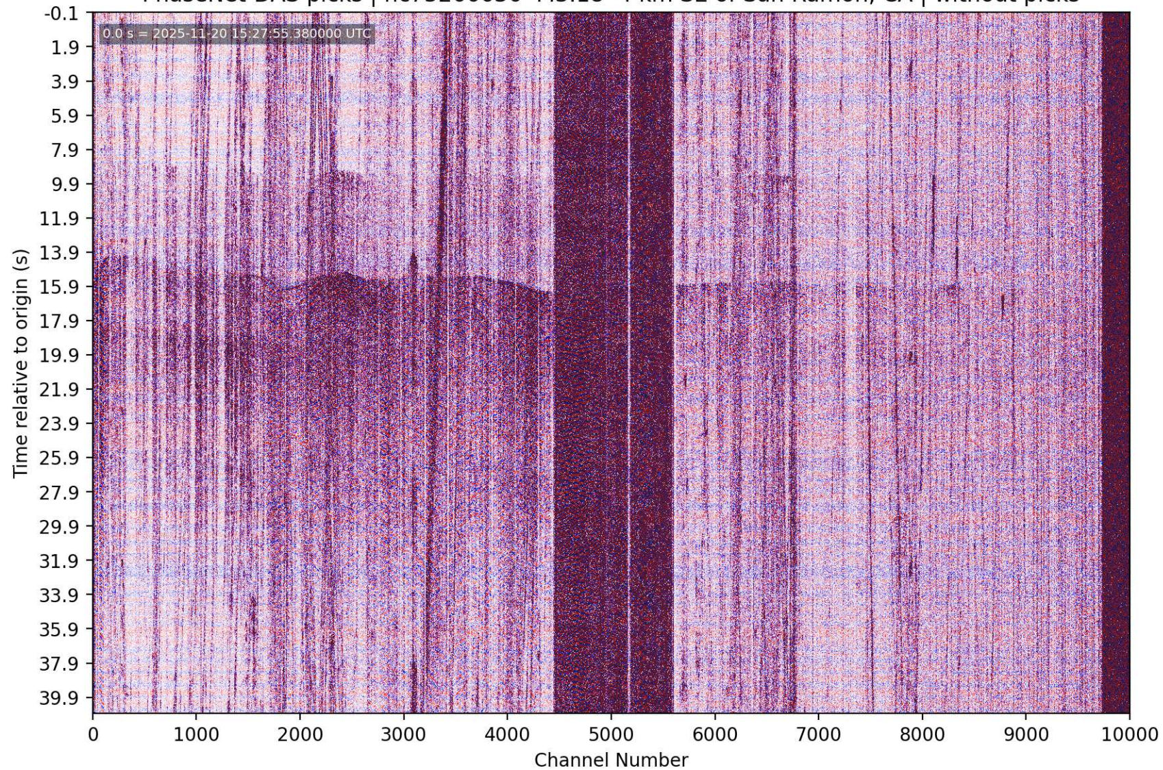
PhaseNet-DAS picks | nc75266636 M3.18 4 km SE of San Ramon, CA | without picks
