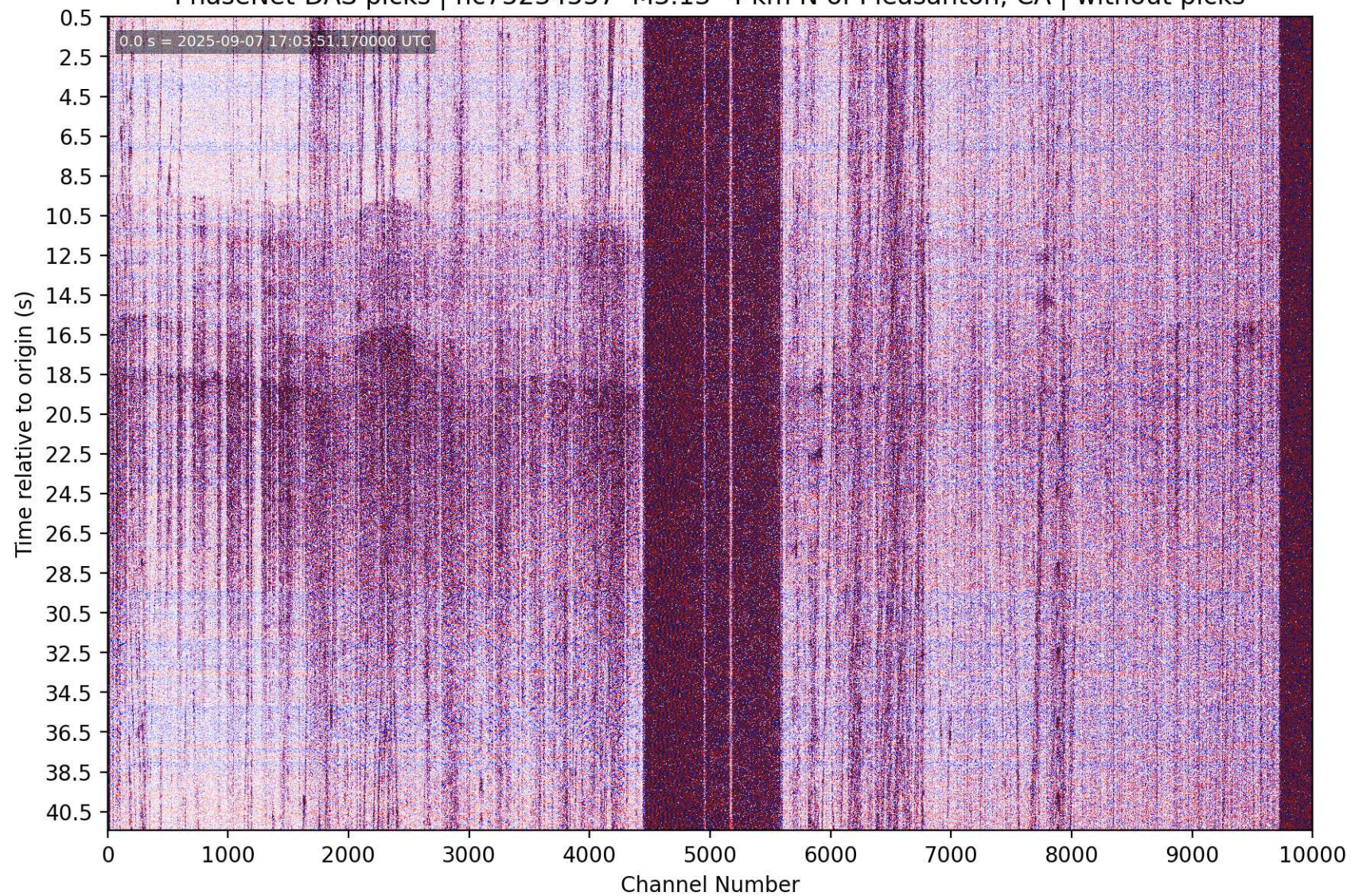
PhaseNet-DAS picks | nc75234557 M3.13 4 km N of Pleasanton, CA | without picks
