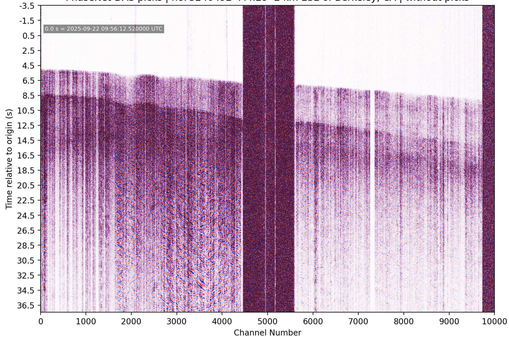
PhaseNet-DAS picks | nc75240492 M4.29 2 km ESE of Berkeley, CA | without picks
