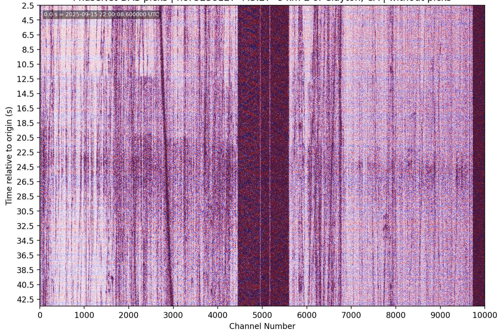
PhaseNet-DAS picks | nc75238127 M3.27 8 km E of Clayton, CA | without picks
