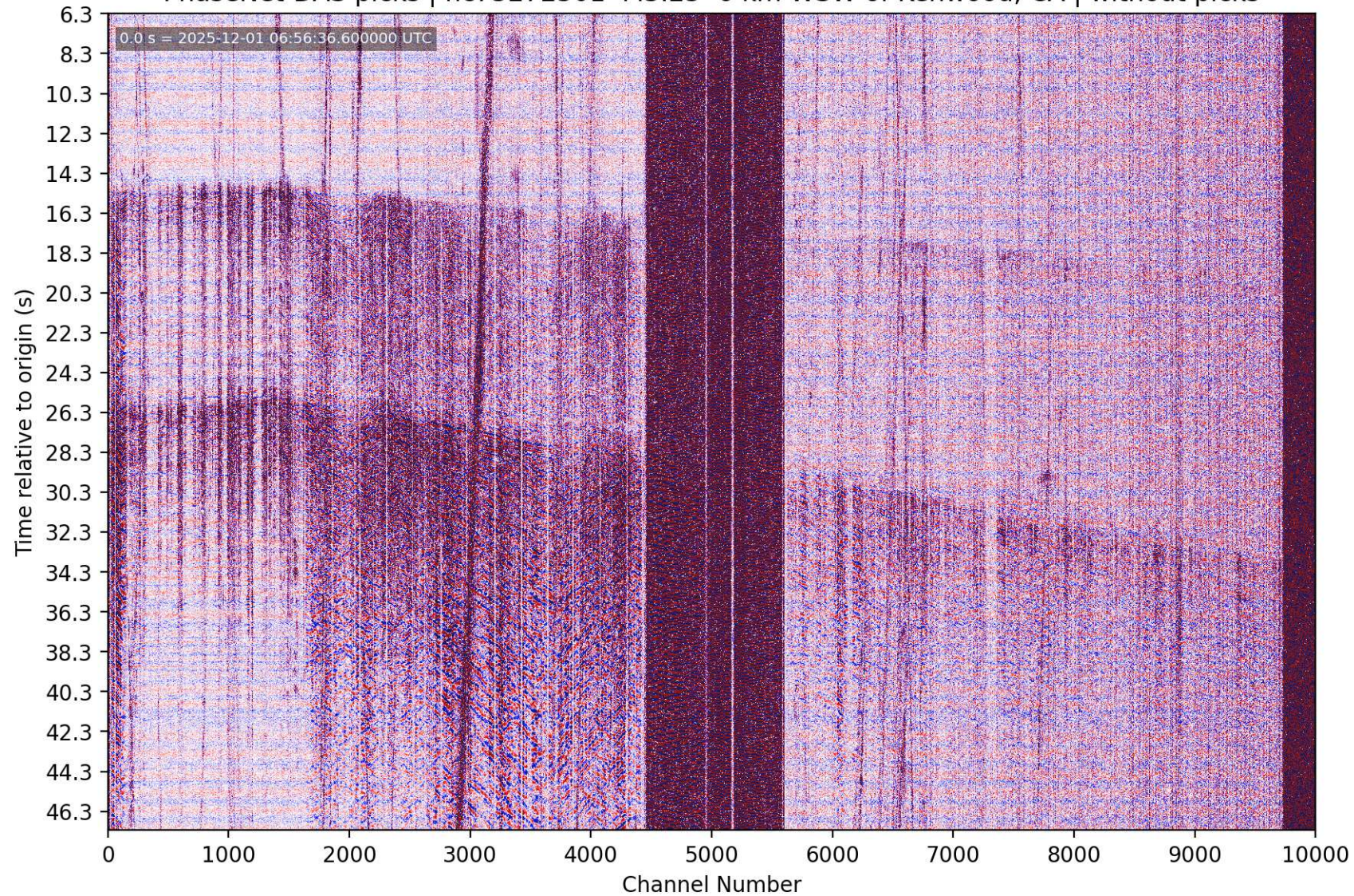
PhaseNet-DAS picks | nc75272501 M3.25 6 km WSW of Kenwood, CA | without picks
