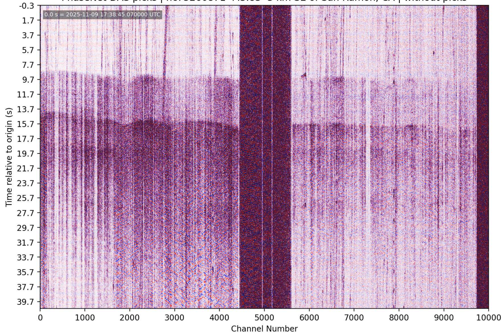
PhaseNet-DAS picks | nc75260871 M3.83 3 km SE of San Ramon, CA | without picks
