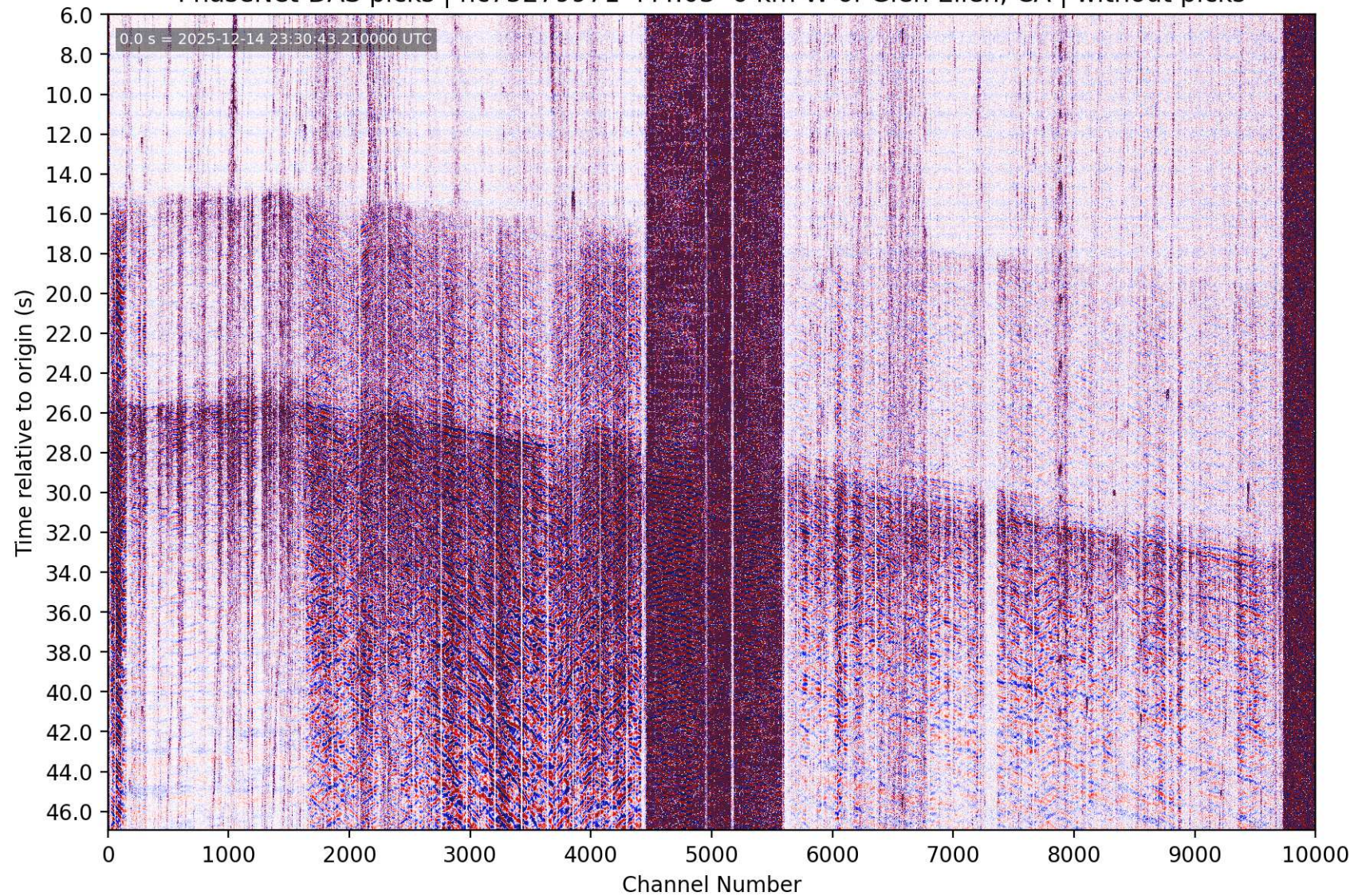
PhaseNet-DAS picks | nc75279971 M4.03 6 km W of Glen Ellen, CA | without picks
