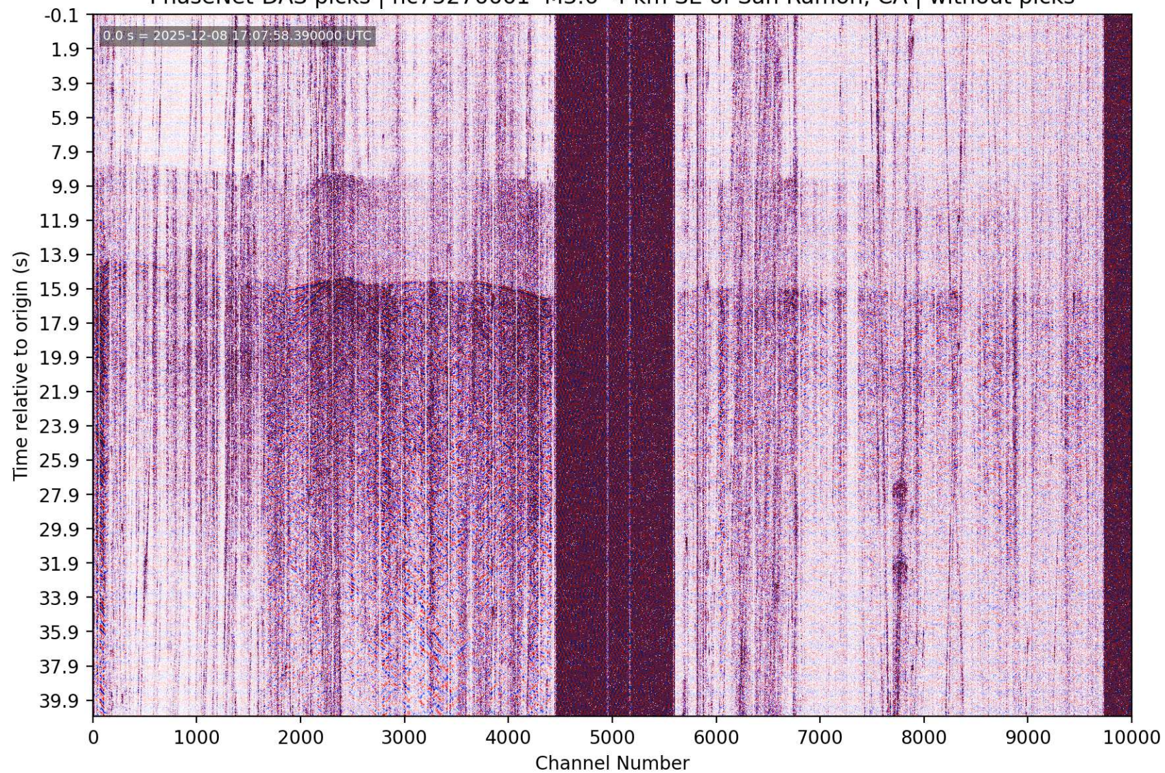
PhaseNet-DAS picks | nc75276661 M3.6 4 km SE of San Ramon, CA | without picks
