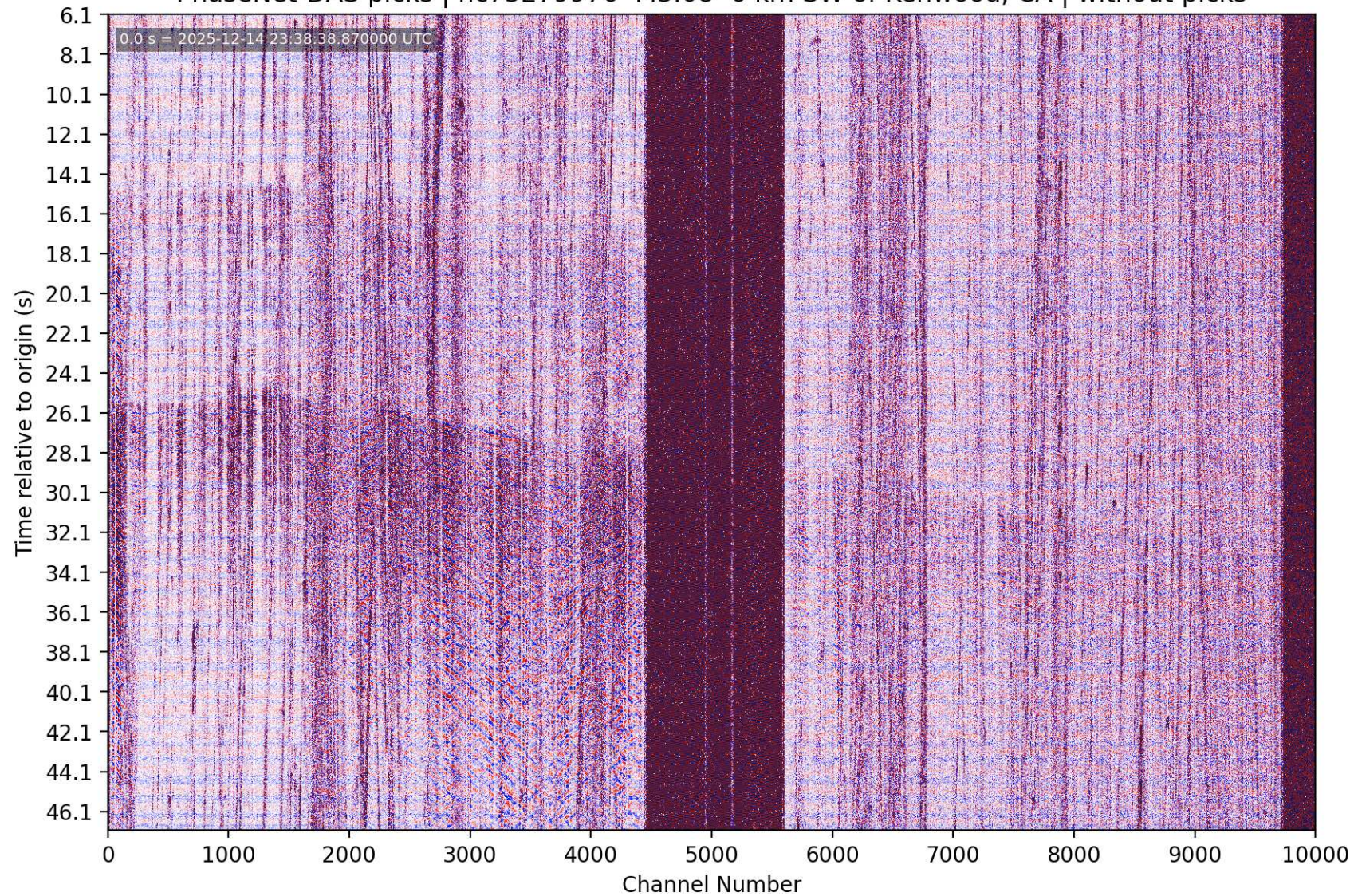
PhaseNet-DAS picks | nc75279976 M3.08 6 km SW of Kenwood, CA | without picks
