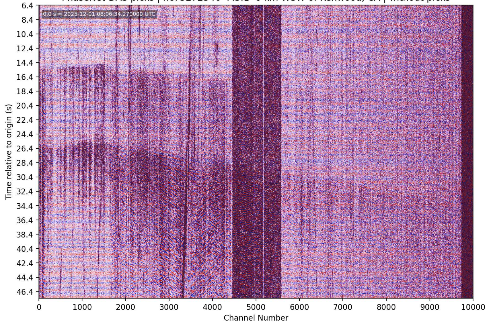
PhaseNet-DAS picks | nc75272546 M3.1 6 km WSW of Kenwood, CA | without picks
