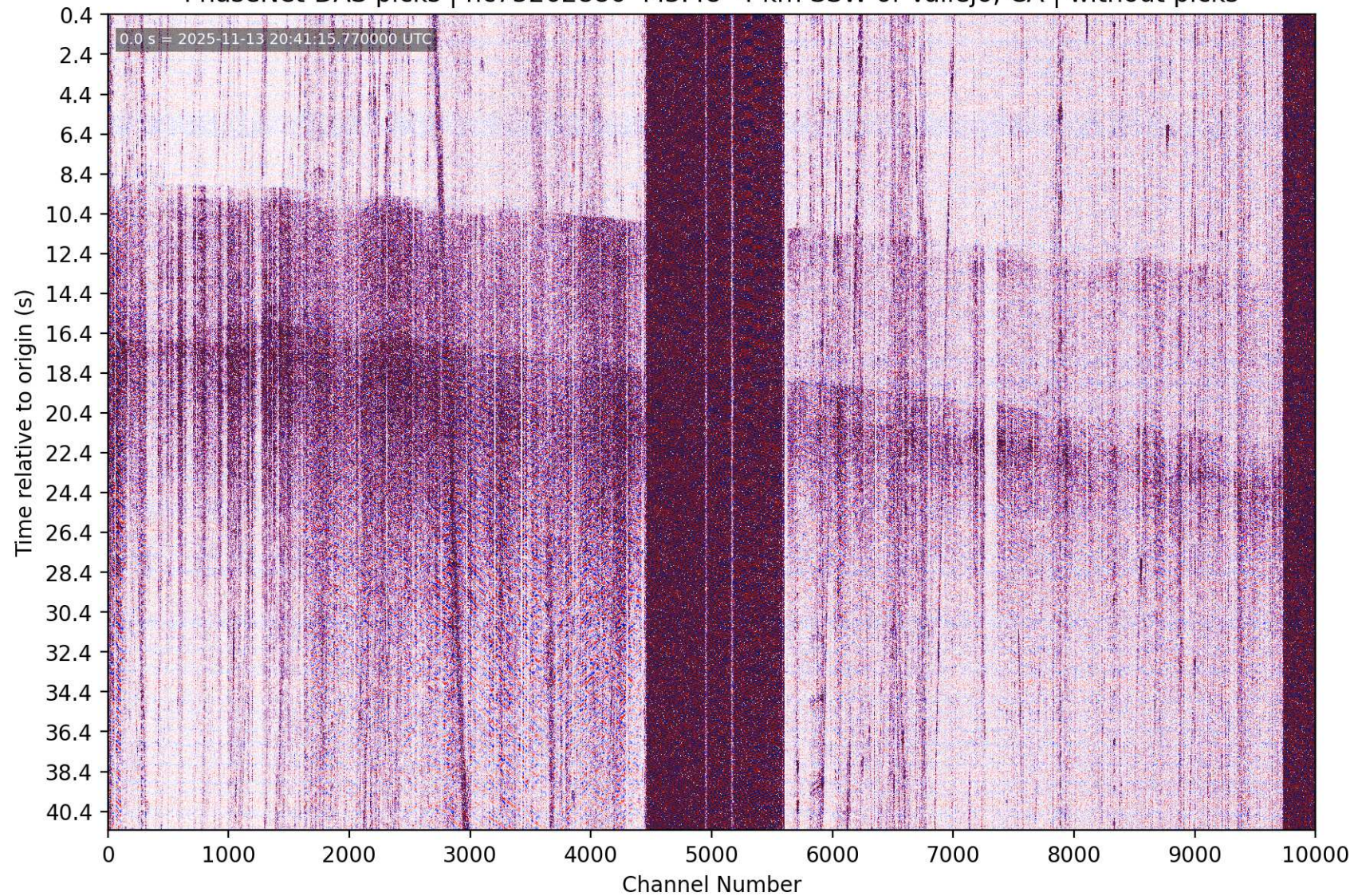
PhaseNet-DAS picks | nc75262886 M3.48 4 km SSW of Vallejo, CA | without picks
