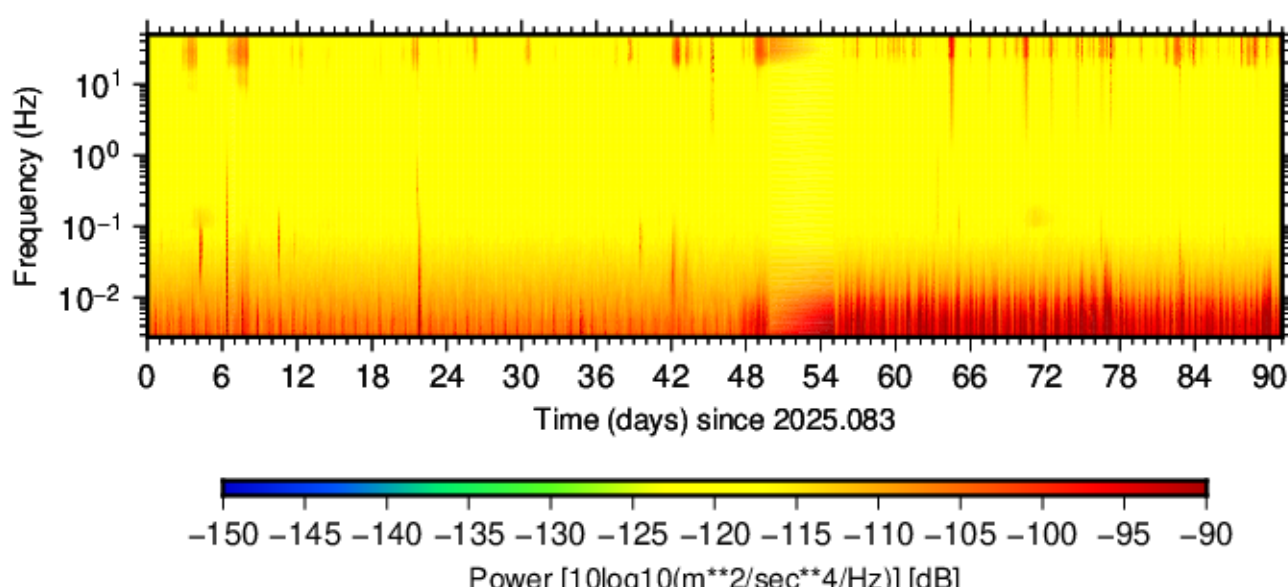
BK.YUBA.HNN.00 (2025.083 - 2025.173)
