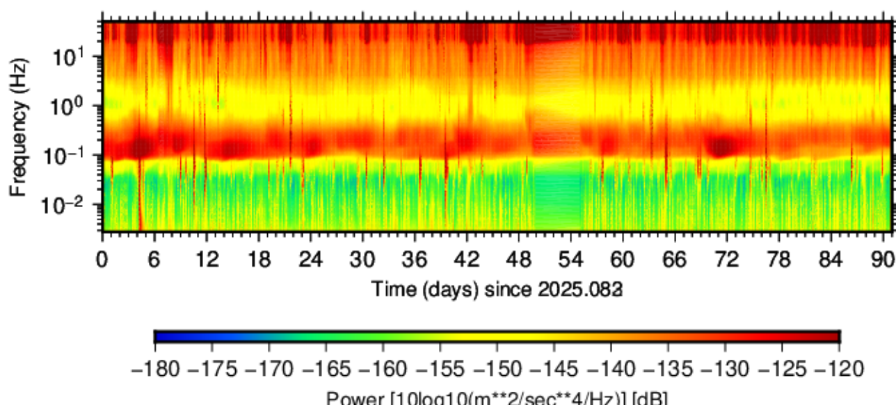
BK.YUBA.HHZ.00 (2025.083 - 2025.173)
