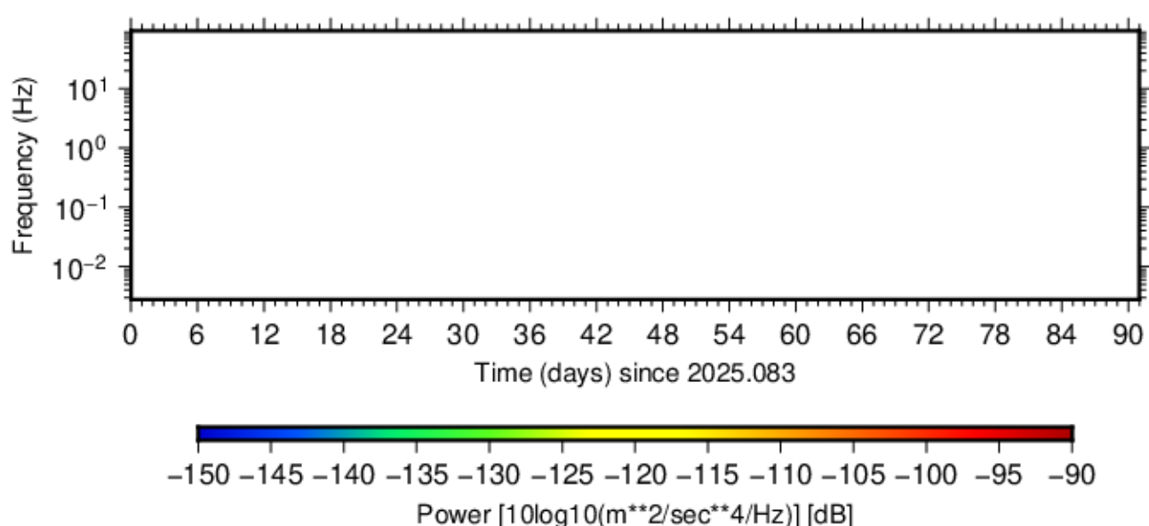
BK.TRAM.HNN.00 (2025.083 - 2025.173)
