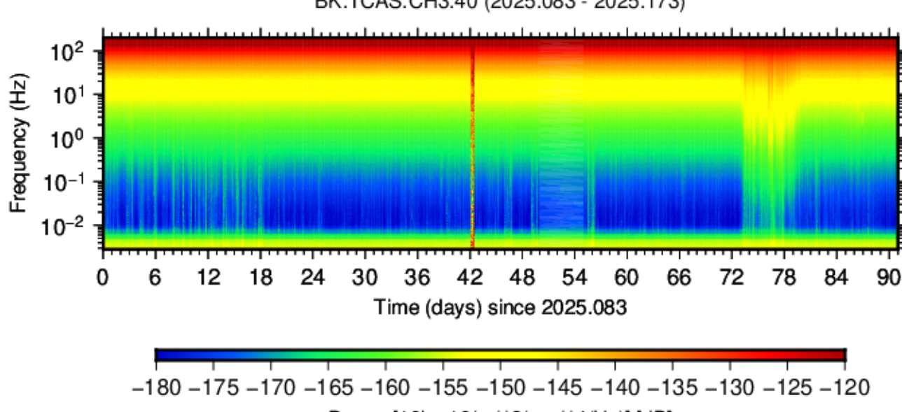
BK.TCAS.CH3.40 (2025.083 - 2025.173)
