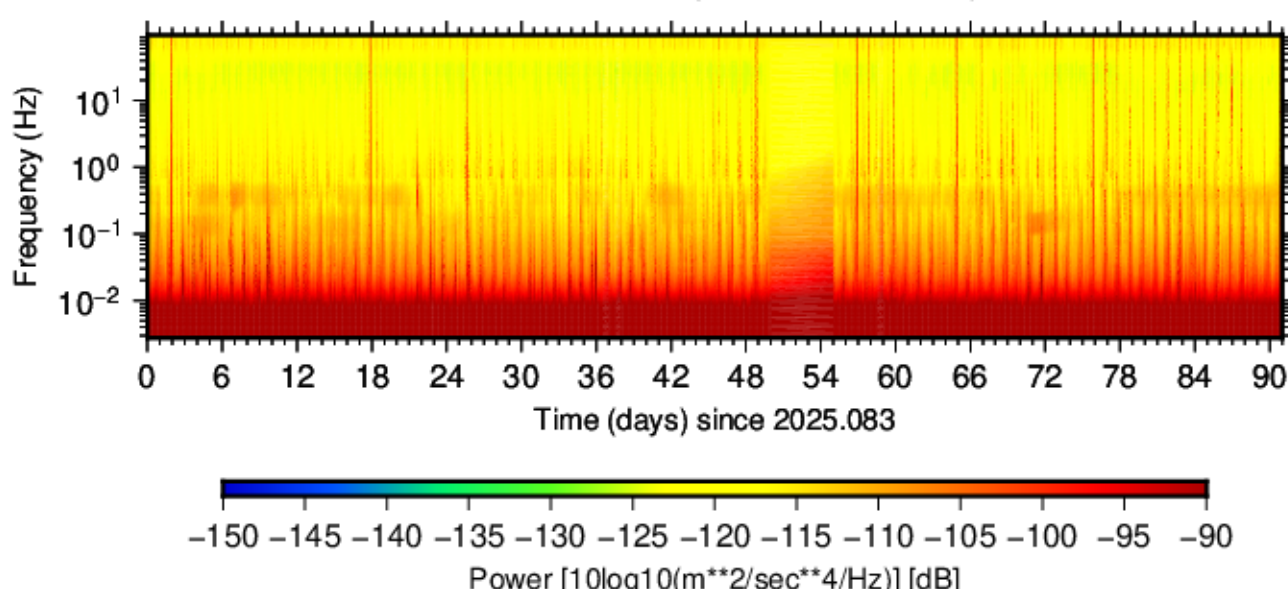
BK.TCAS.HN1.40 (2025.083 - 2025.173)
