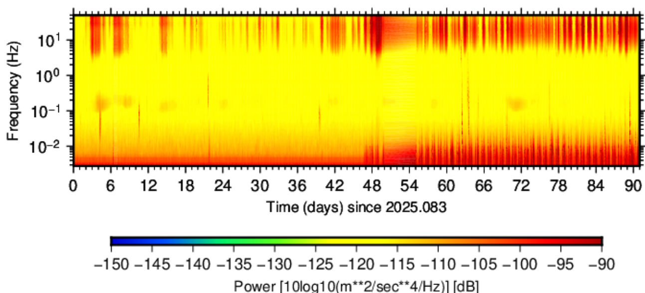
BK.SWNM.HNN.00 (2025.083 - 2025.173)
