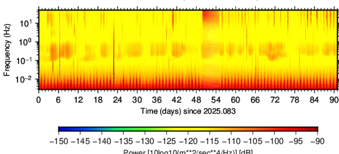
BK.SPAN.HNN.00 (2025.083 - 2025.173)
