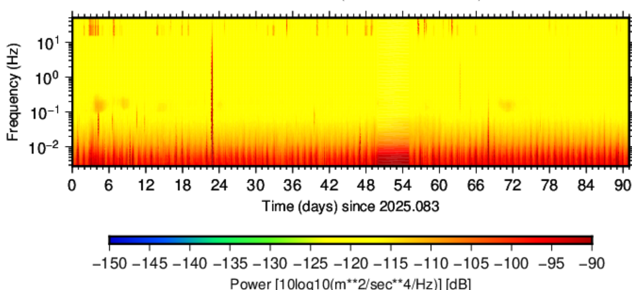
BK.SCOT.HNZ.01 (2025.083 - 2025.173)
