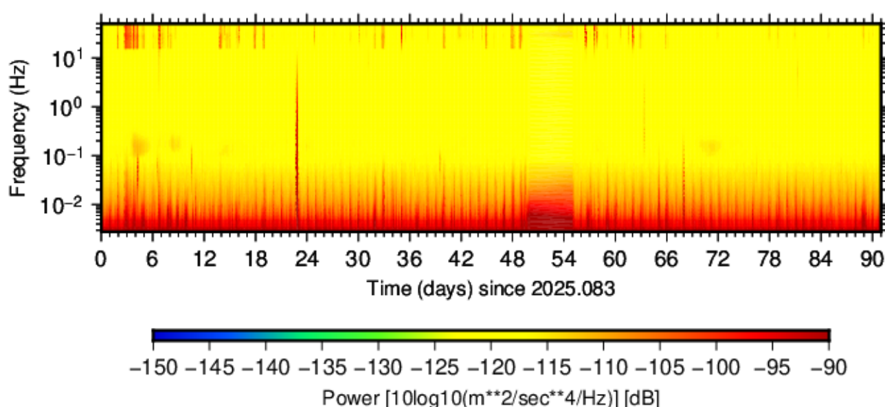
BK.SCOT.HNN.01 (2025.083 - 2025.173)
