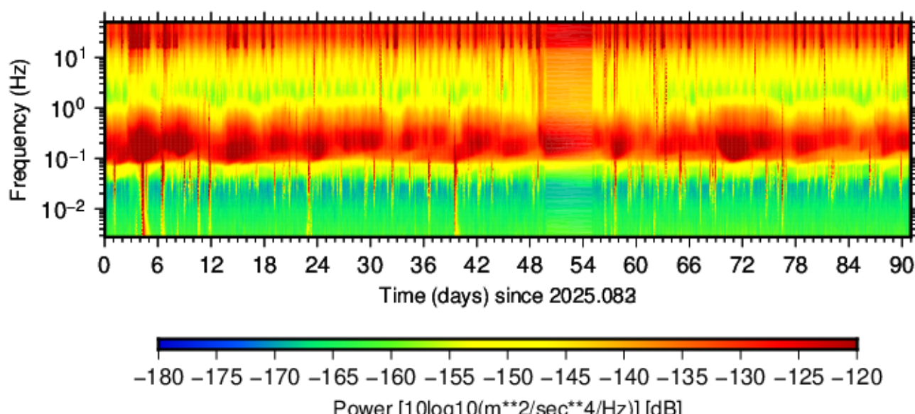
BK.SCOT.HHZ.01 (2025.083 - 2025.173)
