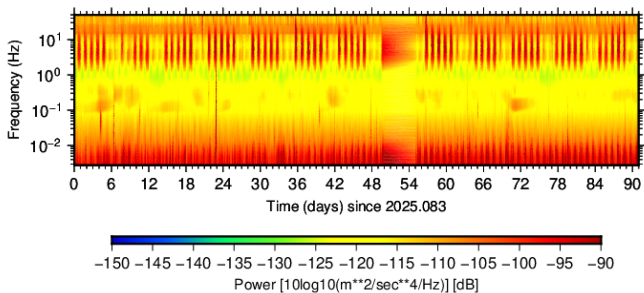
BK.SCCB.HNN.00 (2025.083 - 2025.173)
