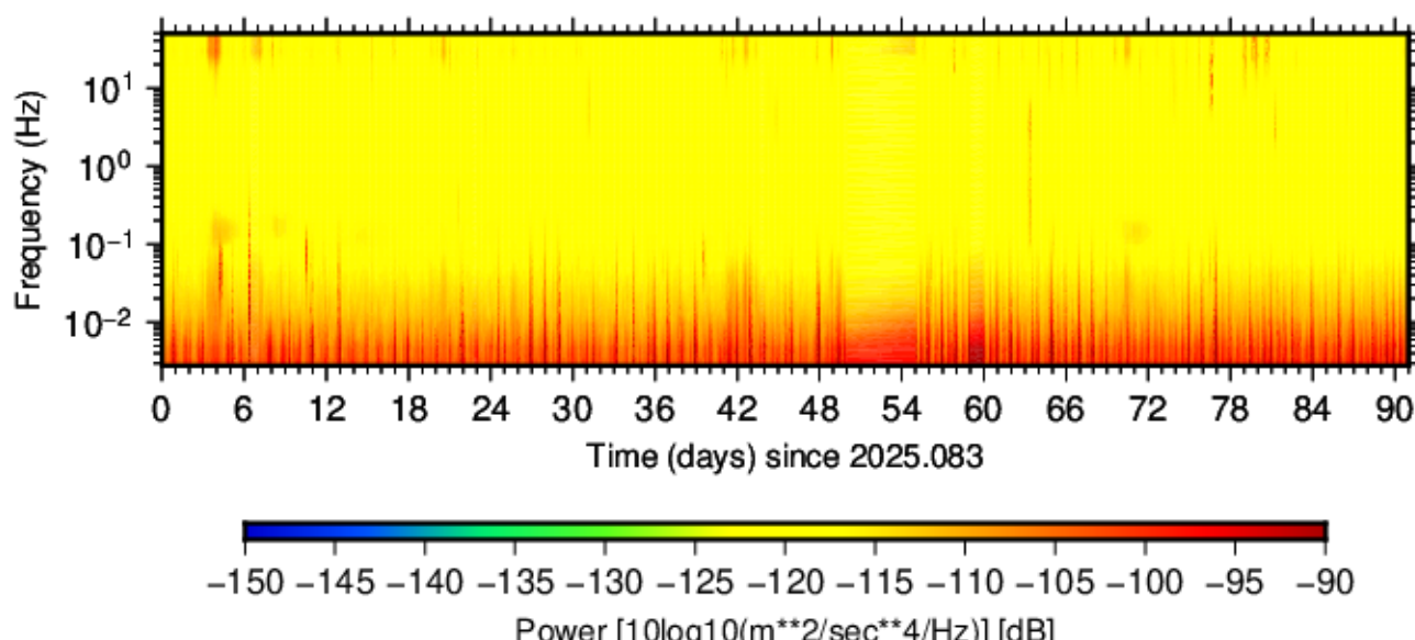
BK.SAGE.HNN.00 (2025.083 - 2025.173)
