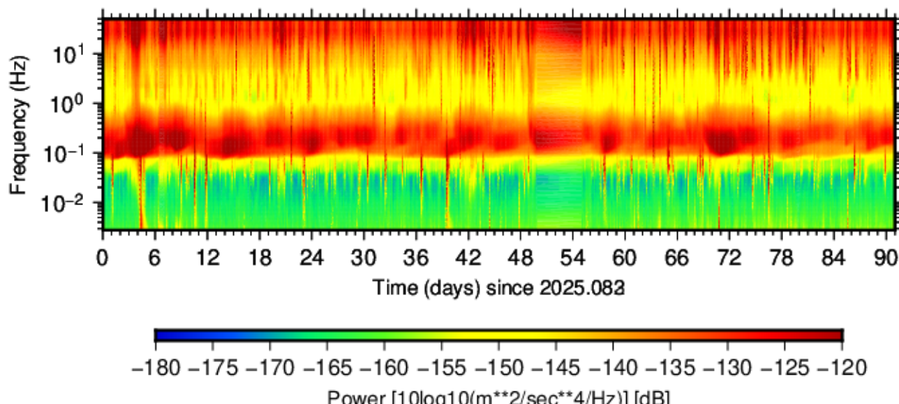
BK.SAGE.HHZ.00 (2025.083 - 2025.173)
