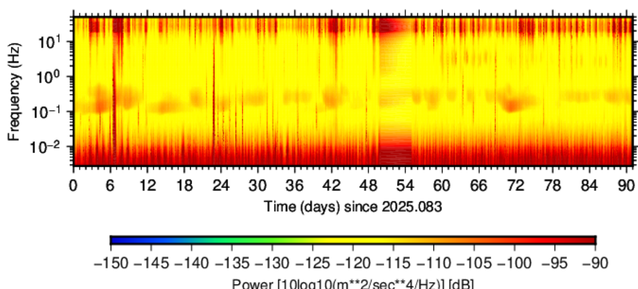
BK.ROMB.HNN.00 (2025.083 - 2025.173)
