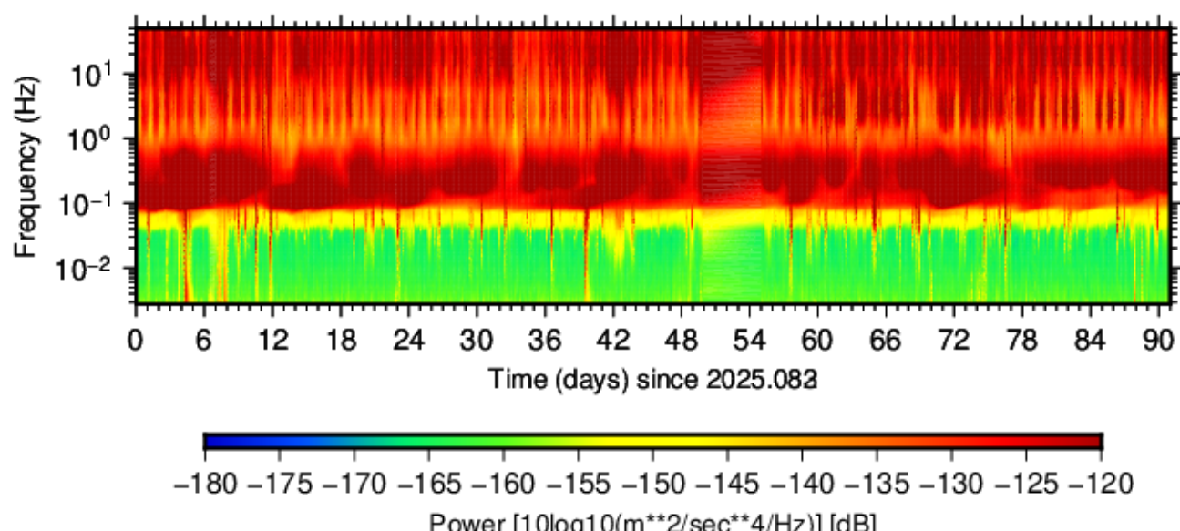
BK.ROMB.HHZ.00 (2025.083 - 2025.173)
