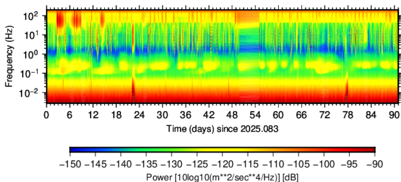
BG.RGP.DPN. (2025.083 - 2025.173)
