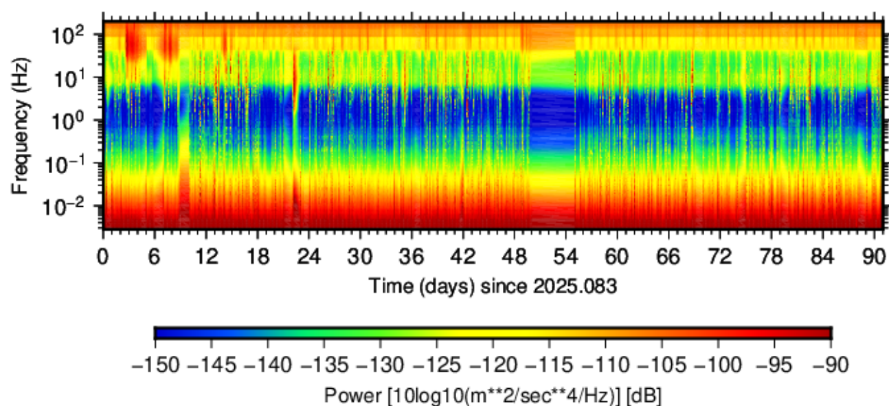
BG.RGP.DPE. (2025.083 - 2025.173)
