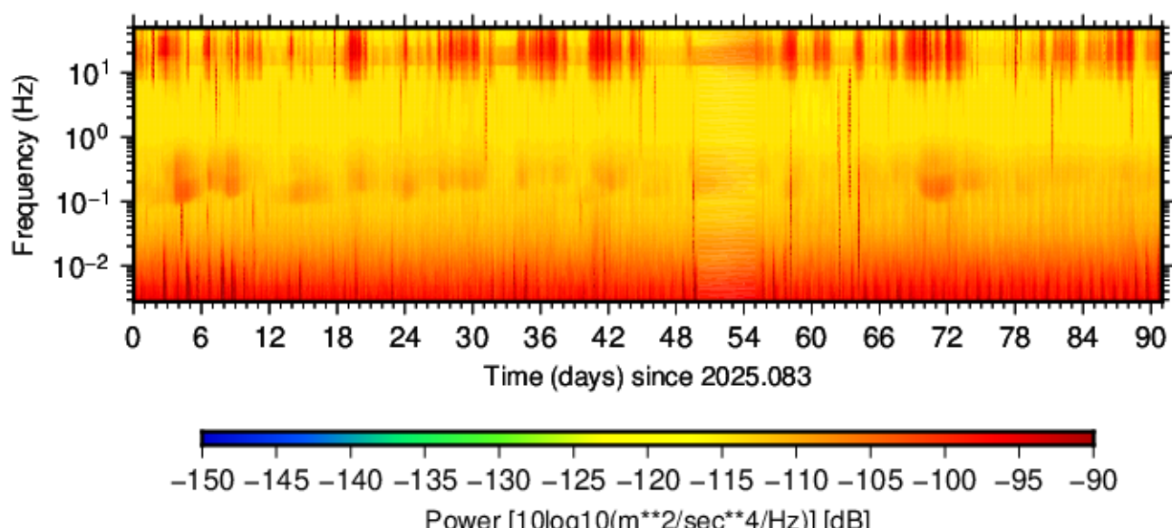
BK.RBOW.HNN.00 (2025.083 - 2025.173)
