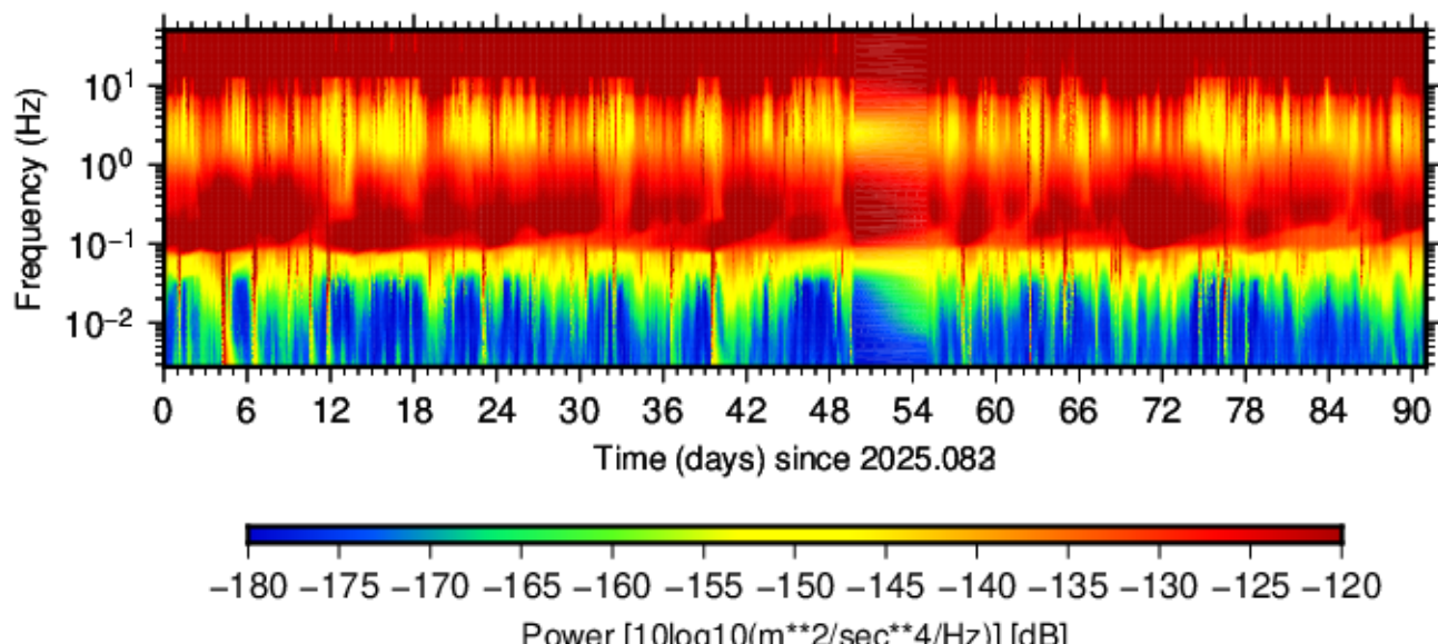
BK.RBOW.HHZ.00 (2025.083 - 2025.173)
