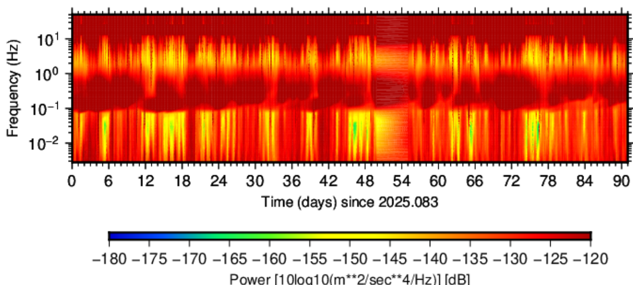
BK.RBOW.HHN.00 (2025.083 - 2025.173)
