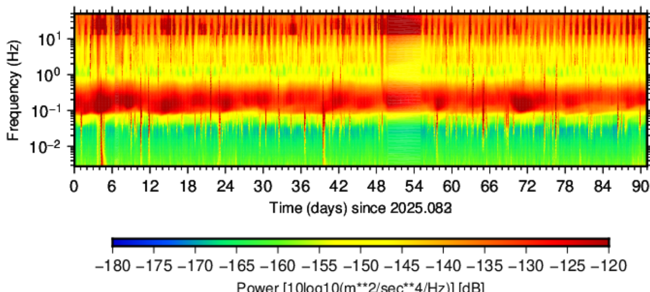
BK.RAVE.HHZ.00 (2025.083 - 2025.173)
