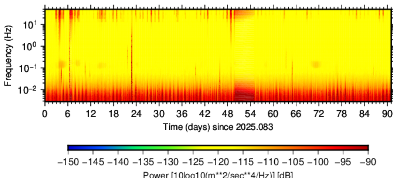
BK.RAVE.HNN.00 (2025.083 - 2025.173)
