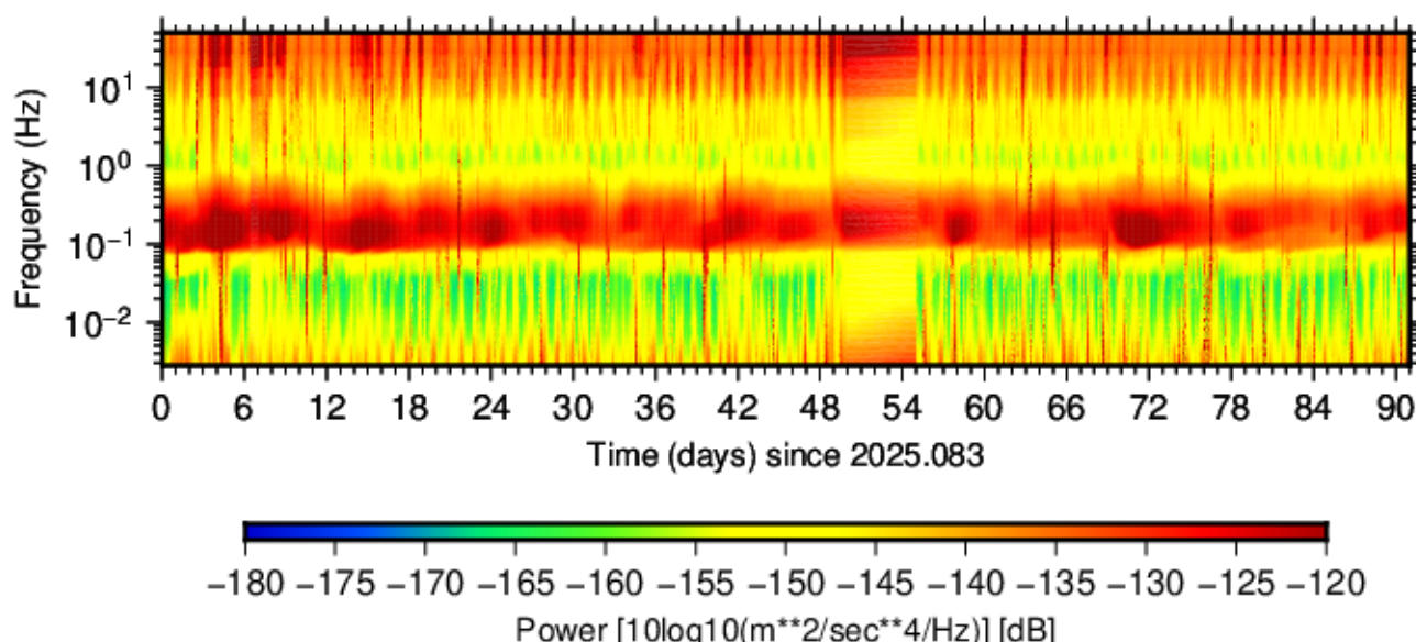
BK.RAVE.HHN.00 (2025.083 - 2025.173)
