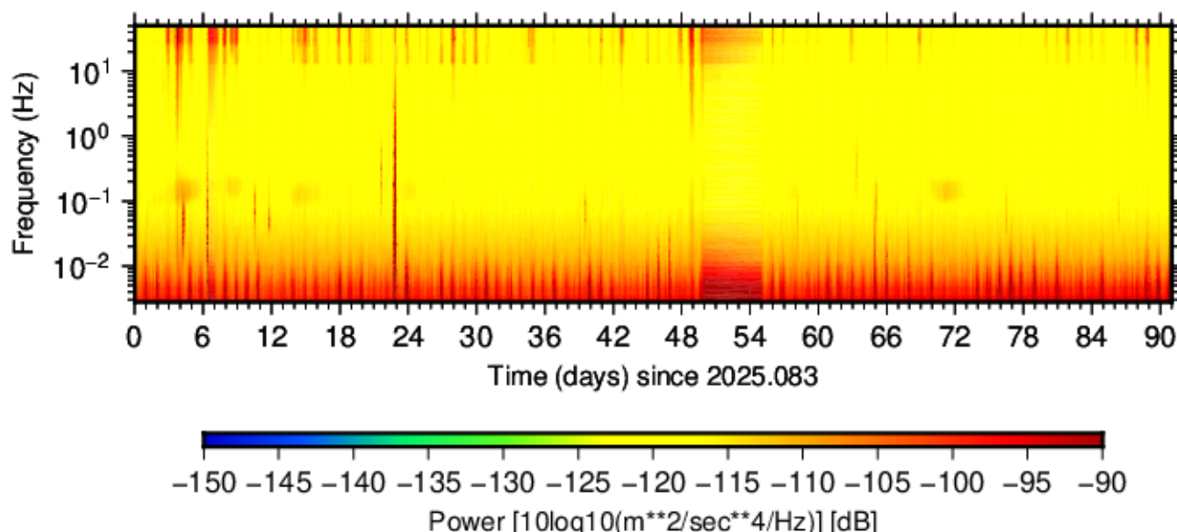
BK.RAVE.HNE.00 (2025.083 - 2025.173)
