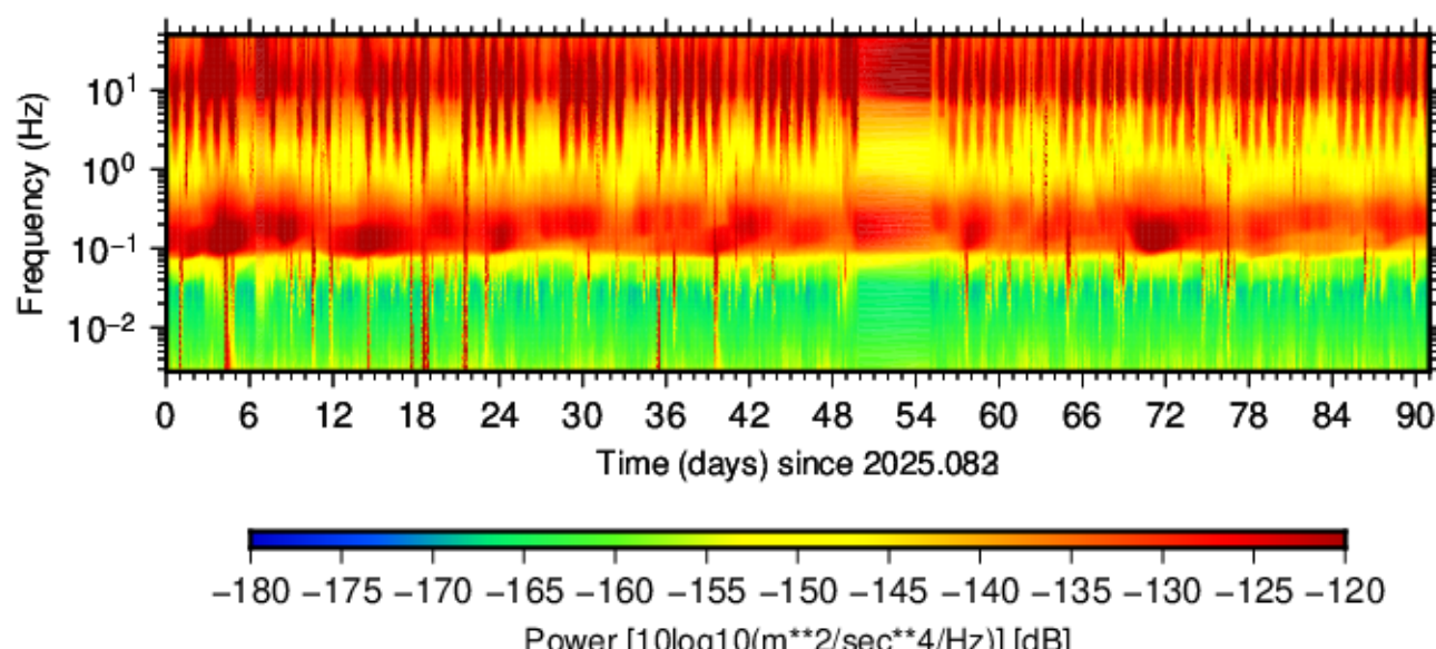
BK.PWAY.HHZ.00 (2025.083 - 2025.173)
