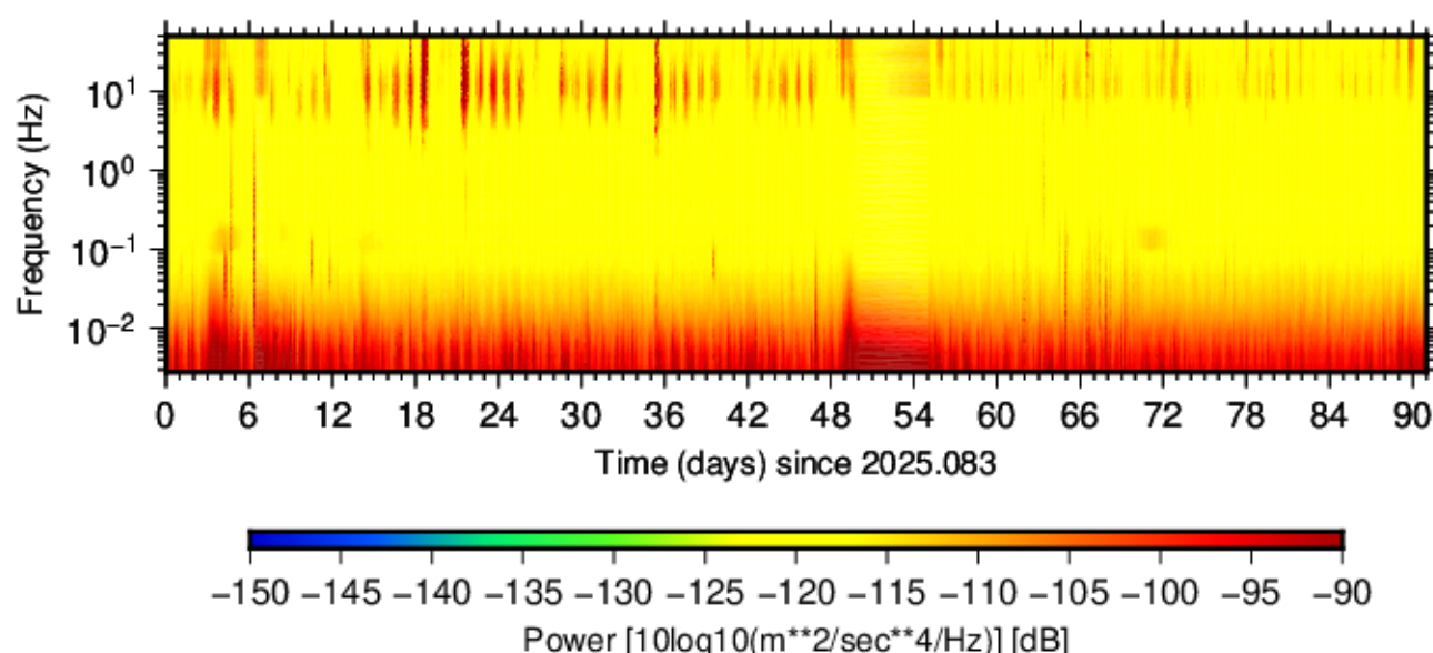
BK.PWAY.HNZ.00 (2025.083 - 2025.173)
