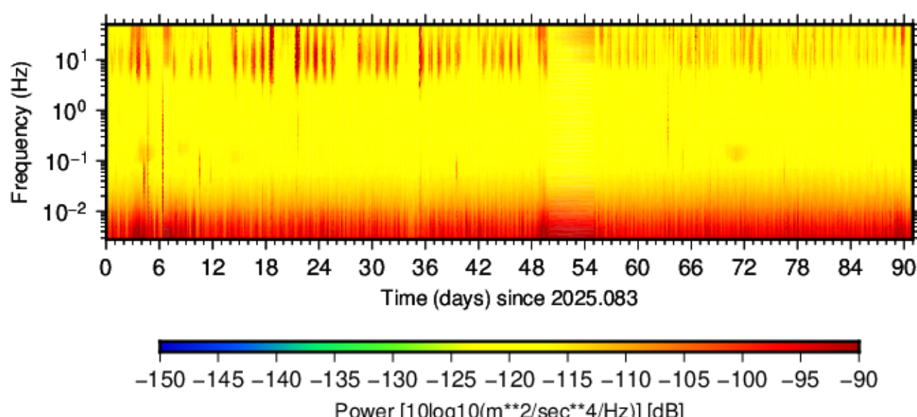
BK.PWAY.HNN.00 (2025.083 - 2025.173)
