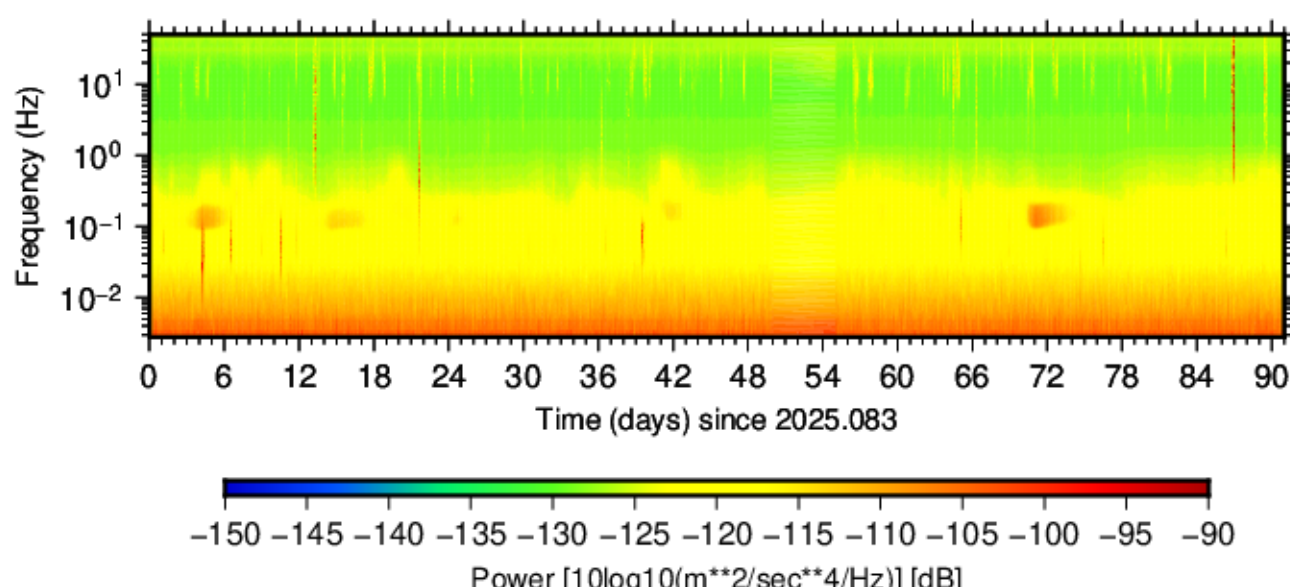
BK.PKD.HNN.00 (2025.083 - 2025.173)
