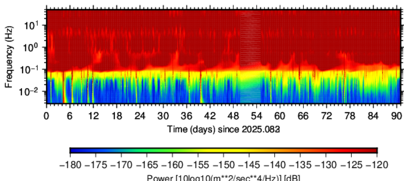
BK.PINL.HHZ.00 (2025.083 - 2025.173)
