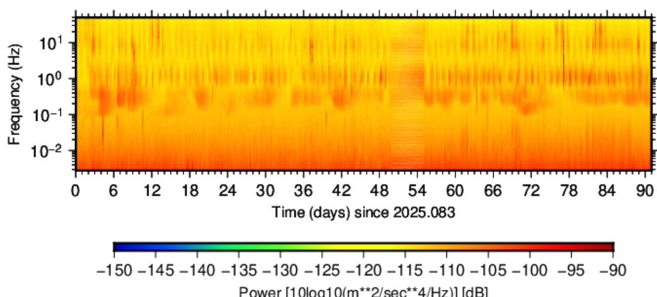
BK.PINL.HNN.00 (2025.083 - 2025.173)
