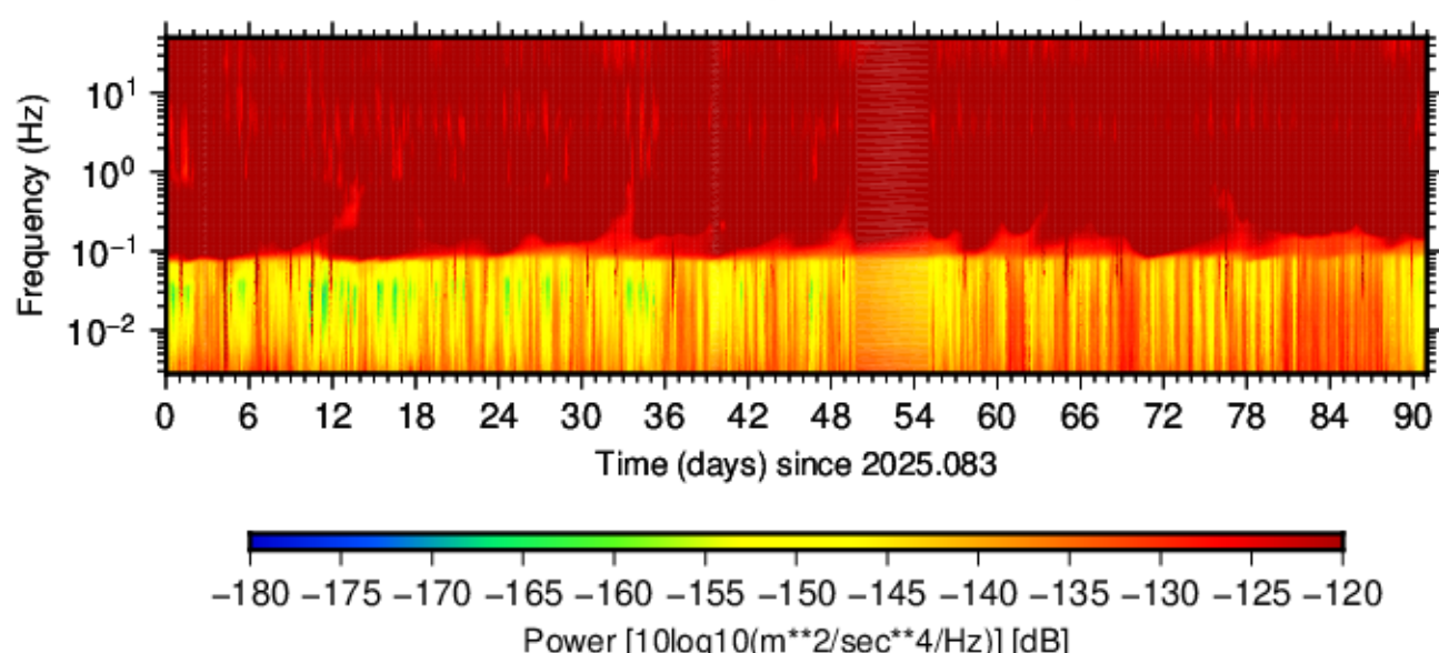
BK.PINL.HHN.00 (2025.083 - 2025.173)
