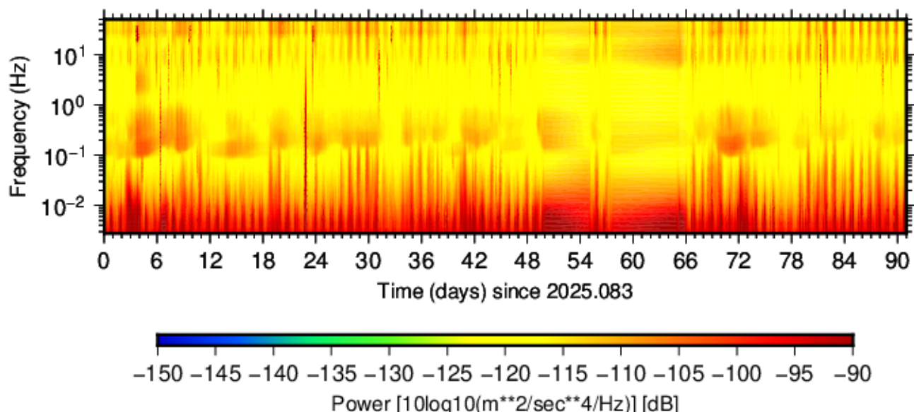
BK.PETL.HNZ.00 (2025.083 - 2025.173)
