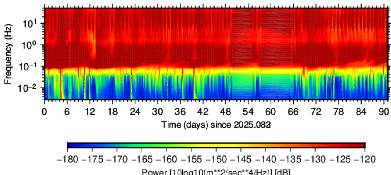
BK.PETL.HHZ.00 (2025.083 - 2025.173)
