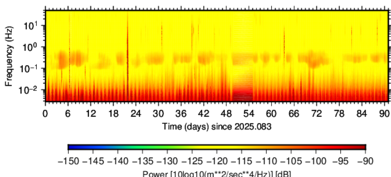
BK.ORRS.HNN.00 (2025.083 - 2025.173)
