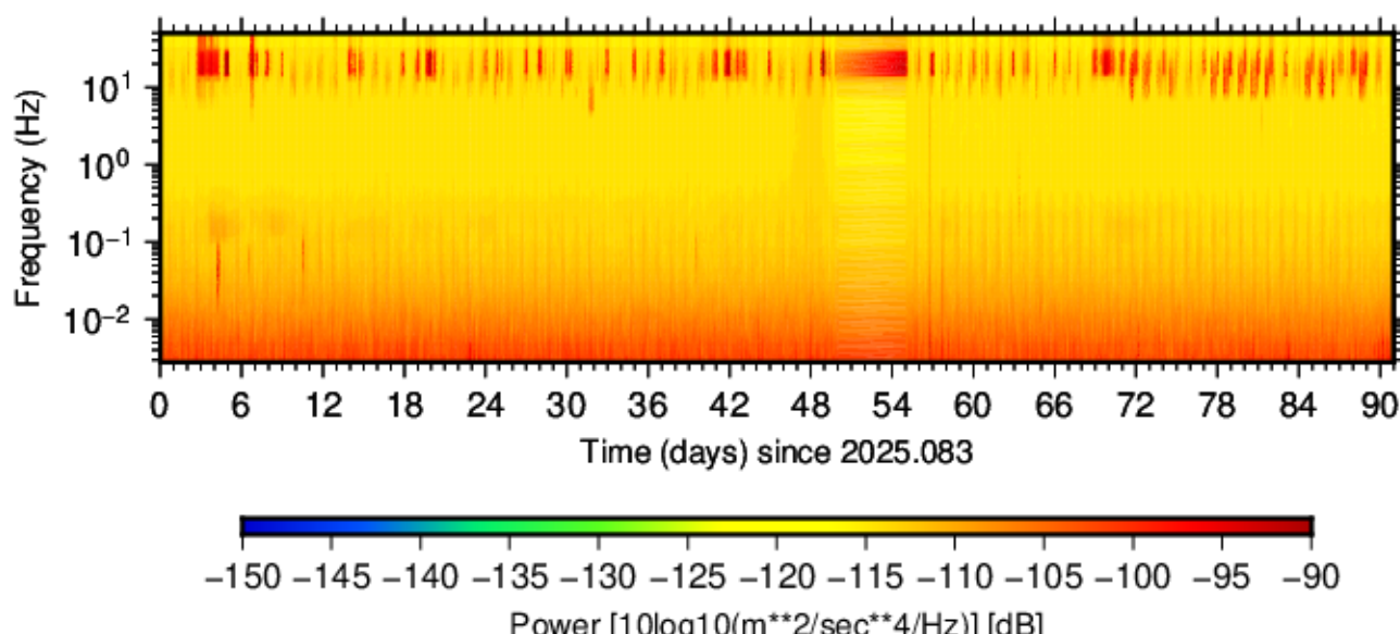
BK.MOGU.HNN.00 (2025.083 - 2025.173)
