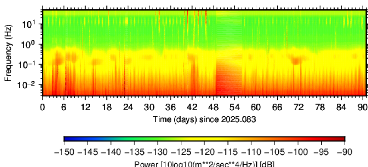
BK.MNRC.HNN.00 (2025.083 - 2025.173)
