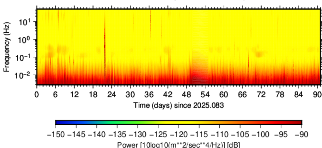
BK.MLKN.HNZ.00 (2025.083 - 2025.173)
