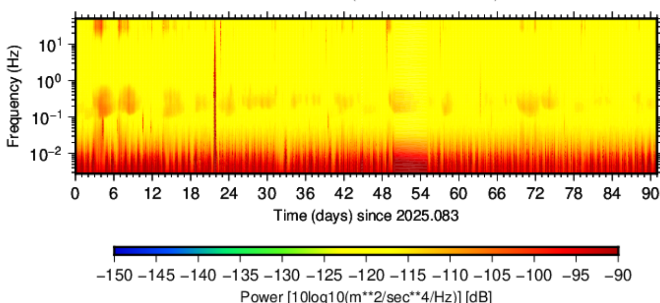
BK.MILL.HNZ.00 (2025.083 - 2025.173)
