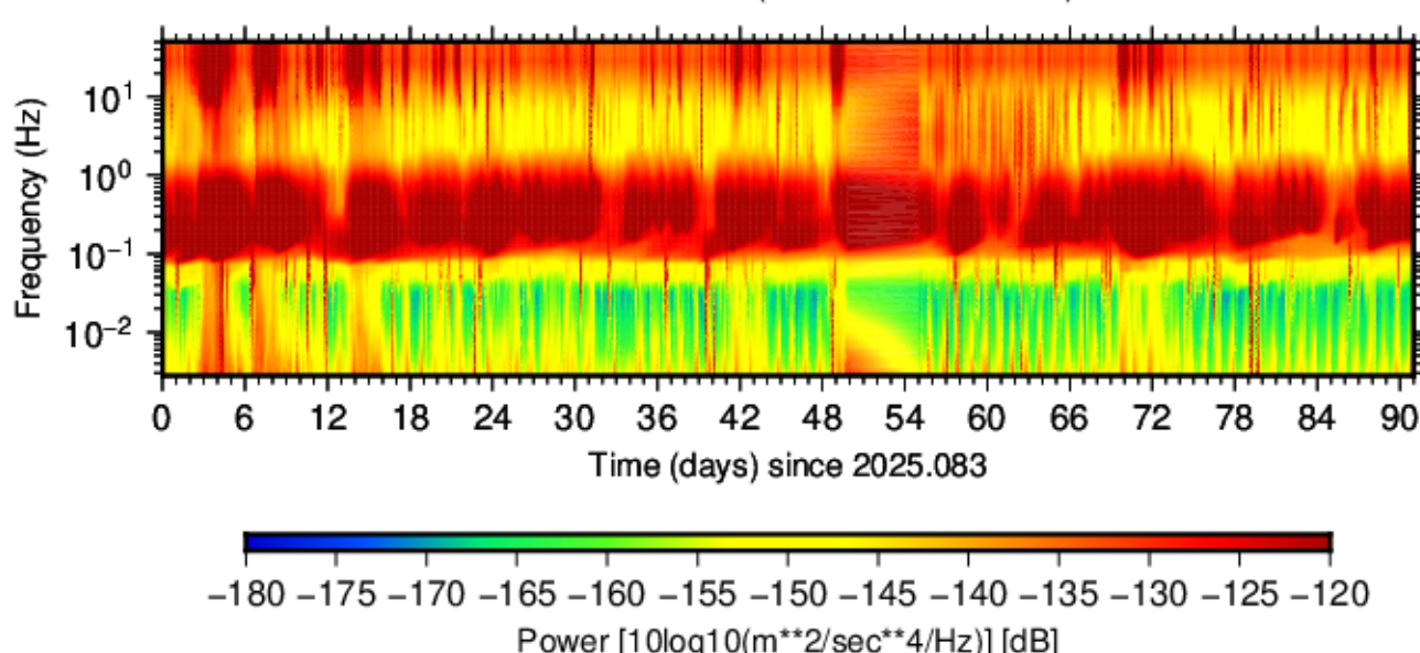
BK.MILL.HHN.00 (2025.083 - 2025.173)
