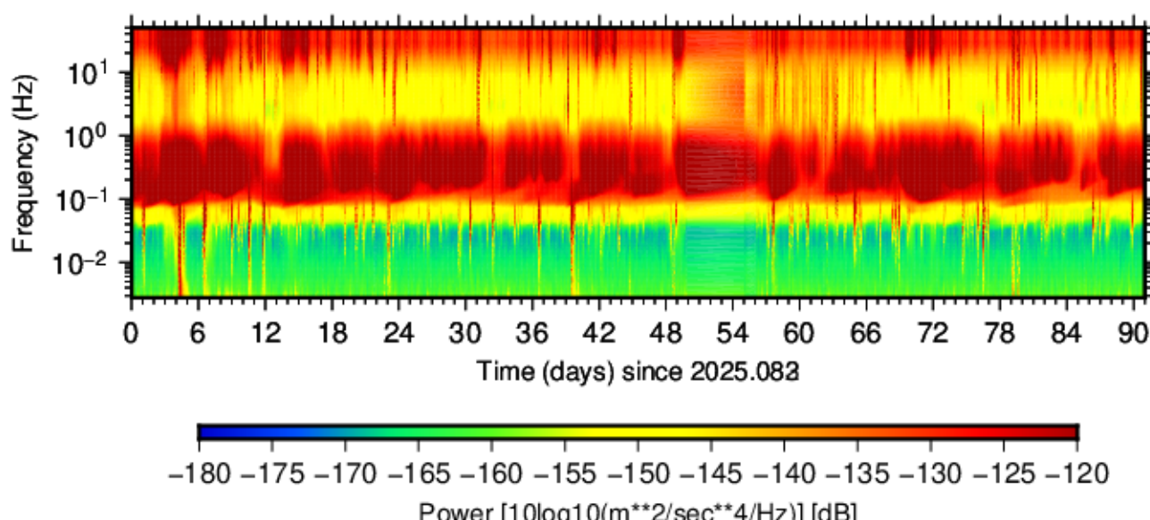
BK.MILL.HHZ.00 (2025.083 - 2025.173)
