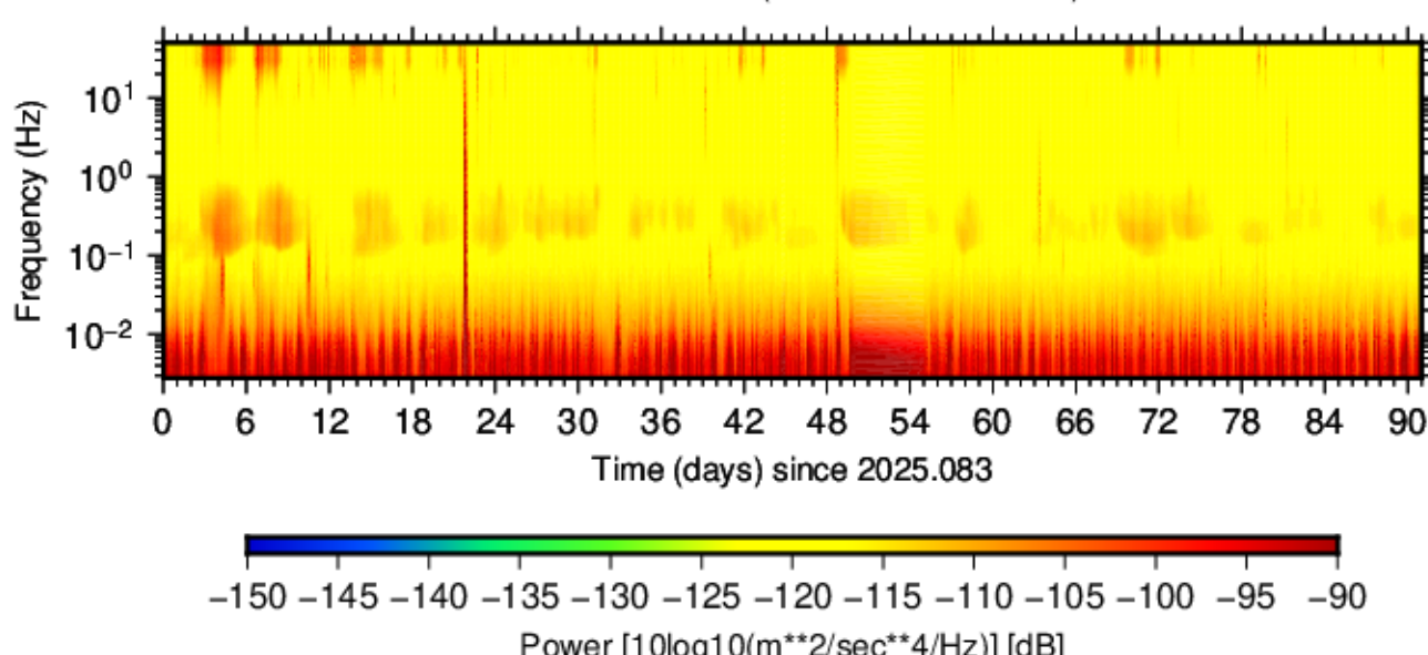
BK.MILL.HNN.00 (2025.083 - 2025.173)
