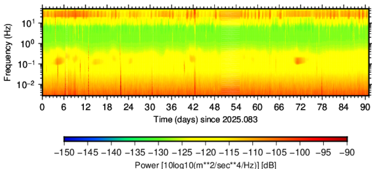
BK.MHC.HNN.00 (2025.083 - 2025.173)
