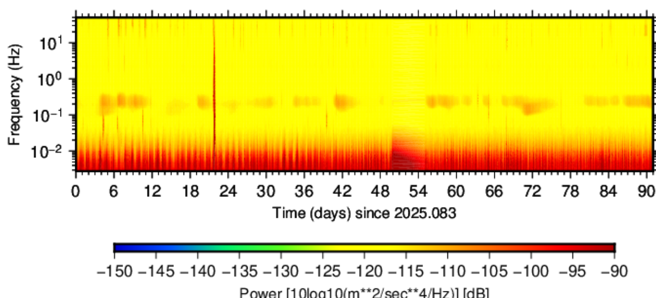
BK.MERC.HNN.00 (2025.083 - 2025.173)
