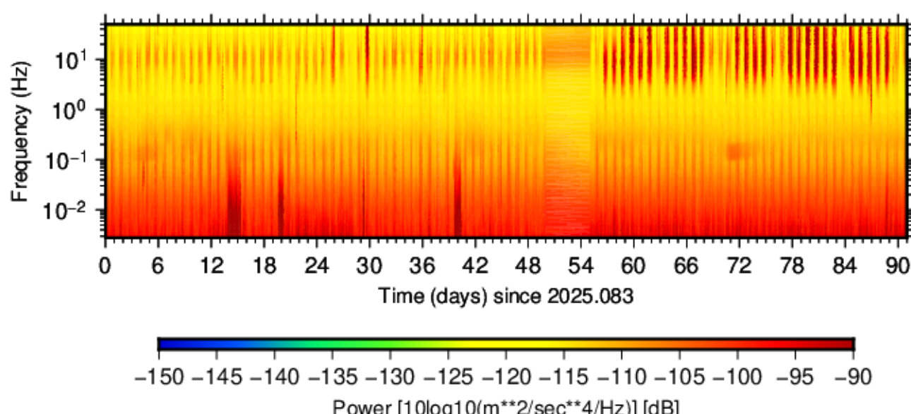
BK.LCUV.HNN.00 (2025.083 - 2025.173)
