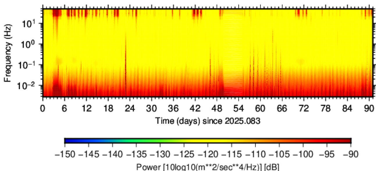
BK.LCOW.HNN.00 (2025.083 - 2025.173)
