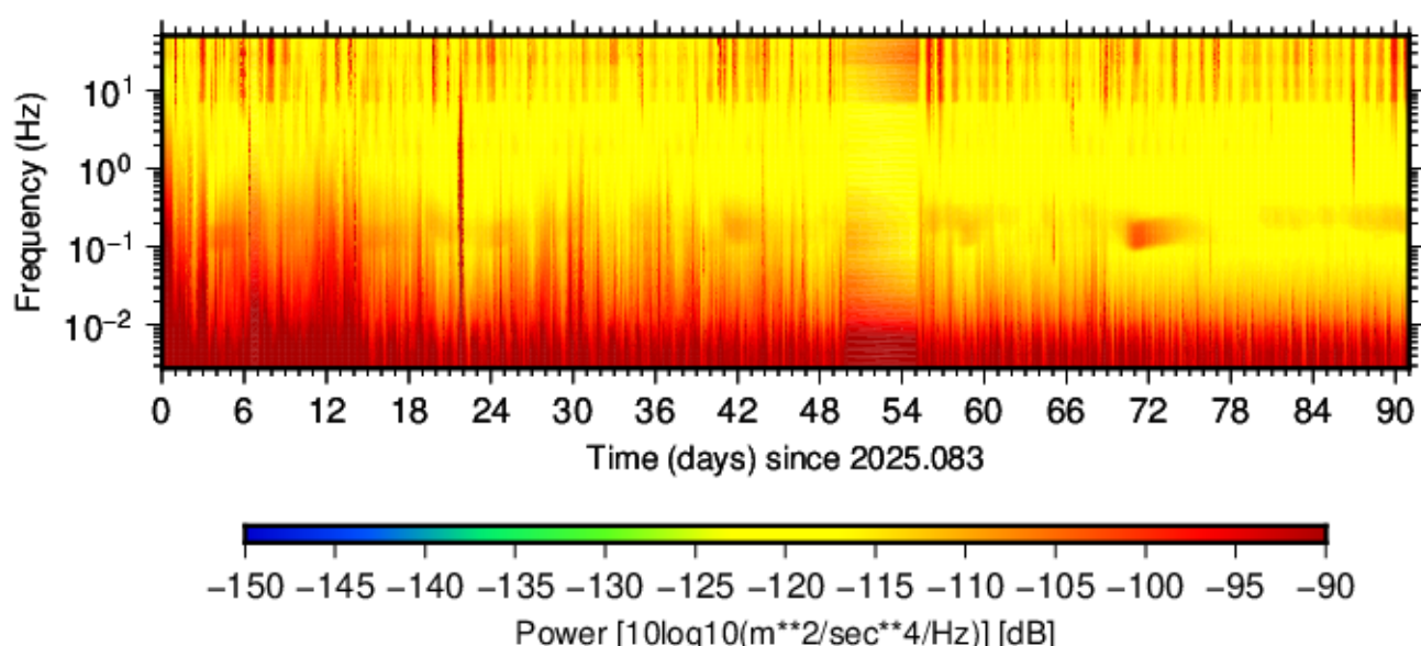
BK.KETL.HNZ.00 (2025.083 - 2025.173)
