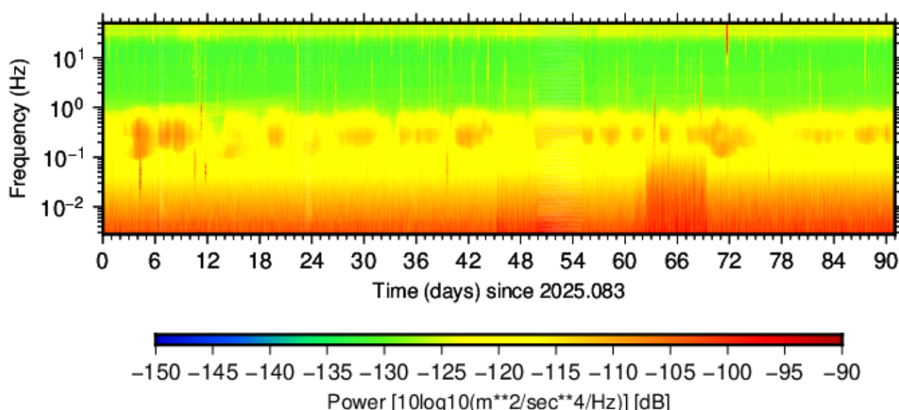
BK.HOPS.HNE.00 (2025.083 - 2025.173)
