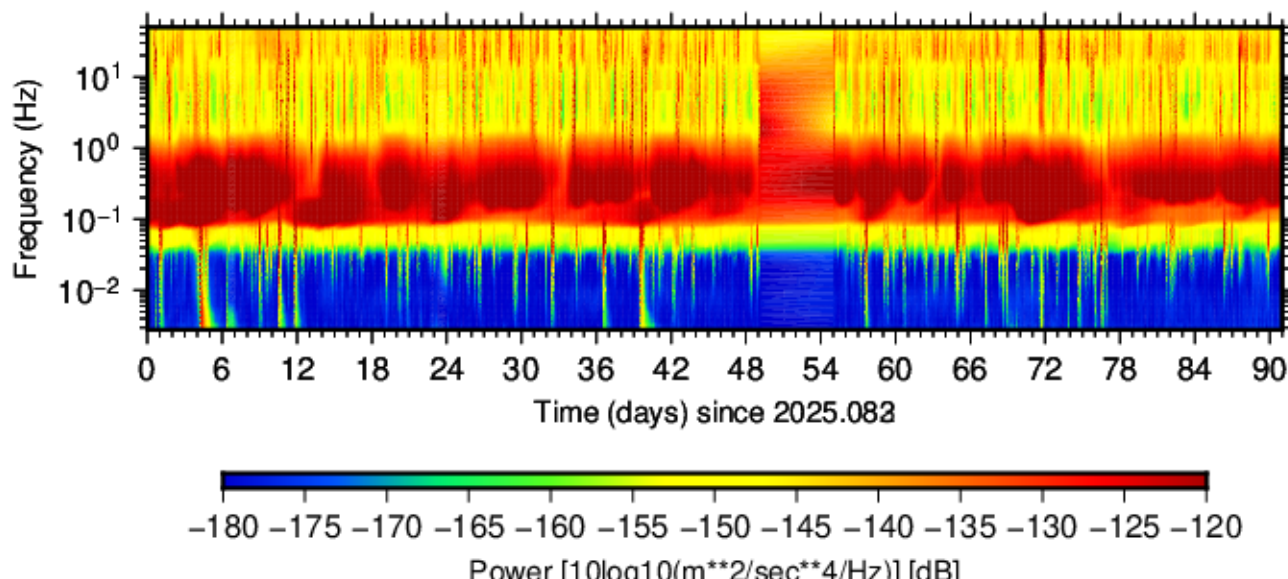
BK.HOPS.HHZ.00 (2025.083 - 2025.173)
