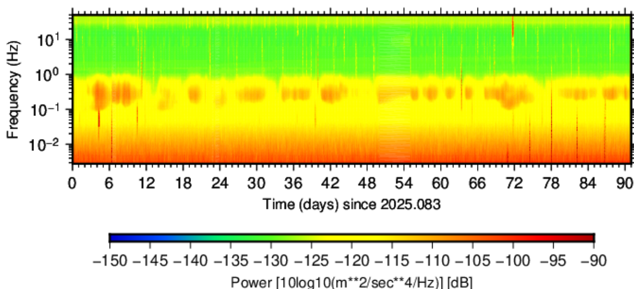
BK.HOPS.HNN.00 (2025.083 - 2025.173)
