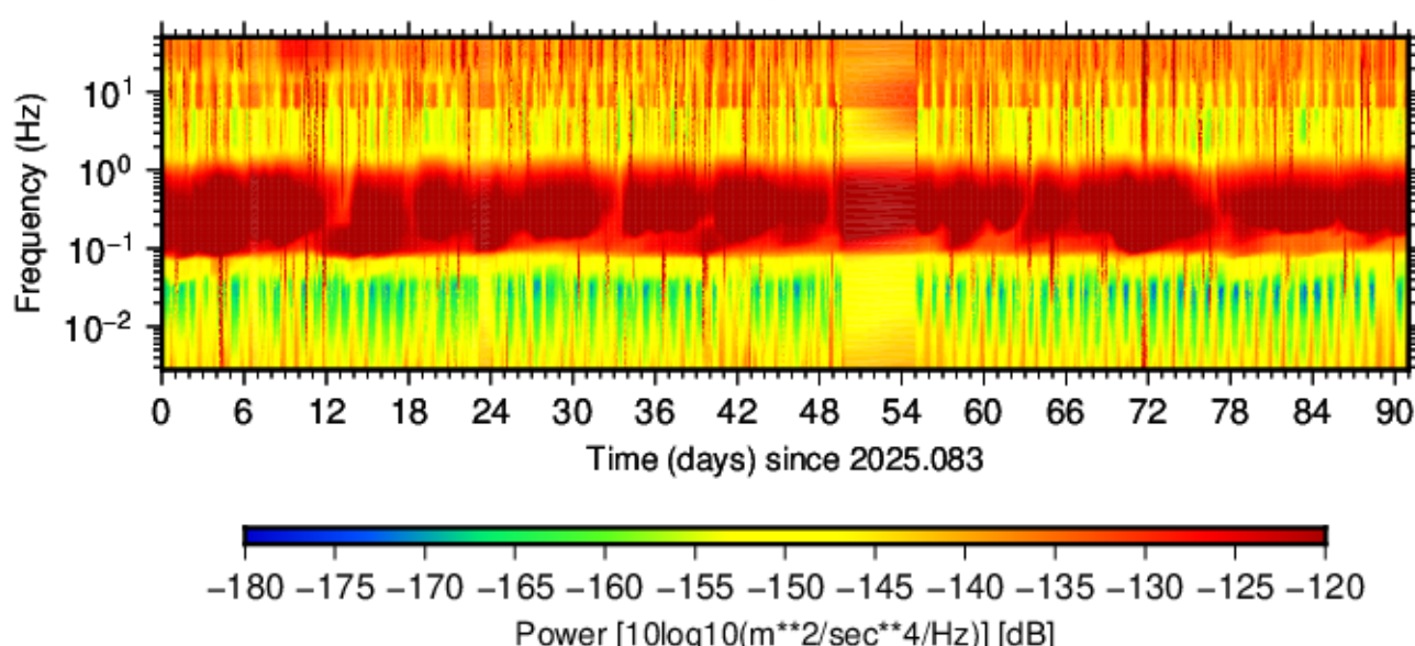
BK.HOPS.HHN.00 (2025.083 - 2025.173)
