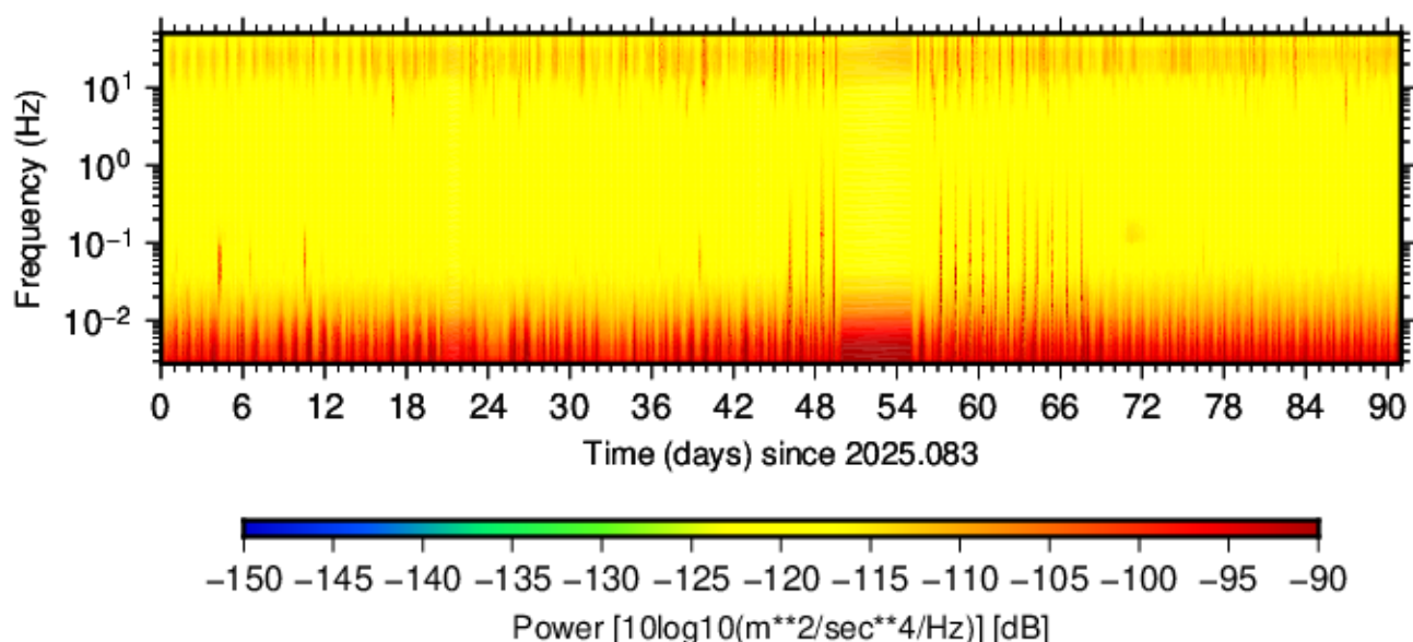
BK.HELL.HNN.00 (2025.083 - 2025.173)
