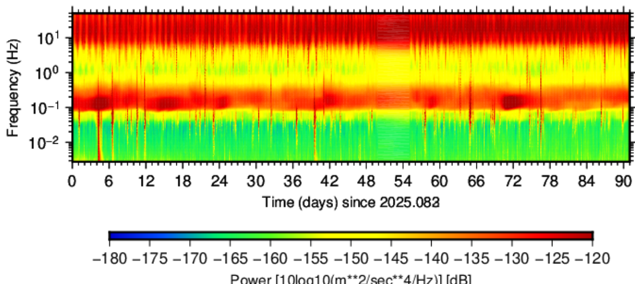
BK.HELL.HHZ.00 (2025.083 - 2025.173)
