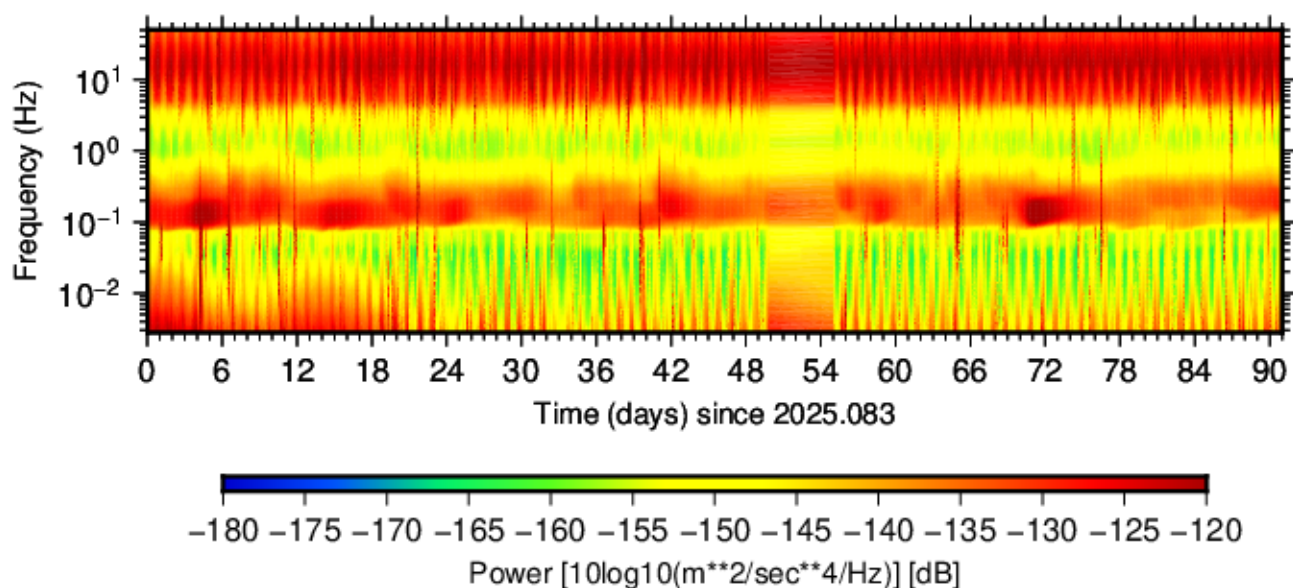
BK.HELL.HHN.00 (2025.083 - 2025.173)
