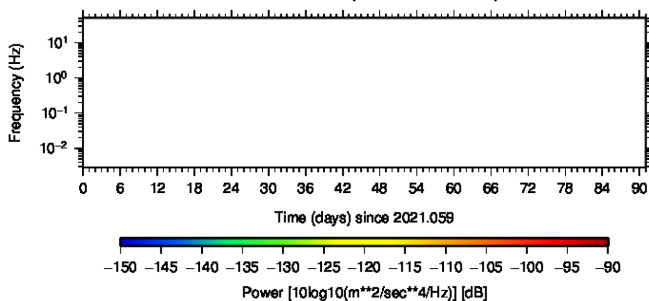
BK.HAST.HHN.00 (2021.059 – 2021.149)
