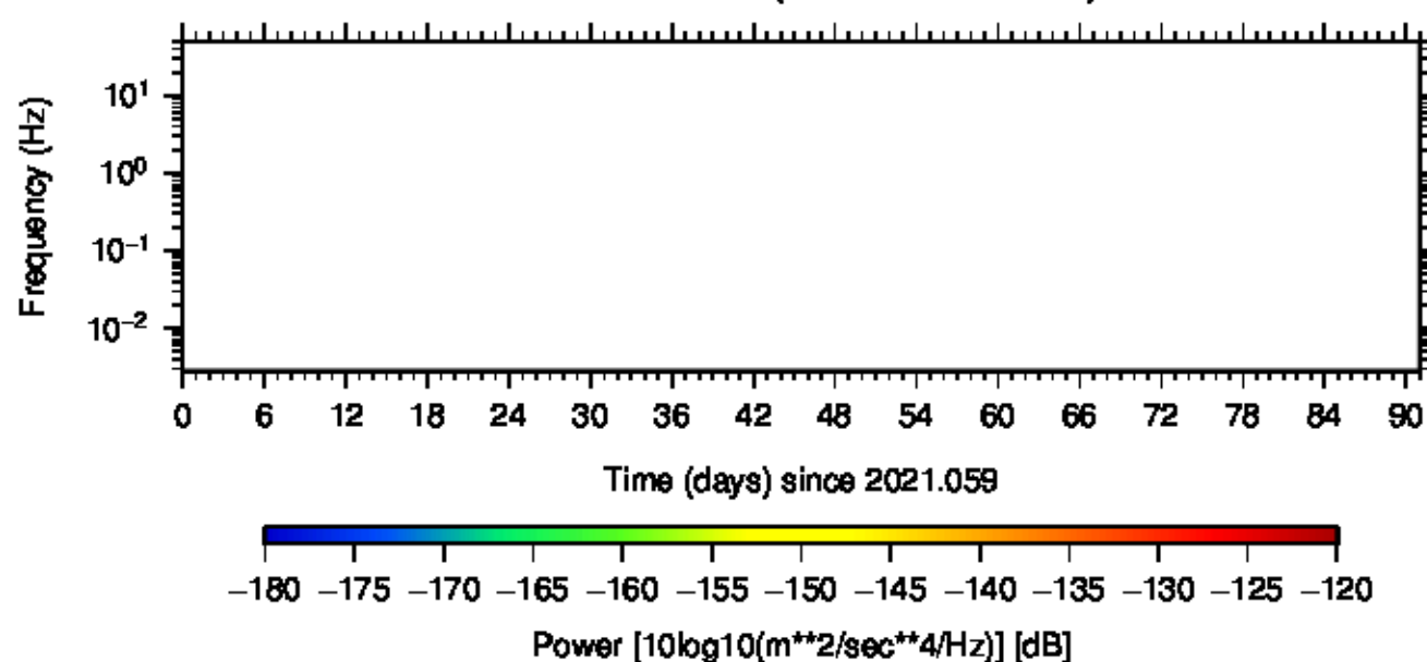
BK.HAST.HNN.00 (2021.059 – 2021.149)
