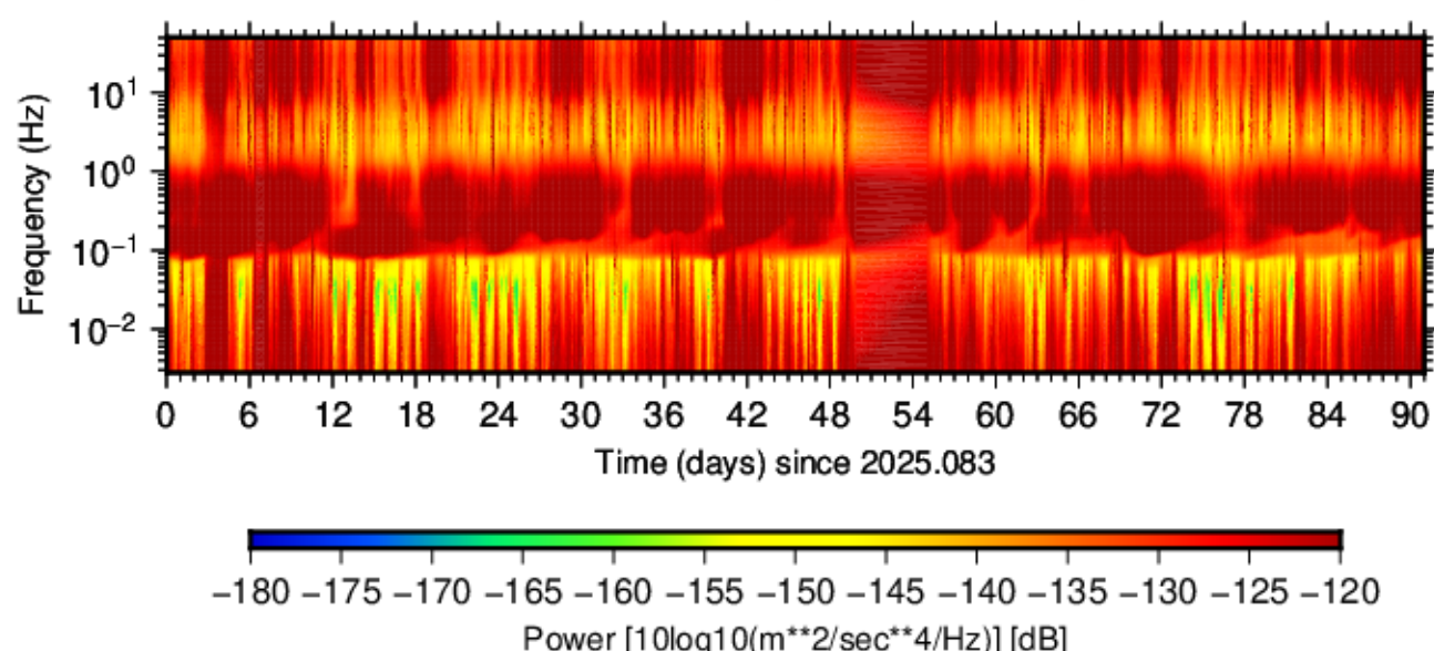
BK.HALS.HHN.00 (2025.083 - 2025.173)
