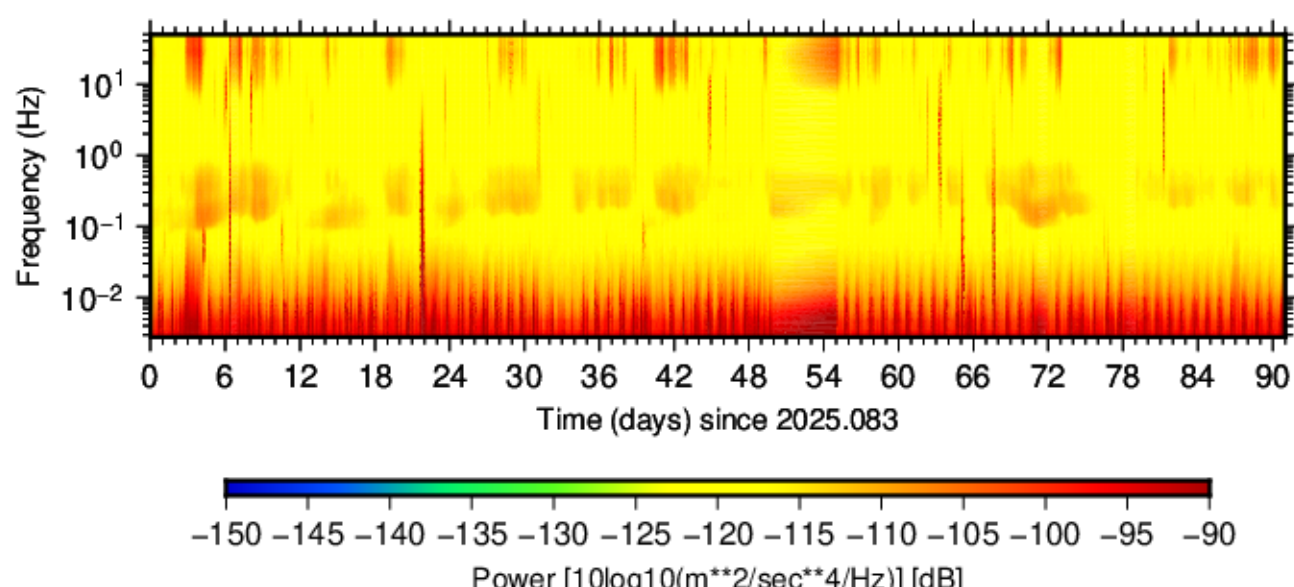
BK.HALS.HNN.00 (2025.083 - 2025.173)
