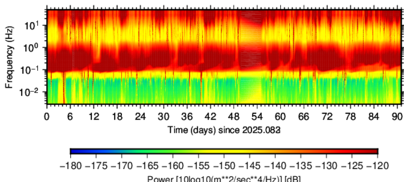
BK.HALS.HHZ.00 (2025.083 - 2025.173)
