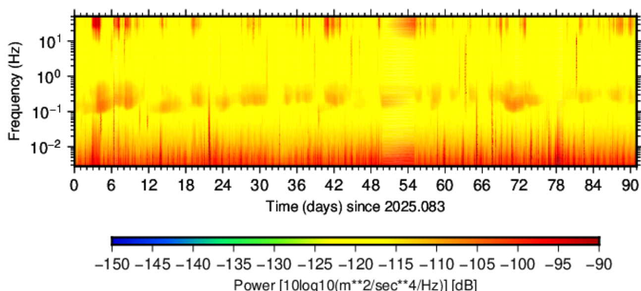
BK.HALS.HNE.00 (2025.083 - 2025.173)
