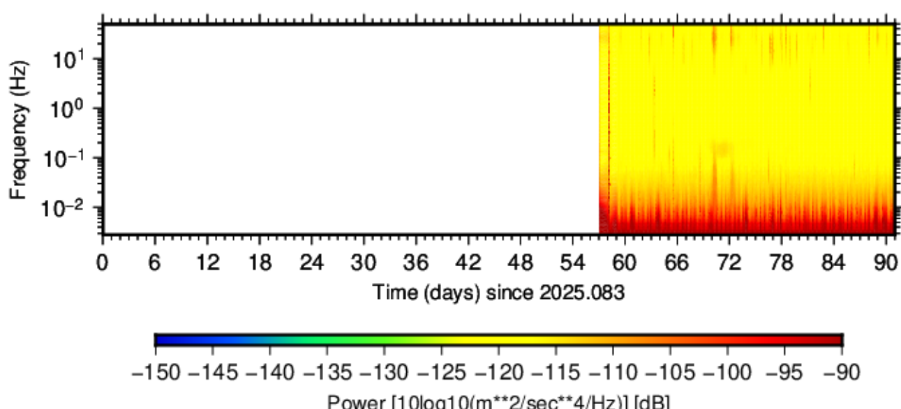
BK.GRPK.HNN.00 (2025.083 - 2025.173)
