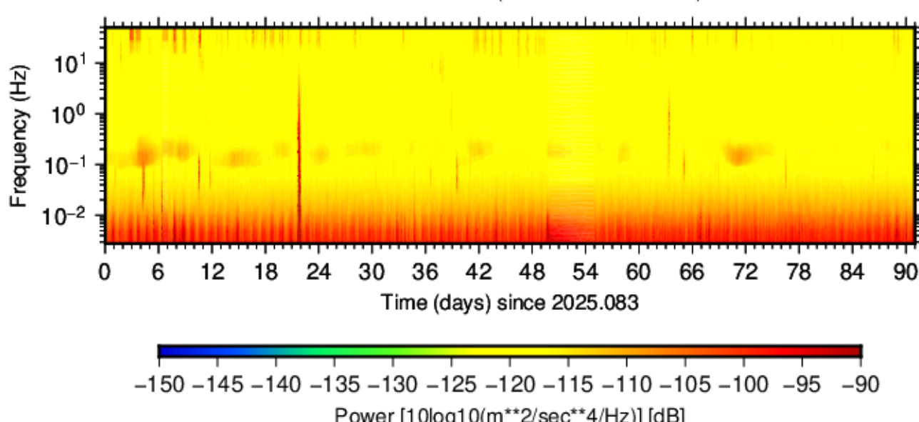
BK.GCKB.HNN.00 (2025.083 - 2025.173)
