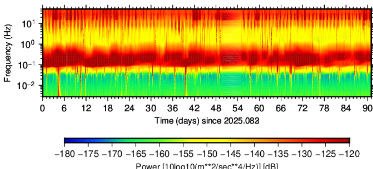
BK.GCKB.HHZ.00 (2025.083 - 2025.173)
