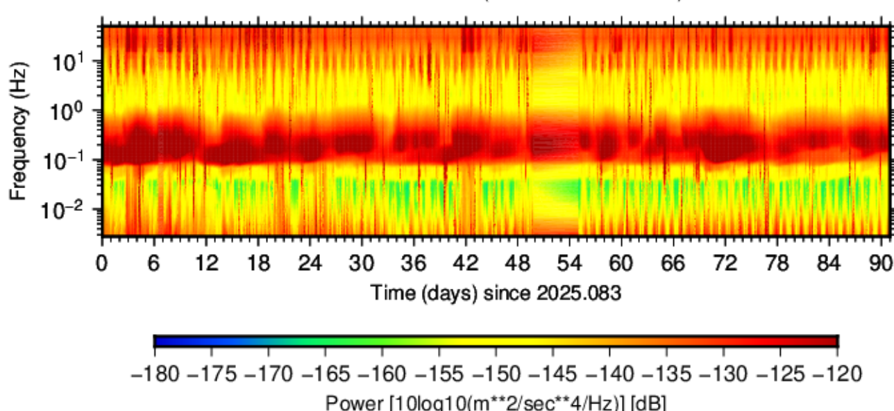
BK.GCKB.HHN.00 (2025.083 - 2025.173)
