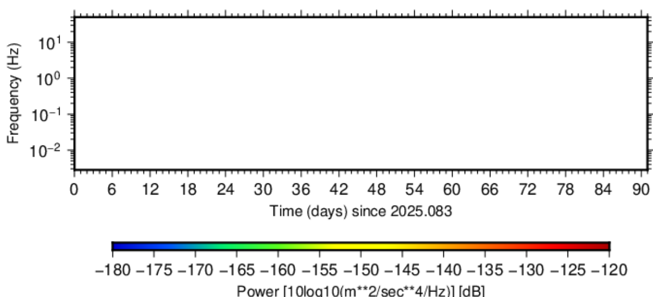
BK.DRDG.HHN.00 (2025.083 - 2025.173)
