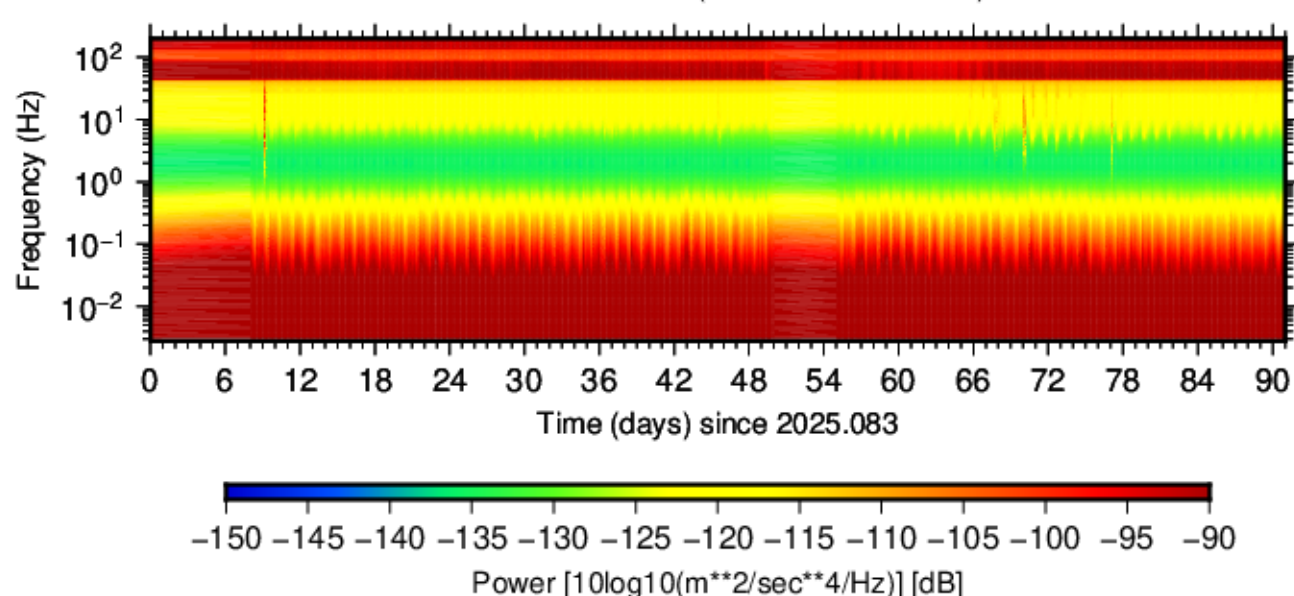
BK.CMSB.DP2.40 (2025.083 - 2025.173)
