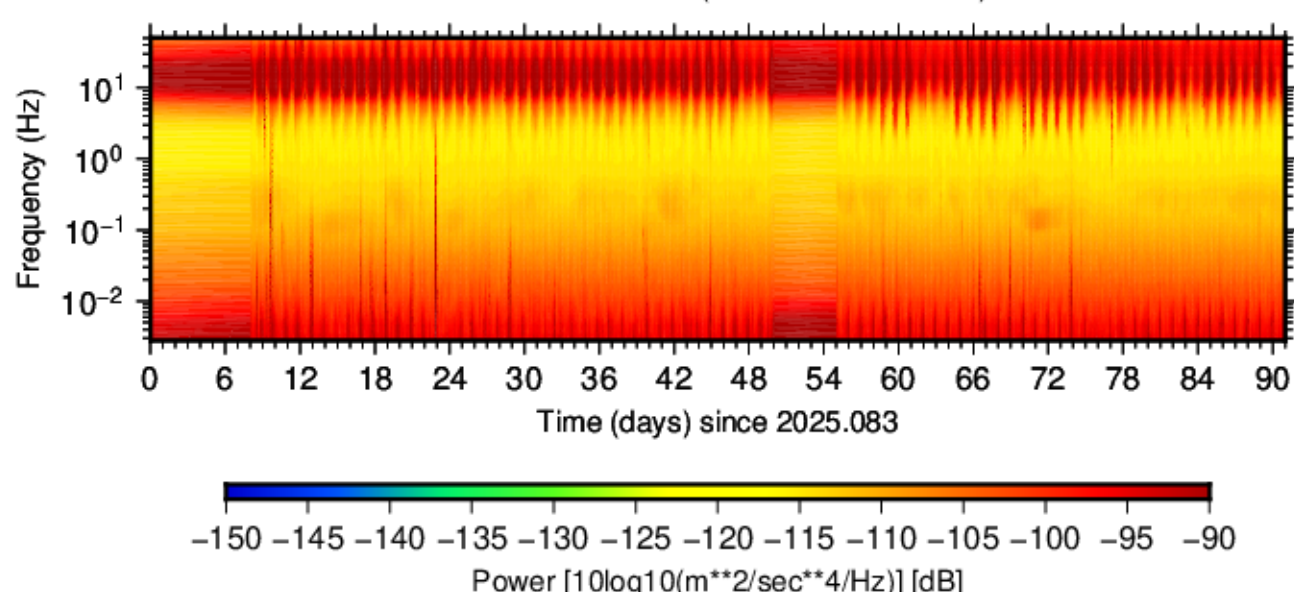
BK.CMSB.HNN.00 (2025.083 - 2025.173)
