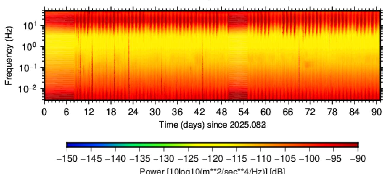
BK.CMSB.HNZ.00 (2025.083 - 2025.173)
