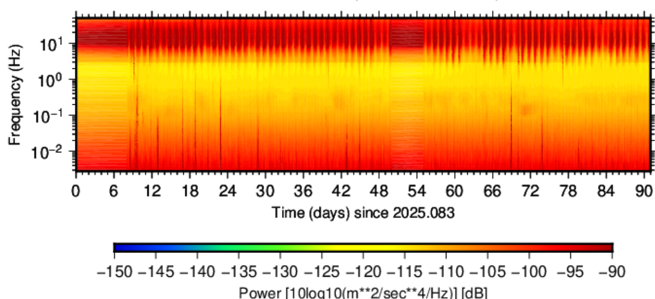
BK.CMSB.HNE.00 (2025.083 - 2025.173)
