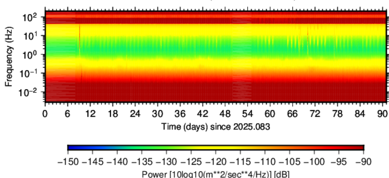
BK.CMSB.DP3.40 (2025.083 - 2025.173)
