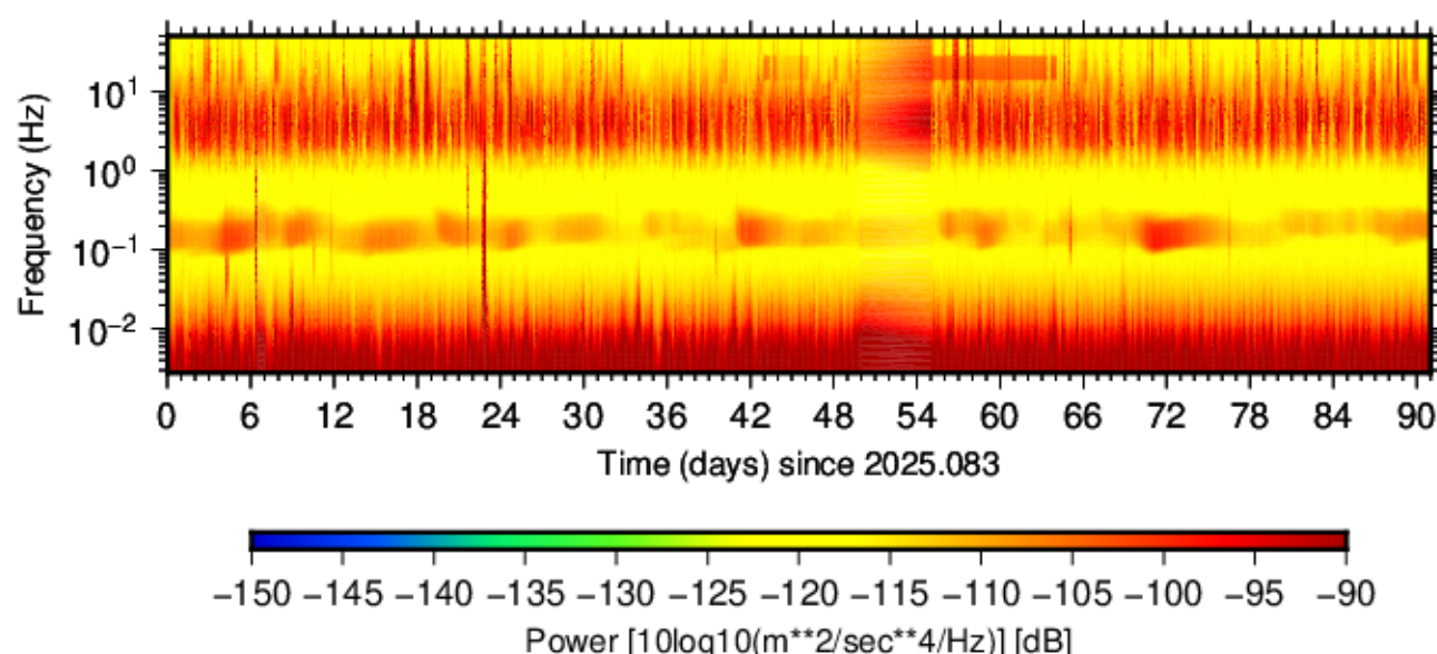
BK.CCOR.HNZ.00 (2025.083 - 2025.173)
