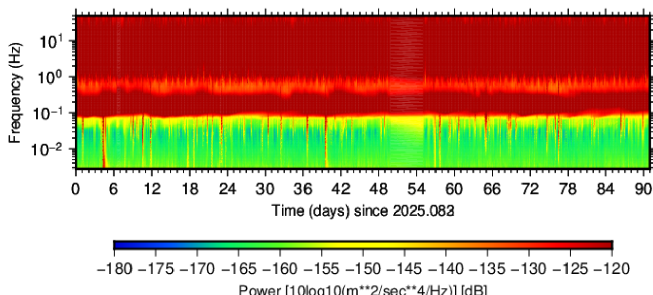
BK.CCOR.HHZ.00 (2025.083 - 2025.173)
