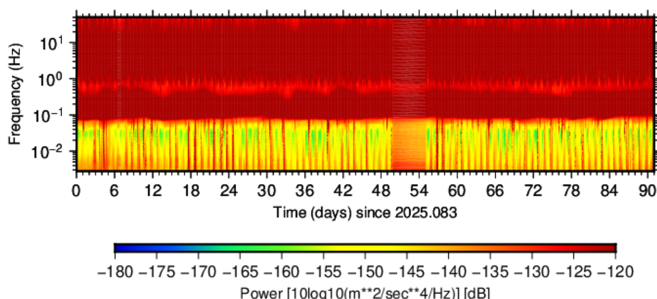
BK.CCOR.HHN.00 (2025.083 - 2025.173)
