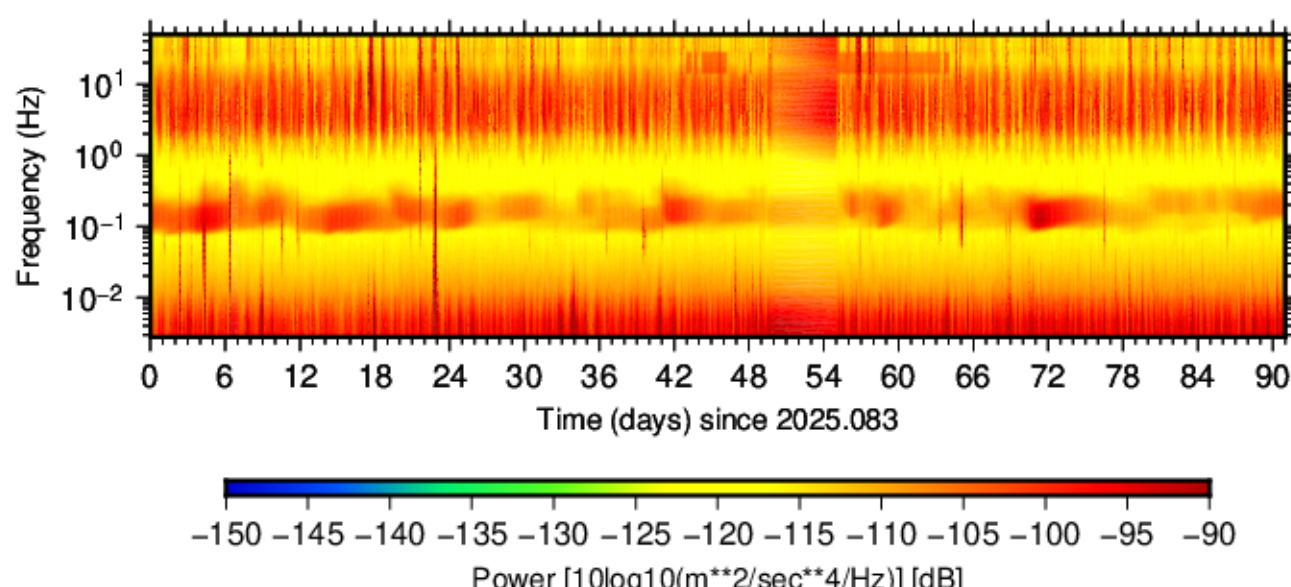
BK.CCOR.HNN.00 (2025.083 - 2025.173)
