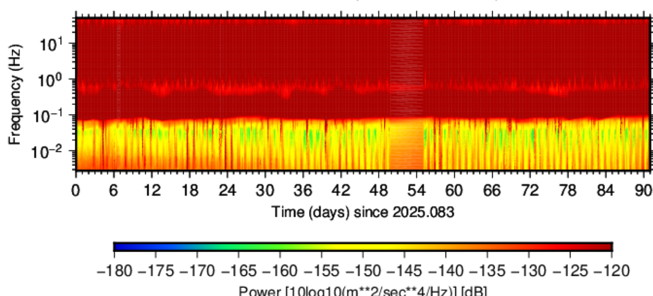
BK.CCOR.HHE.00 (2025.083 - 2025.173)
