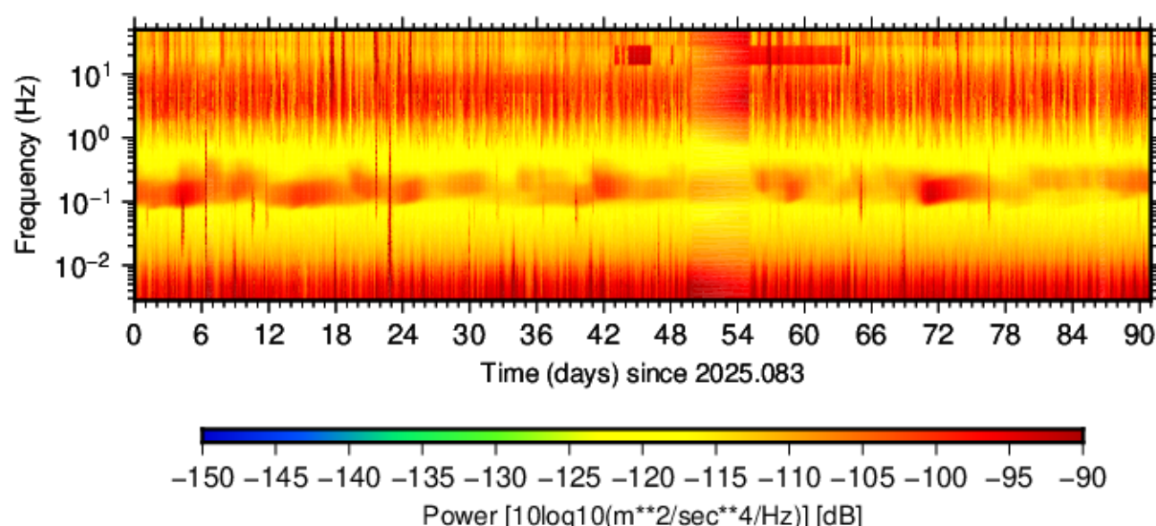
BK.CCOR.HNE.00 (2025.083 - 2025.173)
