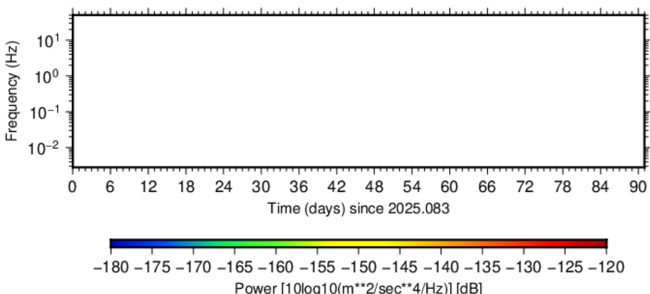
BK.BLUE.HHN.00 (2025.083 - 2025.173)
