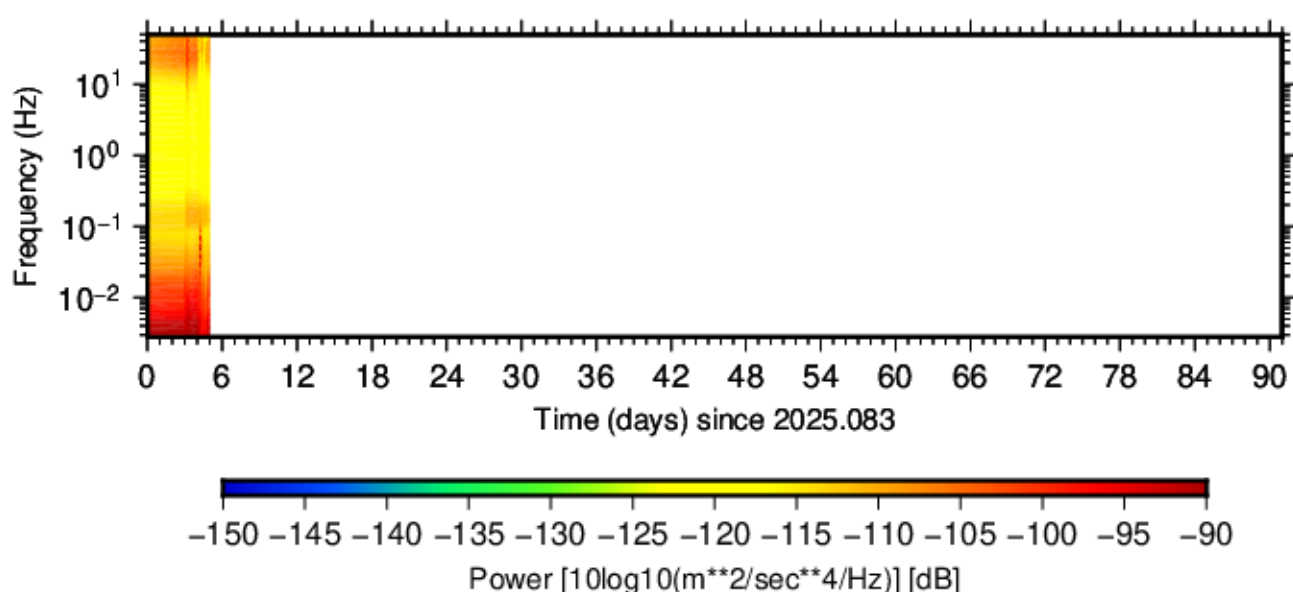
BK.BIGM.HNN.00 (2025.083 - 2025.173)
