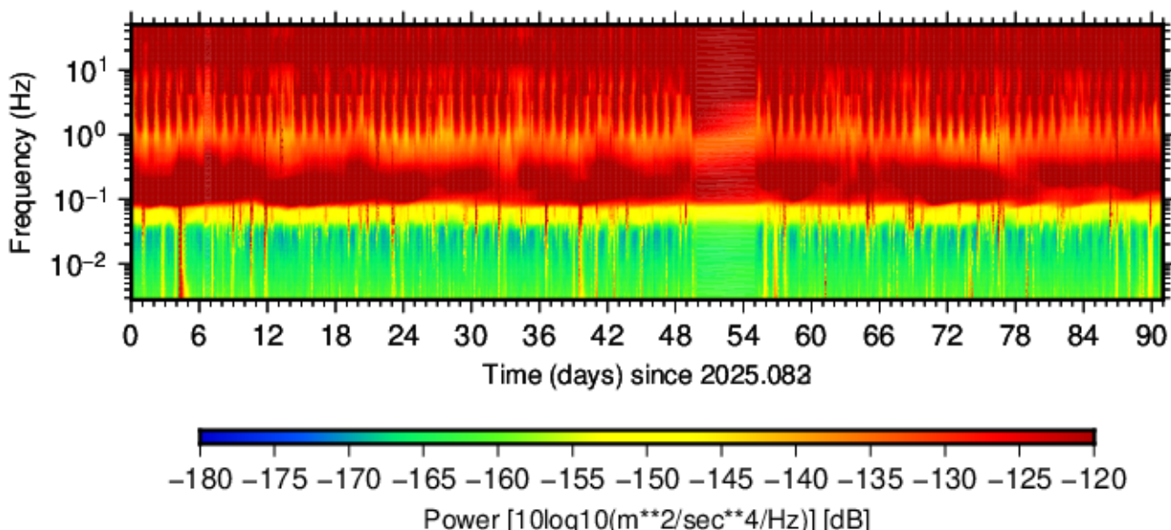
BK.AVSP.HHZ.00 (2025.083 - 2025.173)
