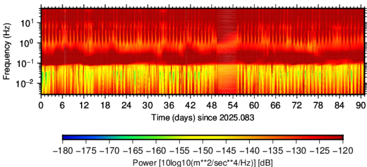
BK.AVSP.HHN.00 (2025.083 - 2025.173)
