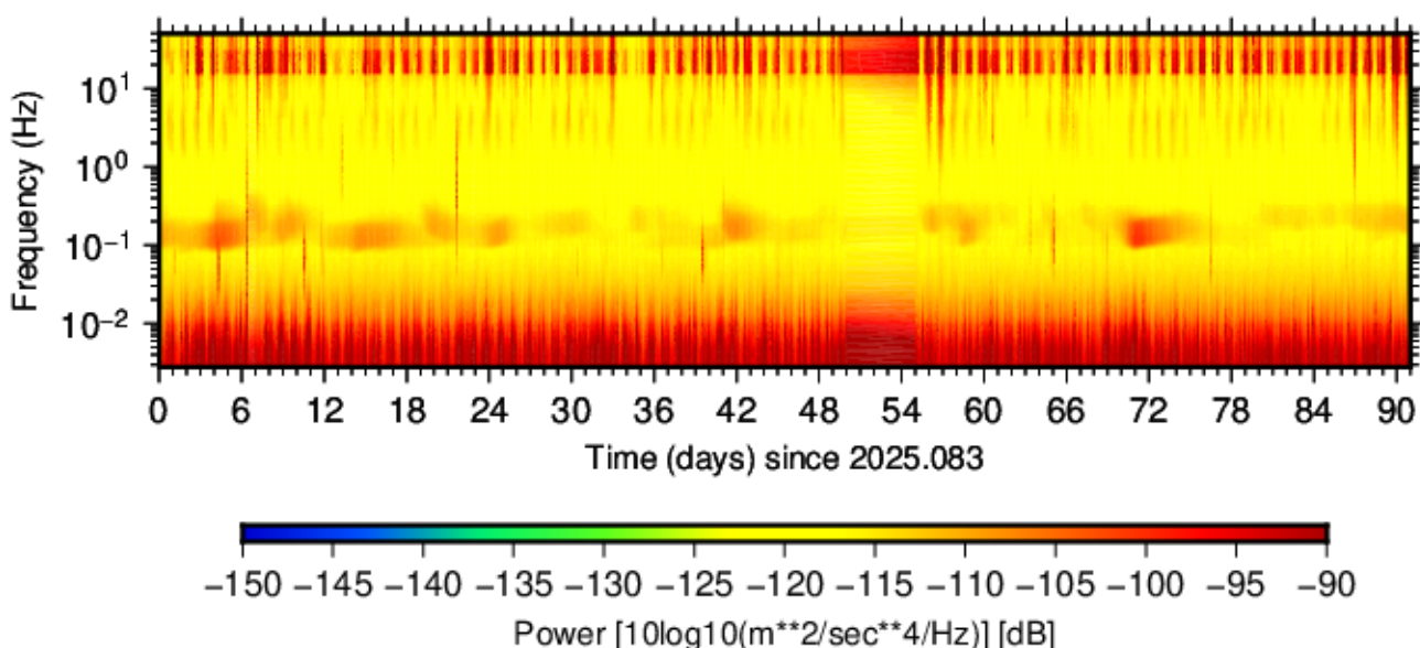
BK.AVSP.HNN.00 (2025.083 - 2025.173)
