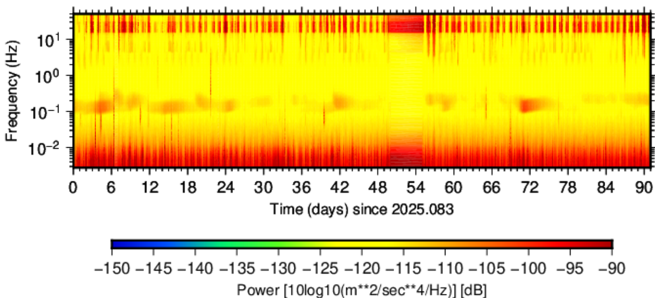
BK.AVSP.HNZ.00 (2025.083 - 2025.173)
