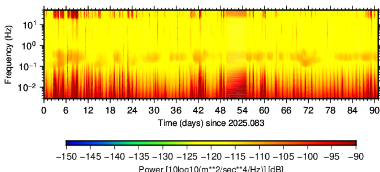
BK.ATP.HNN.00 (2025.083 - 2025.173)
