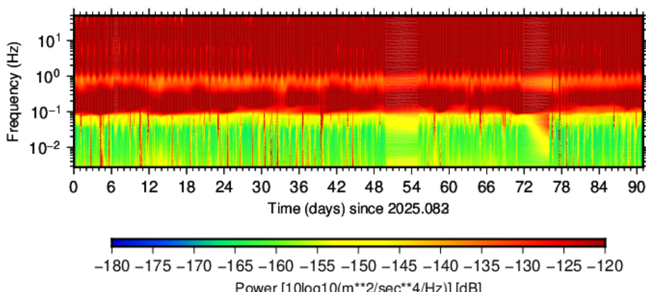
BK.AL VW.HHZ.00 (2025.083 - 2025.173)
