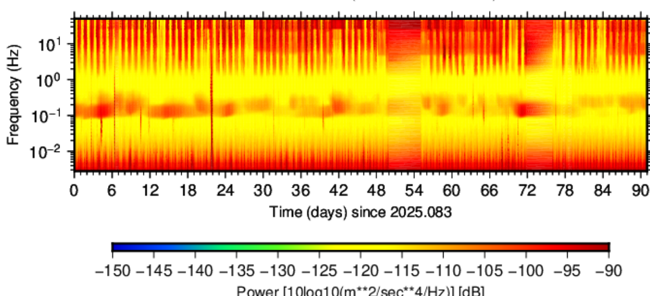
BK.AL VW.HNE.00 (2025.083 - 2025.173)
