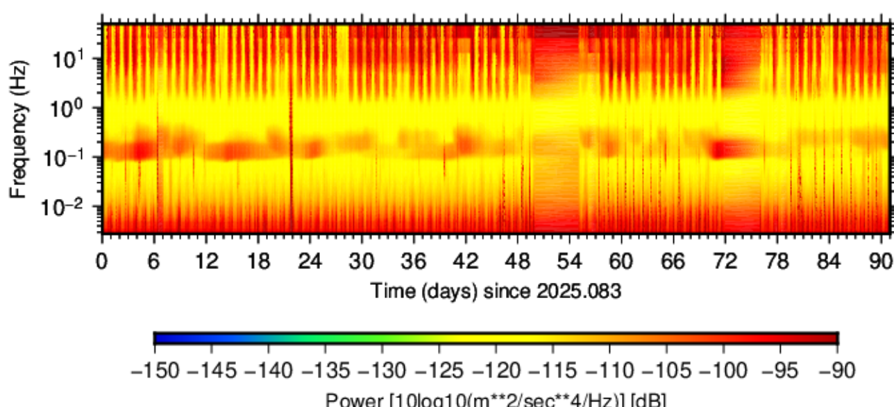
BK.AL VW.HNN.00 (2025.083 - 2025.173)
