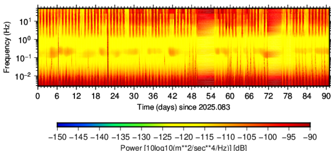
BK.AL VW.HNZ.00 (2025.083 - 2025.173)
