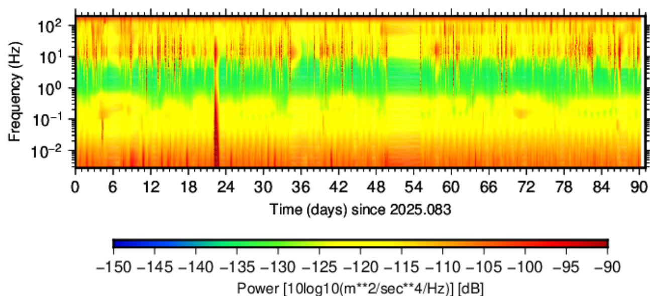
BG.ACR.CNN. (2025.083 - 2025.173)
