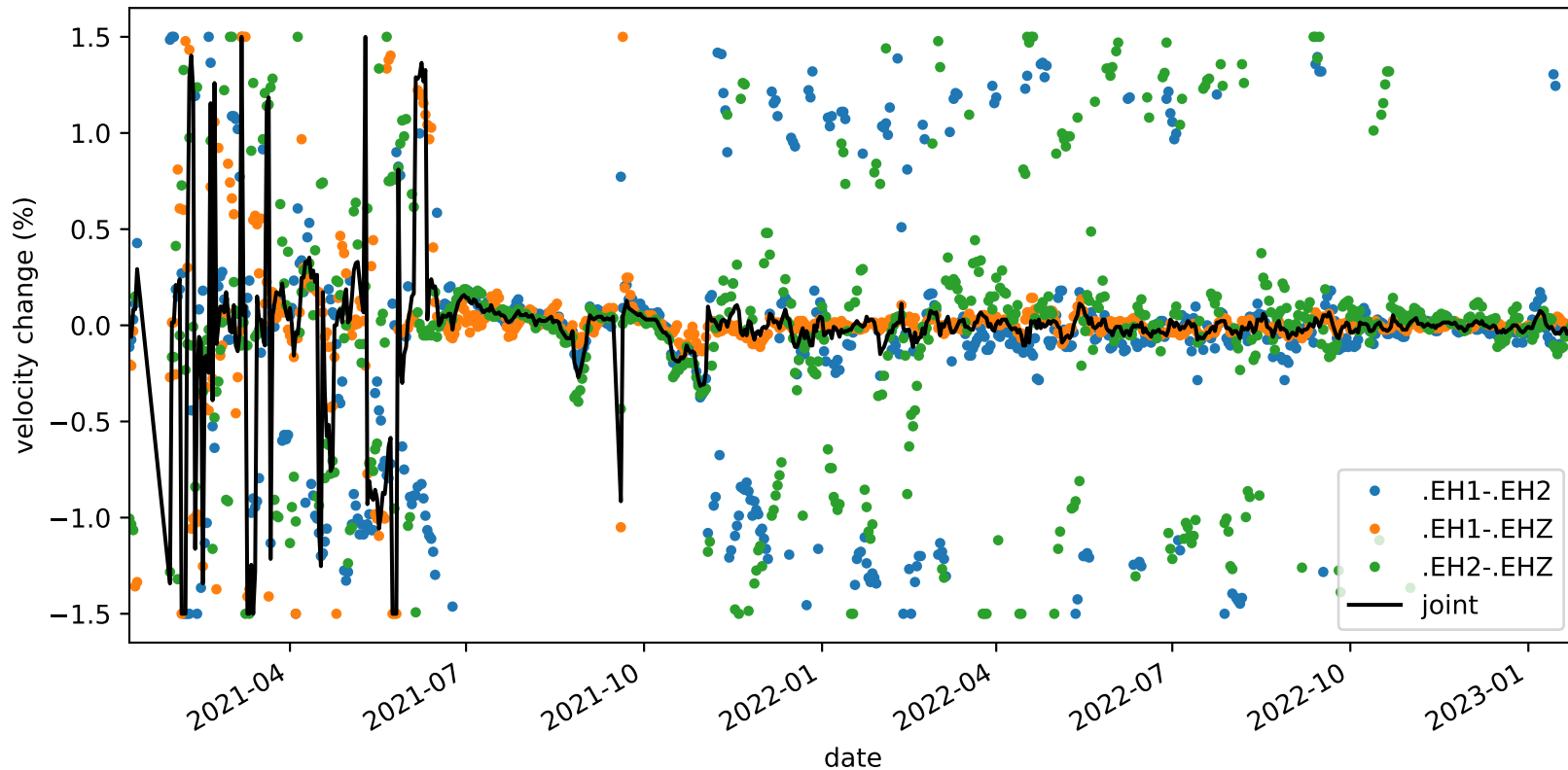
velocity_change_cli_s4_t1b_tw_010.0s-015.0s_PB.B935-PB.B935
