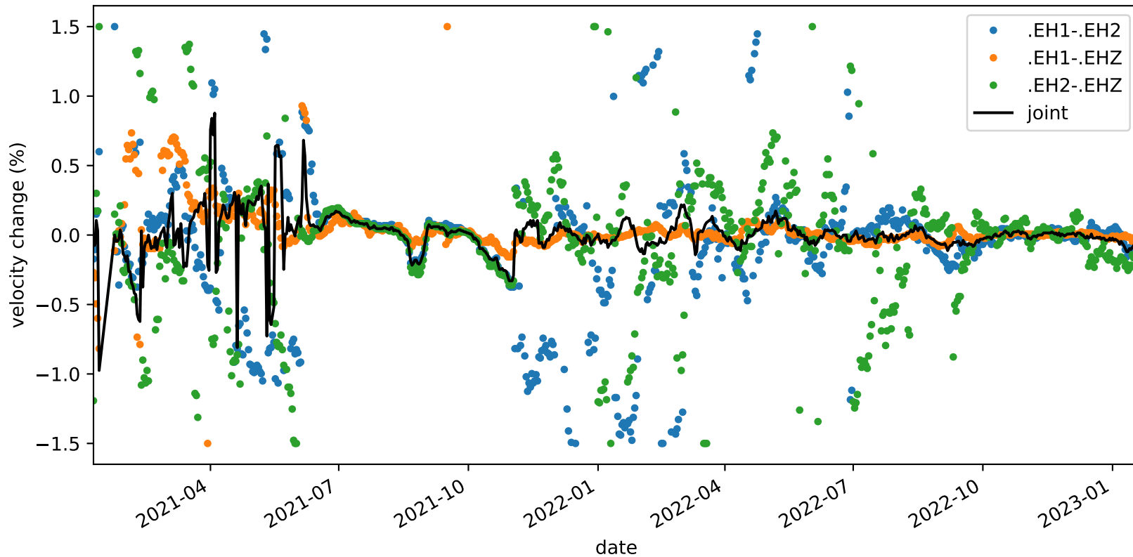
velocity_change_c1h_s3_t1b_tw_010.0s-015.0s_PB.B935-PB.B935
