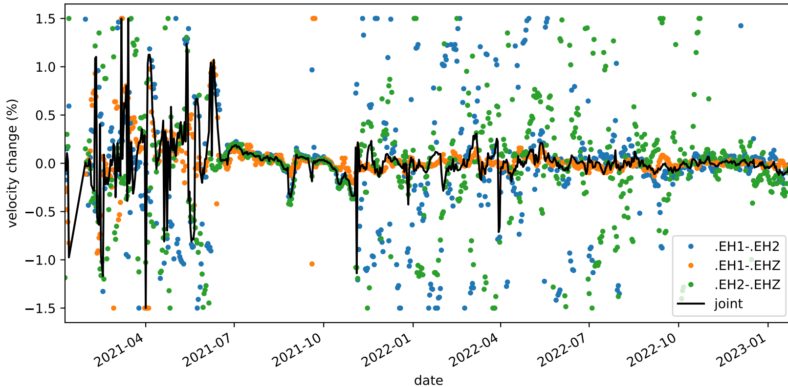
velocity_change_c1h_s4_t1b_tw_010.0s-015.0s_PB.B935-PB.B935
