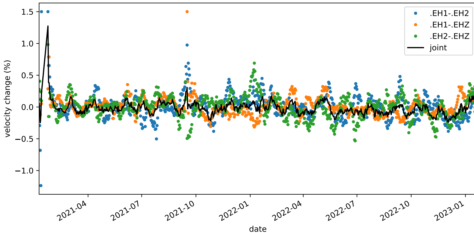
velocity_change_c1e_s3_t1b_tw_010.0s-015.0s_PB.B935-PB.B935
