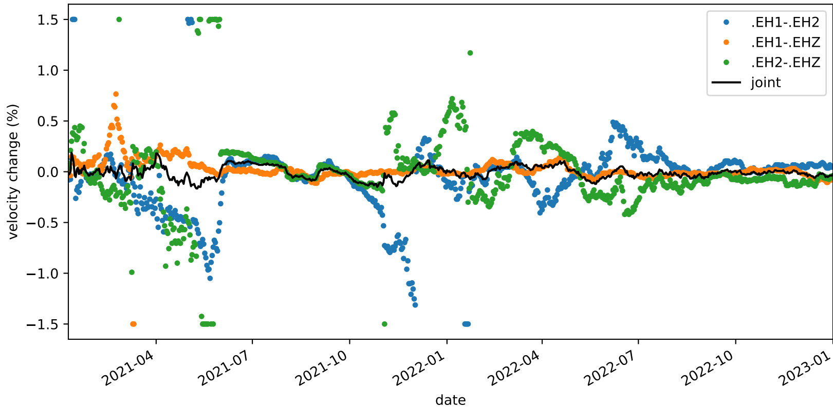
velocity_change_c1b_s2_t1b_tw_010.0s-015.0s_PB.B935-PB.B935
