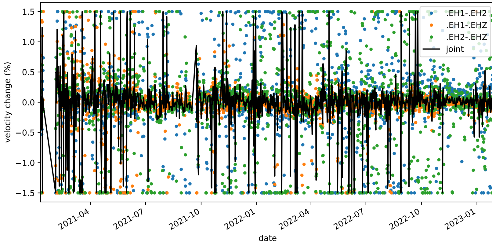
velocity_change_c1c_s1_t1a_tw_005.0s-010.0s_PB.B935-PB.B935
