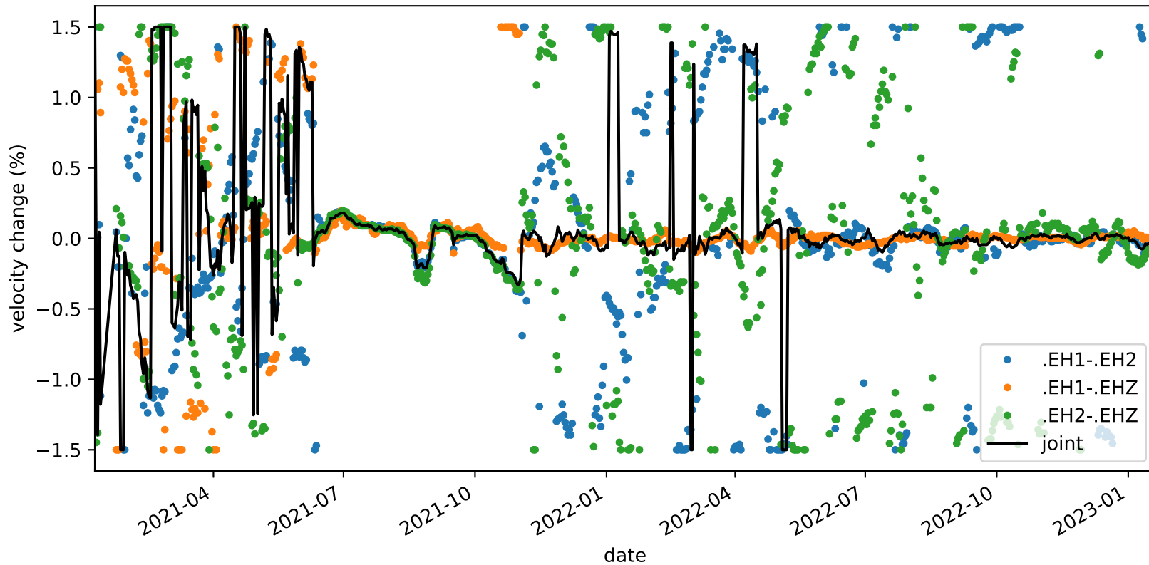
velocity_change_c1_s3_t1b_tw_010.0s-015.0s_PB.B935-PB.B935
