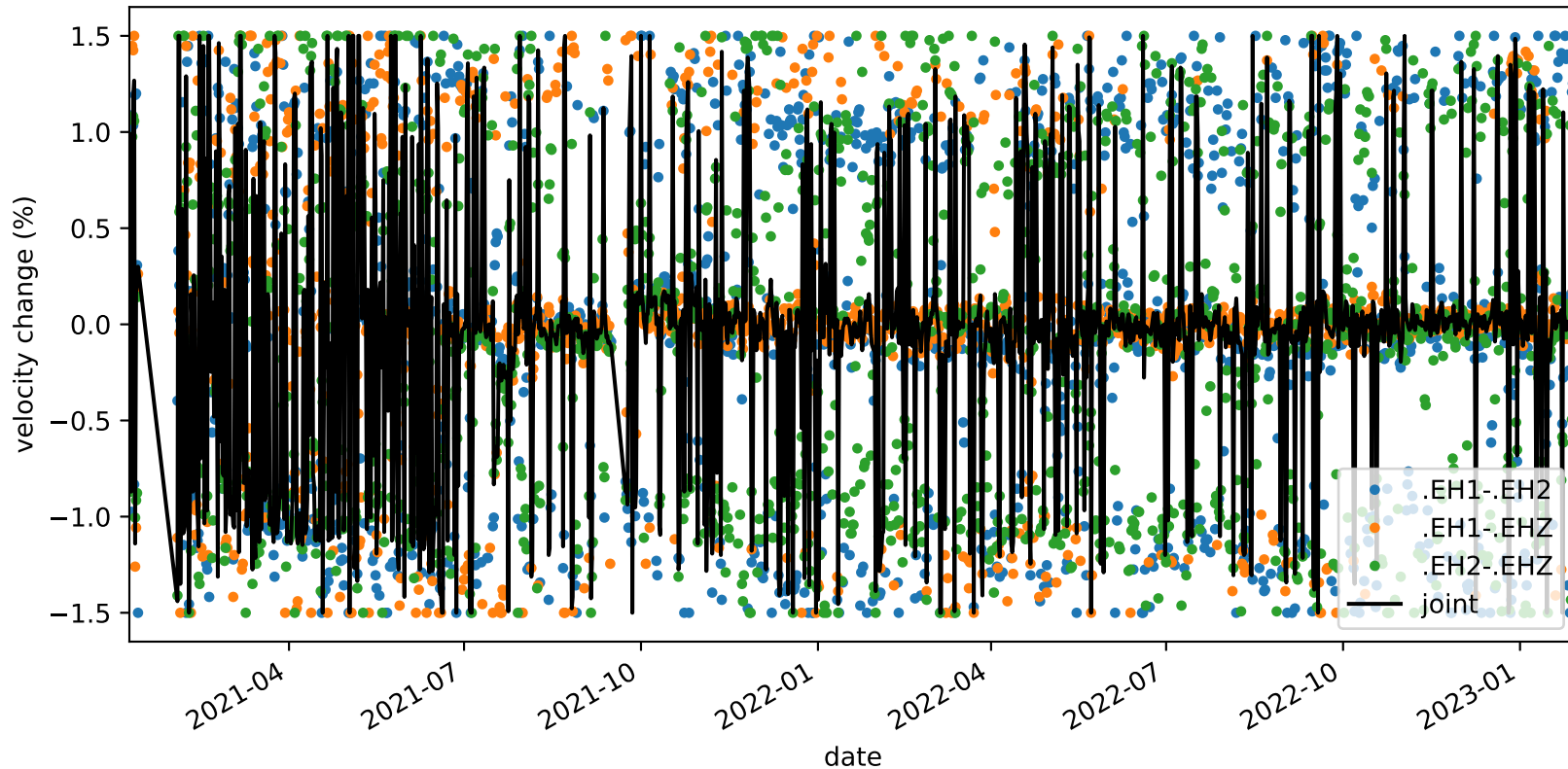
velocity_change_c1c_s1_t1b_tw_010.0s-015.0s_PB.B935-PB.B935
