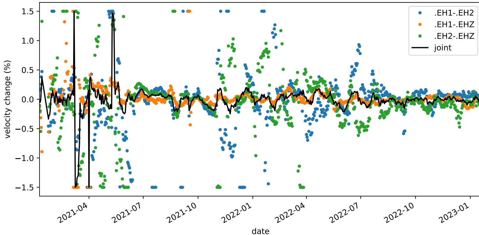
velocity_change_c1b_s3_t1b_tw_010.0s-015.0s_PB.B935-PB.B935
