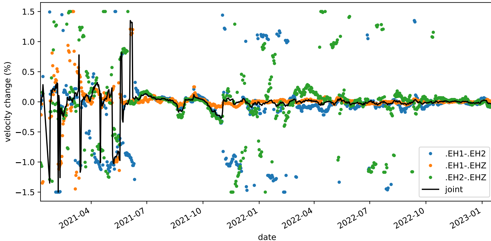
velocity_change_c1i_s3_t1b_tw_010.0s-015.0s_PB.B935-PB.B935
