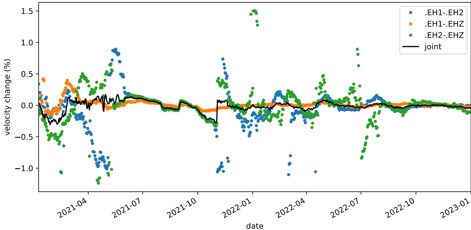
velocity_change_c1h_s2_t1c_tw_005.0s-015.0s_PB.B935-PB.B935
