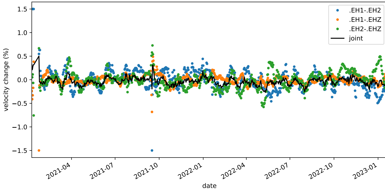
velocity_change_c1f_s3_t1a_tw_005.0s-010.0s_PB.B935-PB.B935
