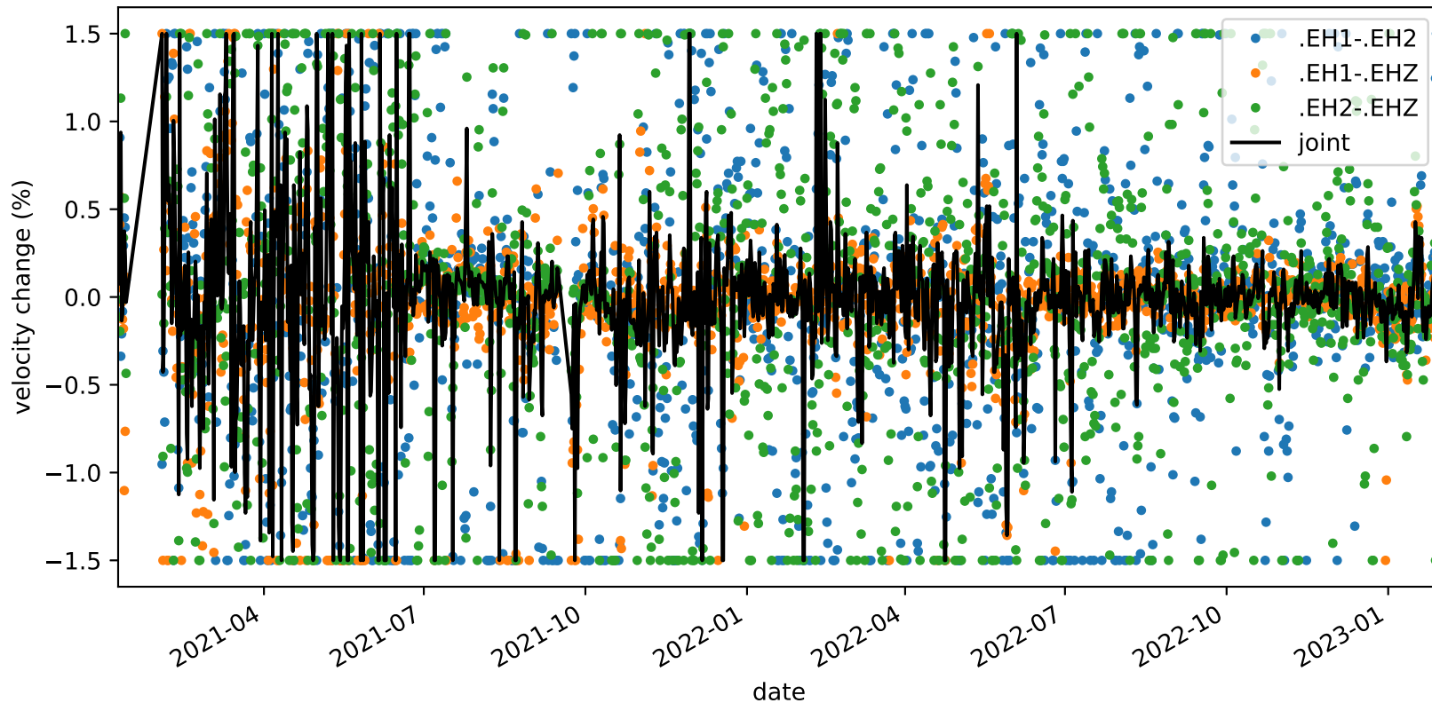
velocity_change_c1b_s1_t1c_tw_005.0s-015.0s_PB.B935-PB.B935
