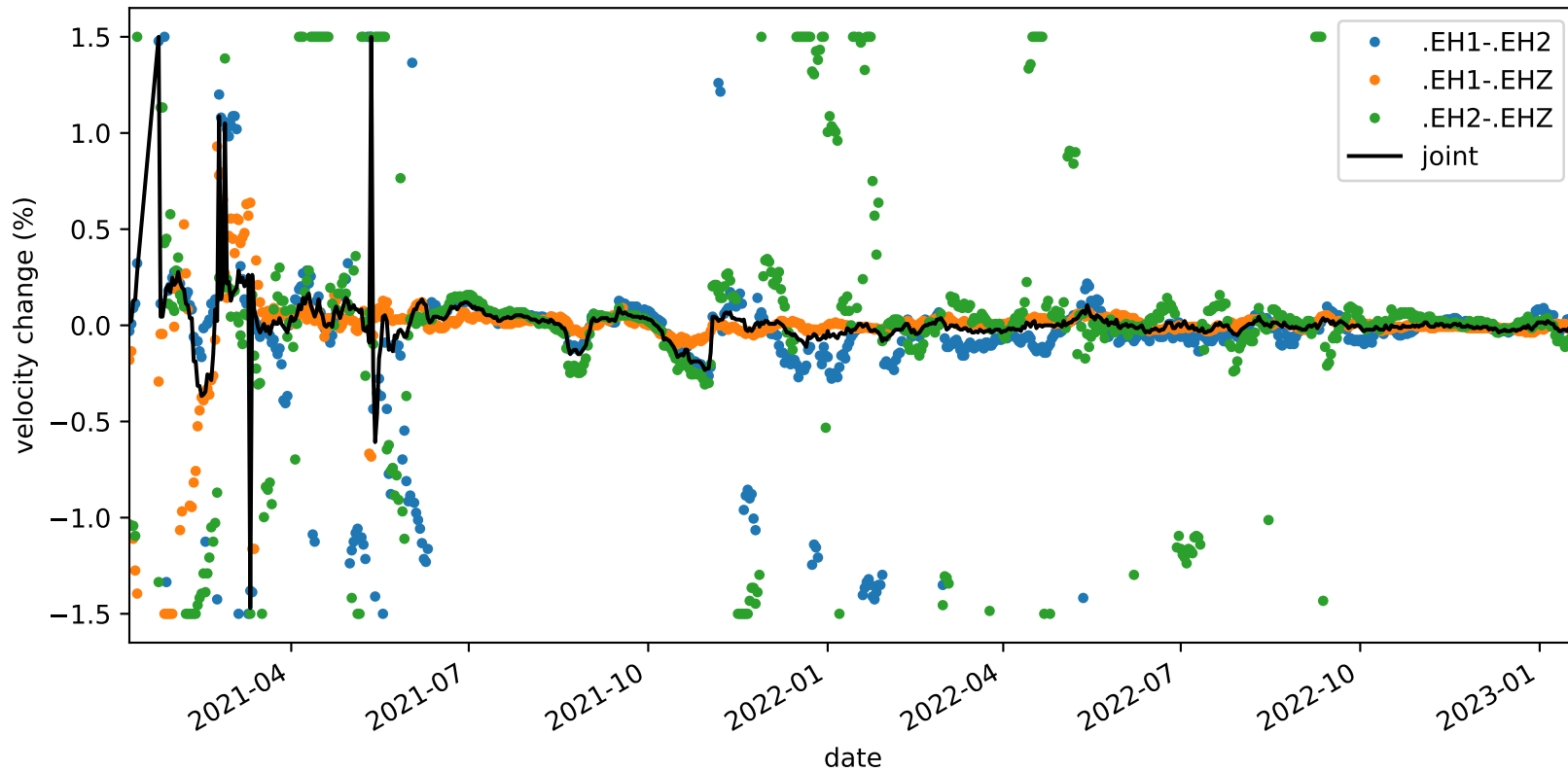
velocity_change_c1i_s3_t1c_tw_005.0s-015.0s_PB.B935-PB.B935
