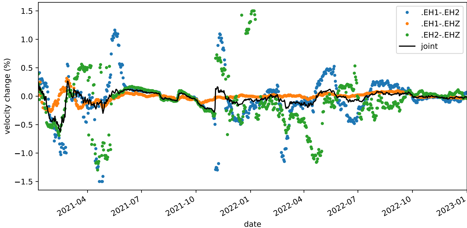
velocity_change_c1h_s2_t1a_tw_005.0s-010.0s_PB.B935-PB.B935
