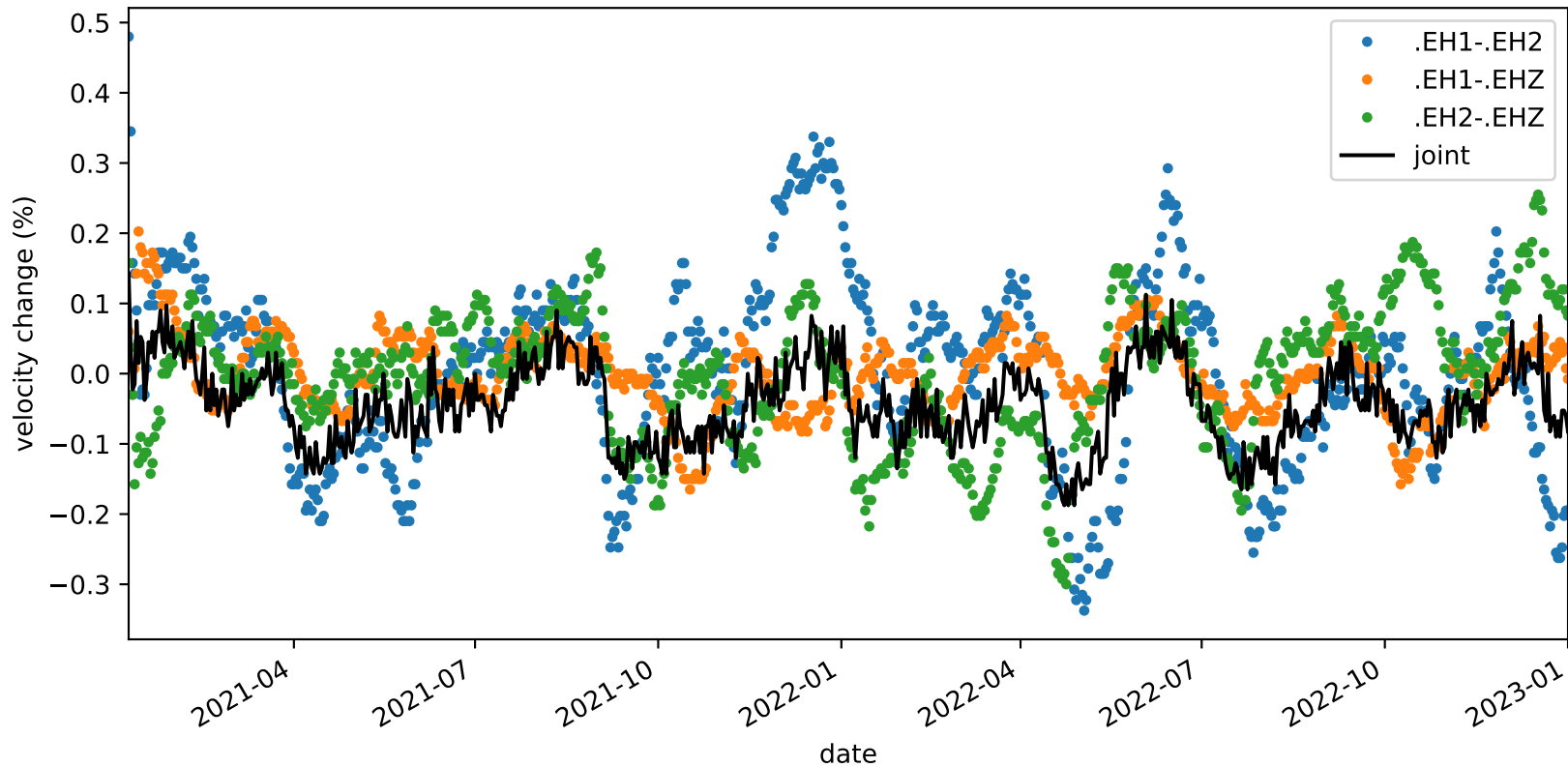
velocity_change_c1e_s2_t1a_tw_005.0s-010.0s_PB.B935-PB.B935
