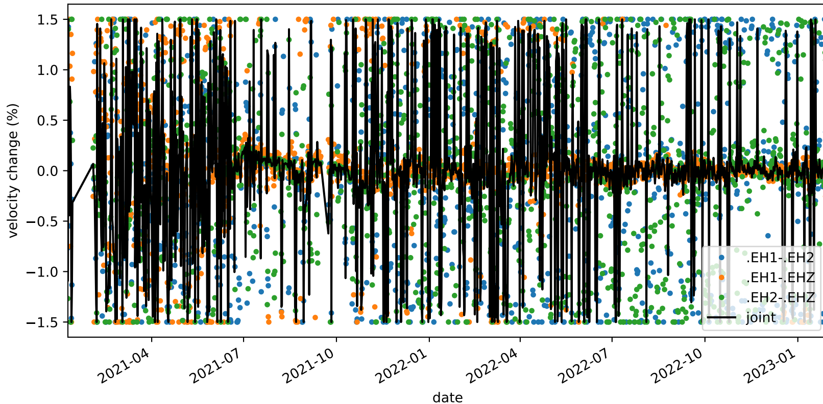
velocity_change_c1_s1_t1b_tw_010.0s-015.0s_PB.B935-PB.B935
