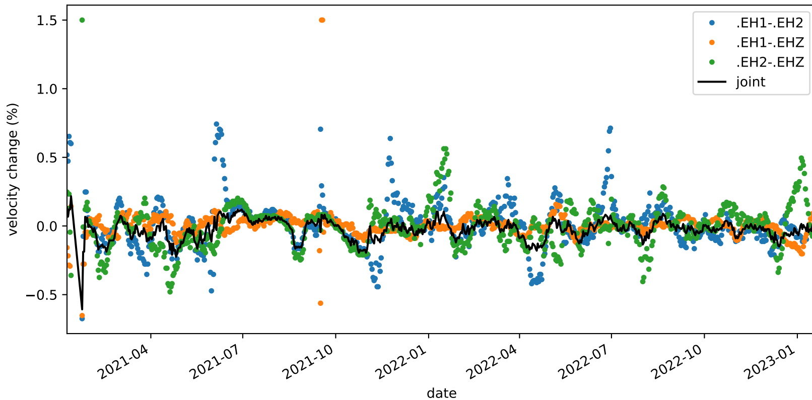
velocity_change_c1g_s3_t1c_tw_005.0s-015.0s_PB.B935-PB.B935
