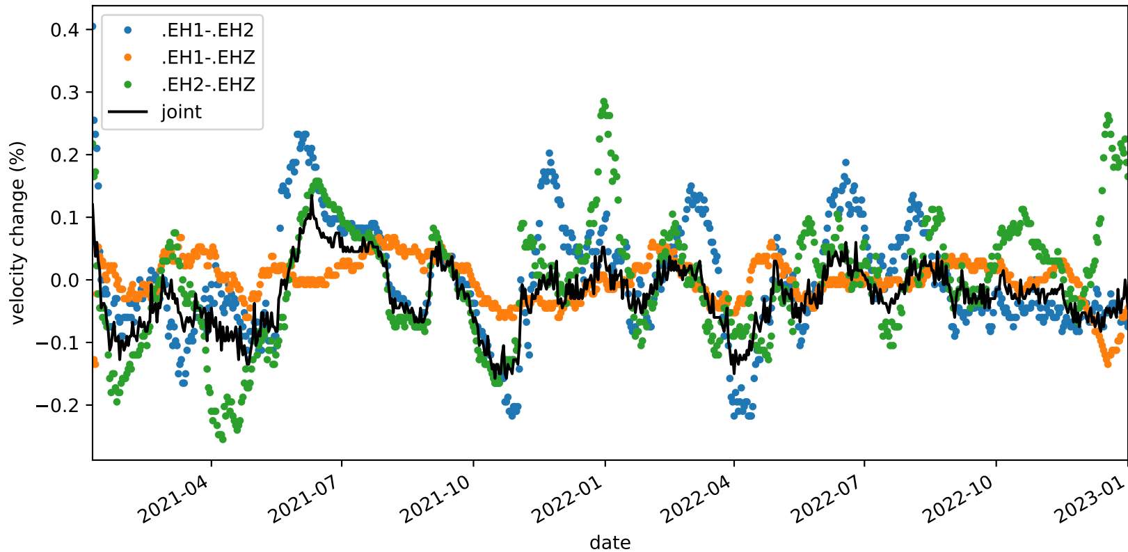
velocity_change_c1g_s2_t1c_tw_005.0s-015.0s_PB.B935-PB.B935
