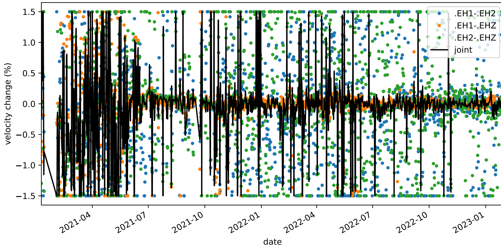
velocity_change_c1_s1_t1c_tw_005.0s-015.0s_PB.B935-PB.B935
