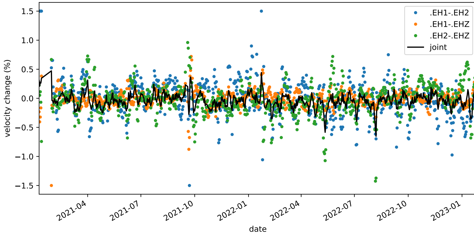
velocity_change_c1f_s4_t1a_tw_005.0s-010.0s_PB.B935-PB.B935
