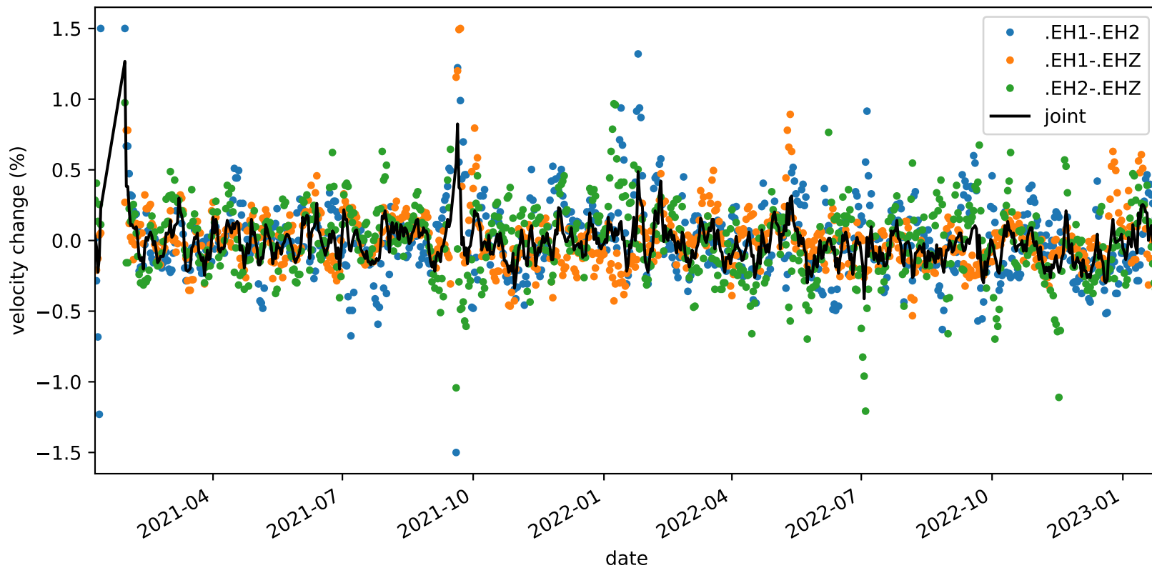
velocity_change_c1e_s4_t1b_tw_010.0s-015.0s_PB.B935-PB.B935
