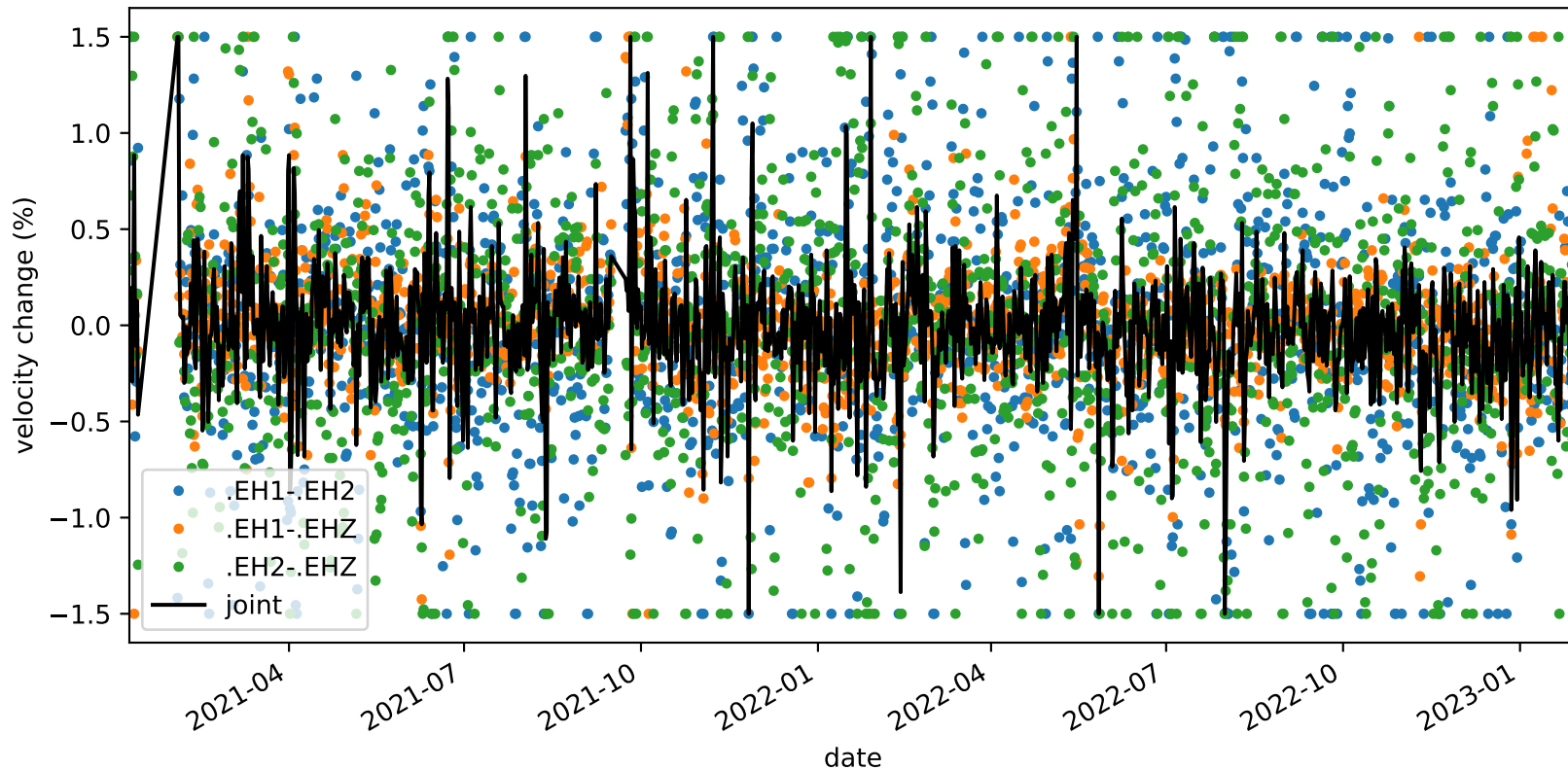
velocity_change_c1f_s1_t1b_tw_010.0s-015.0s_PB.B935-PB.B935
