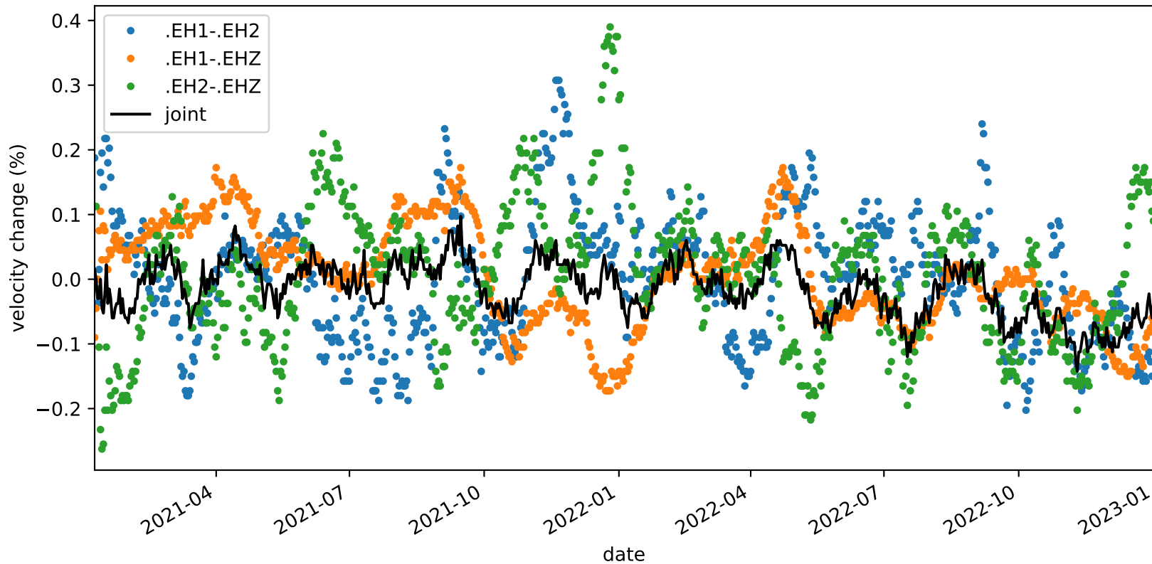
velocity_change_c1f_s2_t1b_tw_010.0s-015.0s_PB.B935-PB.B935
