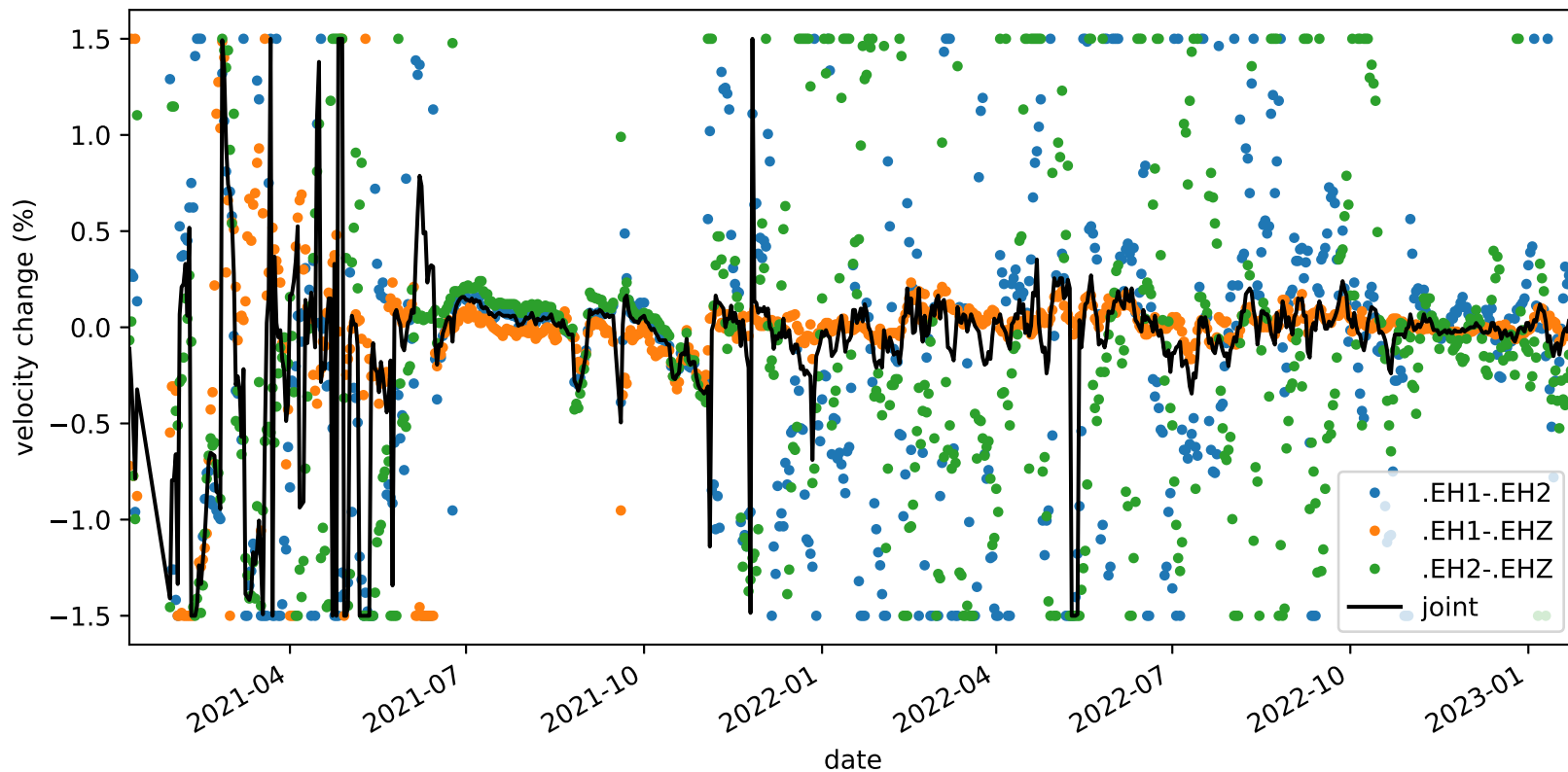
velocity_change_c1_s4_t1a_tw_005.0s-010.0s_PB.B935-PB.B935
