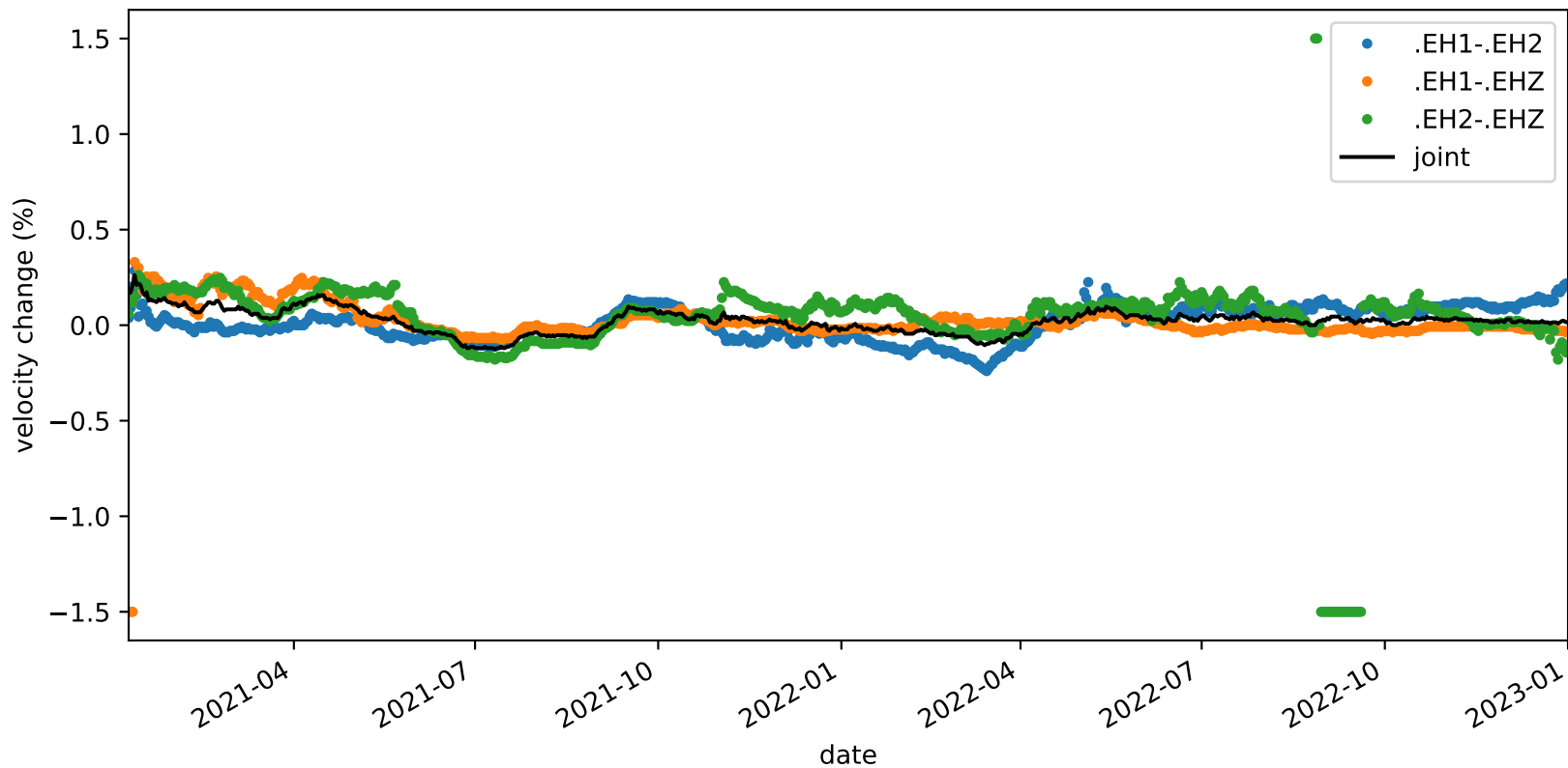
velocity_change_c1c_s2_t1a_tw_005.0s-010.0s_PB.B935-PB.B935
