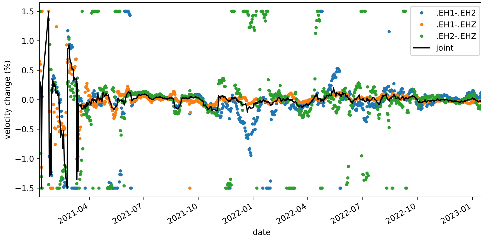
velocity_change_c1i_s3_t1a_tw_005.0s-010.0s_PB.B935-PB.B935
