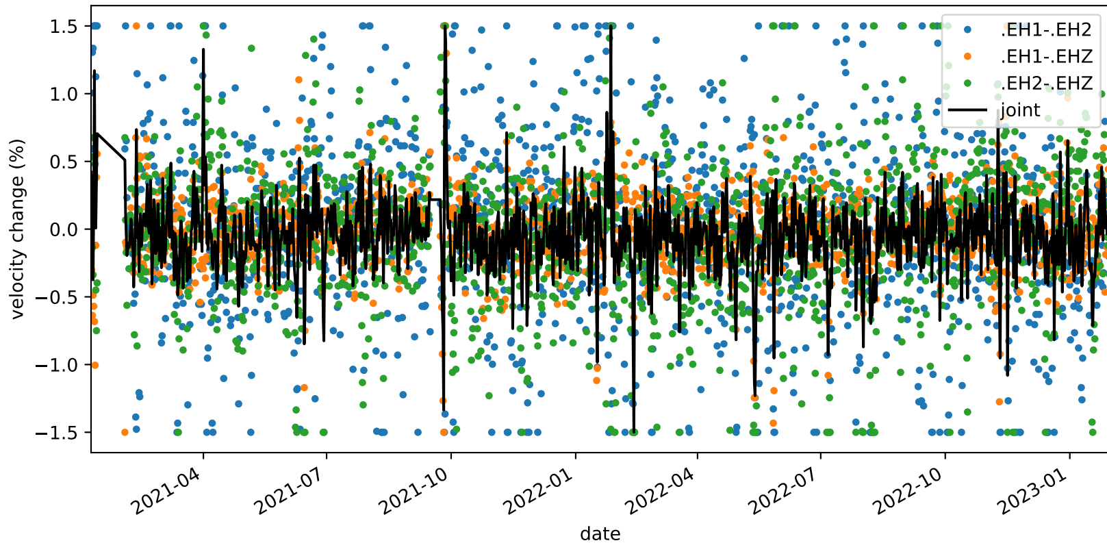
velocity_change_c1f_s1_t1a_tw_005.0s-010.0s_PB.B935-PB.B935
