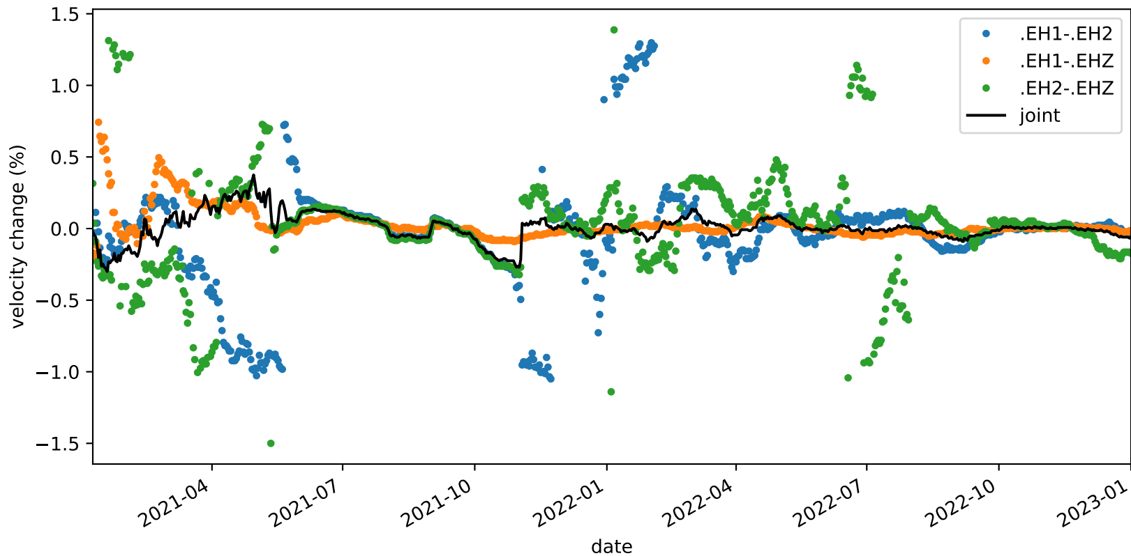
velocity_change_c1h_s2_t1b_tw_010.0s-015.0s_PB.B935-PB.B935
