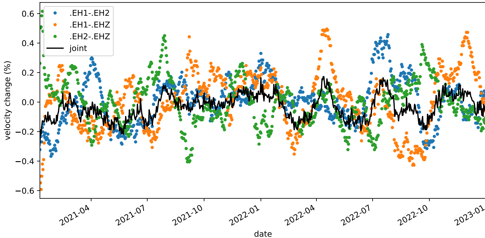
velocity_change_c1d_s2_t1b_tw_010.0s-015.0s_PB.B935-PB.B935
