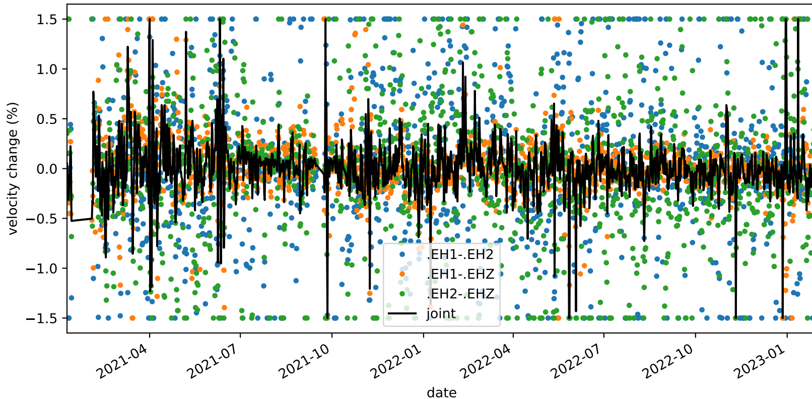
velocity_change_c1g_s1_t1b_tw_010.0s-015.0s_PB.B935-PB.B935
