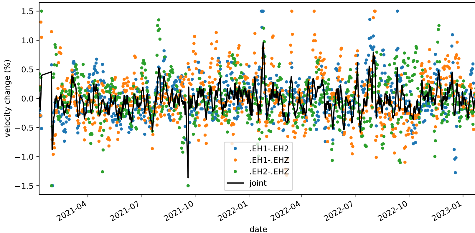
velocity_change_c1d_s4_t1b_tw_010.0s-015.0s_PB.B935-PB.B935
