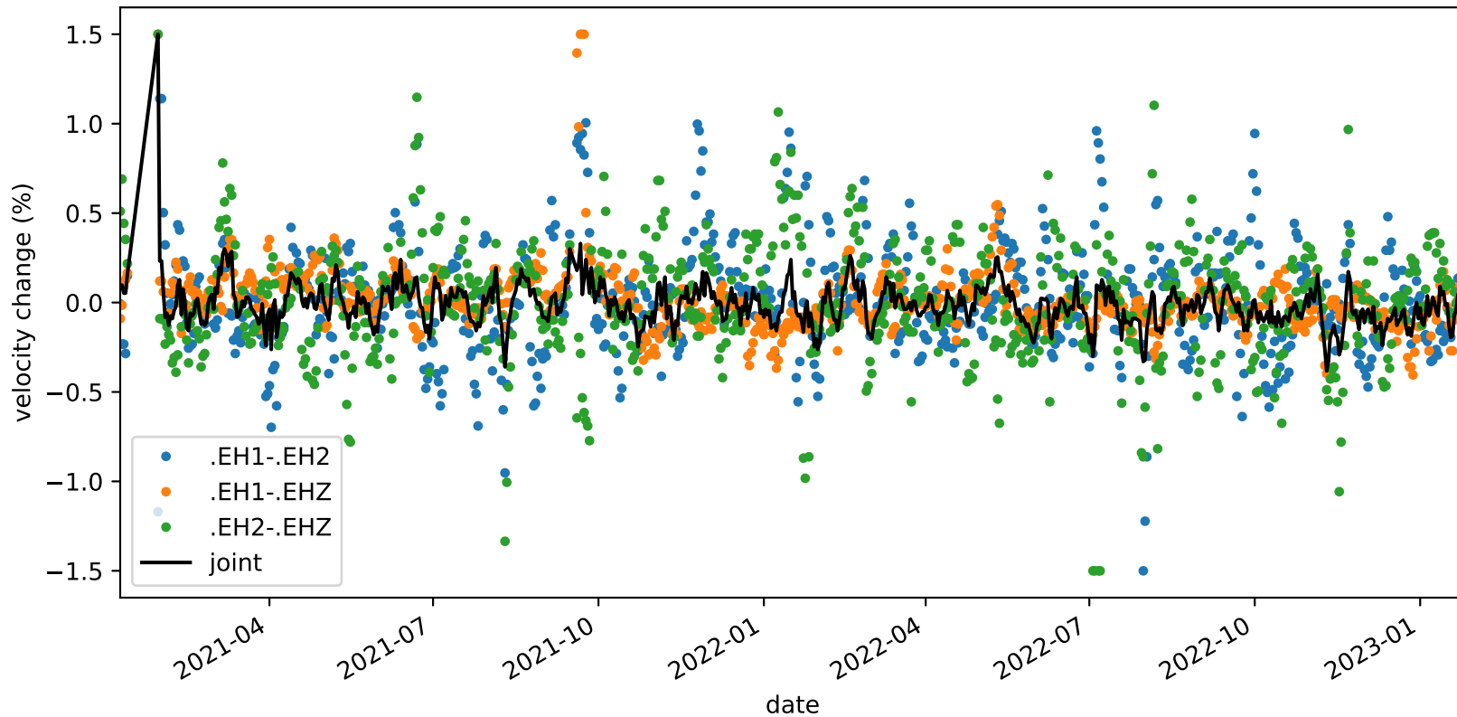
velocity_change_c1f_s4_t1b_tw_010.0s-015.0s_PB.B935-PB.B935
