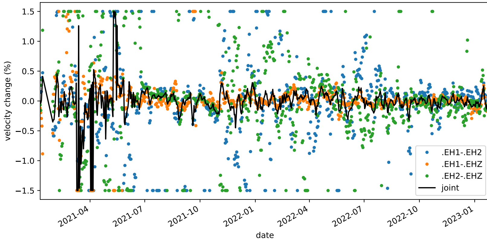
velocity_change_c1b_s4_t1b_tw_010.0s-015.0s_PB.B935-PB.B935
