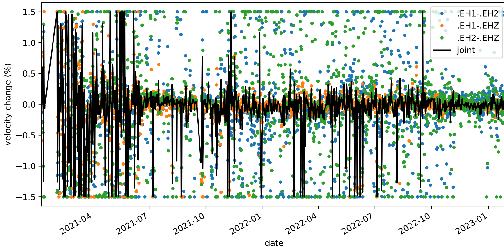
velocity_change_cli_s1_t1a_tw_005.0s-010.0s_PB.B935-PB.B935
