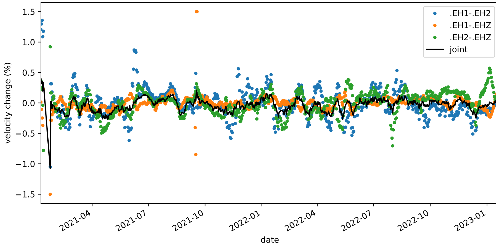
velocity_change_c1g_s3_t1a_tw_005.0s-010.0s_PB.B935-PB.B935
