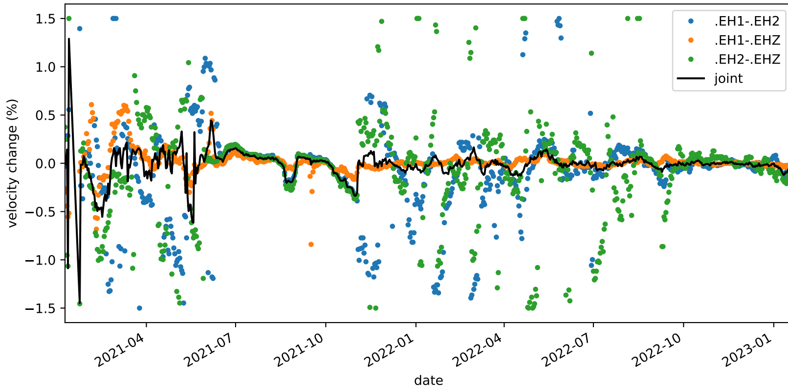
velocity_change_c1h_s3_t1c_tw_005.0s-015.0s_PB.B935-PB.B935
