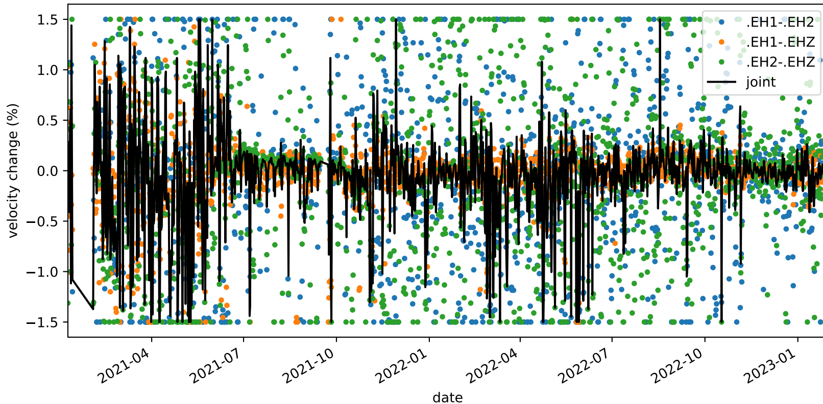
velocity_change_c1h_s1_t1a_tw_005.0s-010.0s_PB.B935-PB.B935
