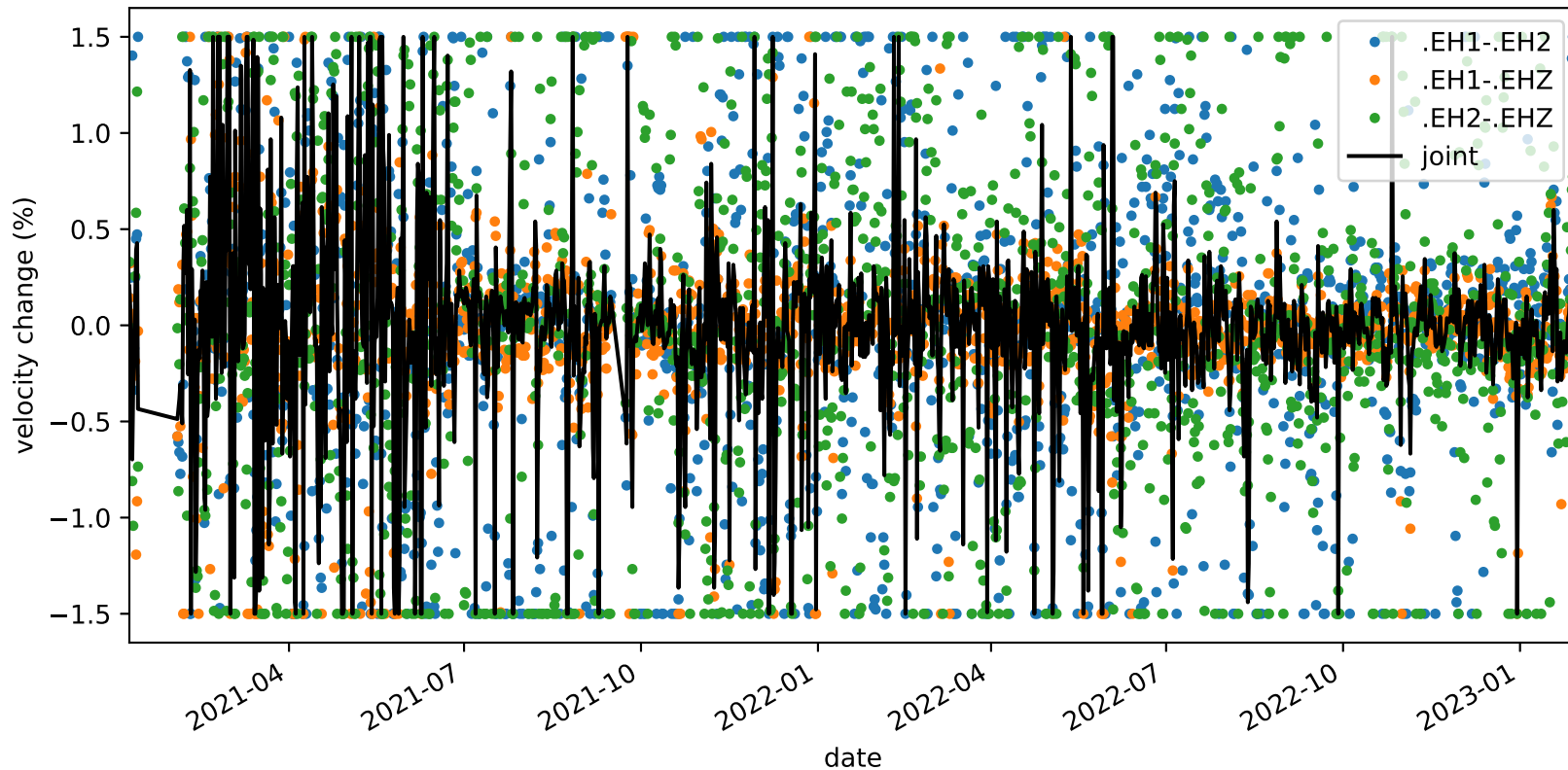
velocity_change_c1b_s1_t1b_tw_010.0s-015.0s_PB.B935-PB.B935
