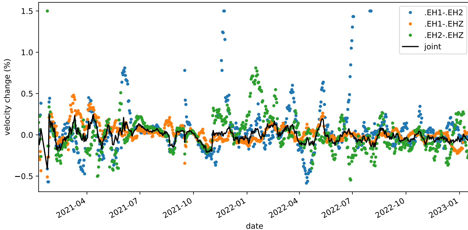
velocity_change_c1g_s3_t1b_tw_010.0s-015.0s_PB.B935-PB.B935
