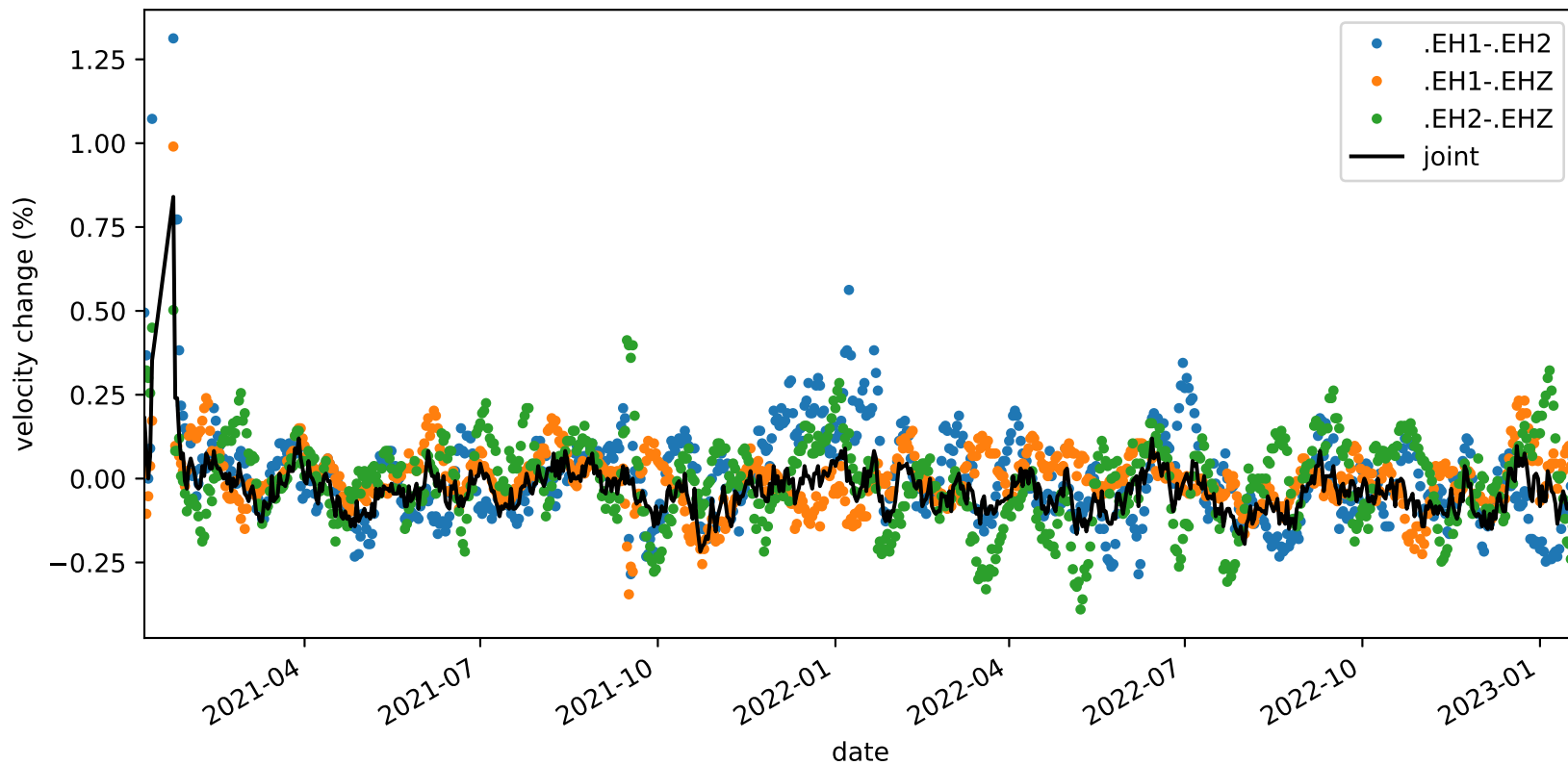
velocity_change_c1e_s3_t1c_tw_005.0s-015.0s_PB.B935-PB.B935
