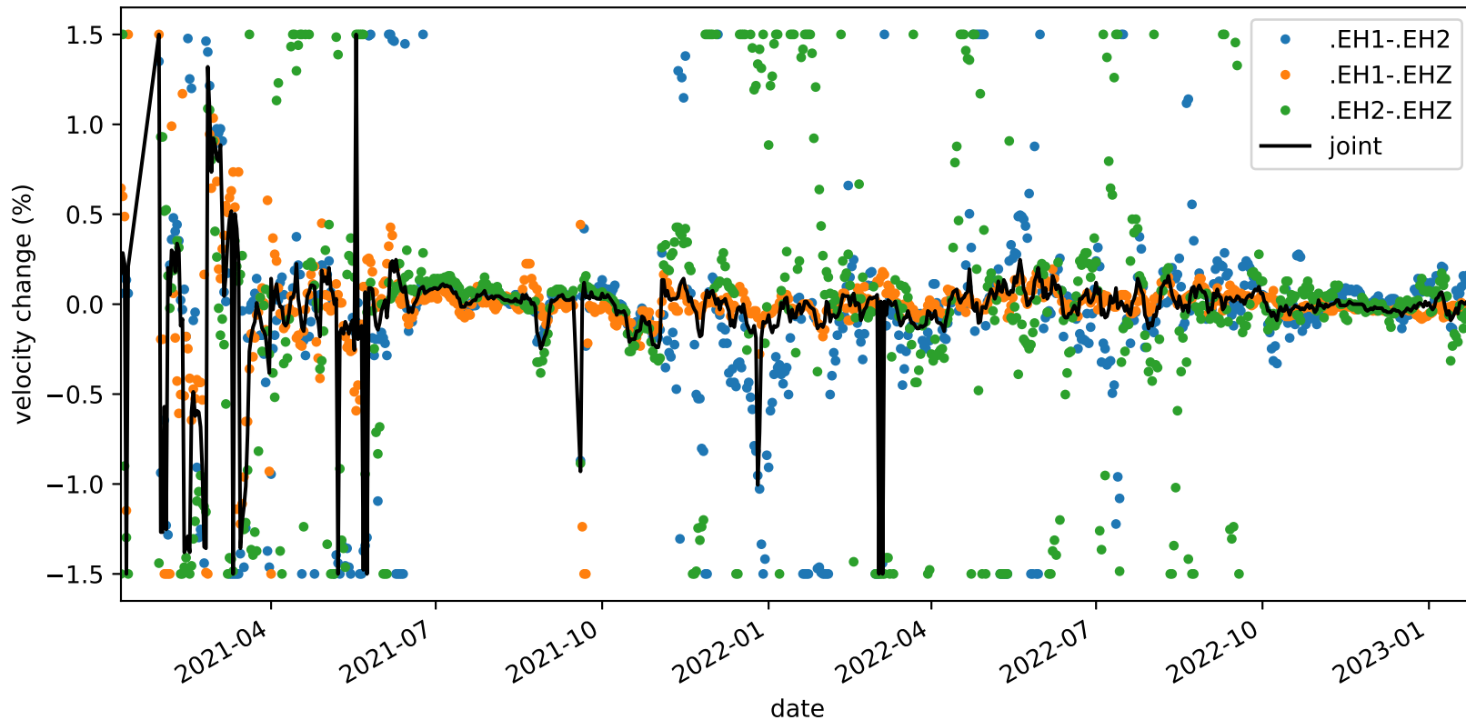
velocity_change_cli_s4_t1a_tw_005.0s-010.0s_PB.B935-PB.B935
