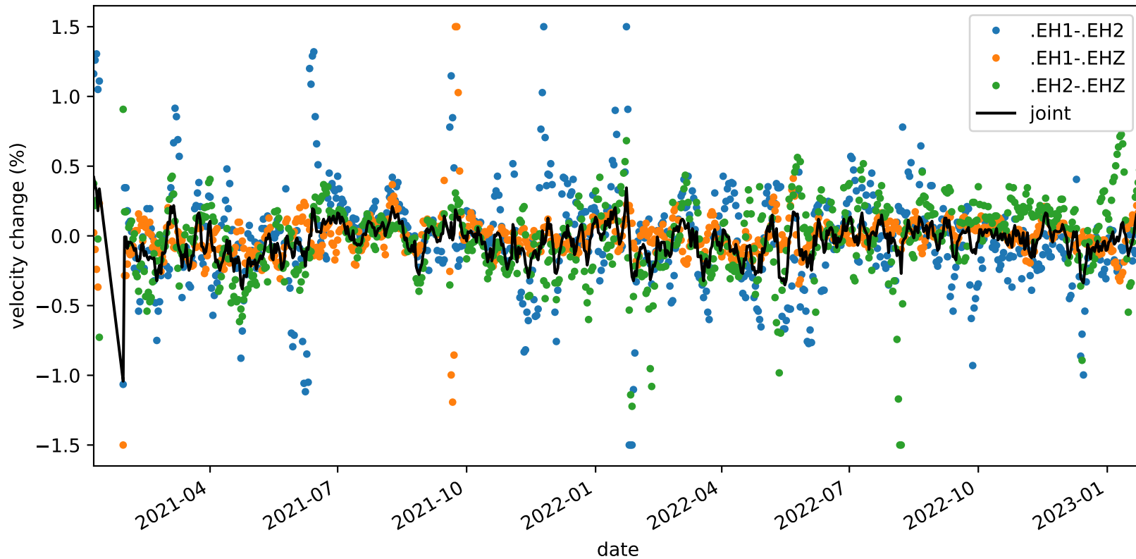
velocity_change_c1g_s4_t1a_tw_005.0s-010.0s_PB.B935-PB.B935
