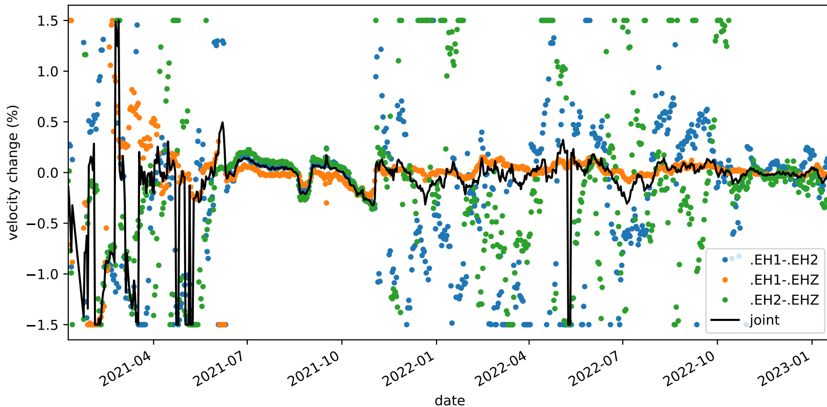
velocity_change_c1_s3_t1a_tw_005.0s-010.0s_PB.B935-PB.B935
