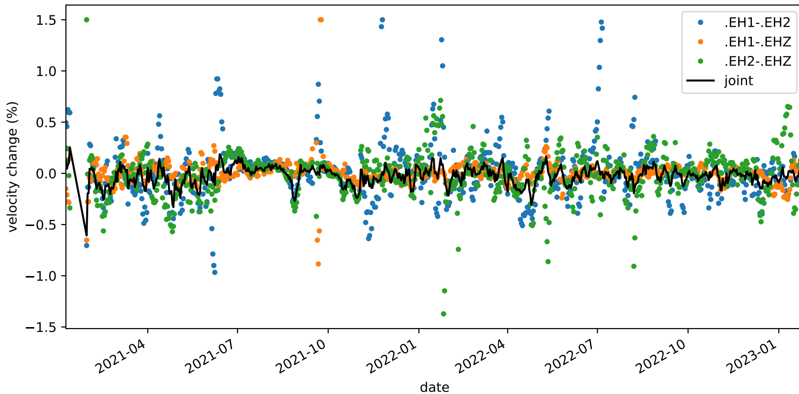
velocity_change_c1g_s4_t1c_tw_005.0s-015.0s_PB.B935-PB.B935
