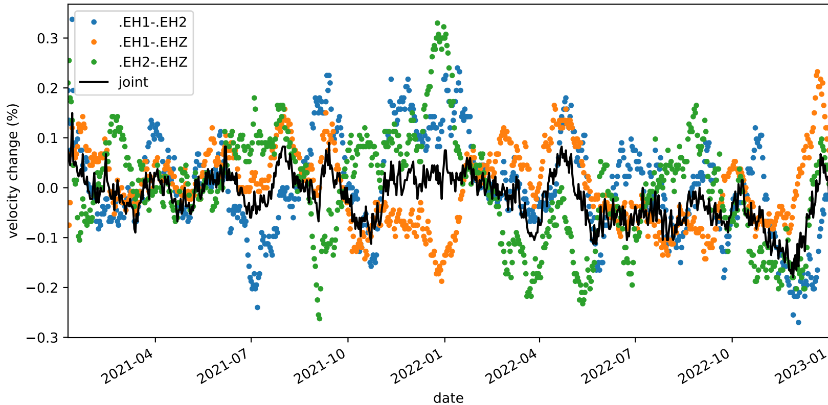
velocity_change_c1e_s2_t1b_tw_010.0s-015.0s_PB.B935-PB.B935
