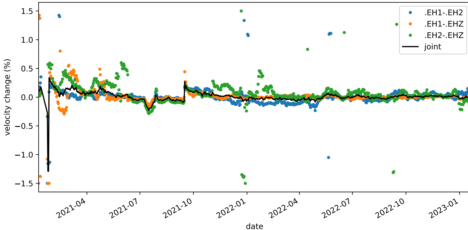
velocity_change_c1c_s3_t1c_tw_005.0s-015.0s_PB.B935-PB.B935
