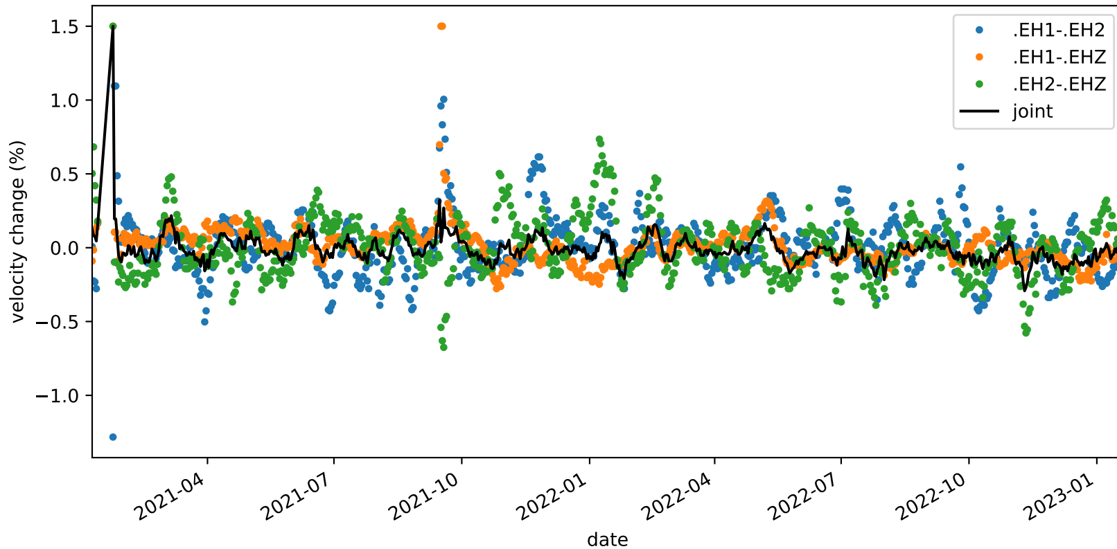
velocity_change_c1f_s3_t1b_tw_010.0s-015.0s_PB.B935-PB.B935
