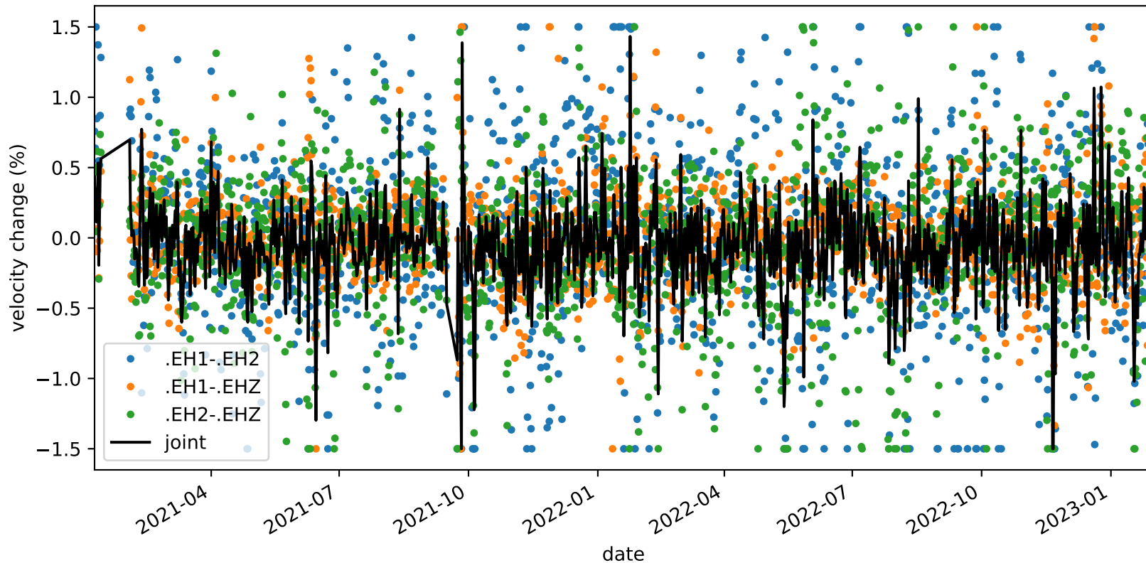
velocity_change_c1e_s1_t1a_tw_005.0s-010.0s_PB.B935-PB.B935
