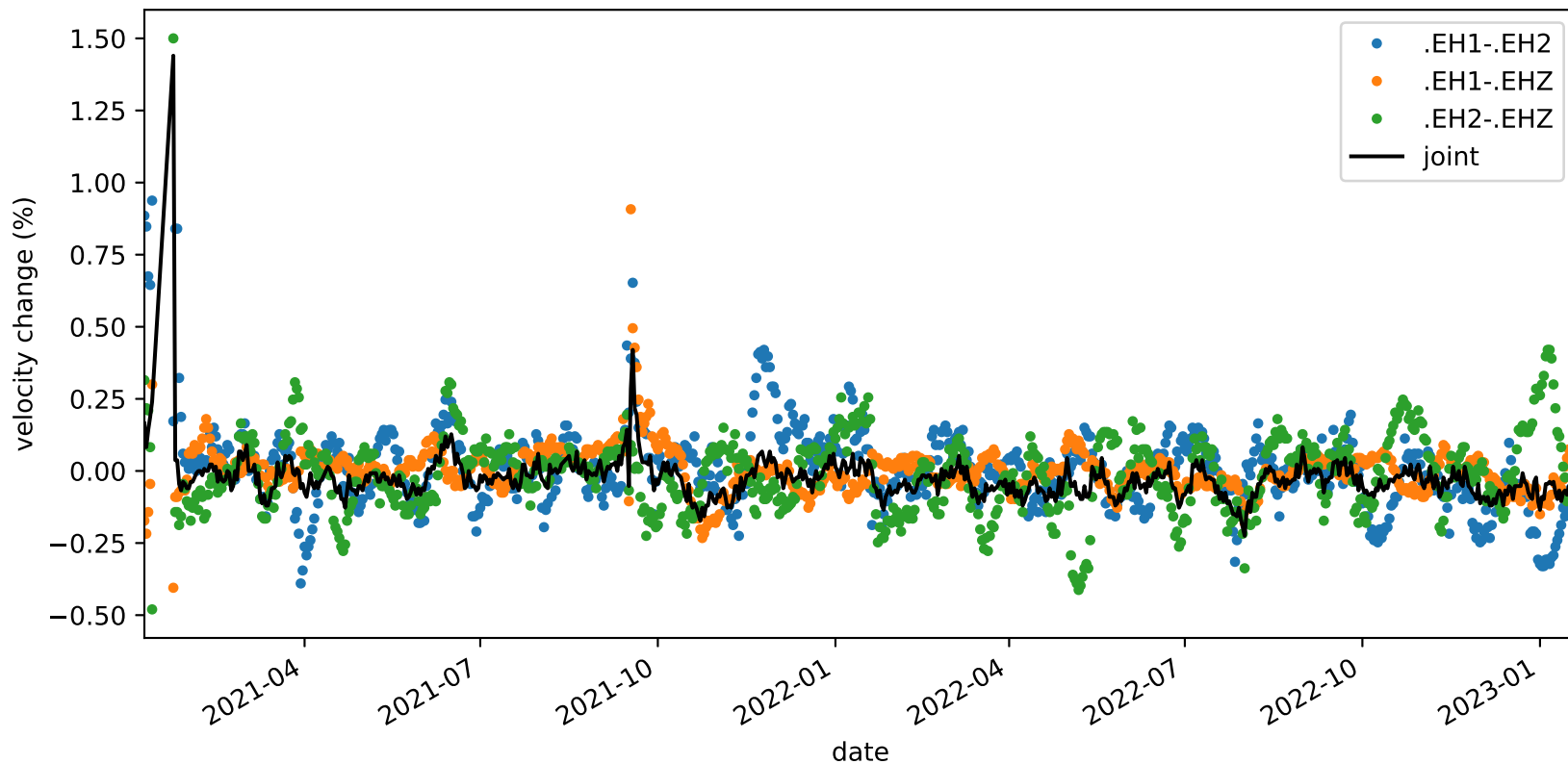
velocity_change_c1f_s3_t1c_tw_005.0s-015.0s_PB.B935-PB.B935
