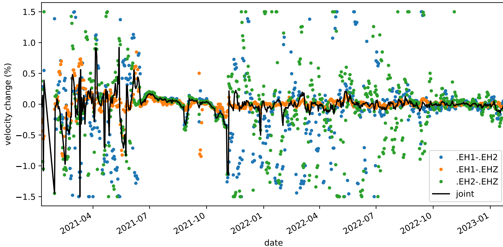
velocity_change_c1h_s4_t1c_tw_005.0s-015.0s_PB.B935-PB.B935
