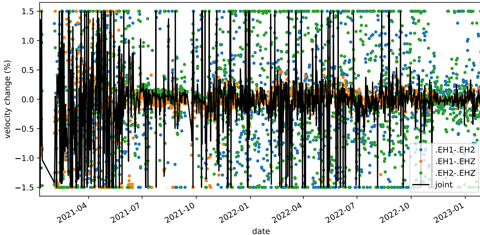
velocity_change_c1_s1_t1a_tw_005.0s-010.0s_PB.B935-PB.B935
