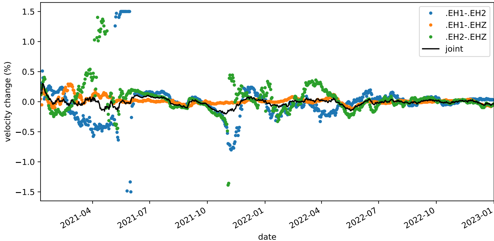
velocity_change_c1b_s2_t1c_tw_005.0s-015.0s_PB.B935-PB.B935
