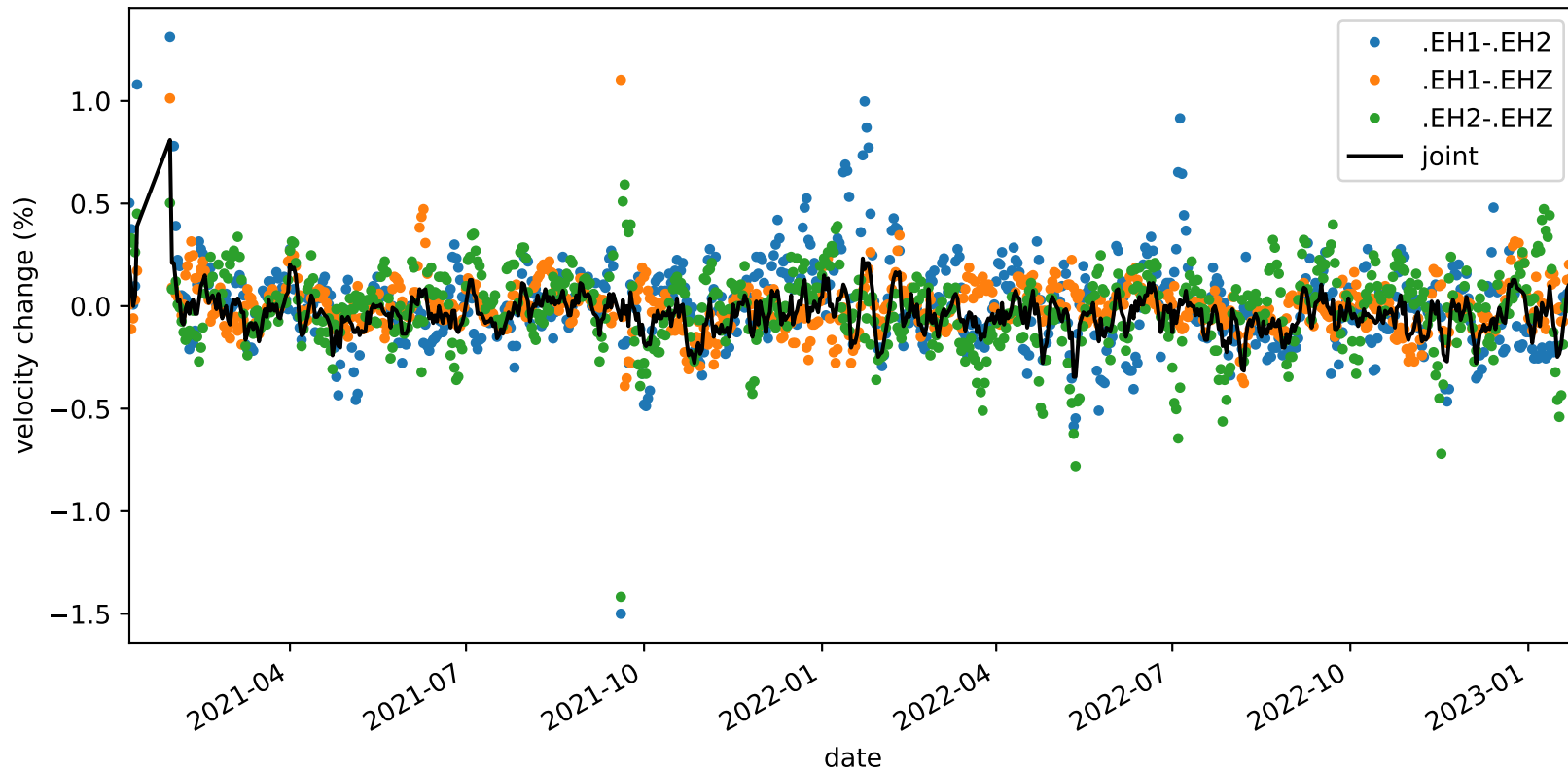
velocity_change_c1e_s4_t1c_tw_005.0s-015.0s_PB.B935-PB.B935
