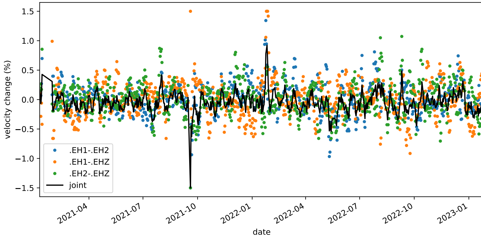
velocity_change_c1d_s4_t1c_tw_005.0s-015.0s_PB.B935-PB.B935
