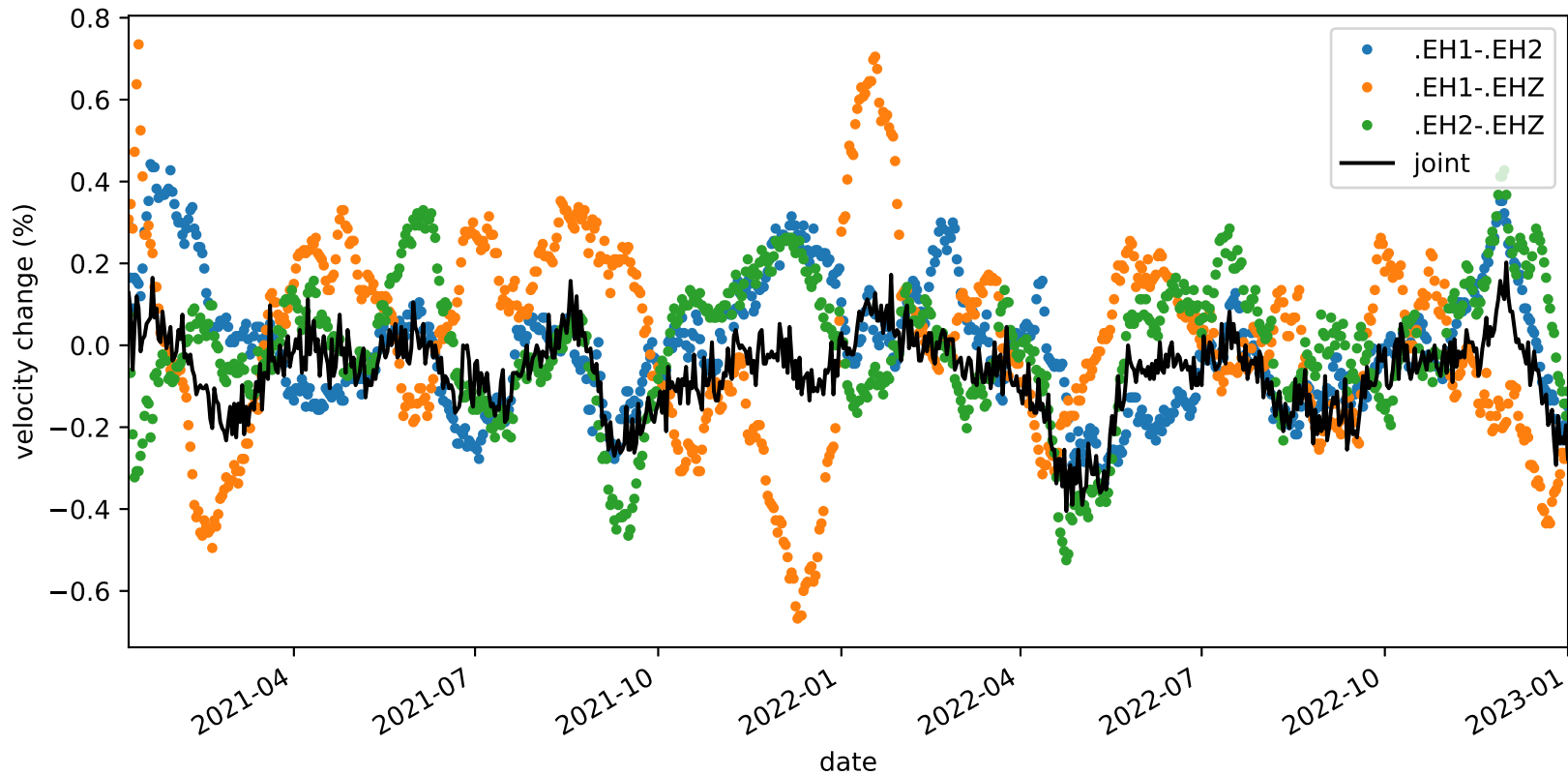
velocity_change_c1d_s2_t1a_tw_005.0s-010.0s_PB.B935-PB.B935
