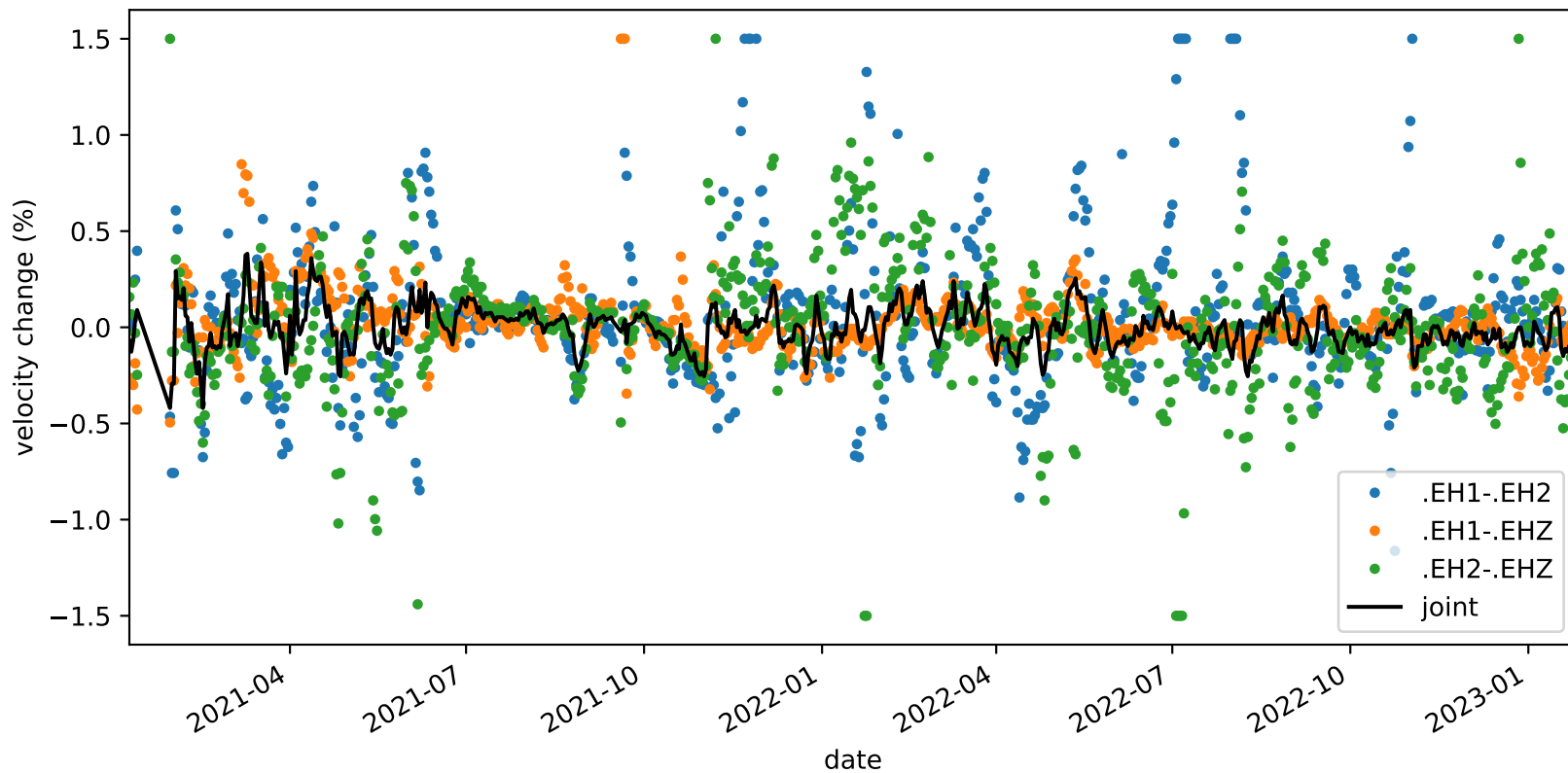
velocity_change_c1g_s4_t1b_tw_010.0s-015.0s_PB.B935-PB.B935
