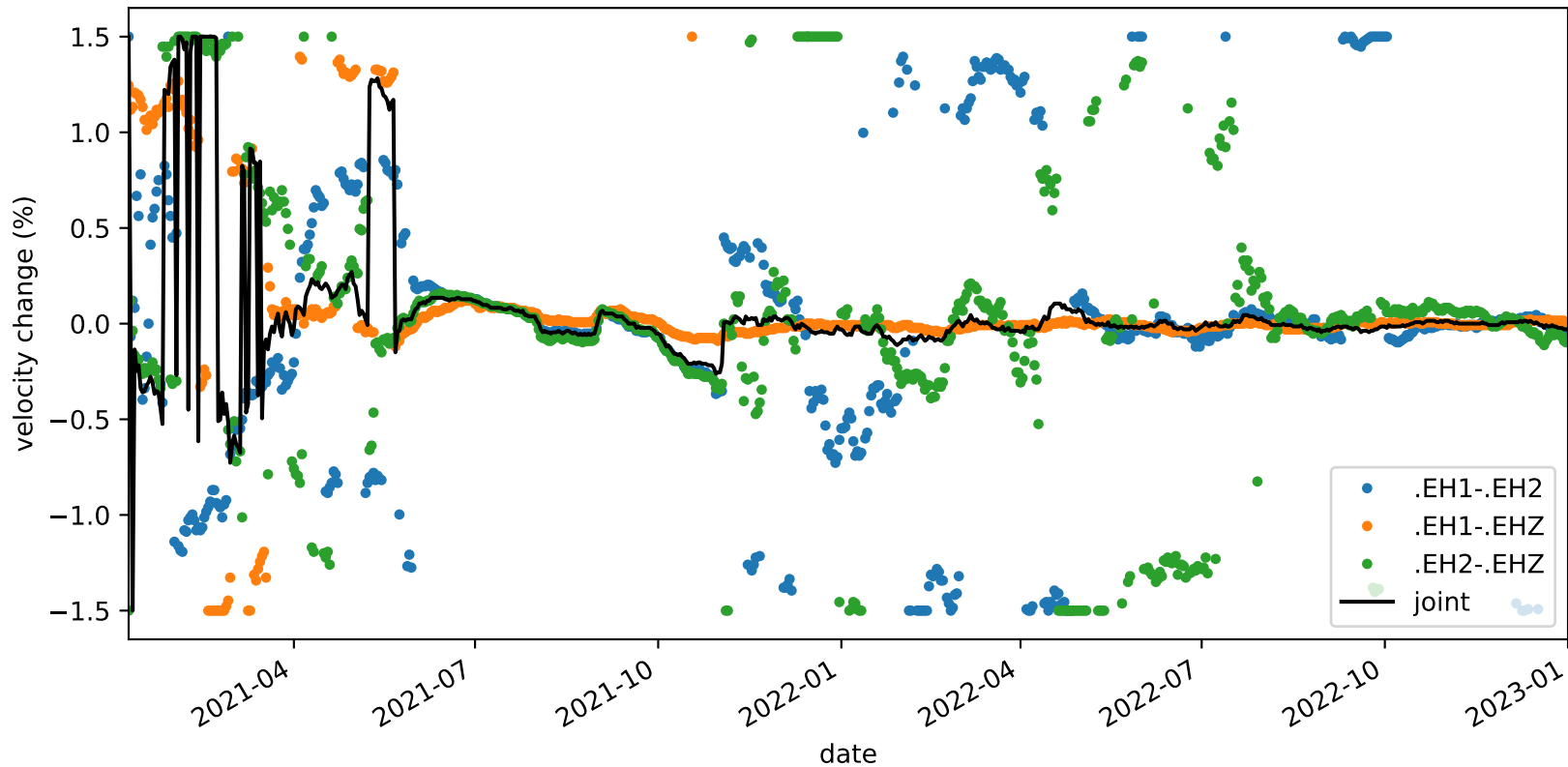
velocity_change_c1_s2_t1b_tw_010.0s-015.0s_PB.B935-PB.B935
