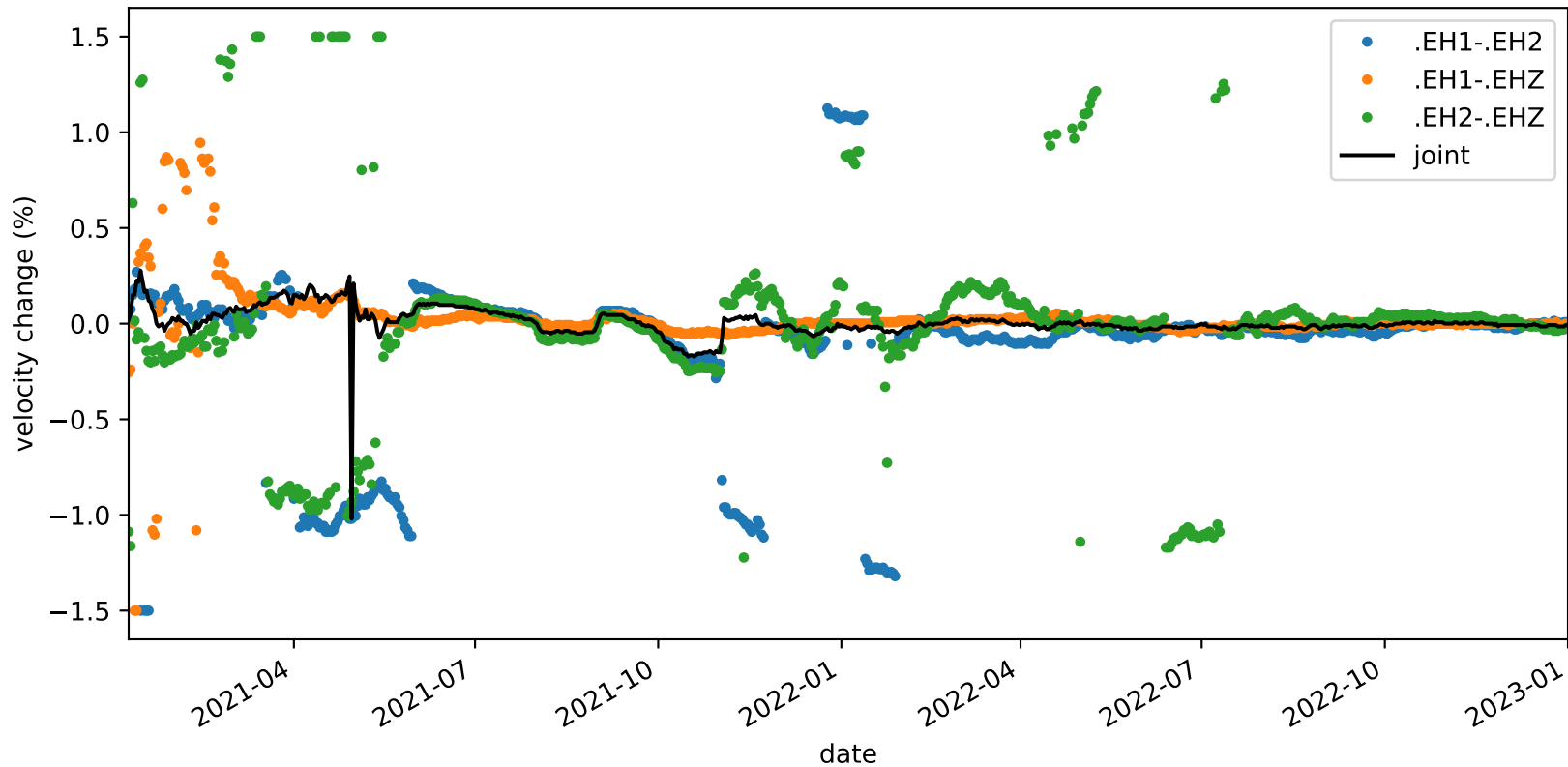
velocity_change_c1i_s2_t1b_tw_010.0s-015.0s_PB.B935-PB.B935
