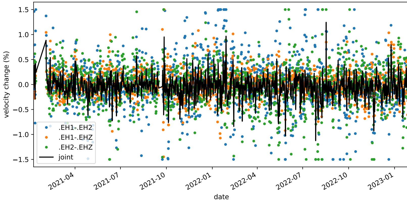
velocity_change_c1e_s1_t1c_tw_005.0s-015.0s_PB.B935-PB.B935
