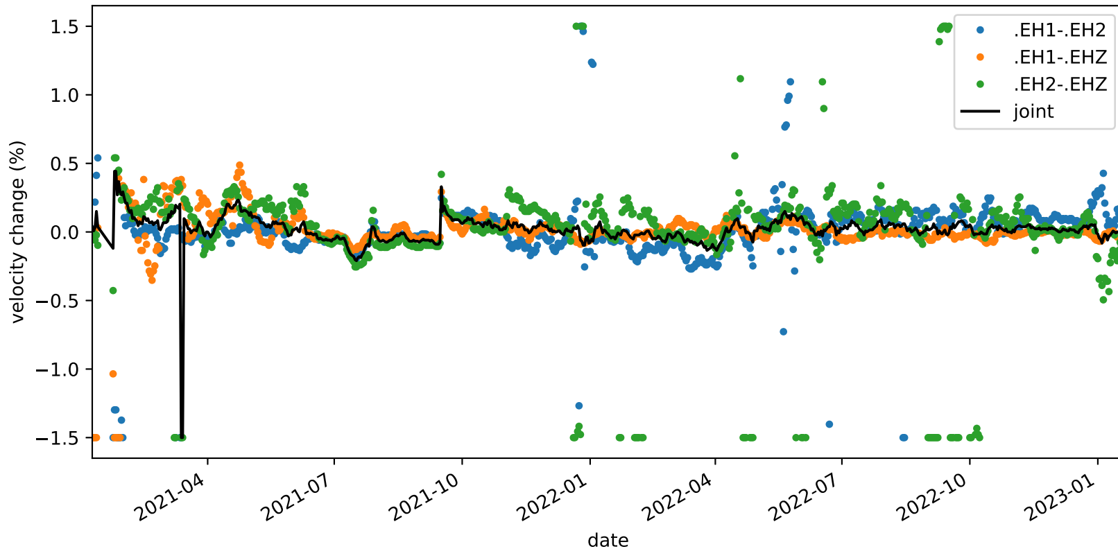
velocity_change_c1c_s3_t1a_tw_005.0s-010.0s_PB.B935-PB.B935
