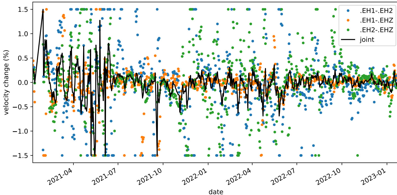
velocity_change_c1b_s4_t1a_tw_005.0s-010.0s_PB.B935-PB.B935
