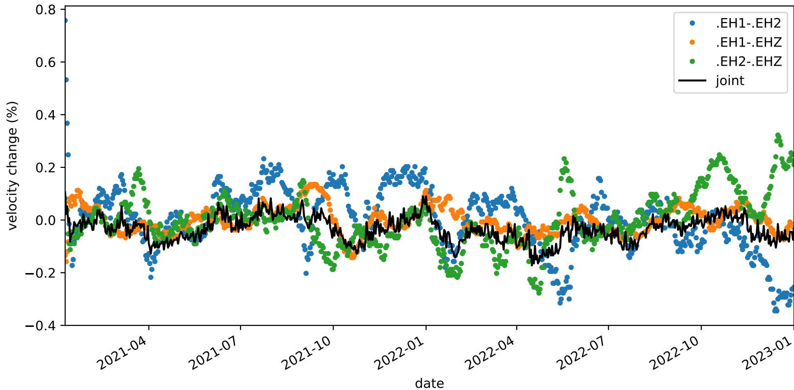
velocity_change_c1f_s2_t1a_tw_005.0s-010.0s_PB.B935-PB.B935
