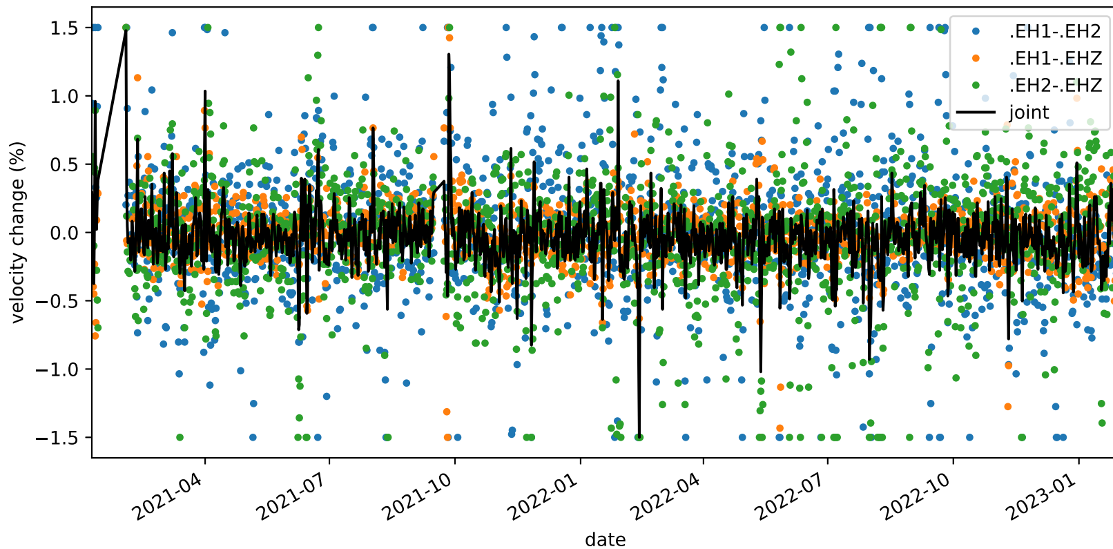
velocity_change_c1f_s1_t1c_tw_005.0s-015.0s_PB.B935-PB.B935
