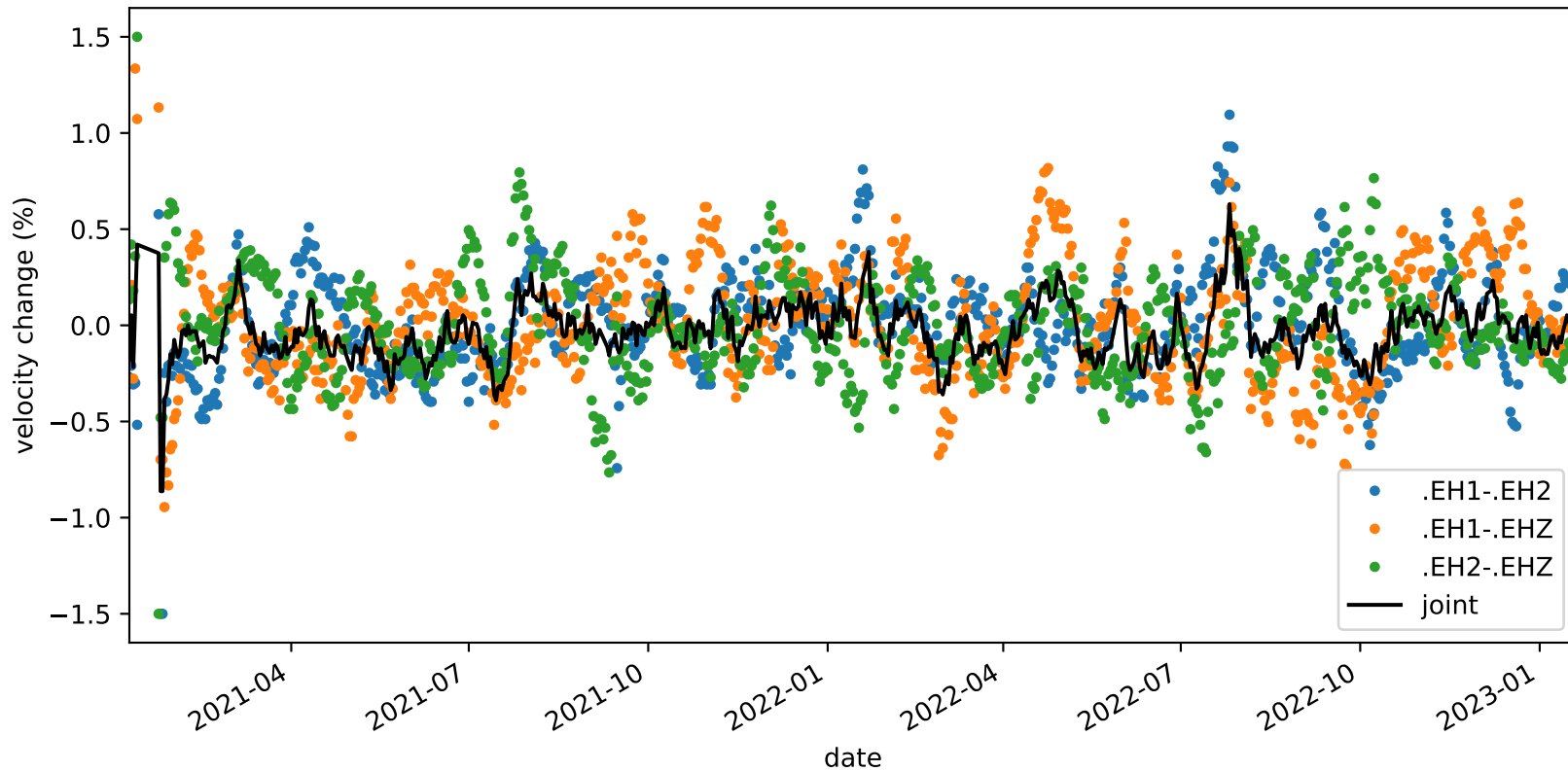
velocity_change_c1d_s3_t1b_tw_010.0s-015.0s_PB.B935-PB.B935
