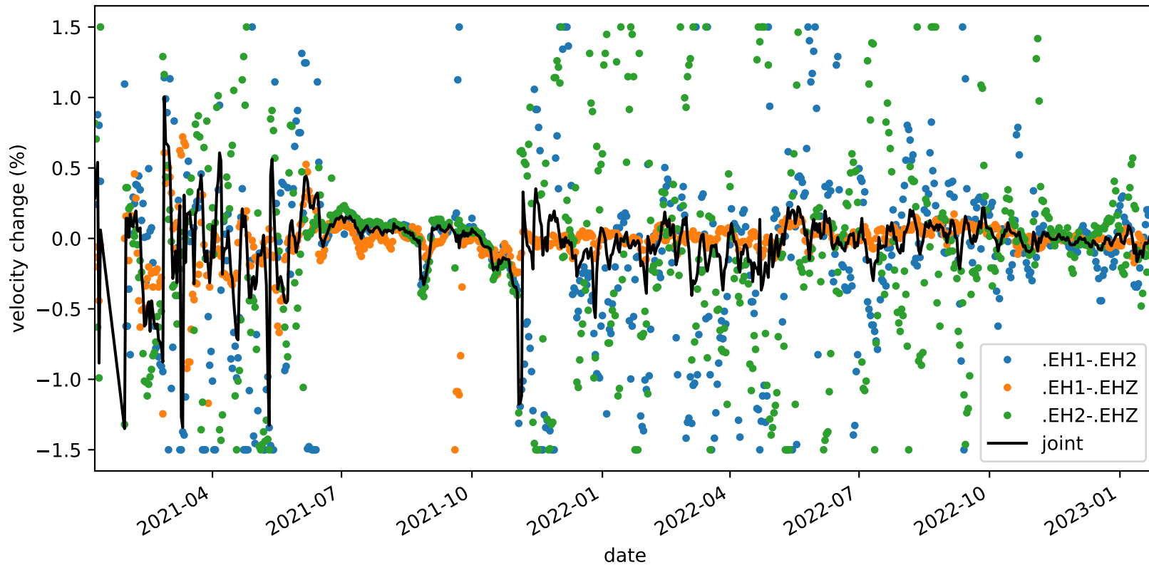
velocity_change_c1h_s4_t1a_tw_005.0s-010.0s_PB.B935-PB.B935
