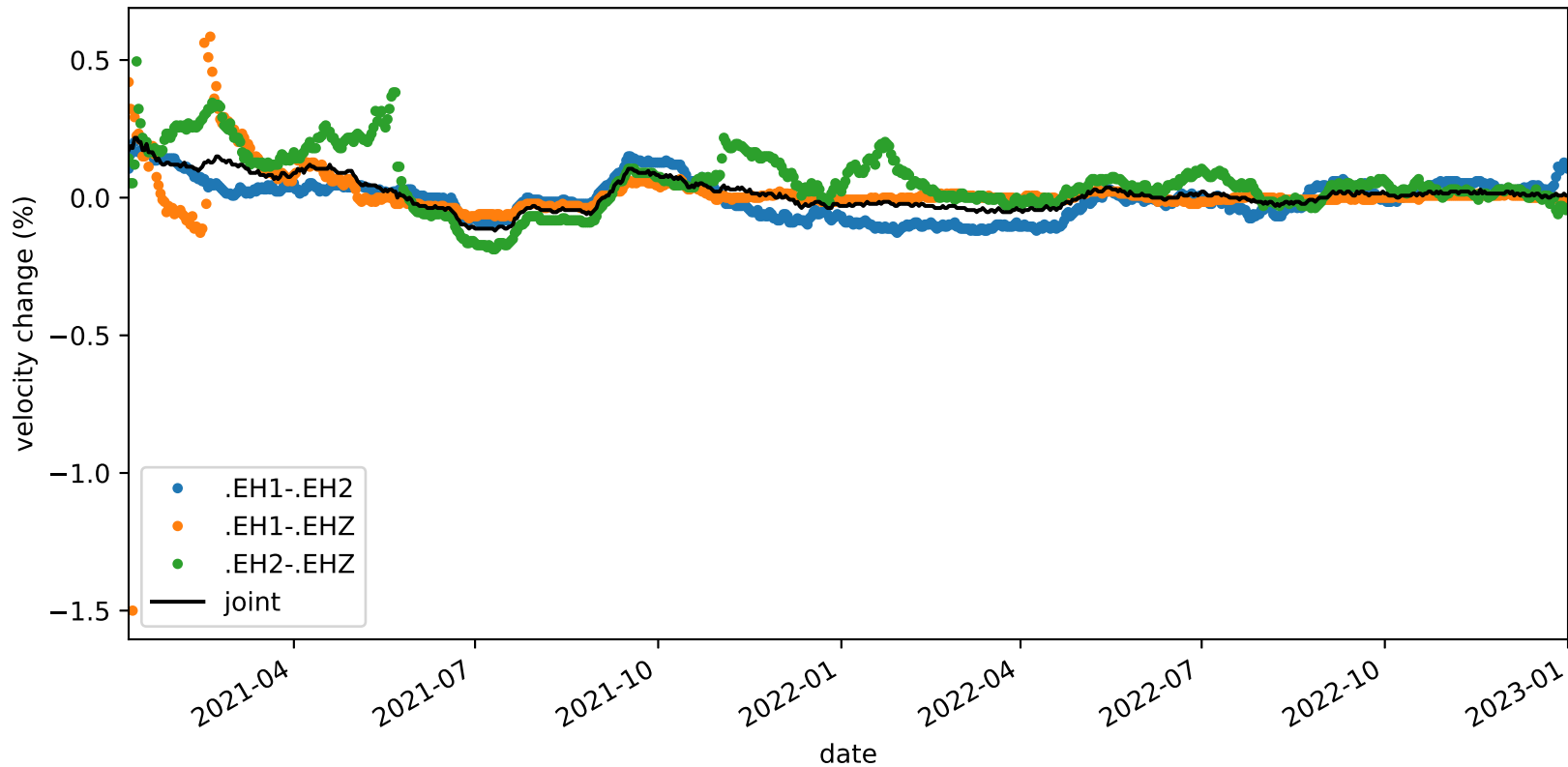
velocity_change_c1c_s2_t1c_tw_005.0s-015.0s_PB.B935-PB.B935
