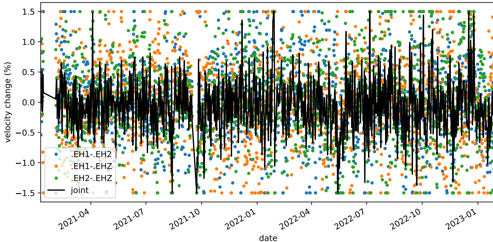
velocity_change_c1d_s1_t1a_tw_005.0s-010.0s_PB.B935-PB.B935
