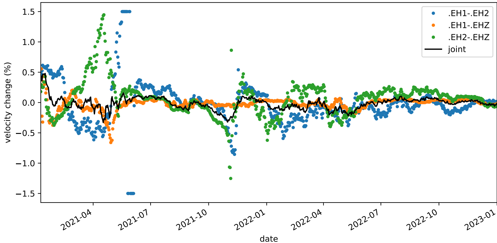
velocity_change_c1b_s2_t1a_tw_005.0s-010.0s_PB.B935-PB.B935
