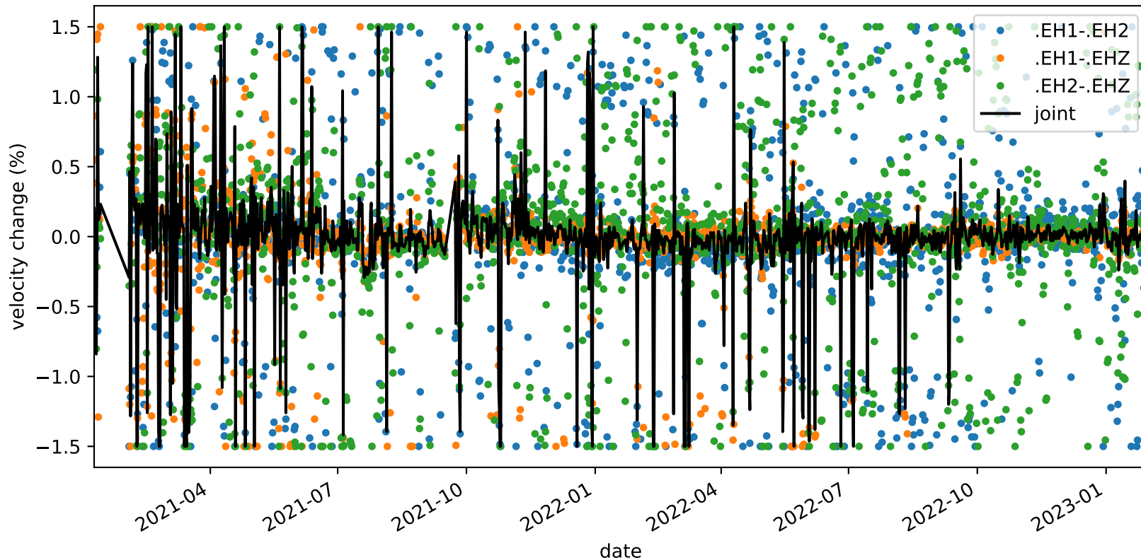
velocity_change_c1c_s1_t1c_tw_005.0s-015.0s_PB.B935-PB.B935
