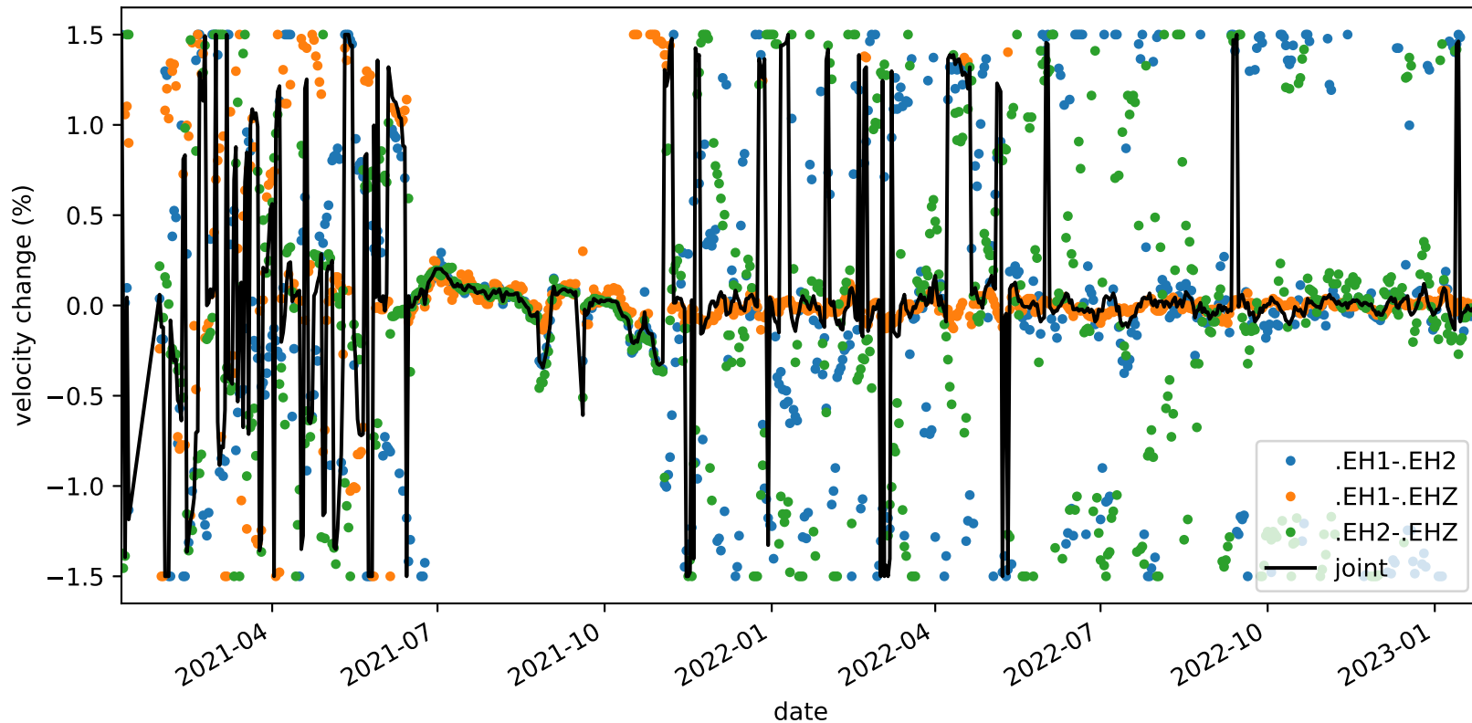
velocity_change_c1_s4_t1b_tw_010.0s-015.0s_PB.B935-PB.B935
