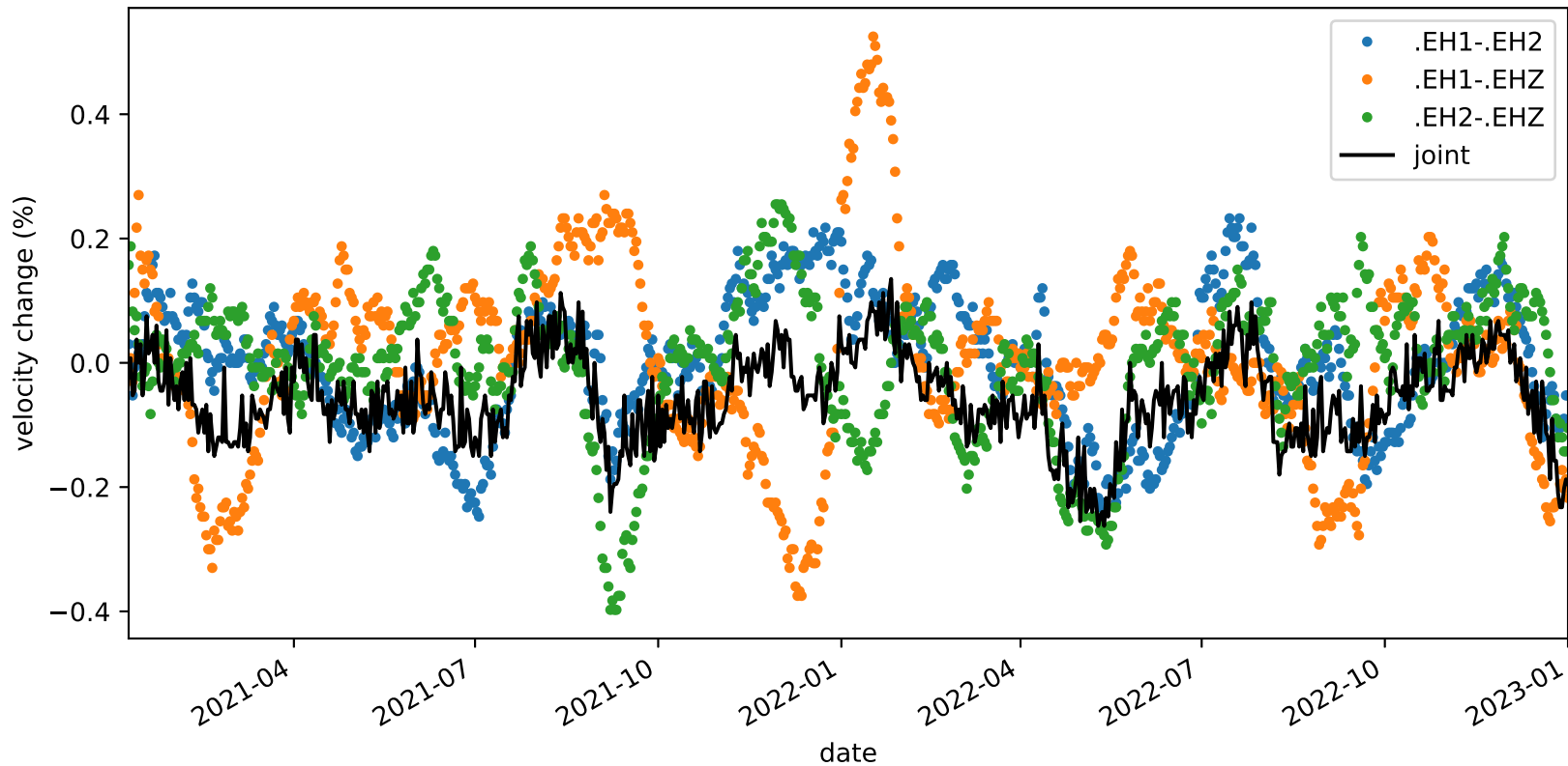
velocity_change_c1d_s2_t1c_tw_005.0s-015.0s_PB.B935-PB.B935
