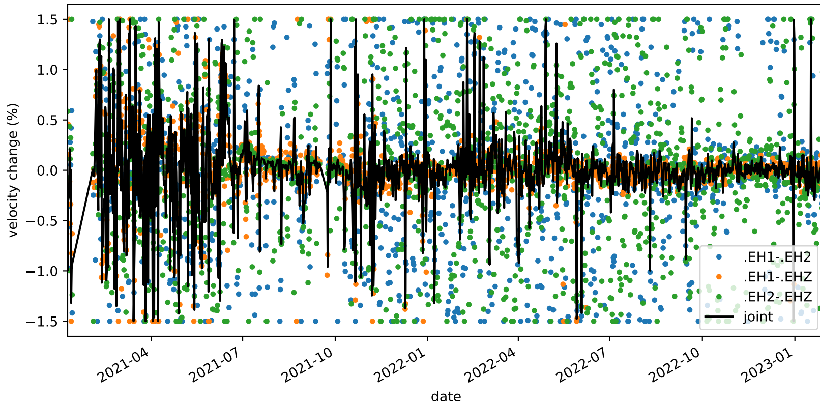
velocity_change_c1h_s1_t1b_tw_010.0s-015.0s_PB.B935-PB.B935
