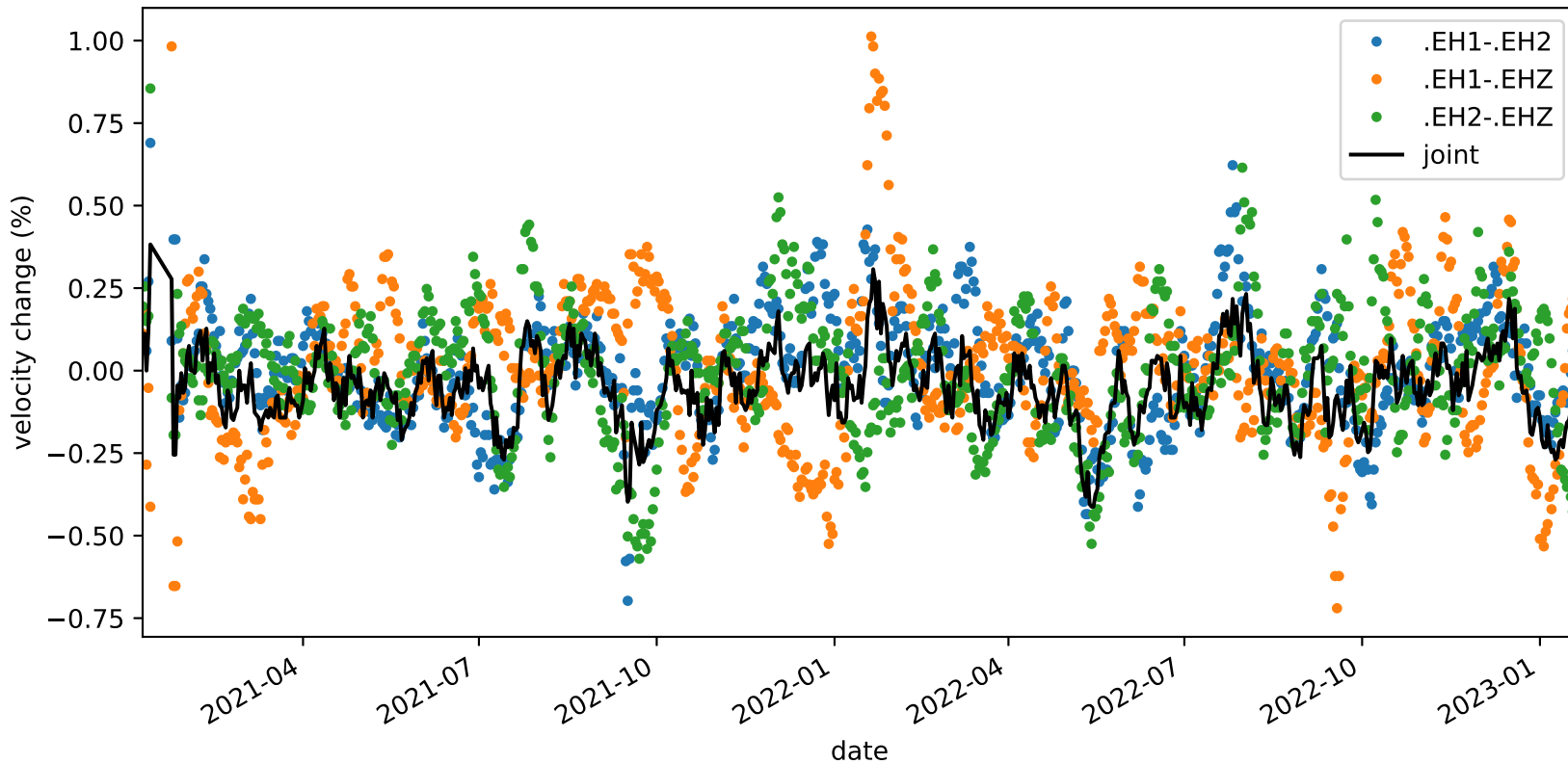
velocity_change_c1d_s3_t1c_tw_005.0s-015.0s_PB.B935-PB.B935
