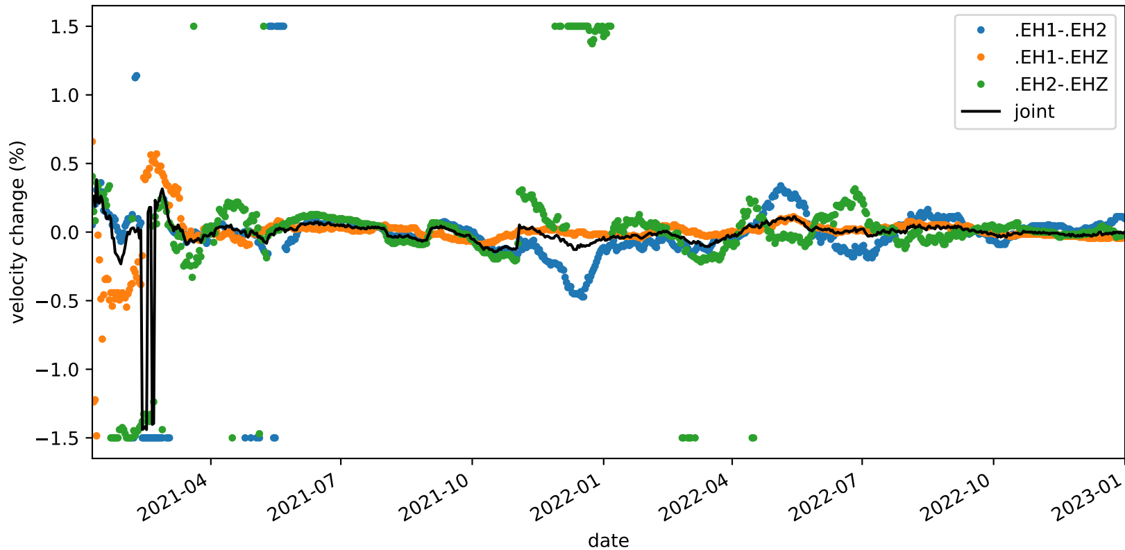
velocity_change_c1i_s2_t1a_tw_005.0s-010.0s_PB.B935-PB.B935
