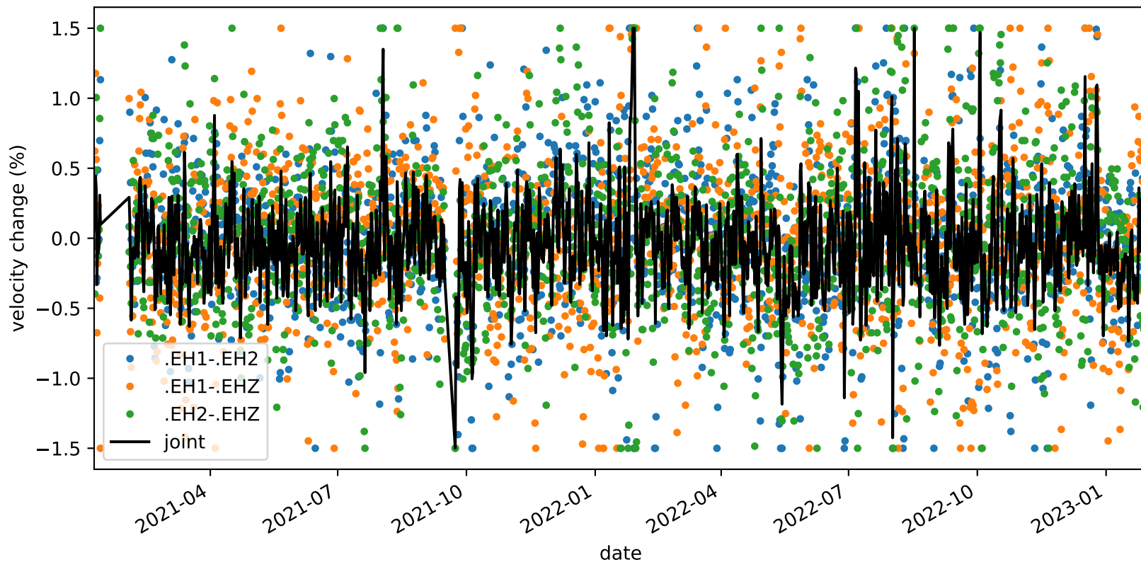
velocity_change_c1d_s1_t1c_tw_005.0s-015.0s_PB.B935-PB.B935
