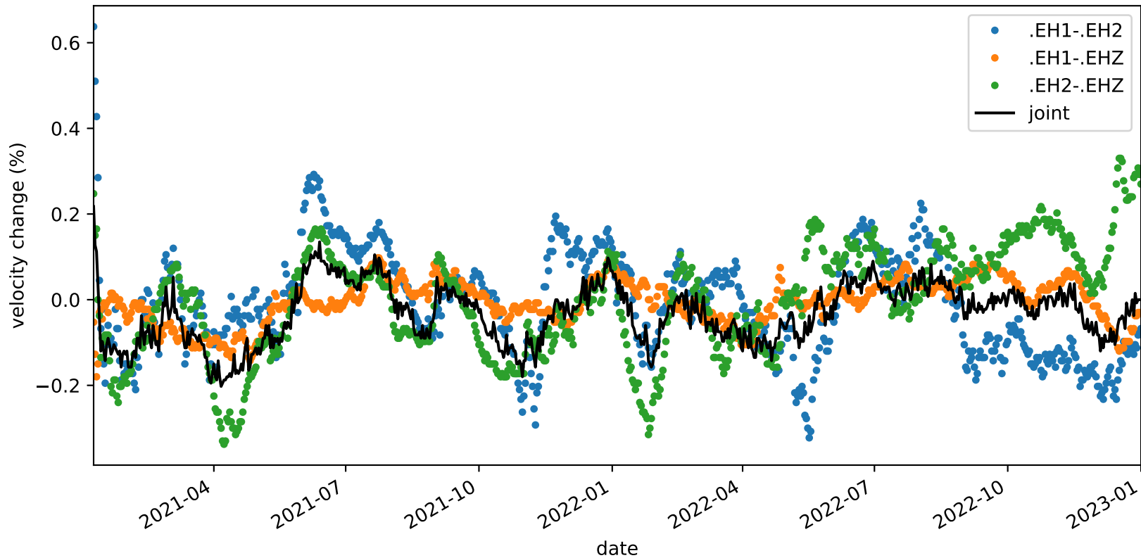
velocity_change_c1g_s2_t1a_tw_005.0s-010.0s_PB.B935-PB.B935
