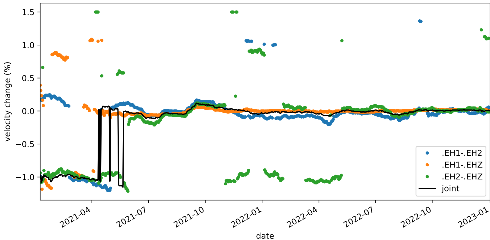
velocity_change_c1c_s2_t1b_tw_010.0s-015.0s_PB.B935-PB.B935
