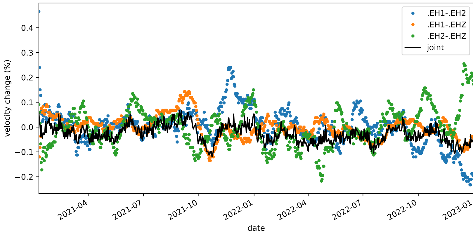
velocity_change_c1f_s2_t1c_tw_005.0s-015.0s_PB.B935-PB.B935
