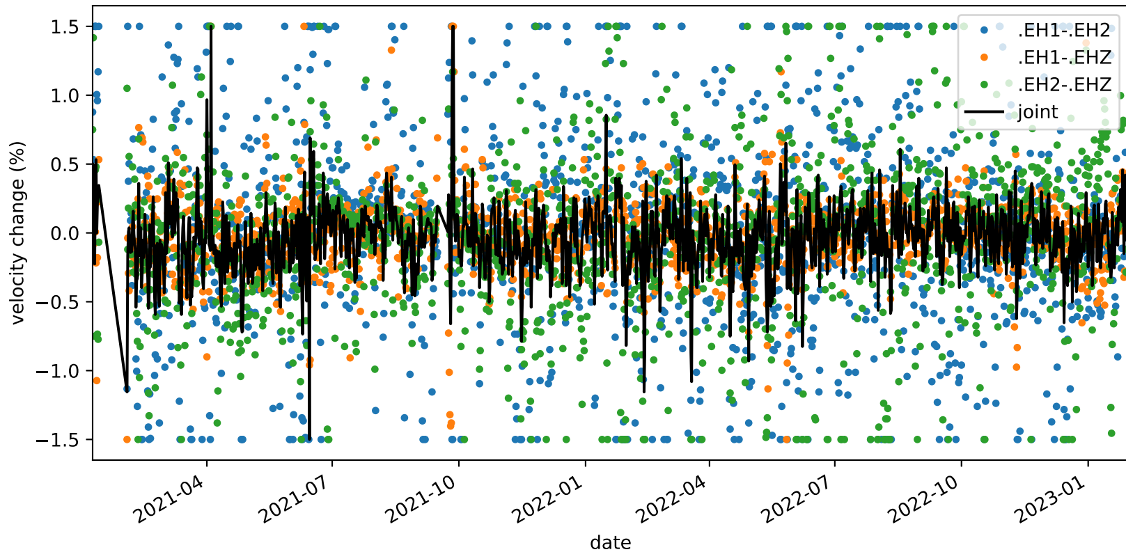
velocity_change_c1g_s1_t1a_tw_005.0s-010.0s_PB.B935-PB.B935
