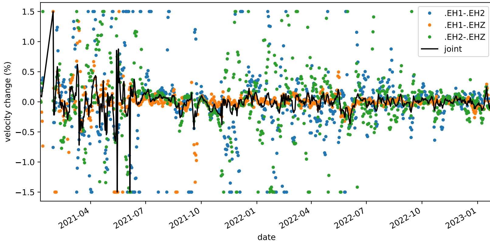
velocity_change_c1b_s4_t1c_tw_005.0s-015.0s_PB.B935-PB.B935
