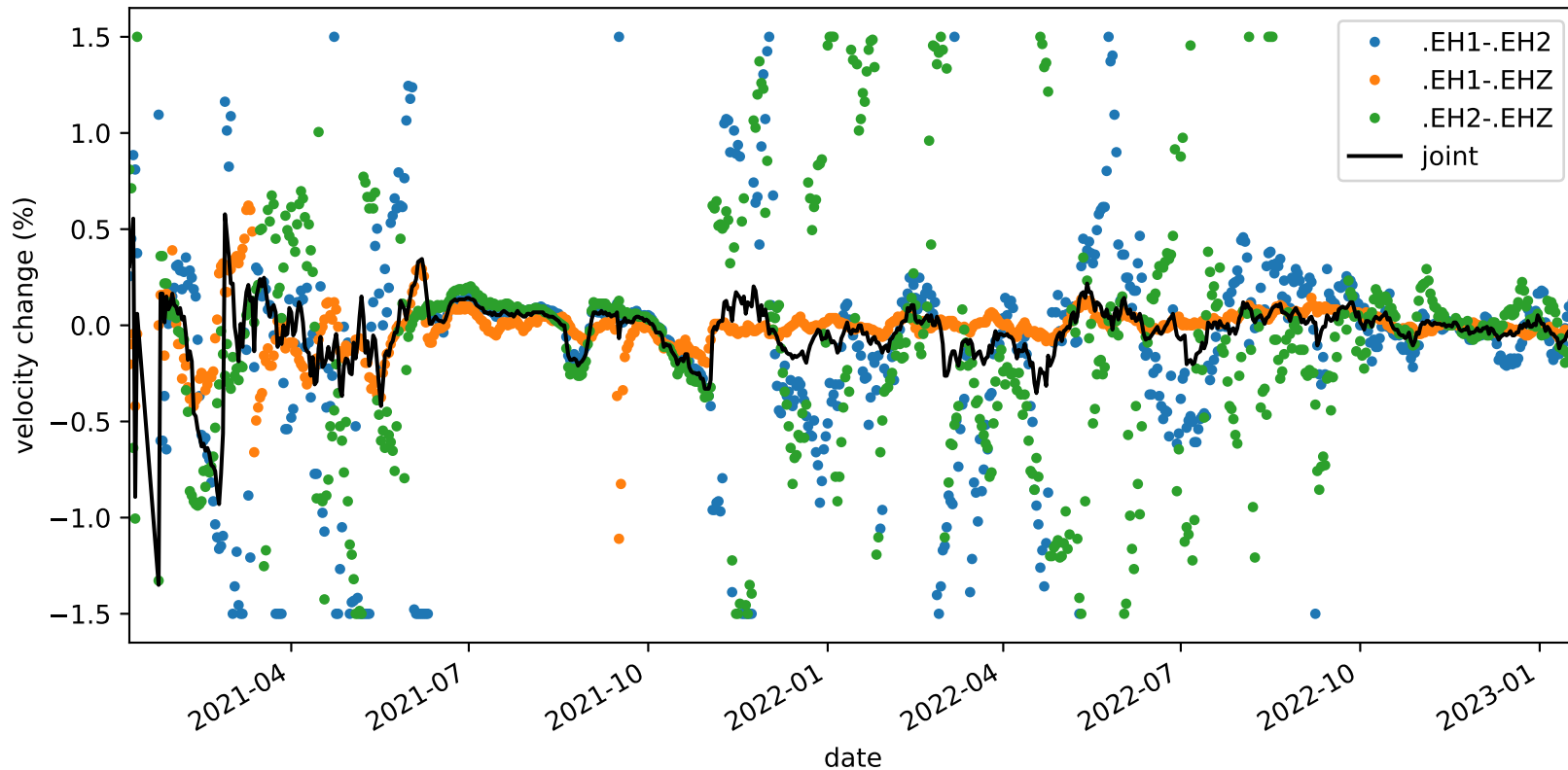
velocity_change_c1h_s3_t1a_tw_005.0s-010.0s_PB.B935-PB.B935
