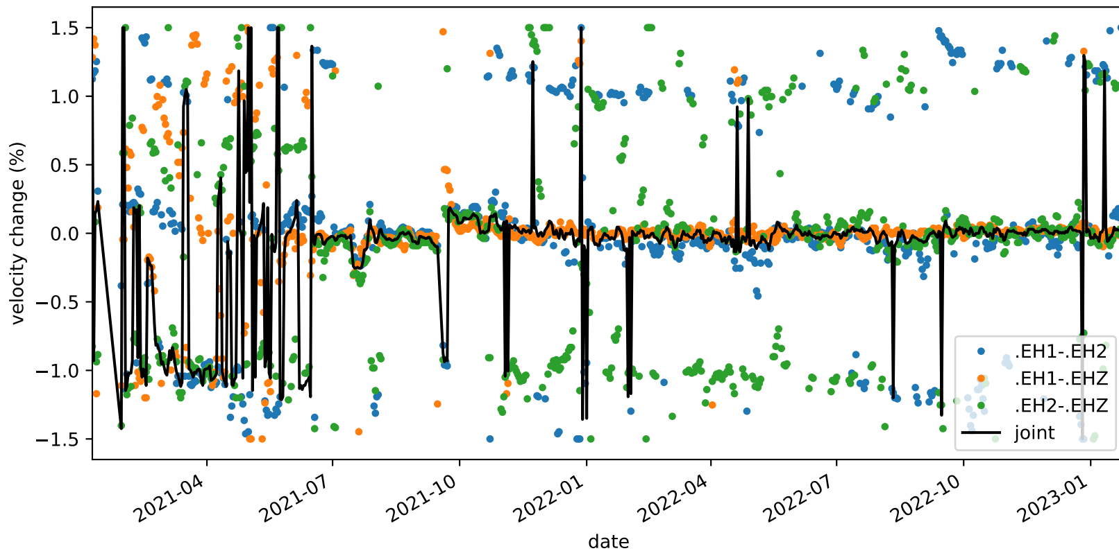
velocity_change_c1c_s4_t1b_tw_010.0s-015.0s_PB.B935-PB.B935
