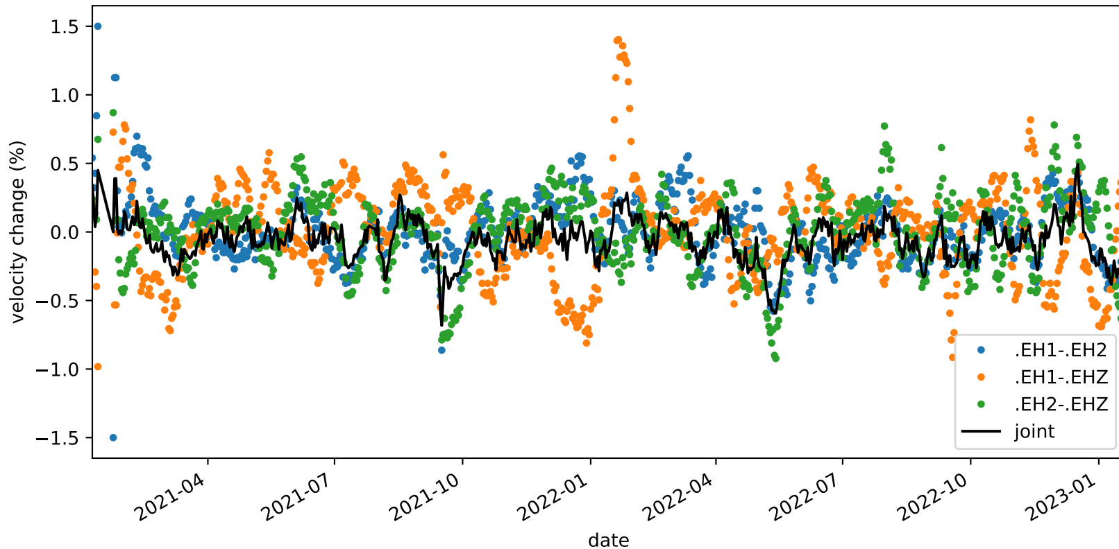
velocity_change_c1d_s3_t1a_tw_005.0s-010.0s_PB.B935-PB.B935
