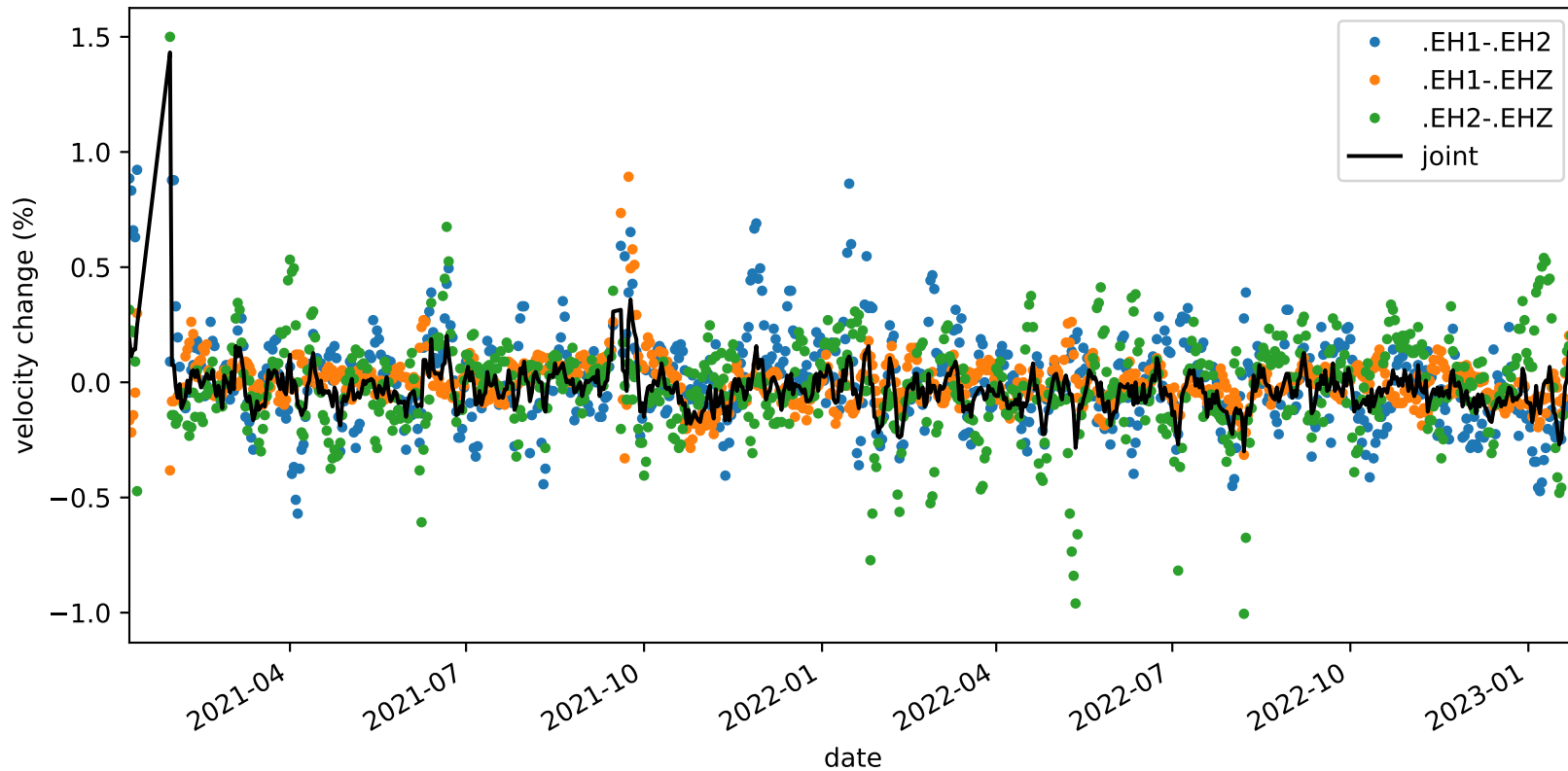
velocity_change_c1f_s4_t1c_tw_005.0s-015.0s_PB.B935-PB.B935
