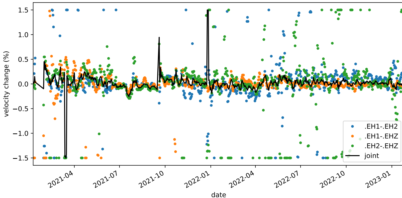
velocity_change_c1c_s4_t1a_tw_005.0s-010.0s_PB.B935-PB.B935
