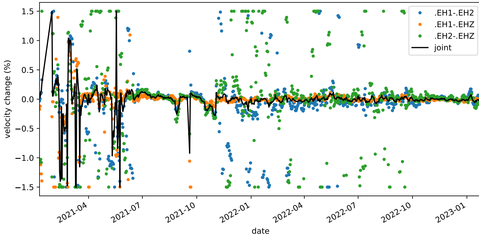
velocity_change_cli_s4_t1c_tw_005.0s-015.0s_PB.B935-PB.B935
