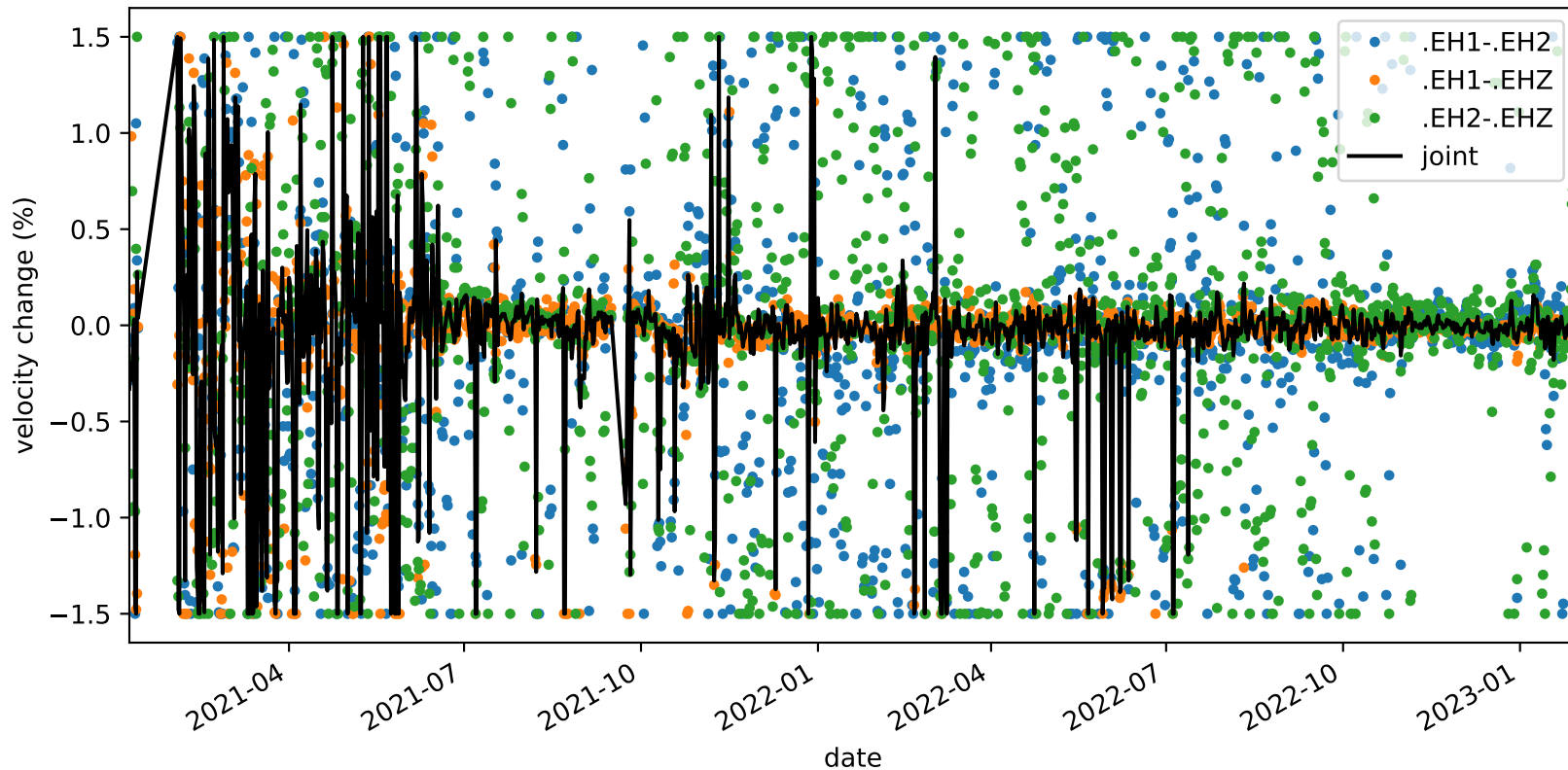
velocity_change_cli_s1_t1c_tw_005.0s-015.0s_PB.B935-PB.B935
