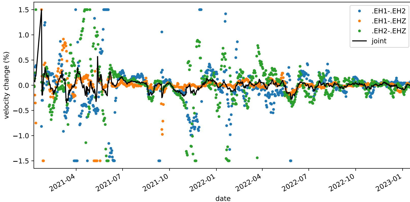
velocity_change_c1b_s3_t1c_tw_005.0s-015.0s_PB.B935-PB.B935
