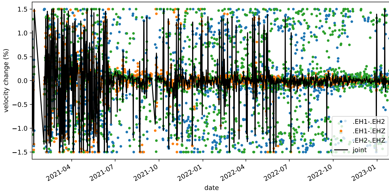
velocity_change_cli_s1_t1b_tw_010.0s-015.0s_PB.B935-PB.B935
