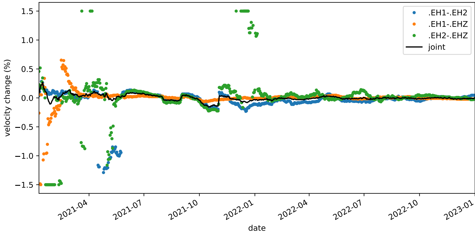
velocity_change_c1i_s2_t1c_tw_005.0s-015.0s_PB.B935-PB.B935
