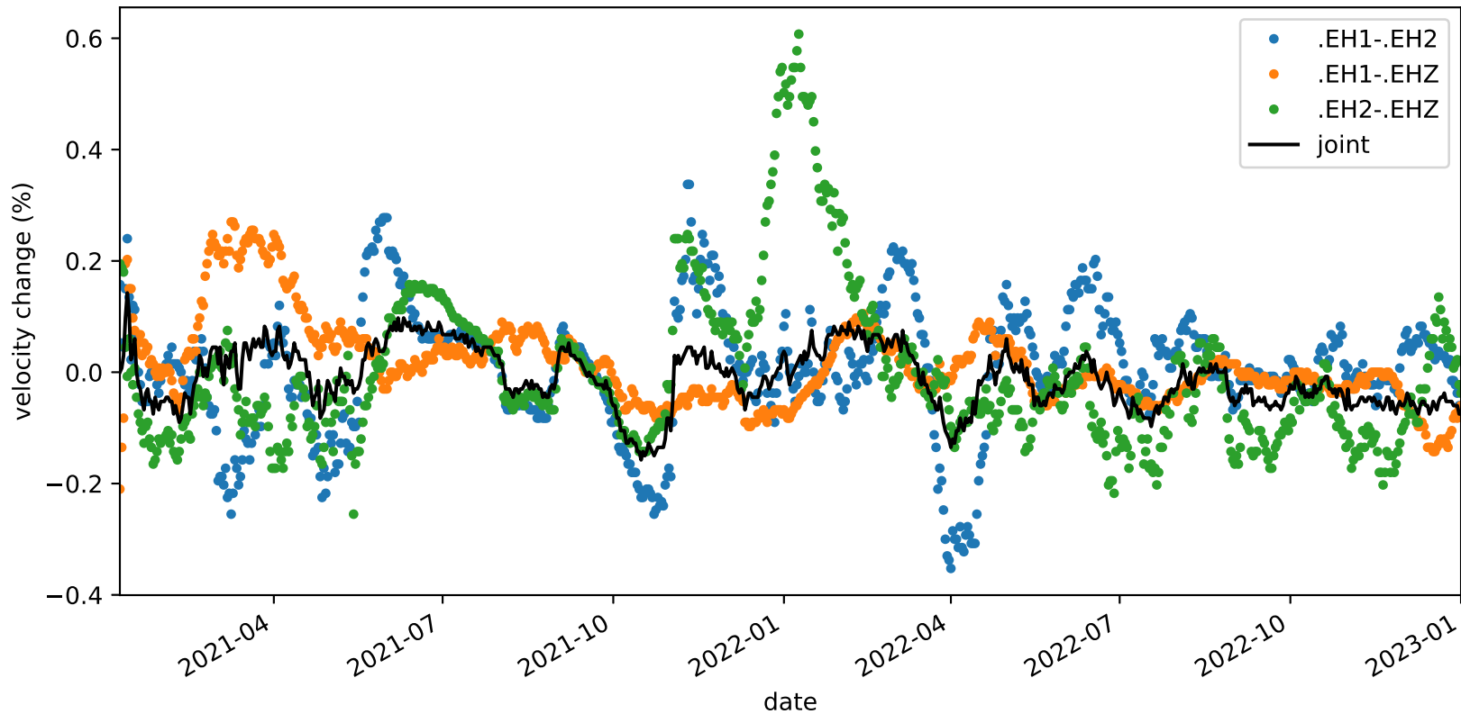
velocity_change_c1g_s2_t1b_tw_010.0s-015.0s_PB.B935-PB.B935
