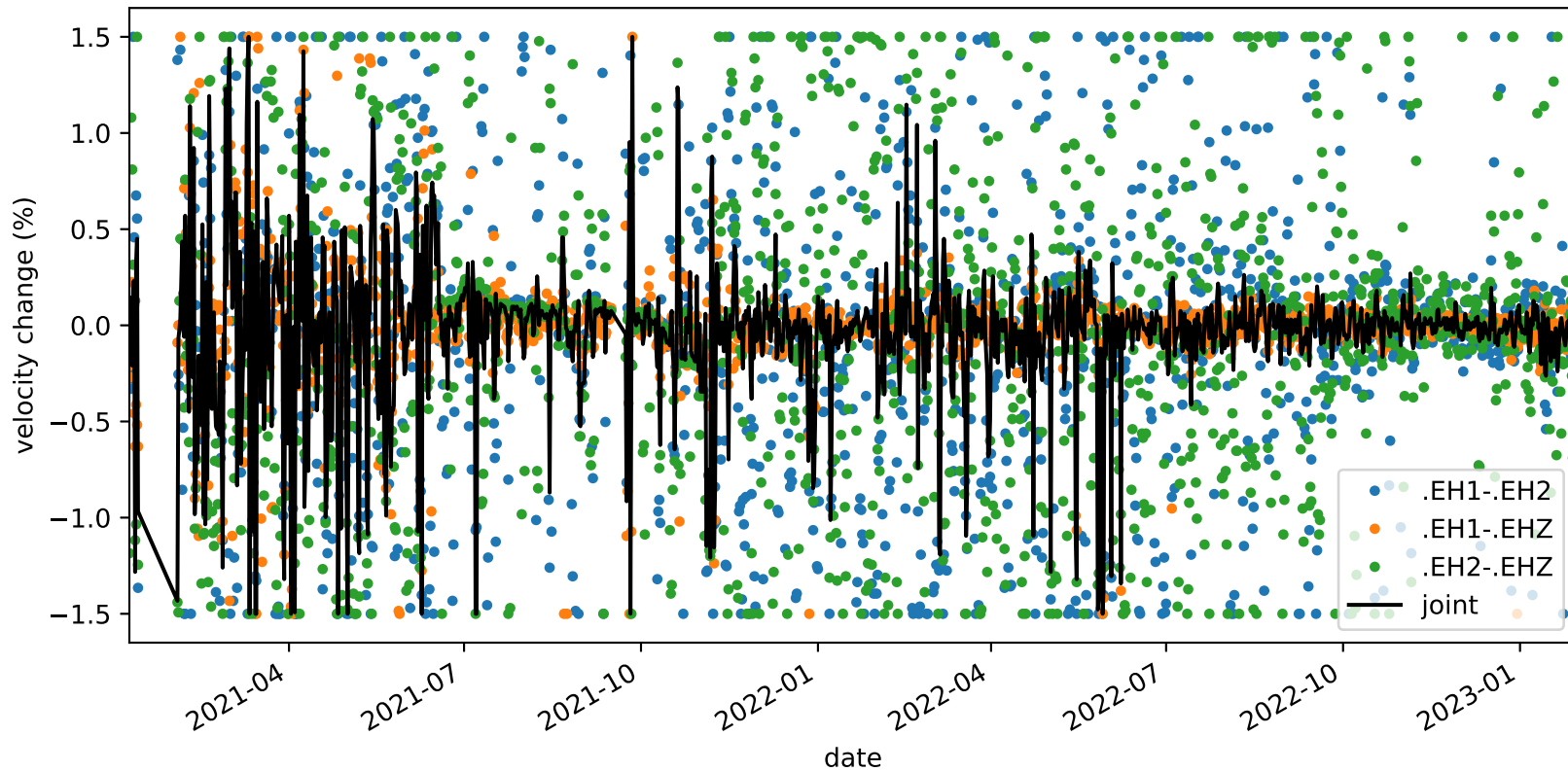
velocity_change_c1h_s1_t1c_tw_005.0s-015.0s_PB.B935-PB.B935
