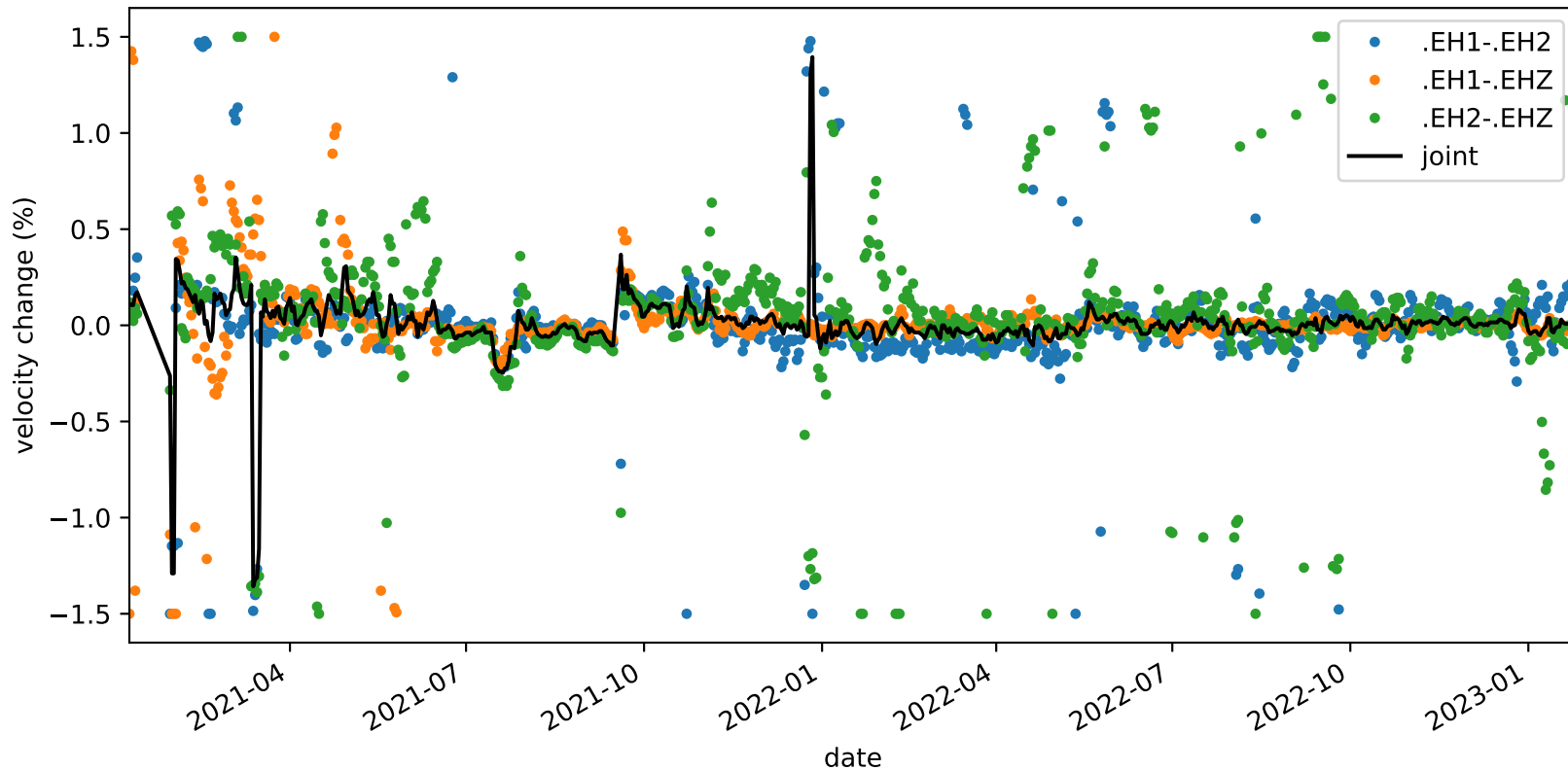
velocity_change_c1c_s4_t1c_tw_005.0s-015.0s_PB.B935-PB.B935
