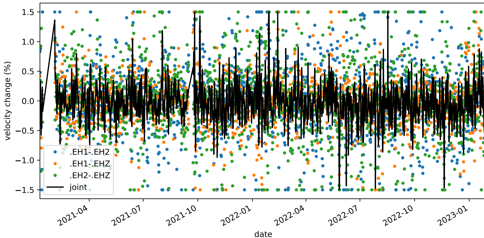
velocity_change_c1e_s1_t1b_tw_010.0s-015.0s_PB.B935-PB.B935
