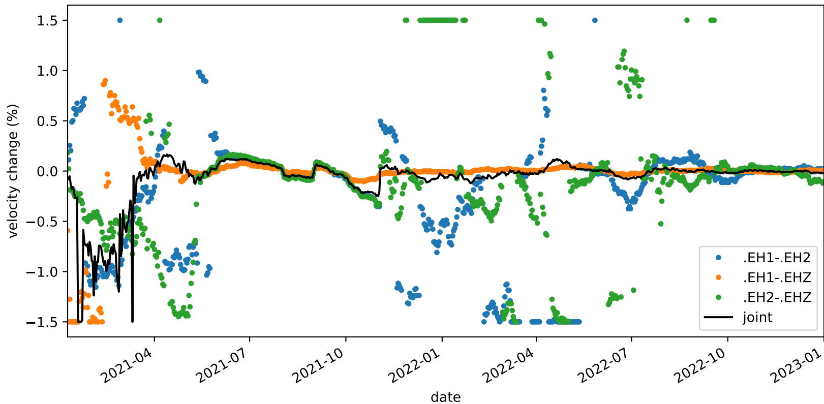
velocity_change_c1_s2_t1c_tw_005.0s-015.0s_PB.B935-PB.B935
