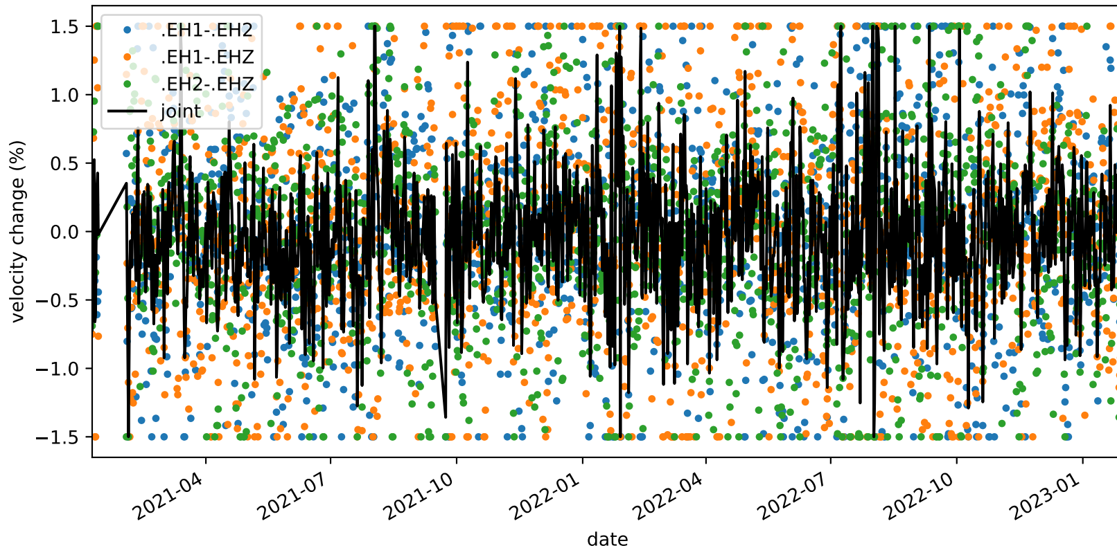
velocity_change_c1d_s1_t1b_tw_010.0s-015.0s_PB.B935-PB.B935
