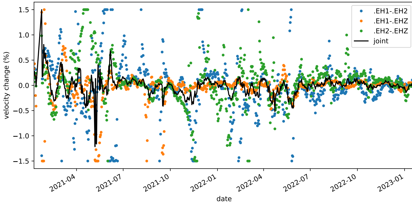
velocity_change_c1b_s3_t1a_tw_005.0s-010.0s_PB.B935-PB.B935
