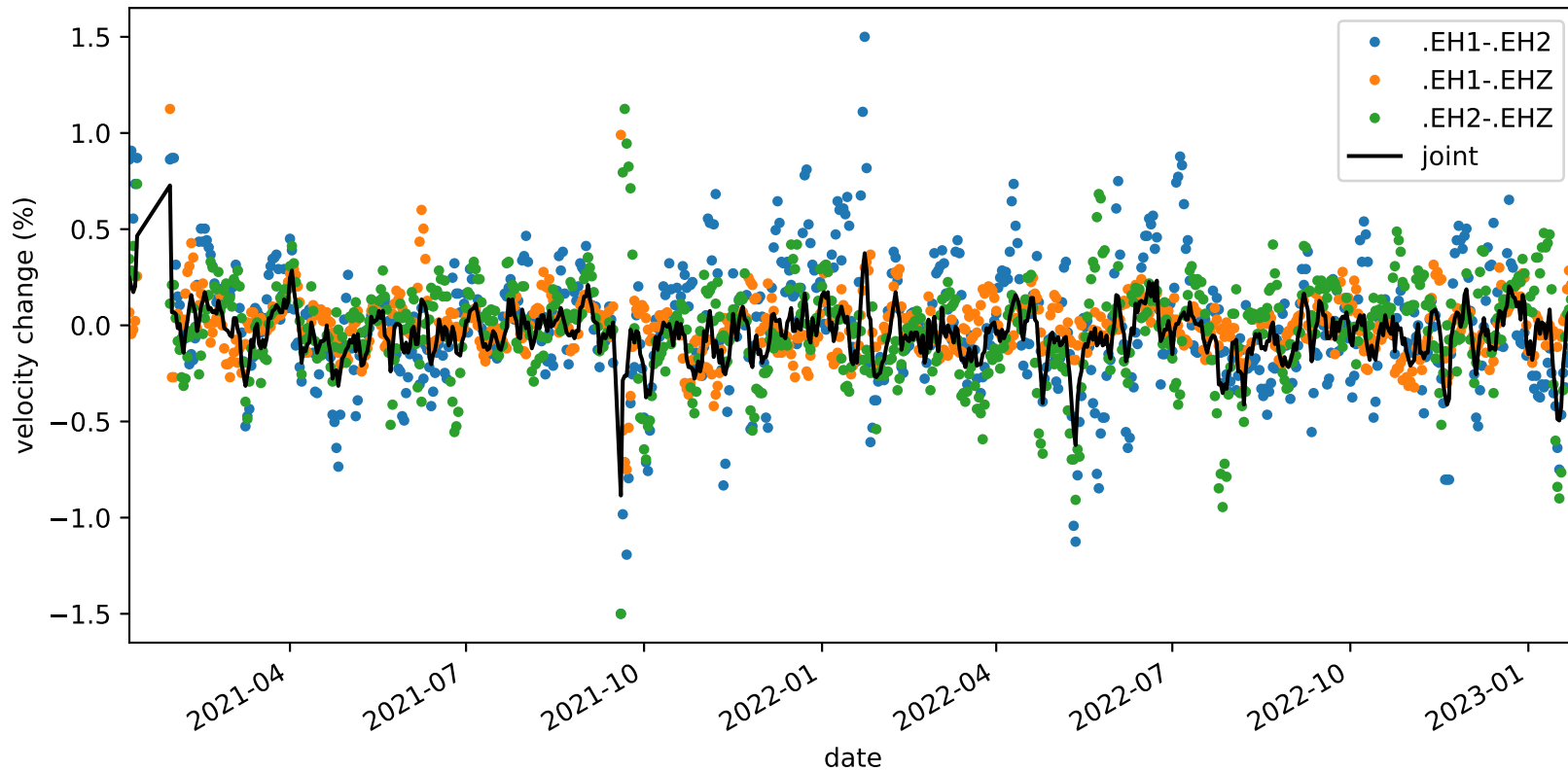
velocity_change_c1e_s4_t1a_tw_005.0s-010.0s_PB.B935-PB.B935
