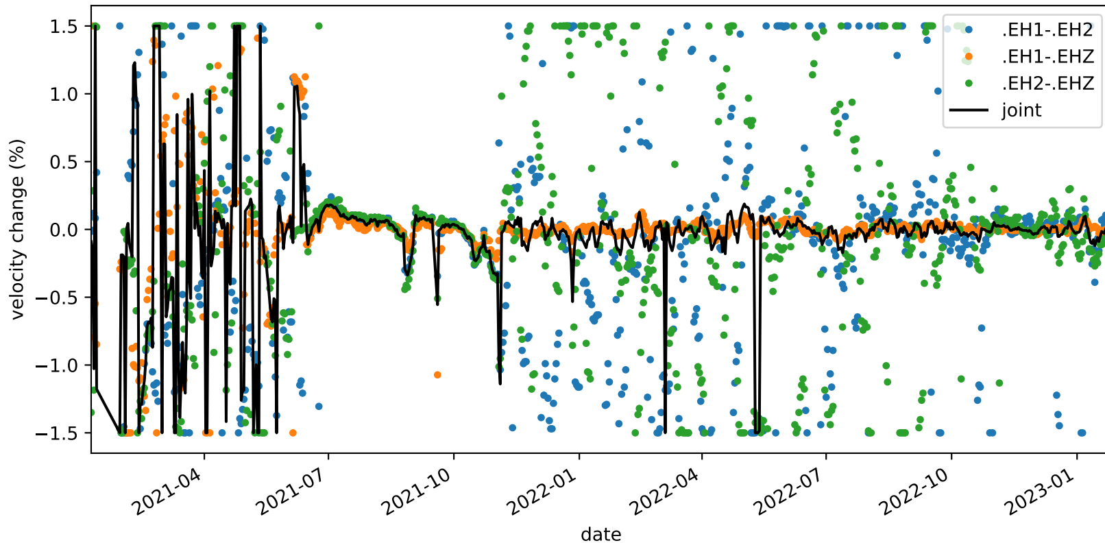
velocity_change_c1_s4_t1c_tw_005.0s-015.0s_PB.B935-PB.B935
