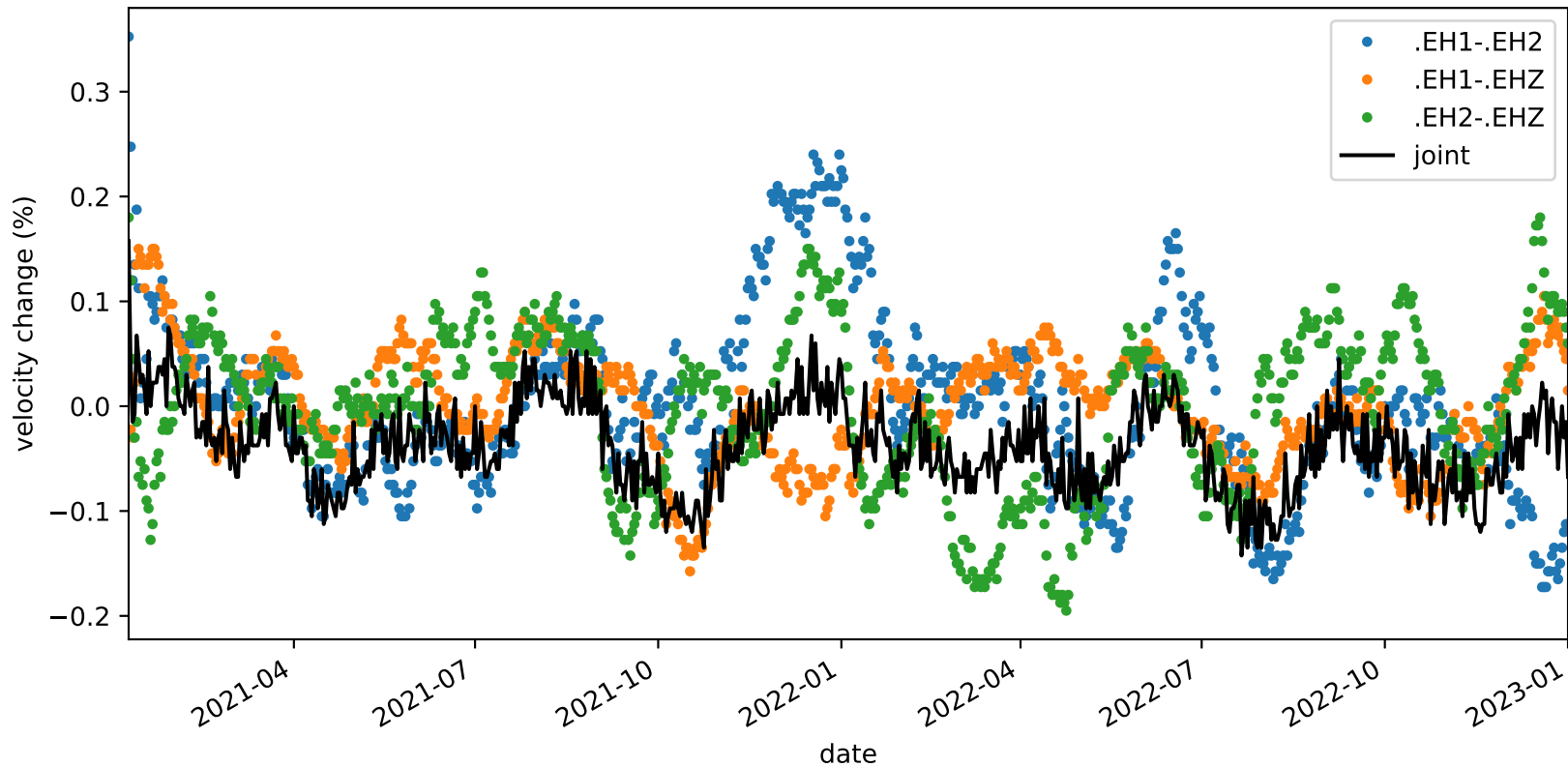
velocity_change_c1e_s2_t1c_tw_005.0s-015.0s_PB.B935-PB.B935
