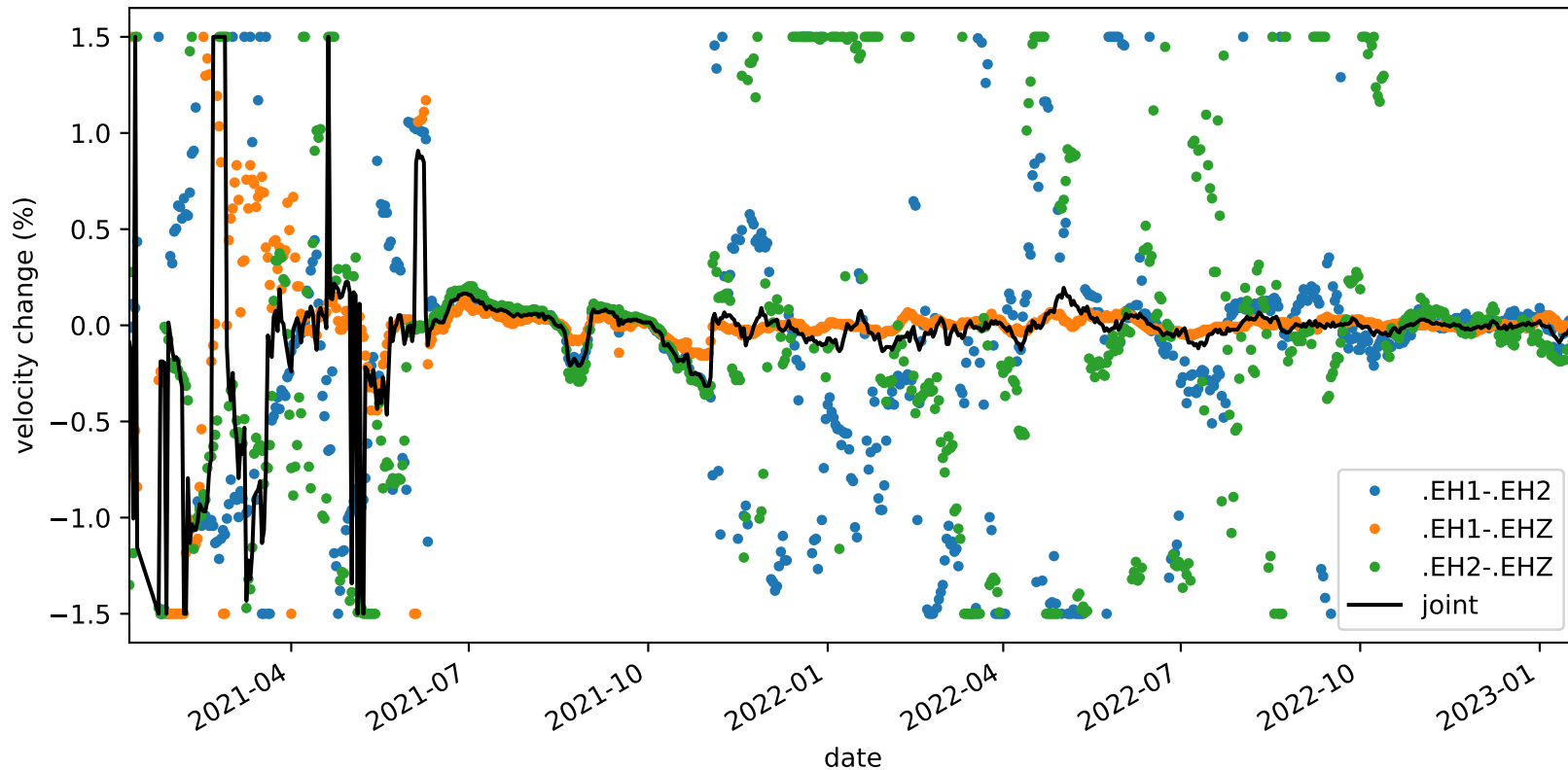
velocity_change_c1_s3_t1c_tw_005.0s-015.0s_PB.B935-PB.B935
