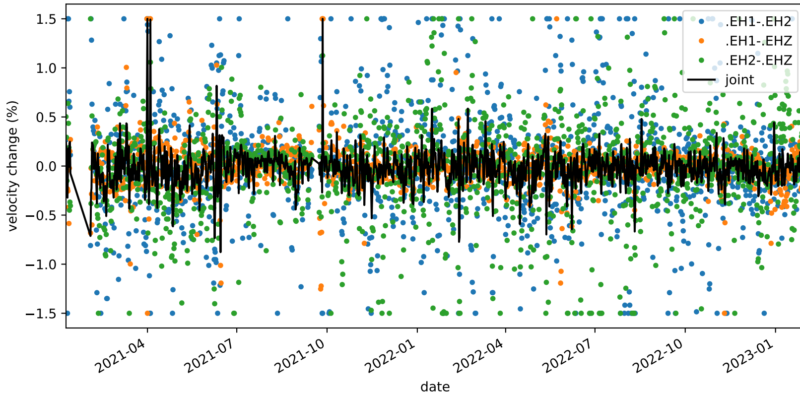
velocity_change_c1g_s1_t1c_tw_005.0s-015.0s_PB.B935-PB.B935
