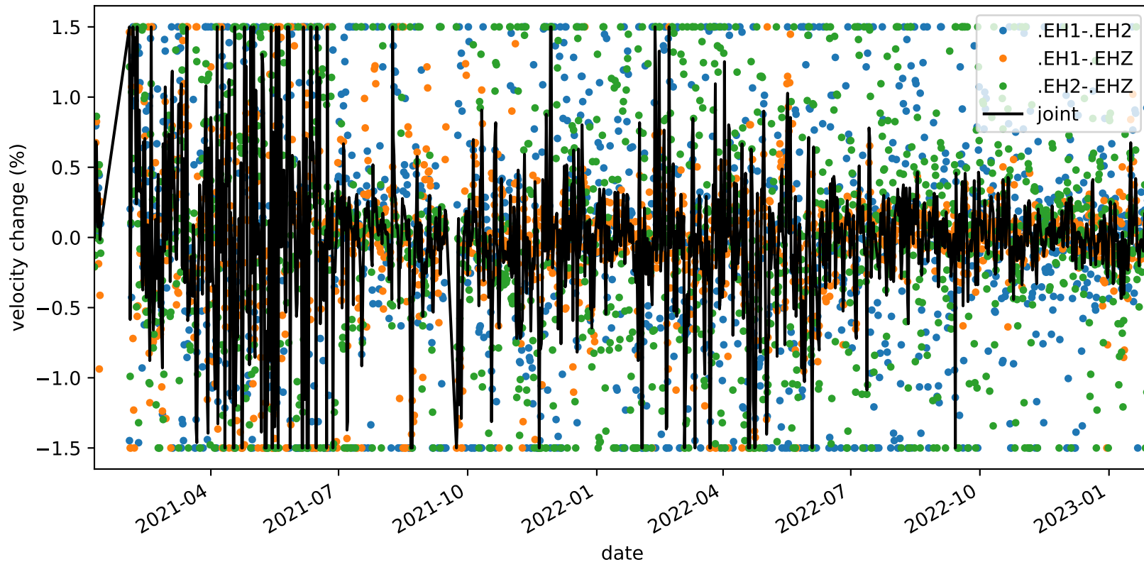
velocity_change_c1b_s1_t1a_tw_005.0s-010.0s_PB.B935-PB.B935
