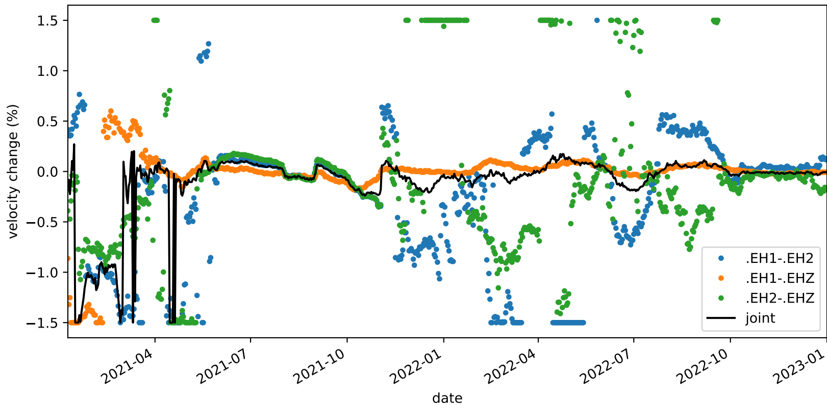
velocity_change_c1_s2_t1a_tw_005.0s-010.0s_PB.B935-PB.B935
