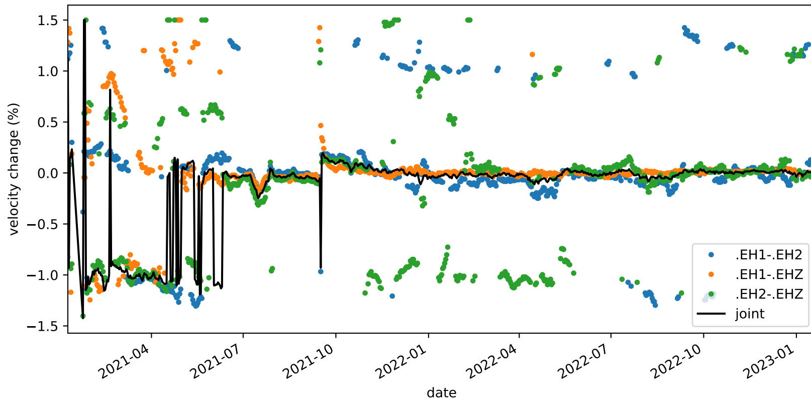
velocity_change_c1c_s3_t1b_tw_010.0s-015.0s_PB.B935-PB.B935
