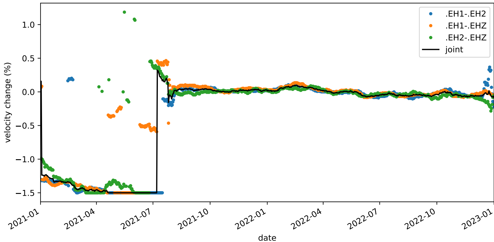
velocity_change_c1c_s2_t1c_tw_005.0s-015.0s_PB.B932-PB.B932
