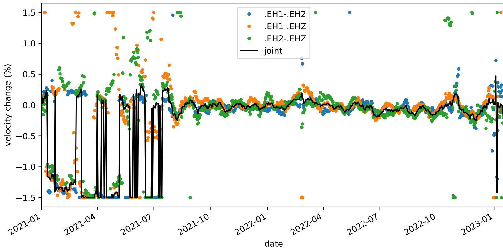
velocity_change_c1c_s3_t1a_tw_005.0s-010.0s_PB.B932-PB.B932
