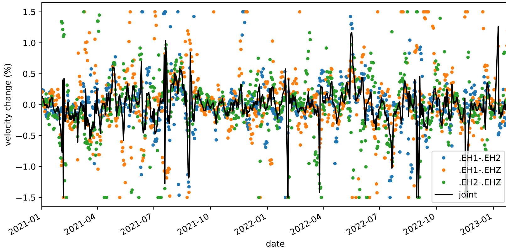
velocity_change_c1_s4_t1a_tw_005.0s-010.0s_PB.B932-PB.B932
