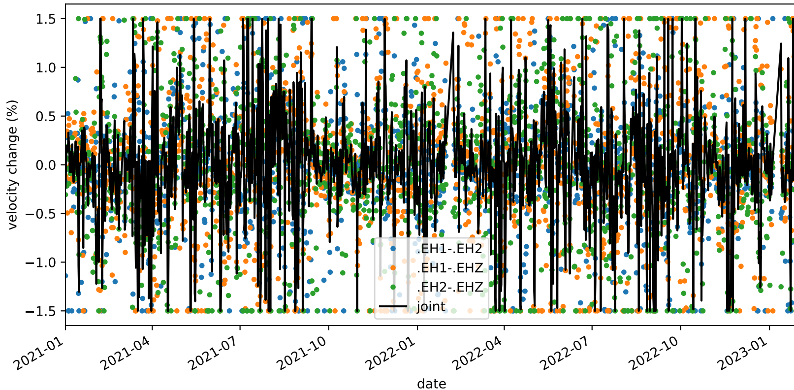
velocity_change_c1_s1_t1a_tw_005.0s-010.0s_PB.B932-PB.B932
