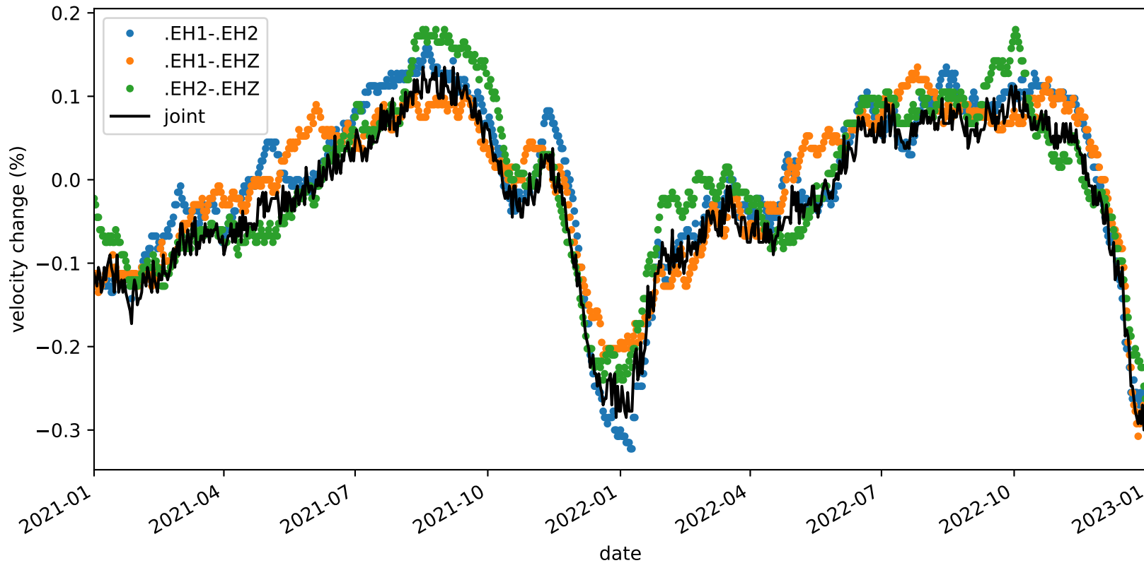
velocity_change_c1g_s2_t1c_tw_005.0s-015.0s_PB.B932-PB.B932
