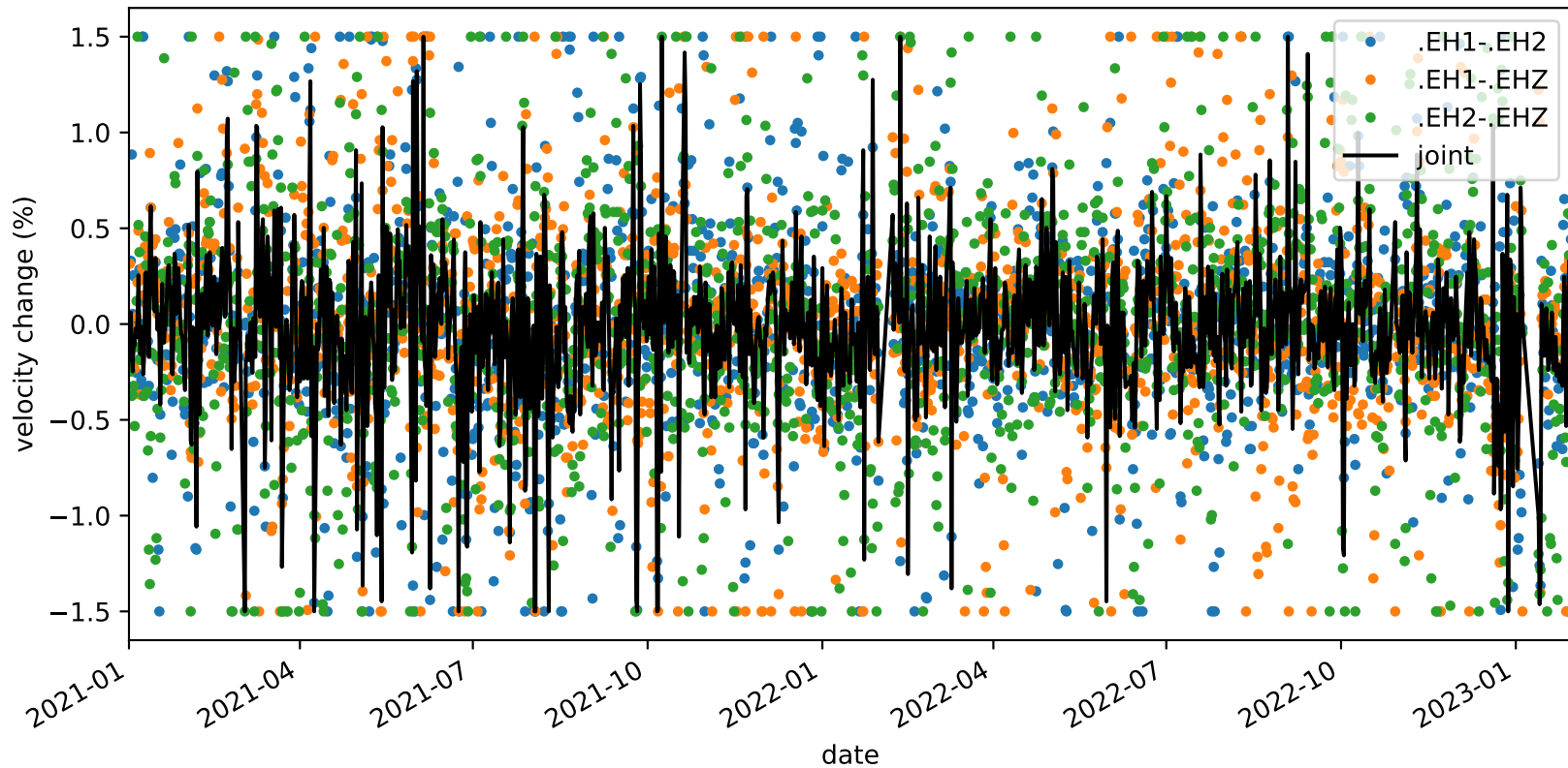
velocity_change_c1b_s1_t1b_tw_010.0s-015.0s_PB.B932-PB.B932
