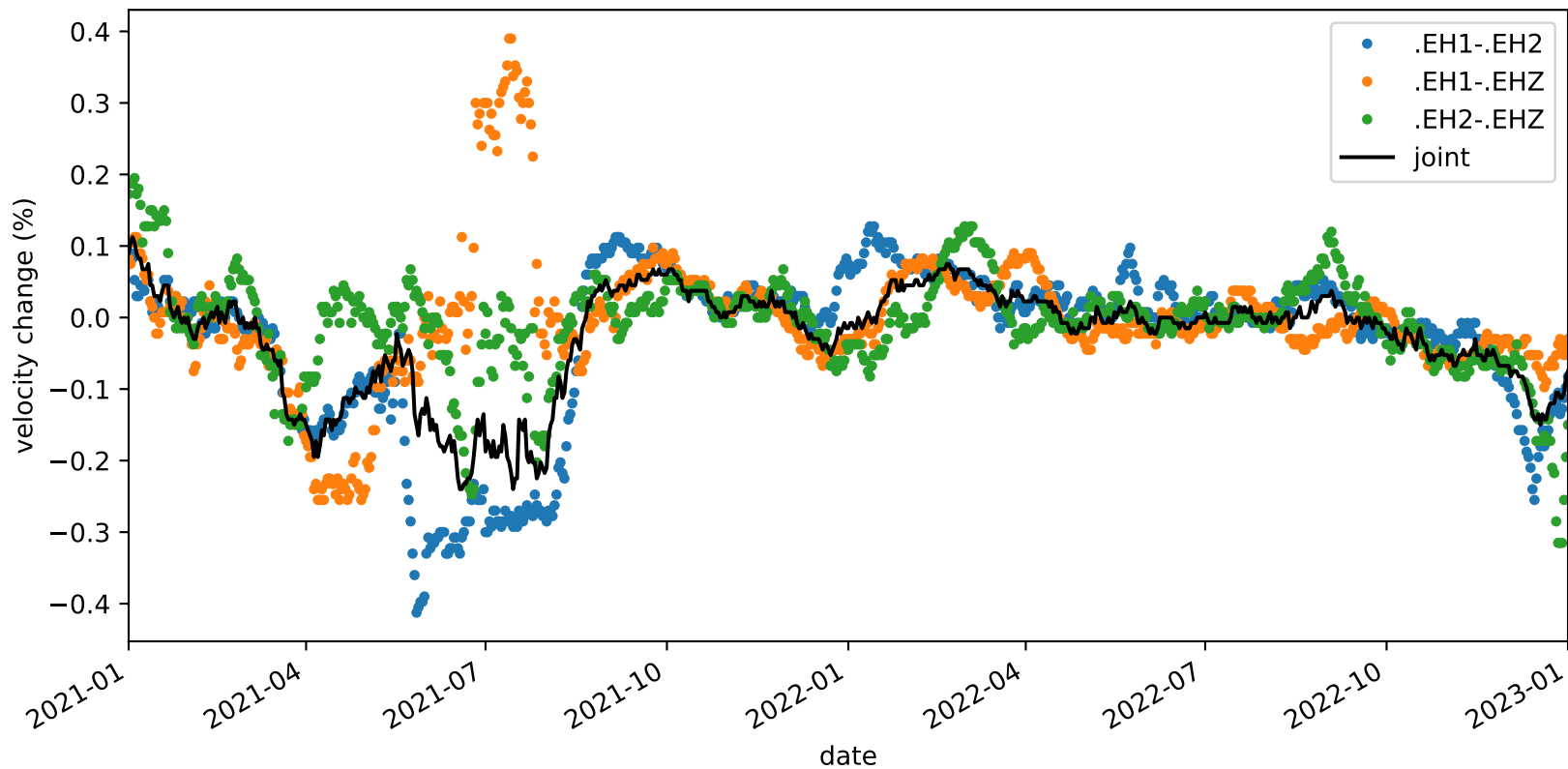
velocity_change_c1i_s2_t1b_tw_010.0s-015.0s_PB.B932-PB.B932
