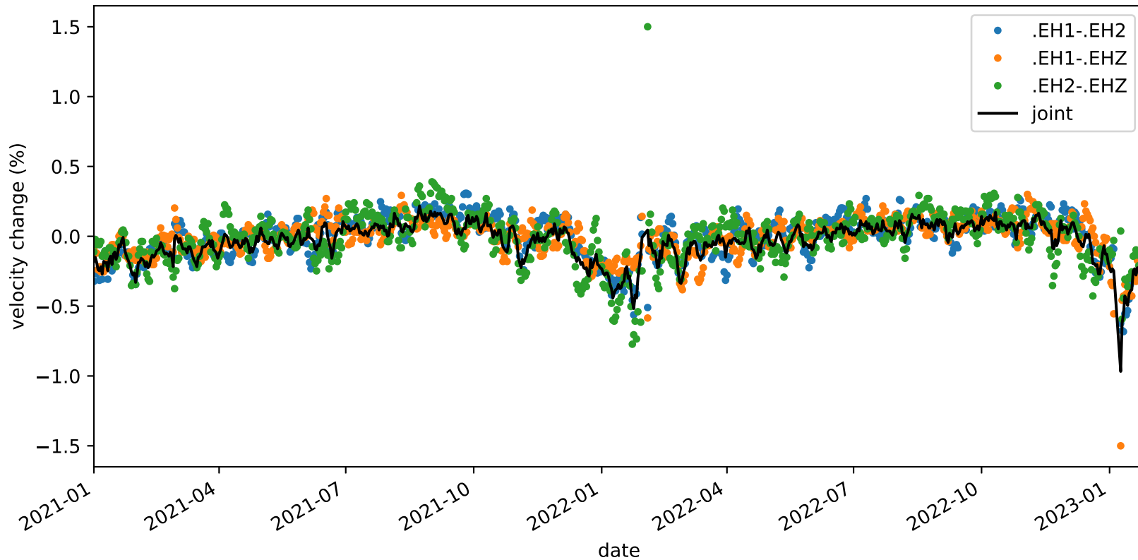
velocity_change_c1f_s4_t1a_tw_005.0s-010.0s_PB.B932-PB.B932
