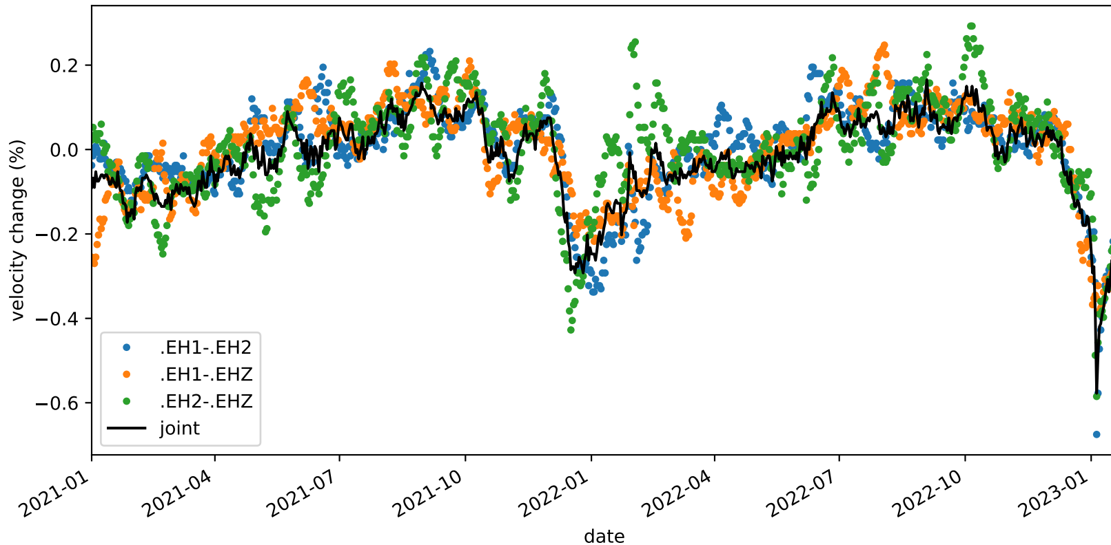
velocity_change_c1h_s3_t1c_tw_005.0s-015.0s_PB.B932-PB.B932
