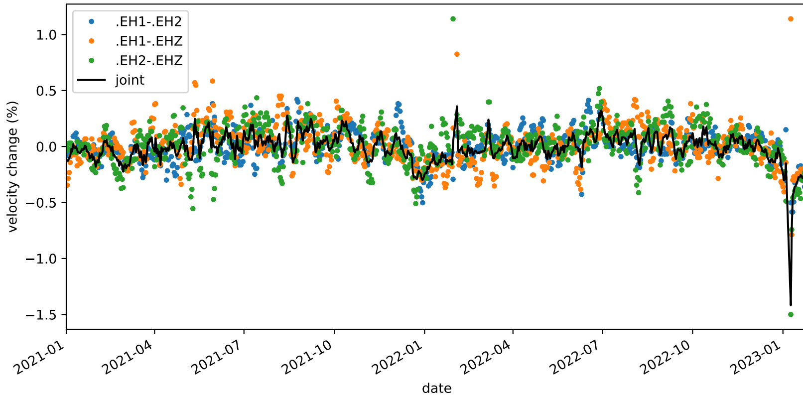
velocity_change_c1b_s4_t1c_tw_005.0s-015.0s_PB.B932-PB.B932
