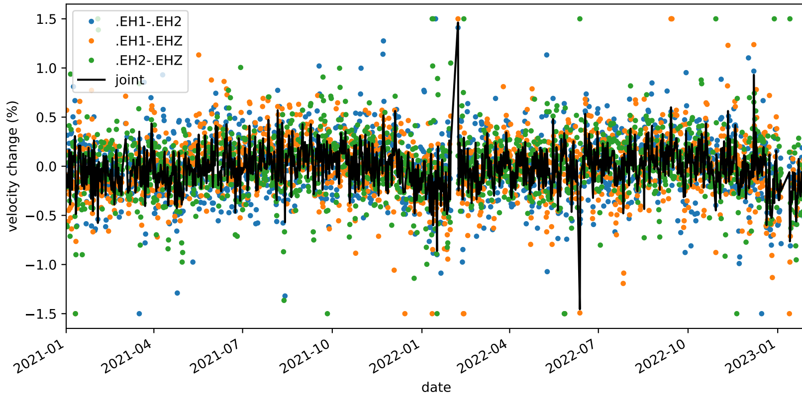
velocity_change_c1g_s1_t1b_tw_010.0s-015.0s_PB.B932-PB.B932
