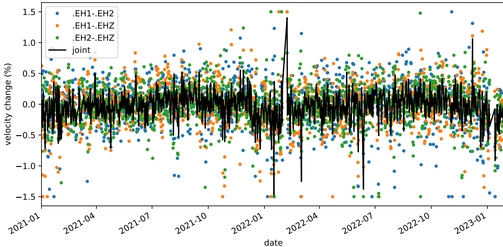
velocity_change_c1f_s1_t1b_tw_010.0s-015.0s_PB.B932-PB.B932
