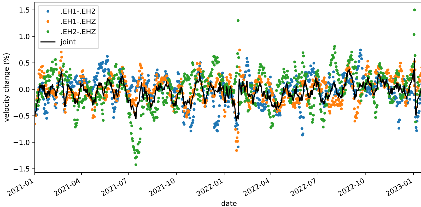
velocity_change_c1d_s3_t1b_tw_010.0s-015.0s_PB.B932-PB.B932
