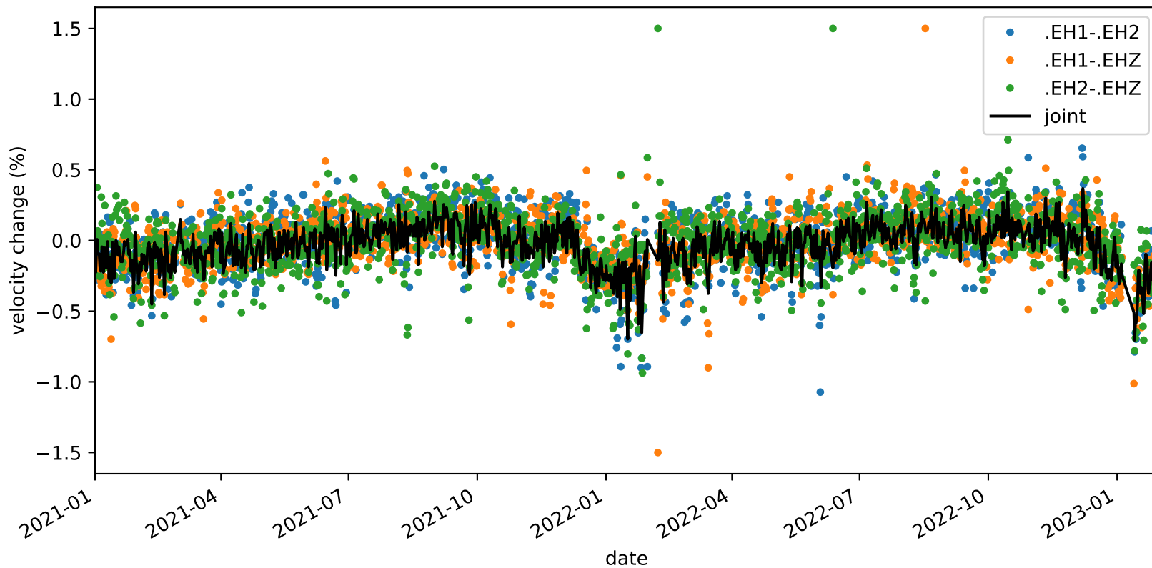
velocity_change_c1g_s1_t1c_tw_005.0s-015.0s_PB.B932-PB.B932
