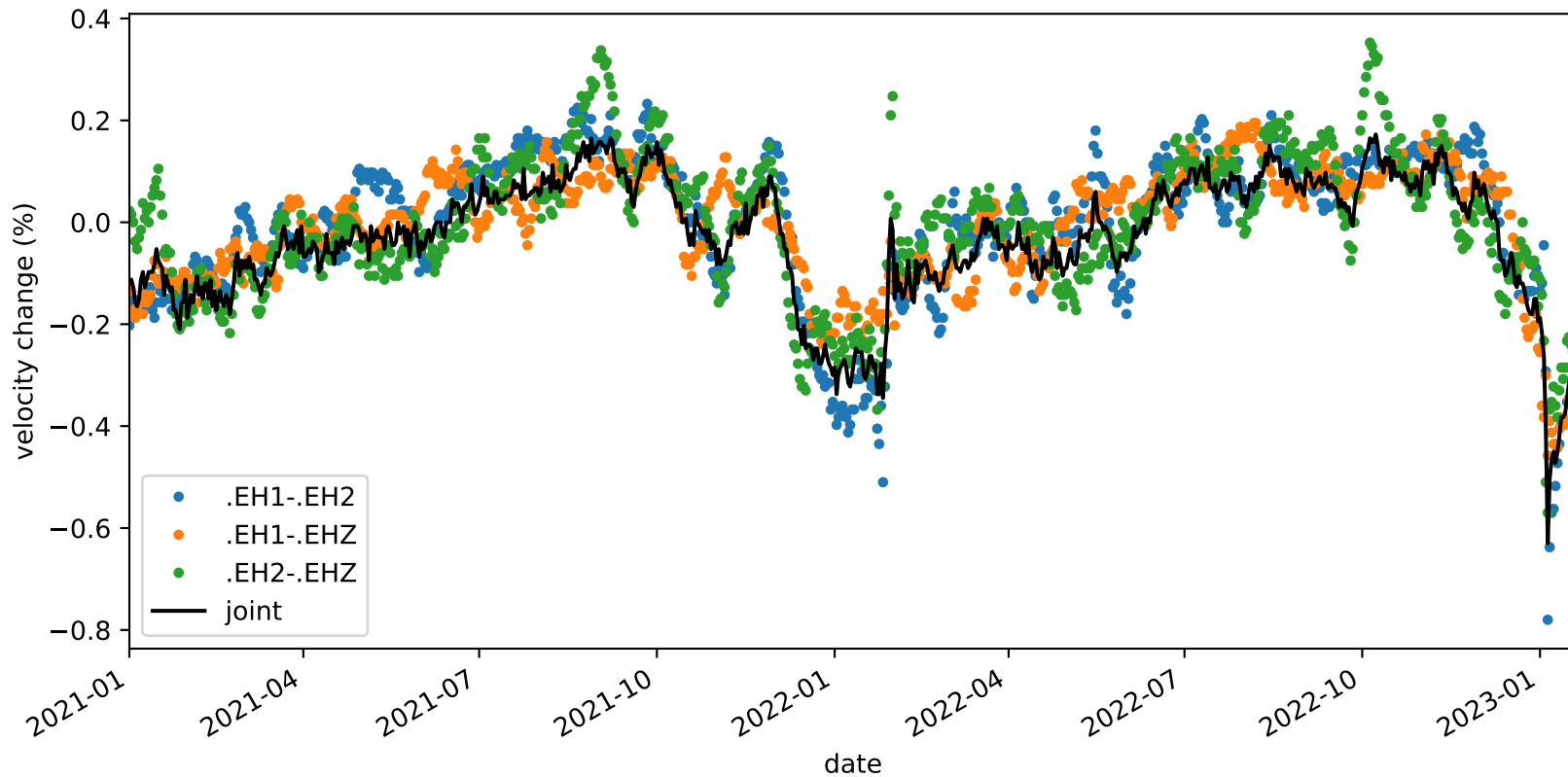
velocity_change_c1g_s3_t1a_tw_005.0s-010.0s_PB.B932-PB.B932
