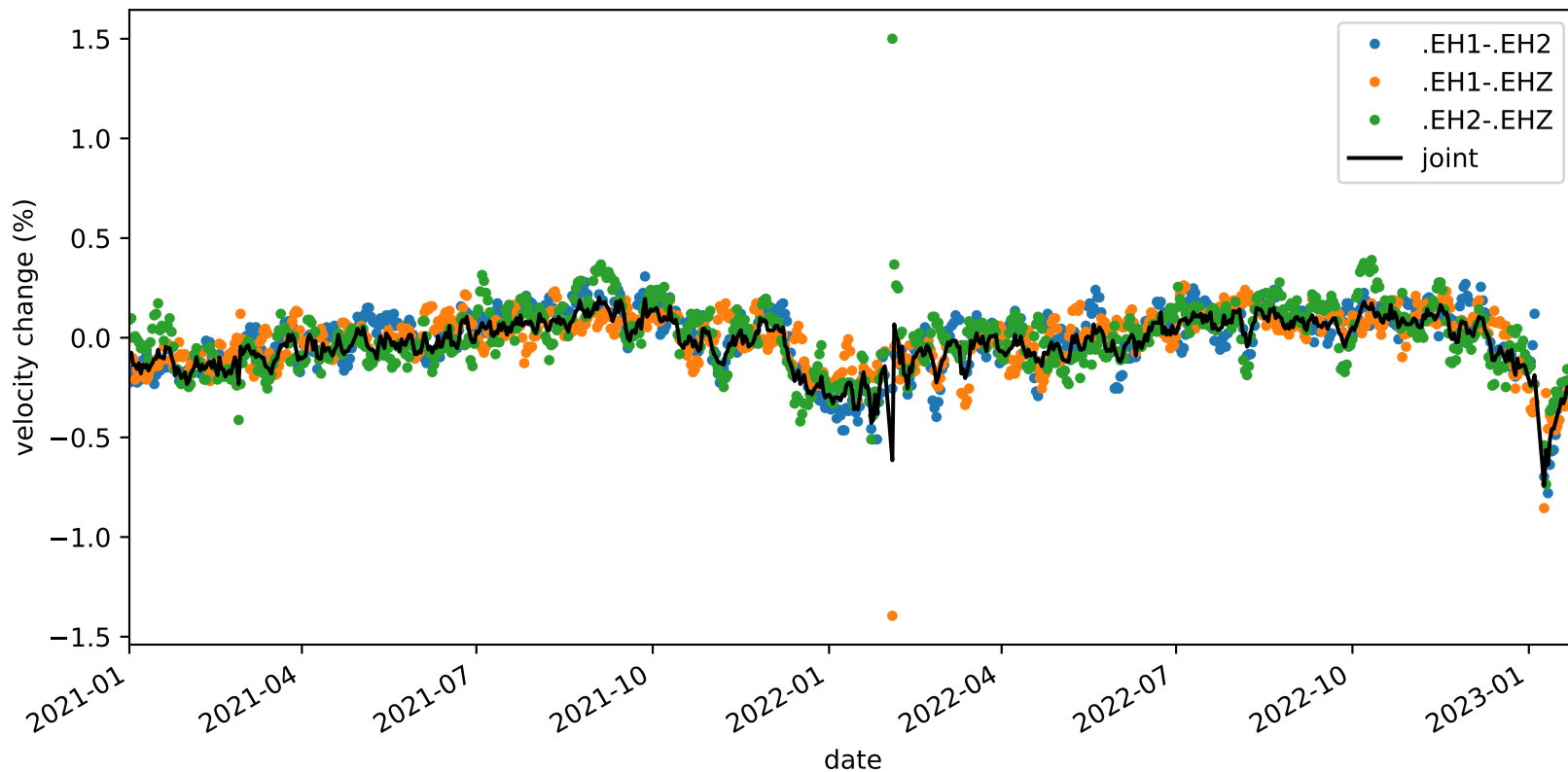
velocity_change_c1g_s4_t1a_tw_005.0s-010.0s_PB.B932-PB.B932
