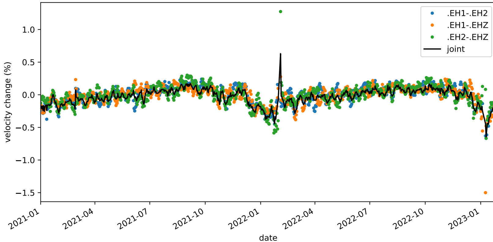
velocity_change_c1f_s4_t1c_tw_005.0s-015.0s_PB.B932-PB.B932
