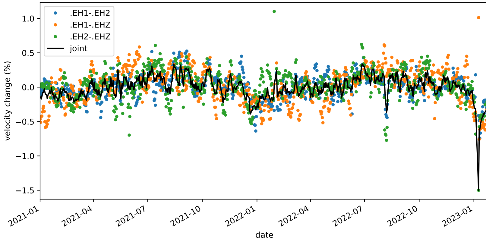
velocity_change_c1b_s4_t1a_tw_005.0s-010.0s_PB.B932-PB.B932
