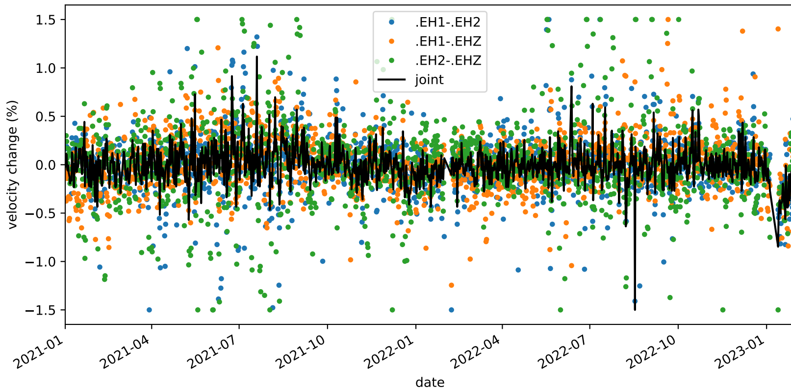
velocity_change_cli_sl_t1a_tw_005.0s-010.0s_PB.B932-PB.B932
