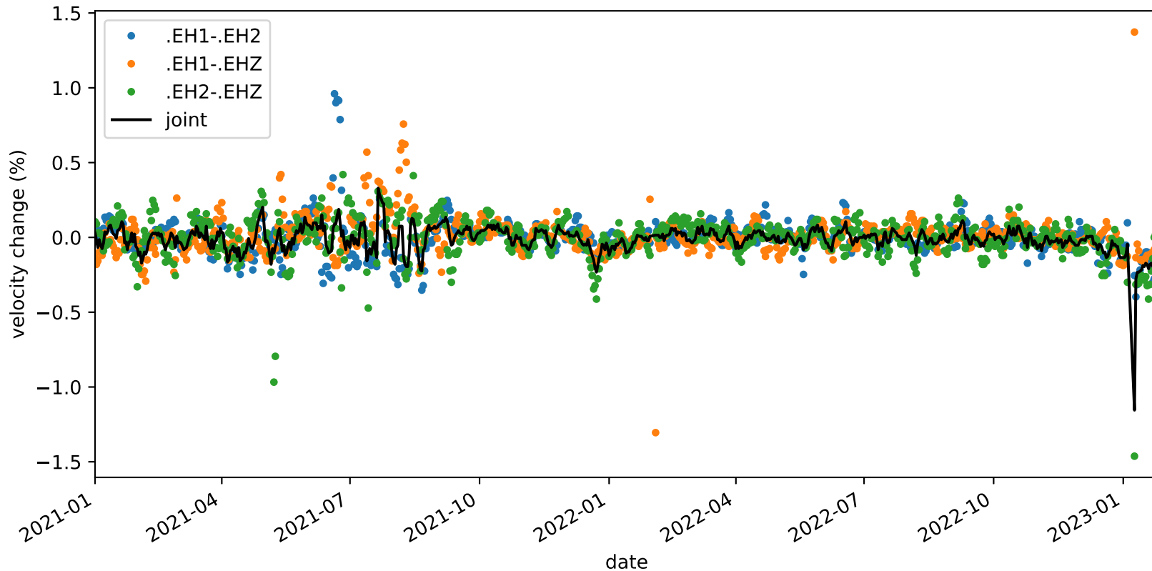
velocity_change_c1i_s4_t1c_tw_005.0s-015.0s_PB.B932-PB.B932
