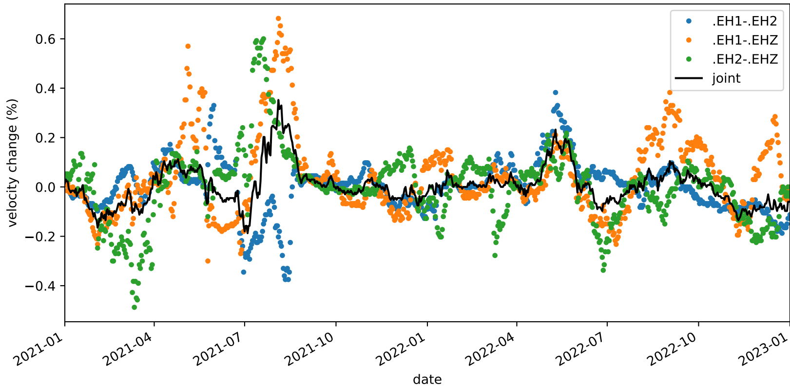
velocity_change_c1_s2_t1c_tw_005.0s-015.0s_PB.B932-PB.B932
