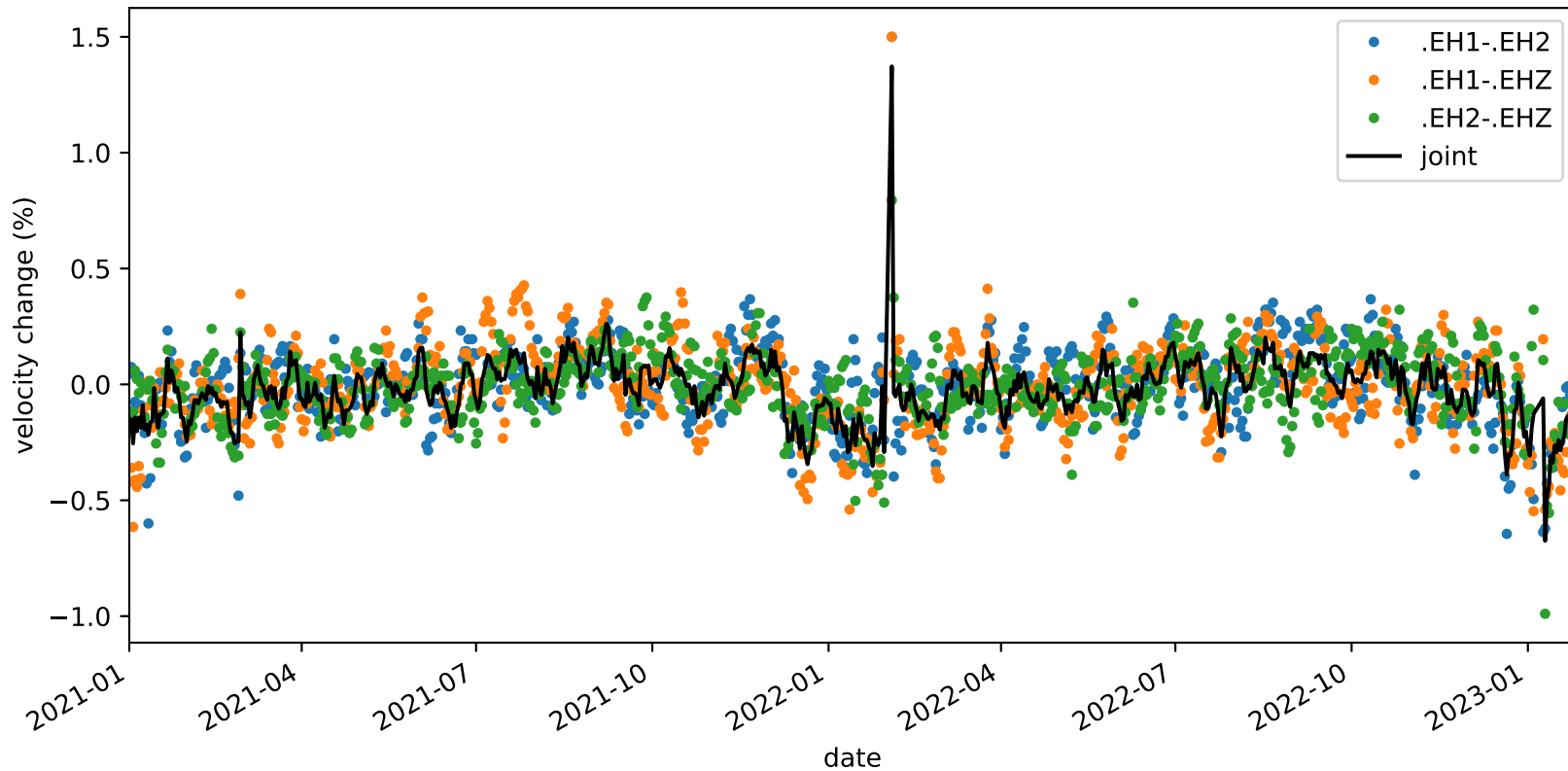
velocity_change_c1f_s4_t1b_tw_010.0s-015.0s_PB.B932-PB.B932
