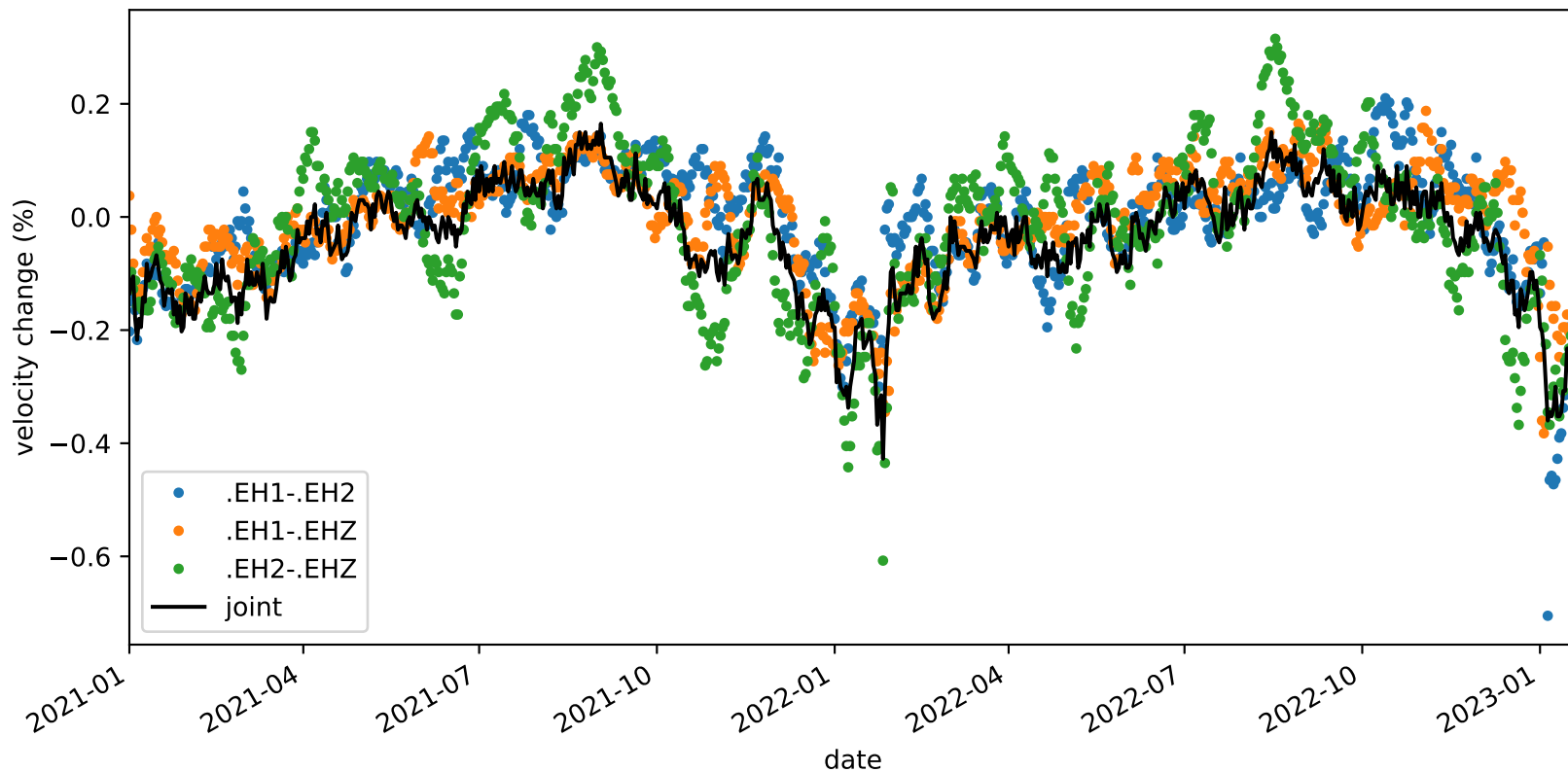
velocity_change_c1e_s3_t1c_tw_005.0s-015.0s_PB.B932-PB.B932
