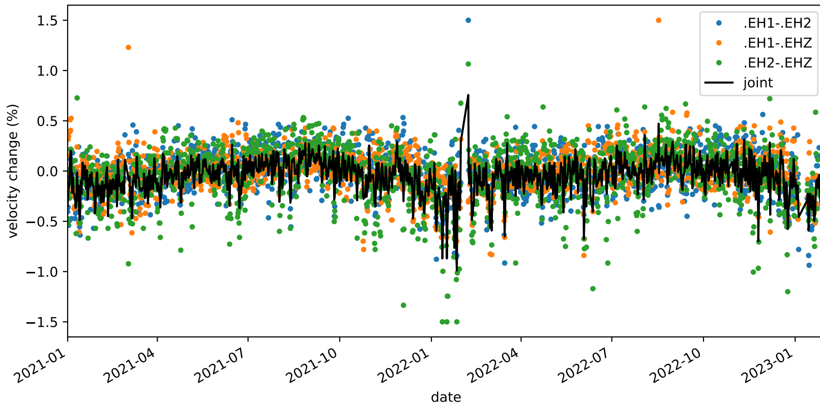
velocity_change_c1e_s1_t1c_tw_005.0s-015.0s_PB.B932-PB.B932
