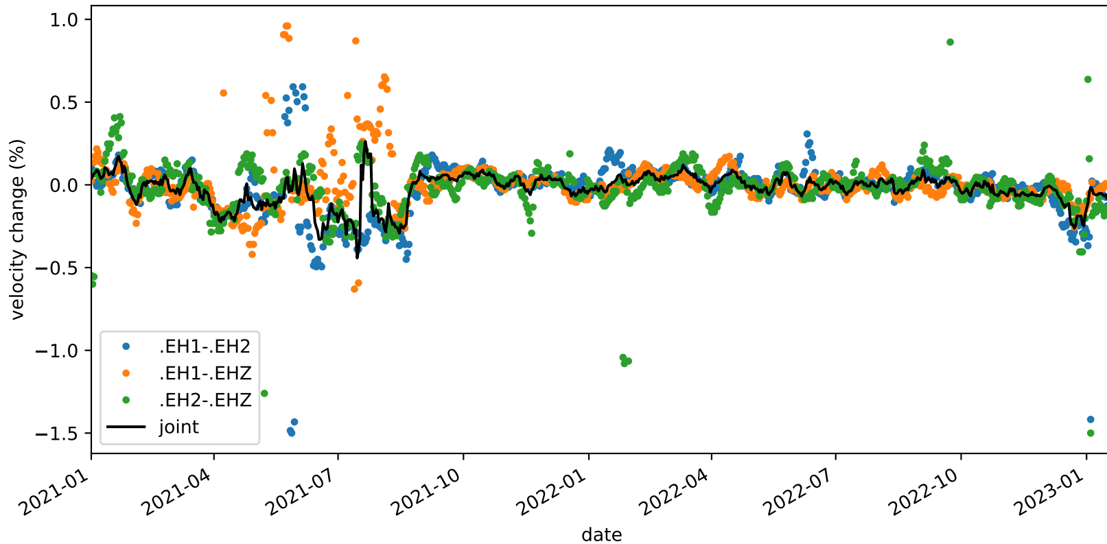
velocity_change_c1i_s3_t1b_tw_010.0s-015.0s_PB.B932-PB.B932
