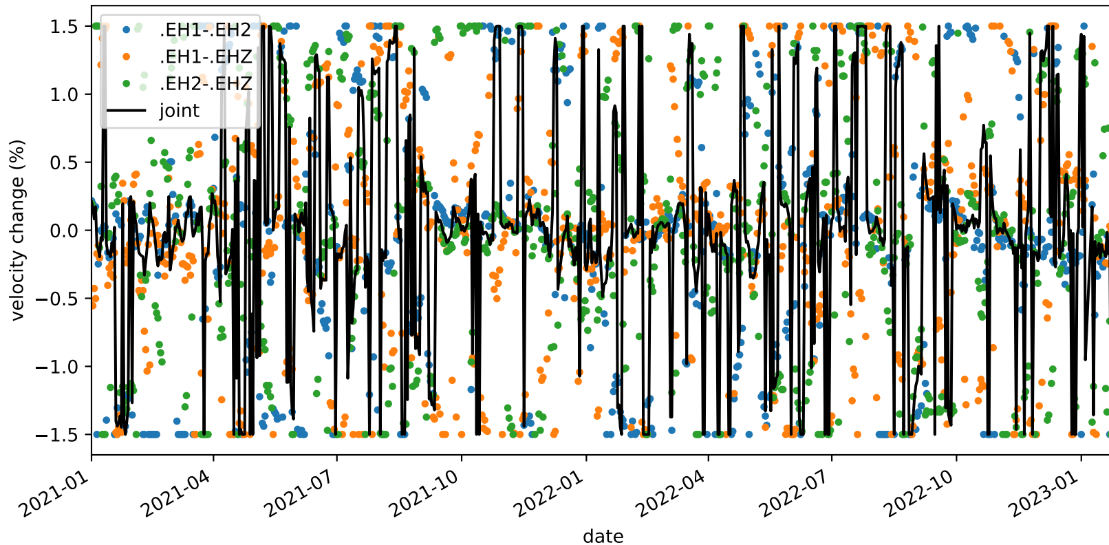
velocity_change_c1_s4_t1b_tw_010.0s-015.0s_PB.B932-PB.B932
