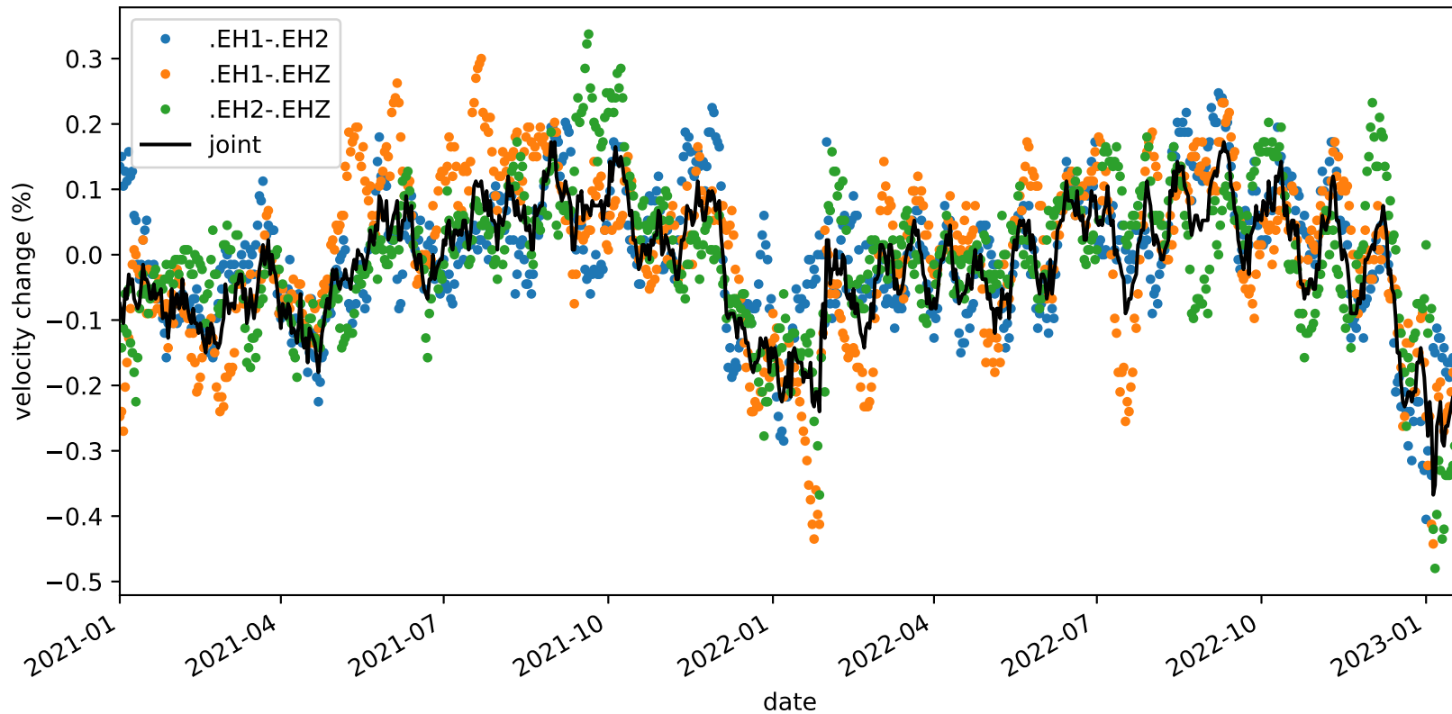
velocity_change_c1g_s3_t1b_tw_010.0s-015.0s_PB.B932-PB.B932
