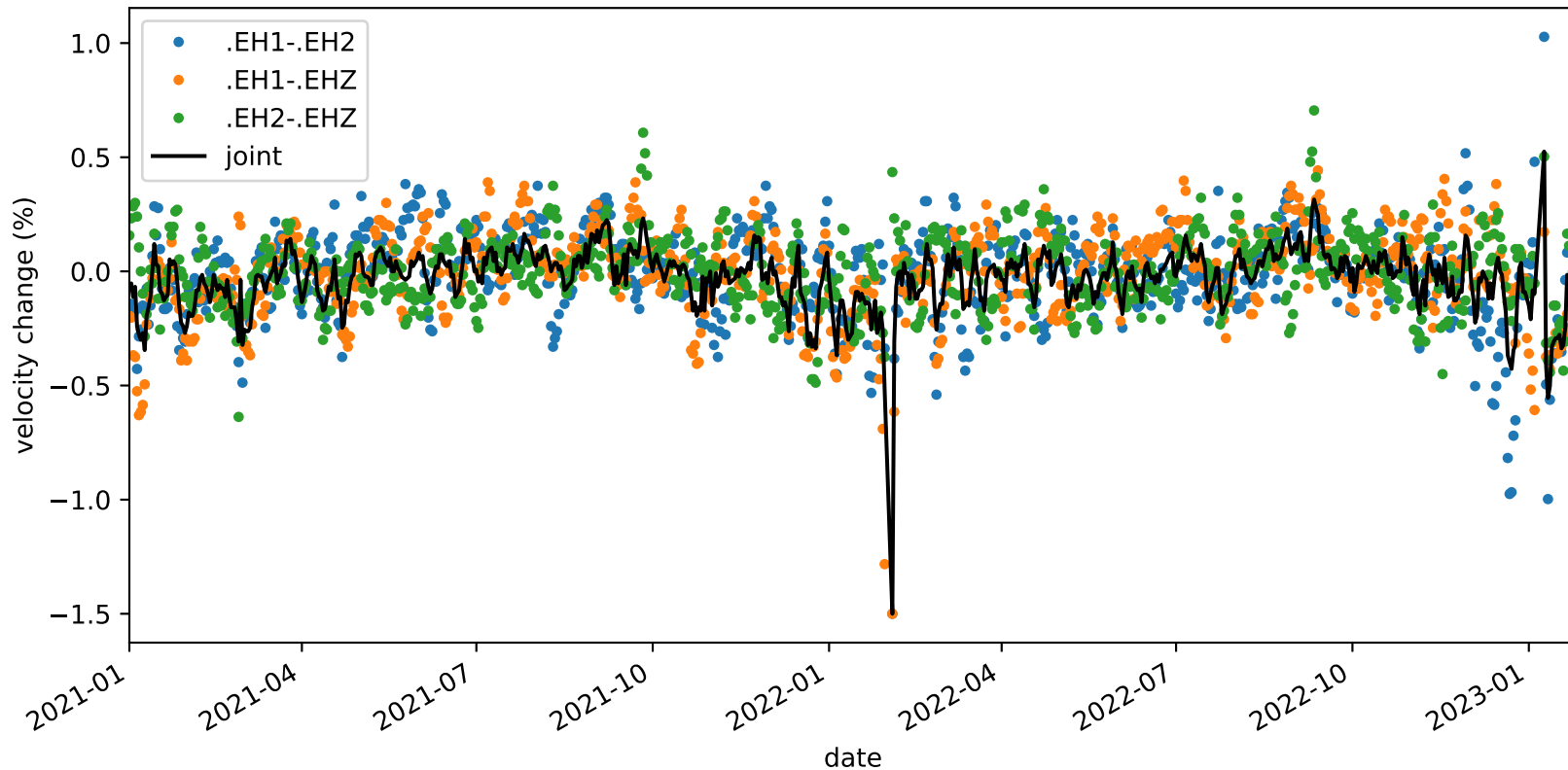
velocity_change_c1e_s4_t1b_tw_010.0s-015.0s_PB.B932-PB.B932
