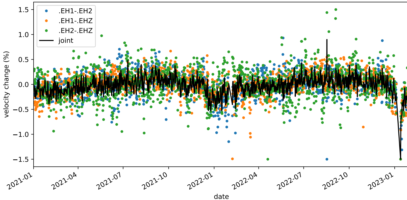
velocity_change_c1h_s1_t1a_tw_005.0s-010.0s_PB.B932-PB.B932
