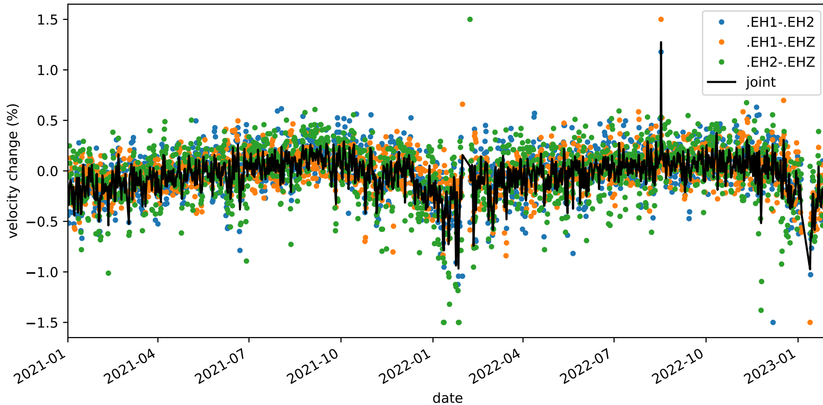
velocity_change_c1f_s1_t1a_tw_005.0s-010.0s_PB.B932-PB.B932
