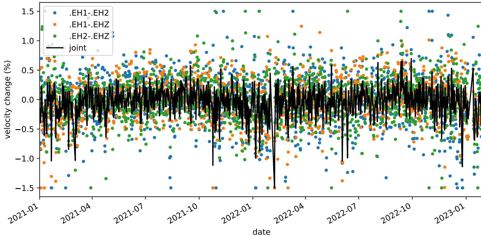
velocity_change_c1e_s1_t1b_tw_010.0s-015.0s_PB.B932-PB.B932
