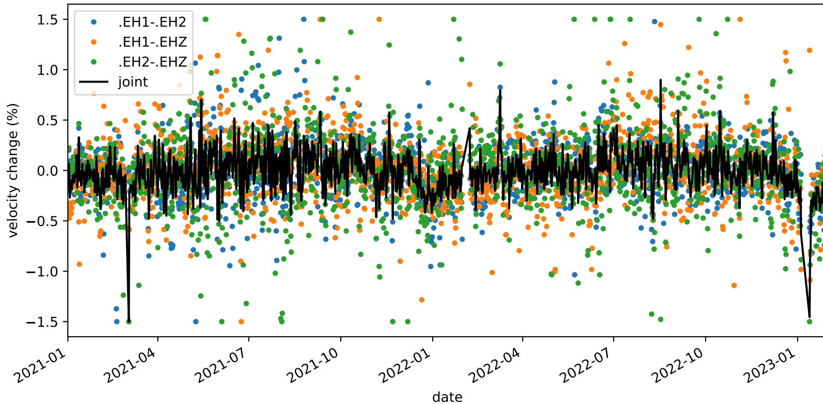
velocity_change_c1b_s1_t1c_tw_005.0s-015.0s_PB.B932-PB.B932
