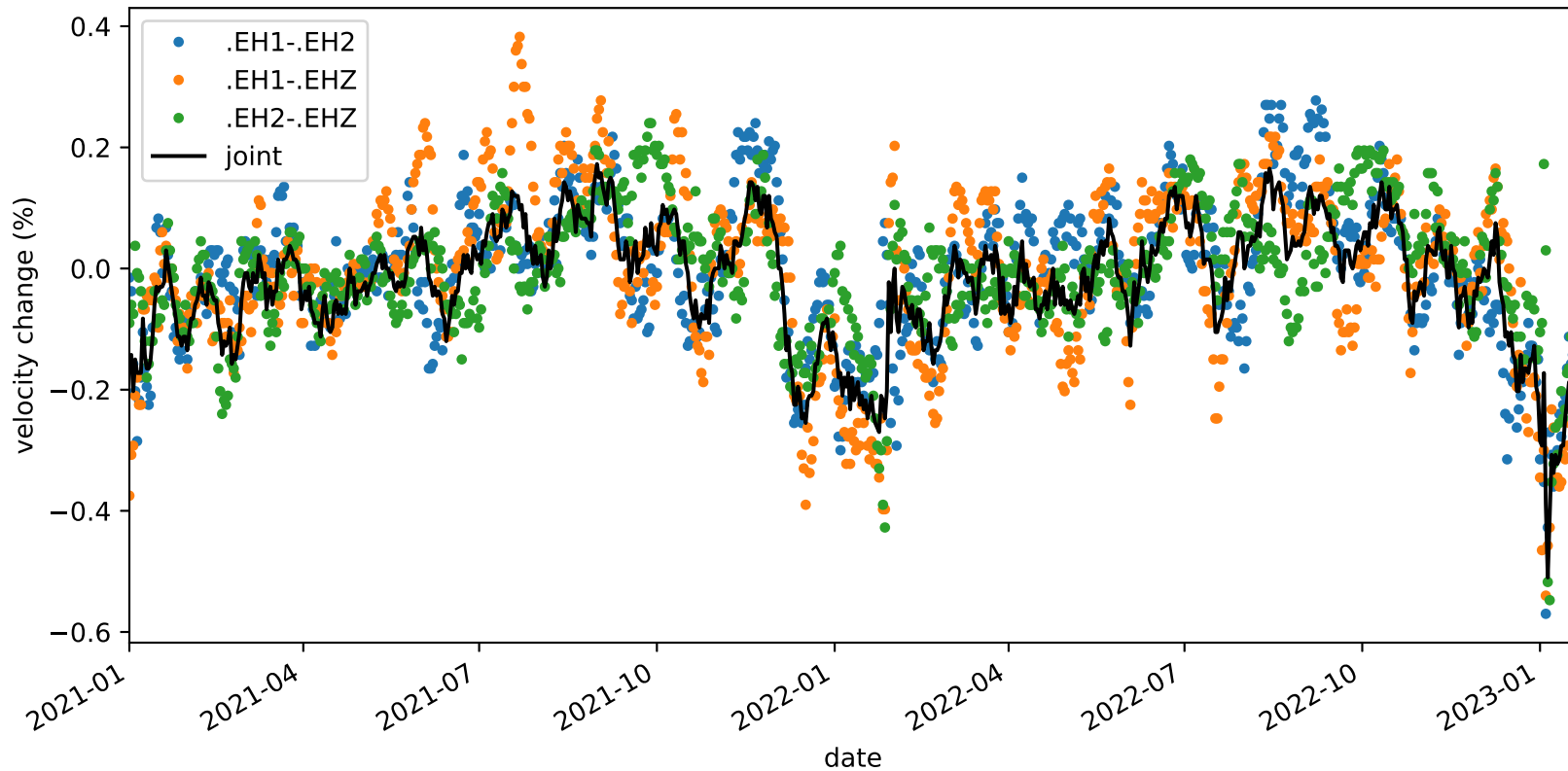
velocity_change_c1f_s3_t1b_tw_010.0s-015.0s_PB.B932-PB.B932
