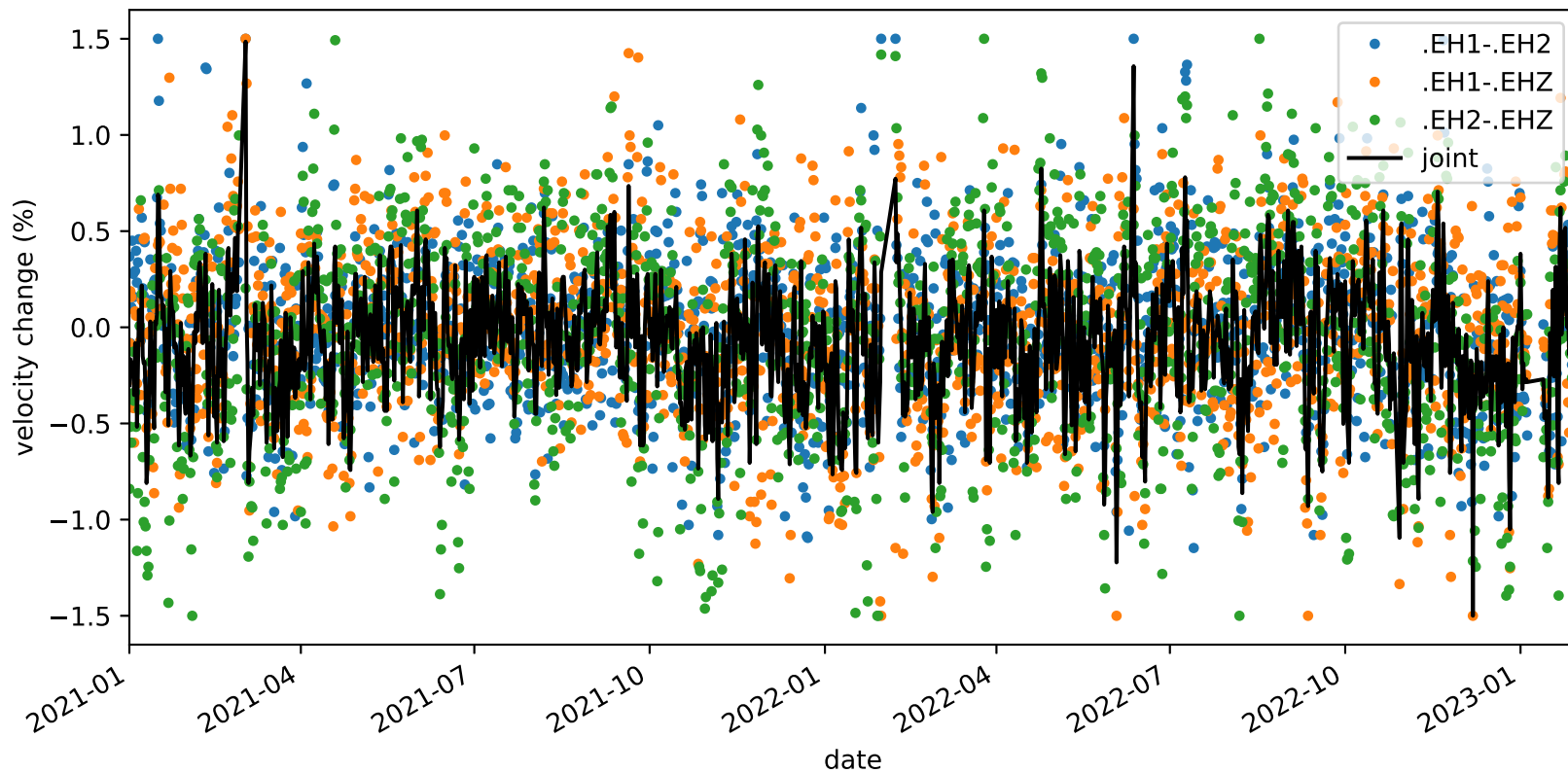
velocity_change_c1d_s1_t1c_tw_005.0s-015.0s_PB.B932-PB.B932
