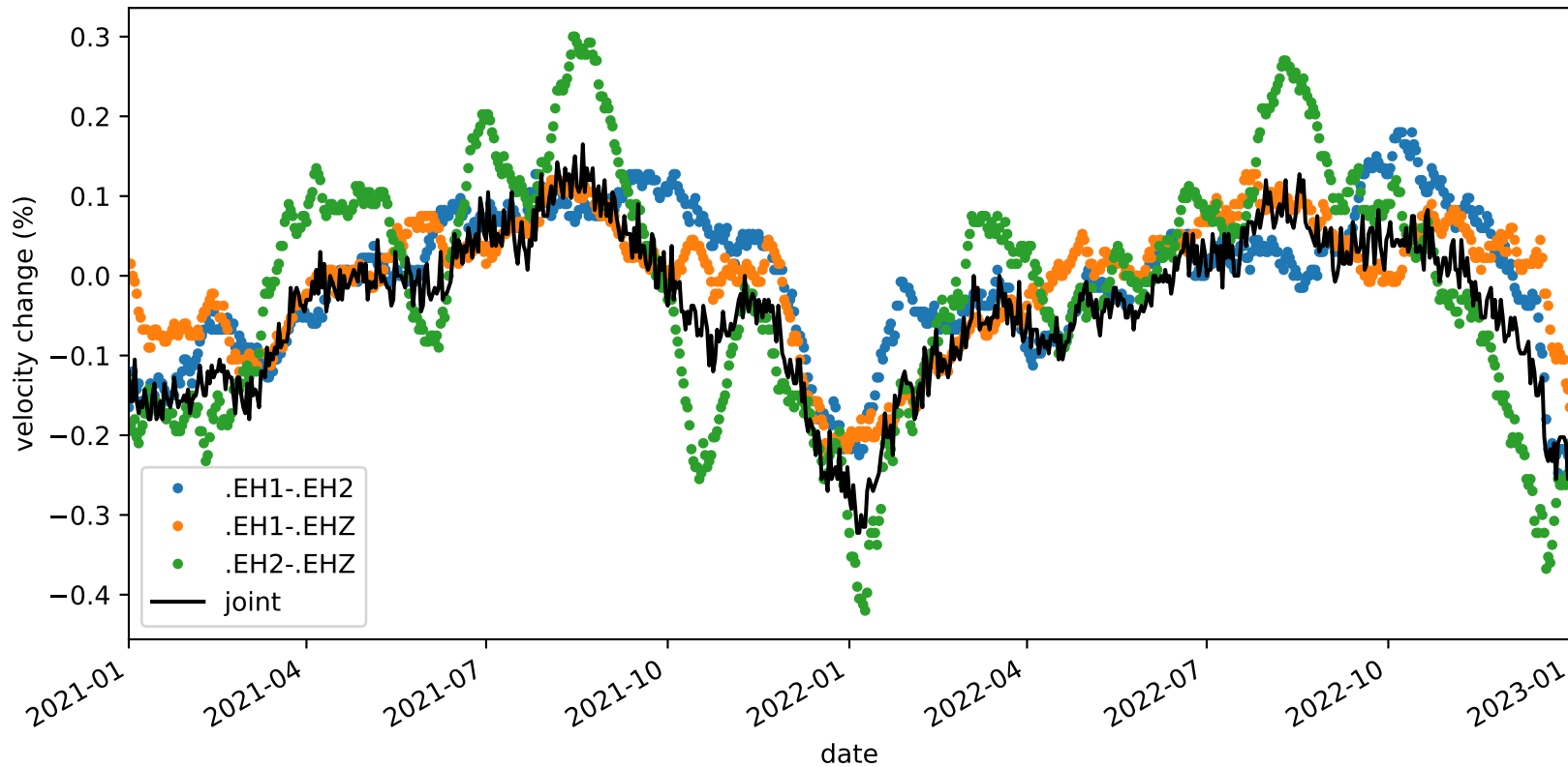
velocity_change_c1e_s2_t1a_tw_005.0s-010.0s_PB.B932-PB.B932
