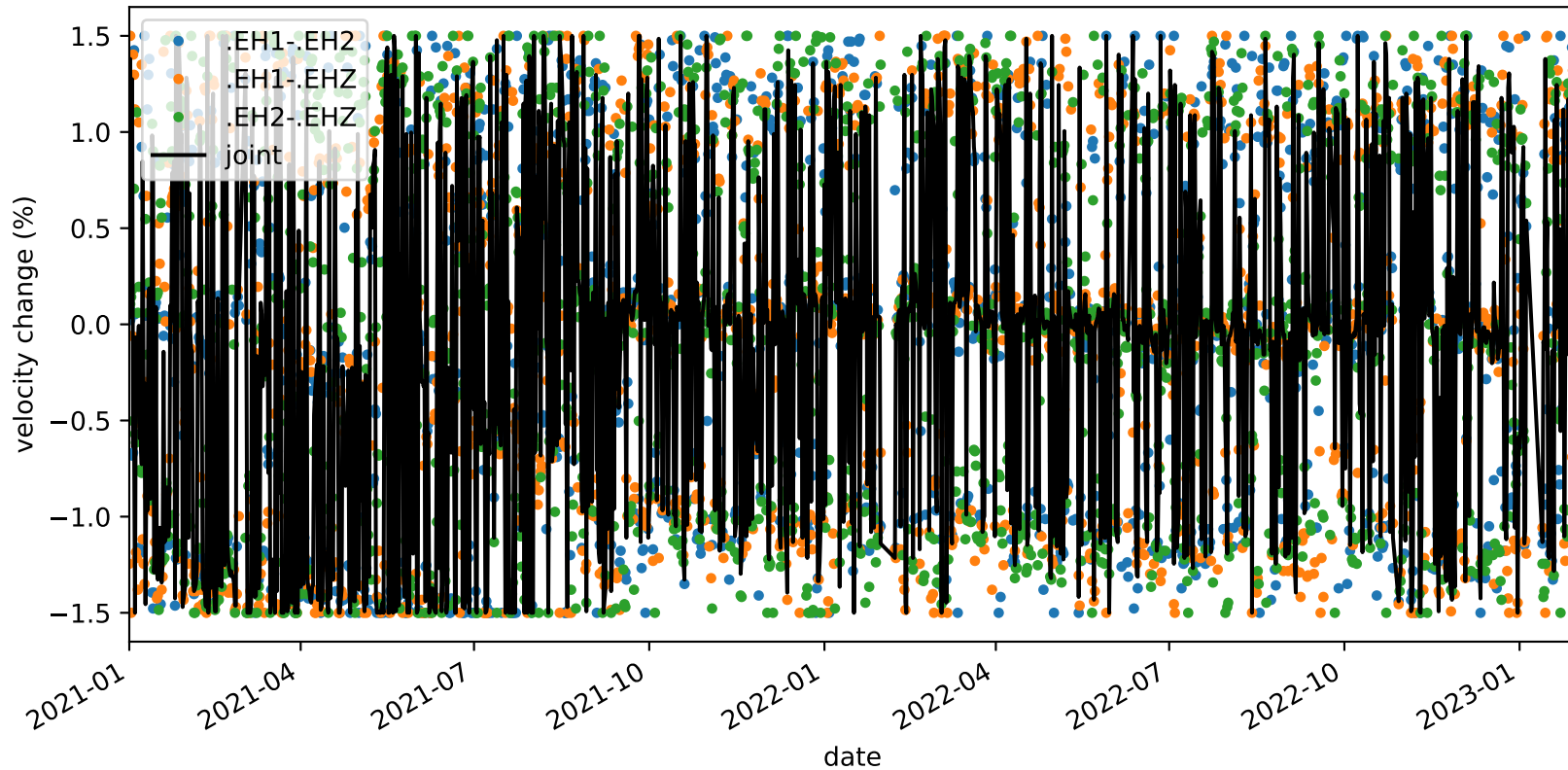
velocity_change_c1c_s1_t1b_tw_010.0s-015.0s_PB.B932-PB.B932
