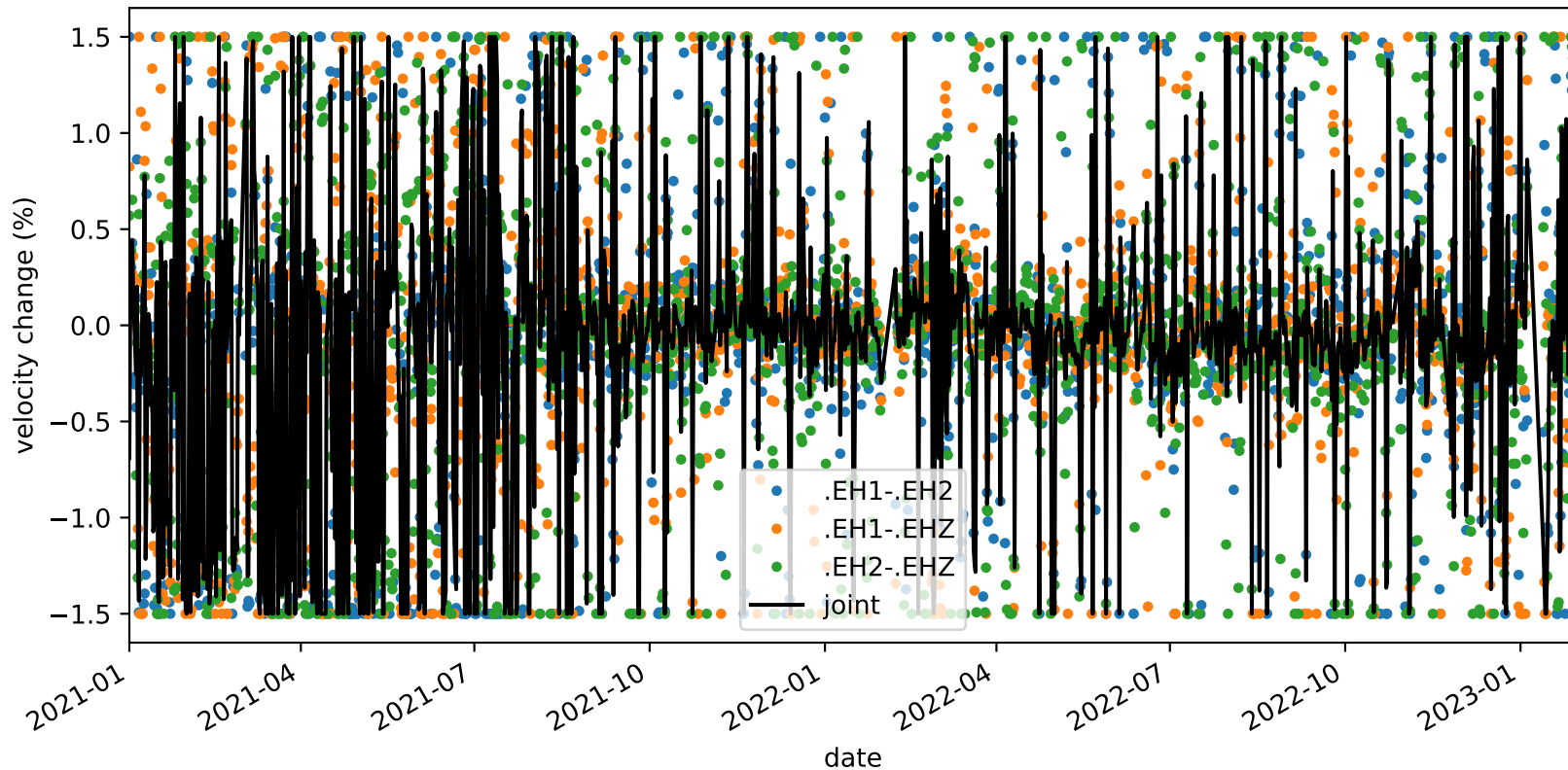
velocity_change_c1c_s1_t1a_tw_005.0s-010.0s_PB.B932-PB.B932
