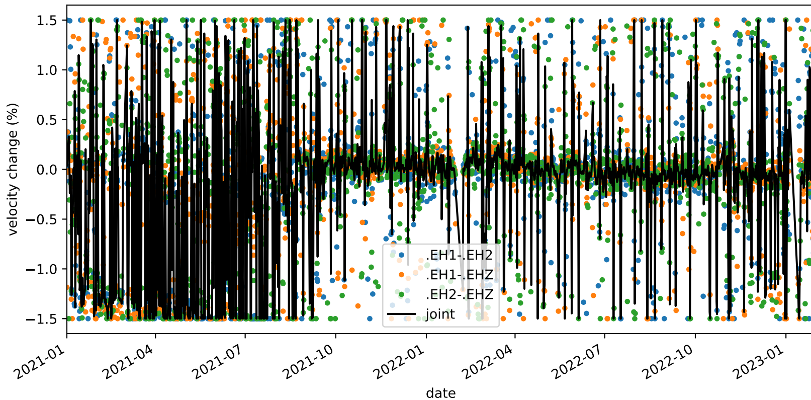
velocity_change_c1c_s1_t1c_tw_005.0s-015.0s_PB.B932-PB.B932
