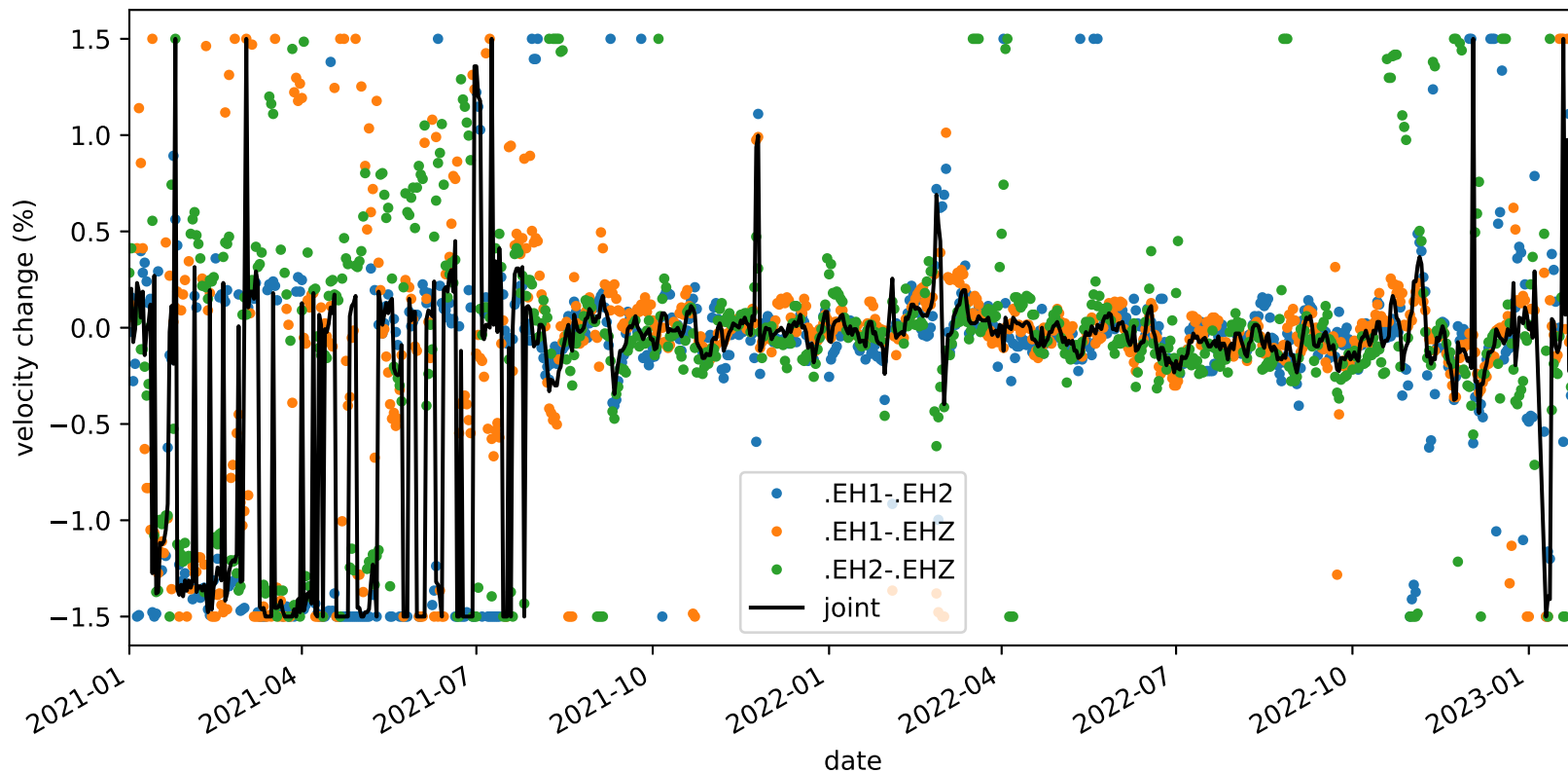
velocity_change_c1c_s4_t1a_tw_005.0s-010.0s_PB.B932-PB.B932
