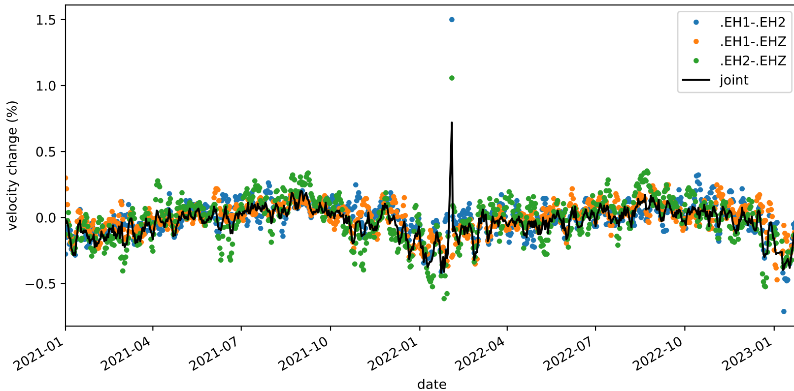
velocity_change_c1e_s4_t1c_tw_005.0s-015.0s_PB.B932-PB.B932
