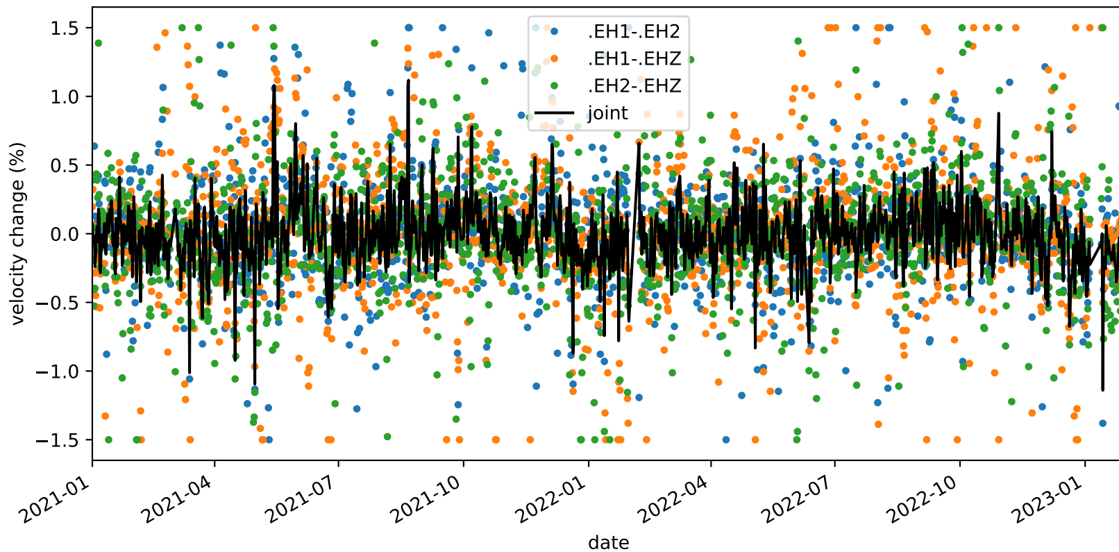
velocity_change_c1h_s1_t1b_tw_010.0s-015.0s_PB.B932-PB.B932
