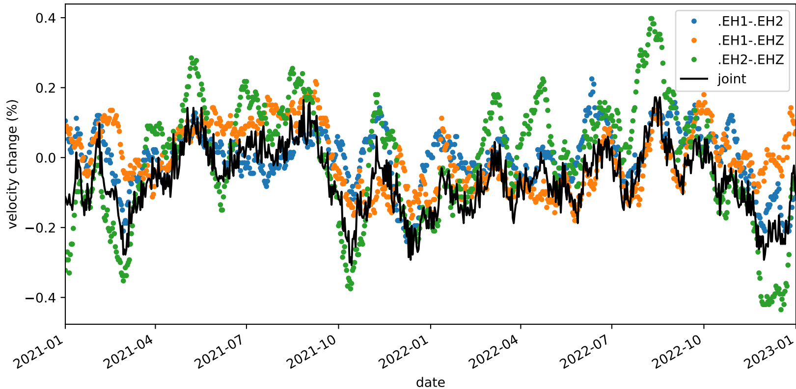
velocity_change_c1d_s2_t1c_tw_005.0s-015.0s_PB.B932-PB.B932
