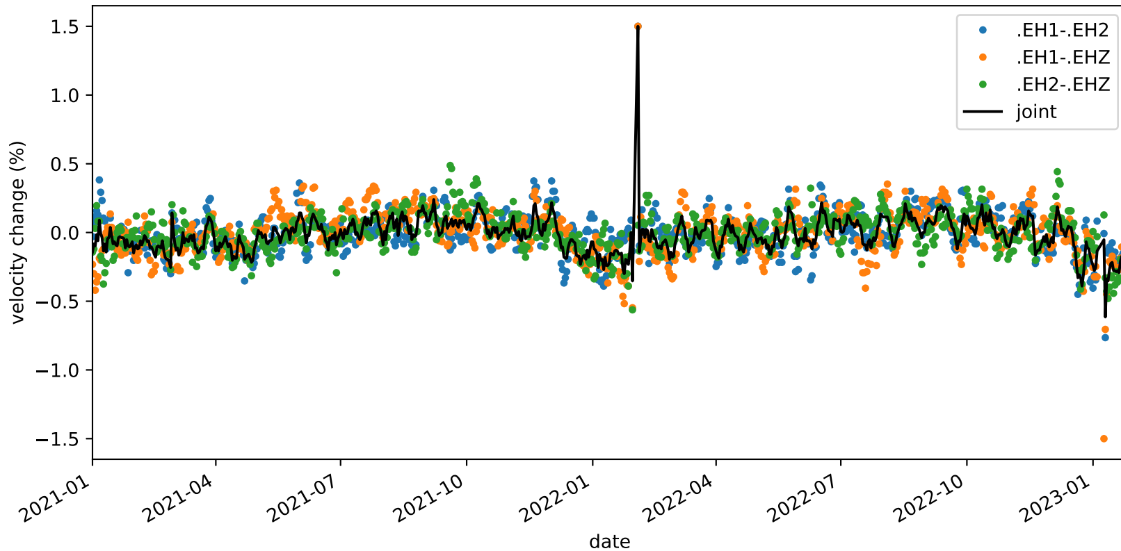
velocity_change_c1g_s4_t1b_tw_010.0s-015.0s_PB.B932-PB.B932
