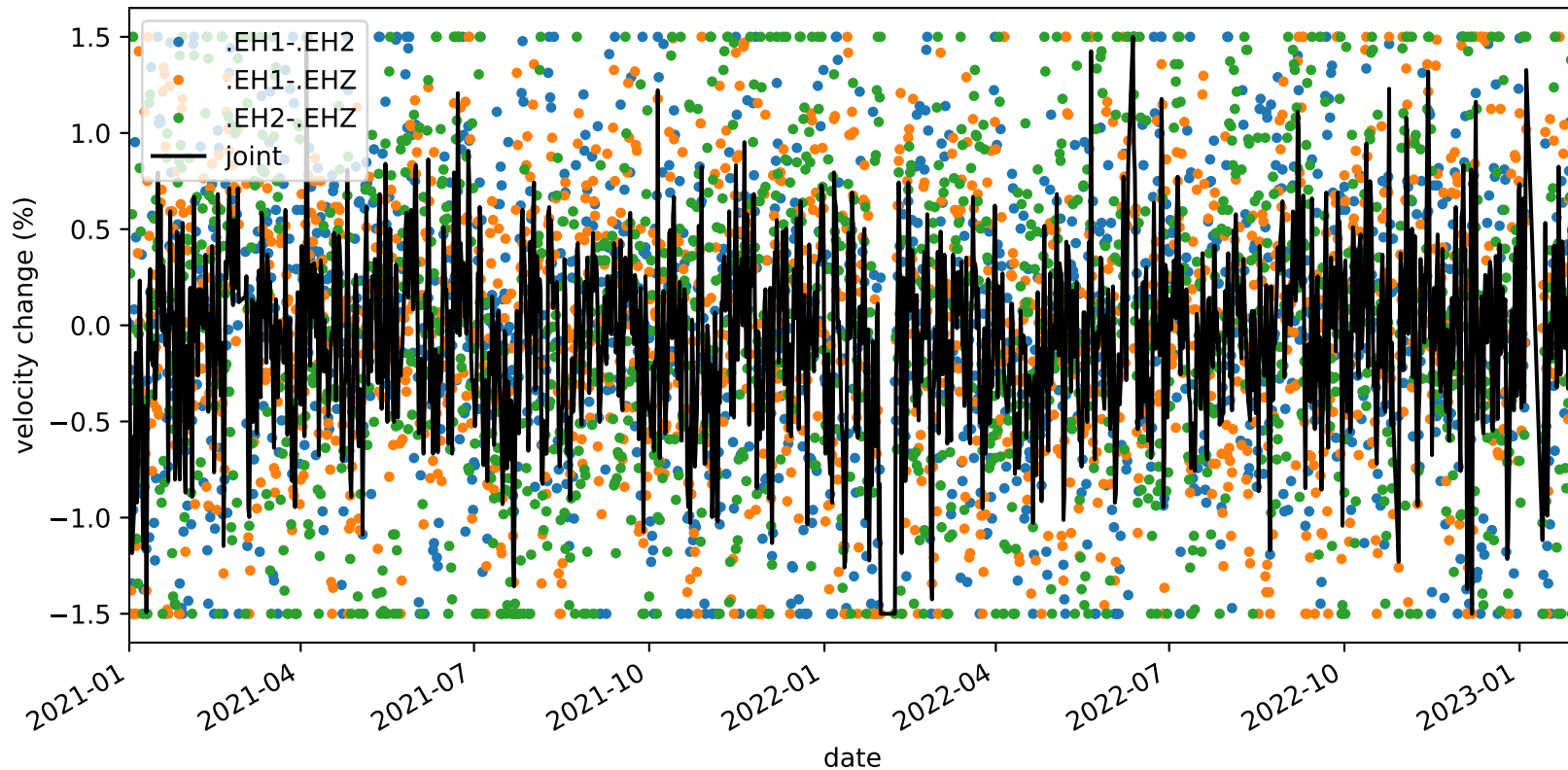
velocity_change_c1d_s1_t1b_tw_010.0s-015.0s_PB.B932-PB.B932
