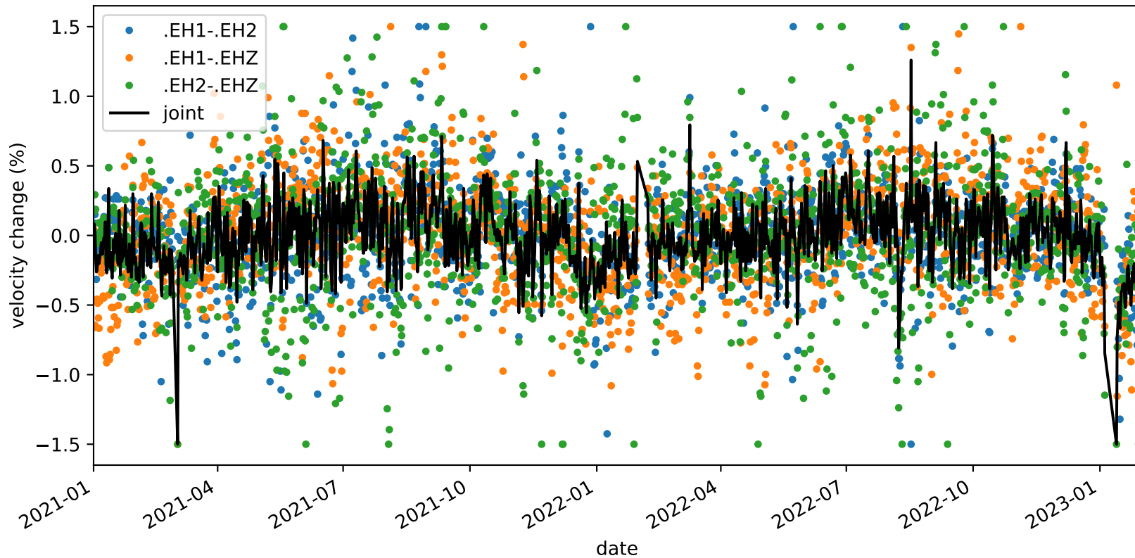
velocity_change_c1b_s1_t1a_tw_005.0s-010.0s_PB.B932-PB.B932
