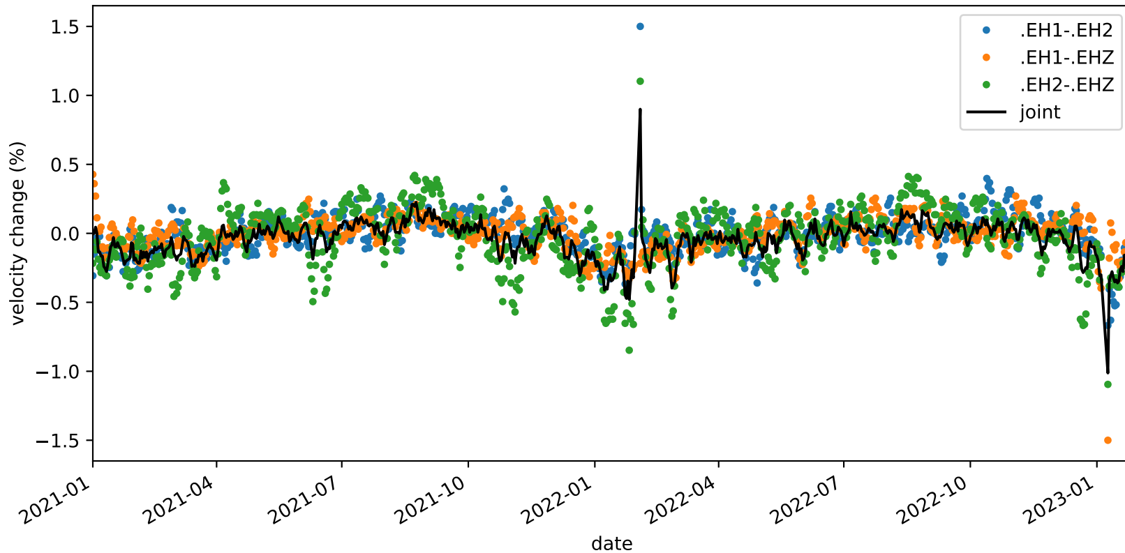
velocity_change_c1e_s4_t1a_tw_005.0s-010.0s_PB.B932-PB.B932
