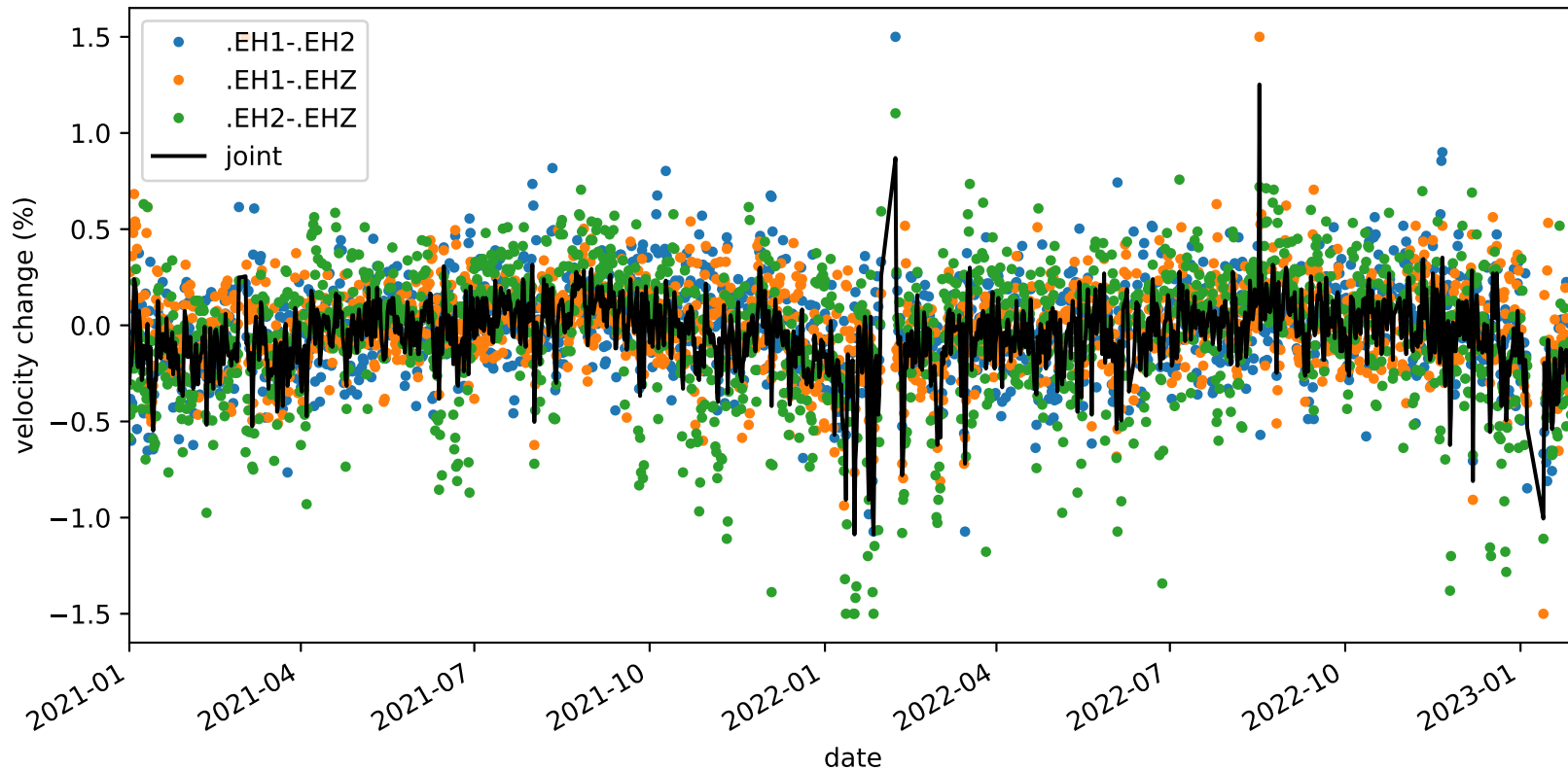
velocity_change_c1e_s1_t1a_tw_005.0s-010.0s_PB.B932-PB.B932
