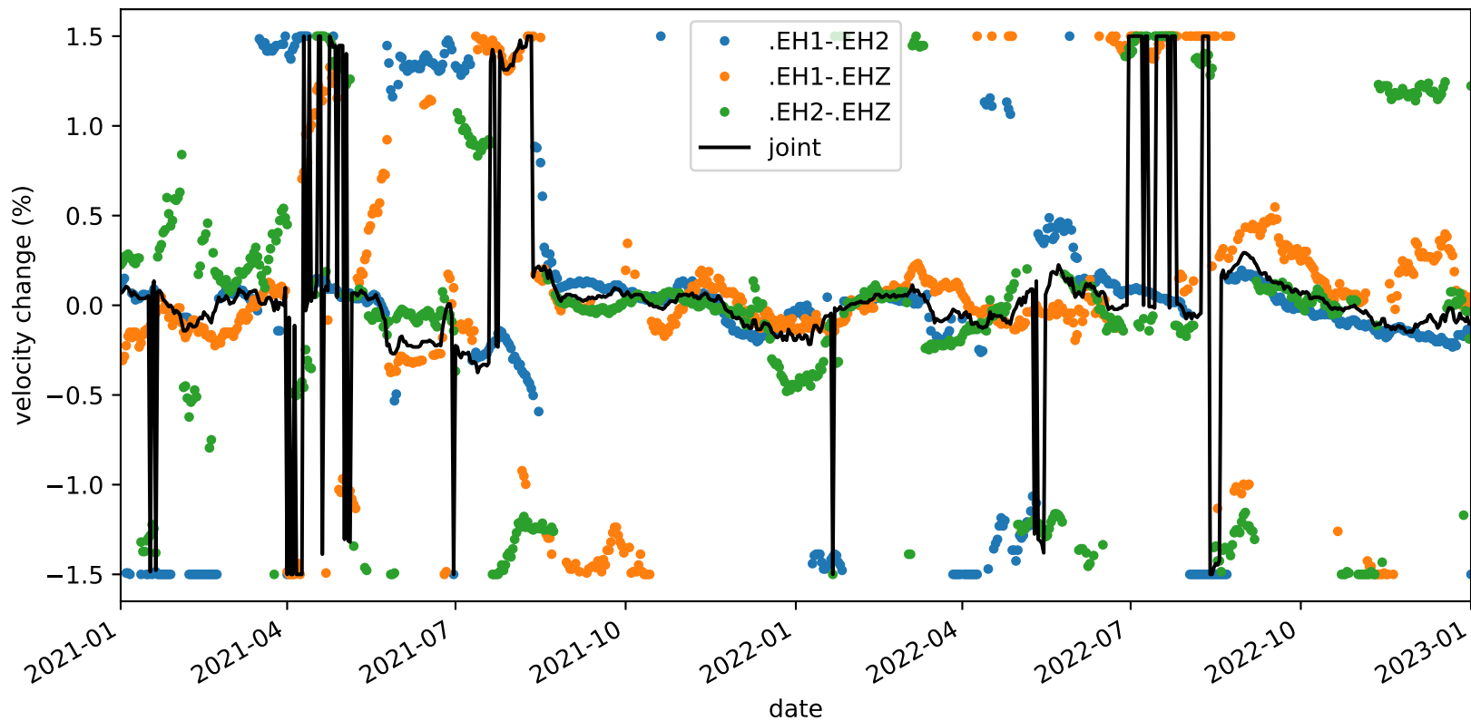
velocity_change_c1_s2_t1b_tw_010.0s-015.0s_PB.B932-PB.B932
