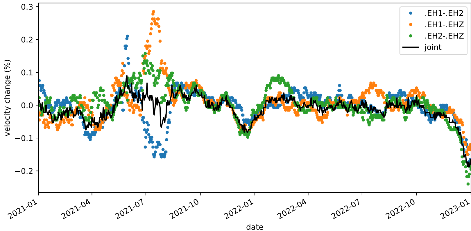
velocity_change_c1i_s2_t1c_tw_005.0s-015.0s_PB.B932-PB.B932
