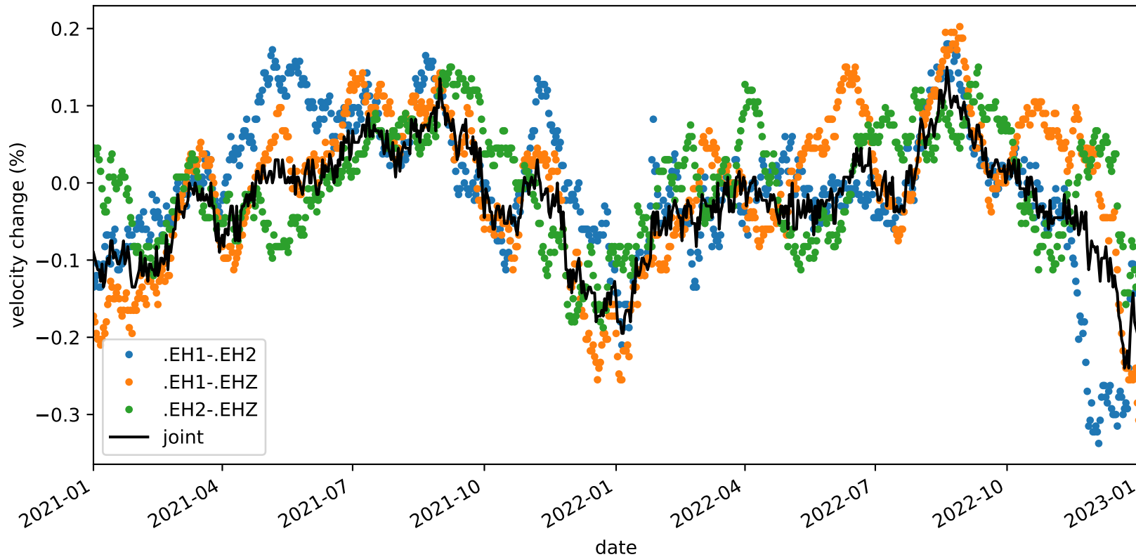
velocity_change_c1e_s2_t1b_tw_010.0s-015.0s_PB.B932-PB.B932
