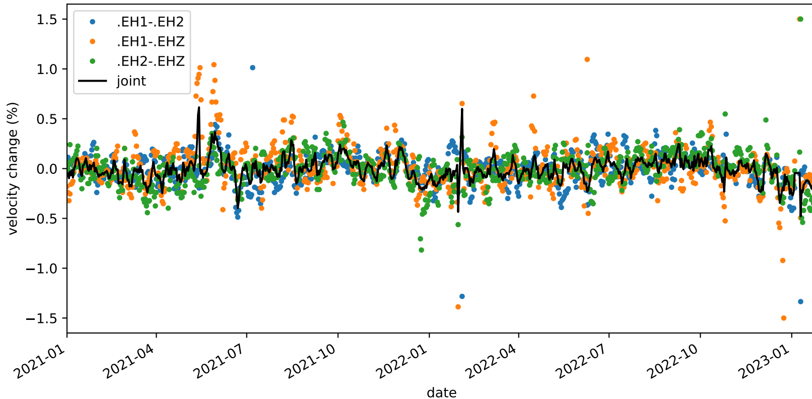
velocity_change_c1h_s4_t1b_tw_010.0s-015.0s_PB.B932-PB.B932
