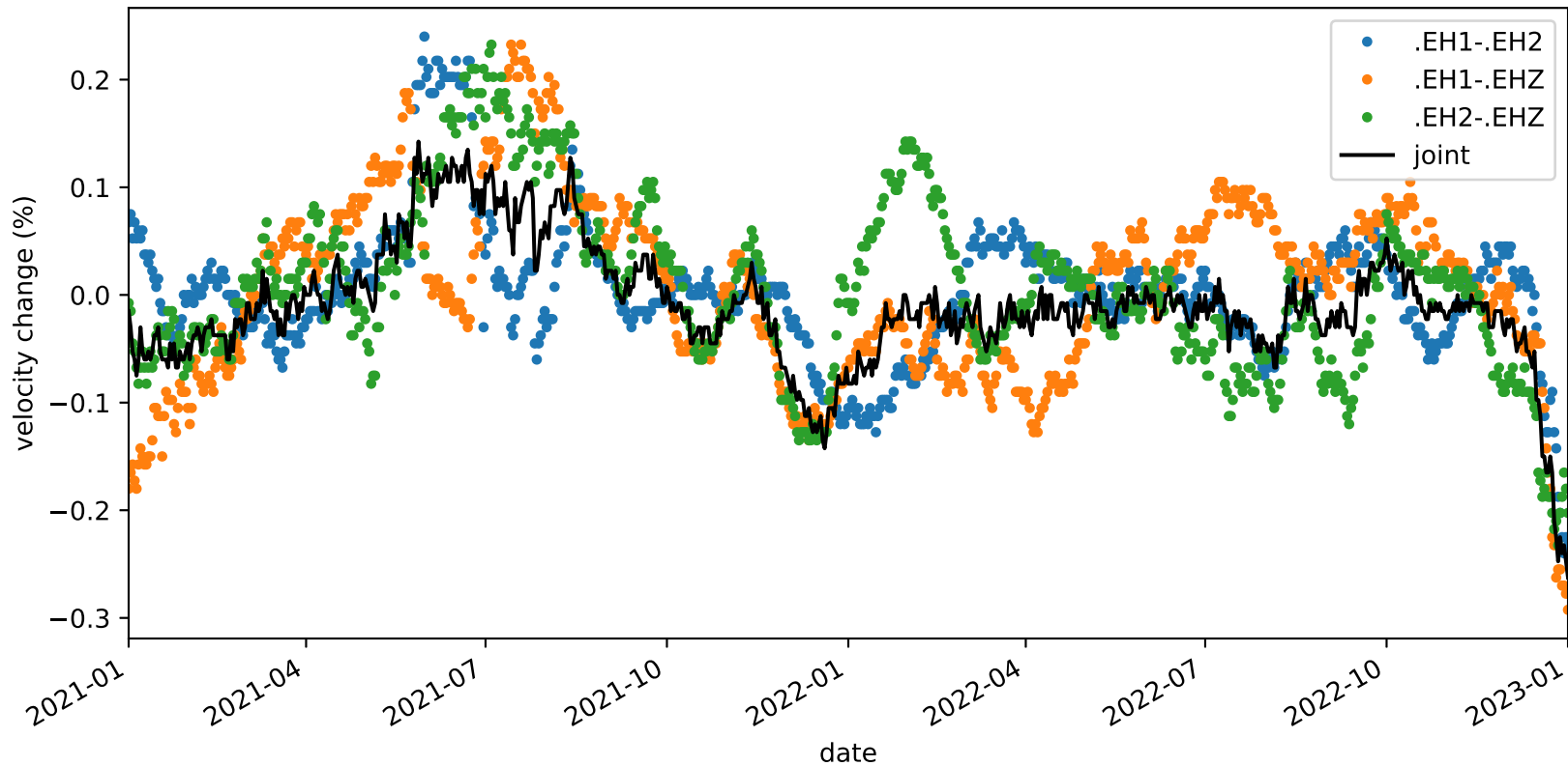
velocity_change_c1i_s2_t1a_tw_005.0s-010.0s_PB.B932-PB.B932
