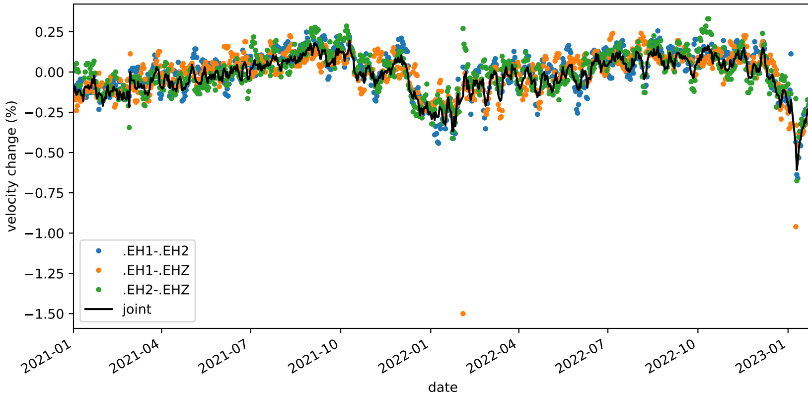
velocity_change_c1g_s4_t1c_tw_005.0s-015.0s_PB.B932-PB.B932
