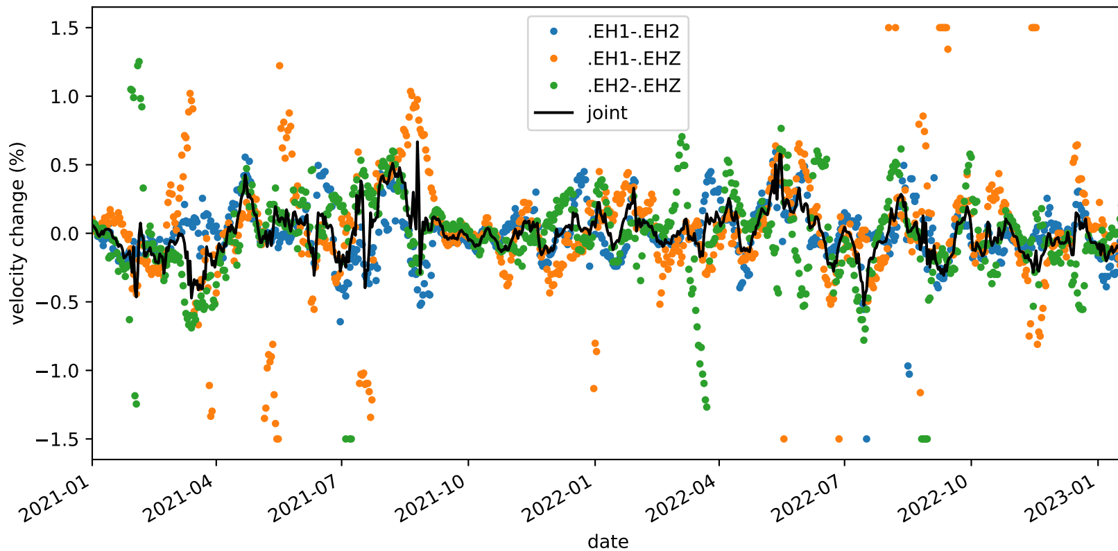
velocity_change_c1_s3_t1a_tw_005.0s-010.0s_PB.B932-PB.B932
