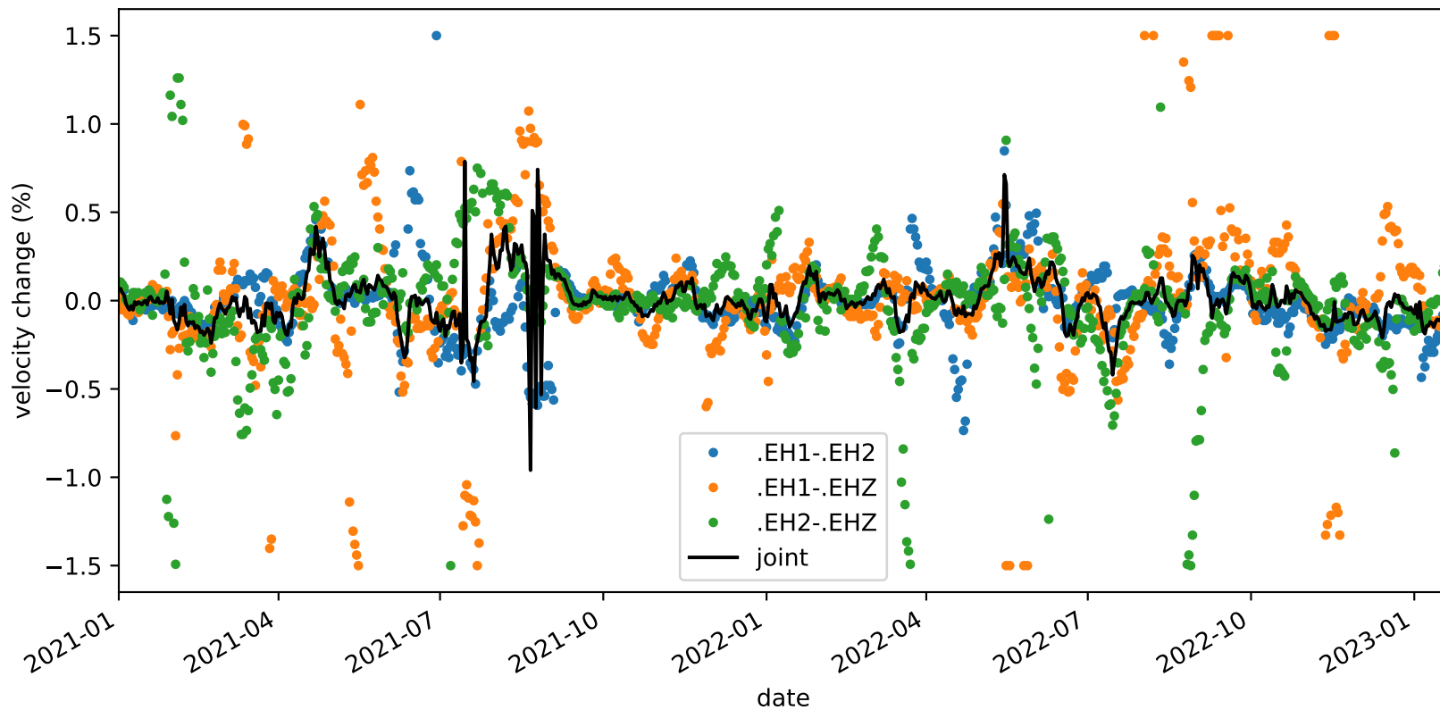
velocity_change_c1_s3_t1c_tw_005.0s-015.0s_PB.B932-PB.B932
