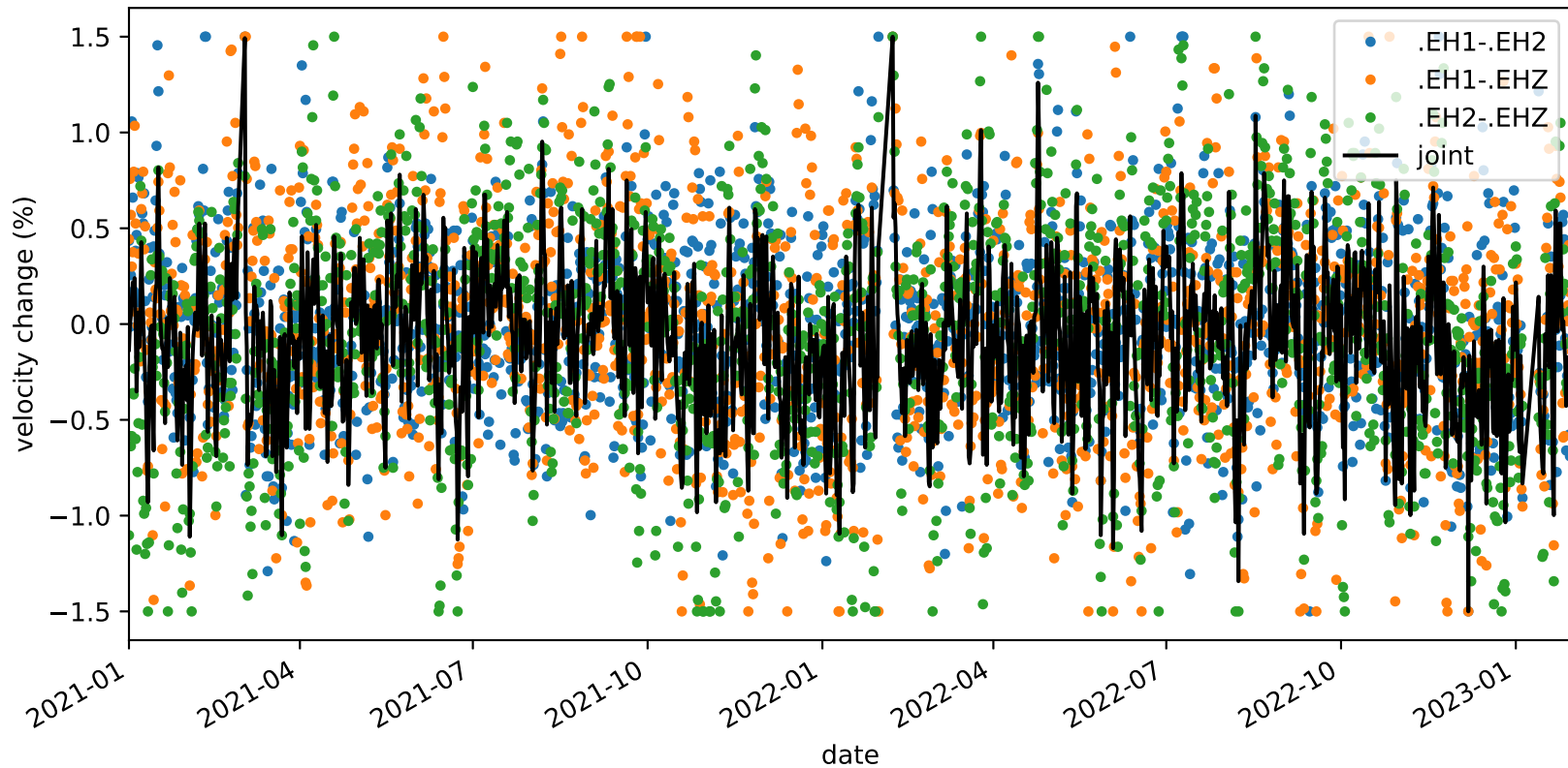
velocity_change_c1d_s1_t1a_tw_005.0s-010.0s_PB.B932-PB.B932
