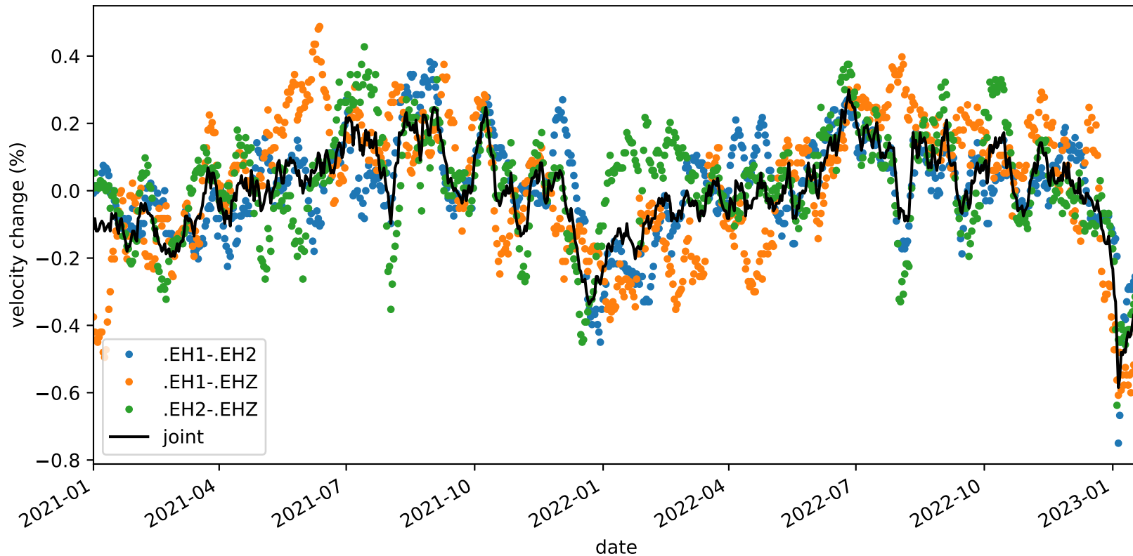
velocity_change_c1b_s3_t1a_tw_005.0s-010.0s_PB.B932-PB.B932
