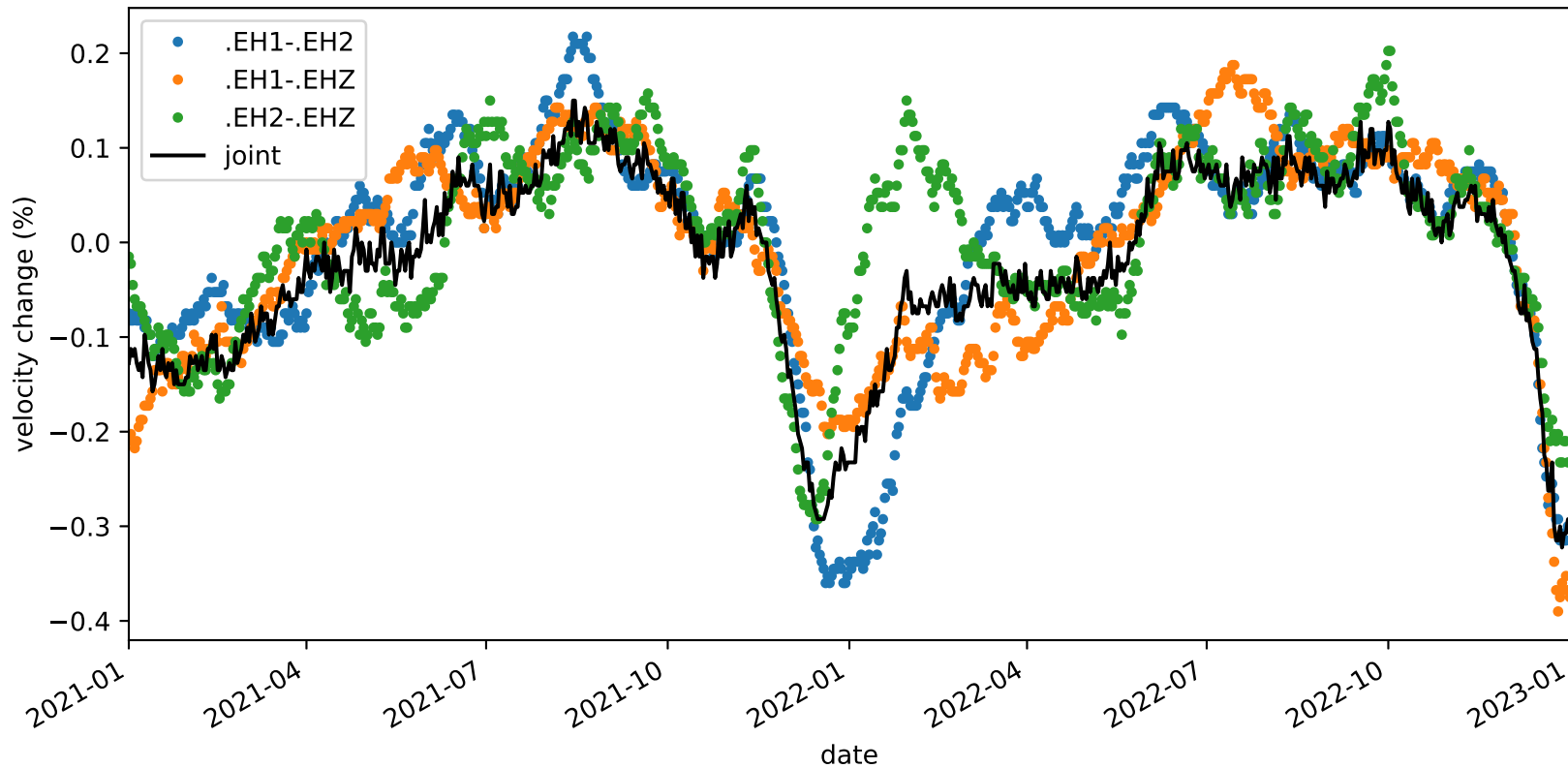
velocity_change_c1h_s2_t1a_tw_005.0s-010.0s_PB.B932-PB.B932
