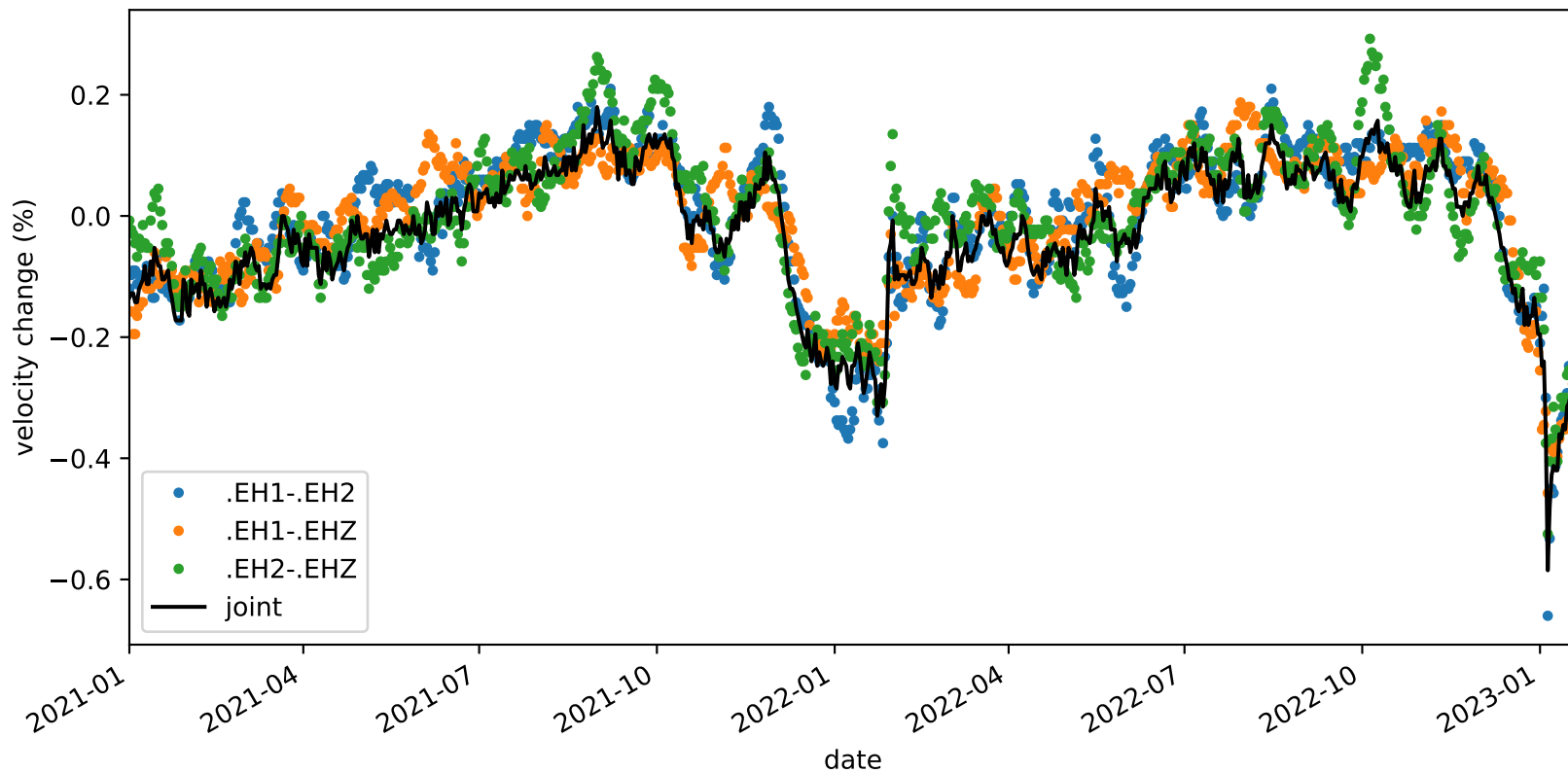
velocity_change_c1g_s3_t1c_tw_005.0s-015.0s_PB.B932-PB.B932
