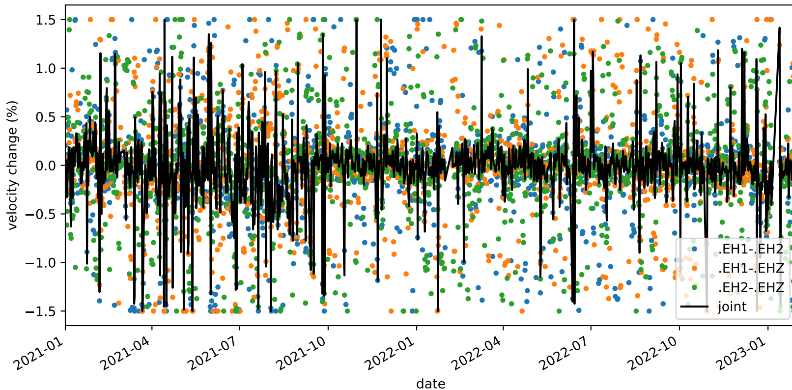
velocity_change_cli_s1_t1b_tw_010.0s-015.0s_PB.B932-PB.B932
