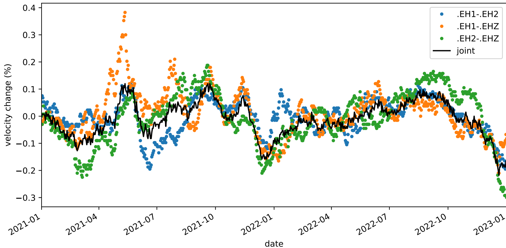
velocity_change_c1h_s2_t1b_tw_010.0s-015.0s_PB.B932-PB.B932
