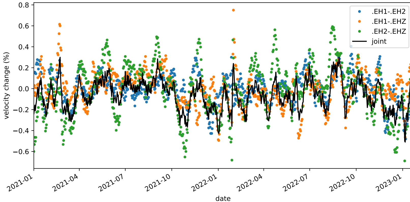
velocity_change_c1d_s3_t1c_tw_005.0s-015.0s_PB.B932-PB.B932
