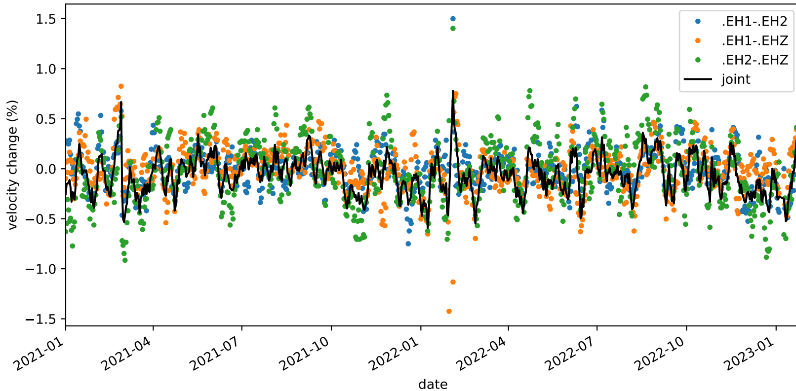
velocity_change_c1d_s4_t1c_tw_005.0s-015.0s_PB.B932-PB.B932
