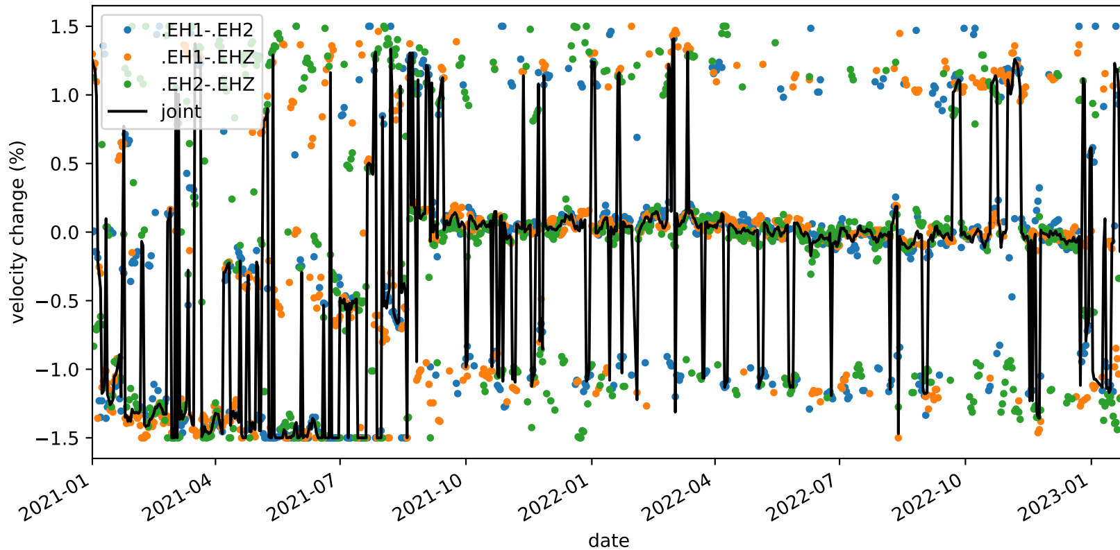
velocity_change_c1c_s4_t1b_tw_010.0s-015.0s_PB.B932-PB.B932
