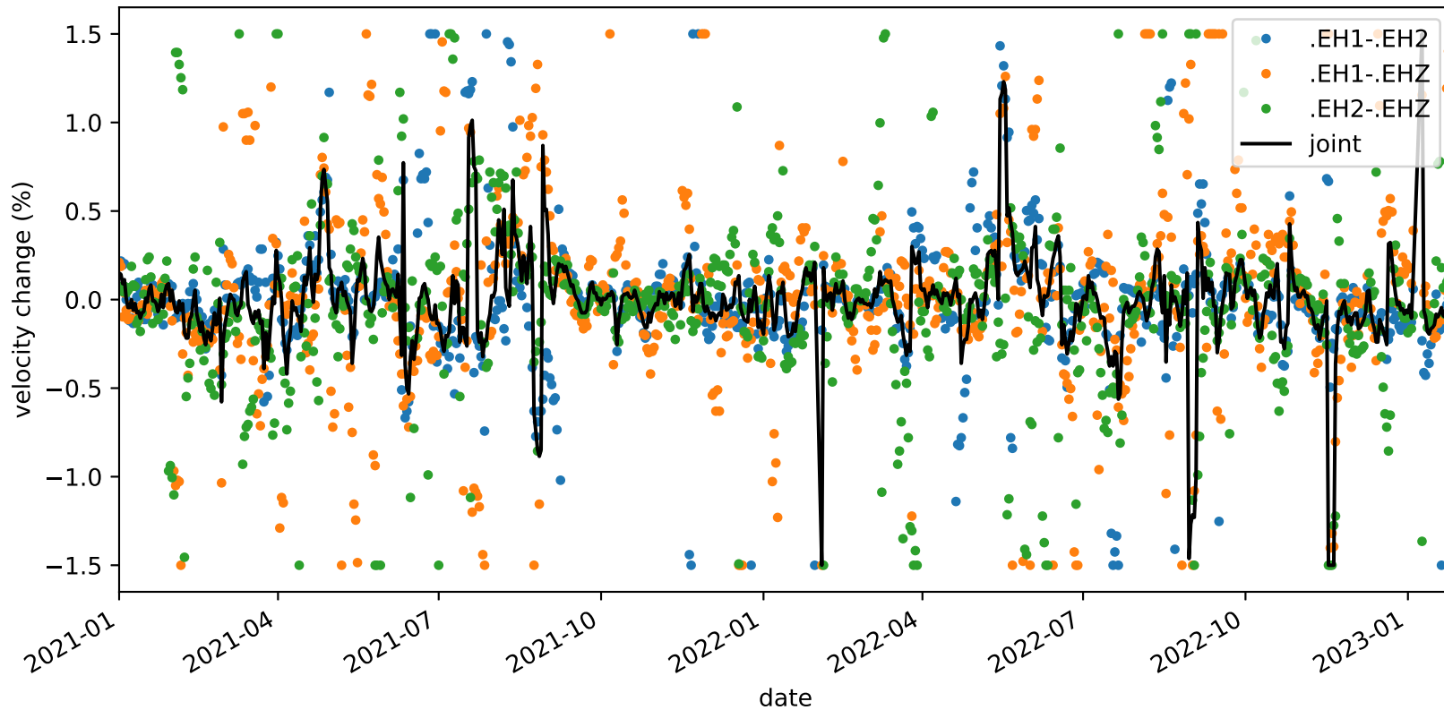
velocity_change_c1_s4_t1c_tw_005.0s-015.0s_PB.B932-PB.B932
