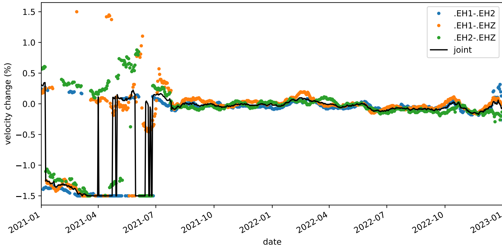
velocity_change_c1c_s2_t1a_tw_005.0s-010.0s_PB.B932-PB.B932
