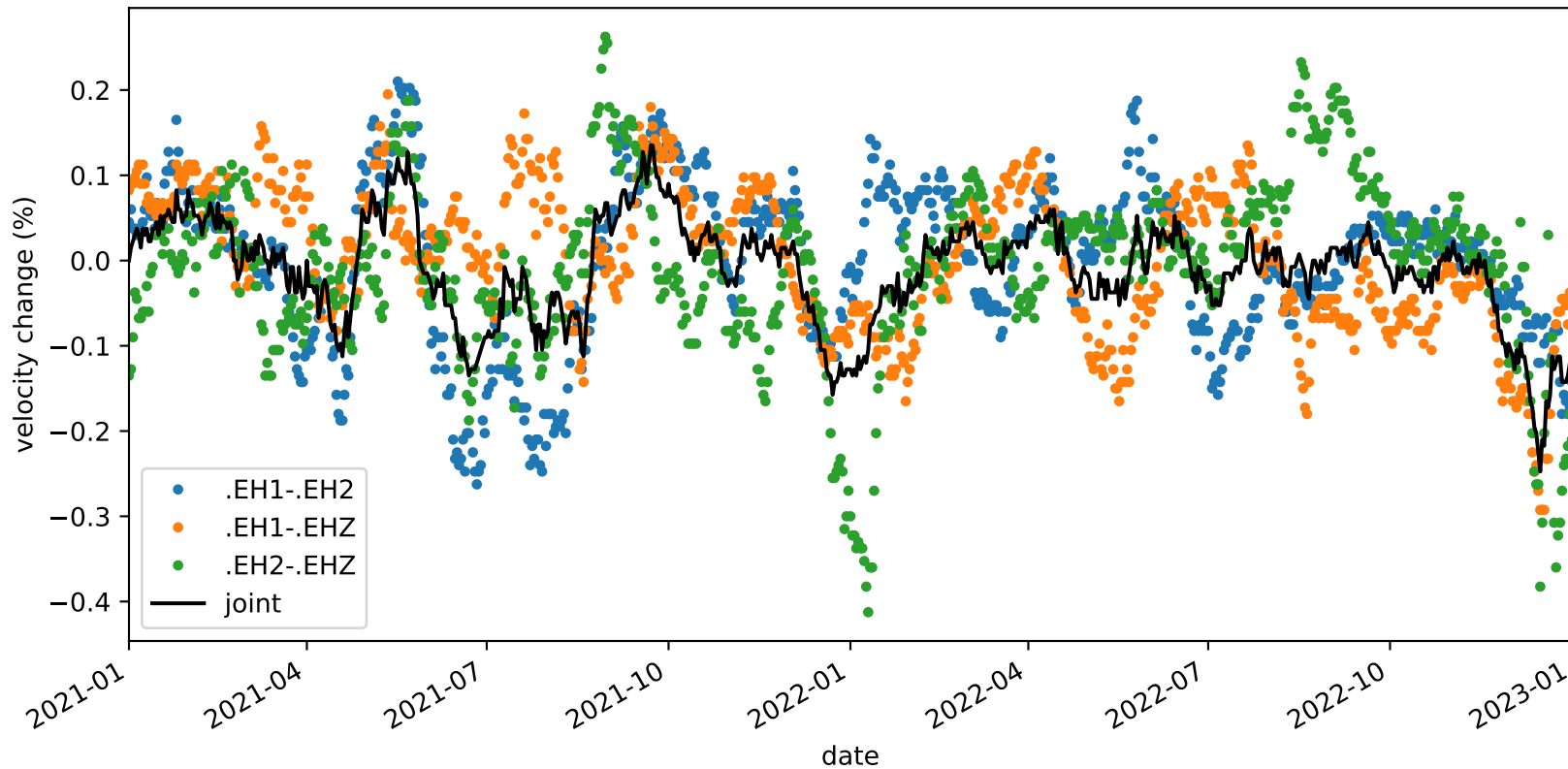
velocity_change_c1b_s2_t1b_tw_010.0s-015.0s_PB.B932-PB.B932
