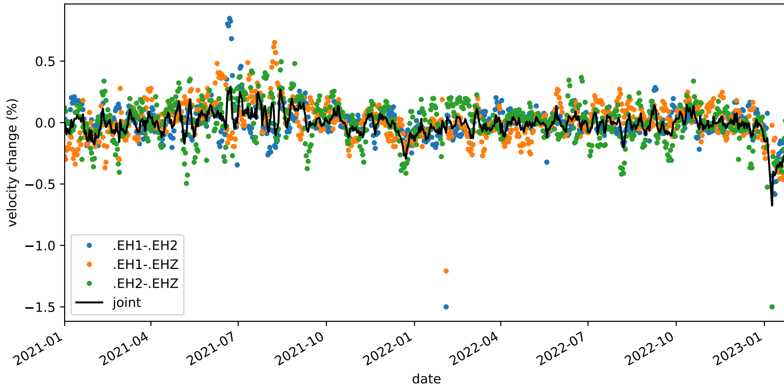
velocity_change_cli_s4_t1a_tw_005.0s-010.0s_PB.B932-PB.B932
