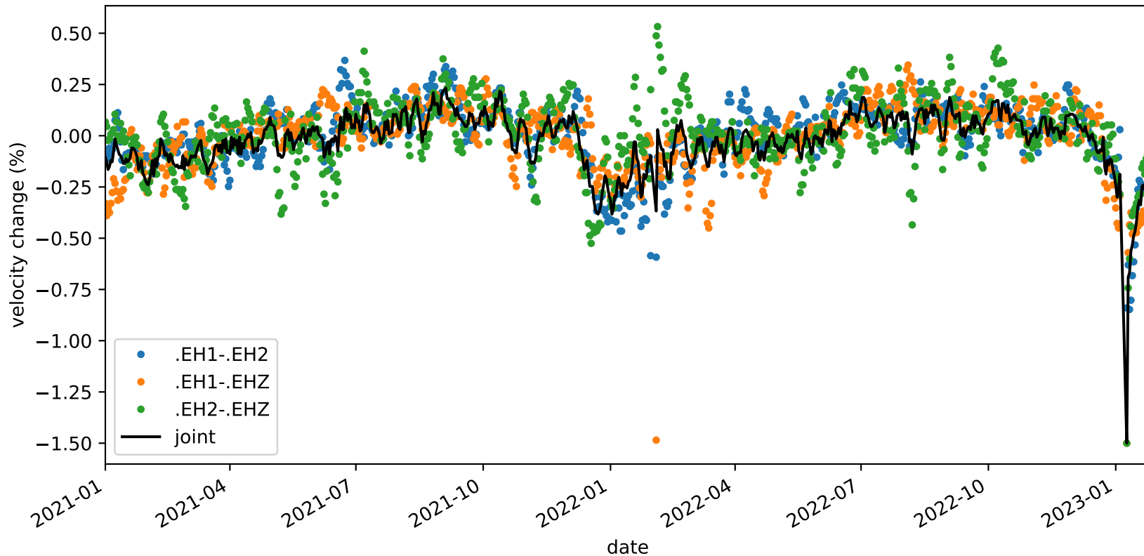
velocity_change_c1h_s4_t1a_tw_005.0s-010.0s_PB.B932-PB.B932
