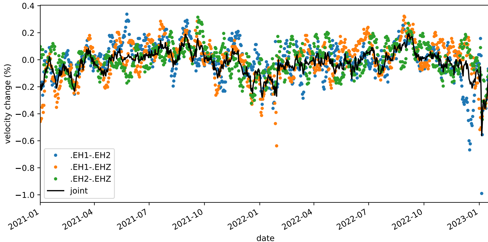
velocity_change_c1e_s3_t1b_tw_010.0s-015.0s_PB.B932-PB.B932
