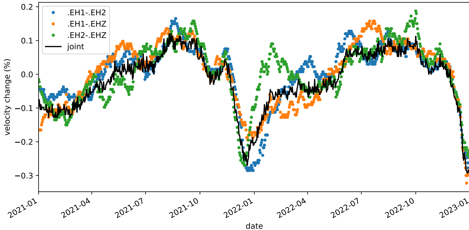
velocity_change_c1h_s2_t1c_tw_005.0s-015.0s_PB.B932-PB.B932
