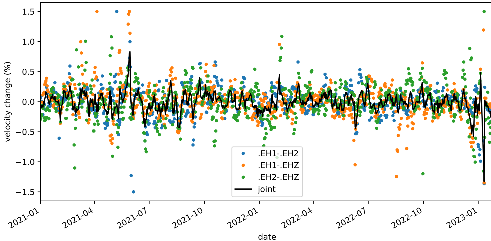
velocity_change_c1b_s4_t1b_tw_010.0s-015.0s_PB.B932-PB.B932
