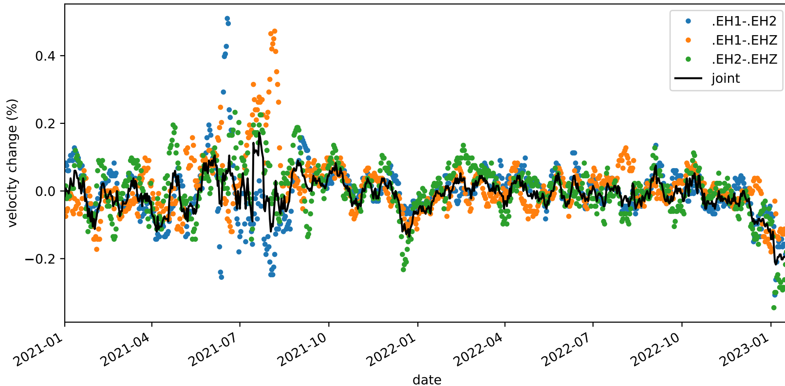
velocity_change_c1i_s3_t1c_tw_005.0s-015.0s_PB.B932-PB.B932
