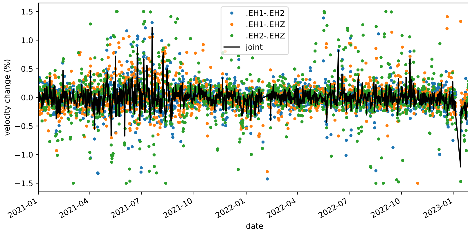
velocity_change_cli_s1_t1c_tw_005.0s-015.0s_PB.B932-PB.B932
