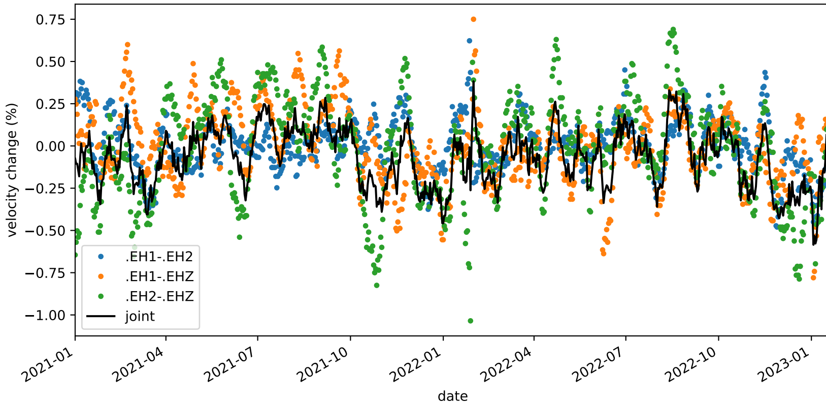
velocity_change_c1d_s3_t1a_tw_005.0s-010.0s_PB.B932-PB.B932
