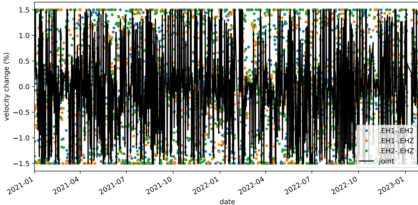
velocity_change_c1_s1_t1b_tw_010.0s-015.0s_PB.B932-PB.B932
