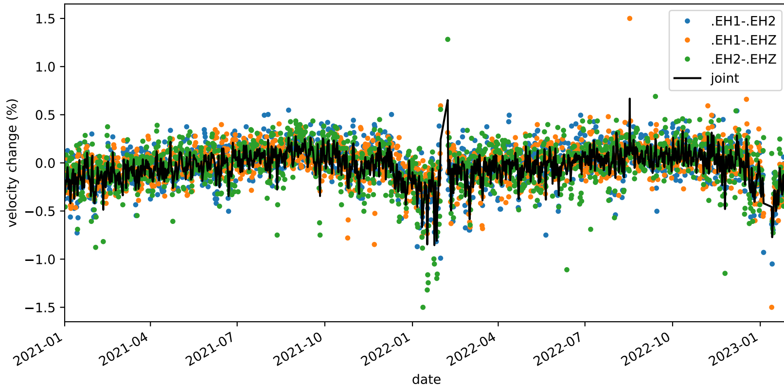
velocity_change_c1f_s1_t1c_tw_005.0s-015.0s_PB.B932-PB.B932
