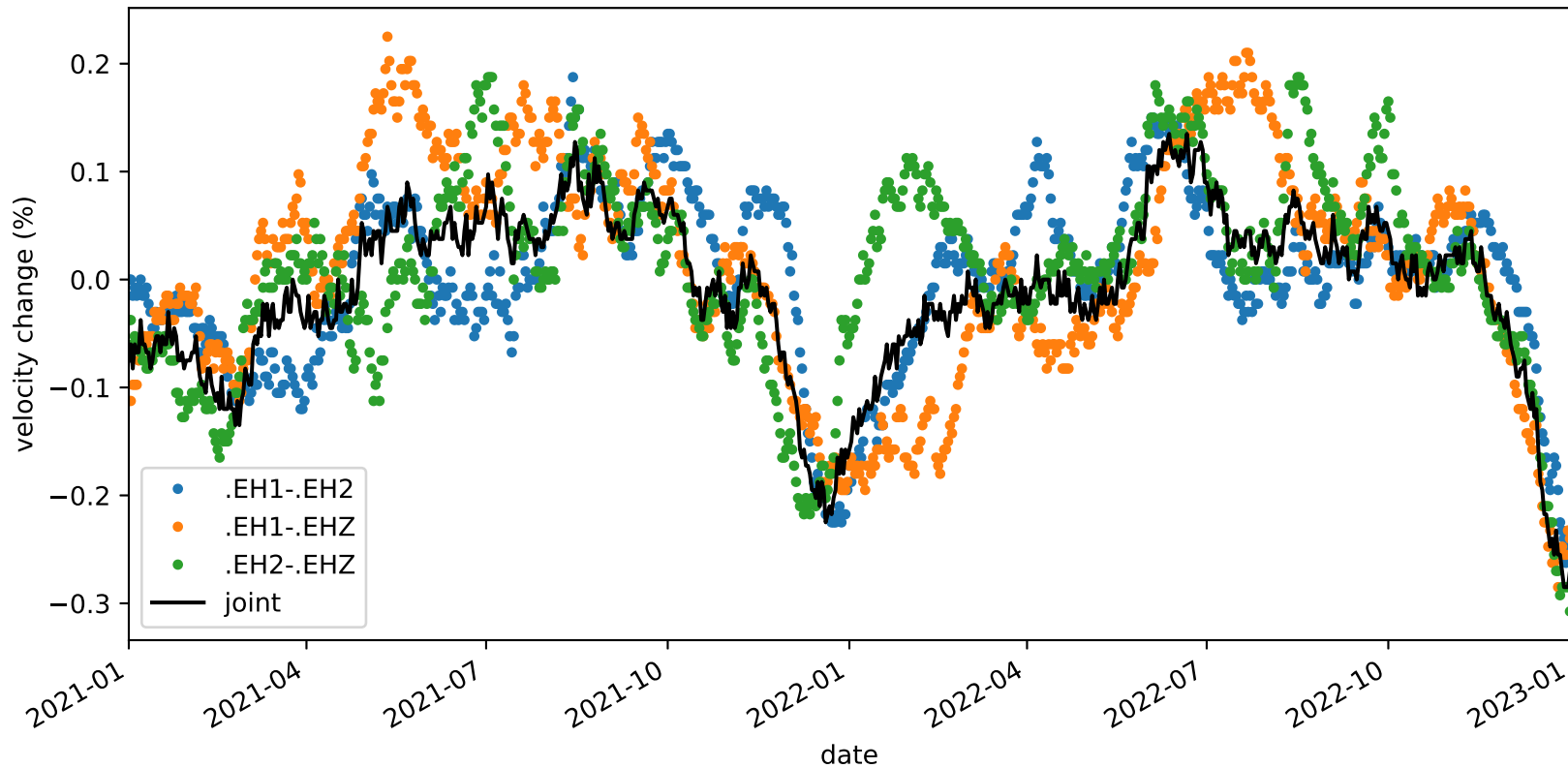
velocity_change_c1b_s2_t1c_tw_005.0s-015.0s_PB.B932-PB.B932
