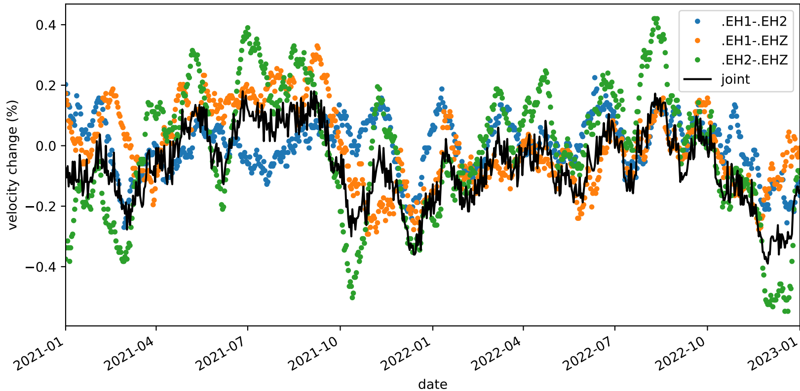
velocity_change_c1d_s2_t1a_tw_005.0s-010.0s_PB.B932-PB.B932
