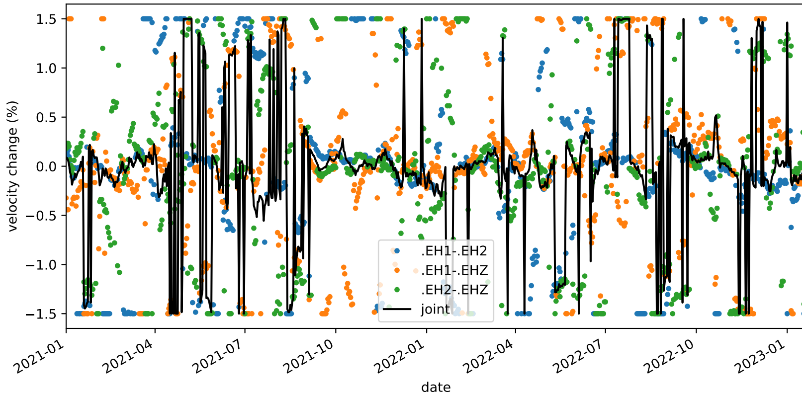
velocity_change_c1_s3_t1b_tw_010.0s-015.0s_PB.B932-PB.B932
