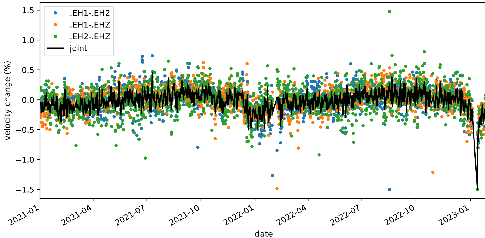
velocity_change_c1h_s1_t1c_tw_005.0s-015.0s_PB.B932-PB.B932
