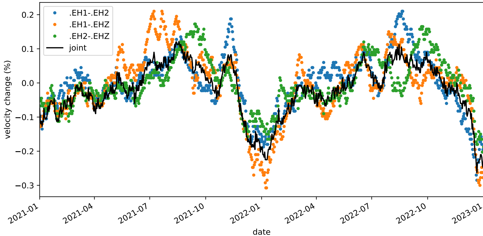
velocity_change_c1f_s2_t1b_tw_010.0s-015.0s_PB.B932-PB.B932
