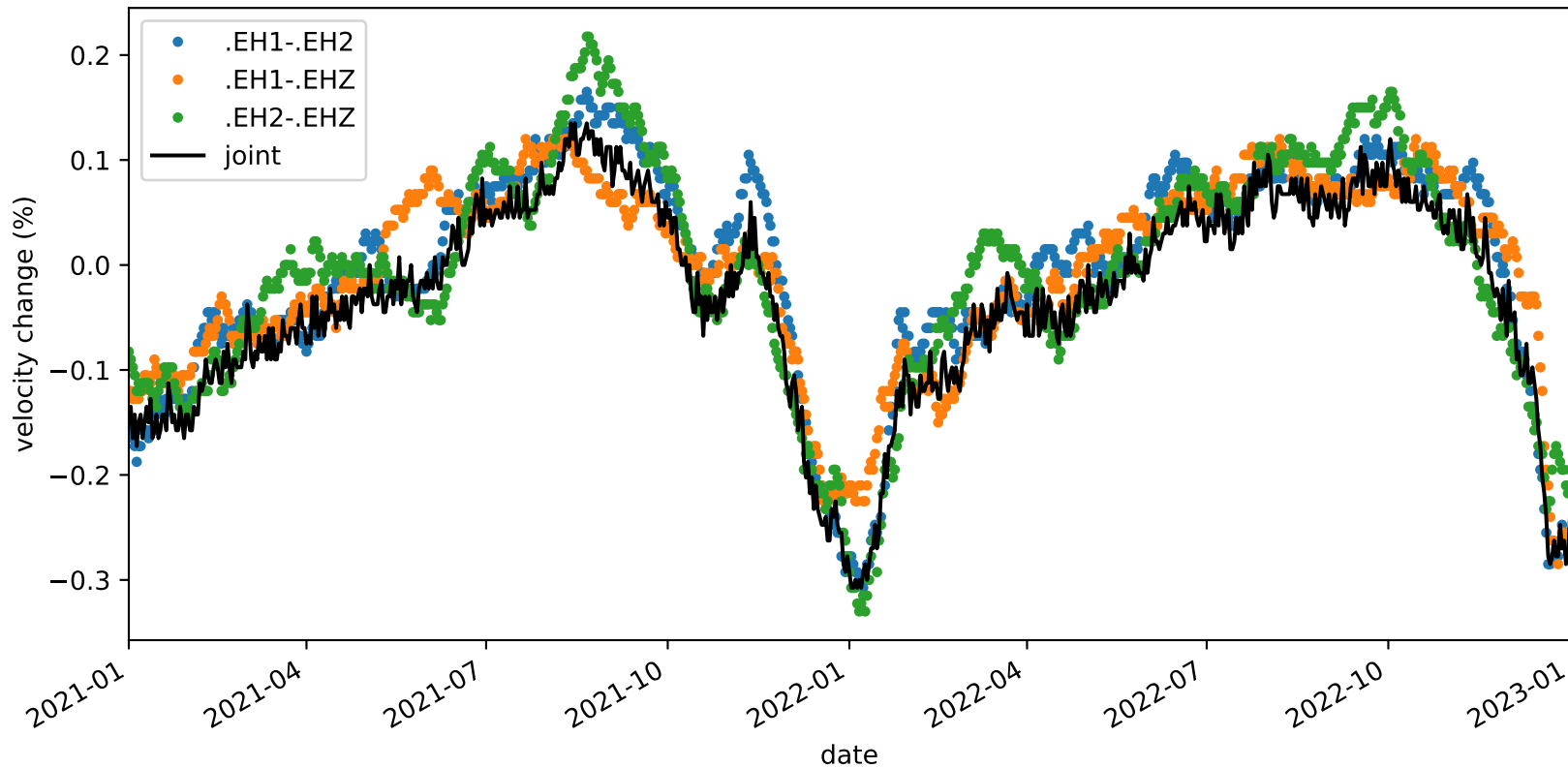
velocity_change_c1f_s2_t1c_tw_005.0s-015.0s_PB.B932-PB.B932
