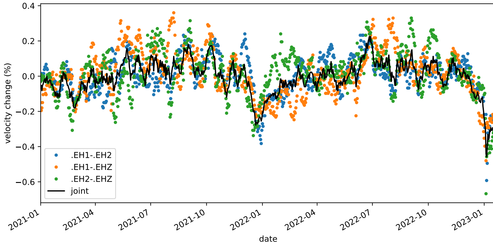
velocity_change_c1b_s3_t1c_tw_005.0s-015.0s_PB.B932-PB.B932
