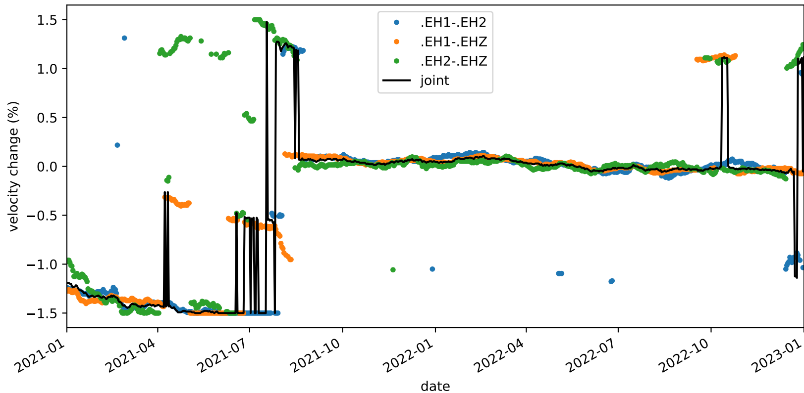
velocity_change_c1c_s2_t1b_tw_010.0s-015.0s_PB.B932-PB.B932
