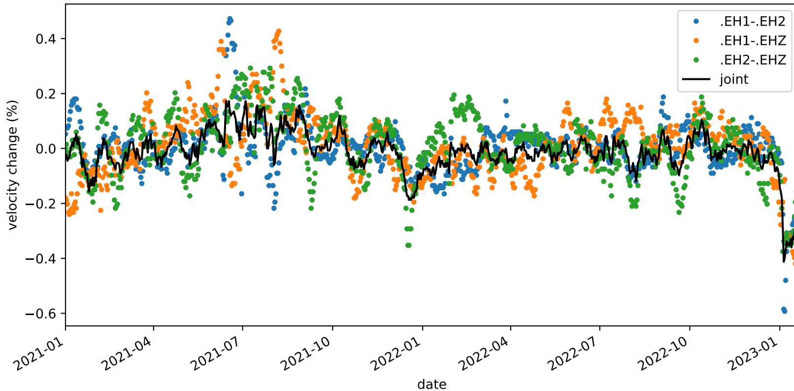
velocity_change_c1i_s3_t1a_tw_005.0s-010.0s_PB.B932-PB.B932
