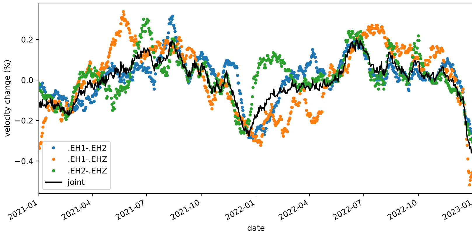
velocity_change_c1b_s2_t1a_tw_005.0s-010.0s_PB.B932-PB.B932
