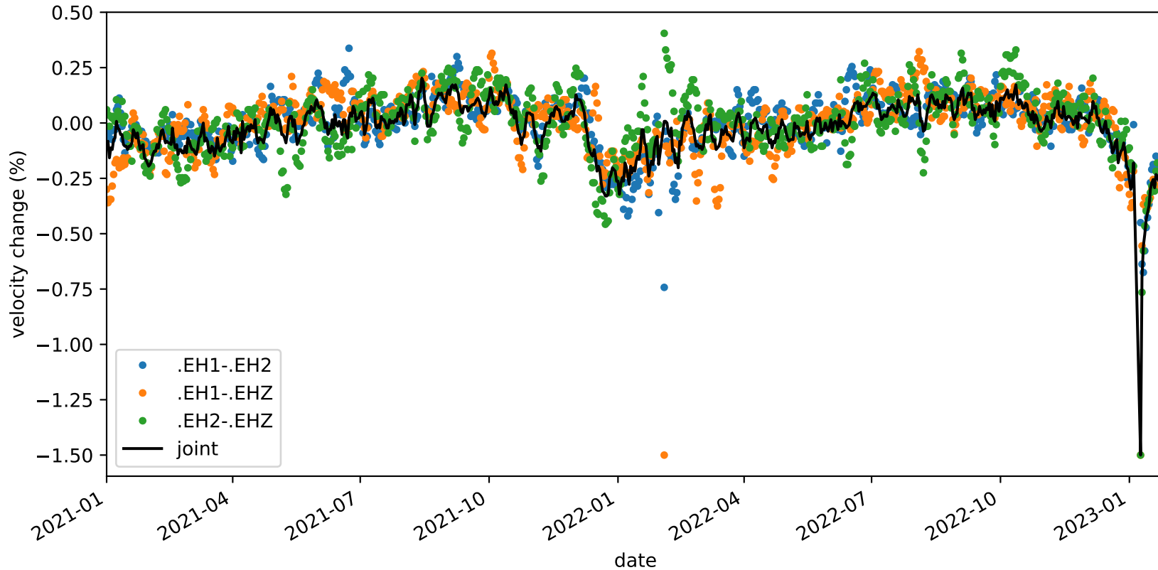
velocity_change_c1h_s4_t1c_tw_005.0s-015.0s_PB.B932-PB.B932
