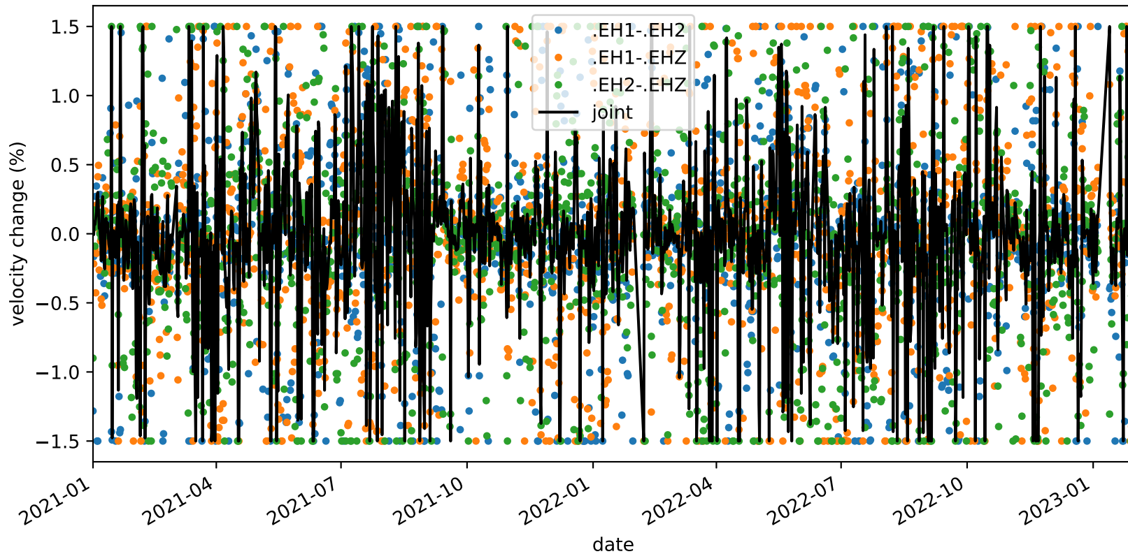
velocity_change_c1_s1_t1c_tw_005.0s-015.0s_PB.B932-PB.B932
