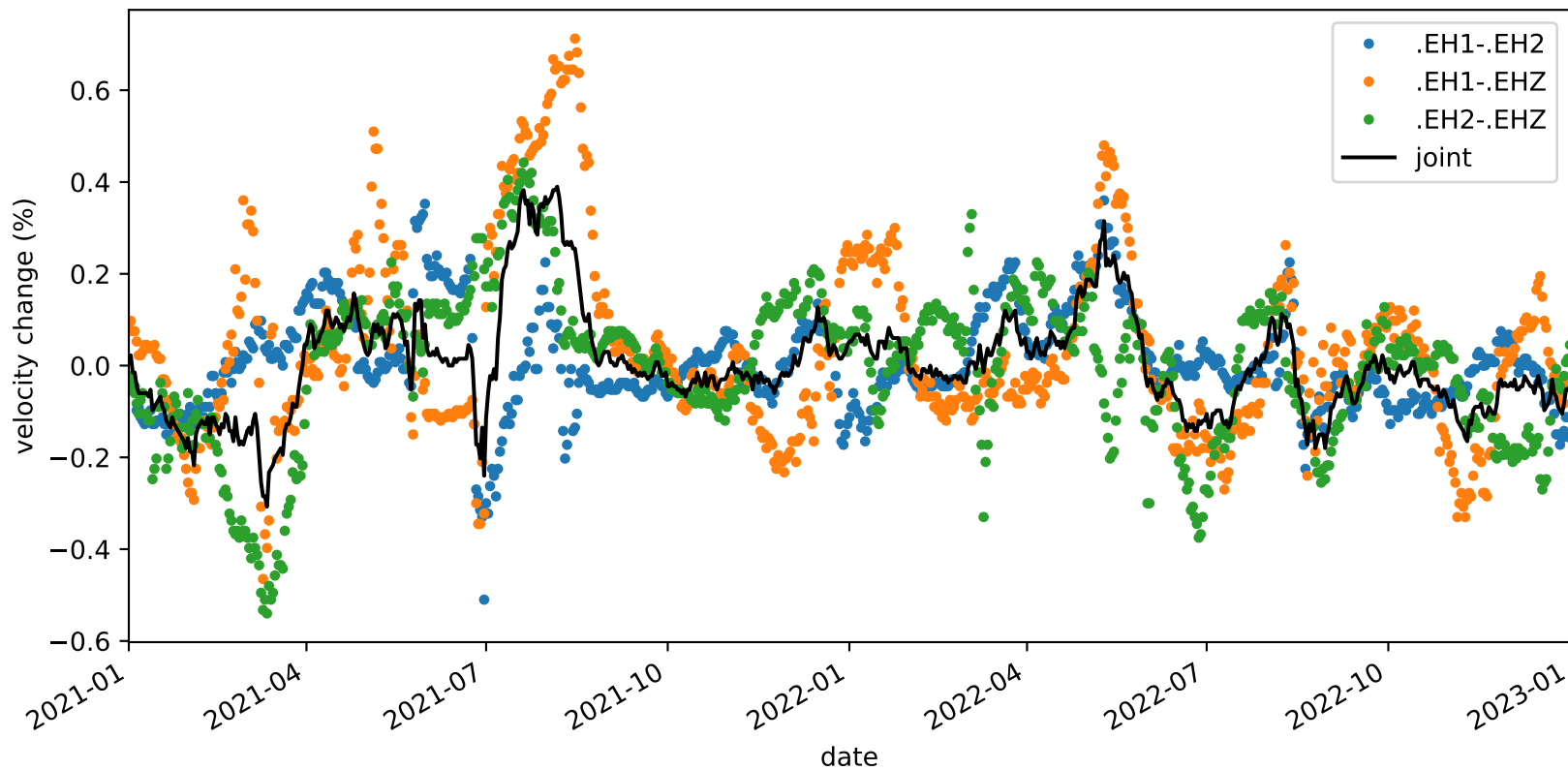
velocity_change_c1_s2_t1a_tw_005.0s-010.0s_PB.B932-PB.B932
