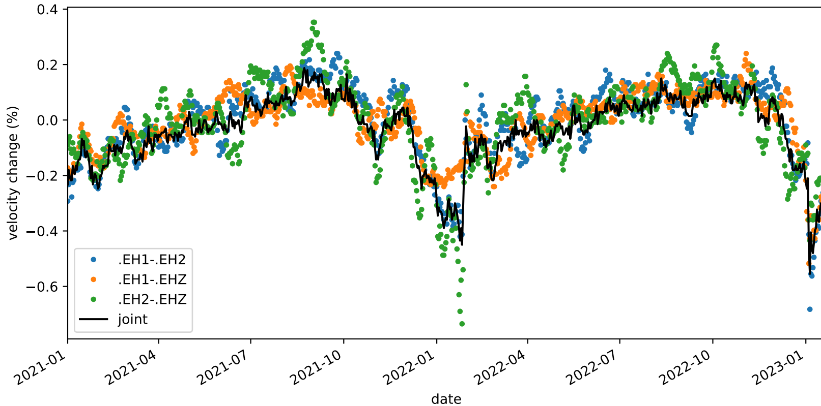
velocity_change_c1f_s3_t1a_tw_005.0s-010.0s_PB.B932-PB.B932
