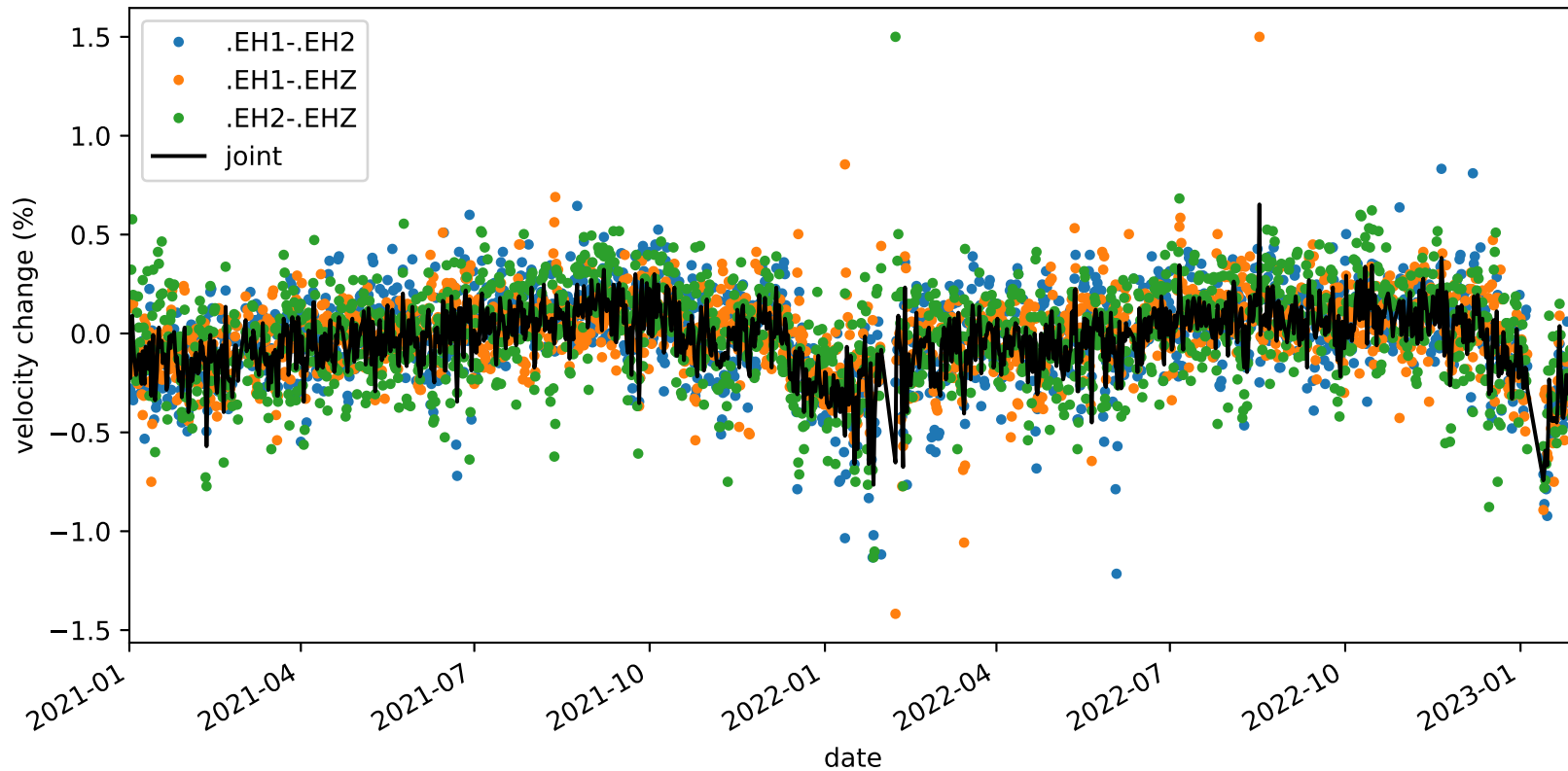
velocity_change_c1g_s1_t1a_tw_005.0s-010.0s_PB.B932-PB.B932
