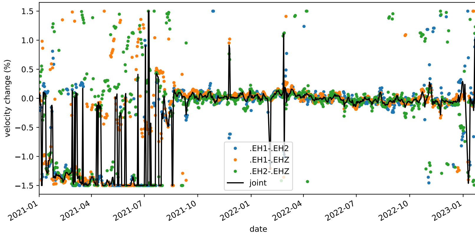
velocity_change_c1c_s4_t1c_tw_005.0s-015.0s_PB.B932-PB.B932
