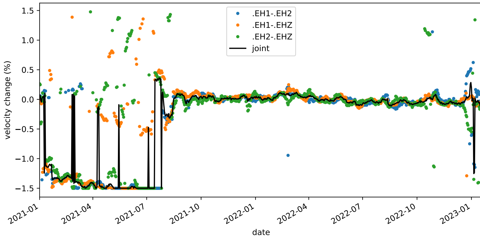
velocity_change_c1c_s3_t1c_tw_005.0s-015.0s_PB.B932-PB.B932
