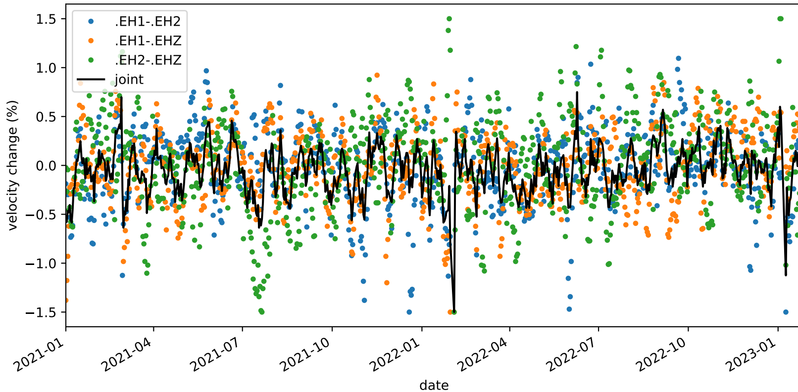
velocity_change_c1d_s4_t1b_tw_010.0s-015.0s_PB.B932-PB.B932
