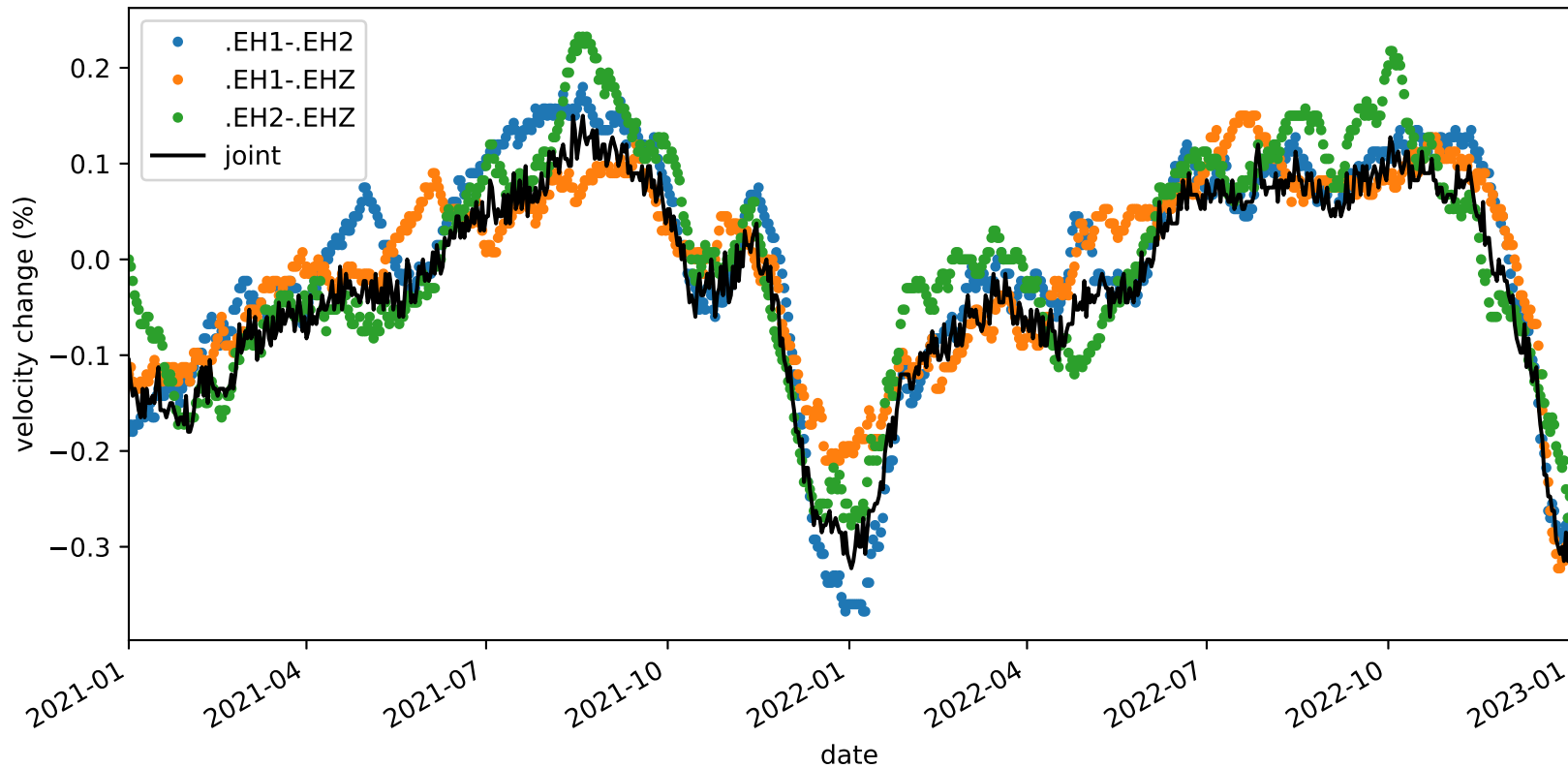
velocity_change_c1g_s2_t1a_tw_005.0s-010.0s_PB.B932-PB.B932
