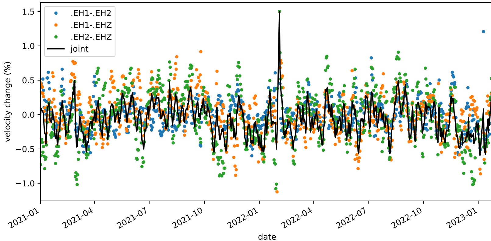
velocity_change_c1d_s4_t1a_tw_005.0s-010.0s_PB.B932-PB.B932
