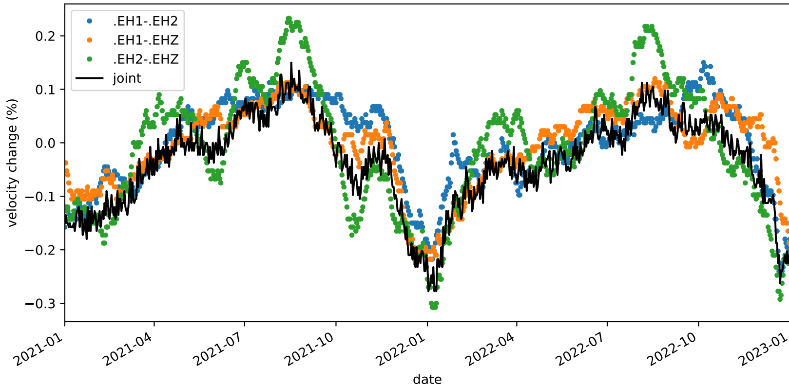
velocity_change_c1e_s2_t1c_tw_005.0s-015.0s_PB.B932-PB.B932
