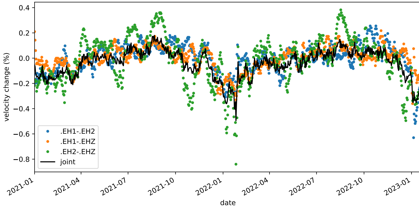
velocity_change_c1e_s3_t1a_tw_005.0s-010.0s_PB.B932-PB.B932
