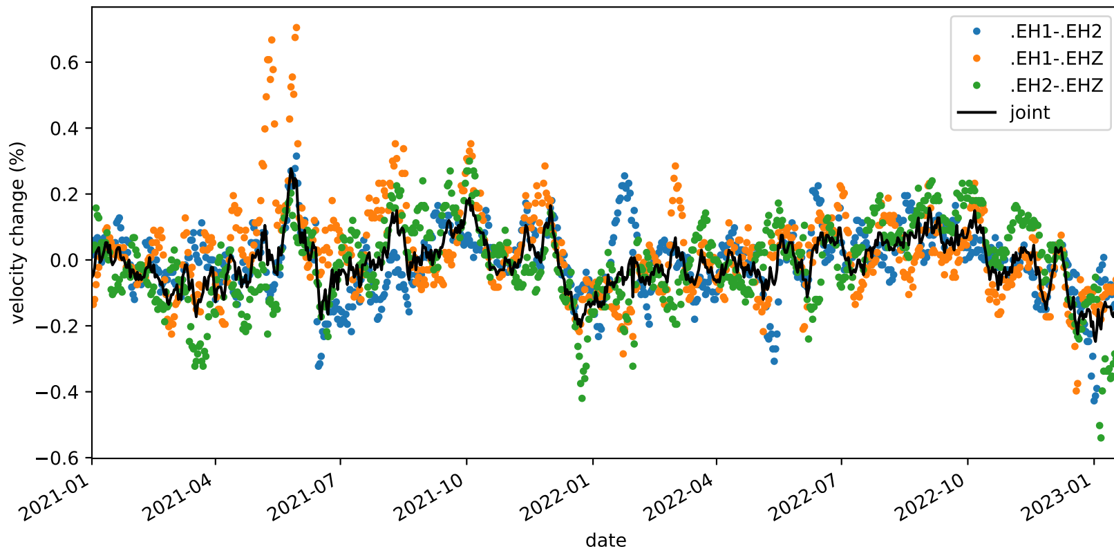
velocity_change_c1h_s3_t1b_tw_010.0s-015.0s_PB.B932-PB.B932
