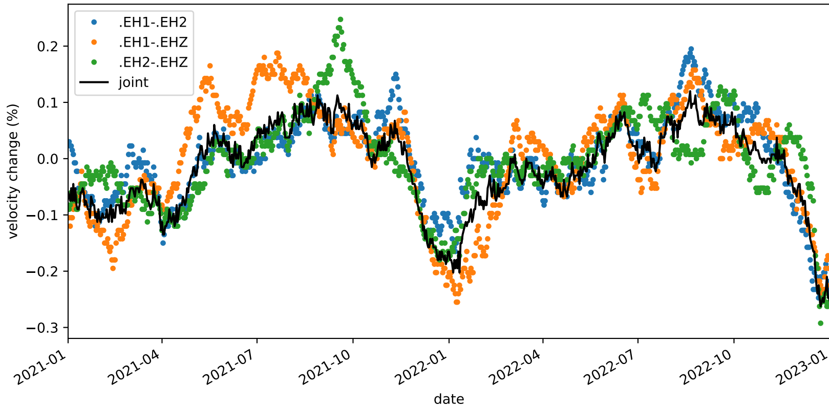
velocity_change_c1g_s2_t1b_tw_010.0s-015.0s_PB.B932-PB.B932
