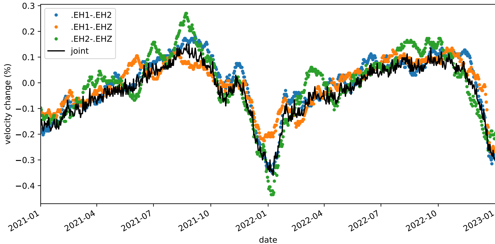
velocity_change_c1f_s2_t1a_tw_005.0s-010.0s_PB.B932-PB.B932
