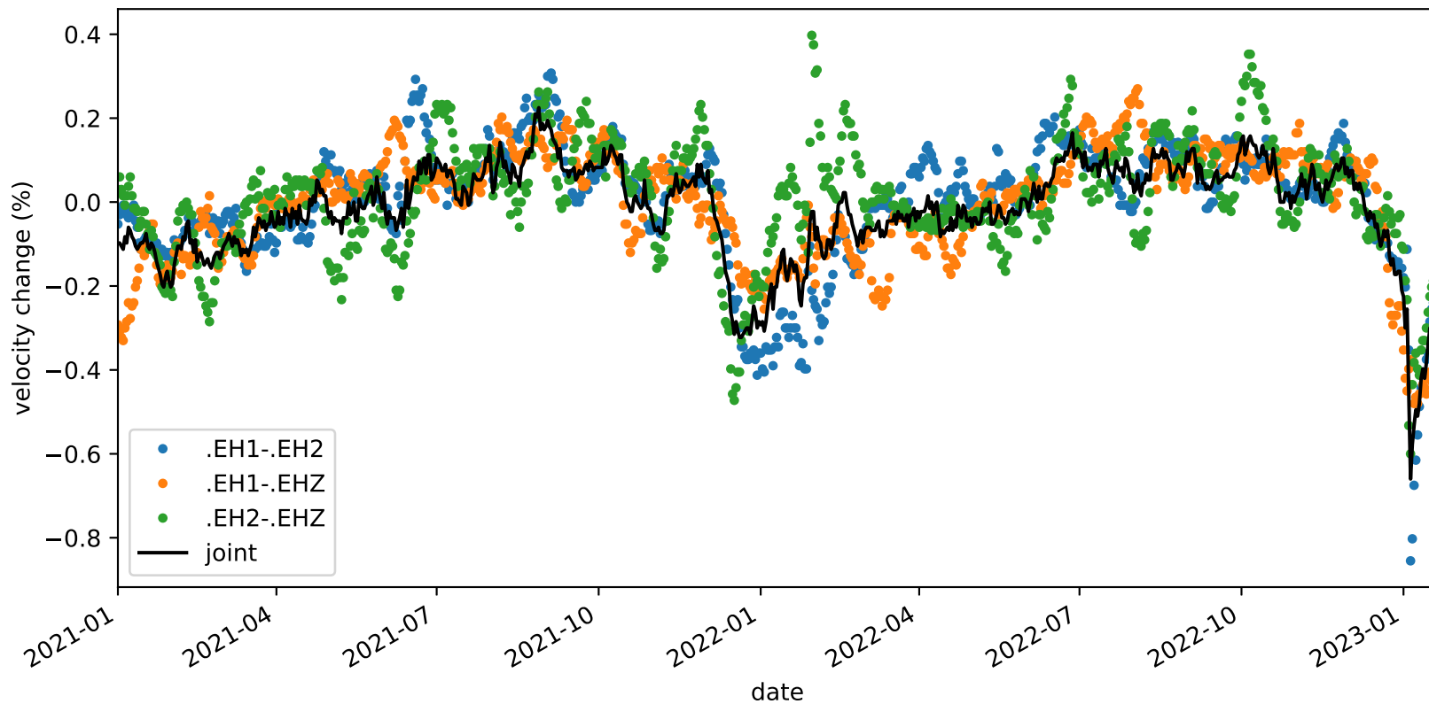
velocity_change_c1h_s3_t1a_tw_005.0s-010.0s_PB.B932-PB.B932
