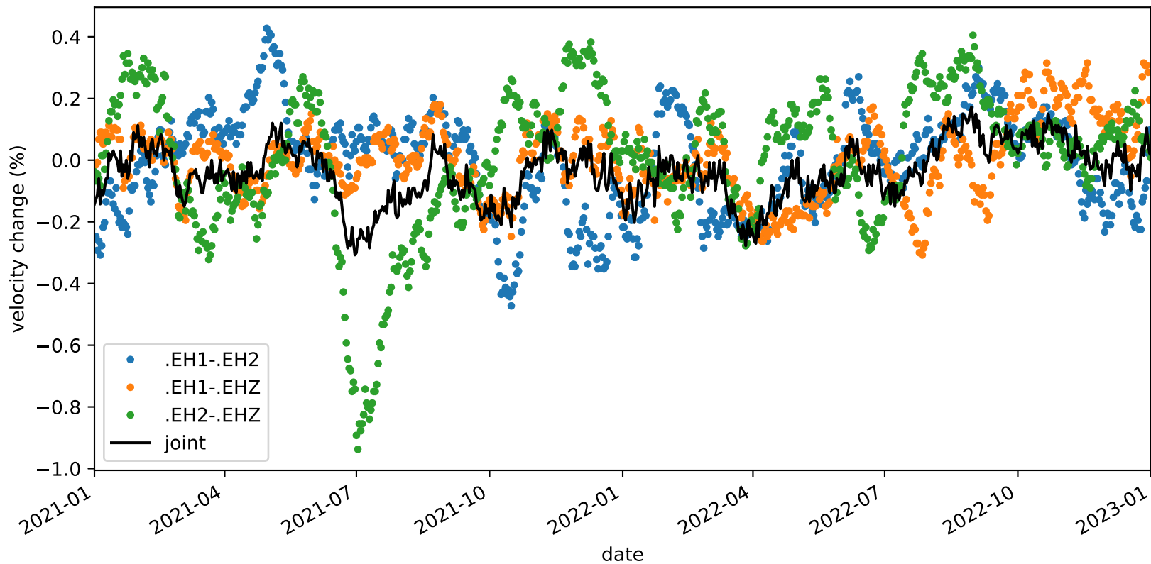
velocity_change_c1d_s2_t1b_tw_010.0s-015.0s_PB.B932-PB.B932
