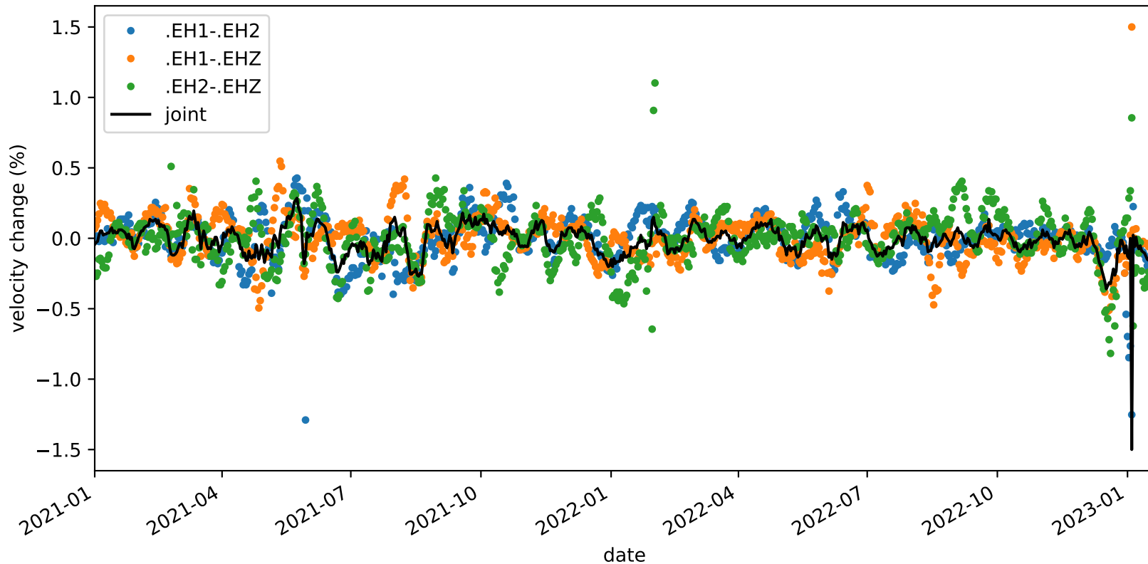
velocity_change_c1b_s3_t1b_tw_010.0s-015.0s_PB.B932-PB.B932
