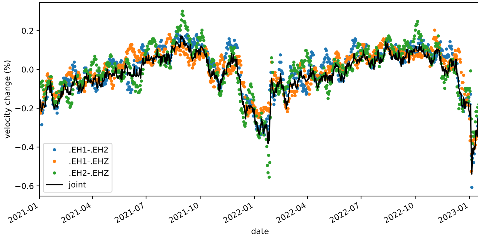
velocity_change_c1f_s3_t1c_tw_005.0s-015.0s_PB.B932-PB.B932
