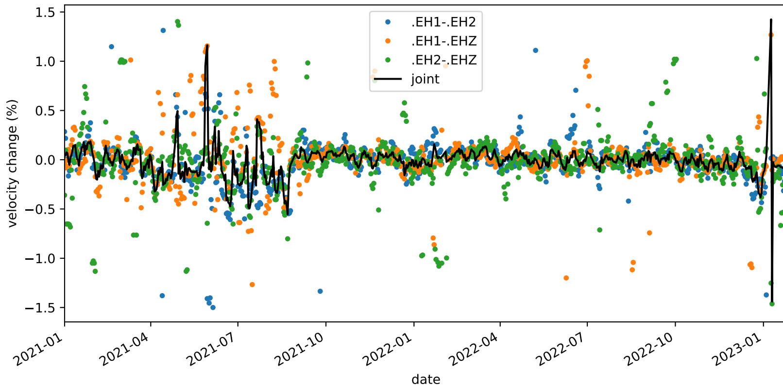
velocity_change_cli_s4_t1b_tw_010.0s-015.0s_PB.B932-PB.B932
