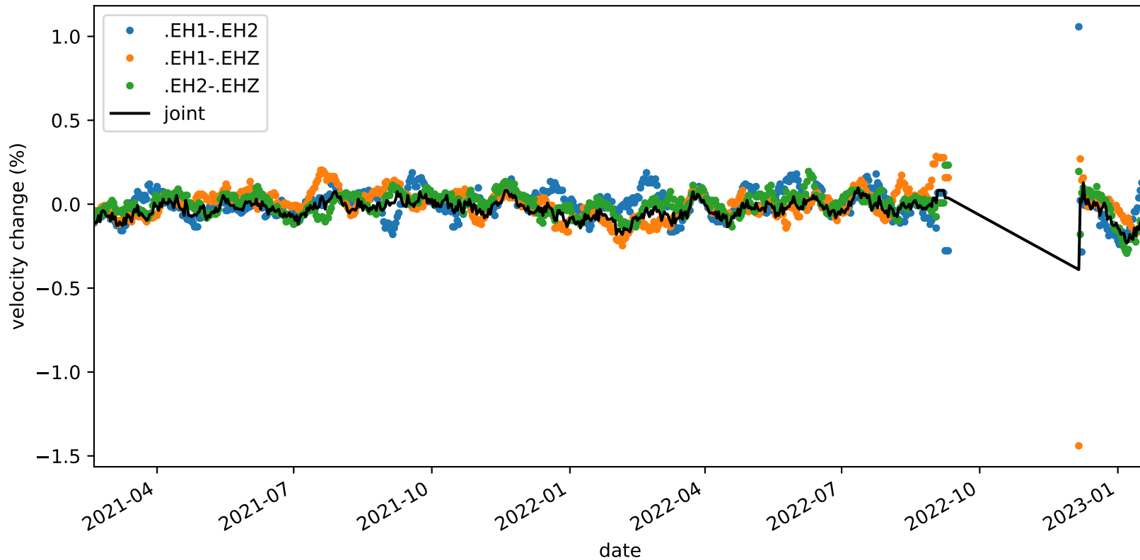
velocity_change_c1e_s3_t1c_tw_005.0s-015.0s_PB.B047-PB.B047
