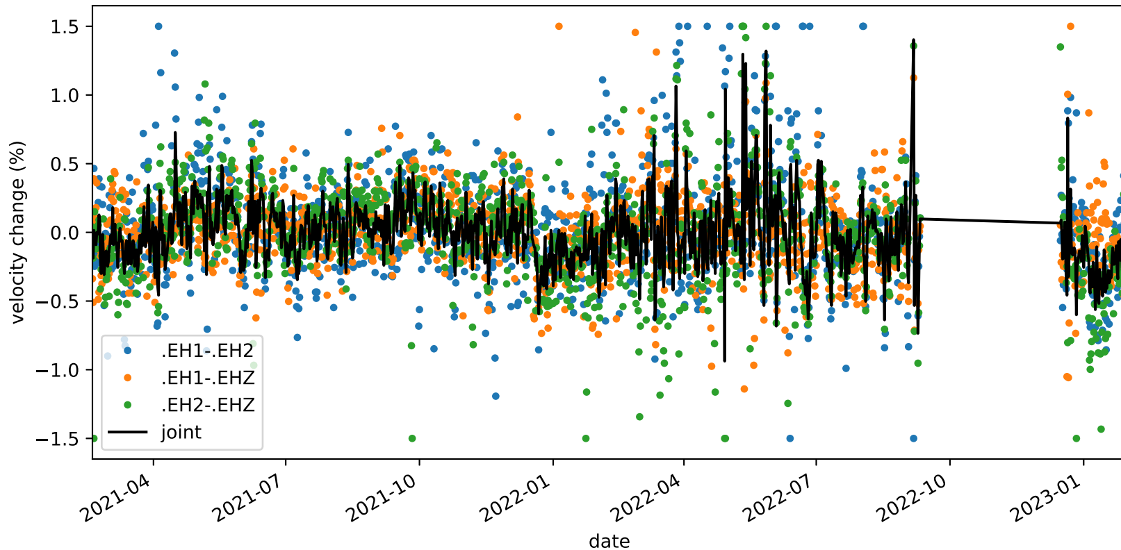
velocity_change_c1h_s1_t1a_tw_005.0s-010.0s_PB.B047-PB.B047
