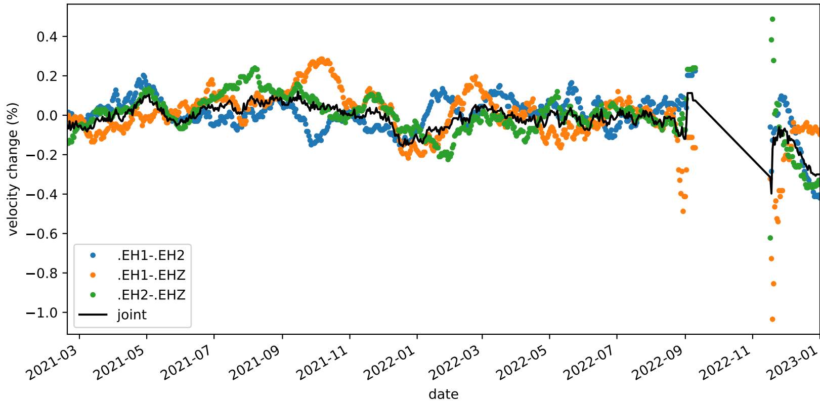
velocity_change_c1b_s2_t1a_tw_005.0s-010.0s_PB.B047-PB.B047
