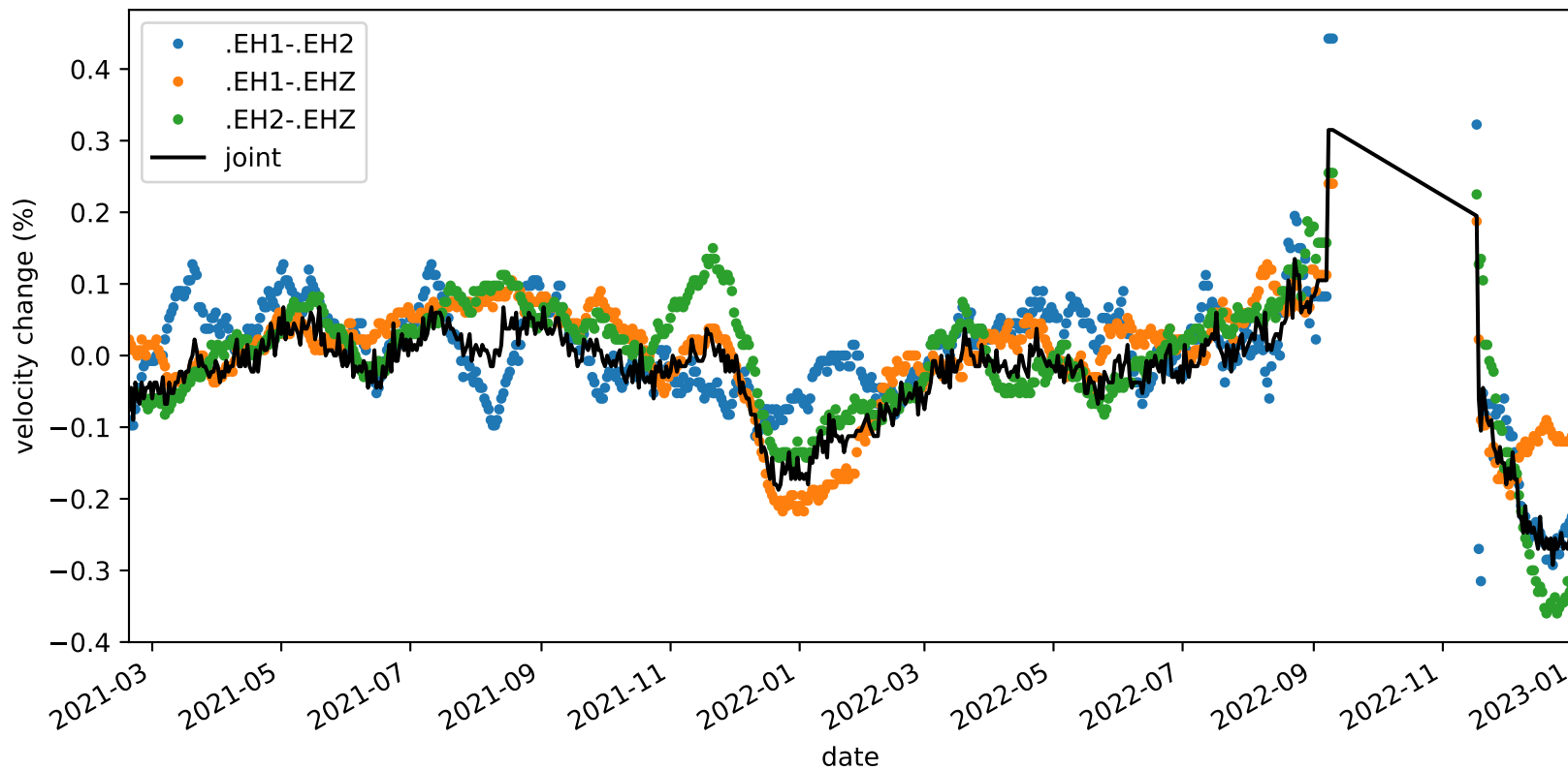
velocity_change_c1g_s2_t1a_tw_005.0s-010.0s_PB.B047-PB.B047
