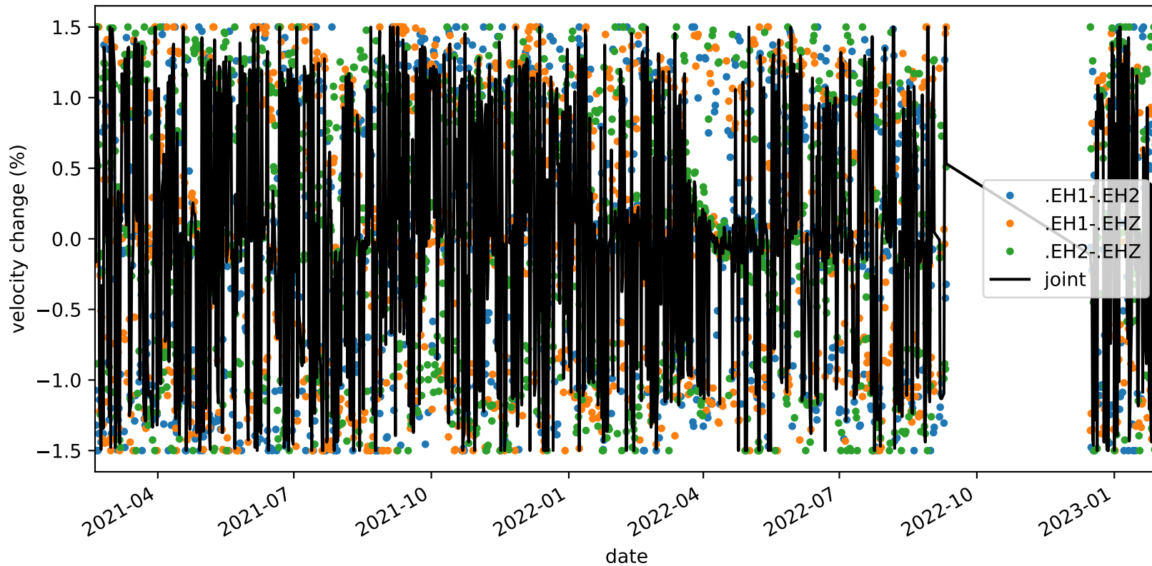
velocity_change_c1c_s1_t1b_tw_010.0s-015.0s_PB.B047-PB.B047
