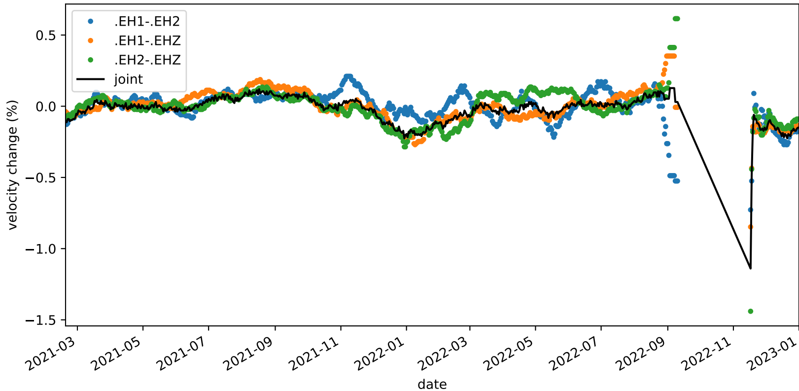
velocity_change_c1f_s2_t1b_tw_010.0s-015.0s_PB.B047-PB.B047
