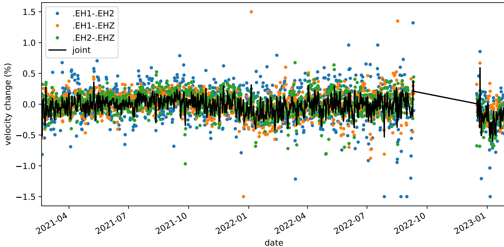
velocity_change_c1g_s1_t1c_tw_005.0s-015.0s_PB.B047-PB.B047
