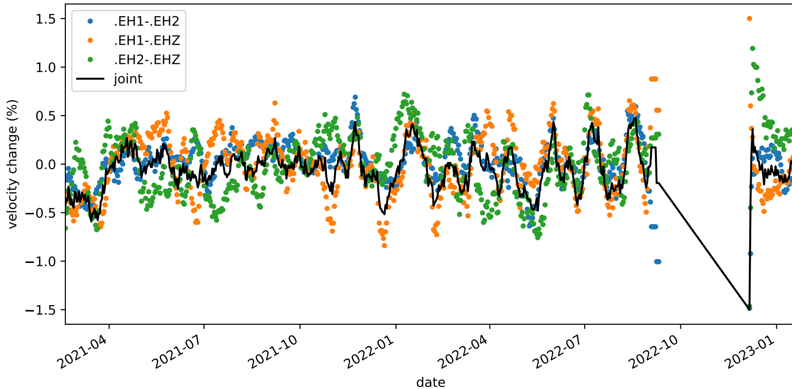
velocity_change_c1d_s3_t1a_tw_005.0s-010.0s_PB.B047-PB.B047
