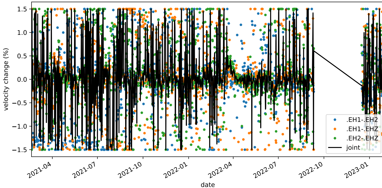
velocity_change_c1c_s1_t1c_tw_005.0s-015.0s_PB.B047-PB.B047
