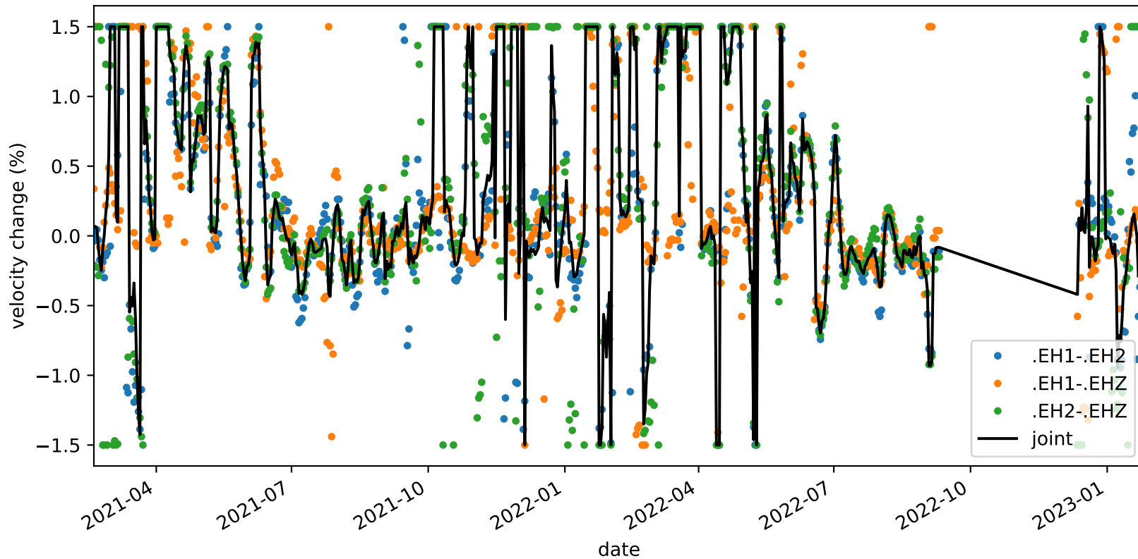
velocity_change_c1_s4_t1c_tw_005.0s-015.0s_PB.B047-PB.B047
