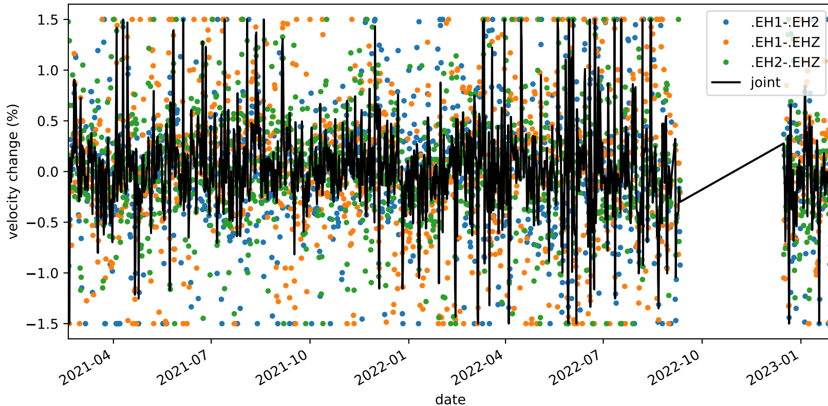
velocity_change_c1b_s1_t1b_tw_010.0s-015.0s_PB.B047-PB.B047
