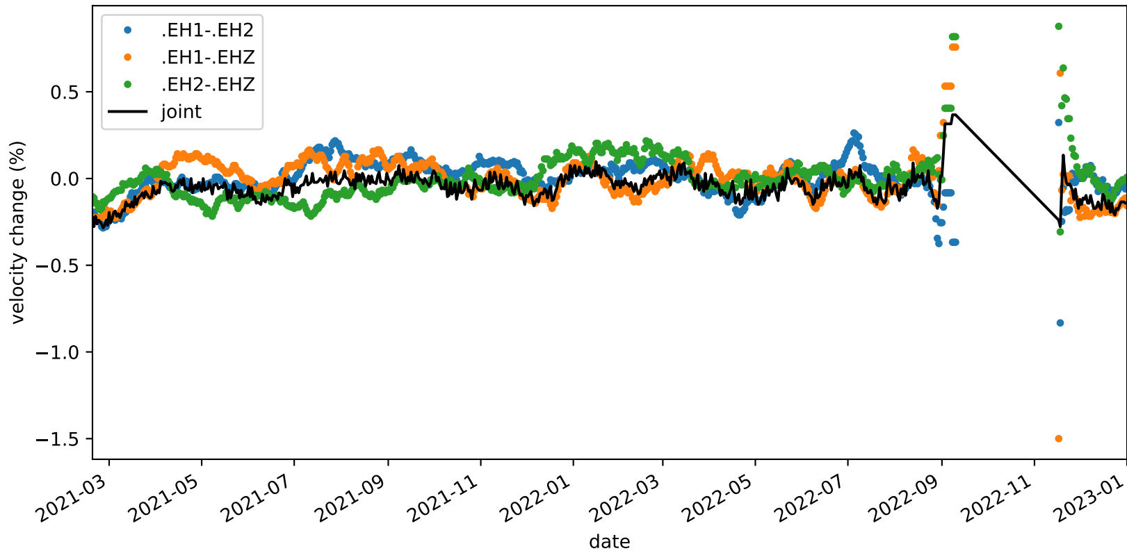
velocity_change_c1d_s2_t1c_tw_005.0s-015.0s_PB.B047-PB.B047
