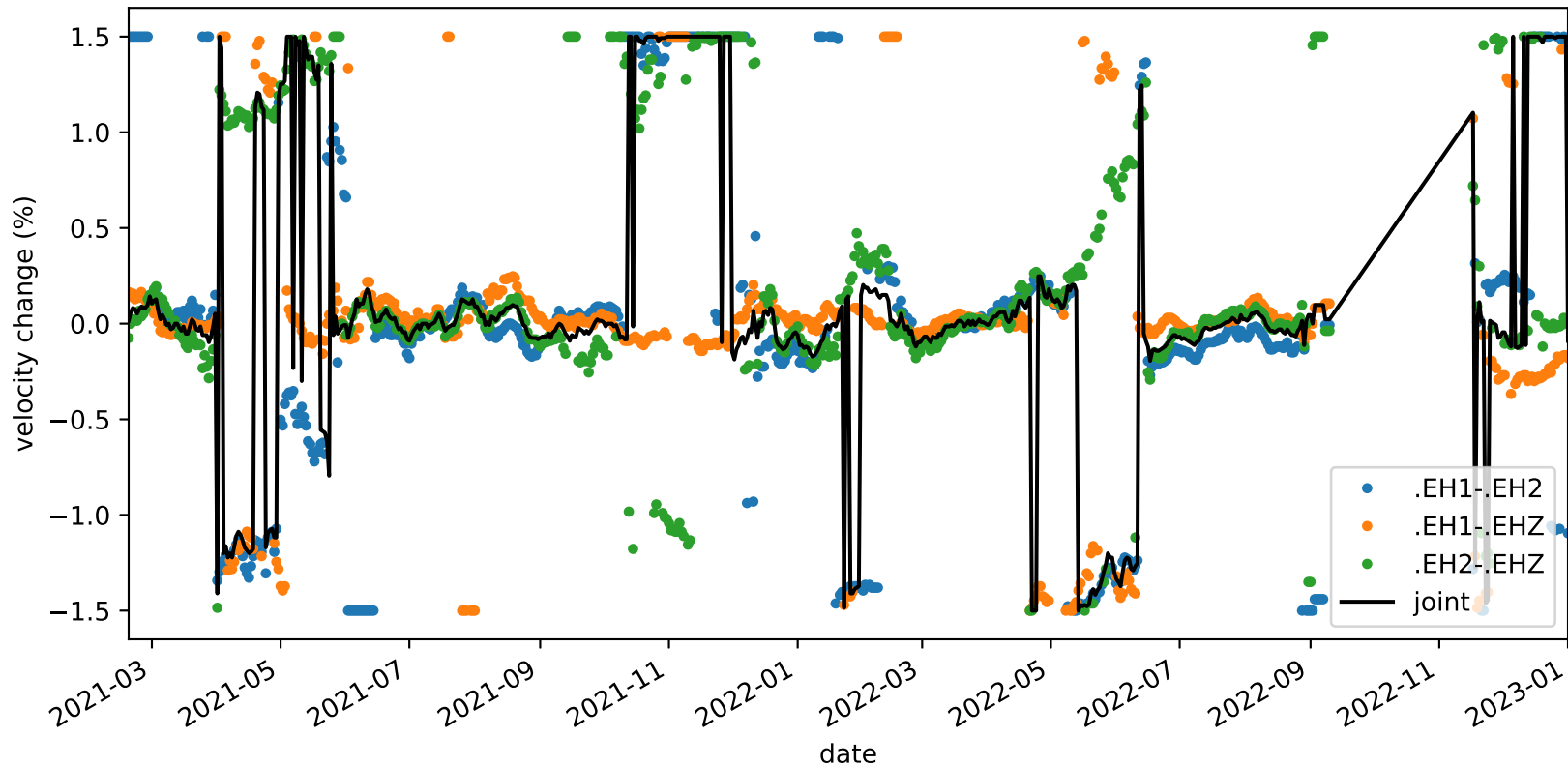
velocity_change_c1_s2_t1b_tw_010.0s-015.0s_PB.B047-PB.B047
