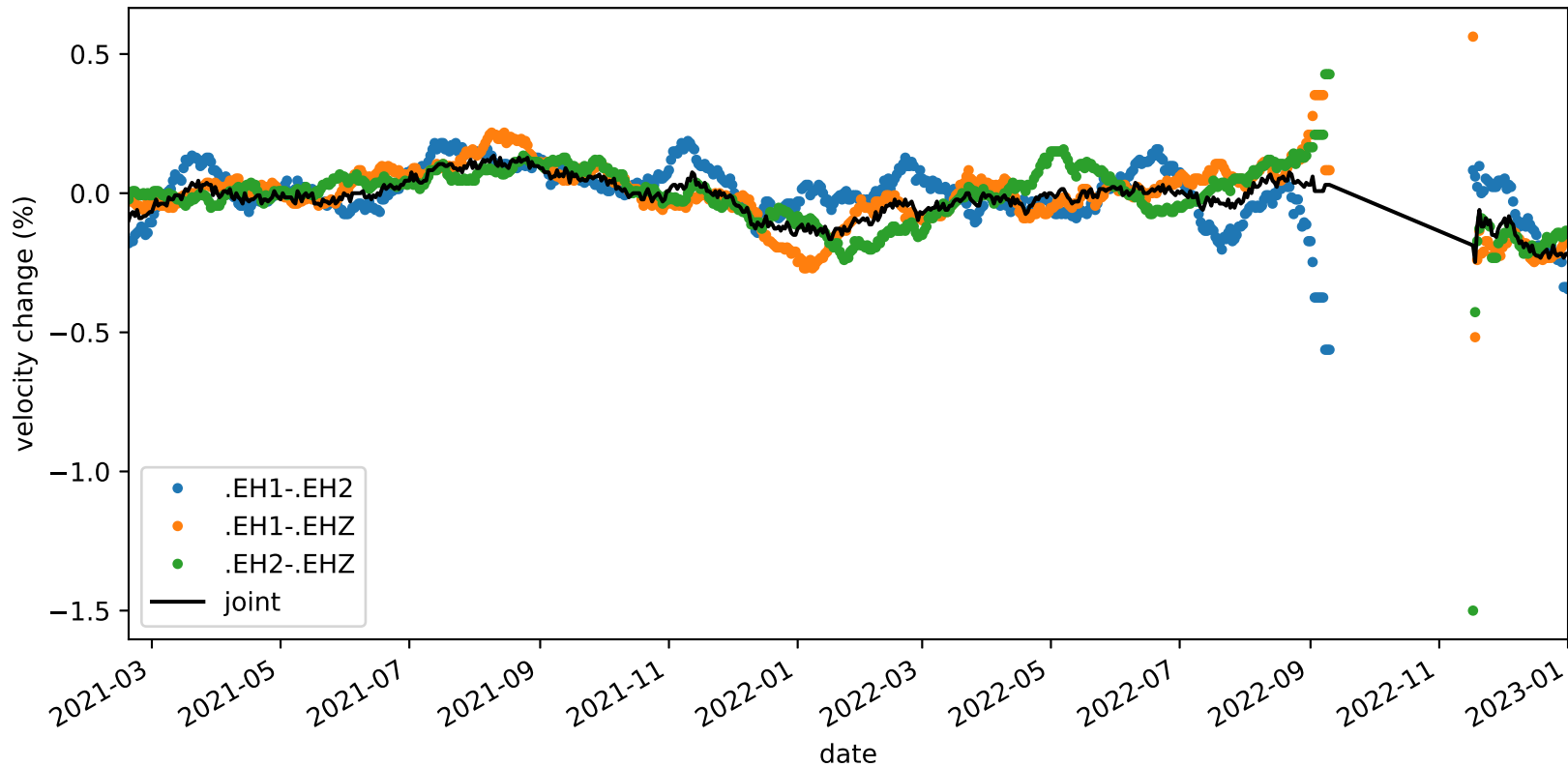
velocity_change_c1g_s2_t1b_tw_010.0s-015.0s_PB.B047-PB.B047
