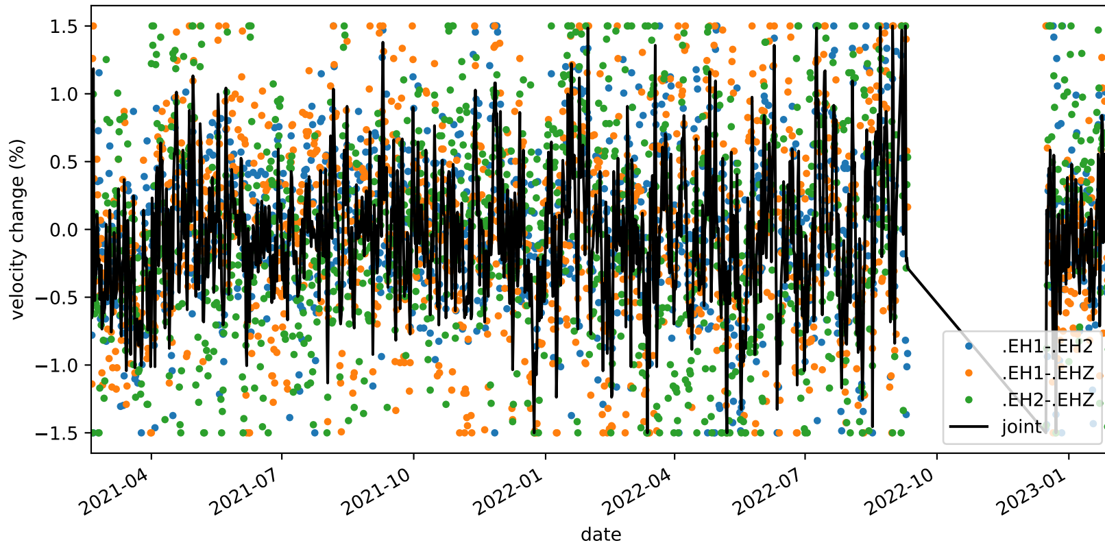
velocity_change_c1d_s1_t1a_tw_005.0s-010.0s_PB.B047-PB.B047
