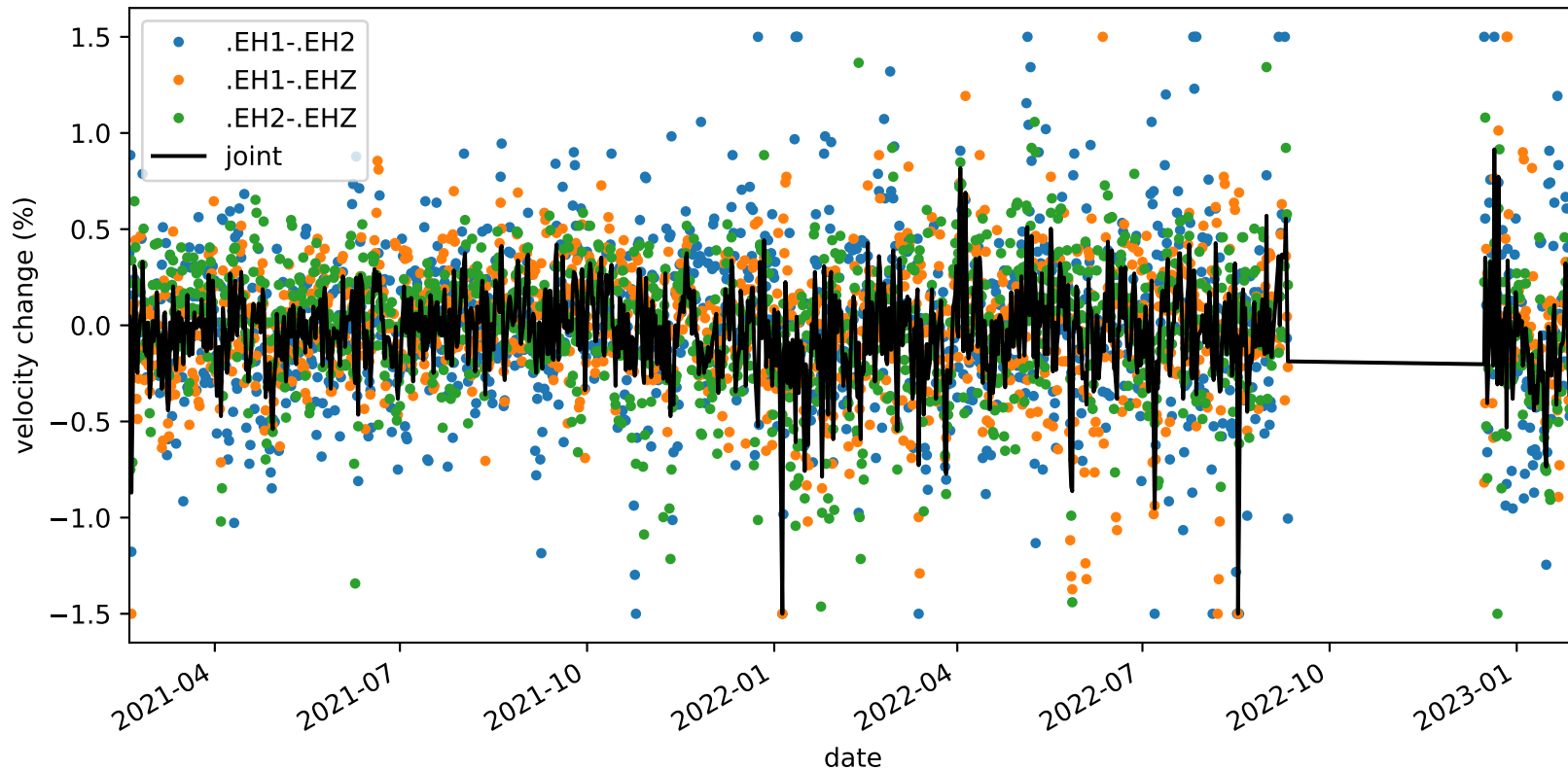
velocity_change_c1e_s1_t1b_tw_010.0s-015.0s_PB.B047-PB.B047
