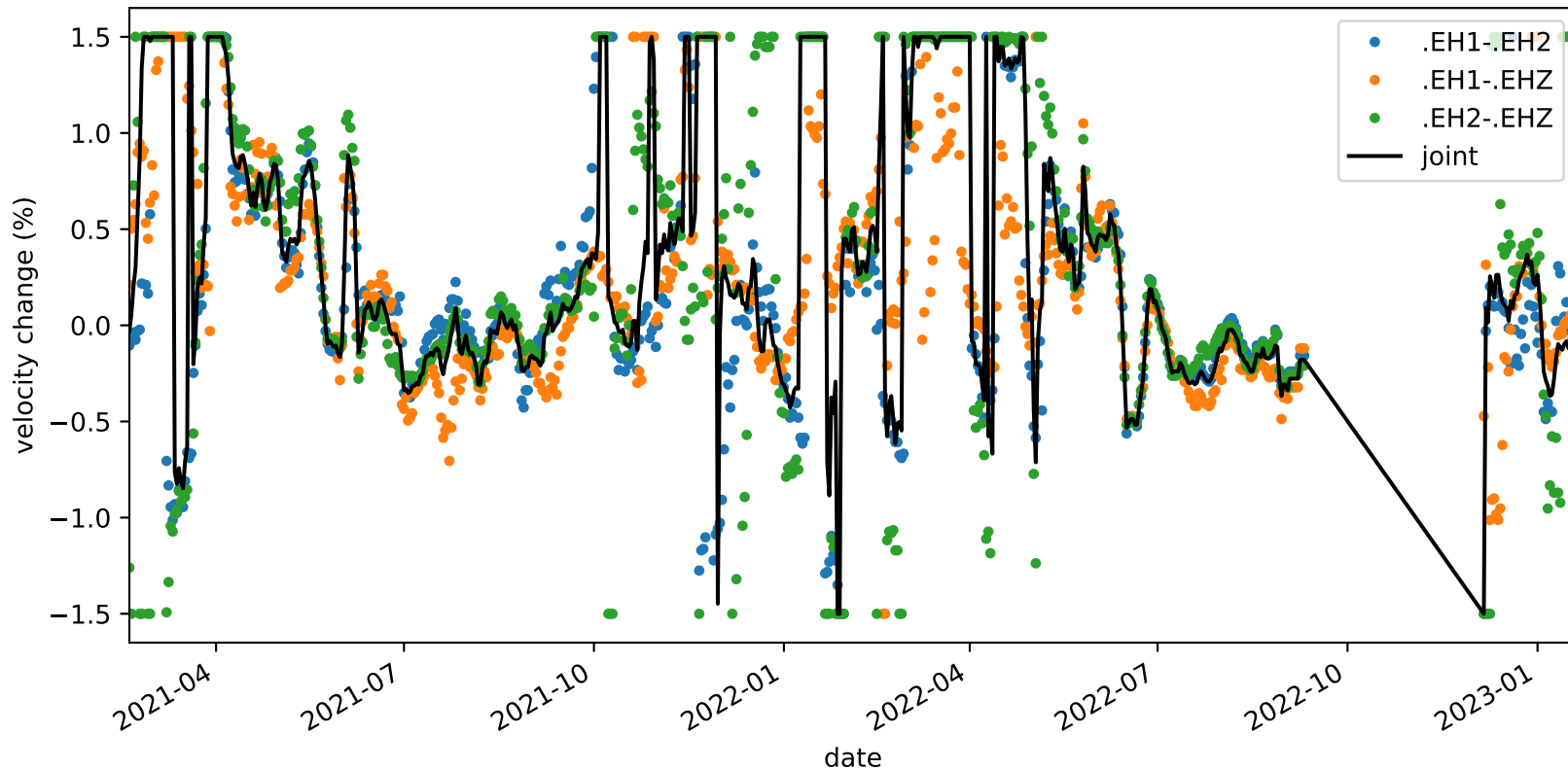
velocity_change_c1_s3_t1a_tw_005.0s-010.0s_PB.B047-PB.B047
