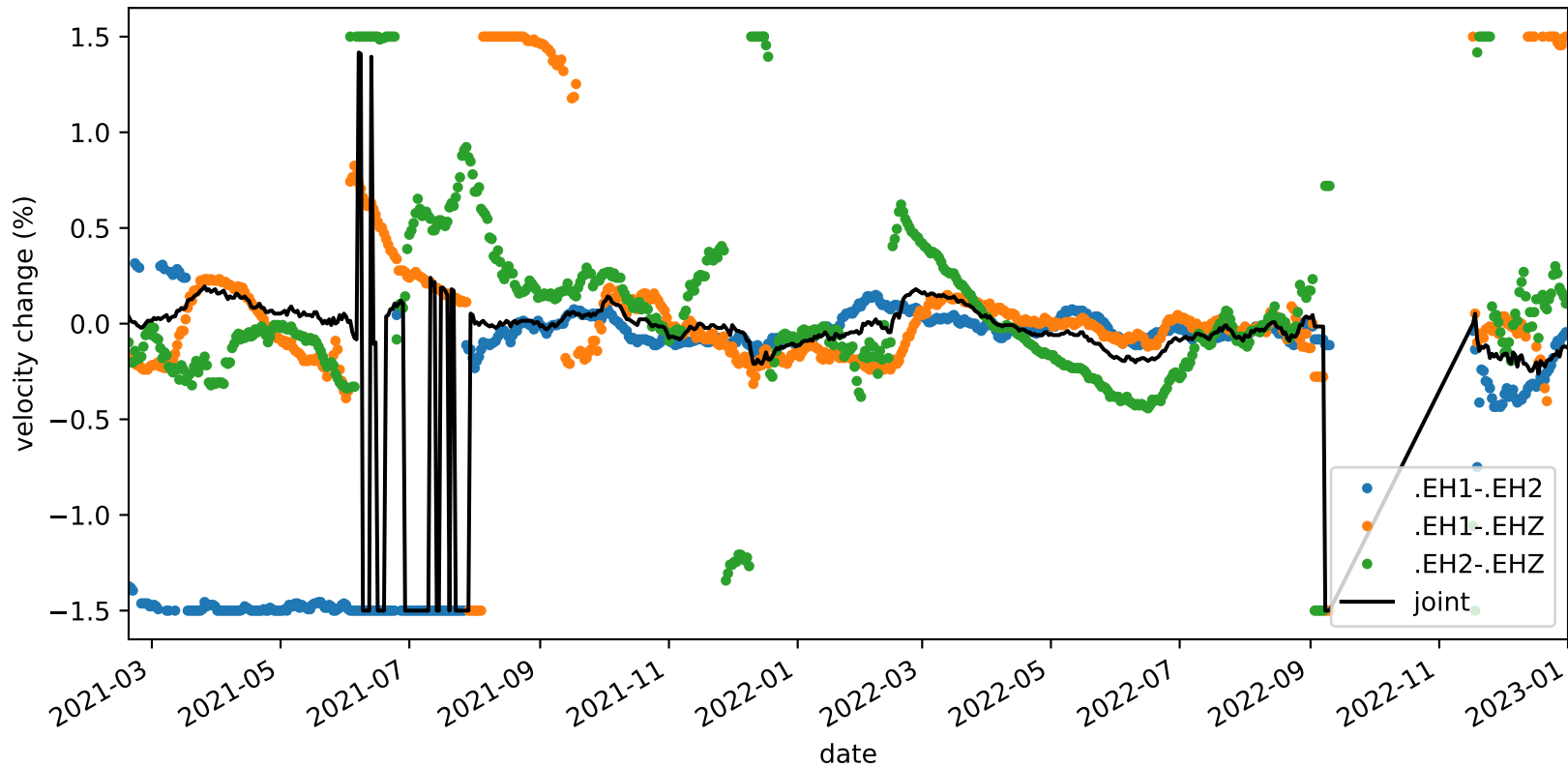
velocity_change_c1c_s2_t1a_tw_005.0s-010.0s_PB.B047-PB.B047
