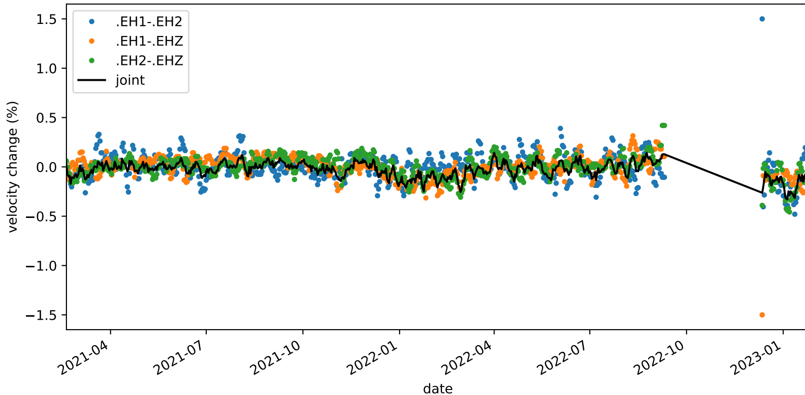
velocity_change_c1f_s4_t1c_tw_005.0s-015.0s_PB.B047-PB.B047
