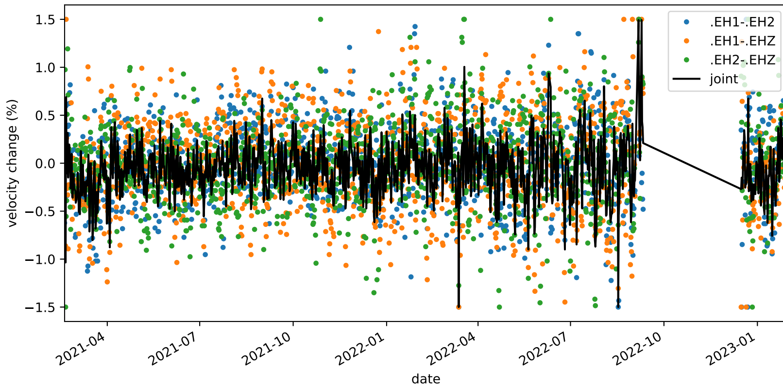
velocity_change_c1d_s1_t1c_tw_005.0s-015.0s_PB.B047-PB.B047
