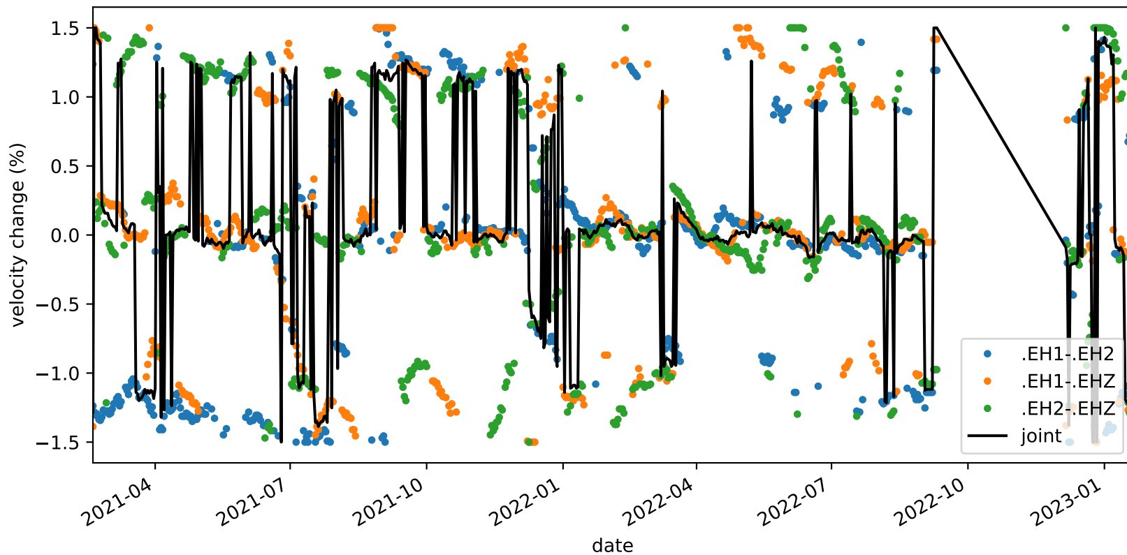
velocity_change_c1c_s3_t1b_tw_010.0s-015.0s_PB.B047-PB.B047
