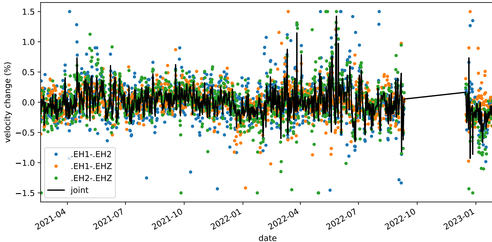
velocity_change_c1h_s1_t1c_tw_005.0s-015.0s_PB.B047-PB.B047
