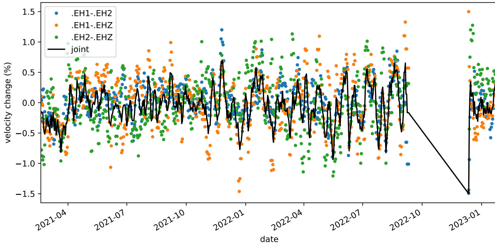
velocity_change_c1d_s4_t1a_tw_005.0s-010.0s_PB.B047-PB.B047
