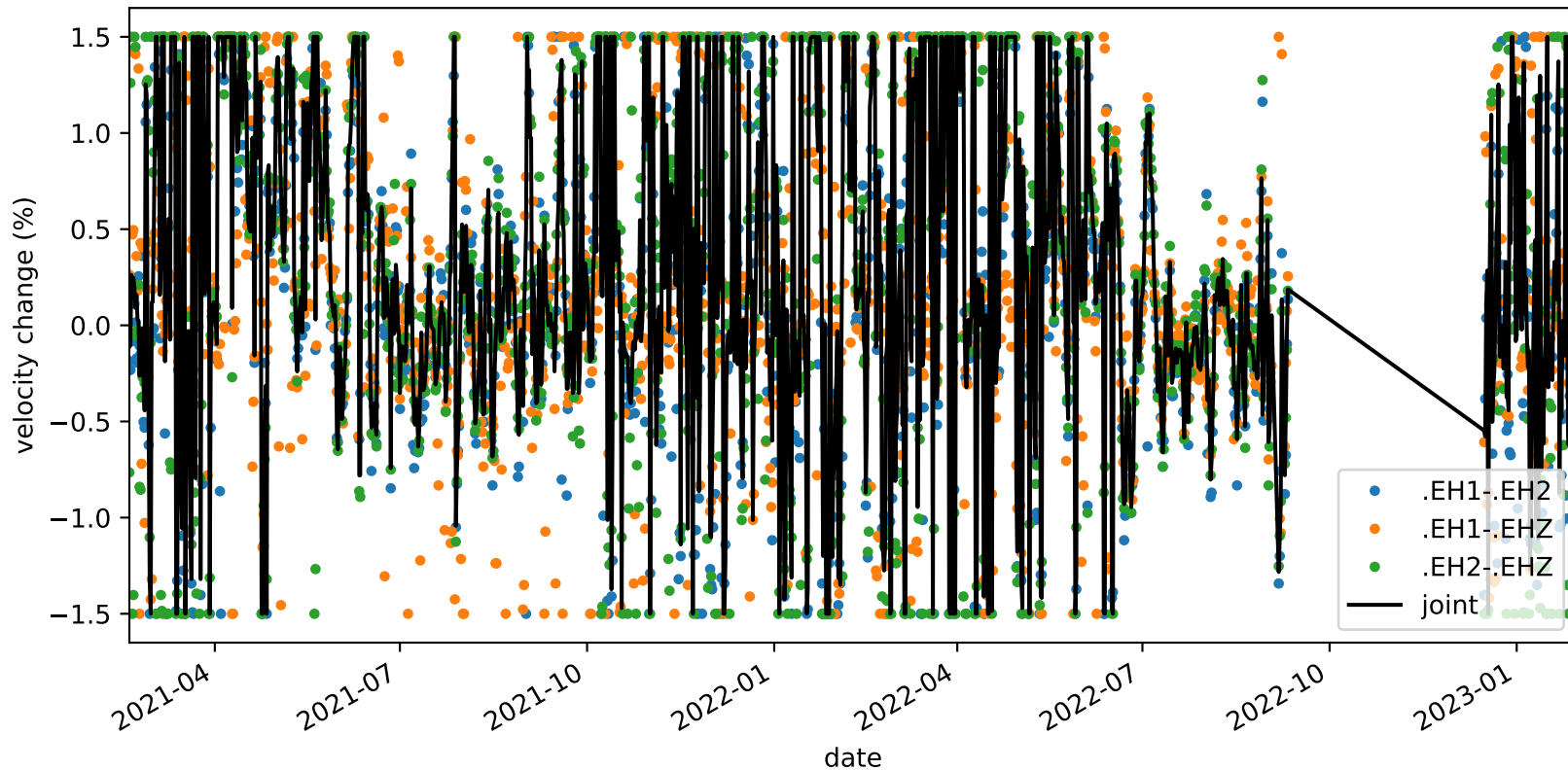
velocity_change_c1_s1_t1c_tw_005.0s-015.0s_PB.B047-PB.B047
