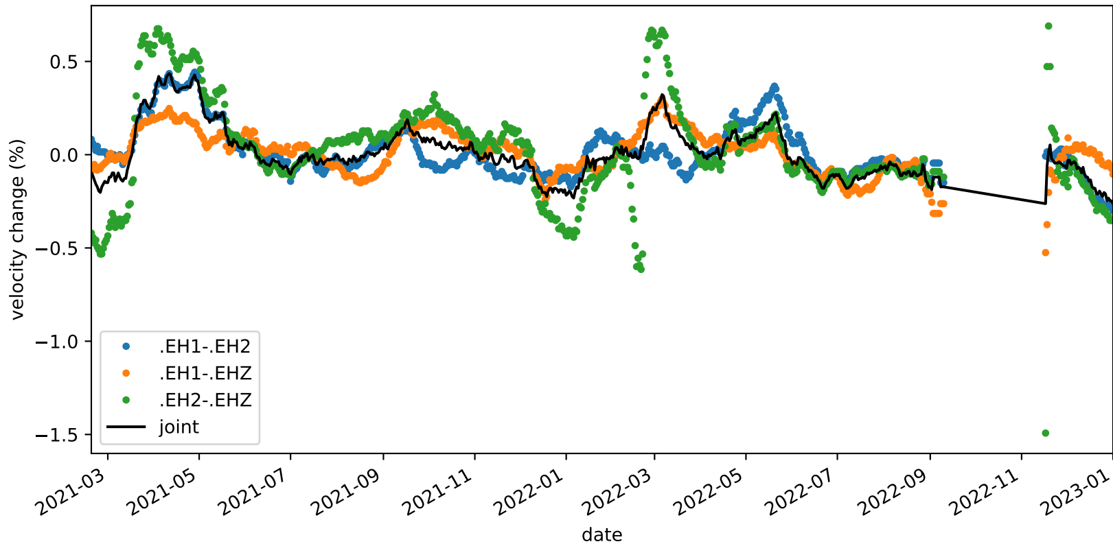
velocity_change_c1i_s2_t1a_tw_005.0s-010.0s_PB.B047-PB.B047
