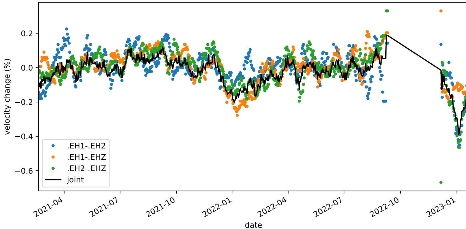
velocity_change_c1g_s3_t1c_tw_005.0s-015.0s_PB.B047-PB.B047
