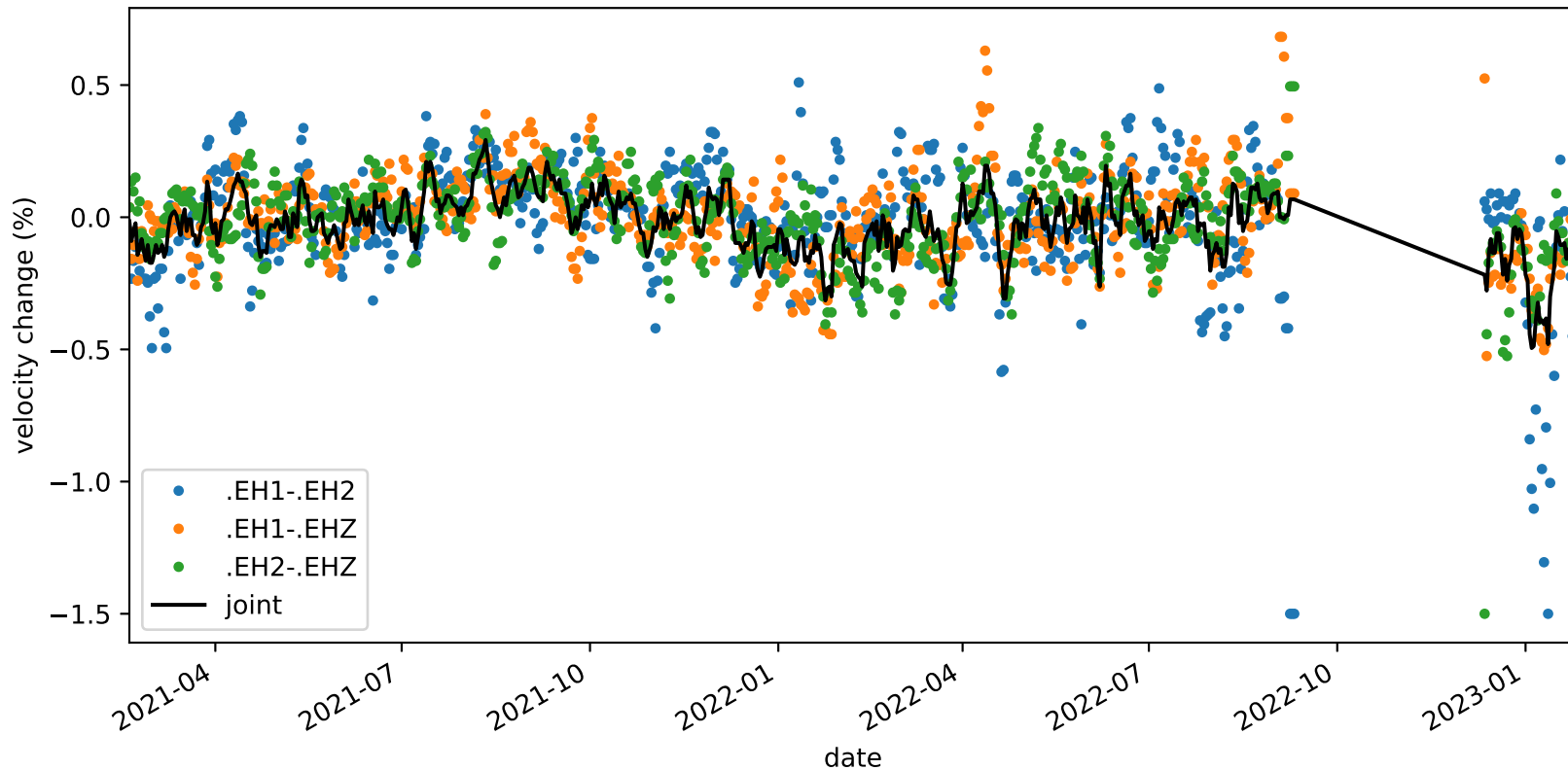
velocity_change_c1g_s4_t1b_tw_010.0s-015.0s_PB.B047-PB.B047
