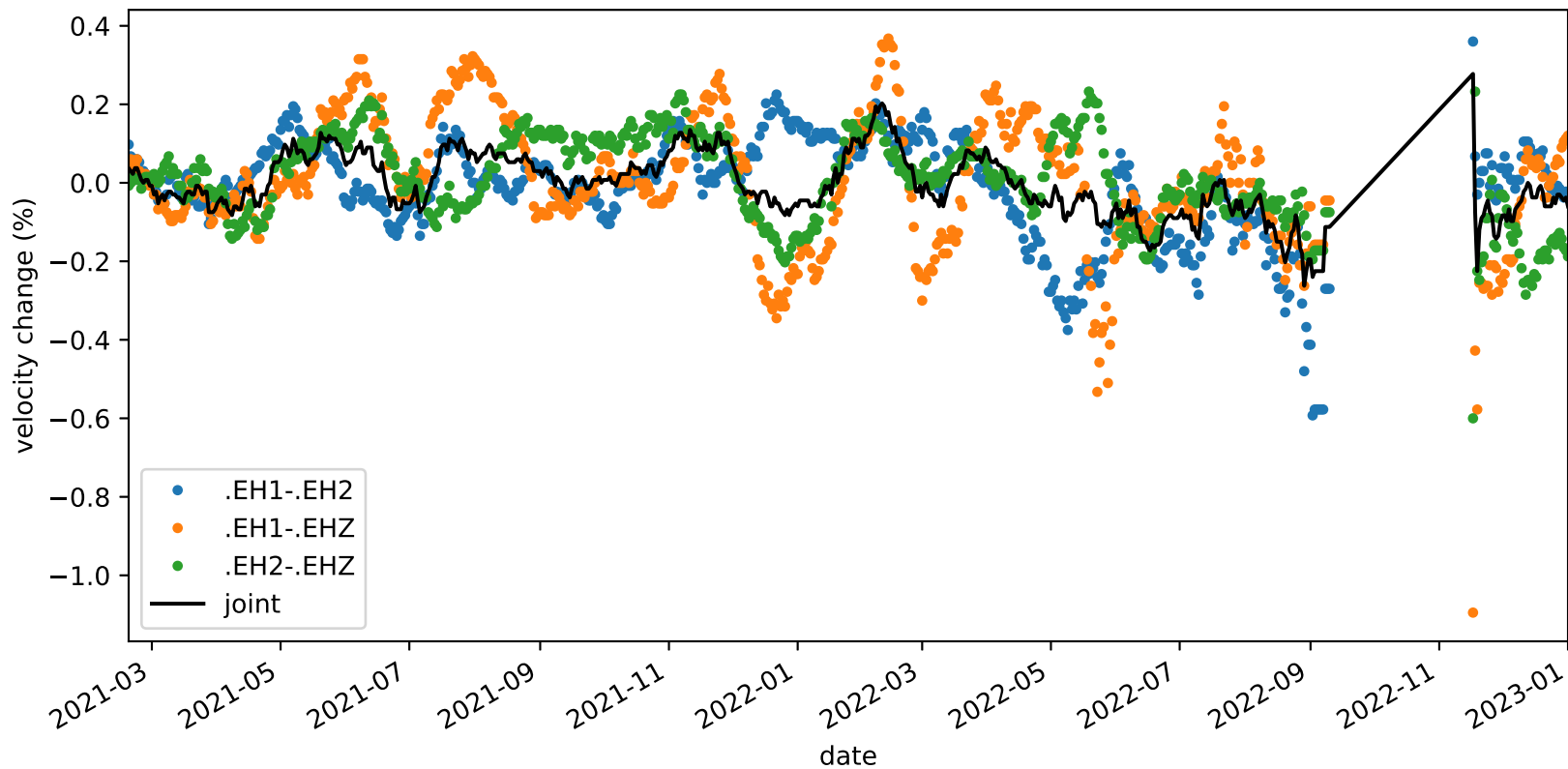
velocity_change_c1b_s2_t1b_tw_010.0s-015.0s_PB.B047-PB.B047
