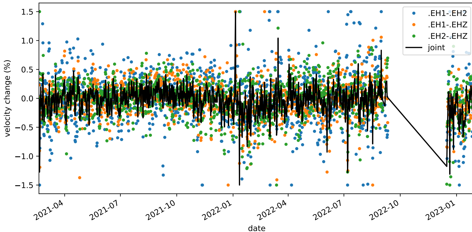
velocity_change_c1f_s1_t1b_tw_010.0s-015.0s_PB.B047-PB.B047
