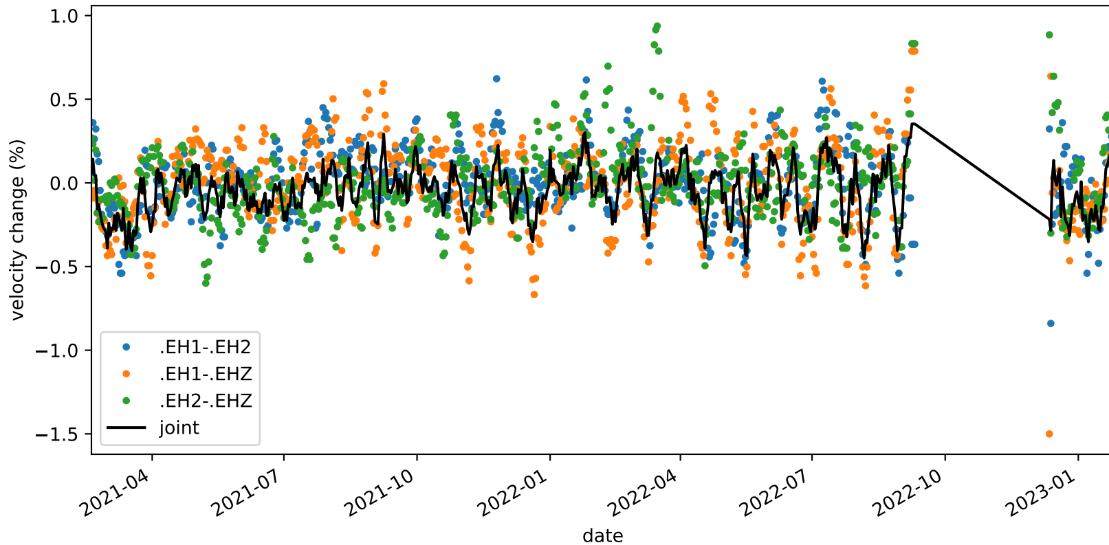
velocity_change_c1d_s4_t1c_tw_005.0s-015.0s_PB.B047-PB.B047
