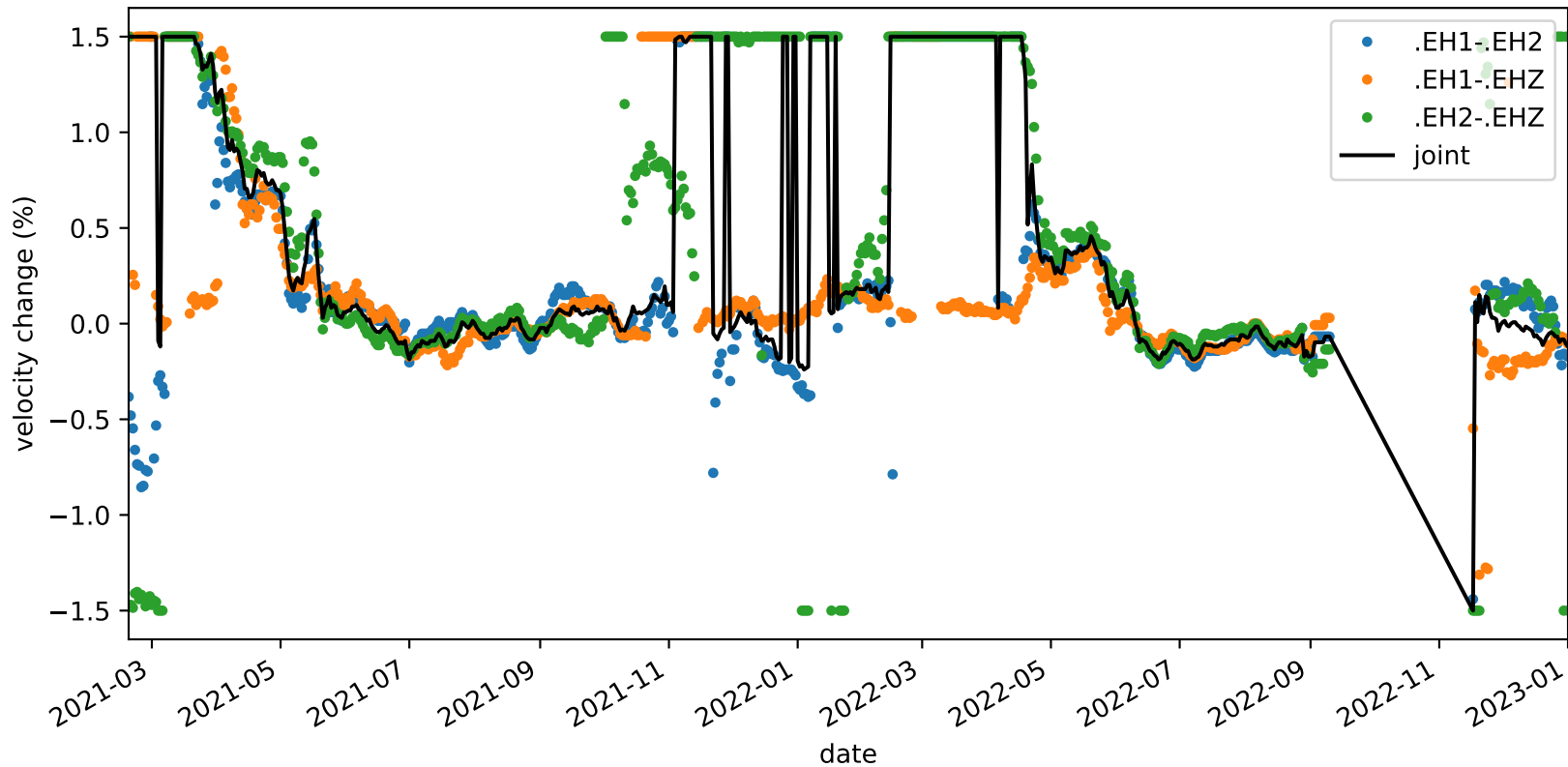
velocity_change_c1_s2_t1c_tw_005.0s-015.0s_PB.B047-PB.B047
