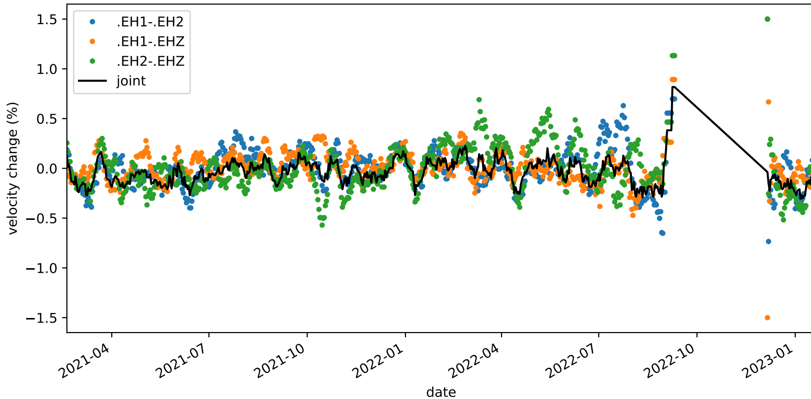
velocity_change_c1d_s3_t1b_tw_010.0s-015.0s_PB.B047-PB.B047
