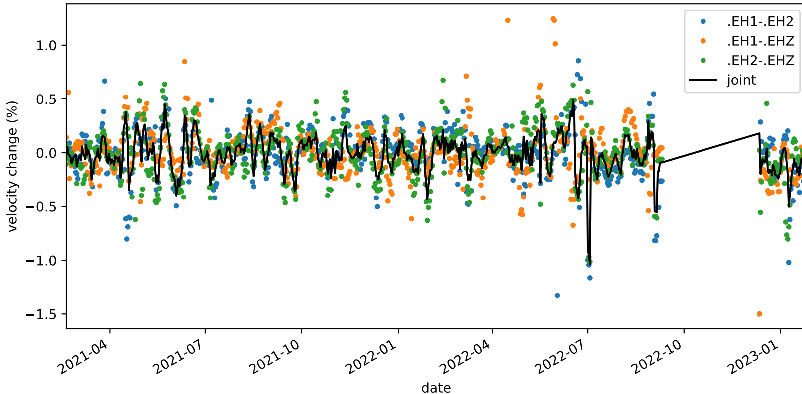
velocity_change_c1h_s4_t1b_tw_010.0s-015.0s_PB.B047-PB.B047
