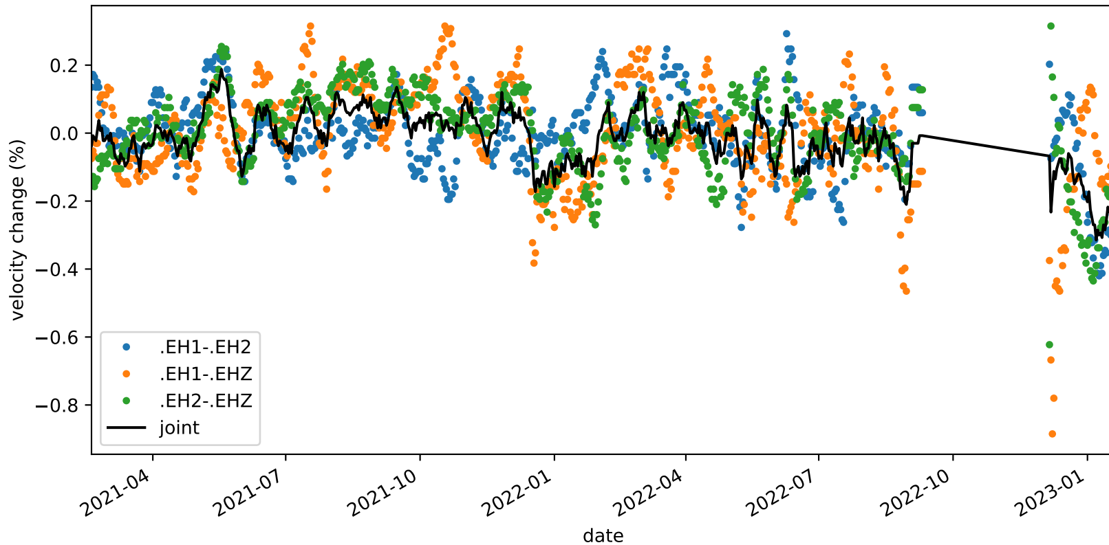
velocity_change_c1b_s3_t1c_tw_005.0s-015.0s_PB.B047-PB.B047
