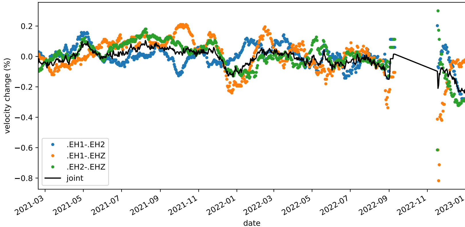
velocity_change_c1b_s2_t1c_tw_005.0s-015.0s_PB.B047-PB.B047
