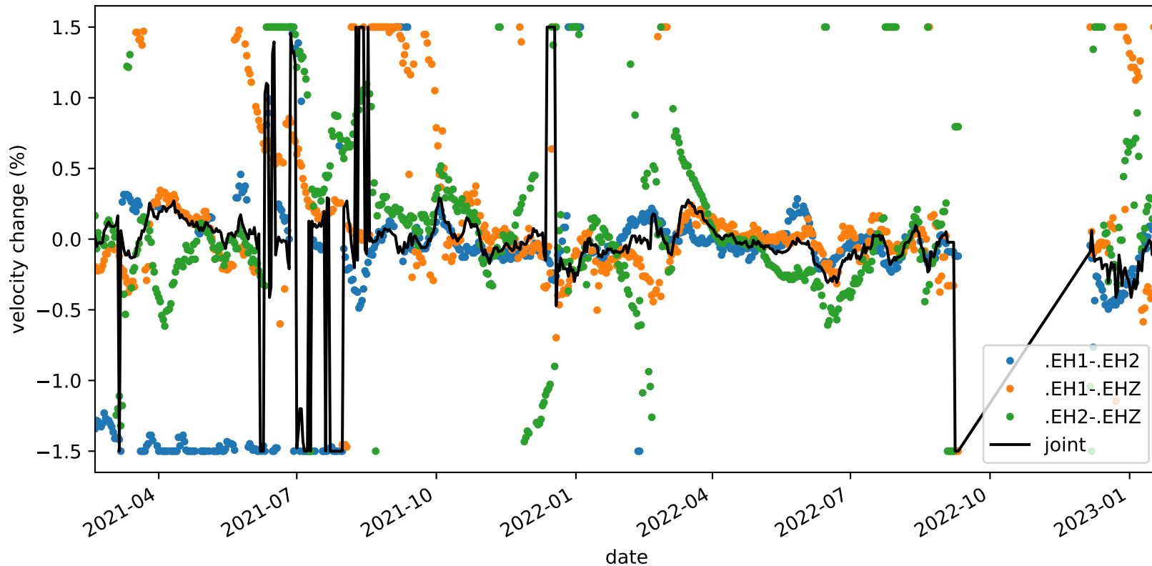
velocity_change_c1c_s3_t1a_tw_005.0s-010.0s_PB.B047-PB.B047
