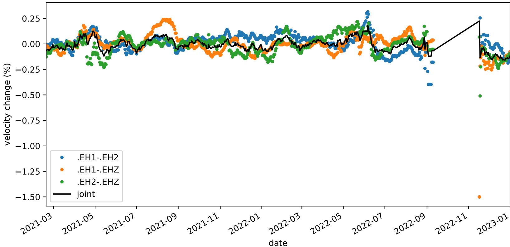
velocity_change_c1h_s2_t1b_tw_010.0s-015.0s_PB.B047-PB.B047
