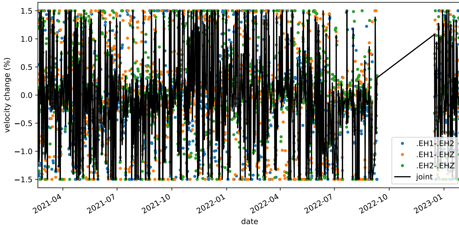
velocity_change_c1_s1_t1b_tw_010.0s-015.0s_PB.B047-PB.B047
