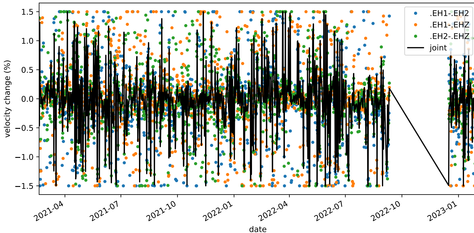
velocity_change_cli_s1_t1b_tw_010.0s-015.0s_PB.B047-PB.B047
