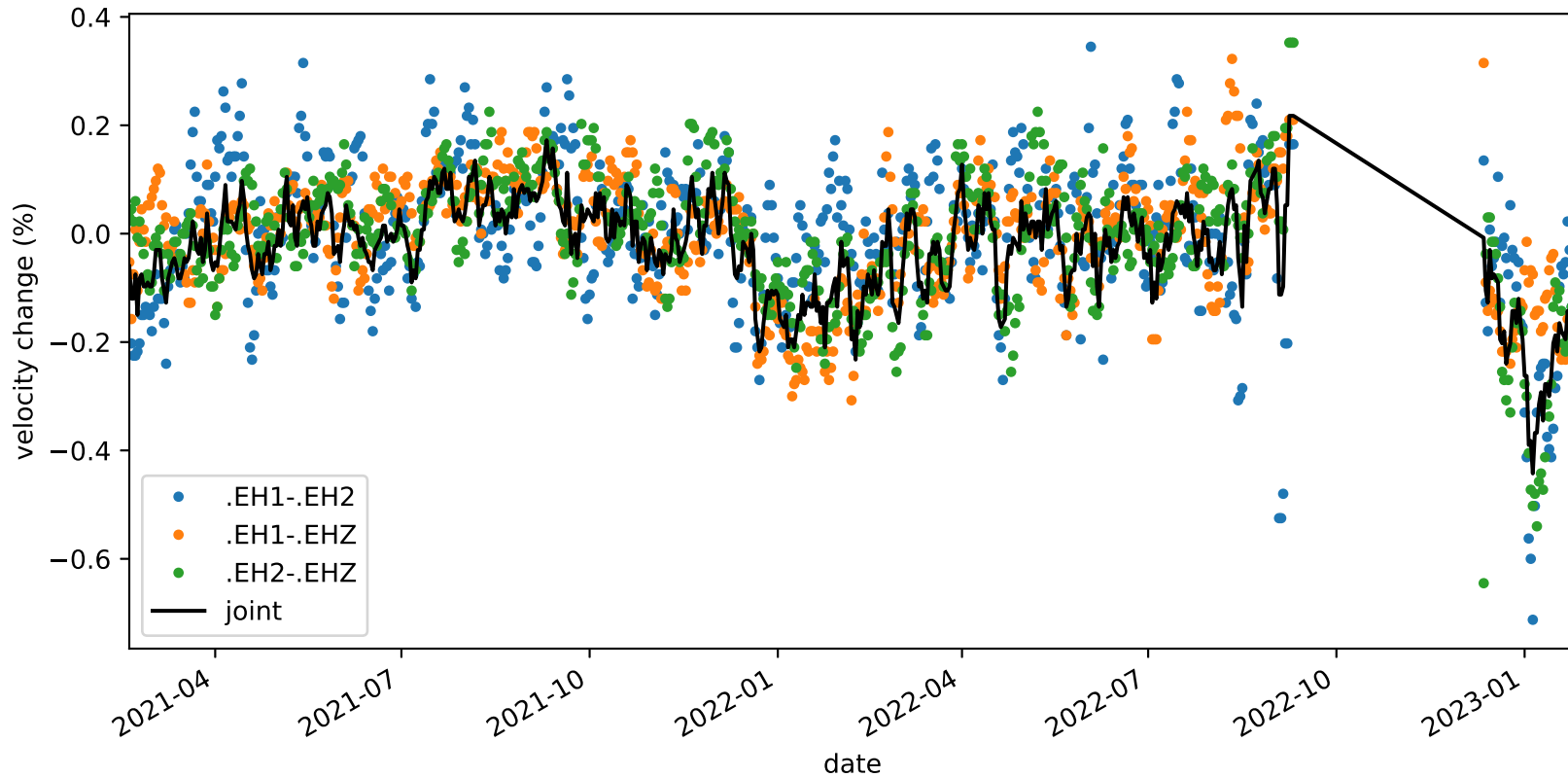
velocity_change_c1g_s4_t1c_tw_005.0s-015.0s_PB.B047-PB.B047
