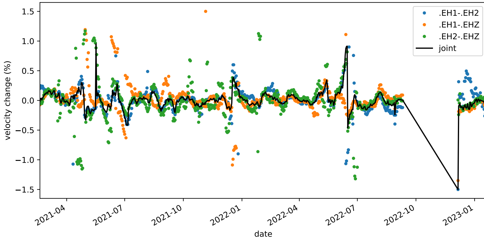
velocity_change_cli_s3_t1b_tw_010.0s-015.0s_PB.B047-PB.B047
