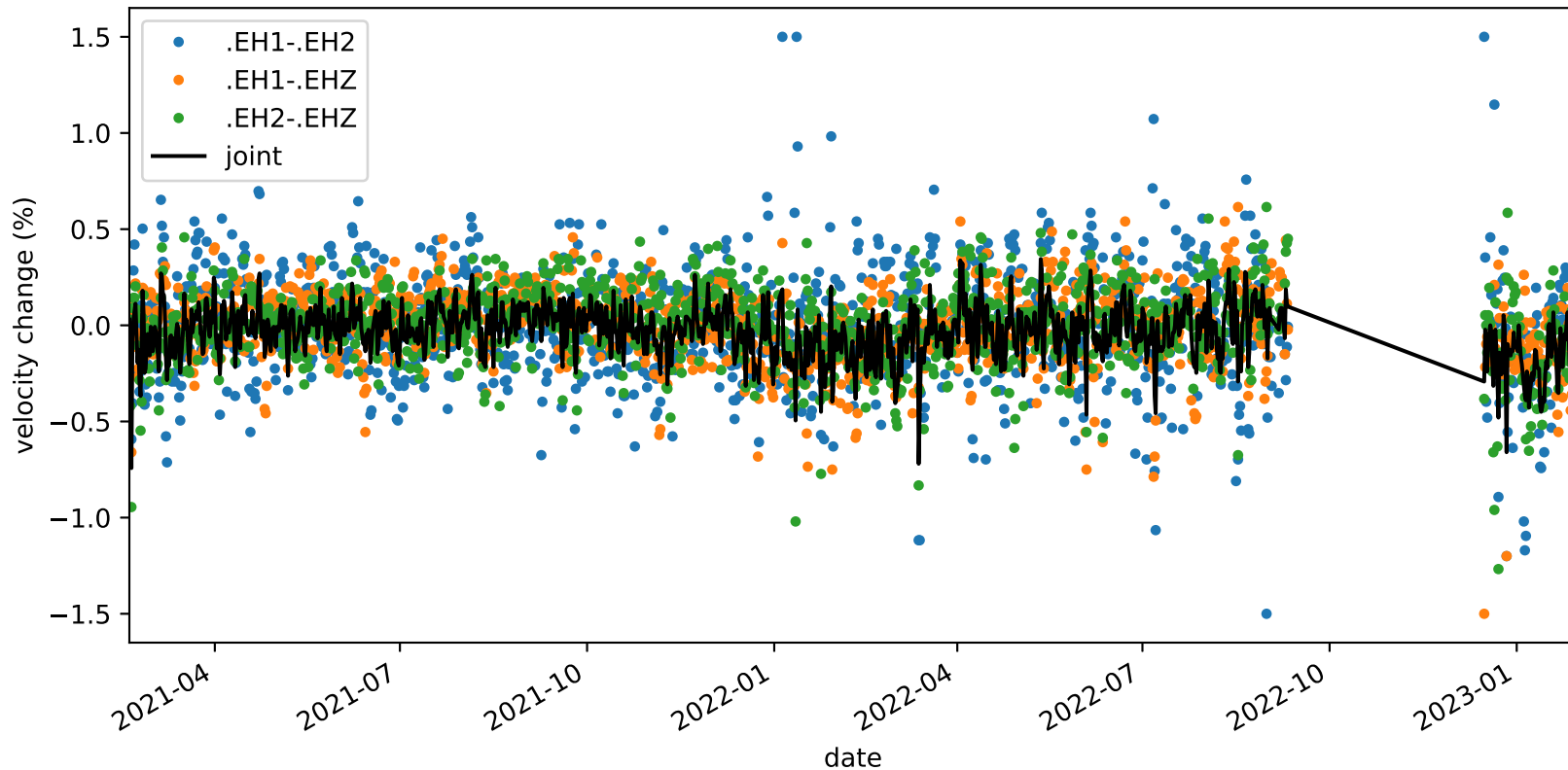
velocity_change_c1f_s1_t1c_tw_005.0s-015.0s_PB.B047-PB.B047
