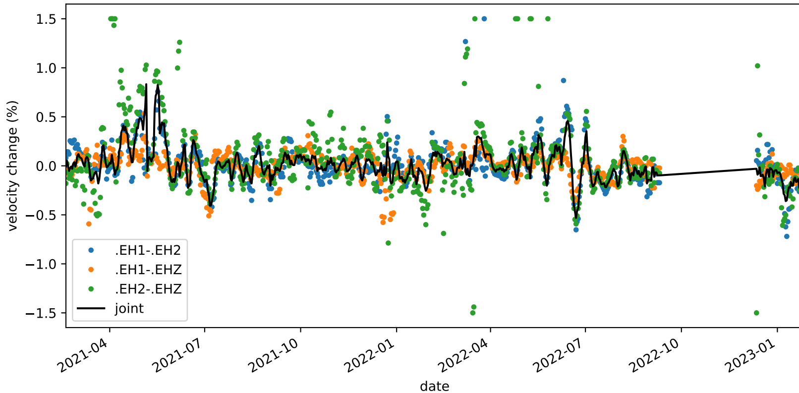
velocity_change_cli_s4_t1c_tw_005.0s-015.0s_PB.B047-PB.B047
