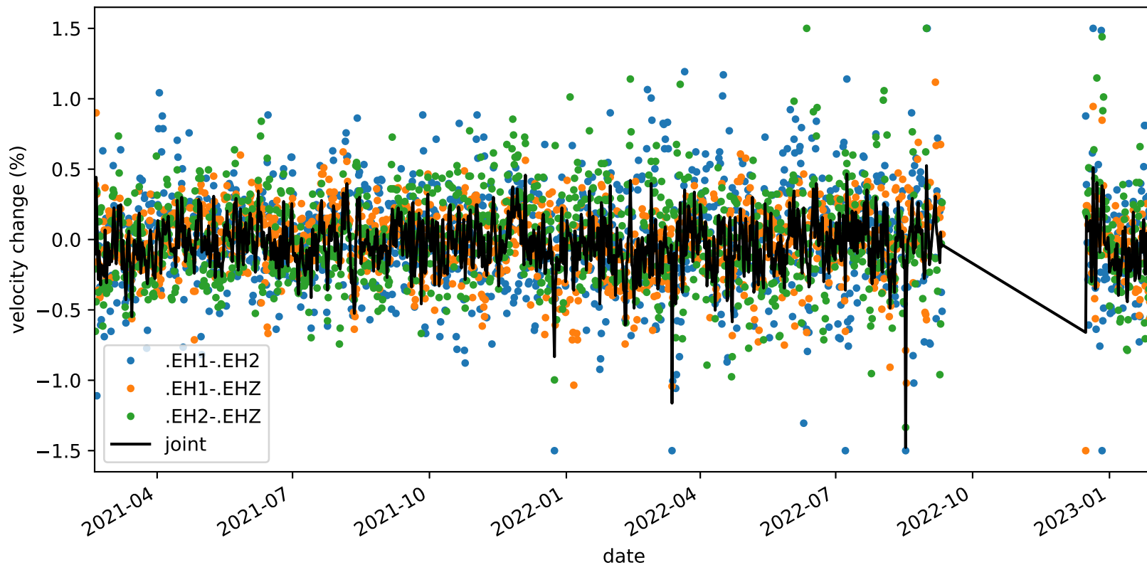
velocity_change_c1e_s1_t1a_tw_005.0s-010.0s_PB.B047-PB.B047
