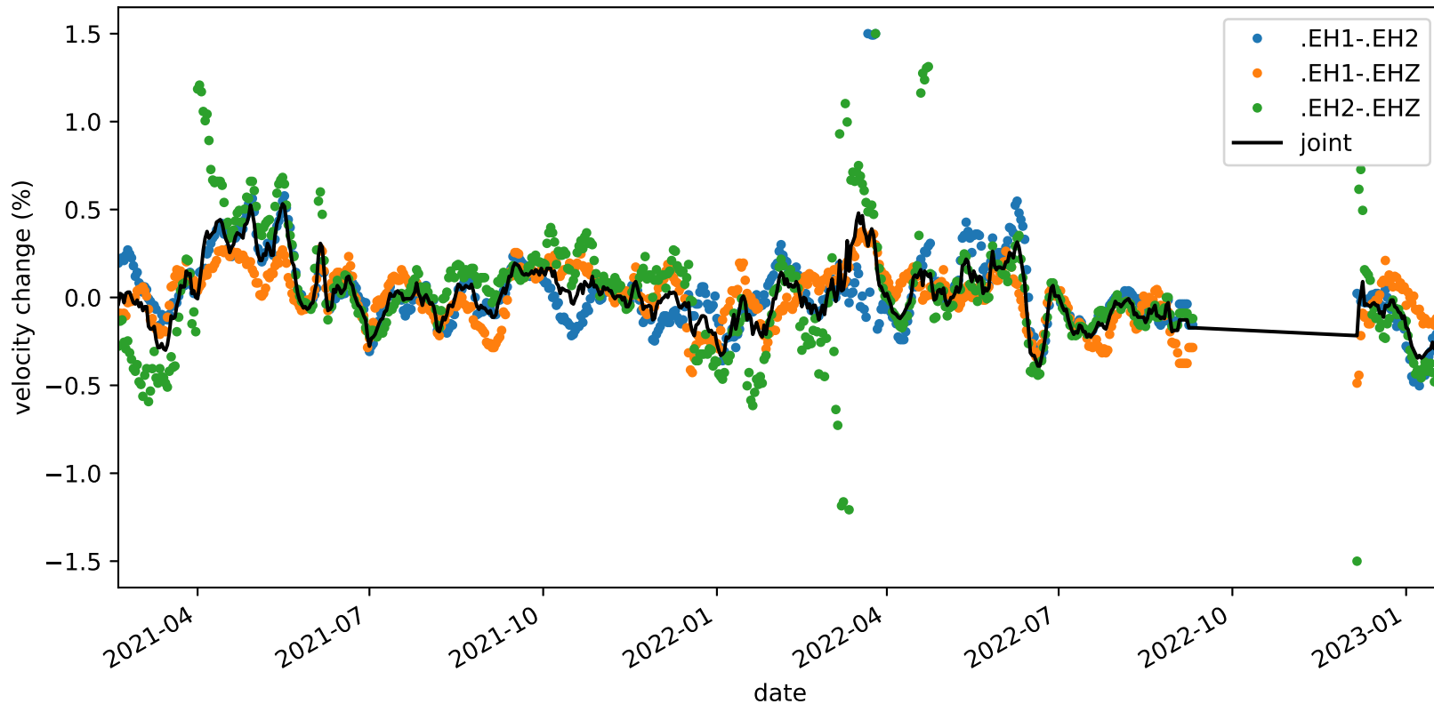
velocity_change_c1i_s3_t1a_tw_005.0s-010.0s_PB.B047-PB.B047
