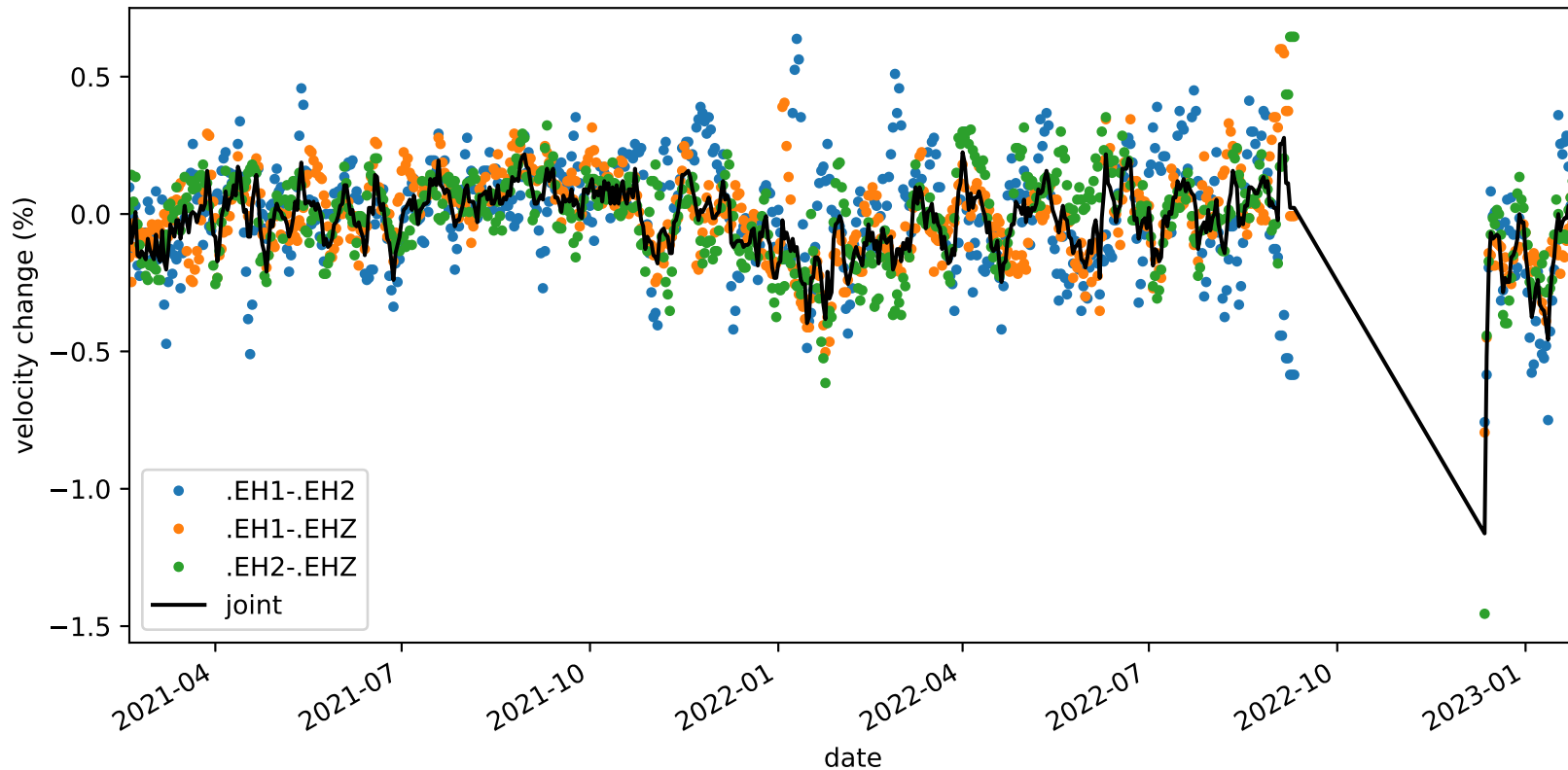
velocity_change_c1f_s4_t1b_tw_010.0s-015.0s_PB.B047-PB.B047
