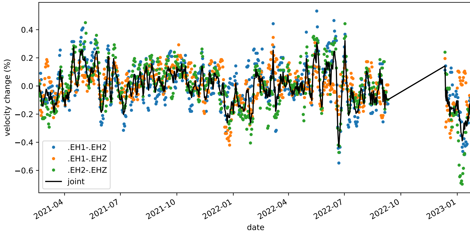
velocity_change_c1h_s4_t1c_tw_005.0s-015.0s_PB.B047-PB.B047
