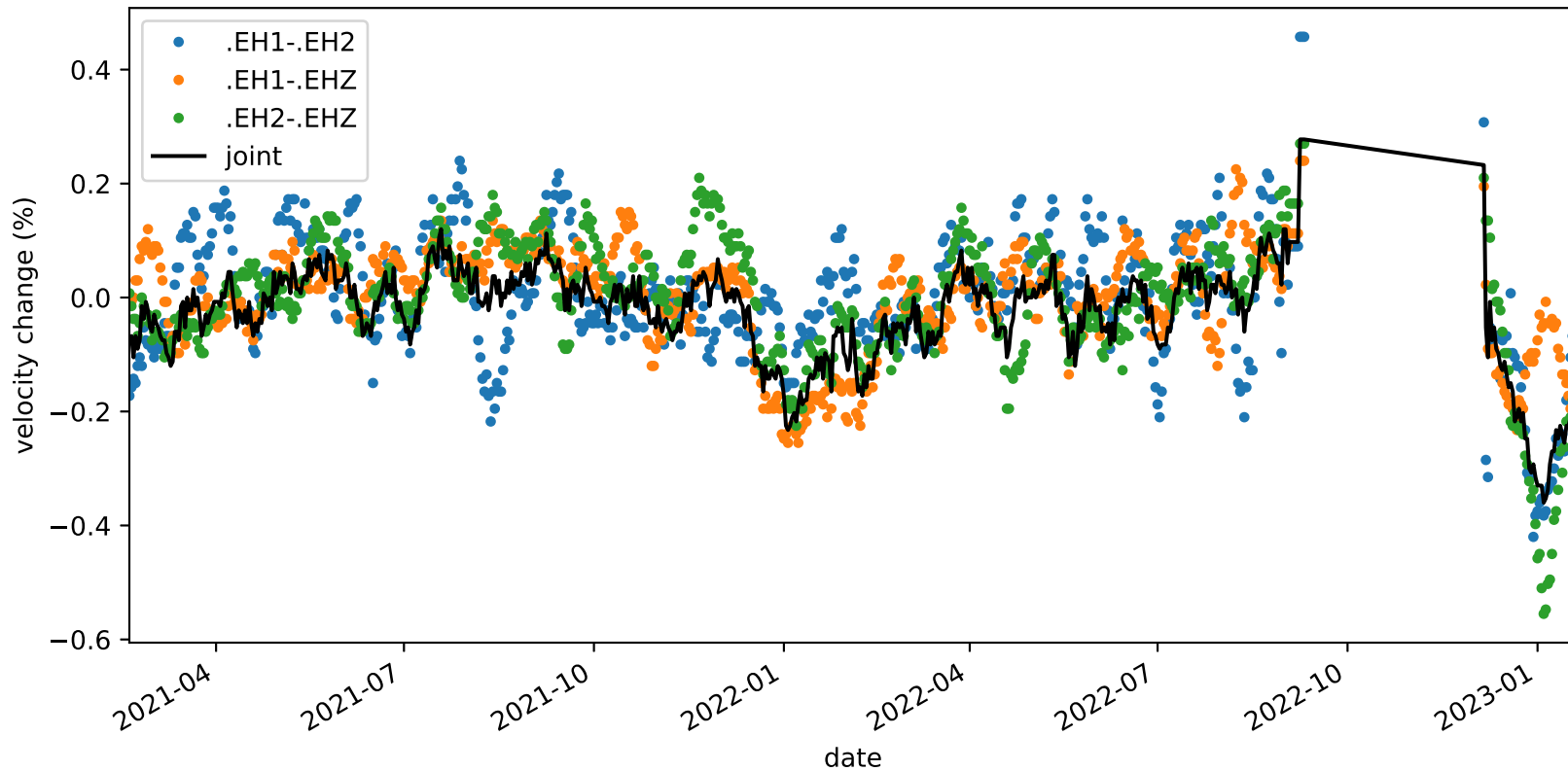
velocity_change_c1g_s3_t1a_tw_005.0s-010.0s_PB.B047-PB.B047
