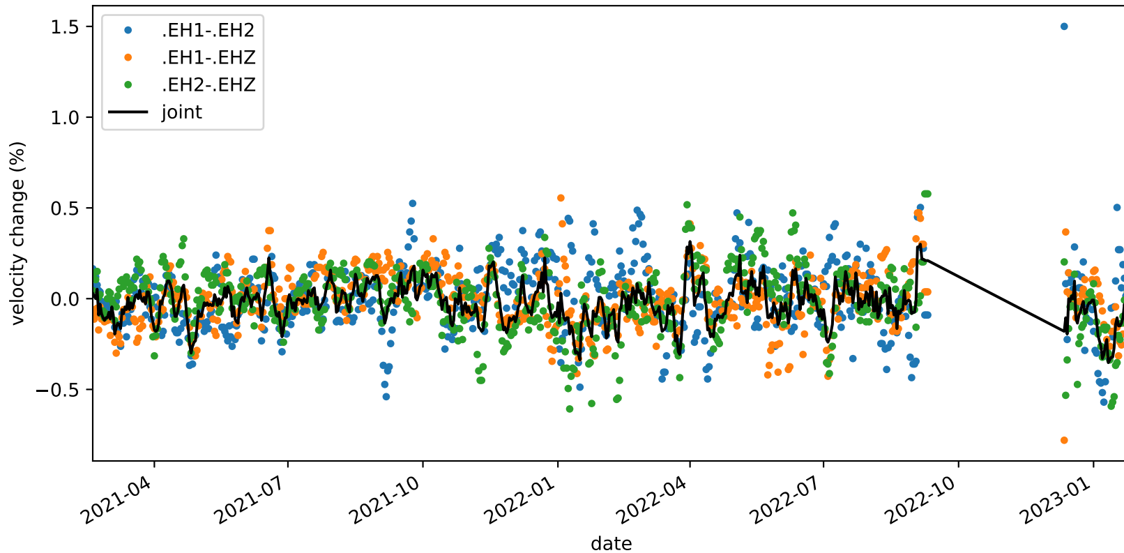
velocity_change_c1e_s4_t1b_tw_010.0s-015.0s_PB.B047-PB.B047
