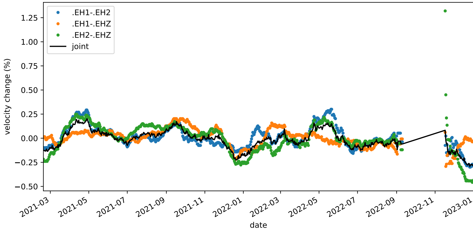
velocity_change_c1h_s2_t1a_tw_005.0s-010.0s_PB.B047-PB.B047
