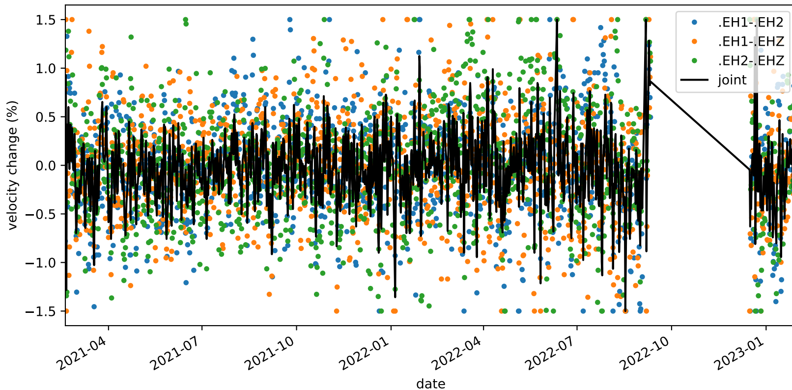
velocity_change_c1d_s1_t1b_tw_010.0s-015.0s_PB.B047-PB.B047
