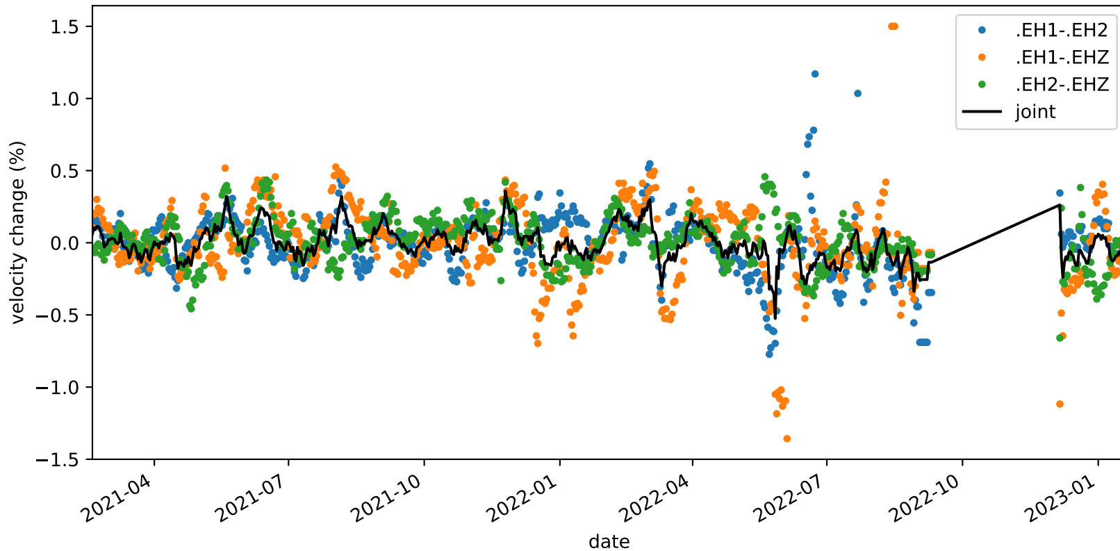
velocity_change_c1b_s3_t1b_tw_010.0s-015.0s_PB.B047-PB.B047
