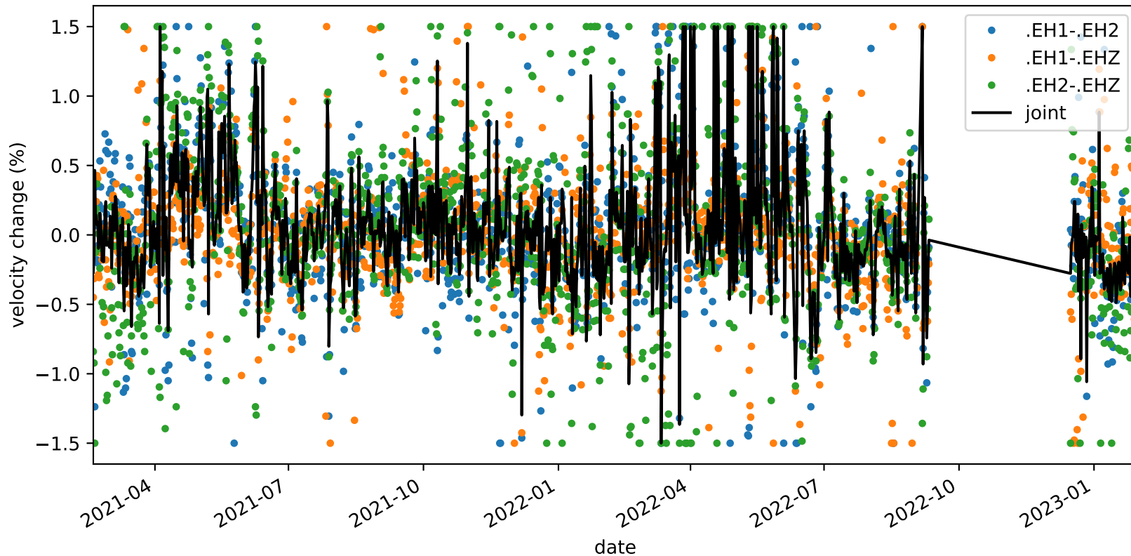
velocity_change_cli_s1_t1a_tw_005.0s-010.0s_PB.B047-PB.B047
