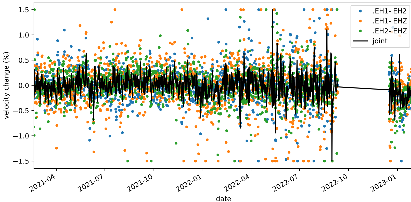
velocity_change_c1b_s1_t1c_tw_005.0s-015.0s_PB.B047-PB.B047
