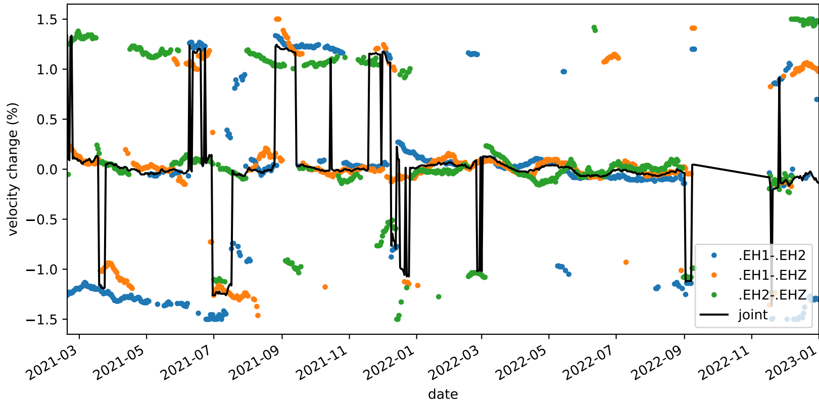
velocity_change_c1c_s2_t1b_tw_010.0s-015.0s_PB.B047-PB.B047
