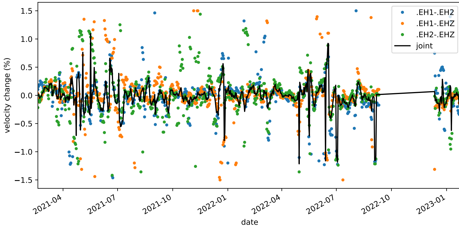
velocity_change_cli_s4_t1b_tw_010.0s-015.0s_PB.B047-PB.B047
