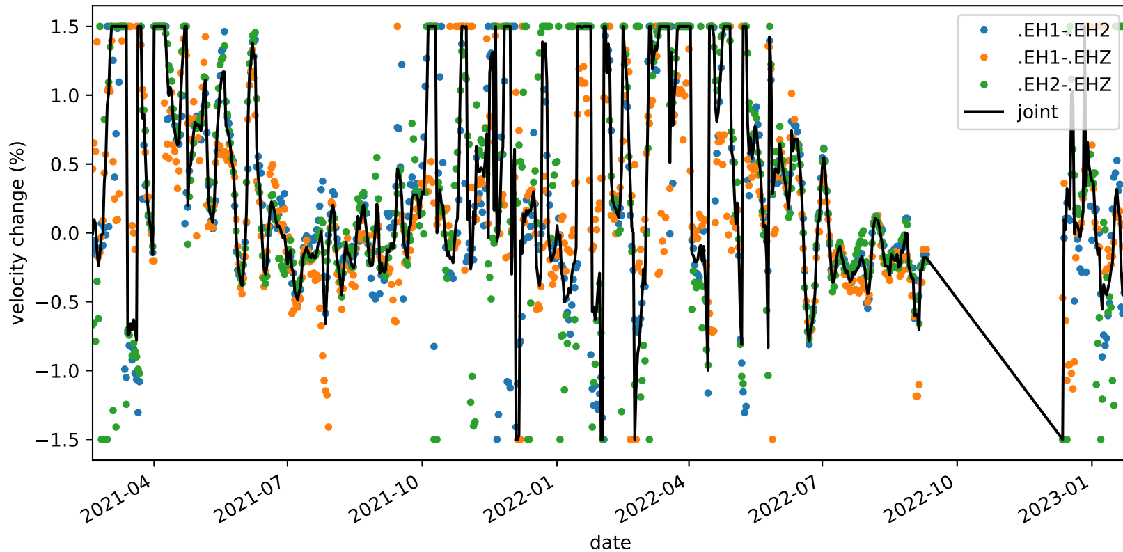
velocity_change_c1_s4_t1a_tw_005.0s-010.0s_PB.B047-PB.B047
