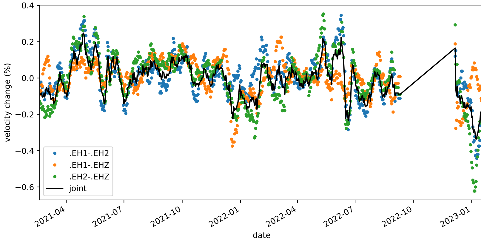
velocity_change_c1h_s3_t1c_tw_005.0s-015.0s_PB.B047-PB.B047
