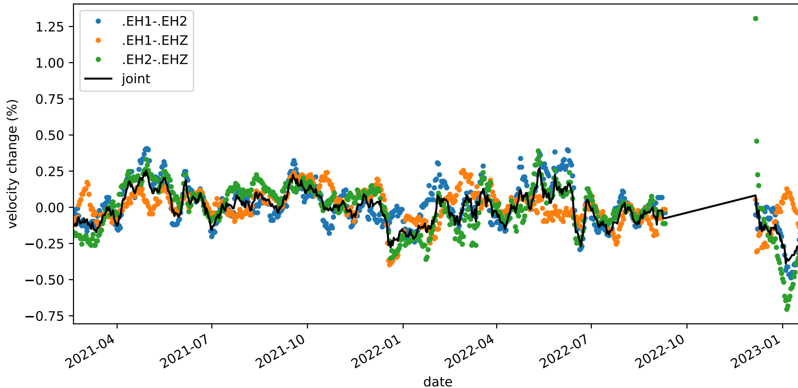
velocity_change_c1h_s3_t1a_tw_005.0s-010.0s_PB.B047-PB.B047
