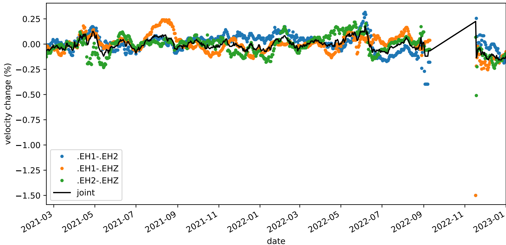
velocity_change_c1h_s2_t1b_tw_010.0s-015.0s_PB.B047-PB.B047
