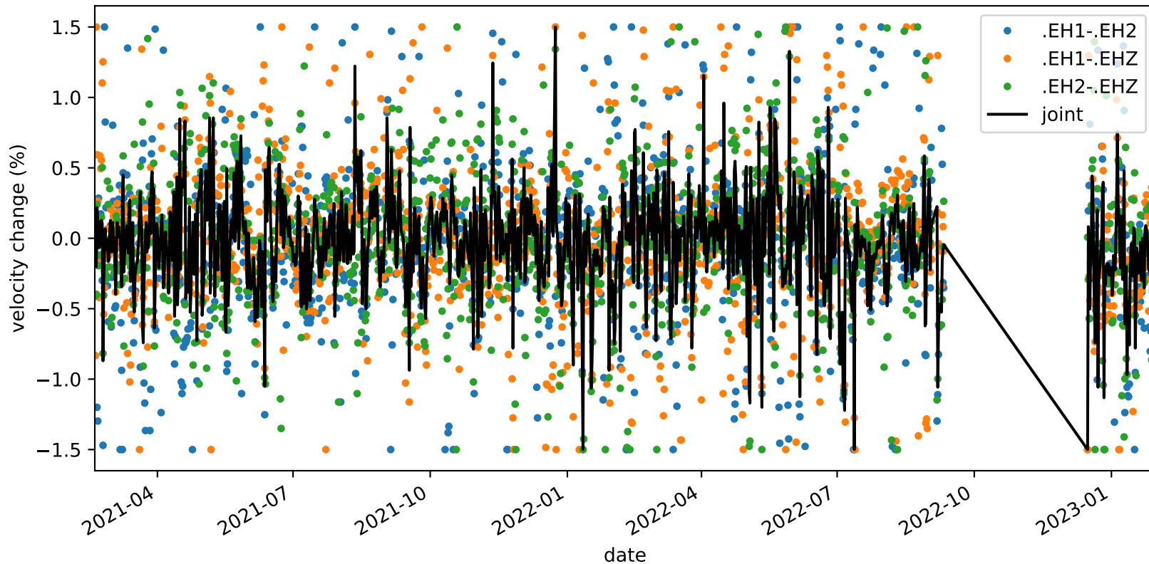
velocity_change_c1h_s1_t1b_tw_010.0s-015.0s_PB.B047-PB.B047
