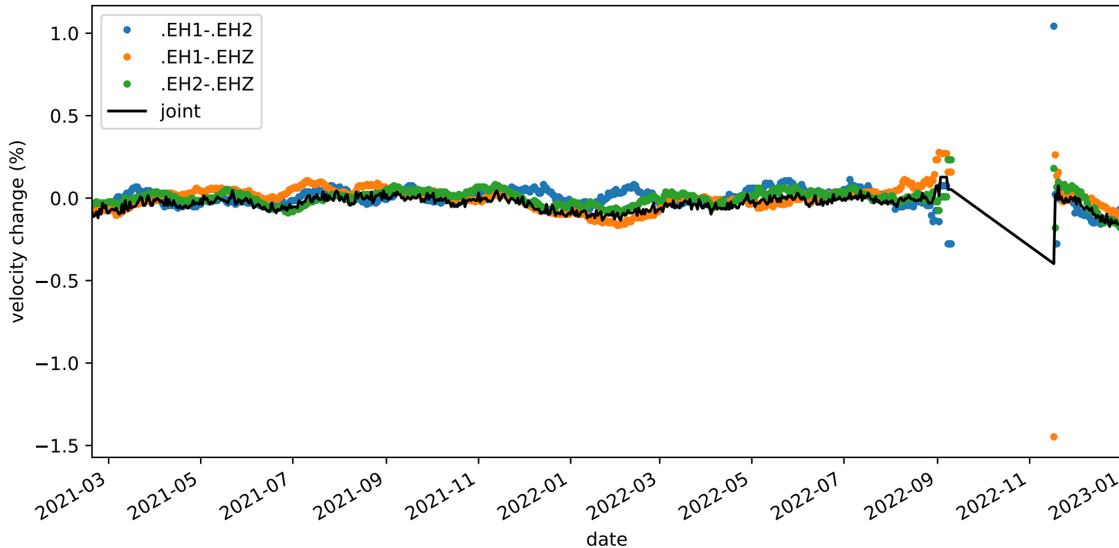
velocity_change_c1e_s2_t1c_tw_005.0s-015.0s_PB.B047-PB.B047
