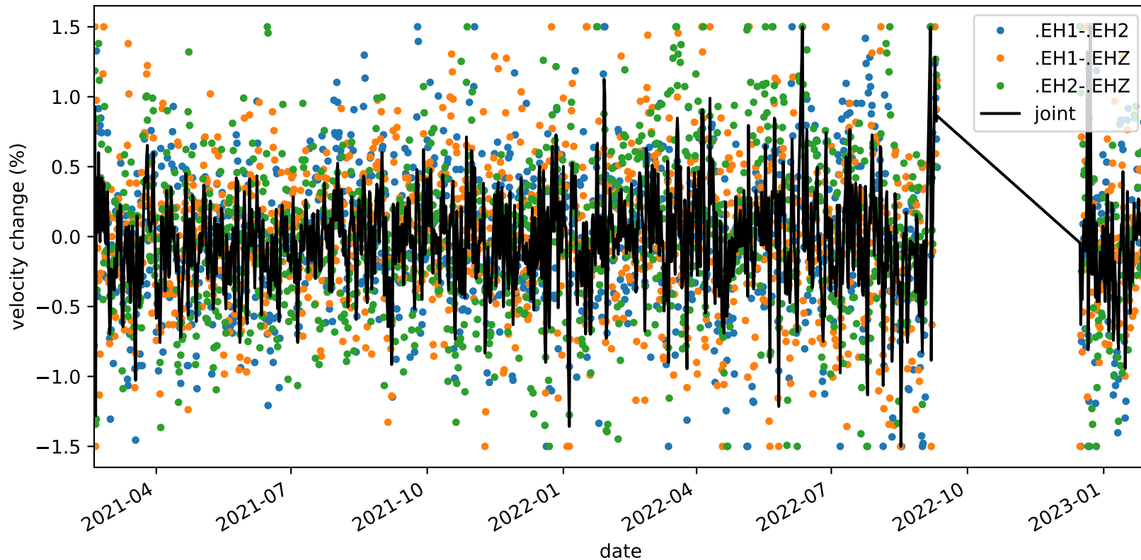
velocity_change_c1d_s1_t1b_tw_010.0s-015.0s_PB.B047-PB.B047
