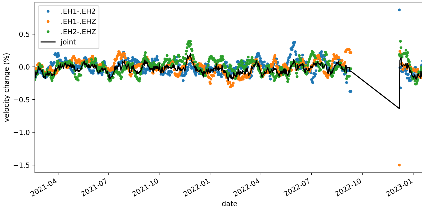
velocity_change_c1e_s3_t1a_tw_005.0s-010.0s_PB.B047-PB.B047
