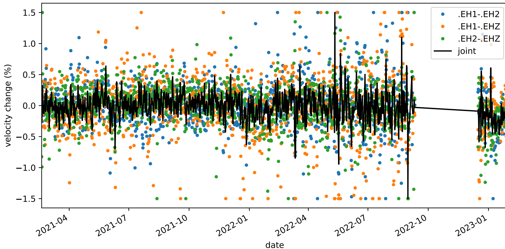
velocity_change_c1b_s1_t1c_tw_005.0s-015.0s_PB.B047-PB.B047
