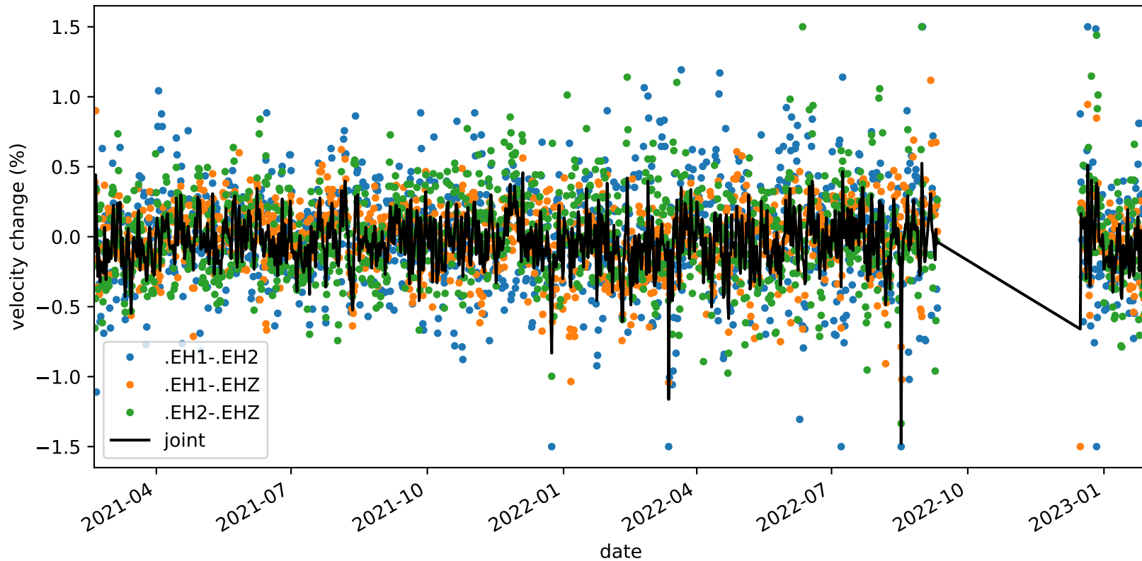
velocity_change_c1e_s1_t1a_tw_005.0s-010.0s_PB.B047-PB.B047
