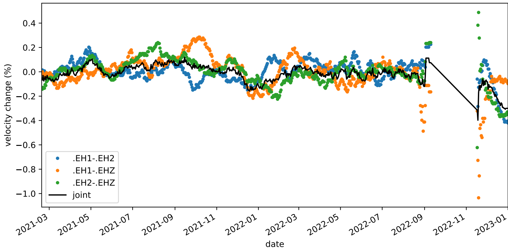
velocity_change_c1b_s2_t1a_tw_005.0s-010.0s_PB.B047-PB.B047
