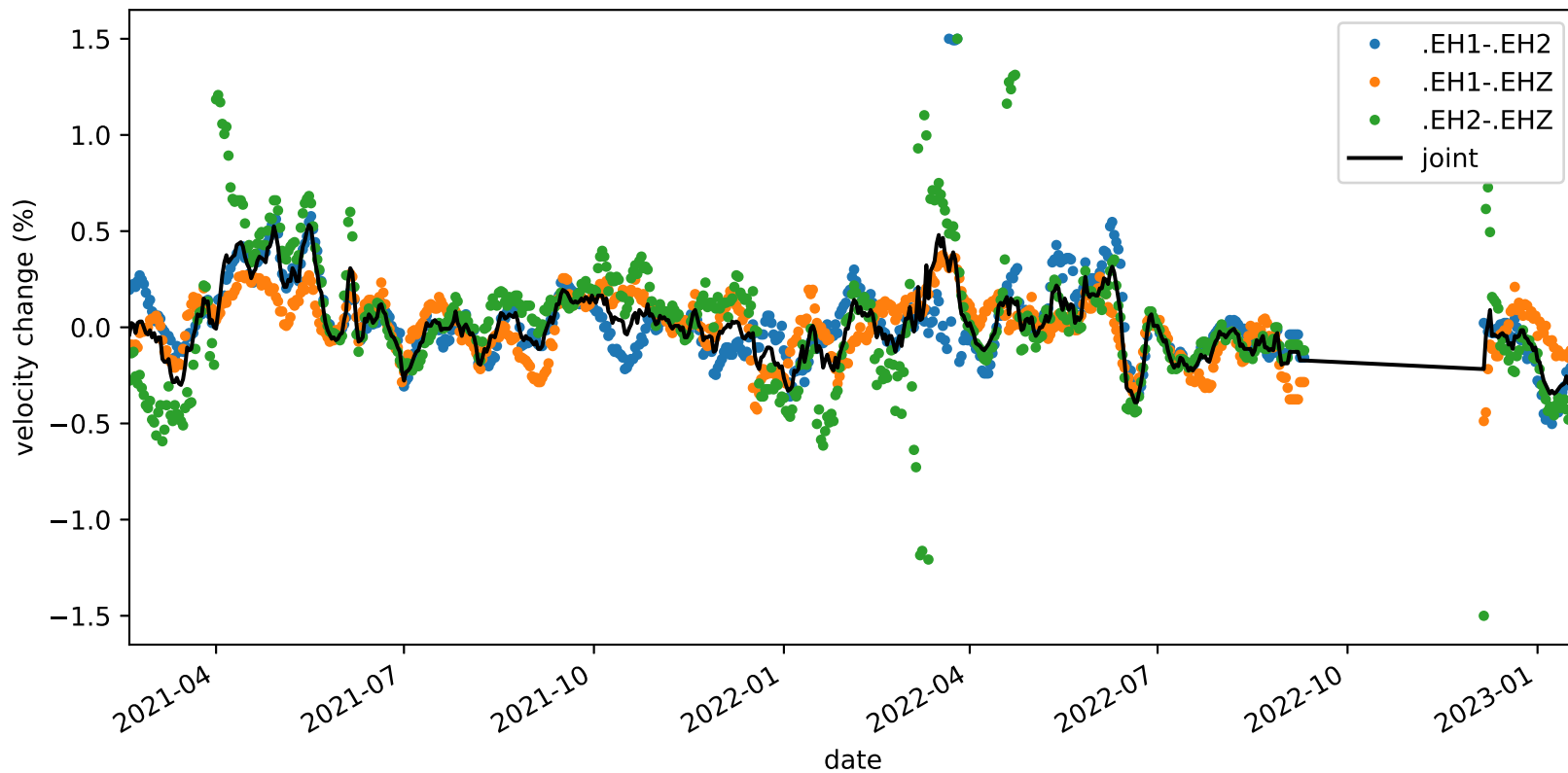
velocity_change_c1i_s3_t1a_tw_005.0s-010.0s_PB.B047-PB.B047
