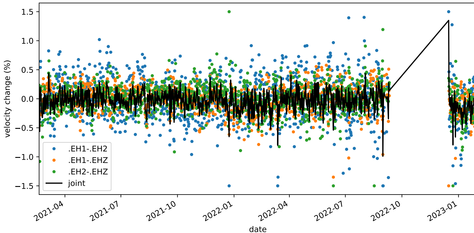
velocity_change_c1f_s1_t1a_tw_005.0s-010.0s_PB.B047-PB.B047
