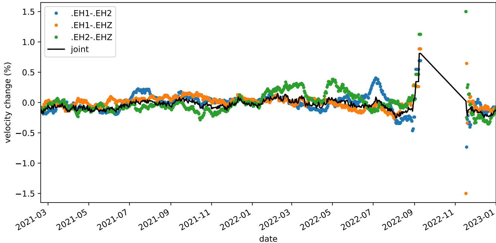
velocity_change_c1d_s2_t1b_tw_010.0s-015.0s_PB.B047-PB.B047
