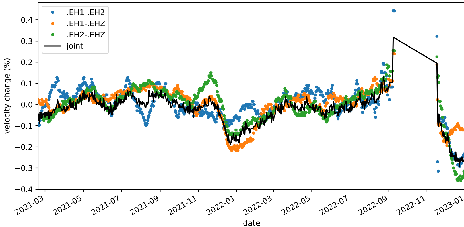
velocity_change_c1g_s2_t1a_tw_005.0s-010.0s_PB.B047-PB.B047
