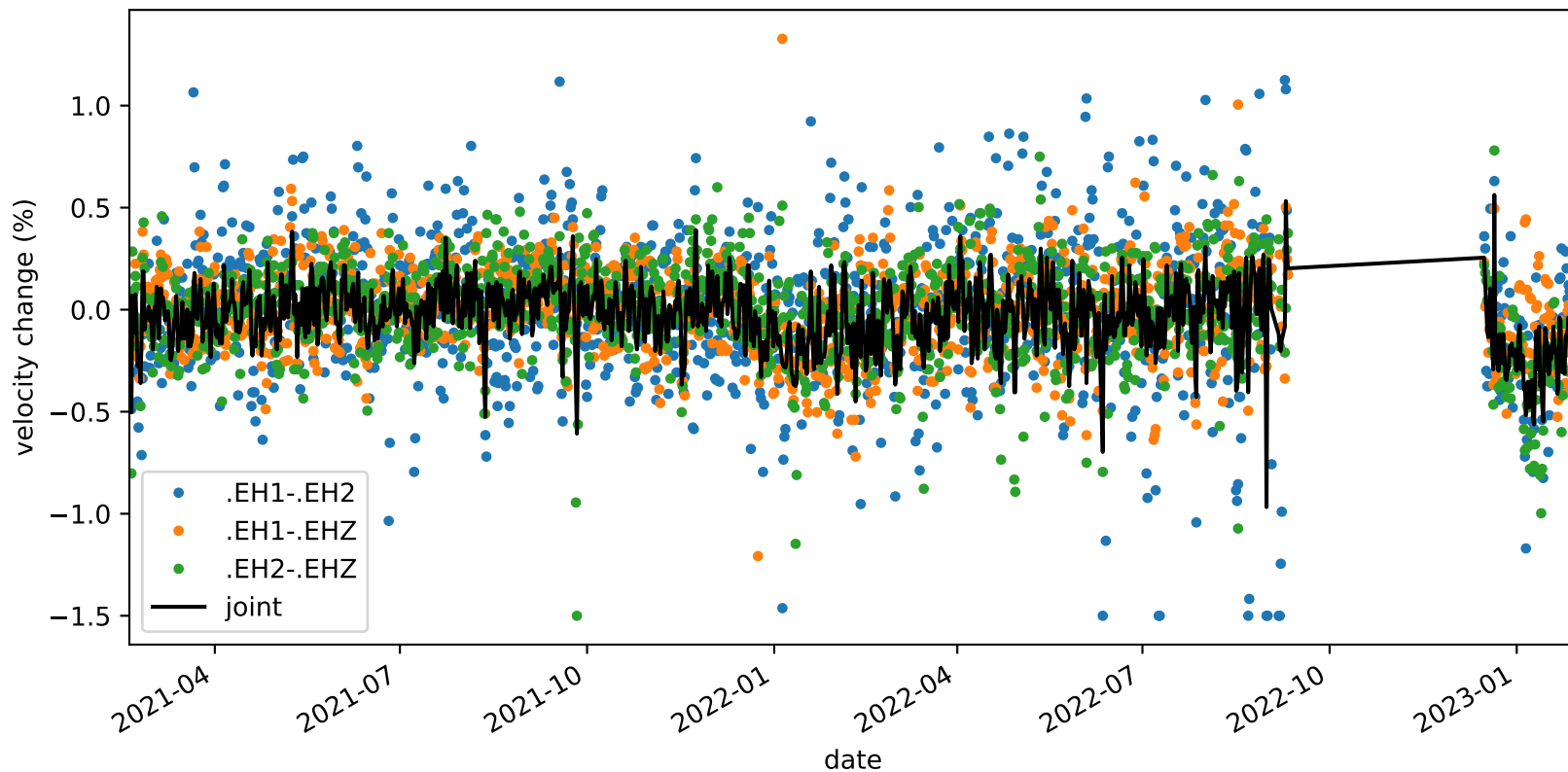
velocity_change_c1g_s1_t1a_tw_005.0s-010.0s_PB.B047-PB.B047
