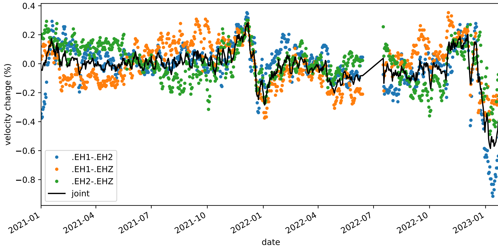
velocity_change_c1h_s4_t1a_tw_005.0s-010.0s_PB.B045-PB.B045
