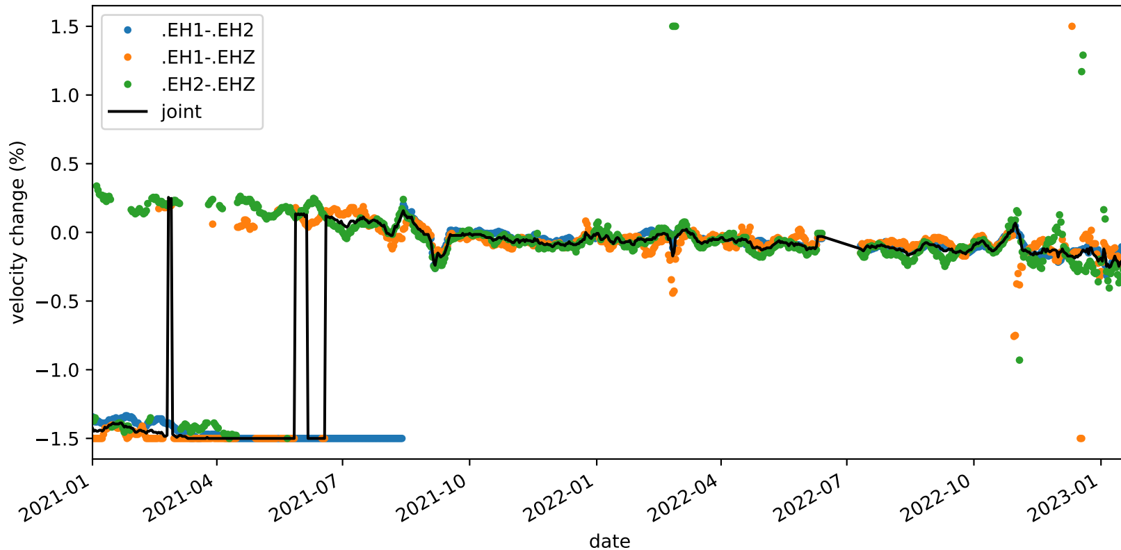
velocity_change_c1c_s3_t1a_tw_005.0s-010.0s_PB.B045-PB.B045
