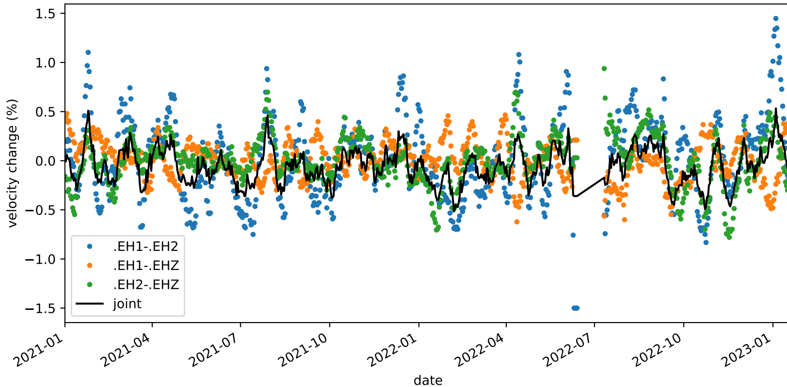
velocity_change_c1d_s3_t1a_tw_005.0s-010.0s_PB.B045-PB.B045
