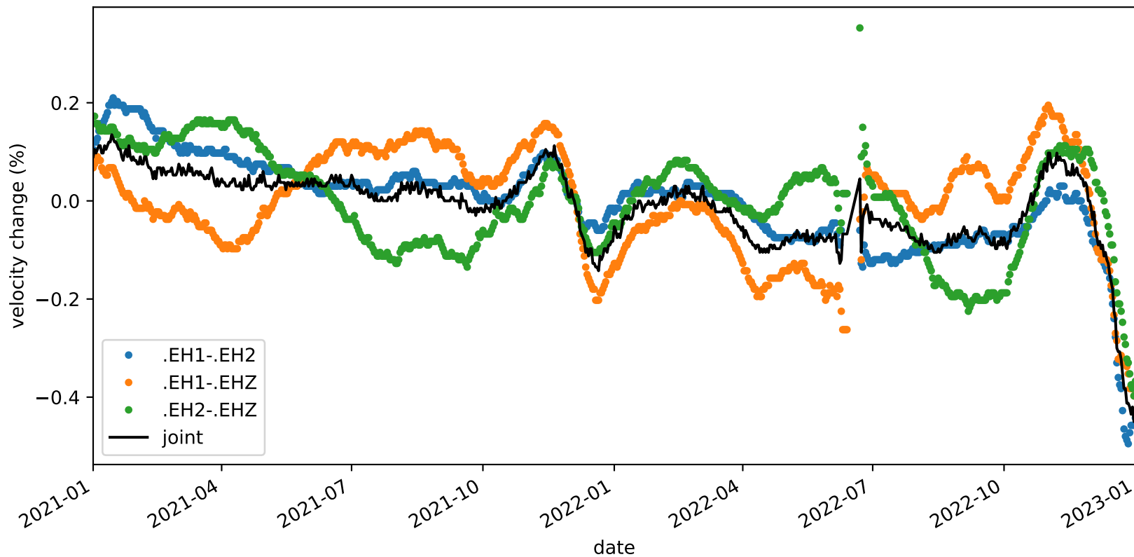
velocity_change_c1i_s2_t1a_tw_005.0s-010.0s_PB.B045-PB.B045
