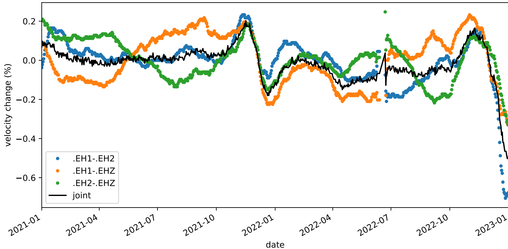
velocity_change_c1h_s2_t1a_tw_005.0s-010.0s_PB.B045-PB.B045
