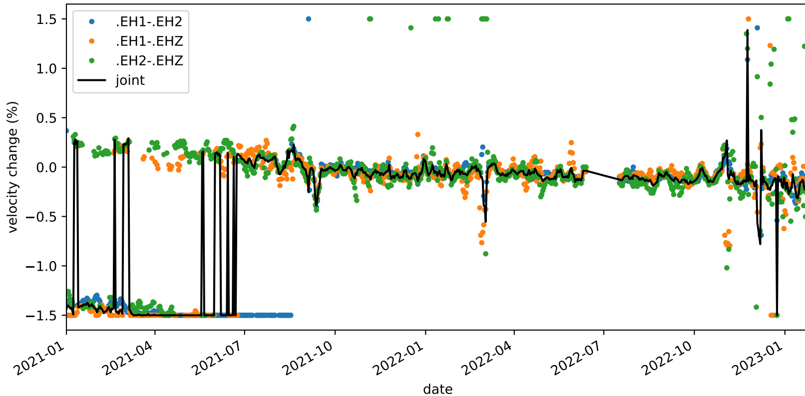
velocity_change_c1c_s4_t1a_tw_005.0s-010.0s_PB.B045-PB.B045
