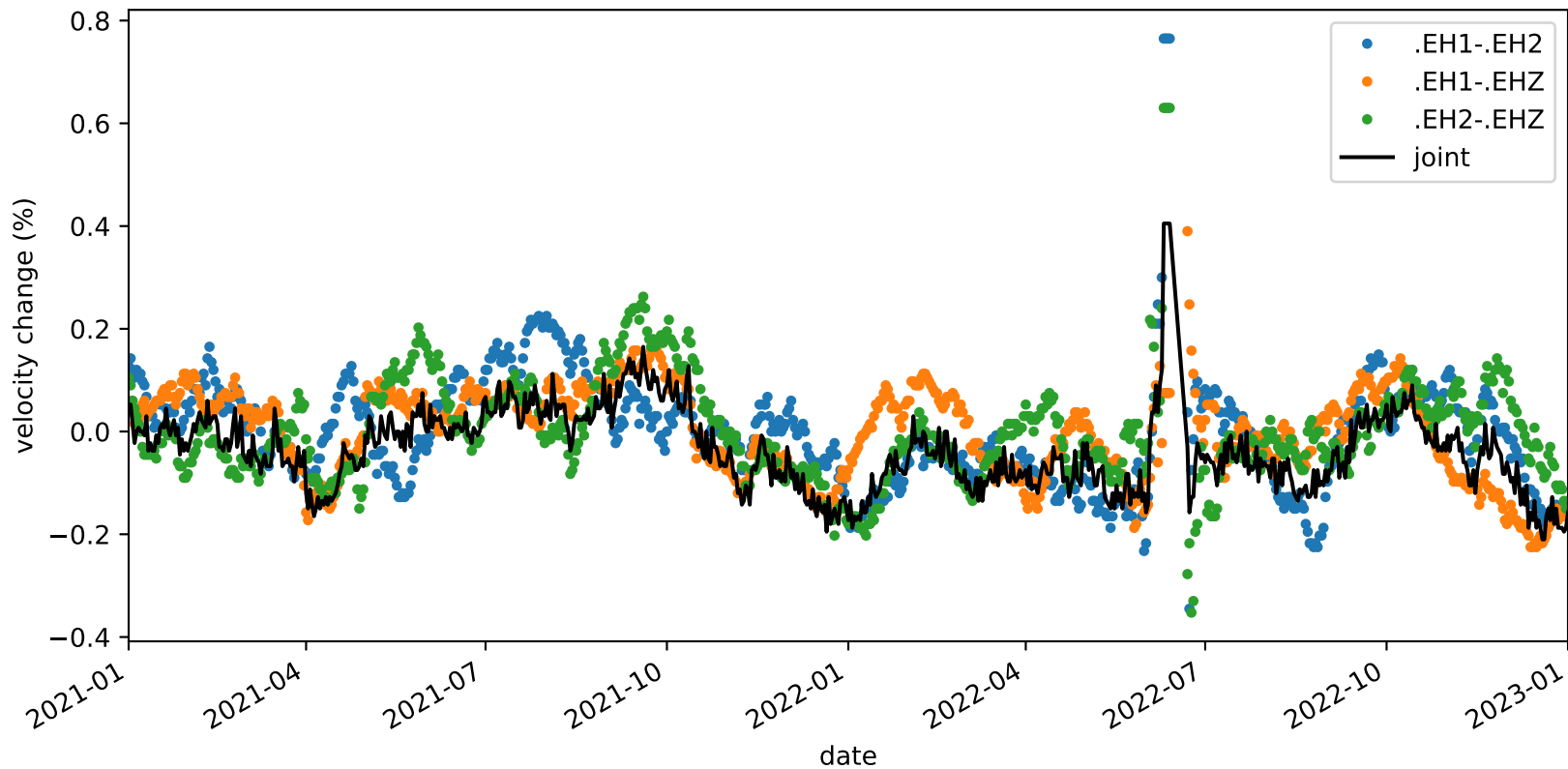
velocity_change_c1d_s2_t1b_tw_010.0s-015.0s_PB.B045-PB.B045
