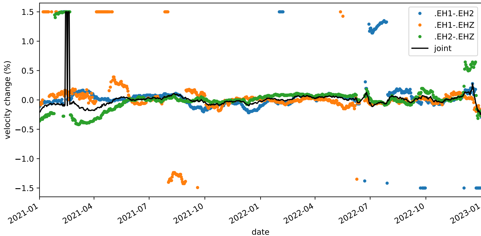
velocity_change_c1_s2_t1b_tw_010.0s-015.0s_PB.B045-PB.B045
