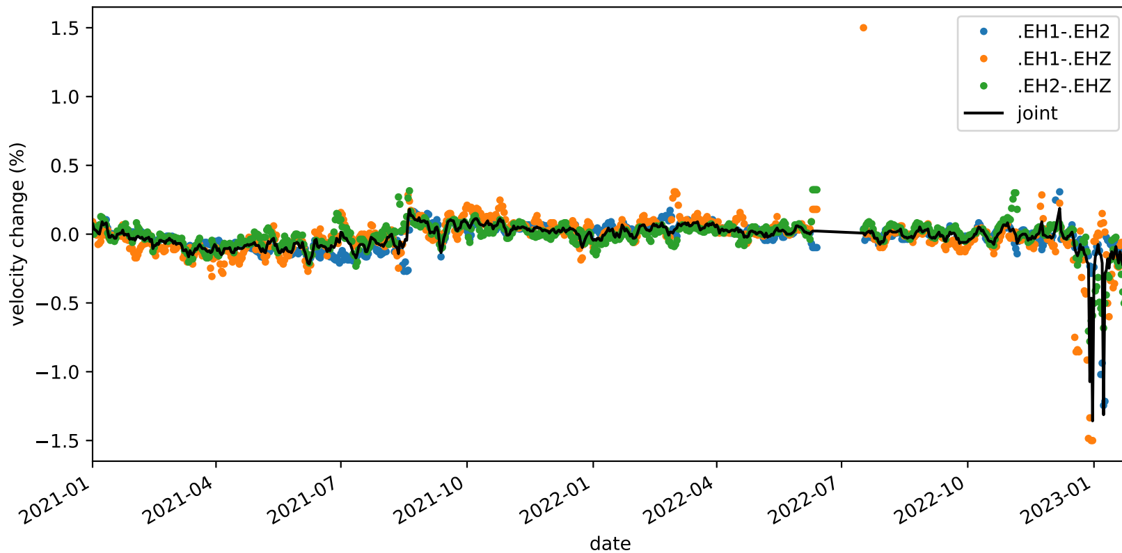
velocity_change_c1i_s4_t1b_tw_010.0s-015.0s_PB.B045-PB.B045
