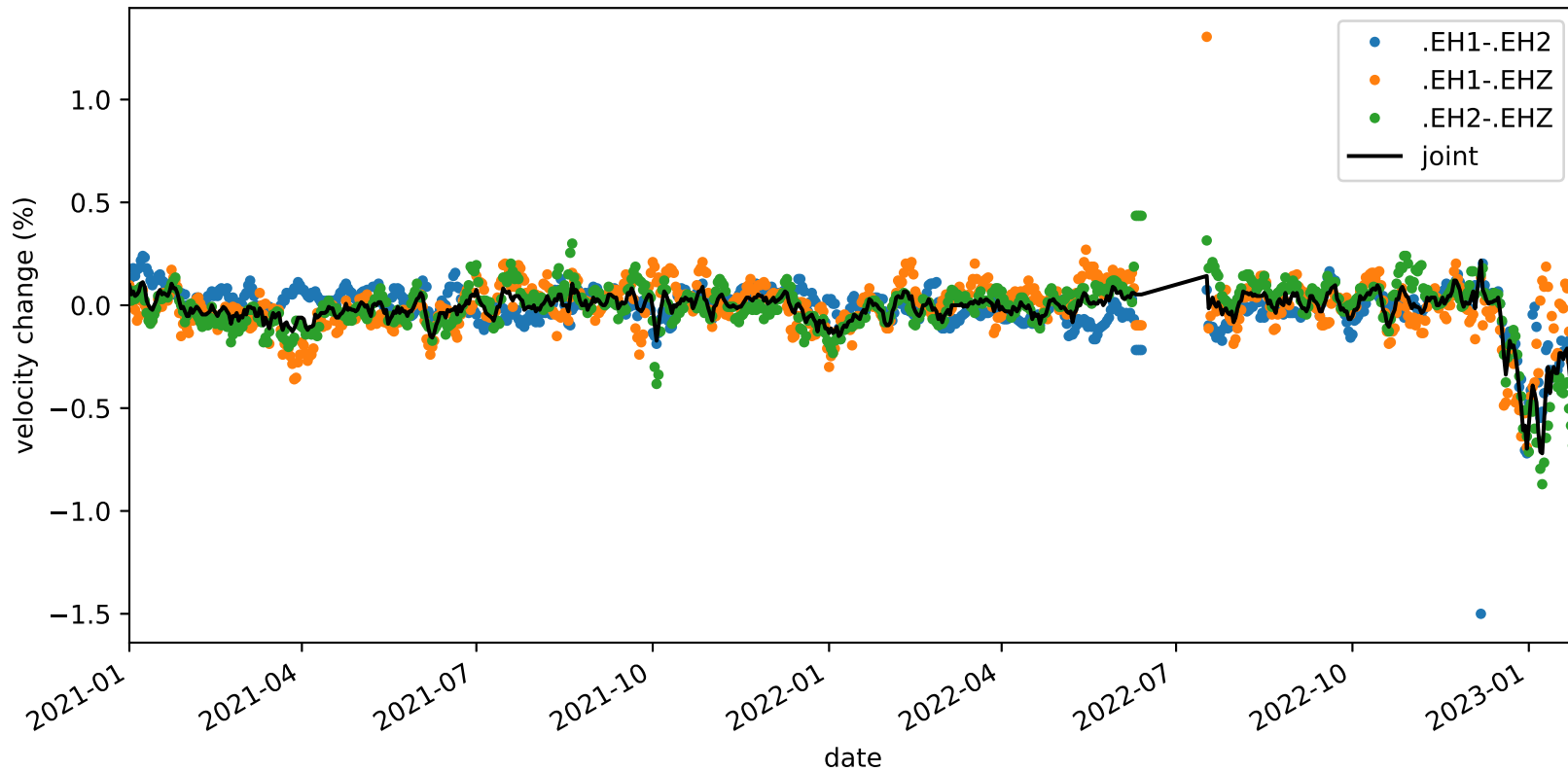
velocity_change_c1h_s4_t1b_tw_010.0s-015.0s_PB.B045-PB.B045
