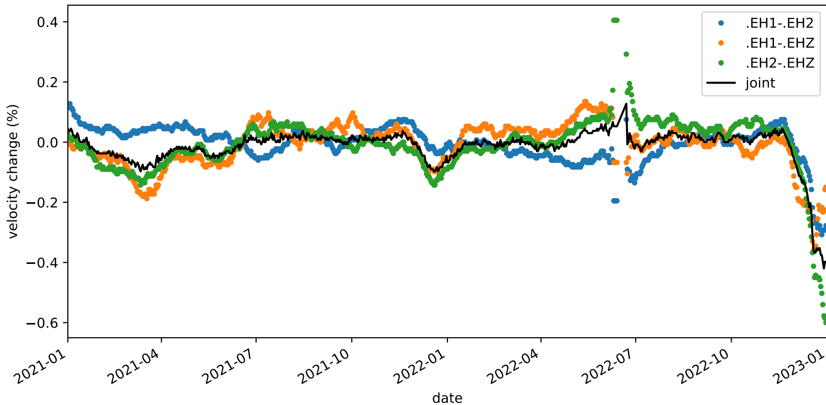
velocity_change_c1h_s2_t1b_tw_010.0s-015.0s_PB.B045-PB.B045
