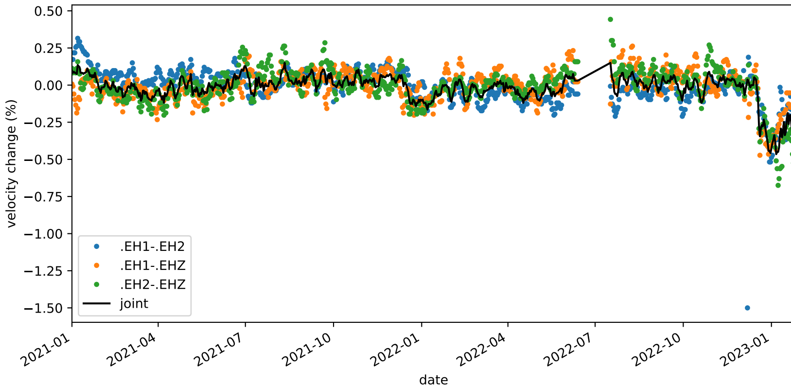
velocity_change_c1g_s4_t1b_tw_010.0s-015.0s_PB.B045-PB.B045
