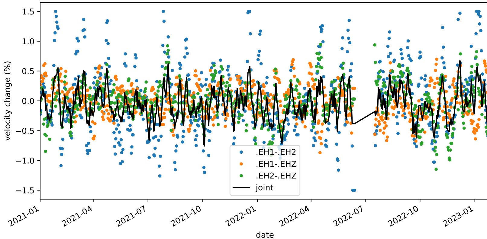
velocity_change_c1d_s4_t1a_tw_005.0s-010.0s_PB.B045-PB.B045
