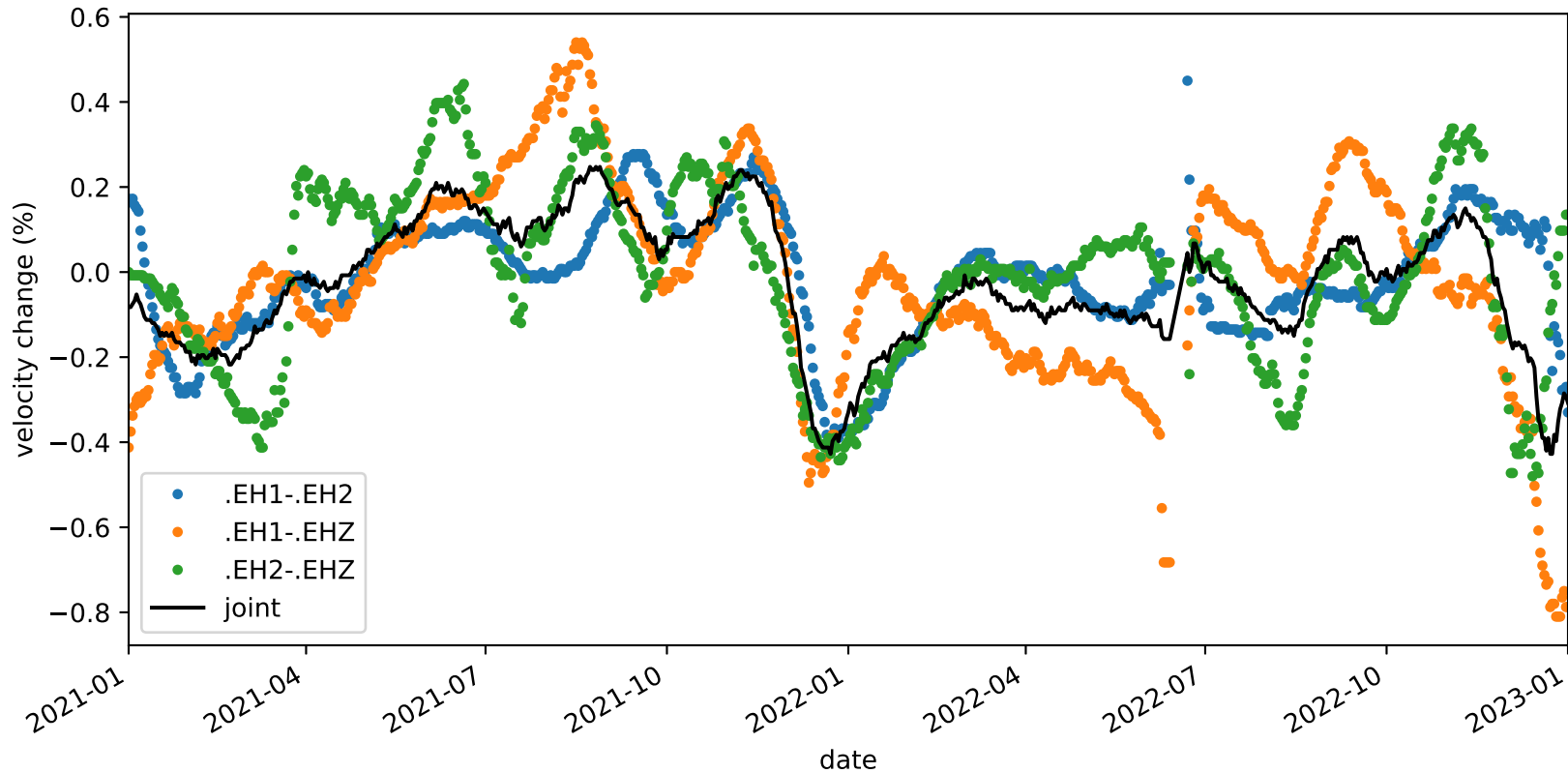
velocity_change_c1_s2_t1a_tw_005.0s-010.0s_PB.B045-PB.B045
