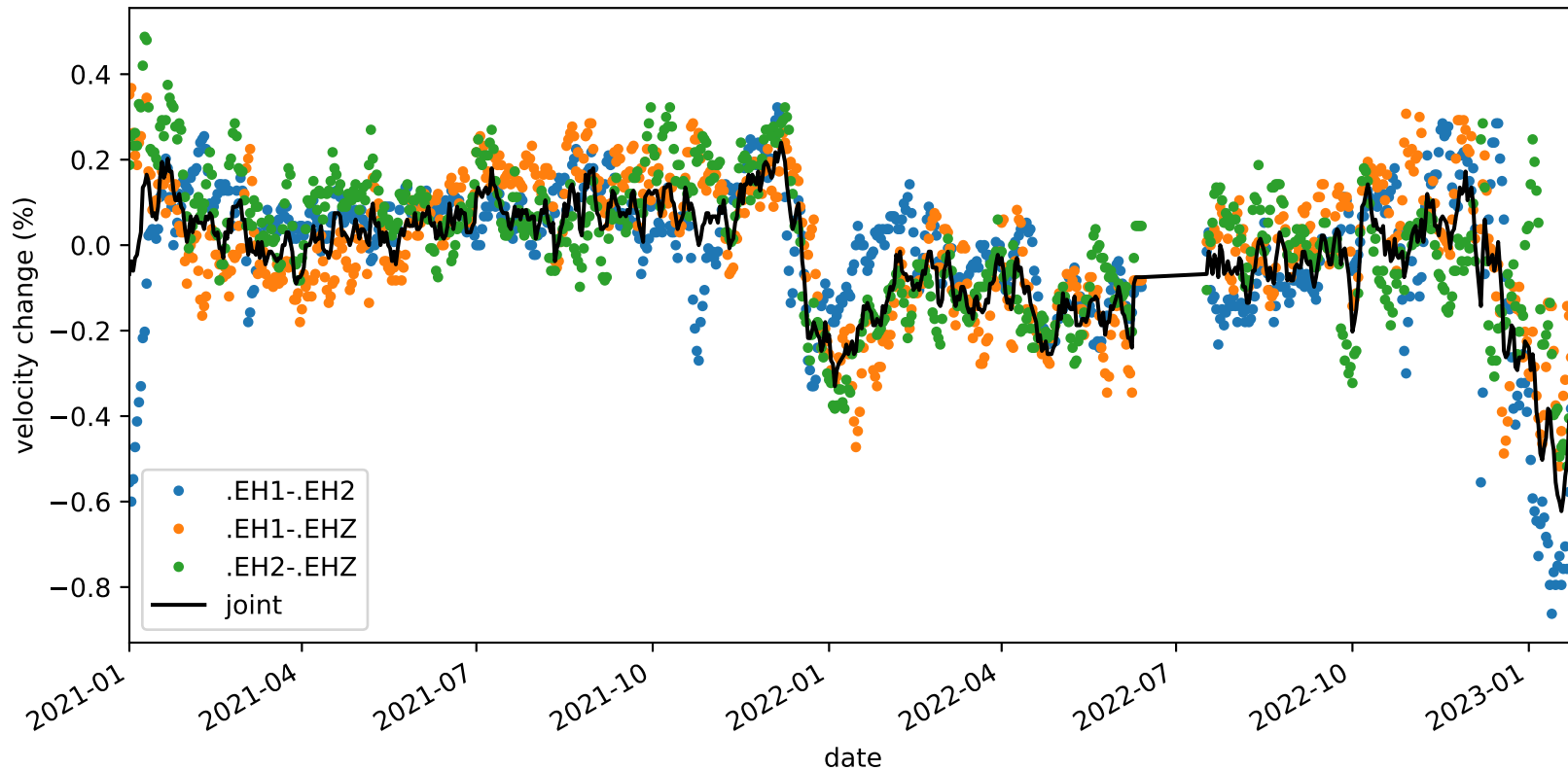
velocity_change_c1f_s4_t1a_tw_005.0s-010.0s_PB.B045-PB.B045
