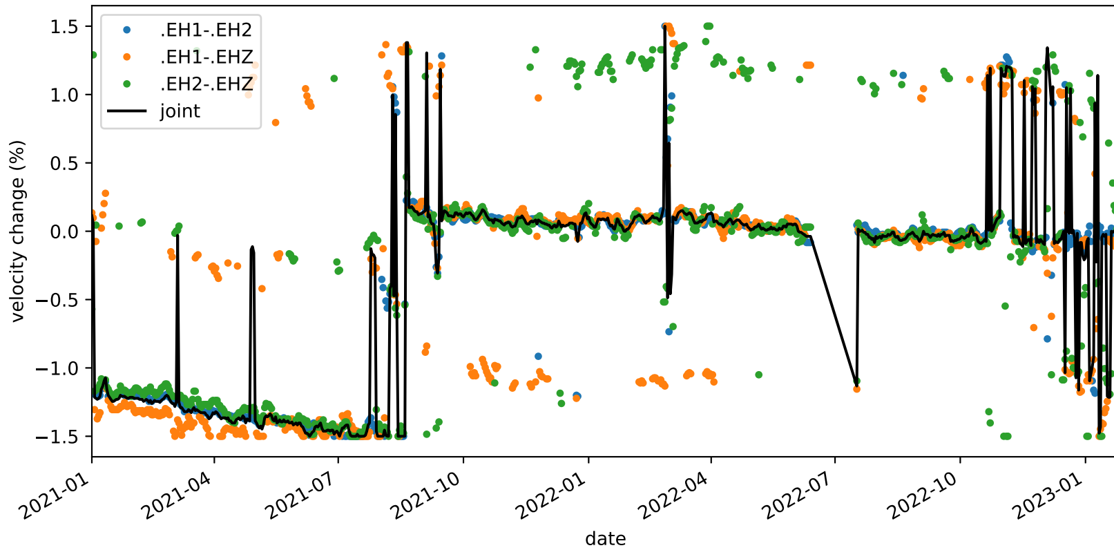
velocity_change_c1c_s4_t1b_tw_010.0s-015.0s_PB.B045-PB.B045
