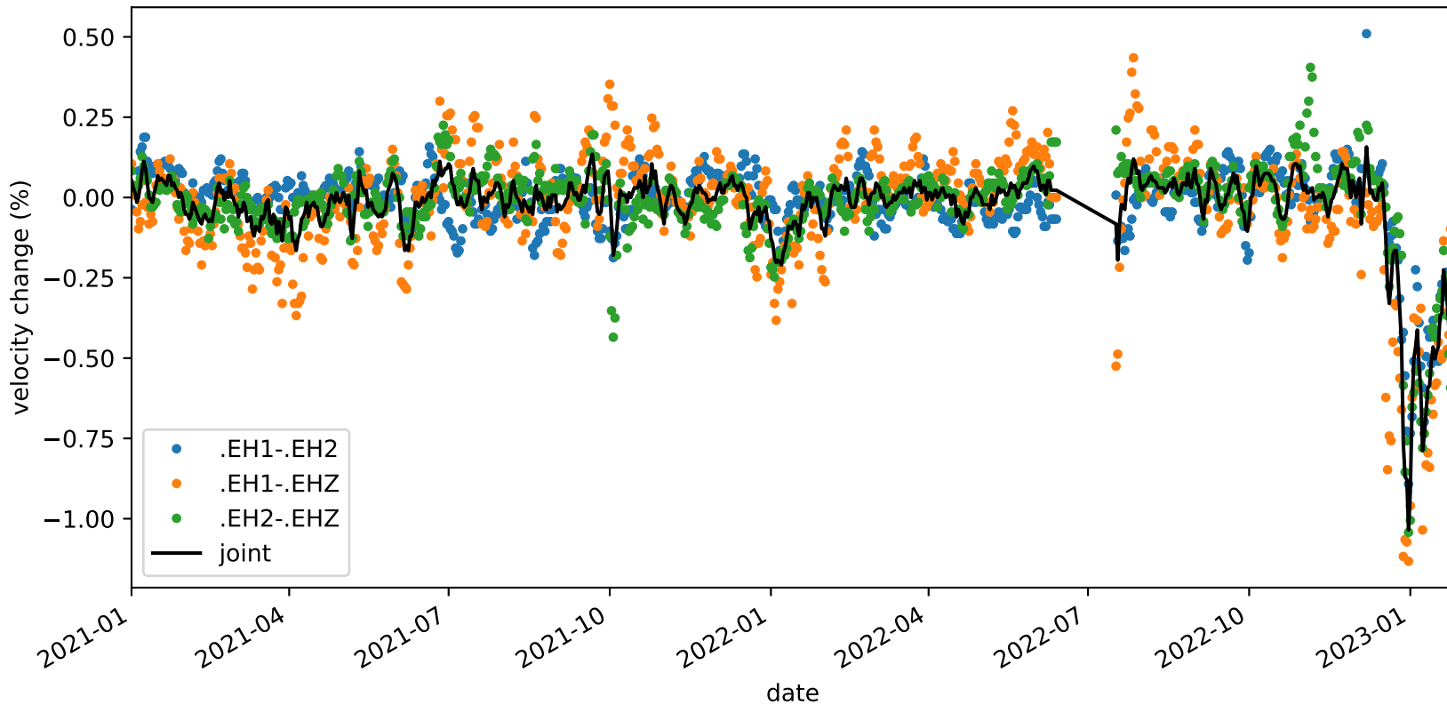
velocity_change_c1b_s4_t1b_tw_010.0s-015.0s_PB.B045-PB.B045
