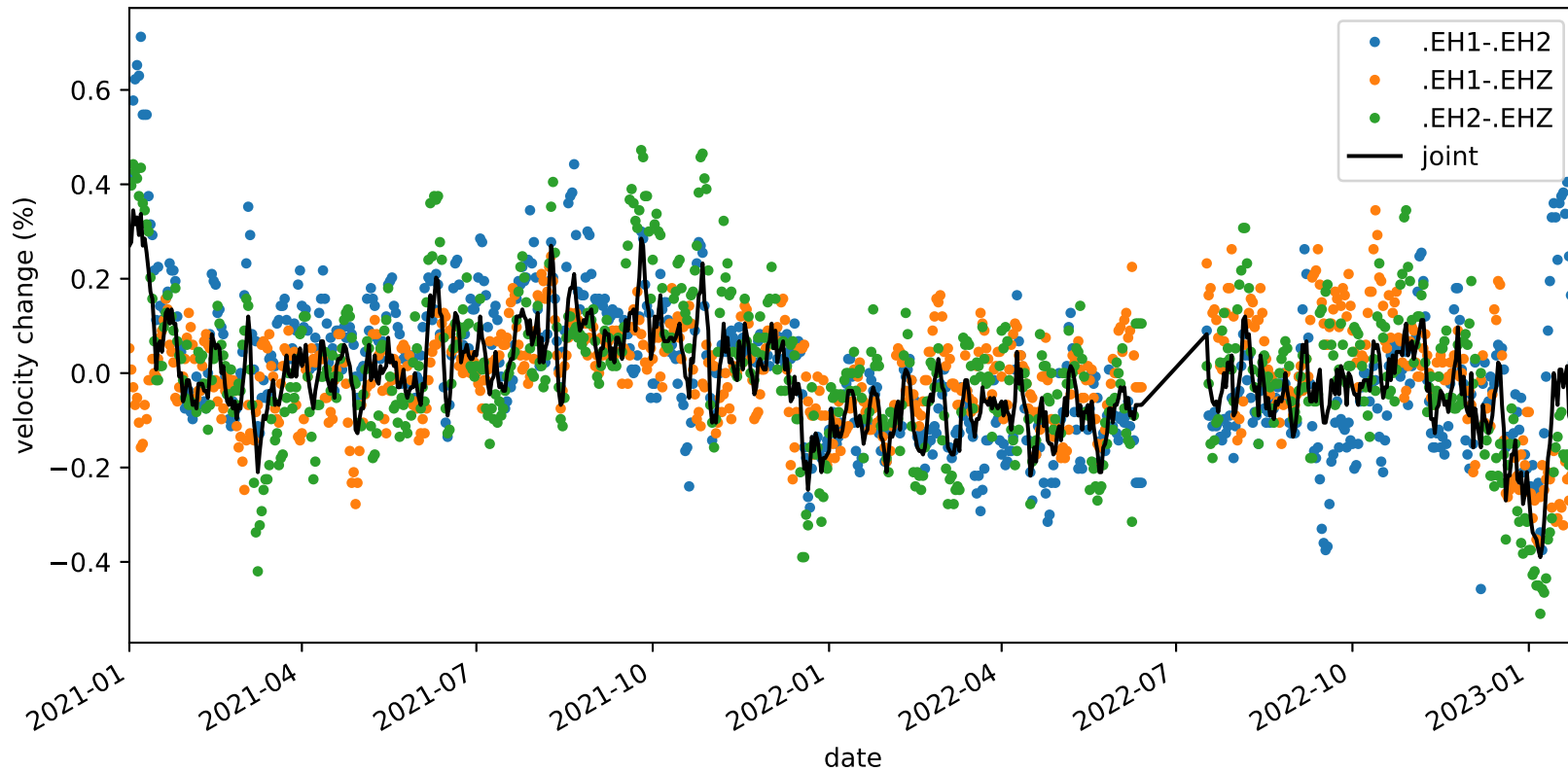
velocity_change_c1e_s4_t1b_tw_010.0s-015.0s_PB.B045-PB.B045
