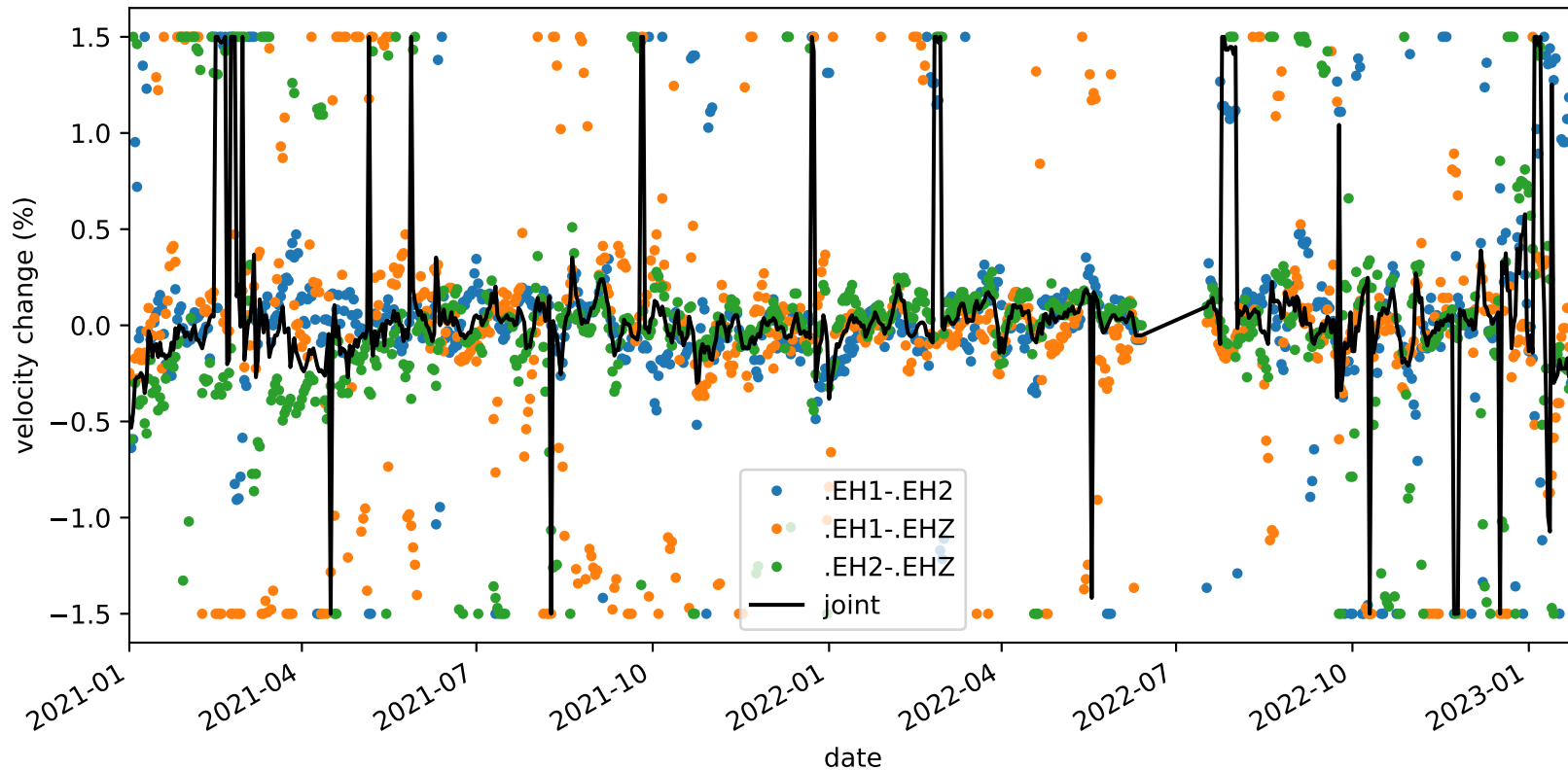
velocity_change_c1_s4_t1b_tw_010.0s-015.0s_PB.B045-PB.B045
