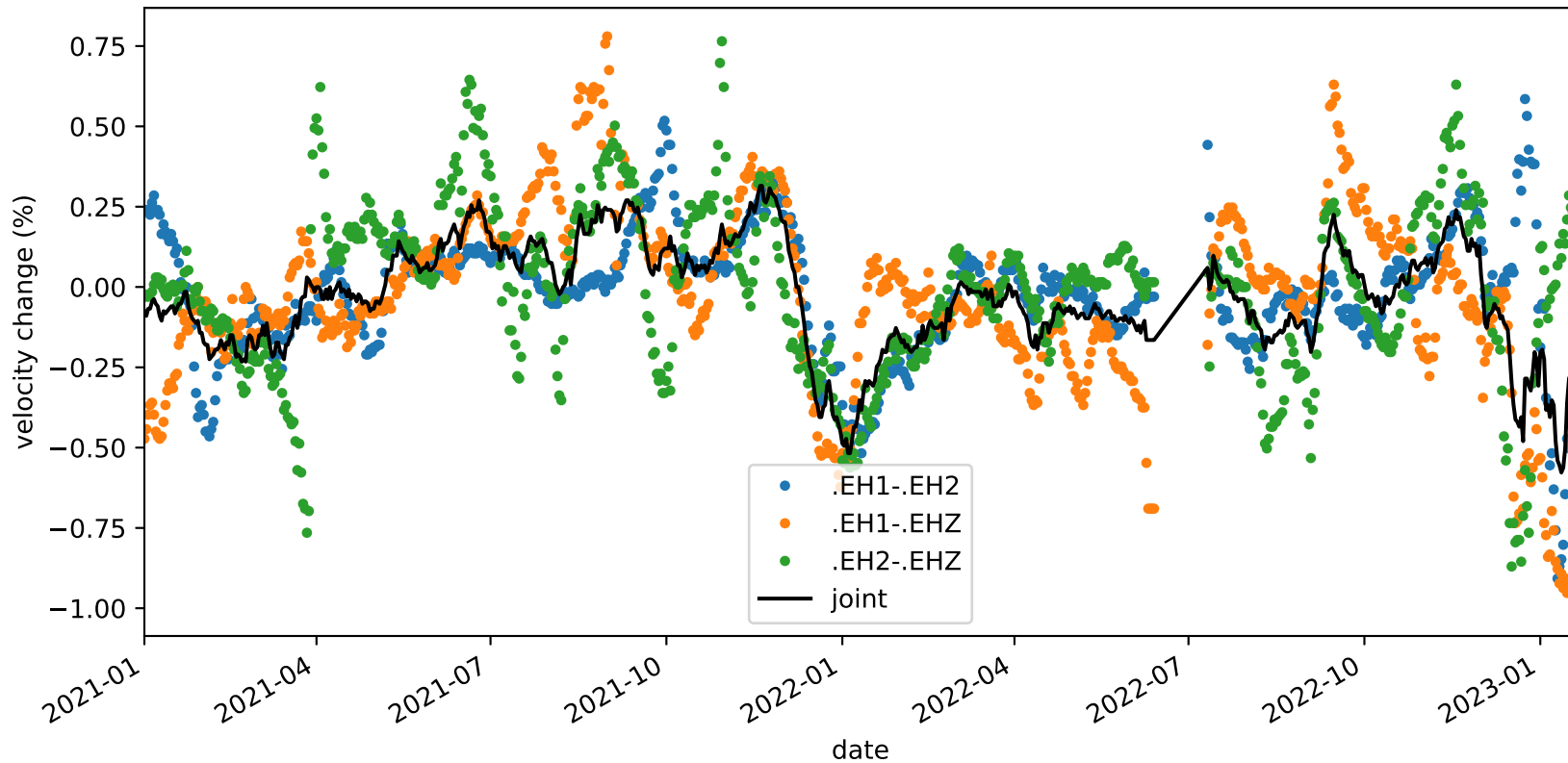
velocity_change_c1_s3_t1a_tw_005.0s-010.0s_PB.B045-PB.B045
