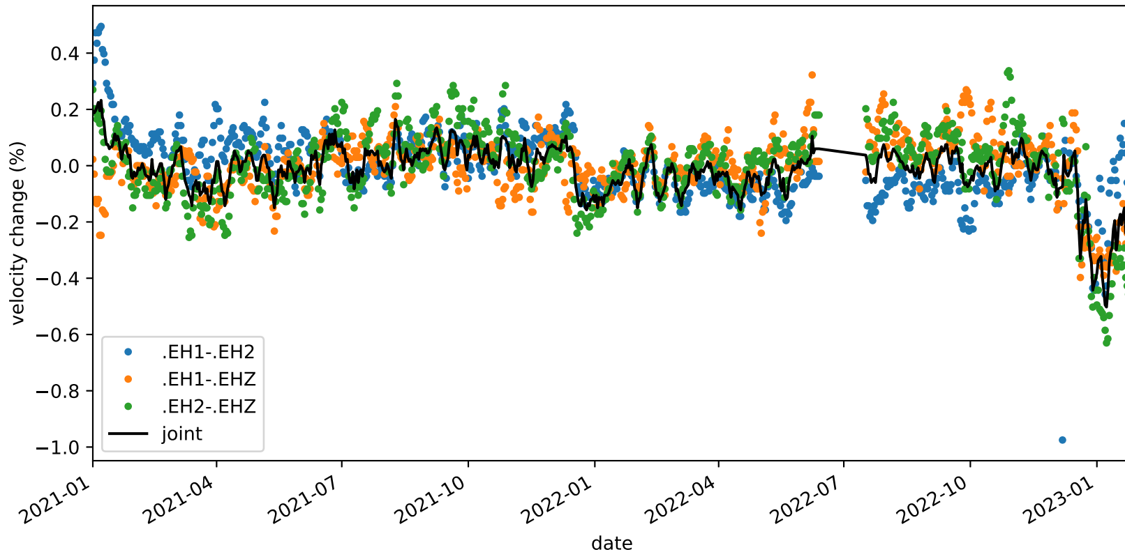
velocity_change_c1f_s4_t1b_tw_010.0s-015.0s_PB.B045-PB.B045
