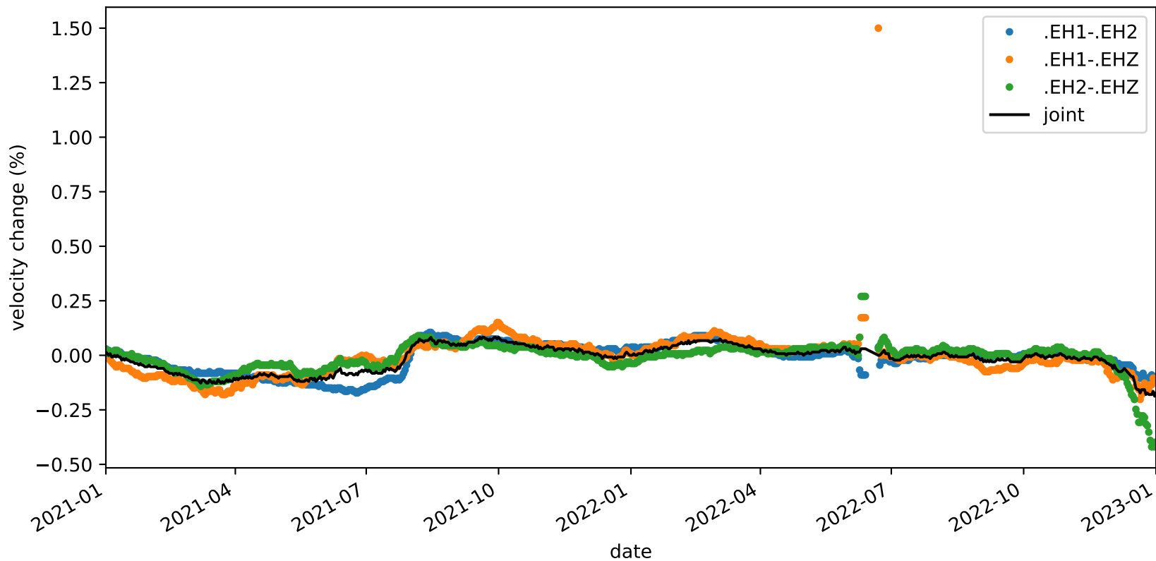
velocity_change_c1i_s2_t1b_tw_010.0s-015.0s_PB.B045-PB.B045
