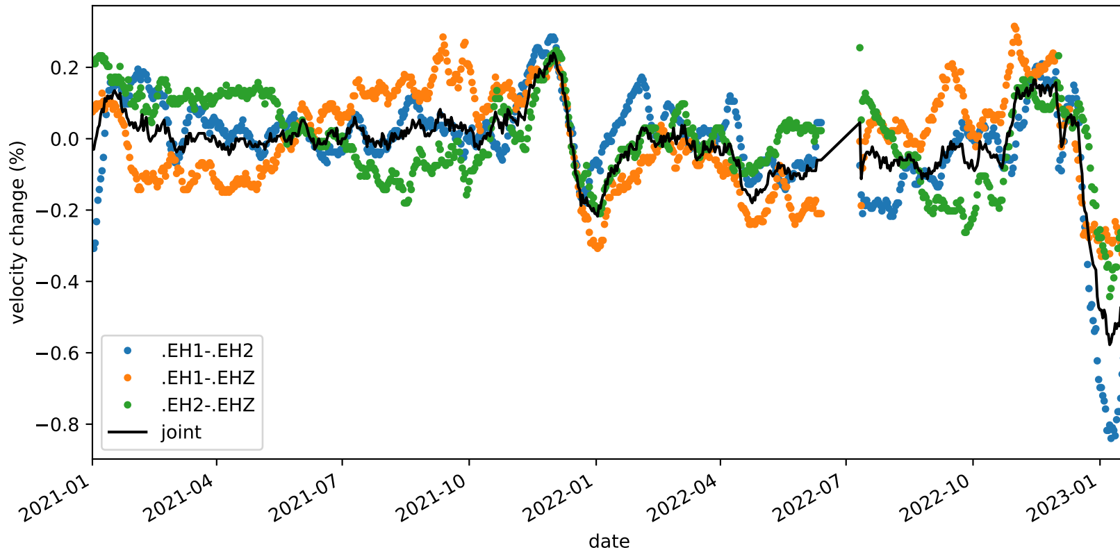
velocity_change_c1h_s3_t1a_tw_005.0s-010.0s_PB.B045-PB.B045
