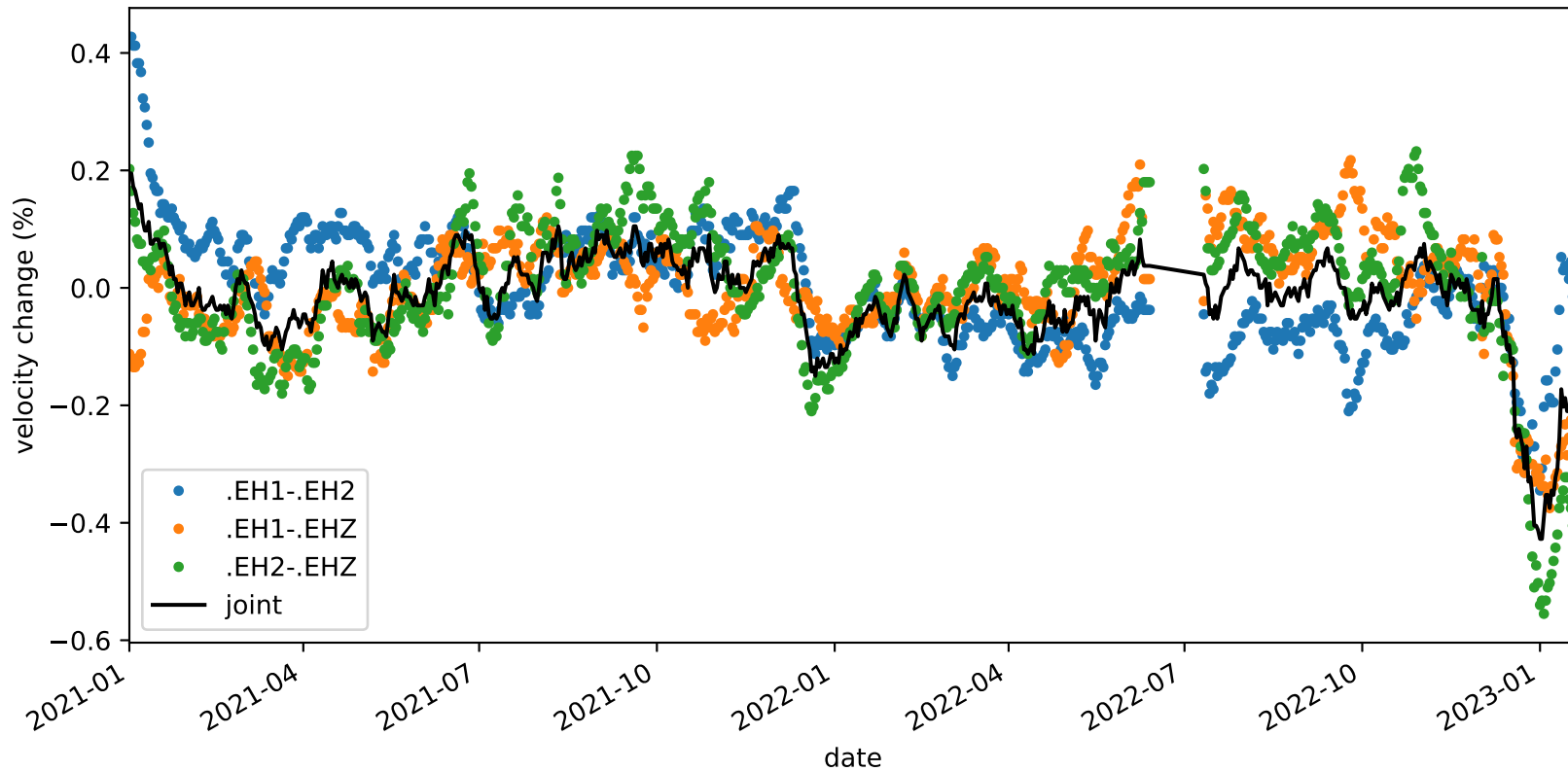
velocity_change_c1f_s3_t1b_tw_010.0s-015.0s_PB.B045-PB.B045
