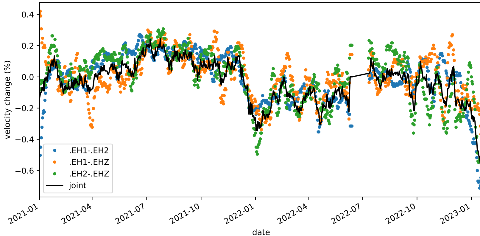
velocity_change_c1e_s3_t1a_tw_005.0s-010.0s_PB.B045-PB.B045
