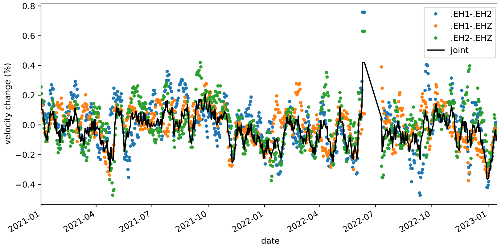
velocity_change_c1d_s3_t1b_tw_010.0s-015.0s_PB.B045-PB.B045
