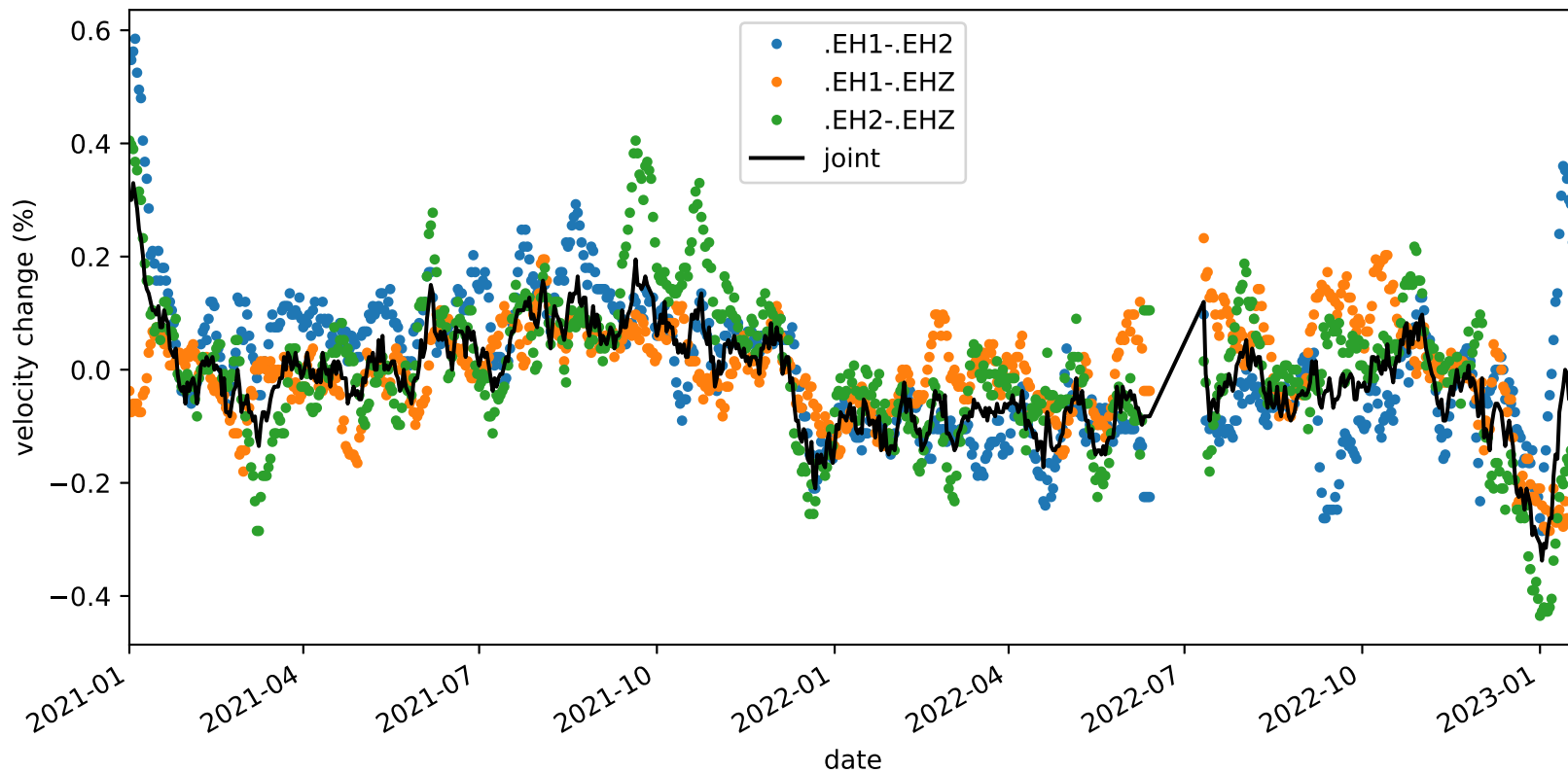
velocity_change_c1e_s3_t1b_tw_010.0s-015.0s_PB.B045-PB.B045
