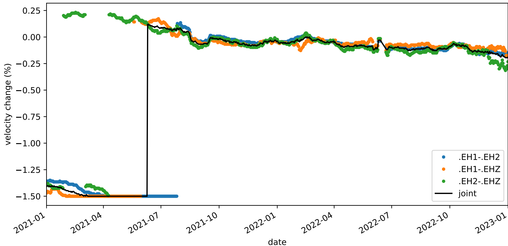
velocity_change_c1c_s2_t1a_tw_005.0s-010.0s_PB.B045-PB.B045
