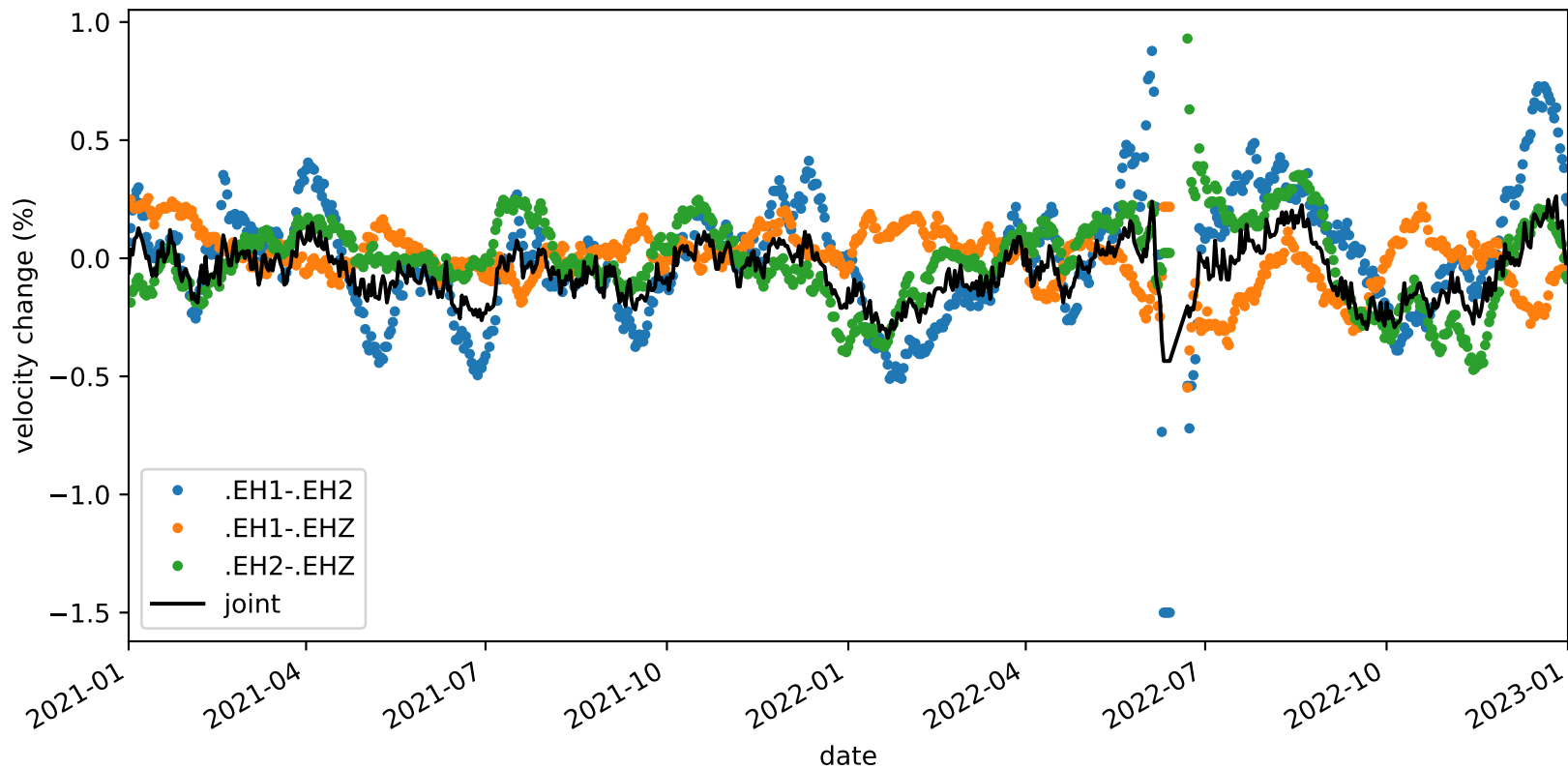
velocity_change_c1d_s2_t1a_tw_005.0s-010.0s_PB.B045-PB.B045
