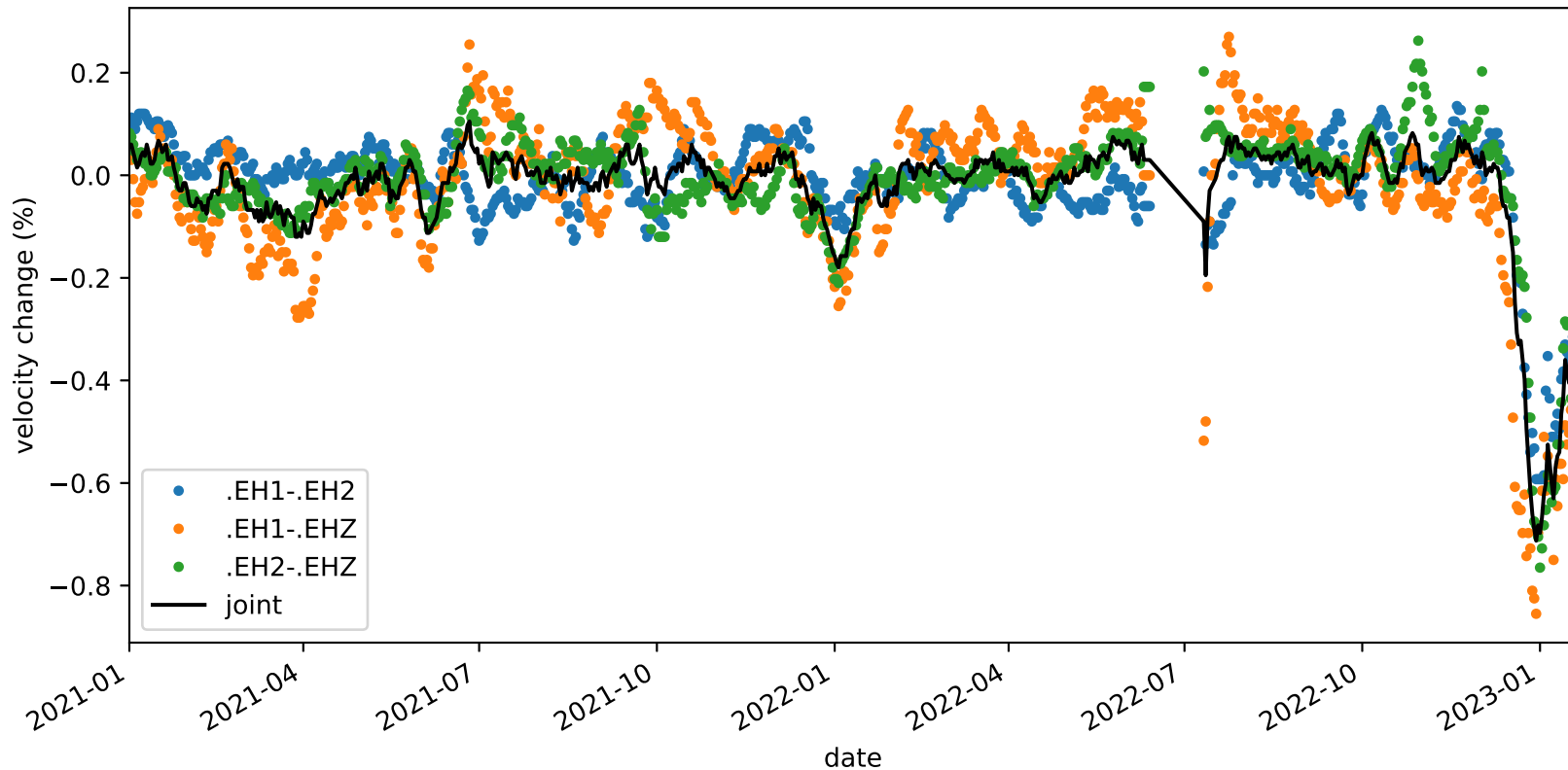
velocity_change_c1b_s3_t1b_tw_010.0s-015.0s_PB.B045-PB.B045
