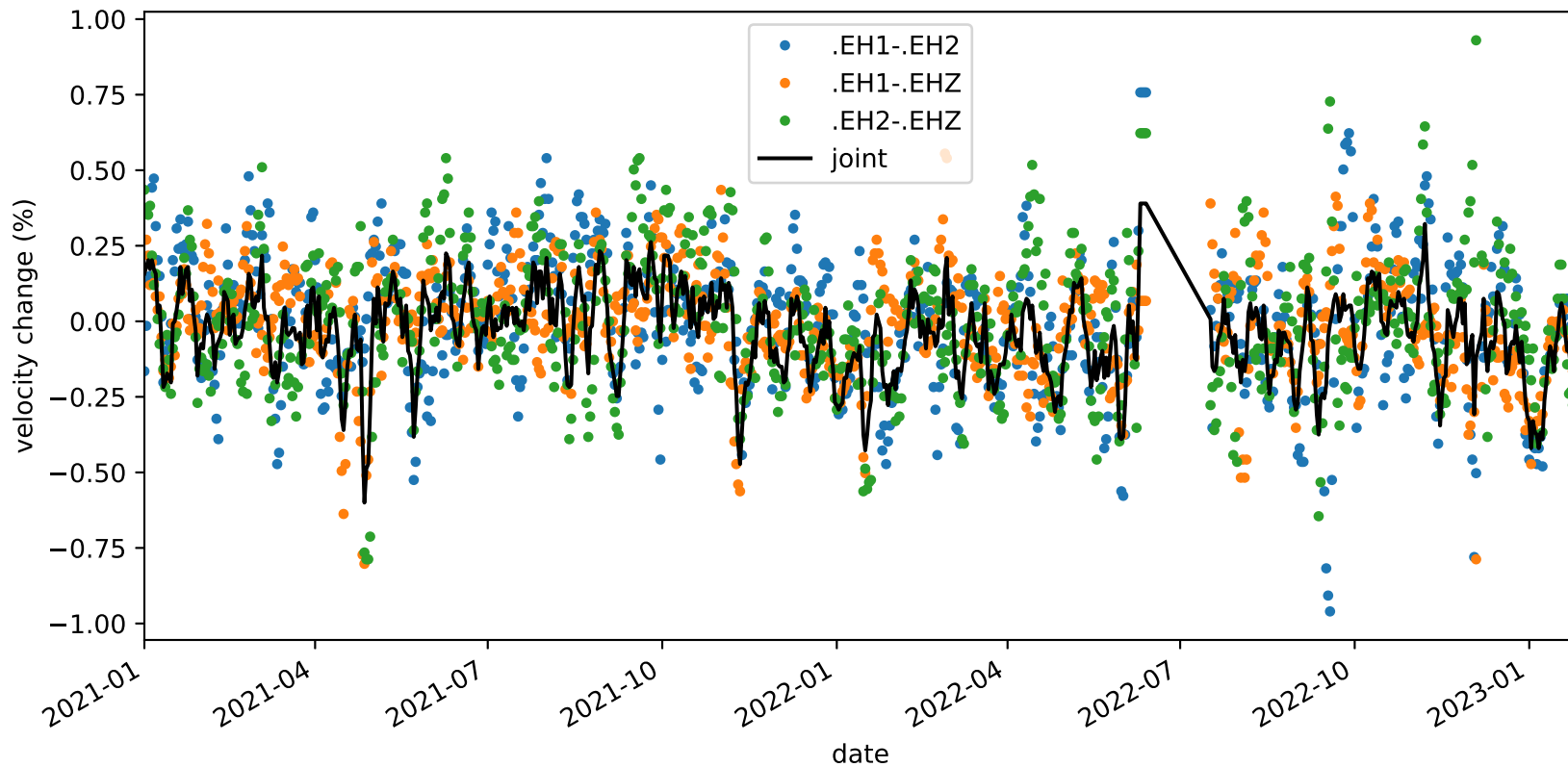
velocity_change_c1d_s4_t1b_tw_010.0s-015.0s_PB.B045-PB.B045
