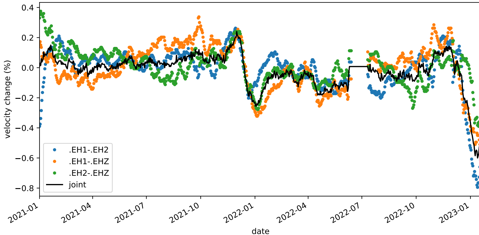
velocity_change_c1g_s3_t1a_tw_005.0s-010.0s_PB.B045-PB.B045
