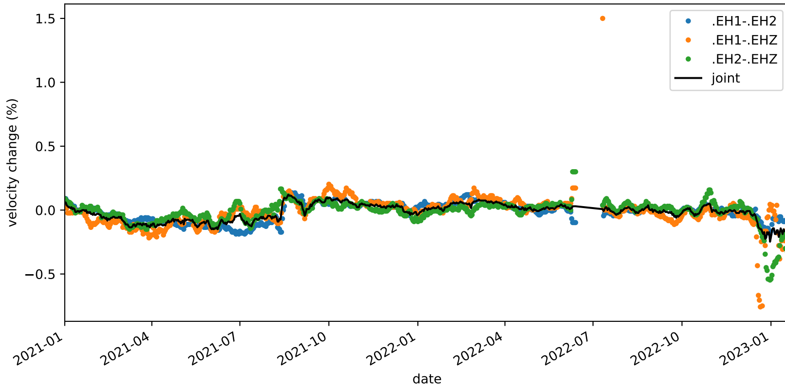
velocity_change_cli_s3_t1b_tw_010.0s-015.0s_PB.B045-PB.B045
