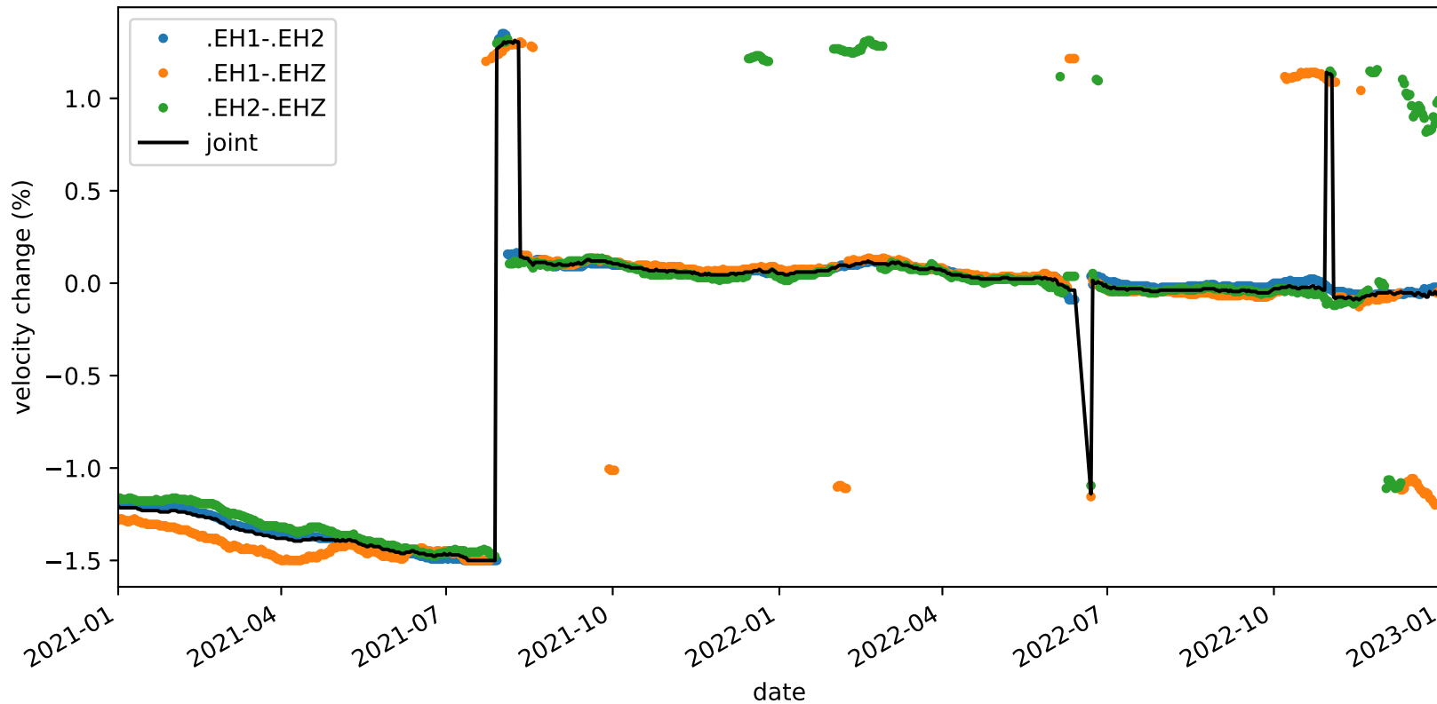
velocity_change_c1c_s2_t1b_tw_010.0s-015.0s_PB.B045-PB.B045
