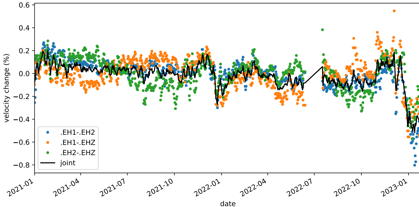
velocity_change_cli_s4_t1a_tw_005.0s-010.0s_PB.B045-PB.B045
