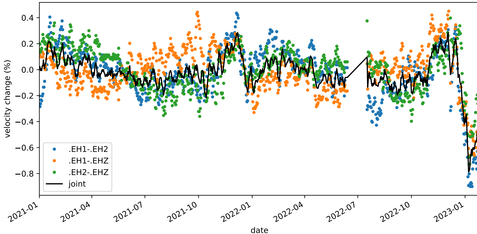
velocity_change_c1b_s4_t1a_tw_005.0s-010.0s_PB.B045-PB.B045
