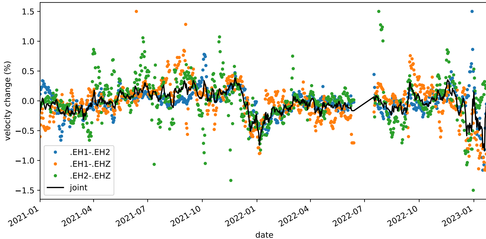
velocity_change_c1_s4_t1a_tw_005.0s-010.0s_PB.B045-PB.B045
