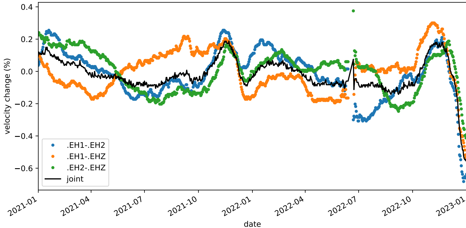
velocity_change_c1b_s2_t1a_tw_005.0s-010.0s_PB.B045-PB.B045
