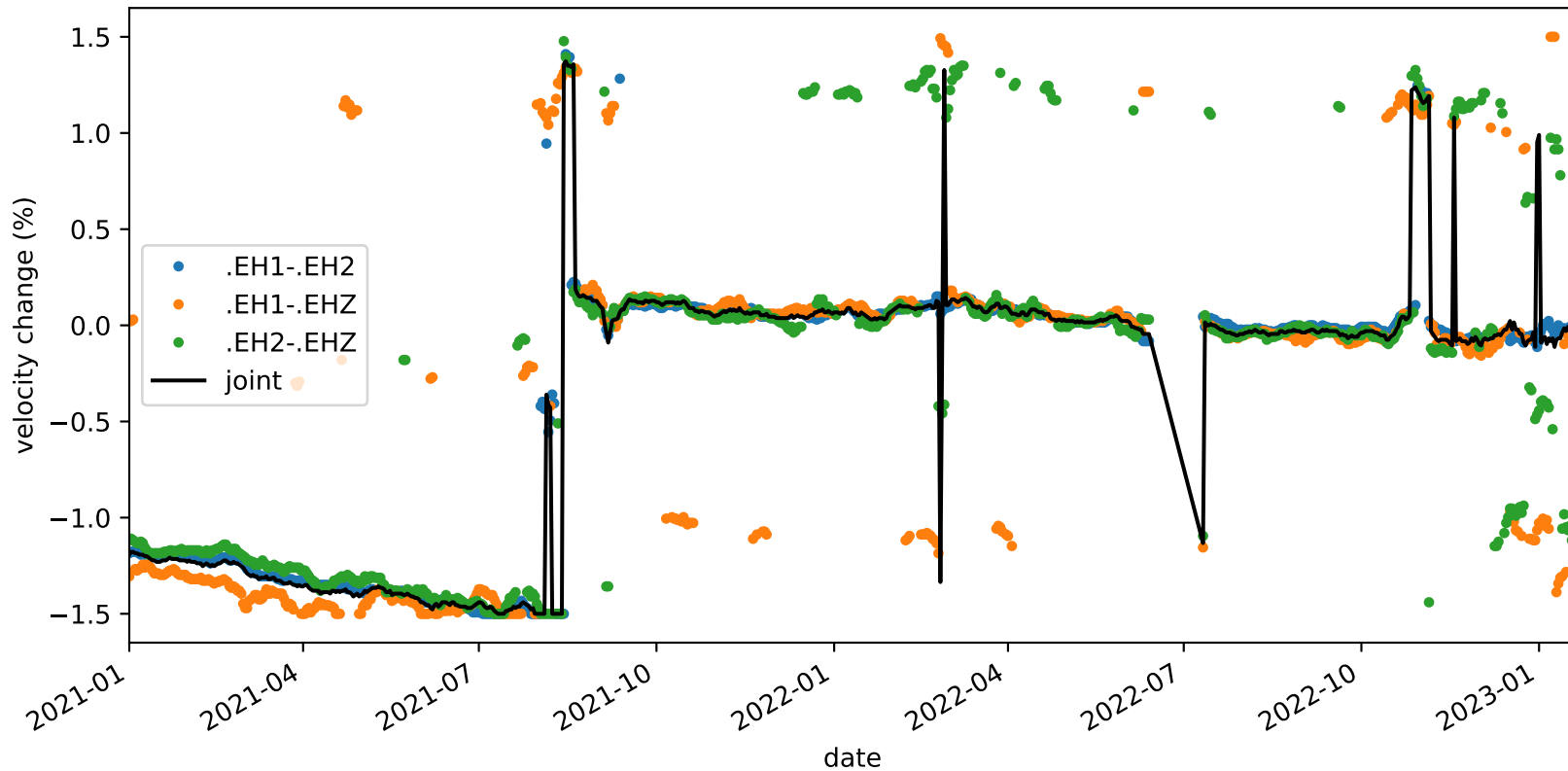
velocity_change_c1c_s3_t1b_tw_010.0s-015.0s_PB.B045-PB.B045
