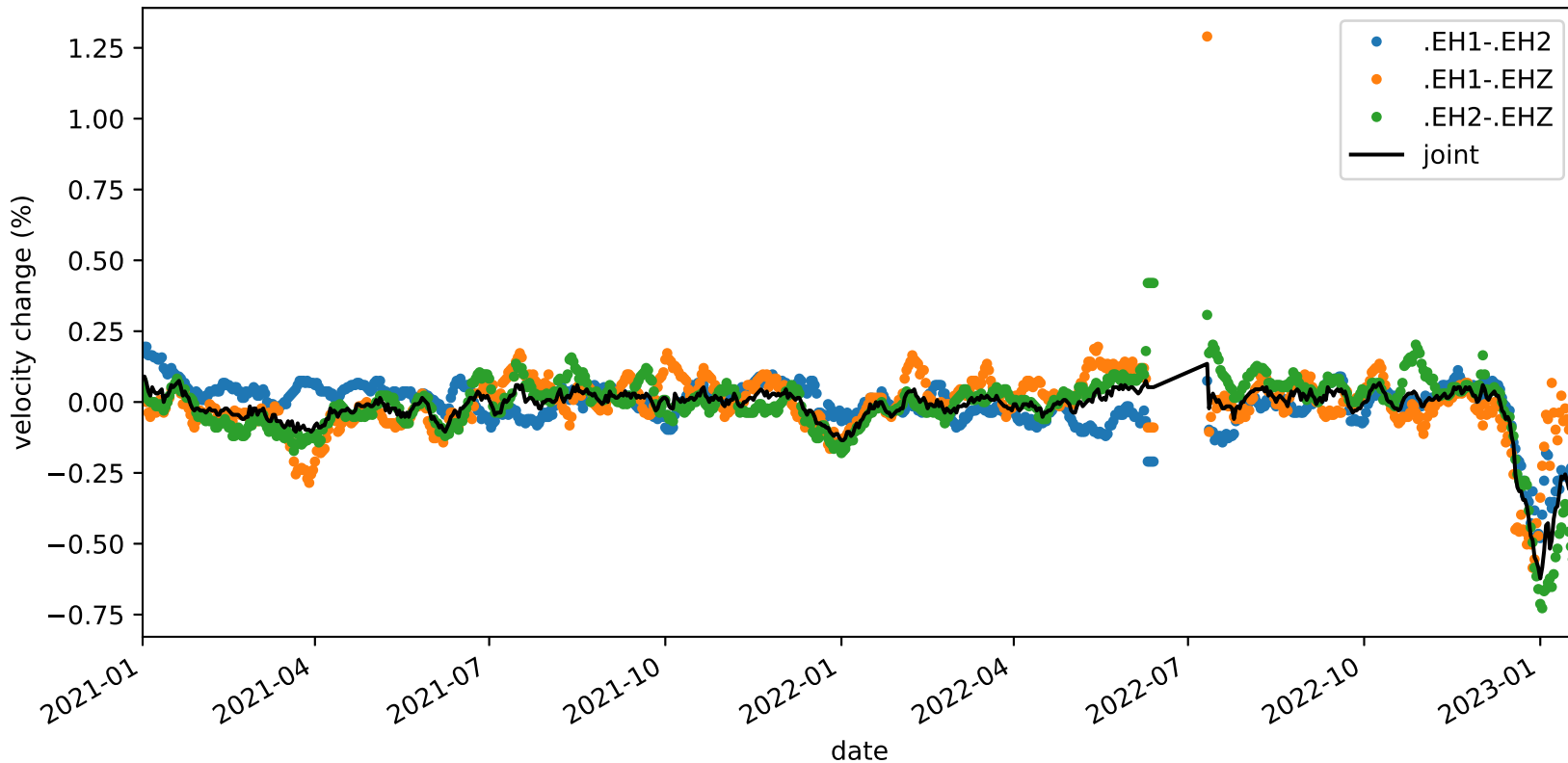
velocity_change_c1h_s3_t1b_tw_010.0s-015.0s_PB.B045-PB.B045
