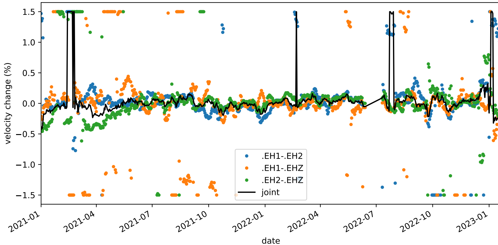
velocity_change_c1_s3_t1b_tw_010.0s-015.0s_PB.B045-PB.B045
