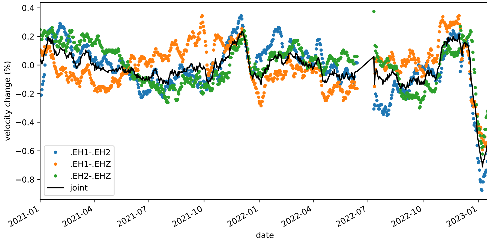
velocity_change_c1b_s3_t1a_tw_005.0s-010.0s_PB.B045-PB.B045
