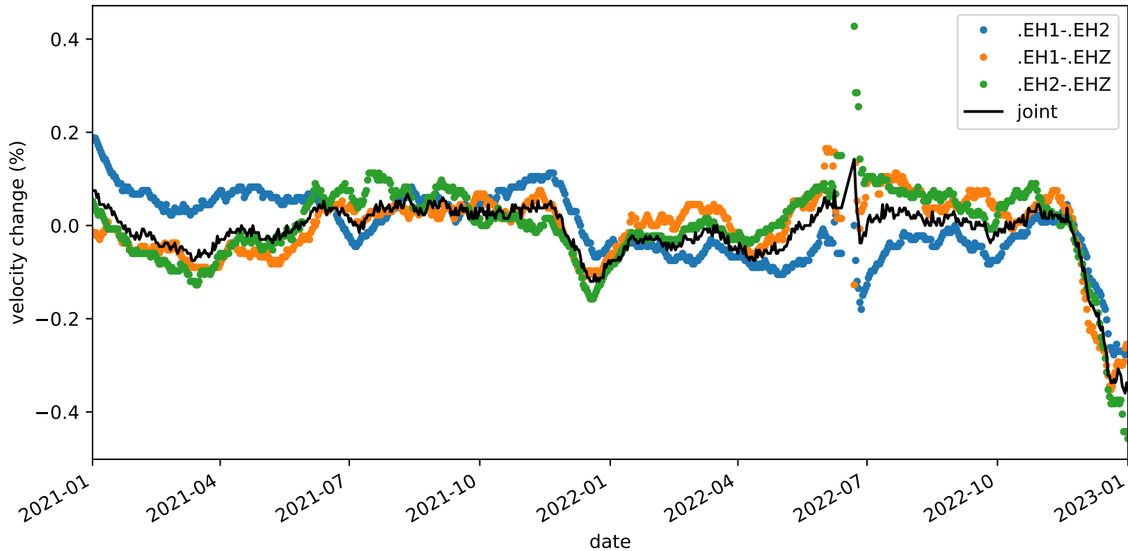
velocity_change_c1g_s2_t1b_tw_010.0s-015.0s_PB.B045-PB.B045
