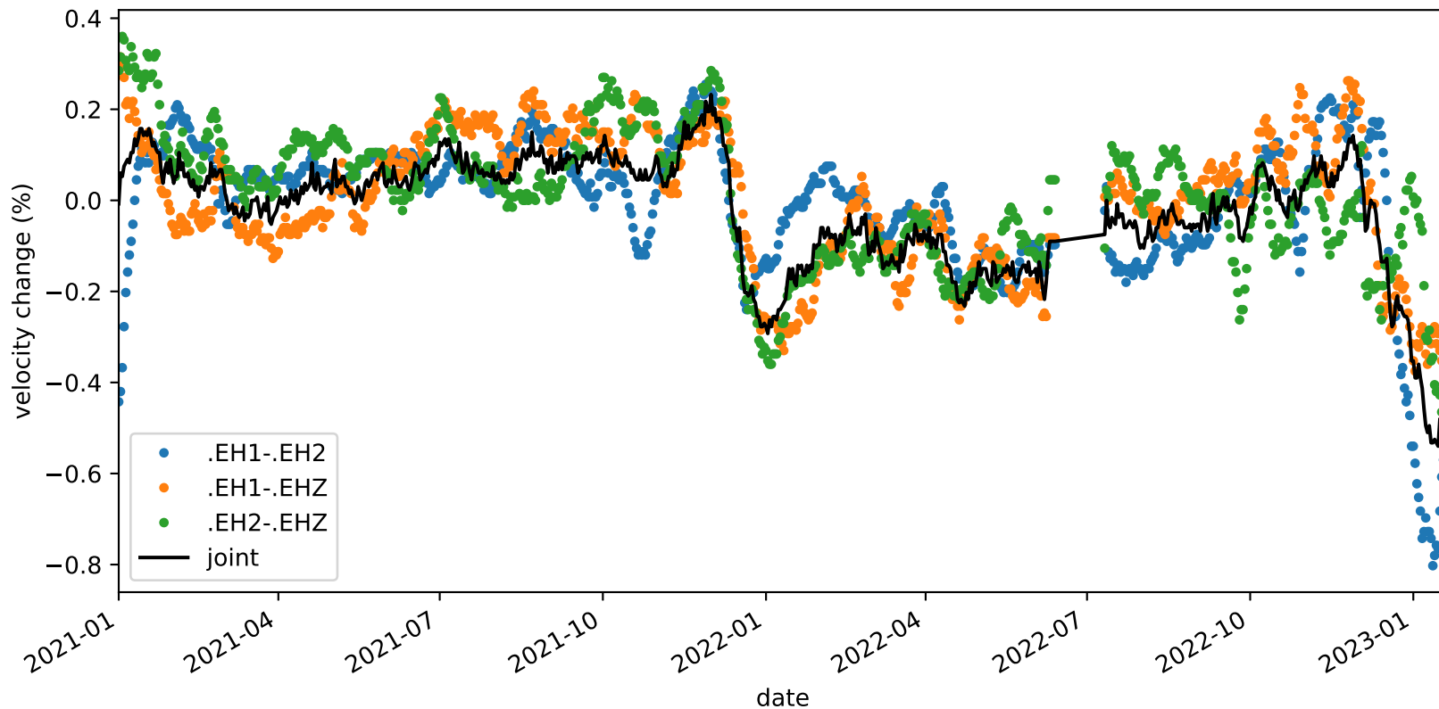
velocity_change_c1f_s3_t1a_tw_005.0s-010.0s_PB.B045-PB.B045
