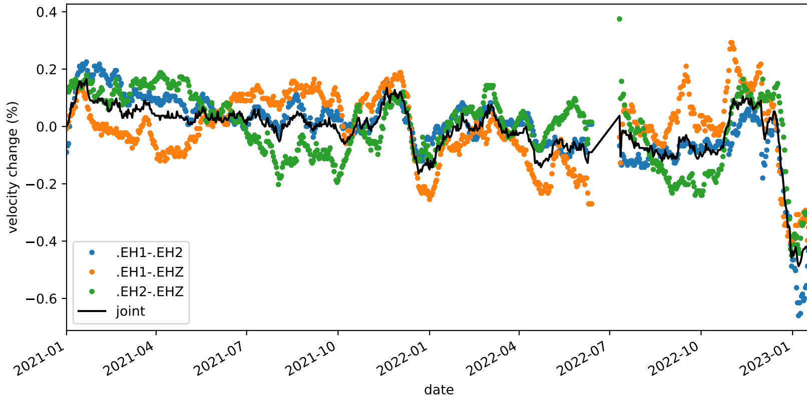
velocity_change_c1i_s3_t1a_tw_005.0s-010.0s_PB.B045-PB.B045
