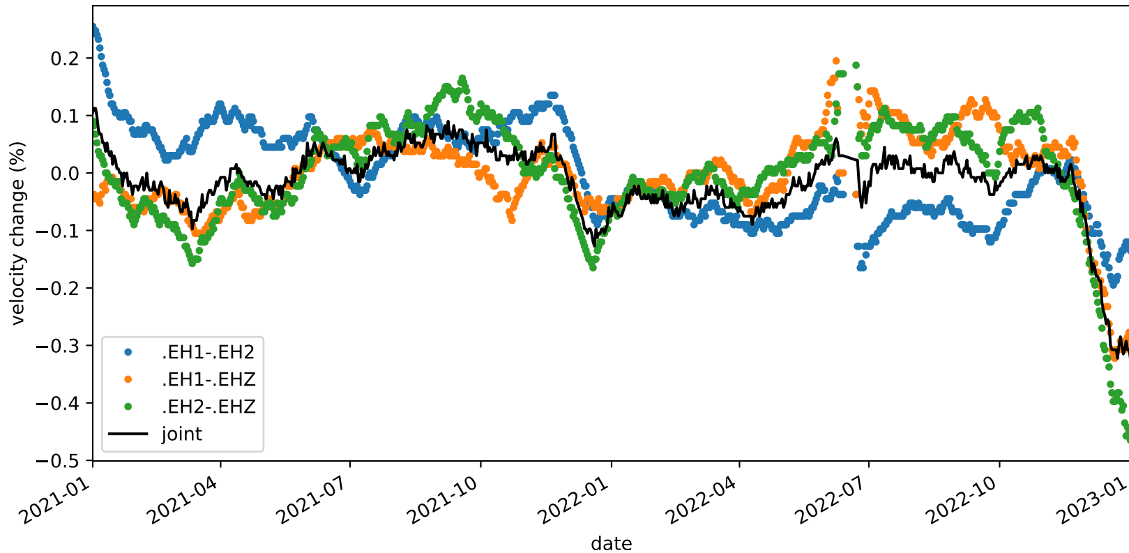
velocity_change_c1f_s2_t1b_tw_010.0s-015.0s_PB.B045-PB.B045
