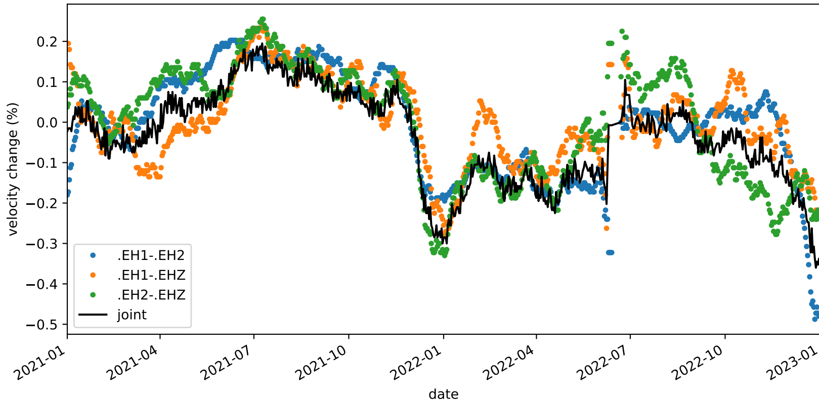
velocity_change_c1e_s2_t1a_tw_005.0s-010.0s_PB.B045-PB.B045
