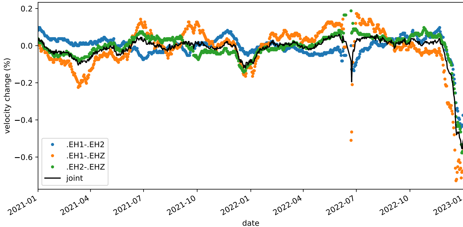
velocity_change_c1b_s2_t1b_tw_010.0s-015.0s_PB.B045-PB.B045
