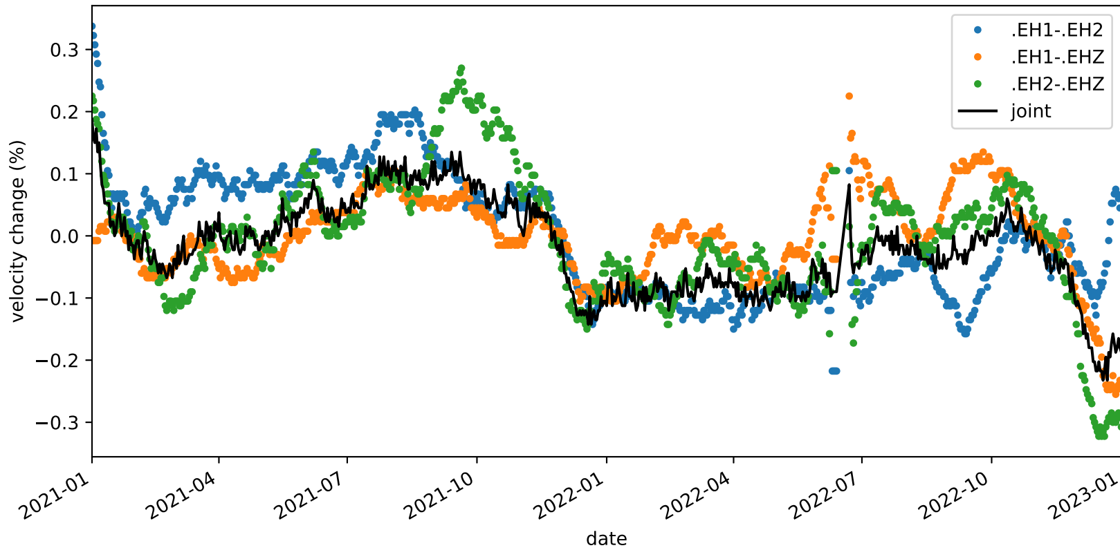
velocity_change_c1e_s2_t1b_tw_010.0s-015.0s_PB.B045-PB.B045
