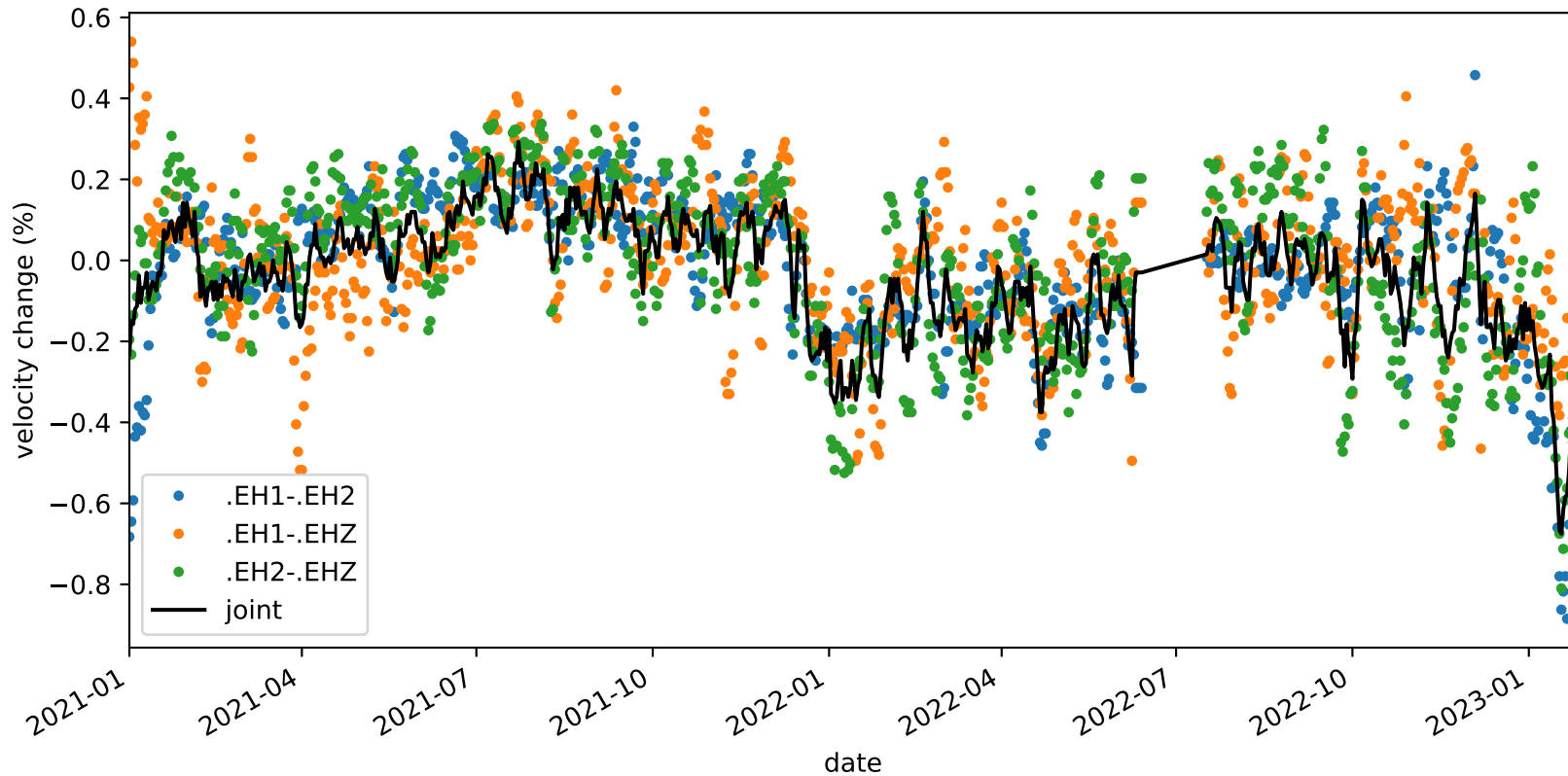
velocity_change_c1e_s4_t1a_tw_005.0s-010.0s_PB.B045-PB.B045
