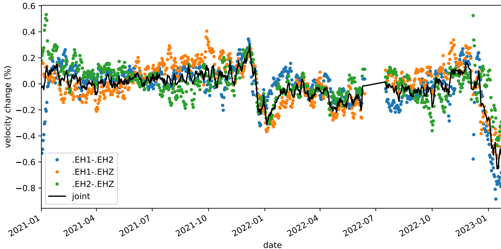
velocity_change_c1g_s4_t1a_tw_005.0s-010.0s_PB.B045-PB.B045
