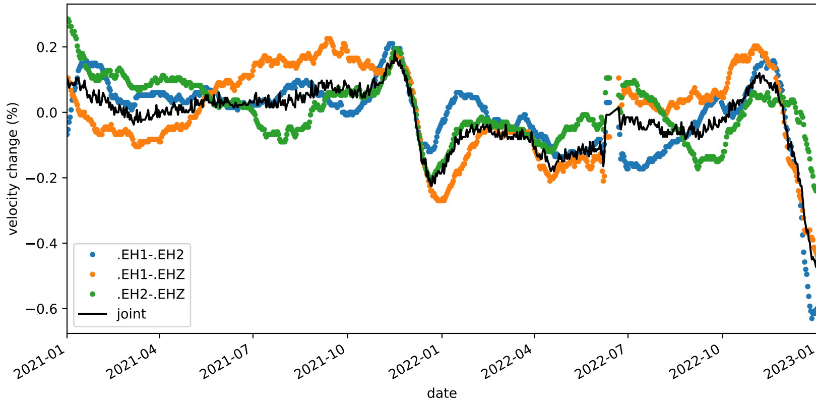
velocity_change_c1g_s2_t1a_tw_005.0s-010.0s_PB.B045-PB.B045
