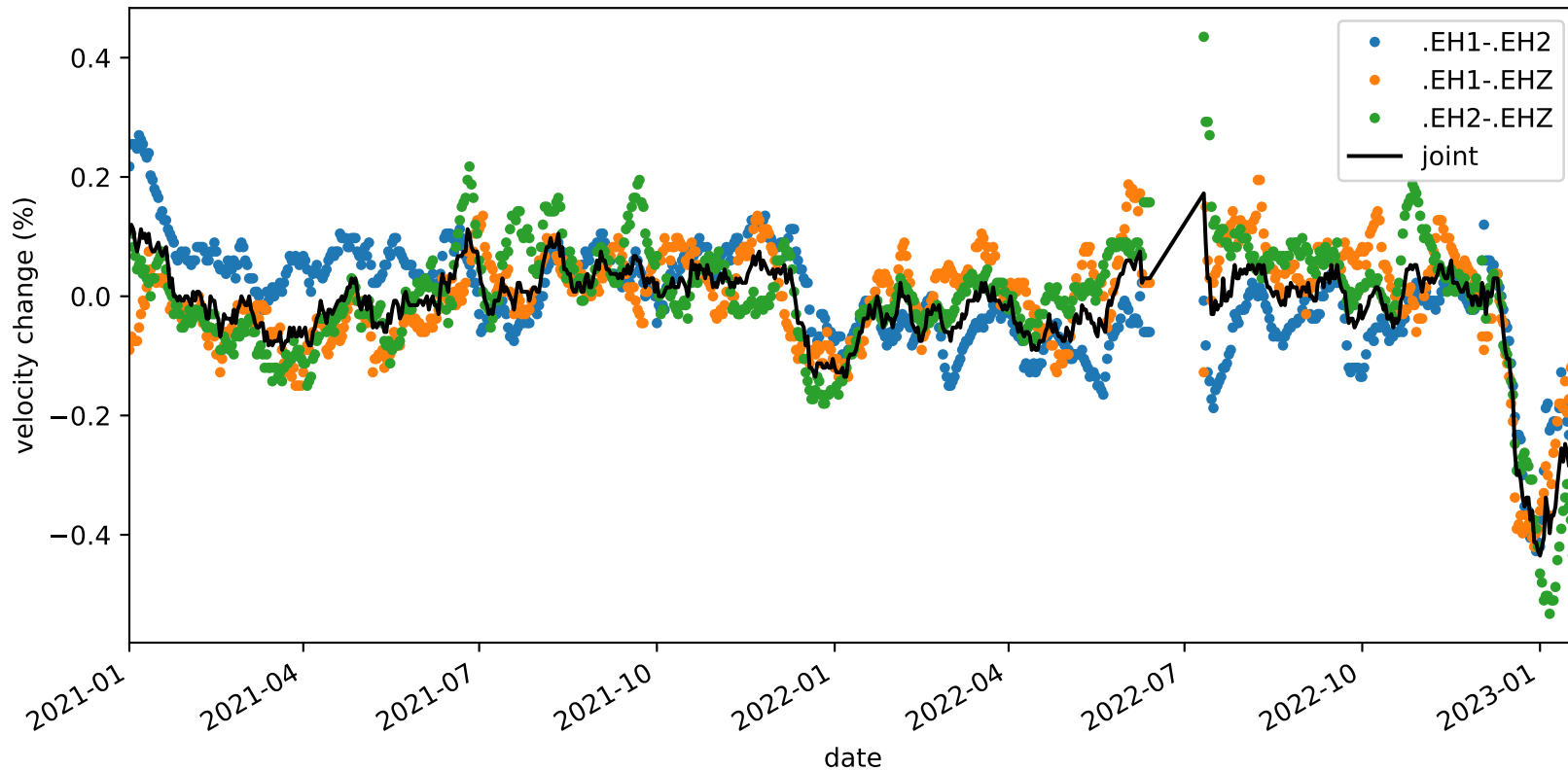
velocity_change_c1g_s3_t1b_tw_010.0s-015.0s_PB.B045-PB.B045
