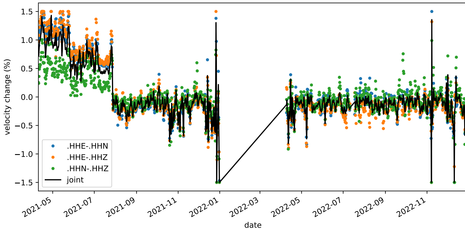
velocity_change_c1b_s1_t1a_tw_005.0s-010.0s_NC.KMPB-NC.KMPB
