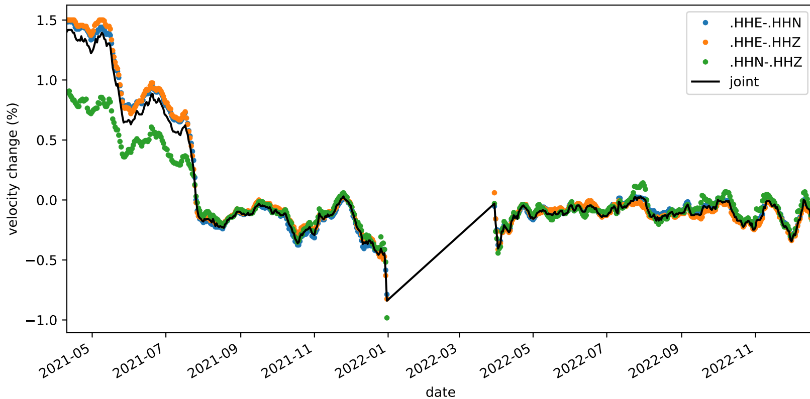
velocity_change_c1g_s3_t1c_tw_005.0s-015.0s_NC.KMPB-NC.KMPB
