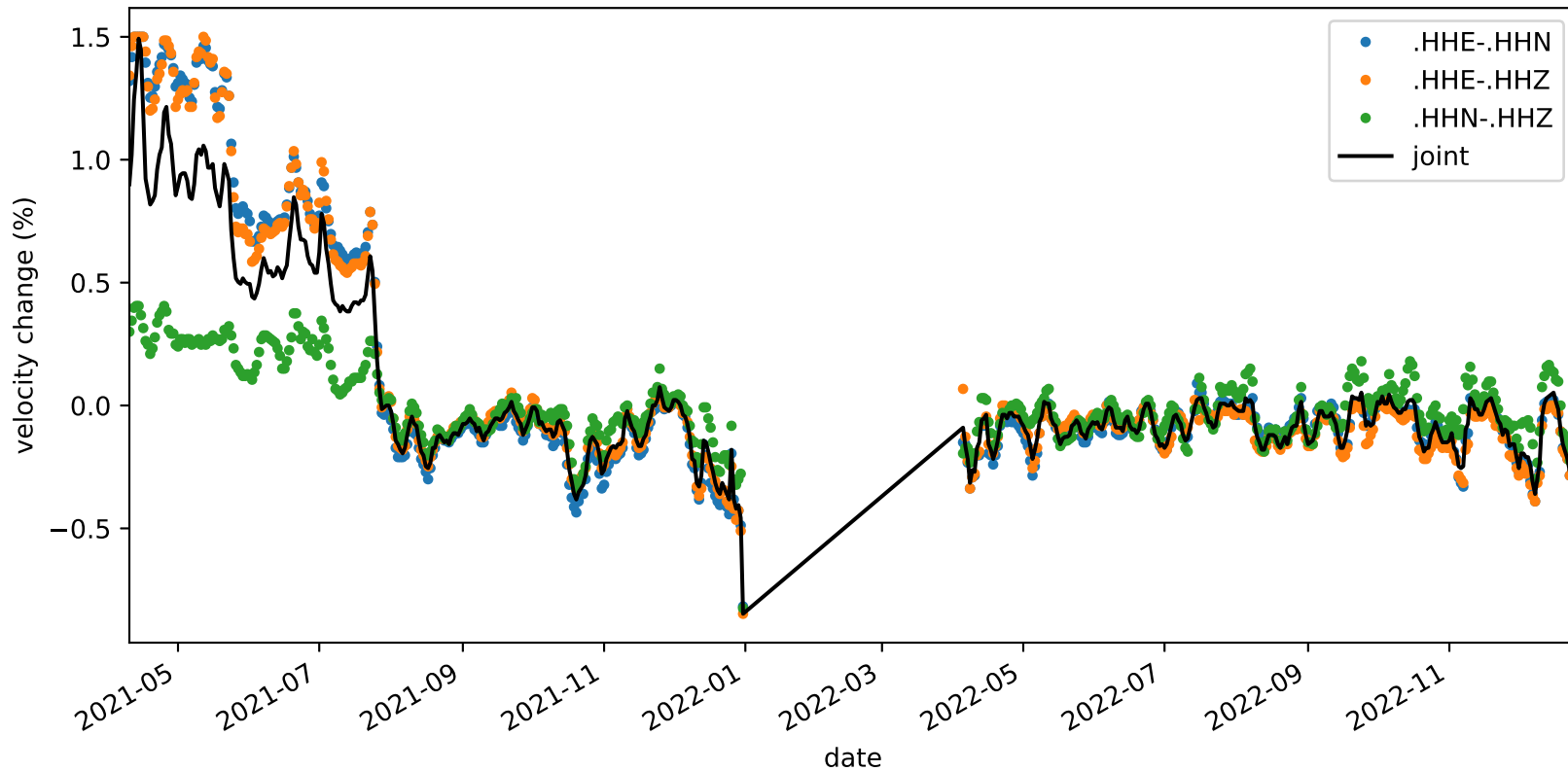
velocity_change_c1b_s4_t1c_tw_005.0s-015.0s_NC.KMPB-NC.KMPB
