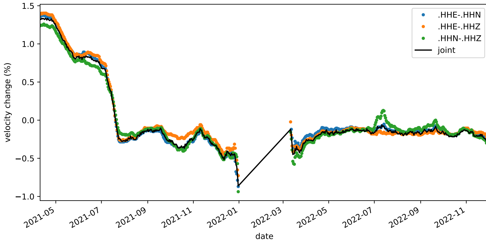
velocity_change_c1f_s2_t1a_tw_005.0s-010.0s_NC.KMPB-NC.KMPB
