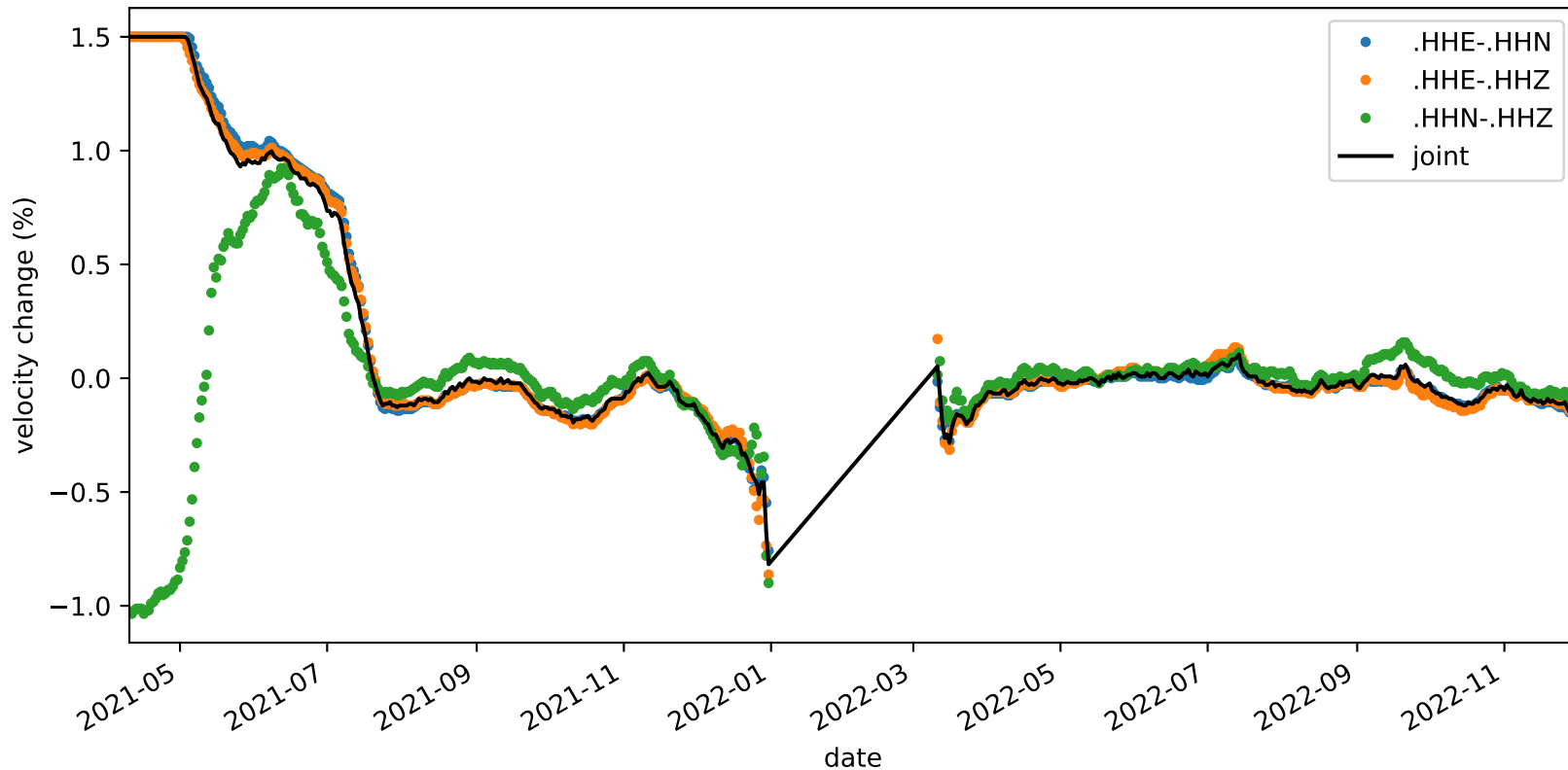
velocity_change_c1f_s2_t1b_tw_010.0s-015.0s_NC.KMPB-NC.KMPB
