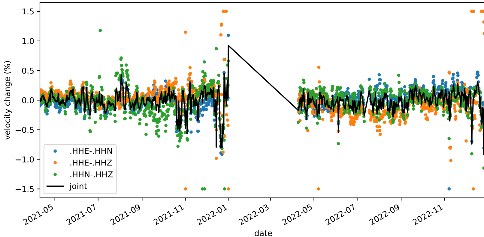
velocity_change_c1_s1_t1a_tw_005.0s-010.0s_NC.KMPB-NC.KMPB
