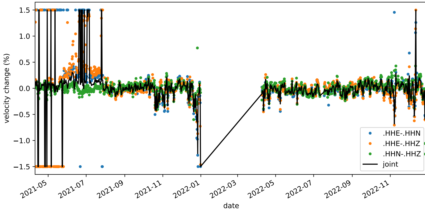
velocity_change_c1h_s1_t1b_tw_010.0s-015.0s_NC.KMPB-NC.KMPB
