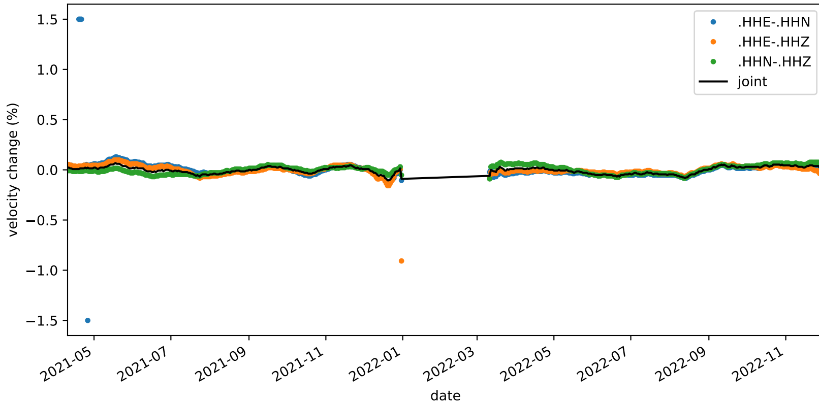
velocity_change_c1i_s2_t1b_tw_010.0s-015.0s_NC.KMPB-NC.KMPB
