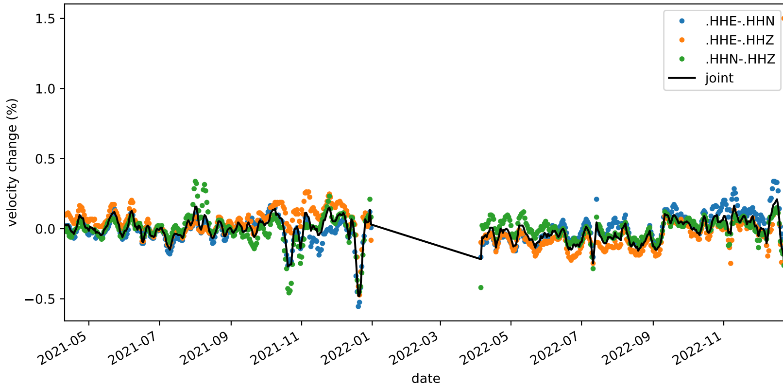
velocity_change_c1_s4_t1c_tw_005.0s-015.0s_NC.KMPB-NC.KMPB
