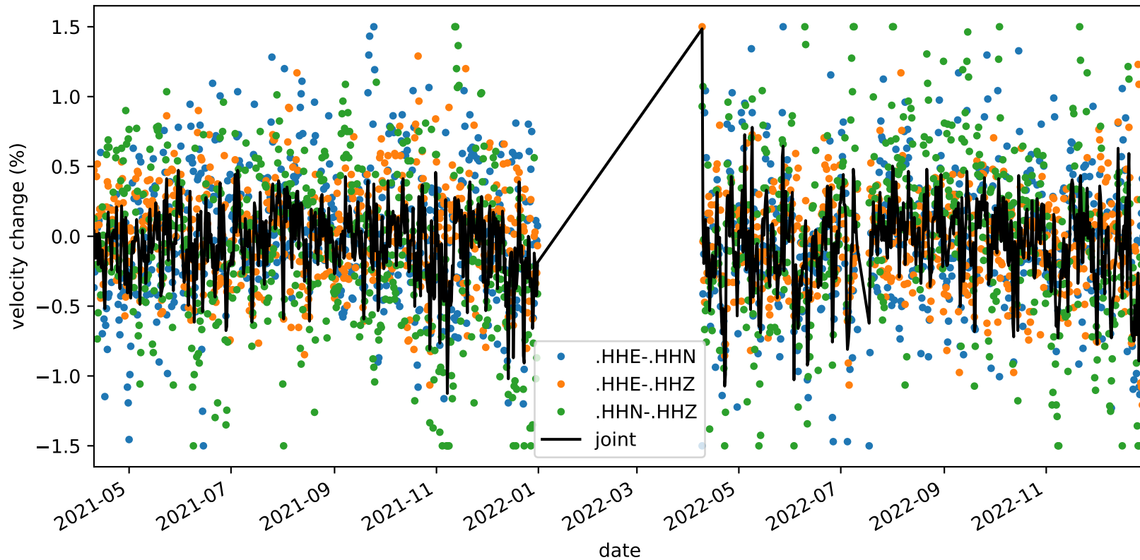
velocity_change_c1e_s1_t1a_tw_005.0s-010.0s_NC.KMPB-NC.KMPB
