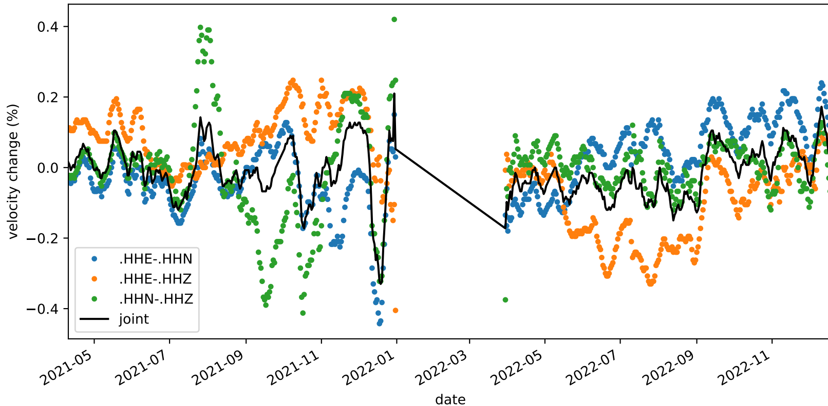
velocity_change_c1_s3_t1a_tw_005.0s-010.0s_NC.KMPB-NC.KMPB
