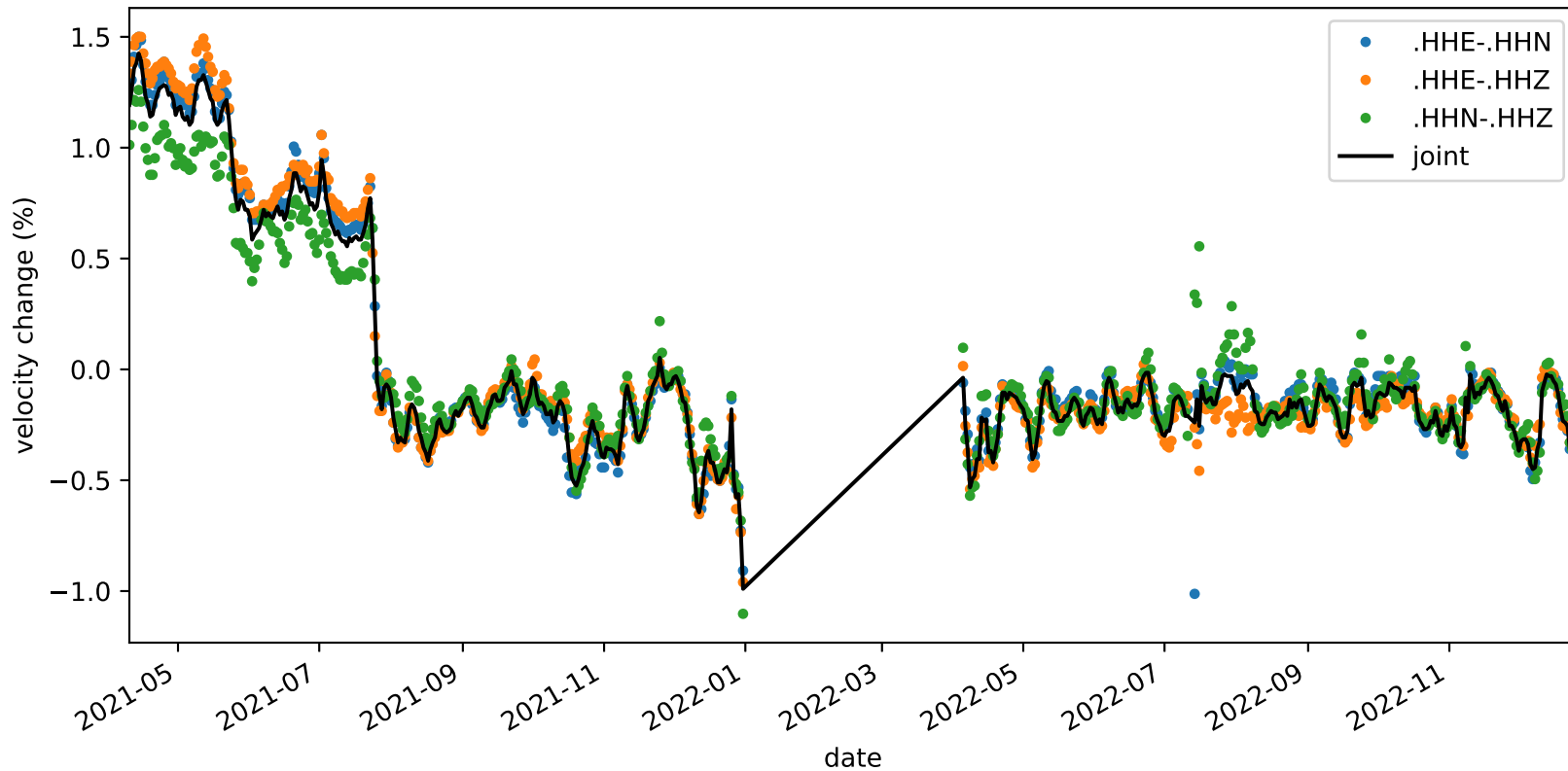
velocity_change_c1g_s4_t1a_tw_005.0s-010.0s_NC.KMPB-NC.KMPB
