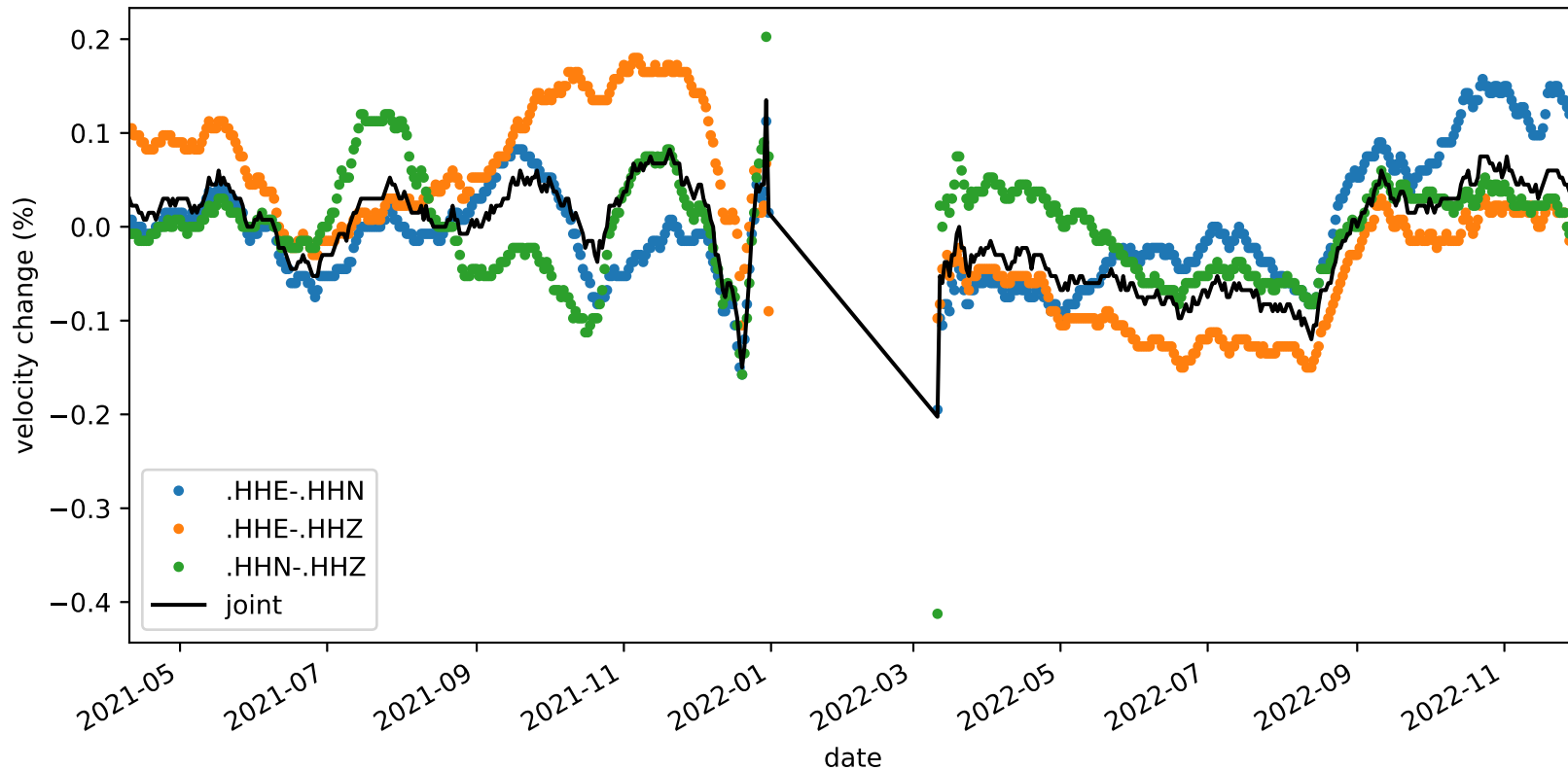
velocity_change_c1_s2_t1c_tw_005.0s-015.0s_NC.KMPB-NC.KMPB
