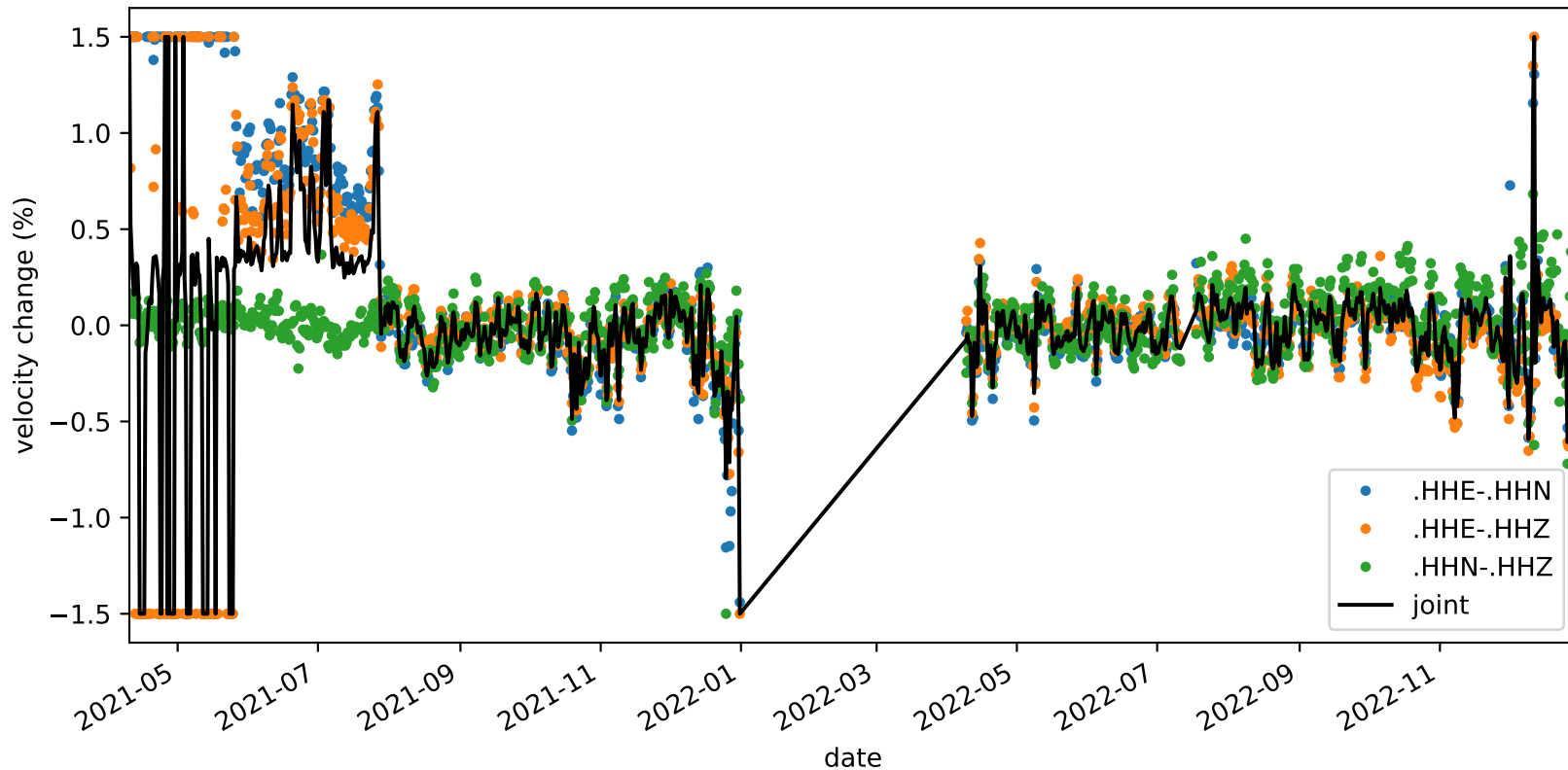
velocity_change_c1b_s1_t1b_tw_010.0s-015.0s_NC.KMPB-NC.KMPB
