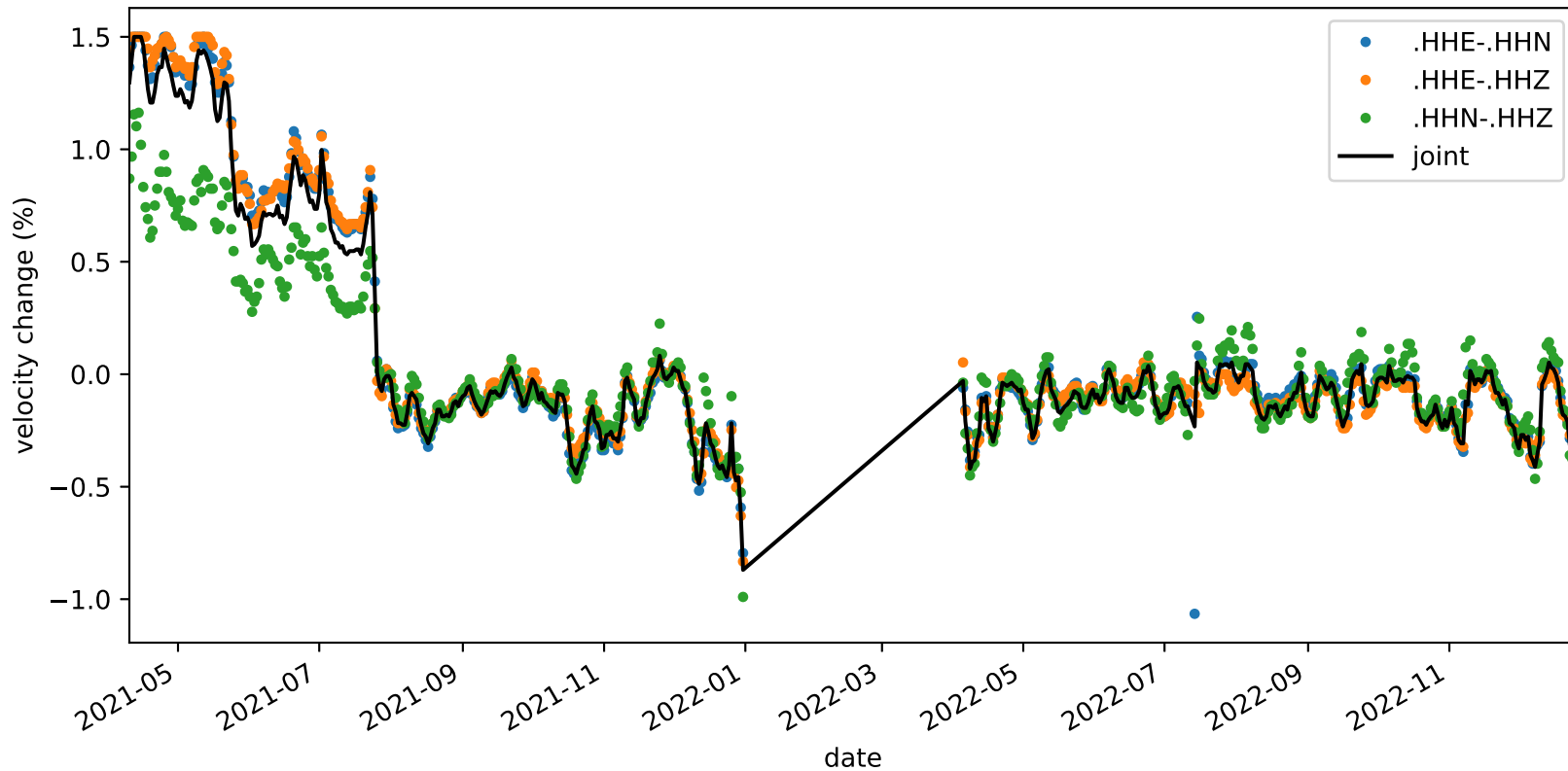
velocity_change_c1g_s4_t1c_tw_005.0s-015.0s_NC.KMPB-NC.KMPB
