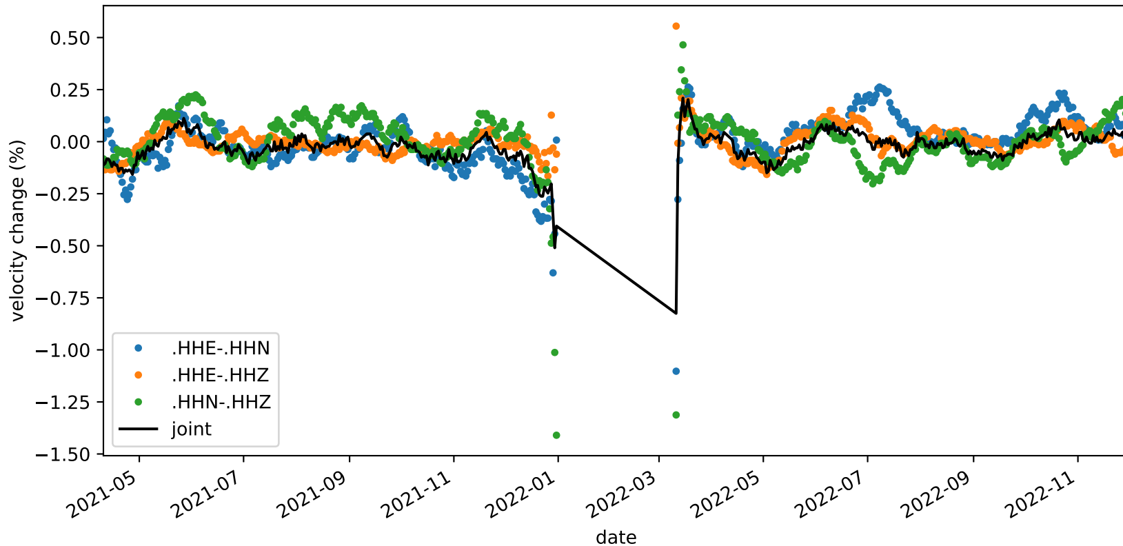
velocity_change_c1e_s2_t1b_tw_010.0s-015.0s_NC.KMPB-NC.KMPB
