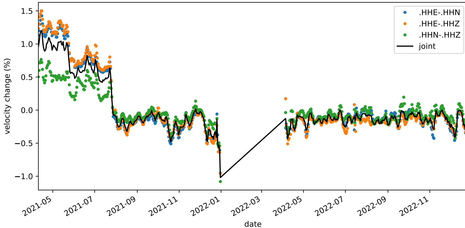
velocity_change_c1b_s4_t1a_tw_005.0s-010.0s_NC.KMPB-NC.KMPB
