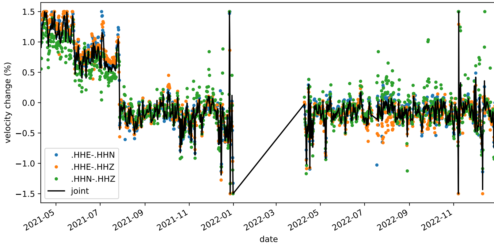
velocity_change_c1g_s1_t1a_tw_005.0s-010.0s_NC.KMPB-NC.KMPB
