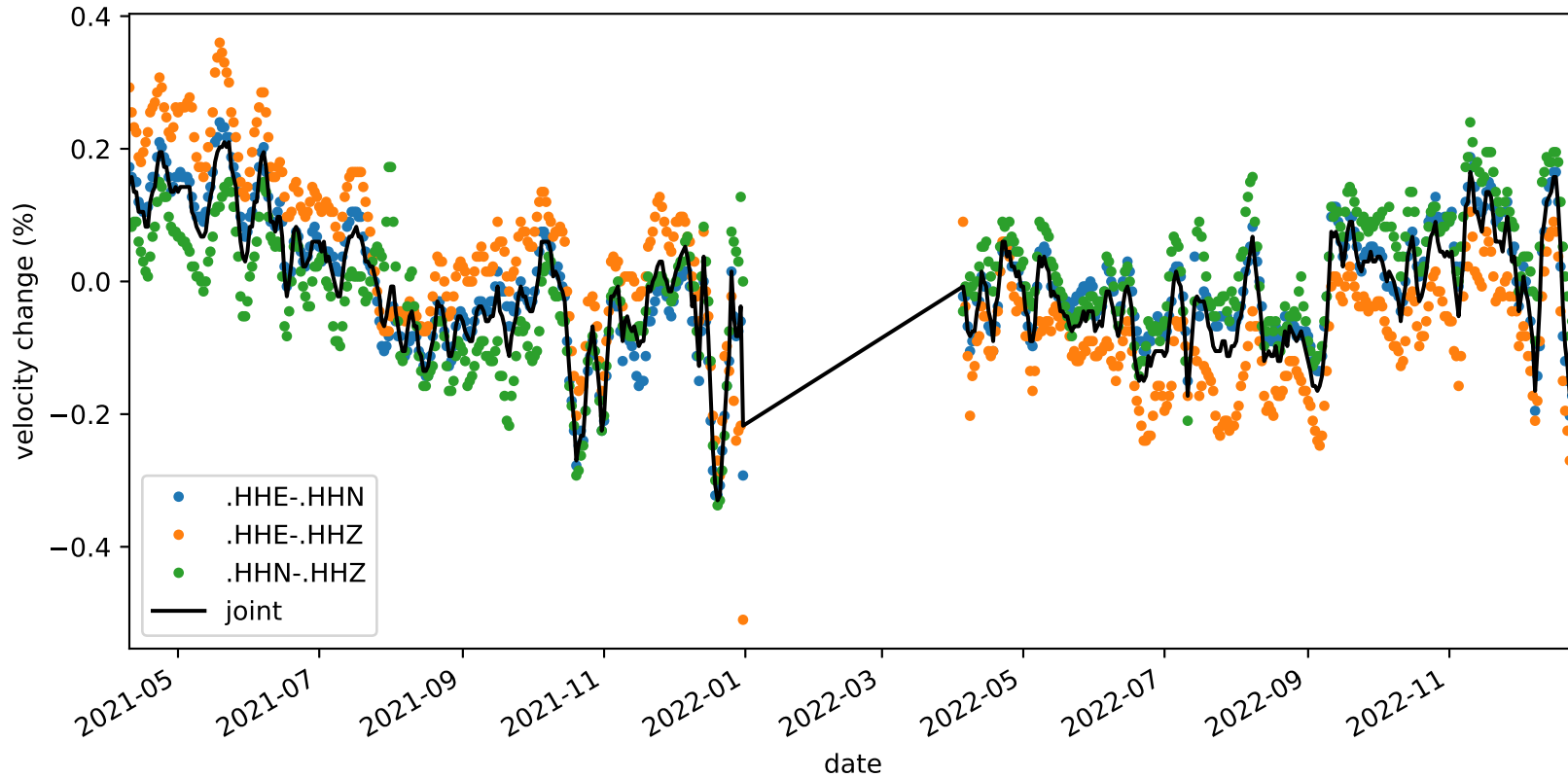
velocity_change_c1i_s4_t1a_tw_005.0s-010.0s_NC.KMPB-NC.KMPB
