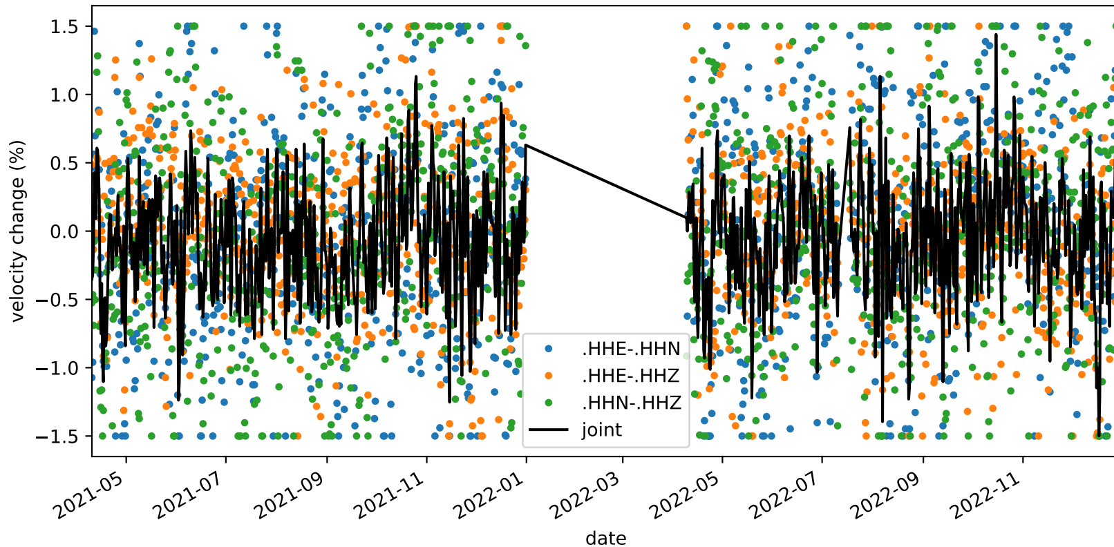
velocity_change_c1d_s1_t1c_tw_005.0s-015.0s_NC.KMPB-NC.KMPB
