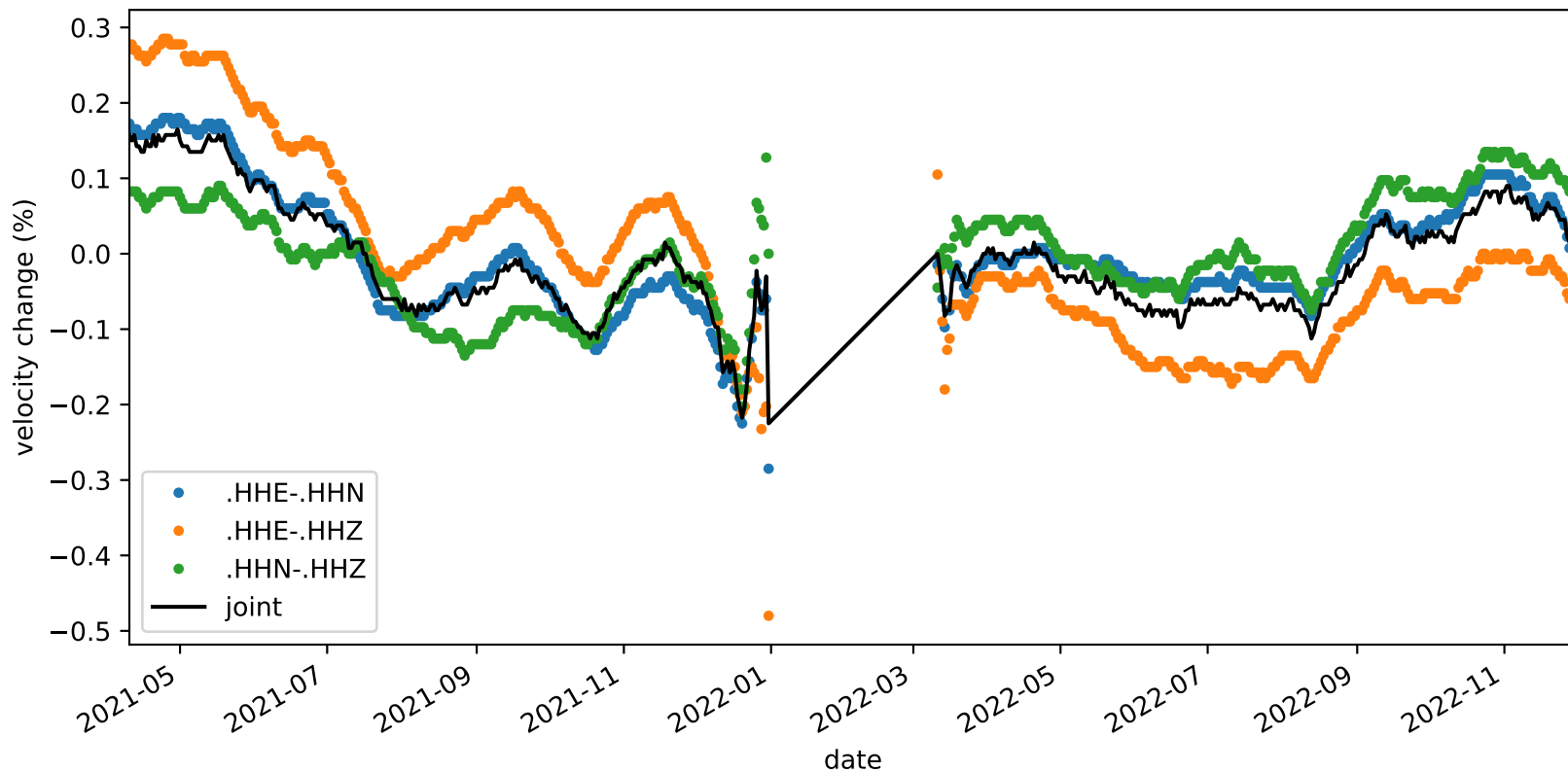
velocity_change_c1i_s2_t1a_tw_005.0s-010.0s_NC.KMPB-NC.KMPB
