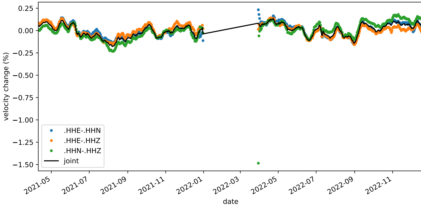
velocity_change_c1c_s3_t1c_tw_005.0s-015.0s_NC.KMPB-NC.KMPB
