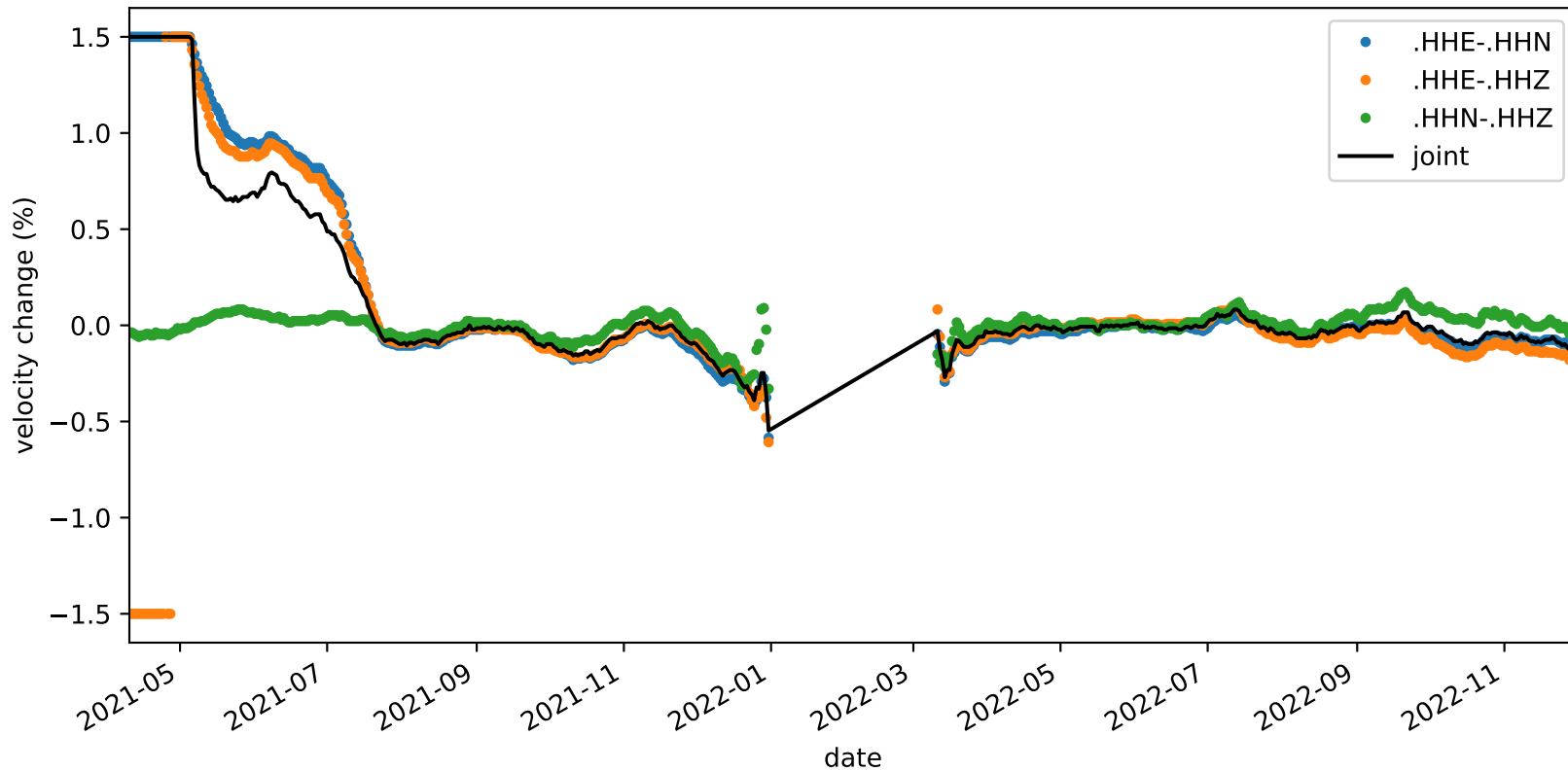
velocity_change_c1g_s2_t1b_tw_010.0s-015.0s_NC.KMPB-NC.KMPB
