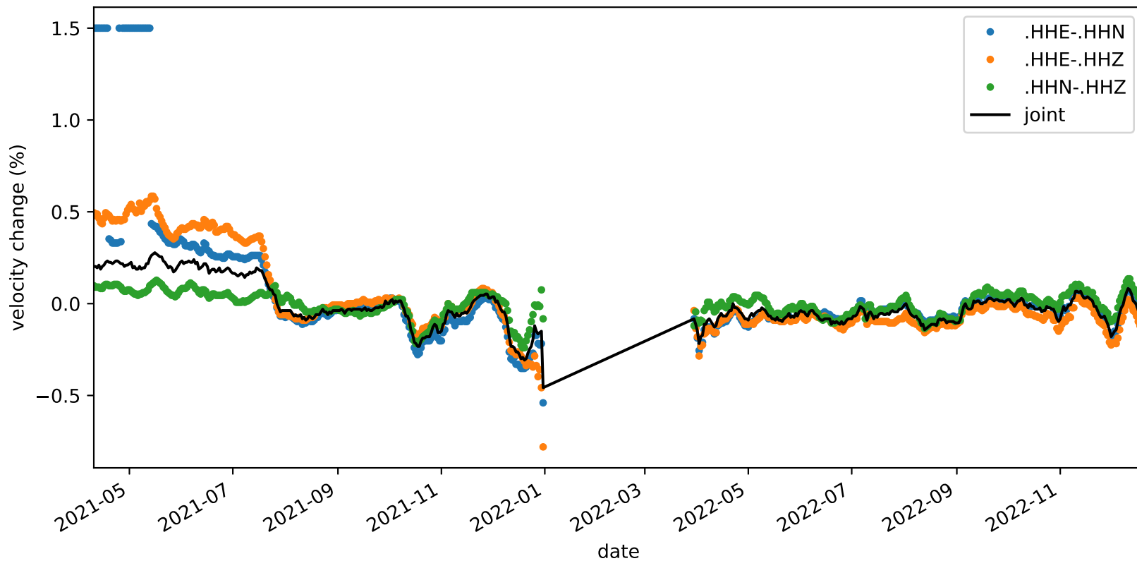
velocity_change_c1h_s3_t1c_tw_005.0s-015.0s_NC.KMPB-NC.KMPB
