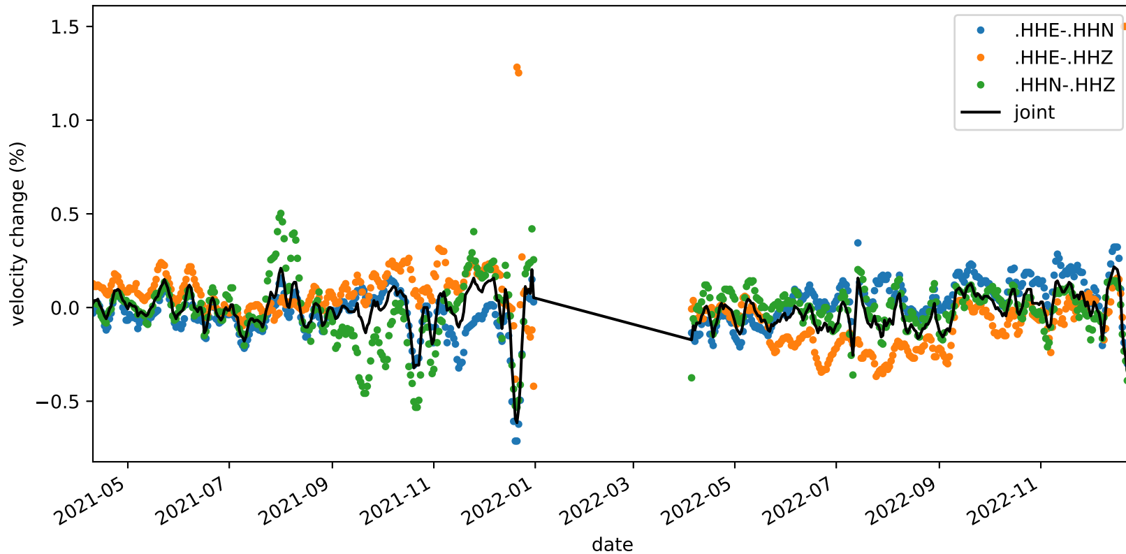
velocity_change_c1_s4_t1a_tw_005.0s-010.0s_NC.KMPB-NC.KMPB
