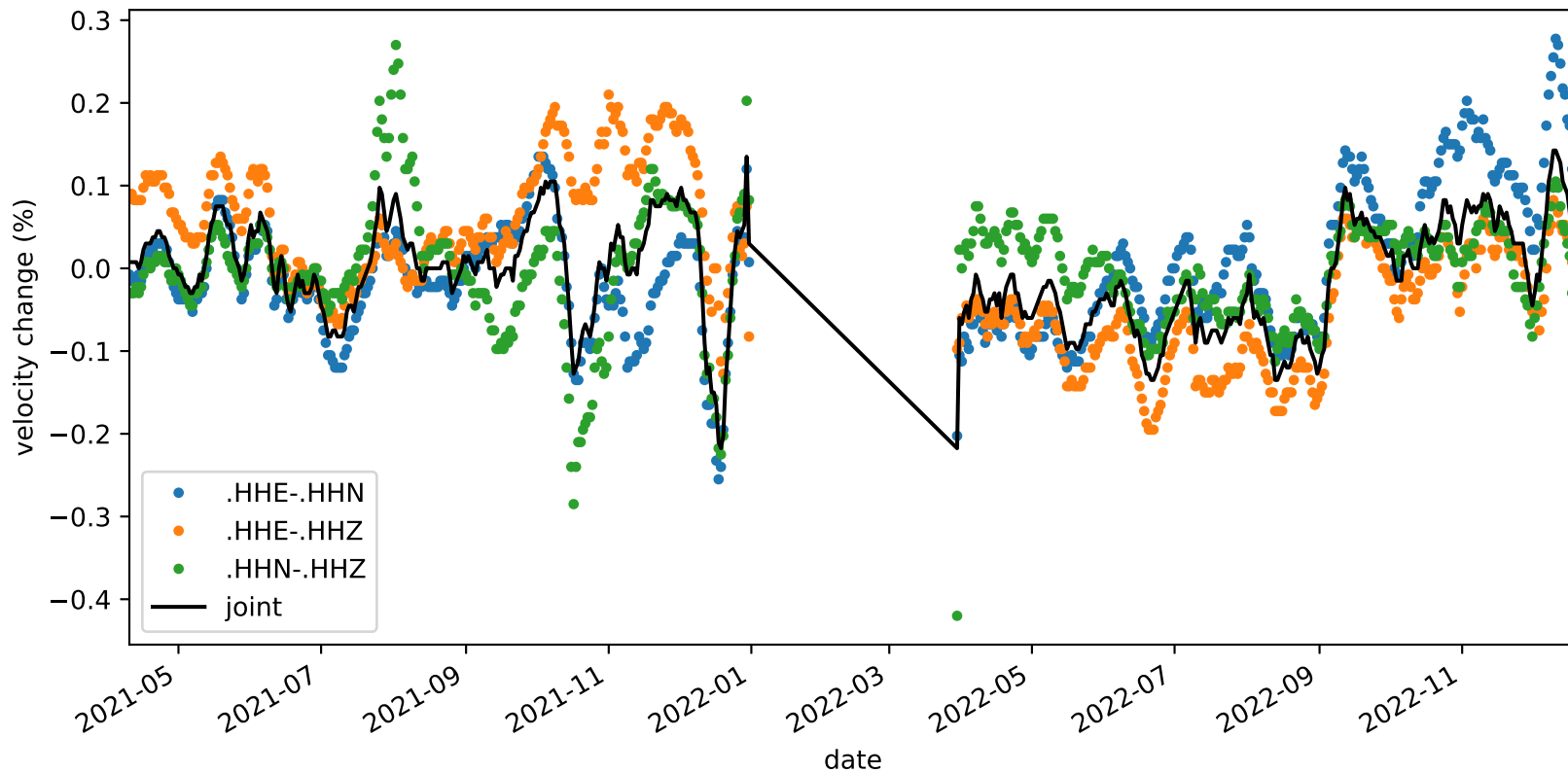
velocity_change_c1_s3_t1c_tw_005.0s-015.0s_NC.KMPB-NC.KMPB
