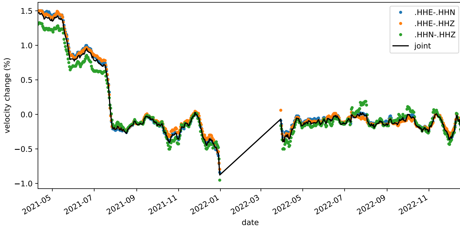
velocity_change_c1f_s3_t1c_tw_005.0s-015.0s_NC.KMPB-NC.KMPB
