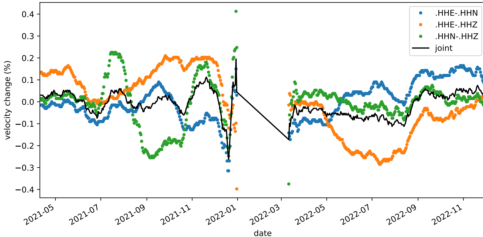
velocity_change_c1_s2_t1a_tw_005.0s-010.0s_NC.KMPB-NC.KMPB
