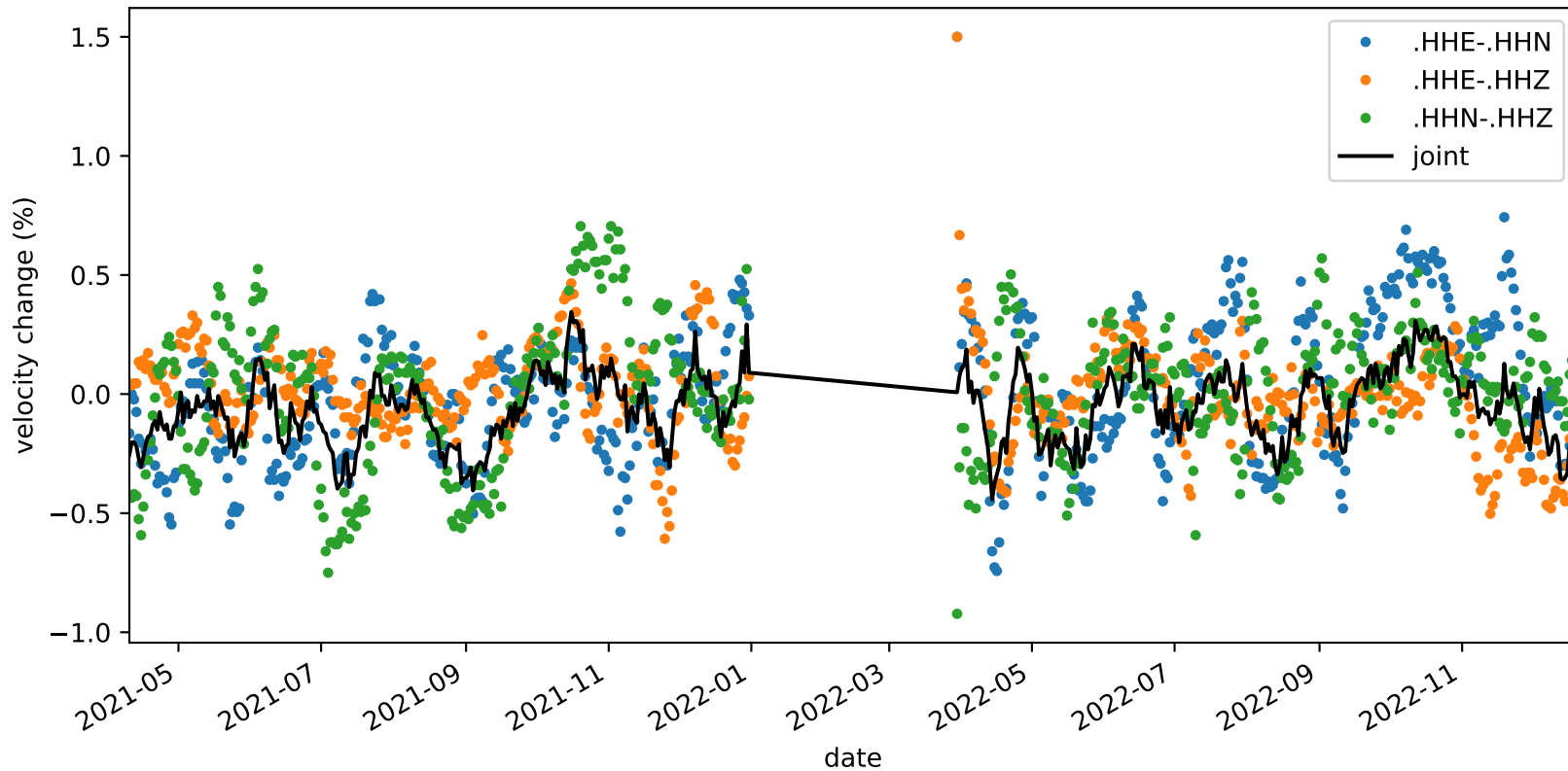
velocity_change_c1d_s3_t1c_tw_005.0s-015.0s_NC.KMPB-NC.KMPB
