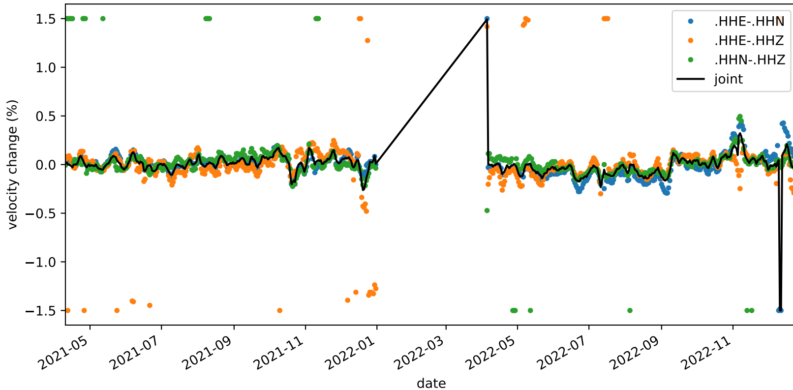
velocity_change_c1_s4_t1b_tw_010.0s-015.0s_NC.KMPB-NC.KMPB
