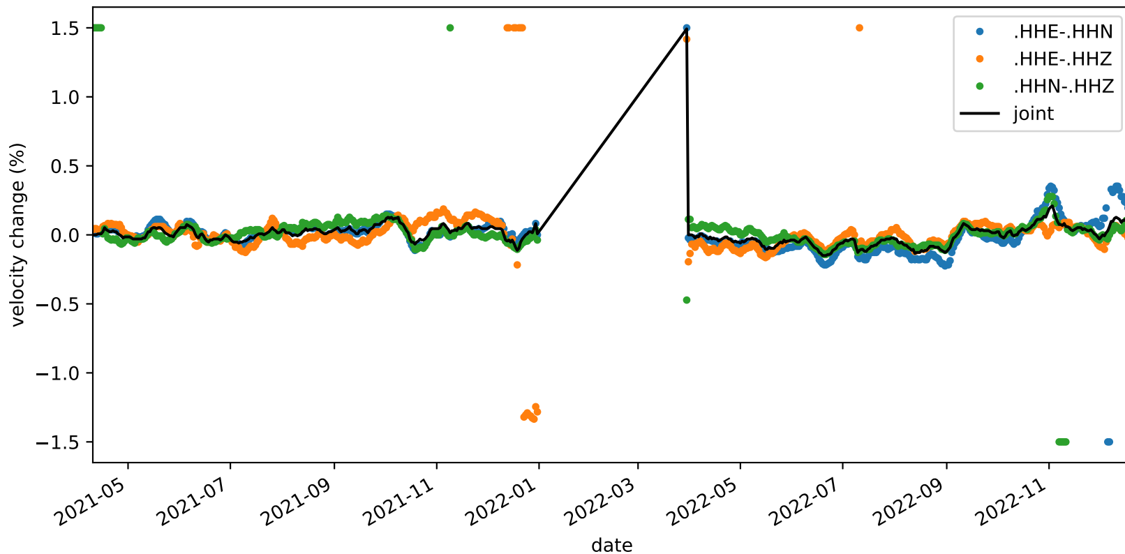
velocity_change_c1_s3_t1b_tw_010.0s-015.0s_NC.KMPB-NC.KMPB
