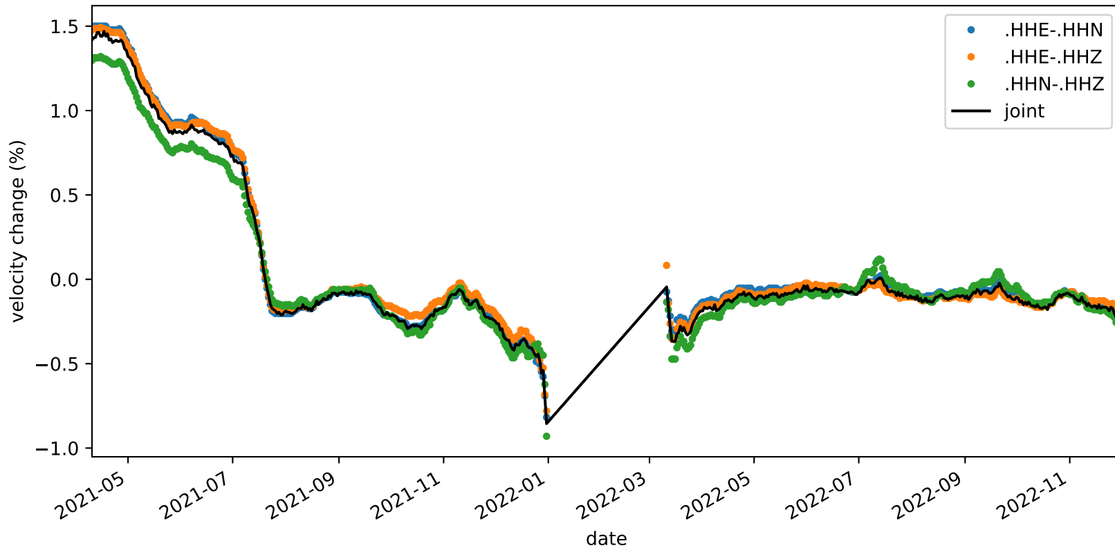
velocity_change_c1f_s2_t1c_tw_005.0s-015.0s_NC.KMPB-NC.KMPB
