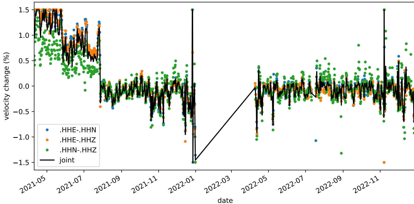
velocity_change_c1g_s1_t1c_tw_005.0s-015.0s_NC.KMPB-NC.KMPB
