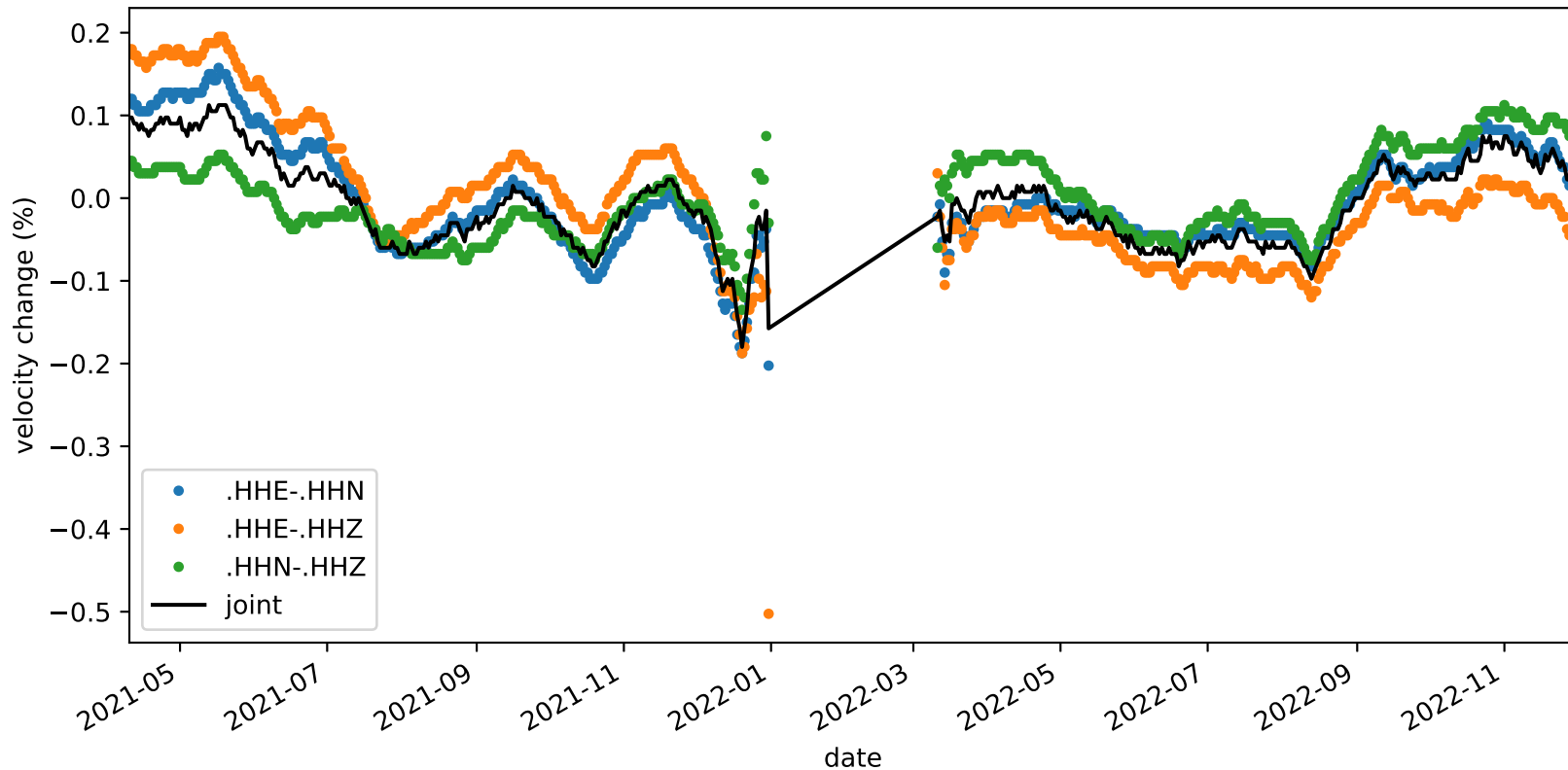
velocity_change_c1i_s2_t1c_tw_005.0s-015.0s_NC.KMPB-NC.KMPB
