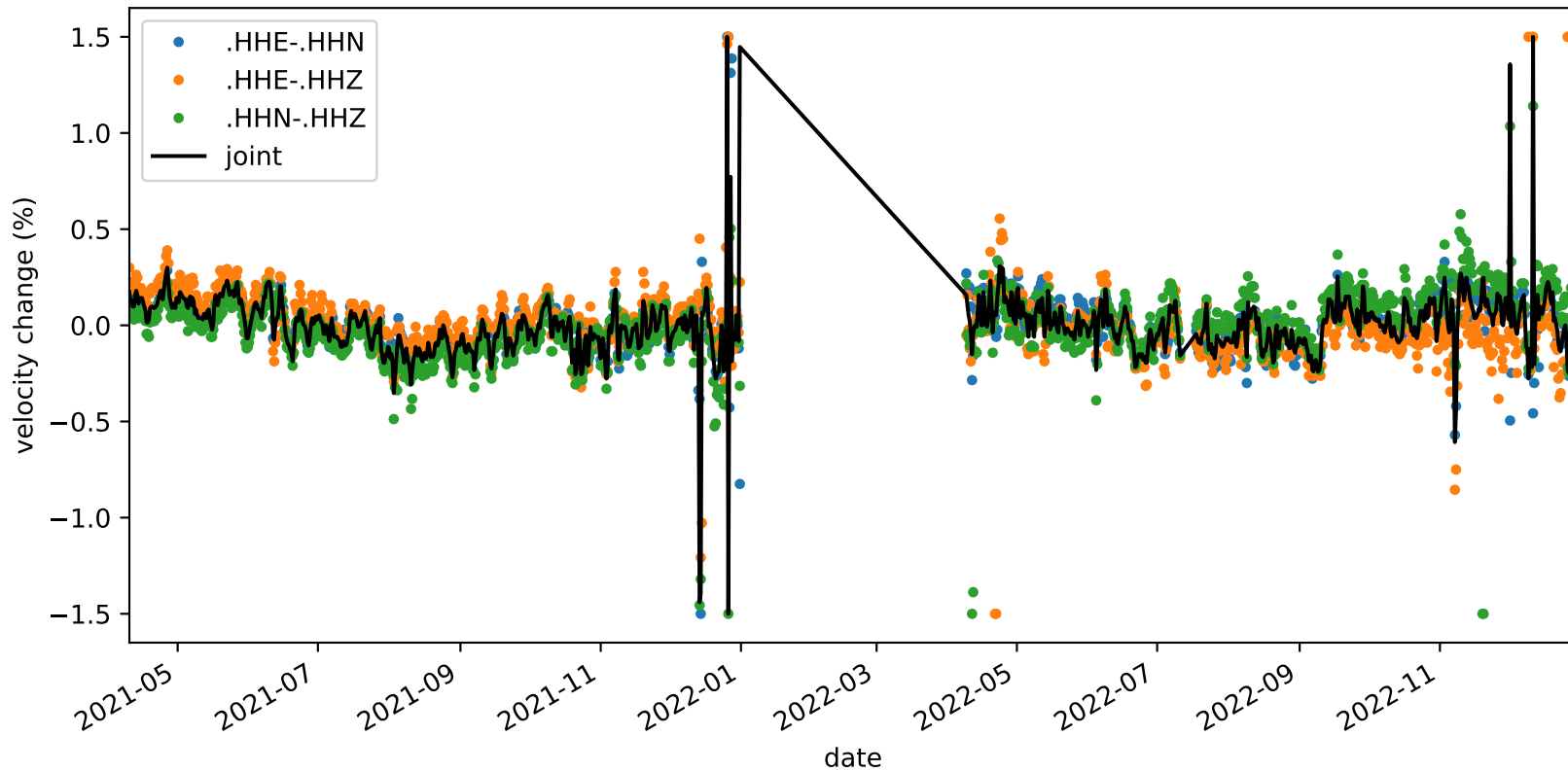
velocity_change_c1c_s1_t1a_tw_005.0s-010.0s_NC.KMPB-NC.KMPB
