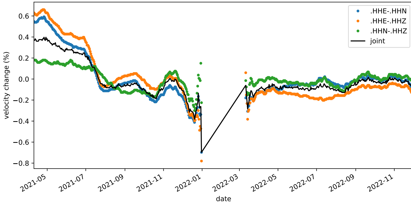
velocity_change_c1h_s2_t1a_tw_005.0s-010.0s_NC.KMPB-NC.KMPB
