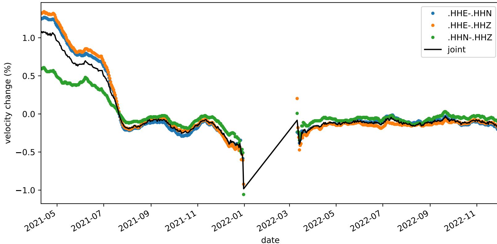
velocity_change_c1b_s2_t1a_tw_005.0s-010.0s_NC.KMPB-NC.KMPB
