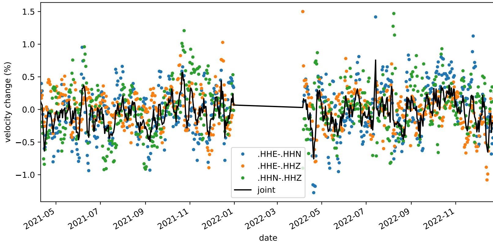
velocity_change_c1d_s4_t1c_tw_005.0s-015.0s_NC.KMPB-NC.KMPB
