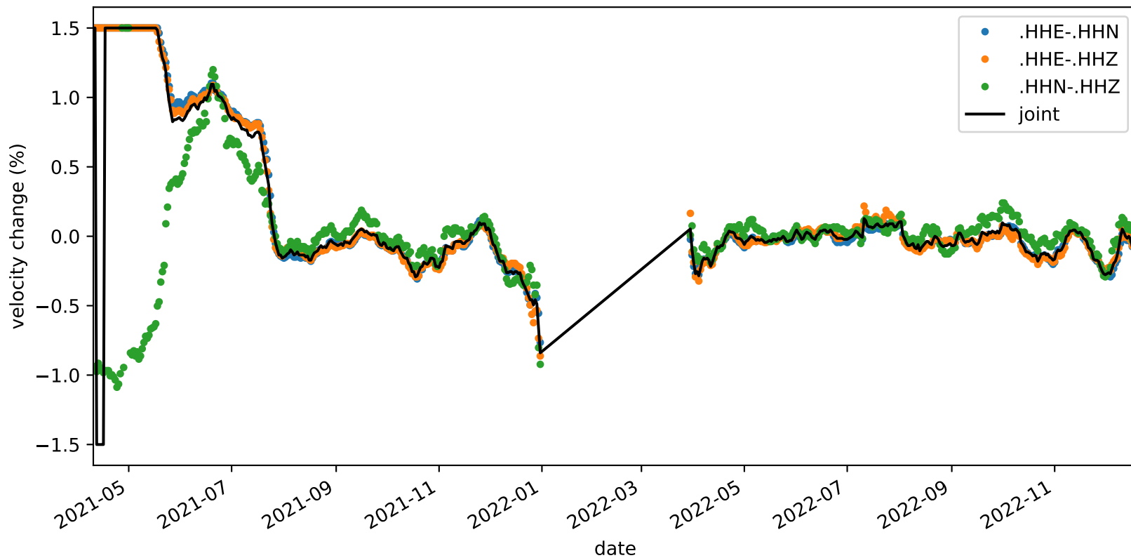
velocity_change_c1f_s3_t1b_tw_010.0s-015.0s_NC.KMPB-NC.KMPB
