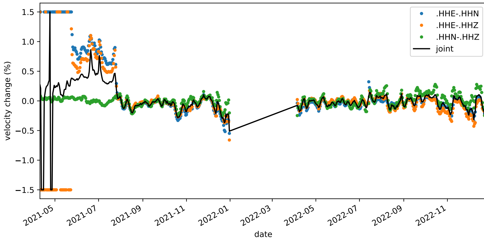
velocity_change_c1b_s4_t1b_tw_010.0s-015.0s_NC.KMPB-NC.KMPB
