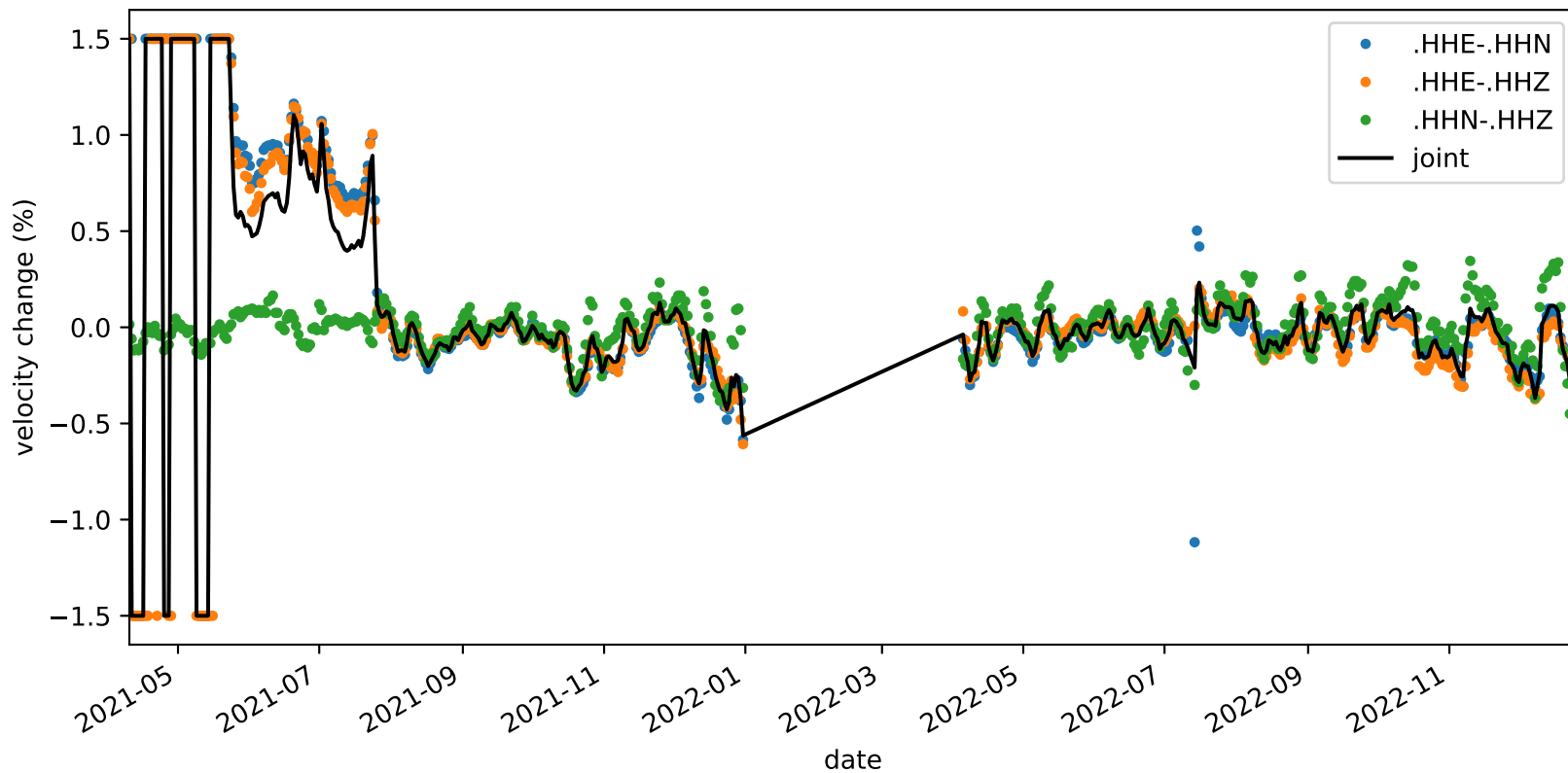
velocity_change_c1g_s4_t1b_tw_010.0s-015.0s_NC.KMPB-NC.KMPB
