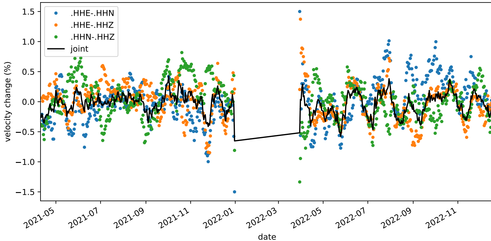
velocity_change_c1d_s3_t1b_tw_010.0s-015.0s_NC.KMPB-NC.KMPB
