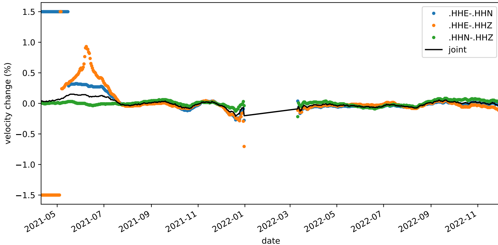
velocity_change_c1h_s2_t1b_tw_010.0s-015.0s_NC.KMPB-NC.KMPB
