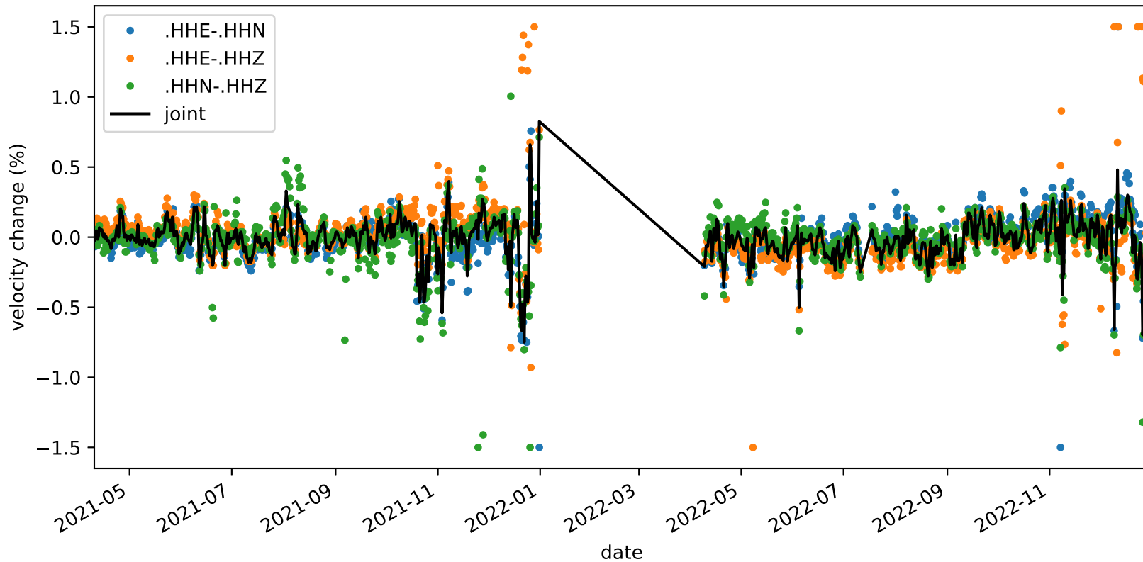
velocity_change_c1_s1_t1c_tw_005.0s-015.0s_NC.KMPB-NC.KMPB
