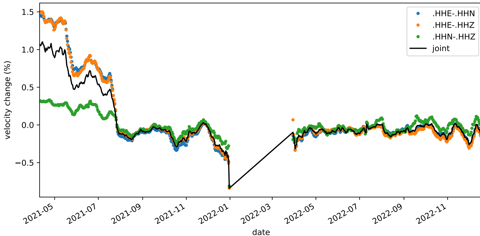
velocity_change_c1b_s3_t1c_tw_005.0s-015.0s_NC.KMPB-NC.KMPB
