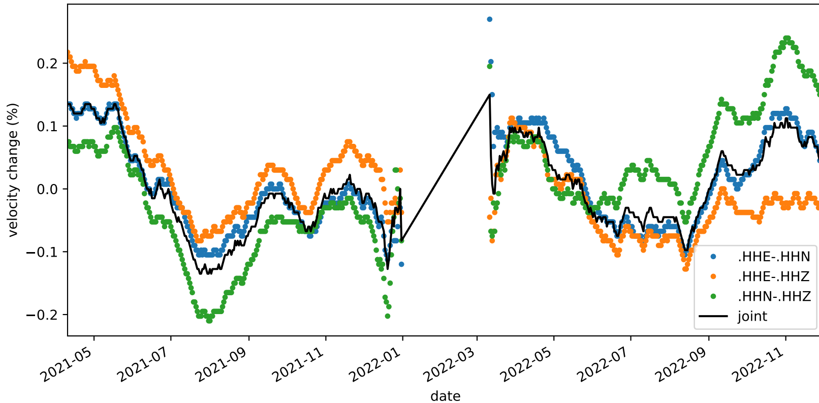
velocity_change_c1c_s2_t1a_tw_005.0s-010.0s_NC.KMPB-NC.KMPB
