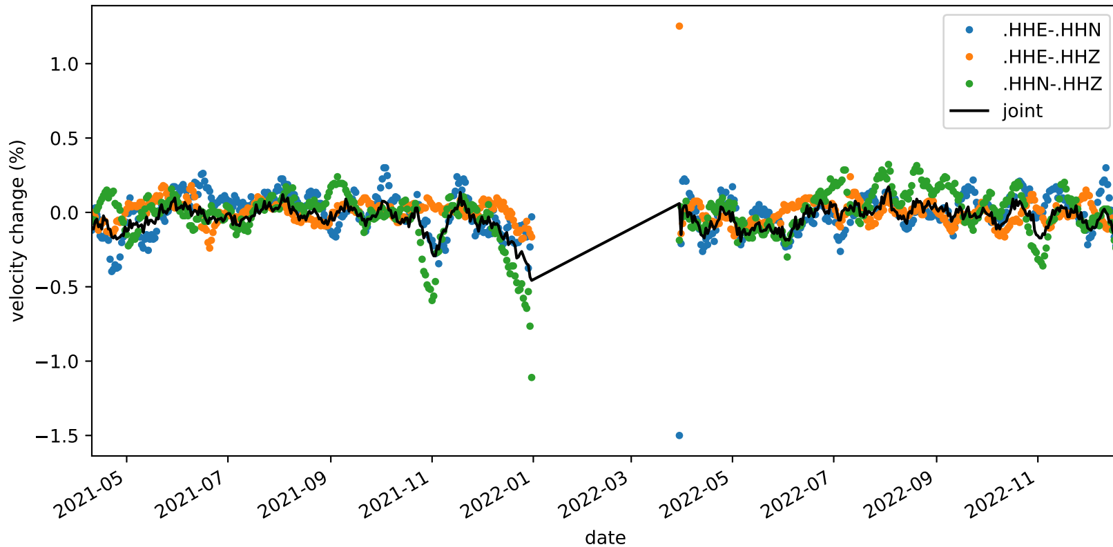
velocity_change_c1e_s3_t1c_tw_005.0s-015.0s_NC.KMPB-NC.KMPB
