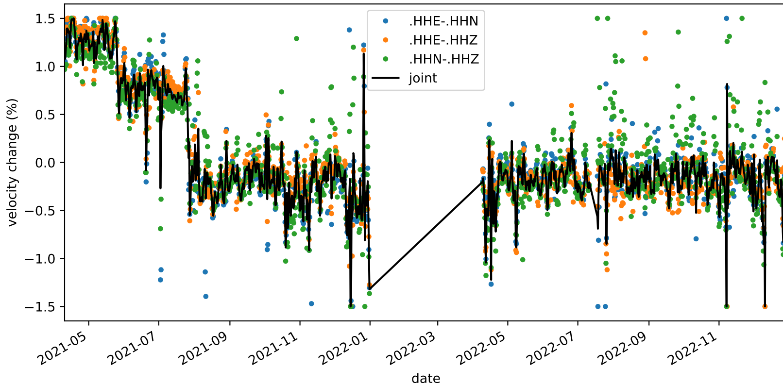
velocity_change_c1f_s1_t1a_tw_005.0s-010.0s_NC.KMPB-NC.KMPB
