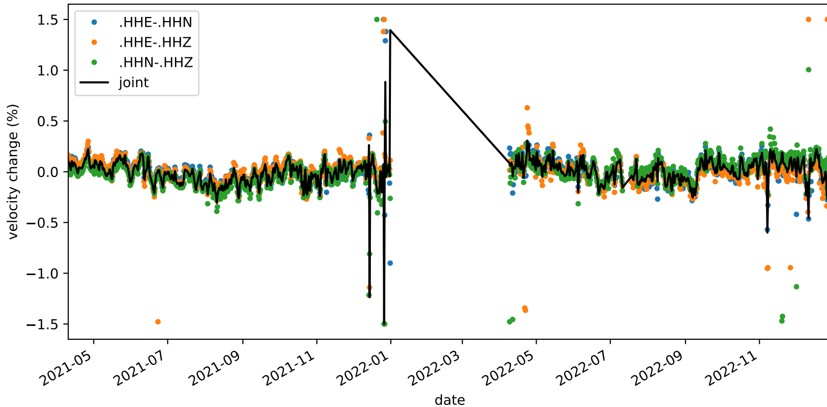
velocity_change_c1c_s1_t1c_tw_005.0s-015.0s_NC.KMPB-NC.KMPB
