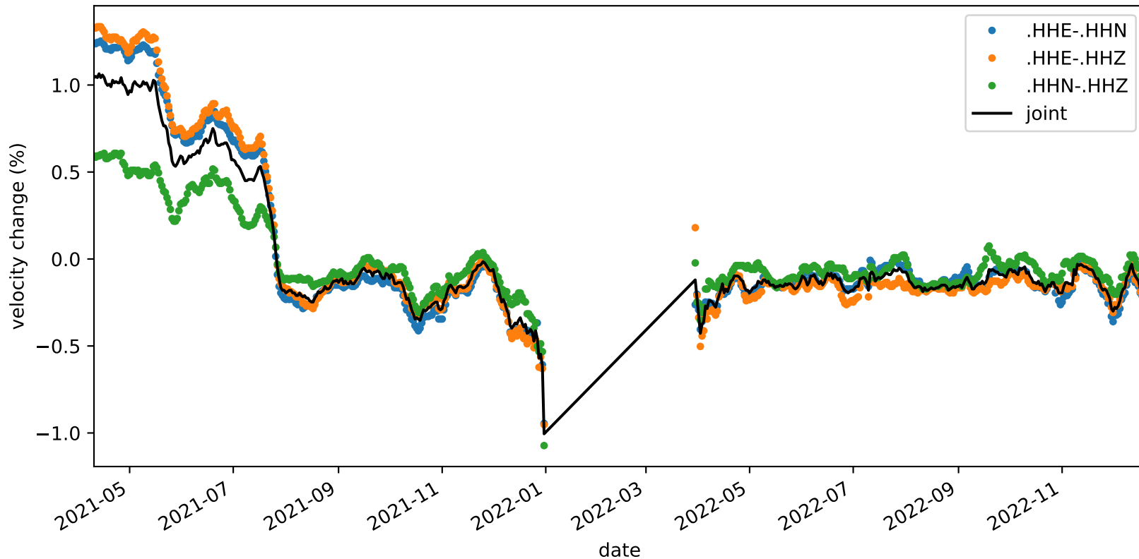
velocity_change_c1b_s3_t1a_tw_005.0s-010.0s_NC.KMPB-NC.KMPB
