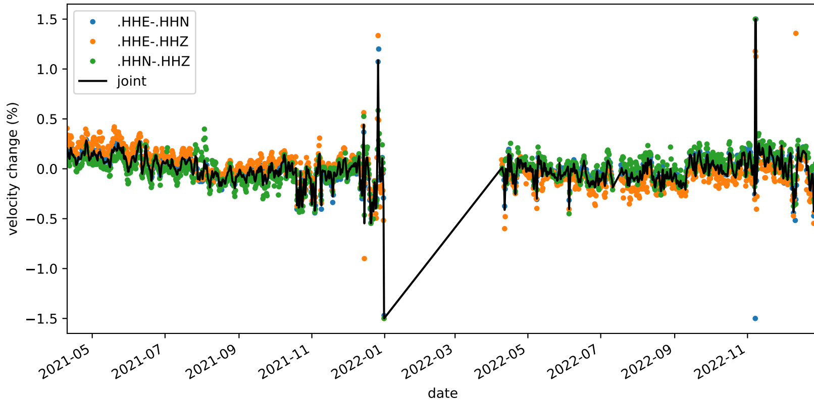
velocity_change_cli_s1_t1a_tw_005.0s-010.0s_NC.KMPB-NC.KMPB
