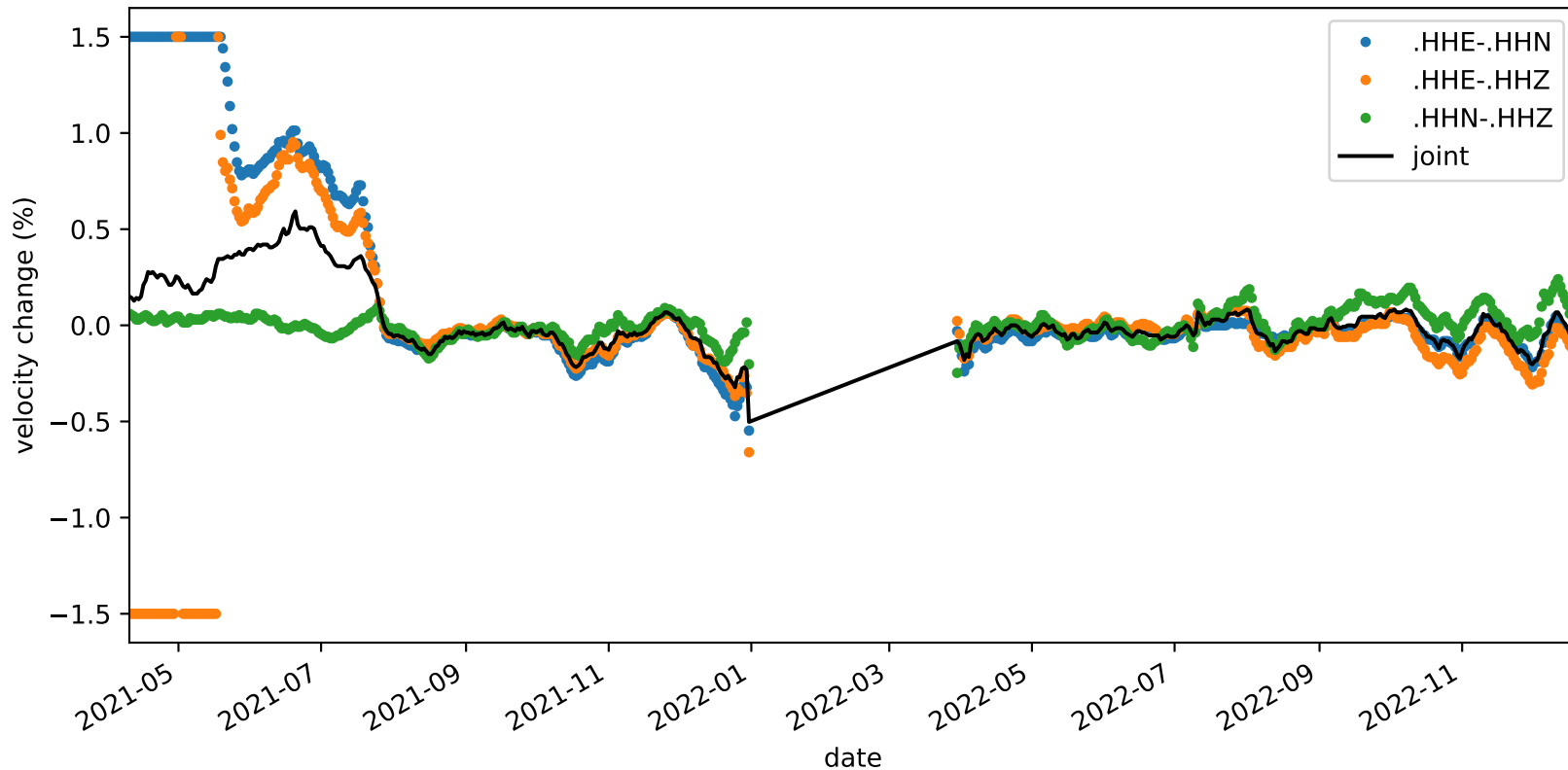
velocity_change_c1b_s3_t1b_tw_010.0s-015.0s_NC.KMPB-NC.KMPB
