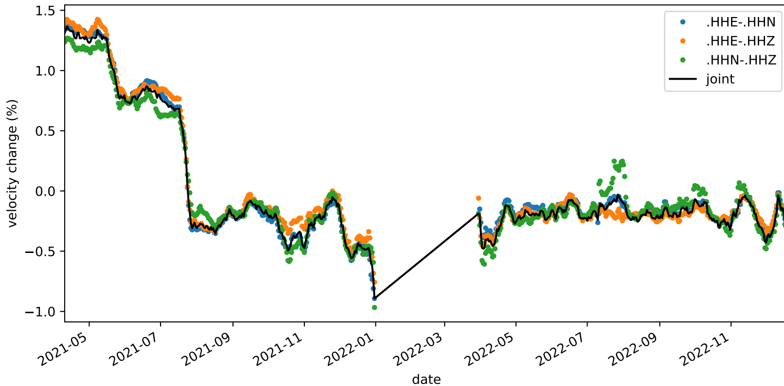
velocity_change_c1f_s3_t1a_tw_005.0s-010.0s_NC.KMPB-NC.KMPB
