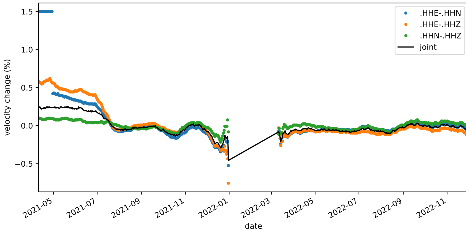
velocity_change_c1h_s2_t1c_tw_005.0s-015.0s_NC.KMPB-NC.KMPB
