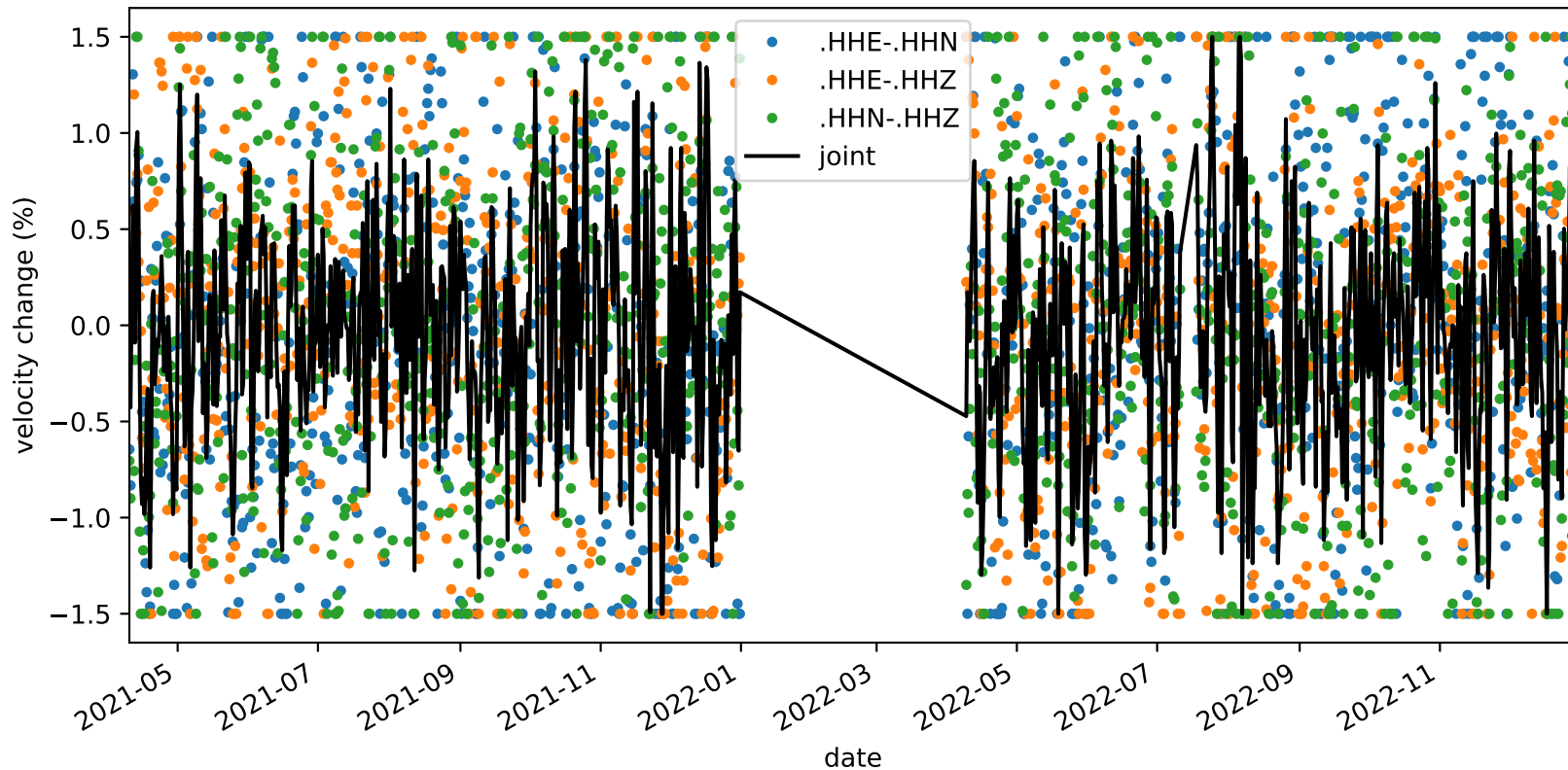
velocity_change_c1d_s1_t1b_tw_010.0s-015.0s_NC.KMPB-NC.KMPB
