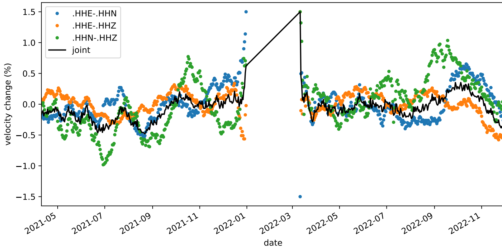
velocity_change_c1d_s2_t1a_tw_005.0s-010.0s_NC.KMPB-NC.KMPB
