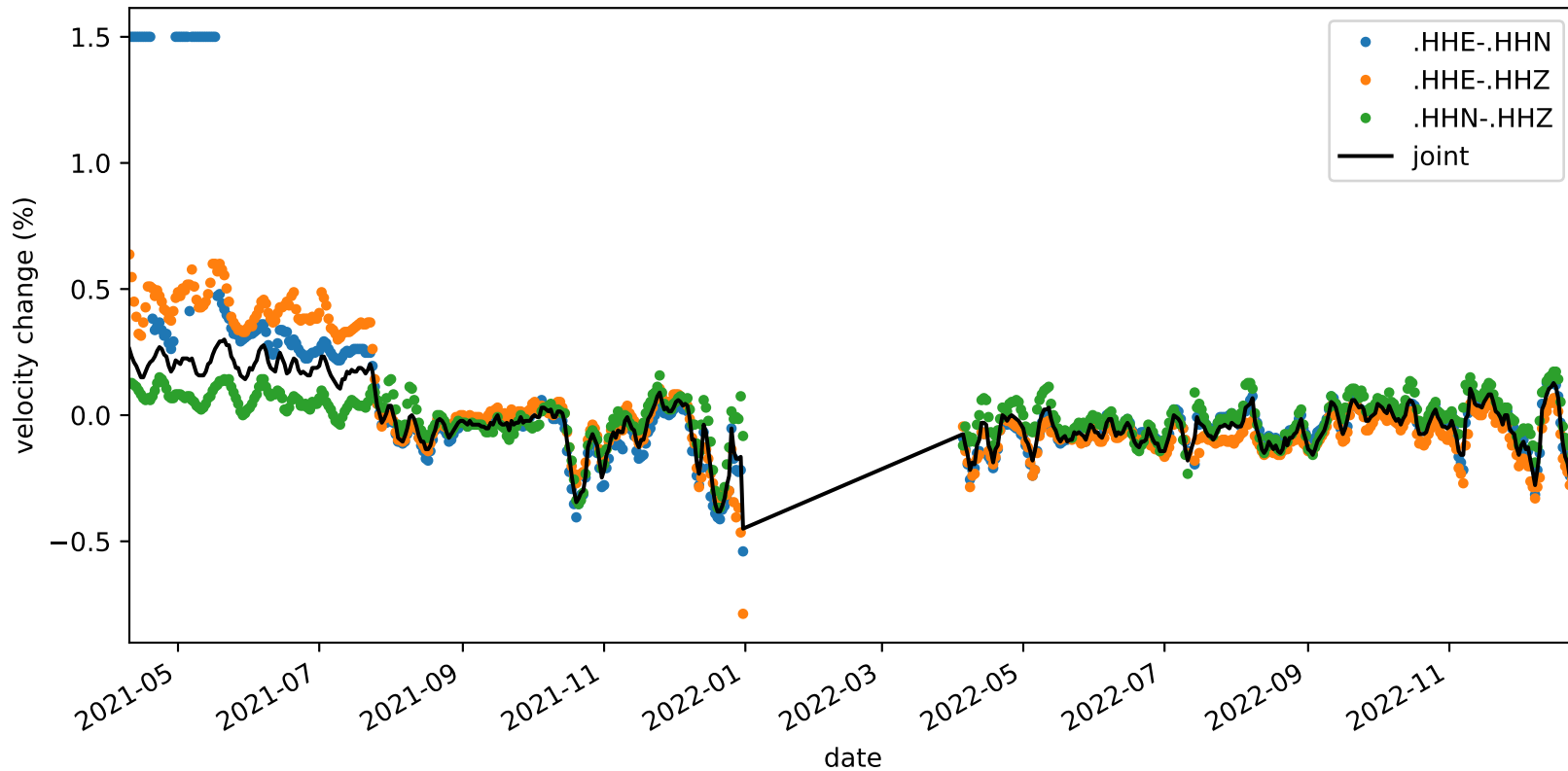
velocity_change_c1h_s4_t1c_tw_005.0s-015.0s_NC.KMPB-NC.KMPB
