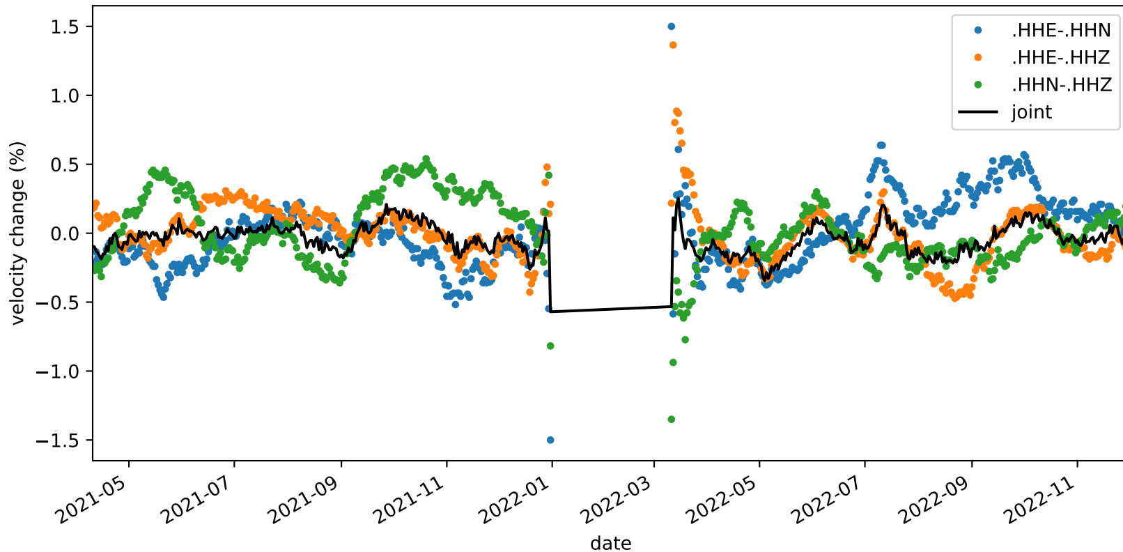
velocity_change_c1d_s2_t1b_tw_010.0s-015.0s_NC.KMPB-NC.KMPB
