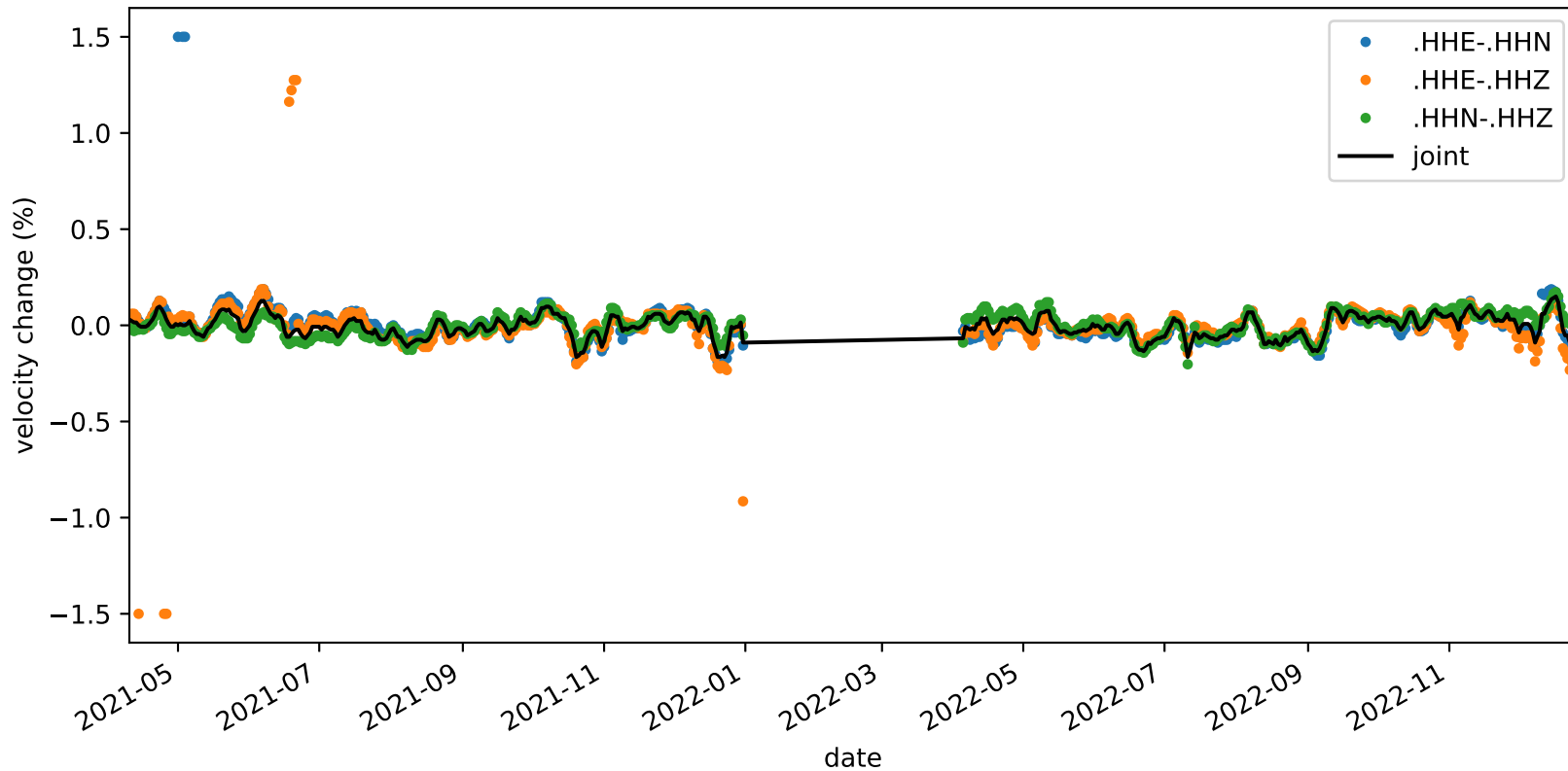
velocity_change_c1i_s4_t1b_tw_010.0s-015.0s_NC.KMPB-NC.KMPB
