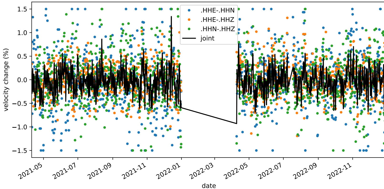
velocity_change_c1e_s1_t1b_tw_010.0s-015.0s_NC.KMPB-NC.KMPB
