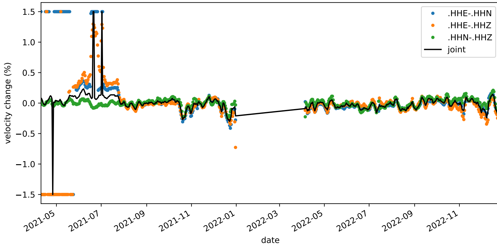
velocity_change_c1h_s4_t1b_tw_010.0s-015.0s_NC.KMPB-NC.KMPB
