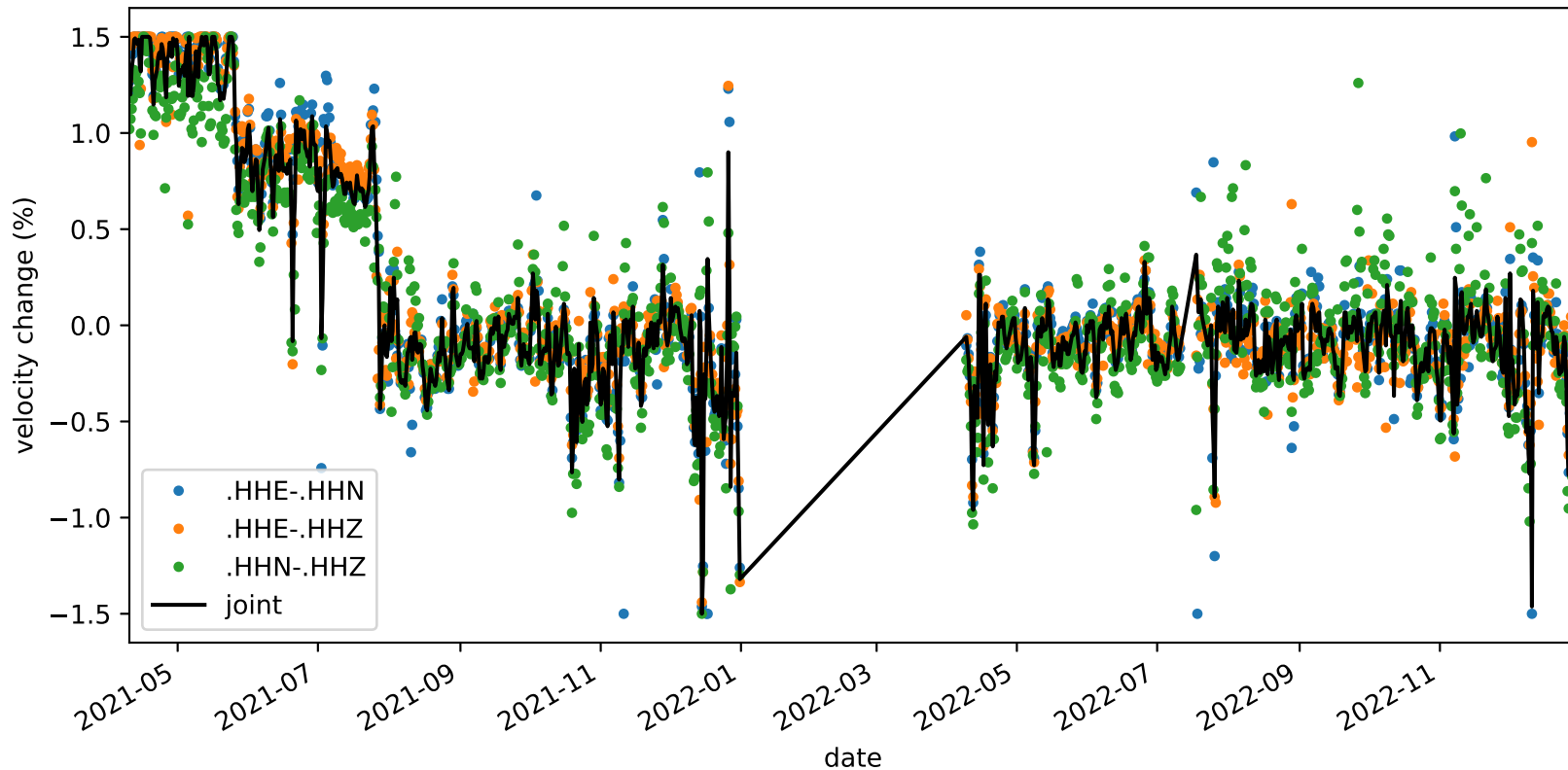
velocity_change_c1f_s1_t1c_tw_005.0s-015.0s_NC.KMPB-NC.KMPB
