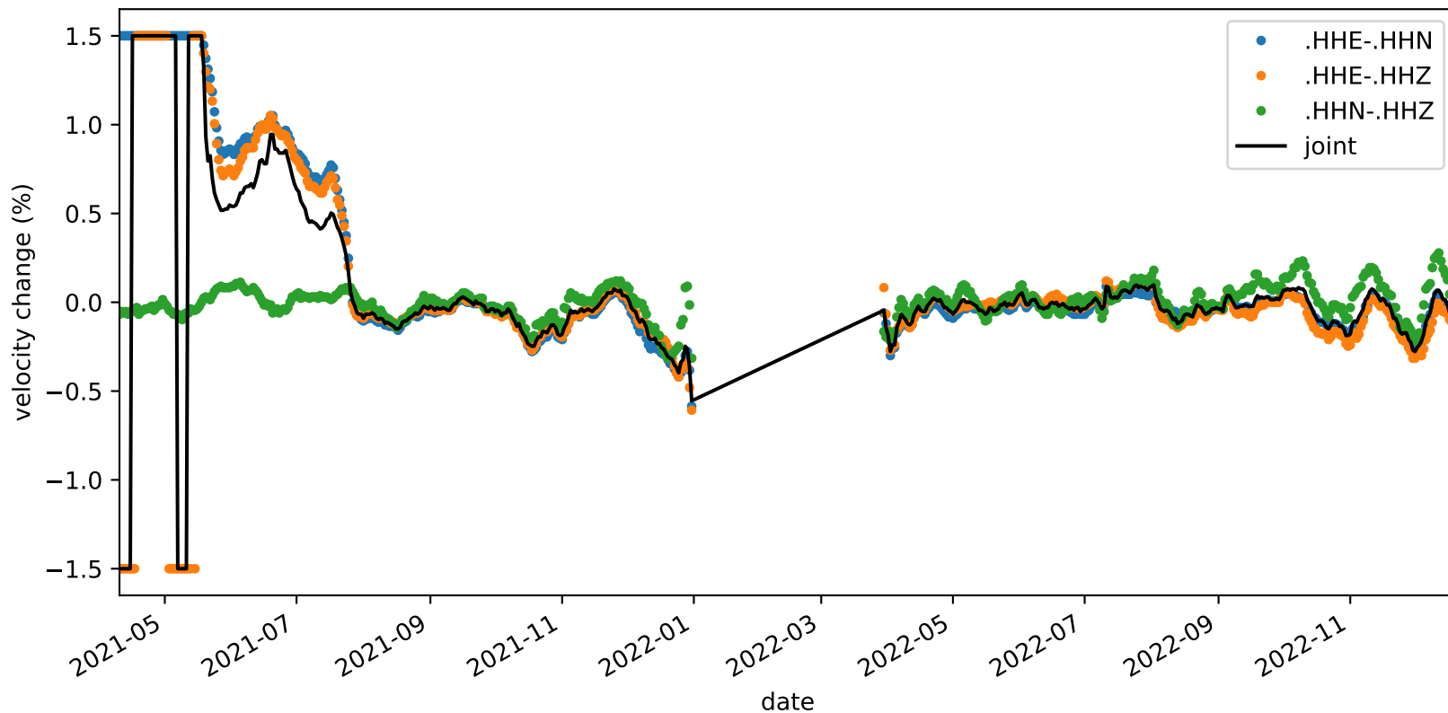
velocity_change_c1g_s3_t1b_tw_010.0s-015.0s_NC.KMPB-NC.KMPB
