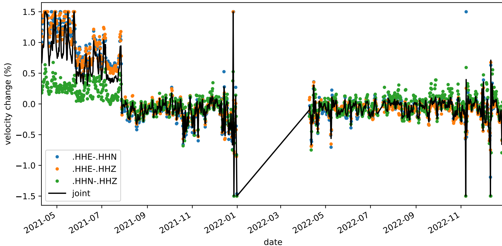
velocity_change_c1b_s1_t1c_tw_005.0s-015.0s_NC.KMPB-NC.KMPB
