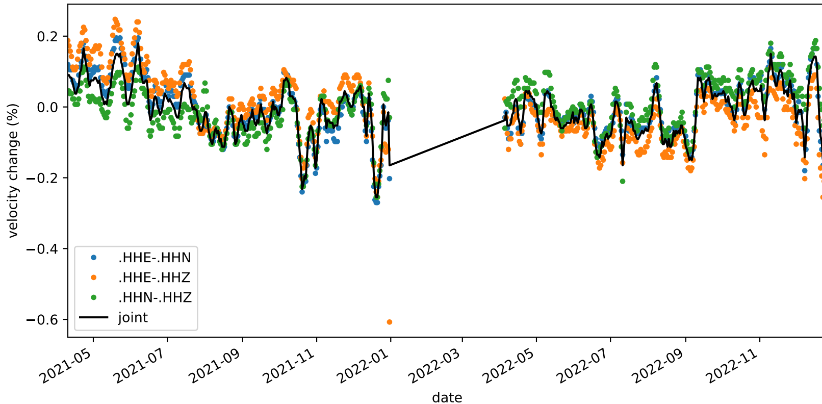
velocity_change_c1i_s4_t1c_tw_005.0s-015.0s_NC.KMPB-NC.KMPB
