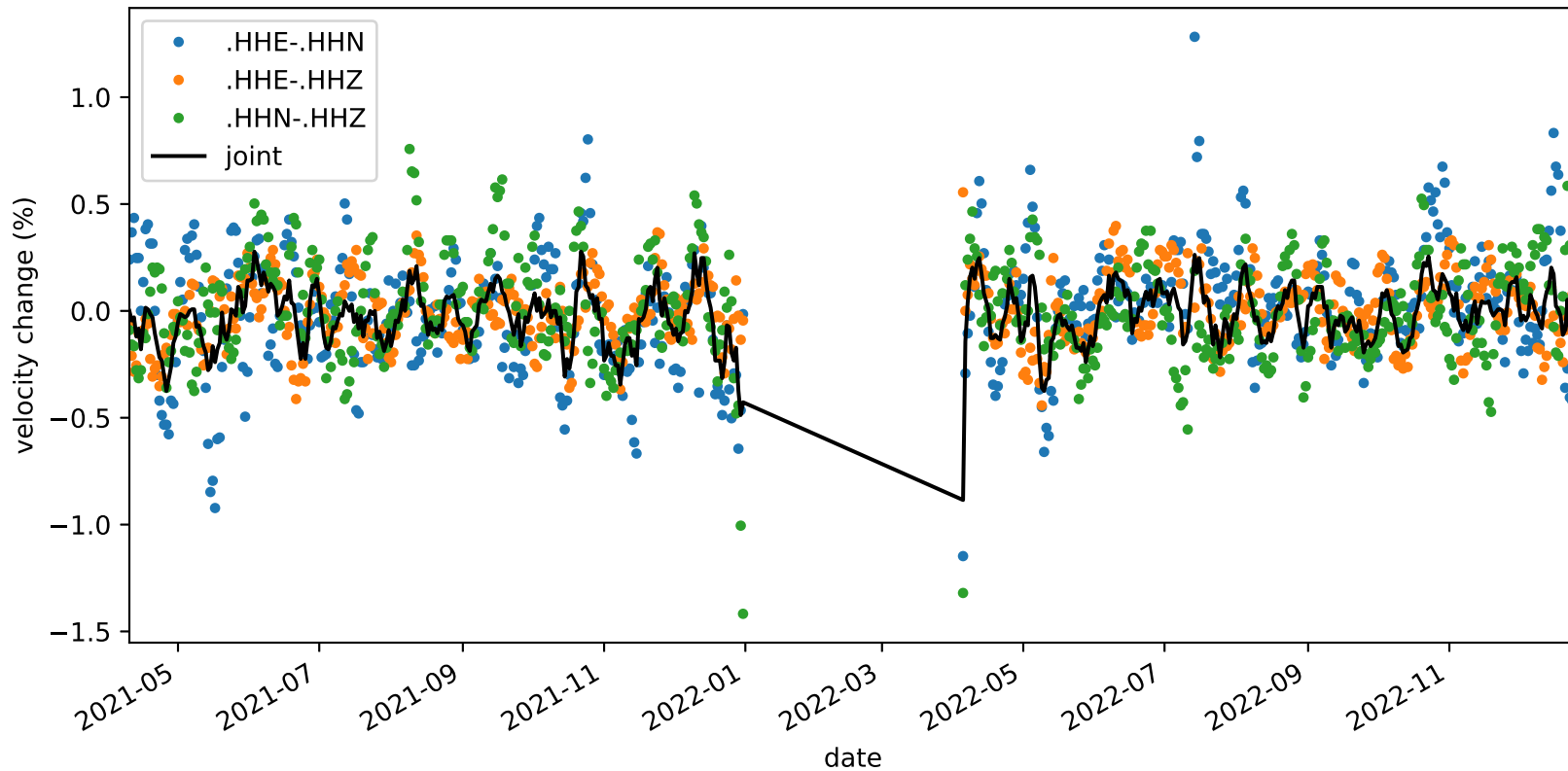
velocity_change_c1e_s4_t1b_tw_010.0s-015.0s_NC.KMPB-NC.KMPB
