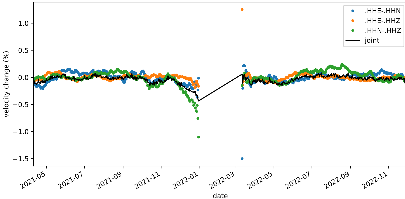
velocity_change_c1e_s2_t1c_tw_005.0s-015.0s_NC.KMPB-NC.KMPB
