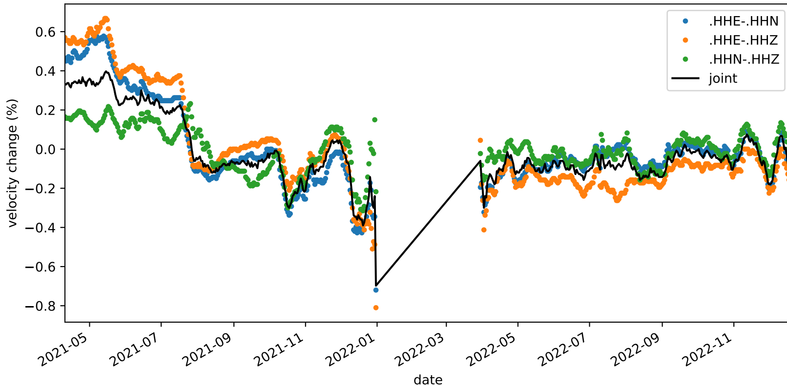
velocity_change_c1h_s3_t1a_tw_005.0s-010.0s_NC.KMPB-NC.KMPB
