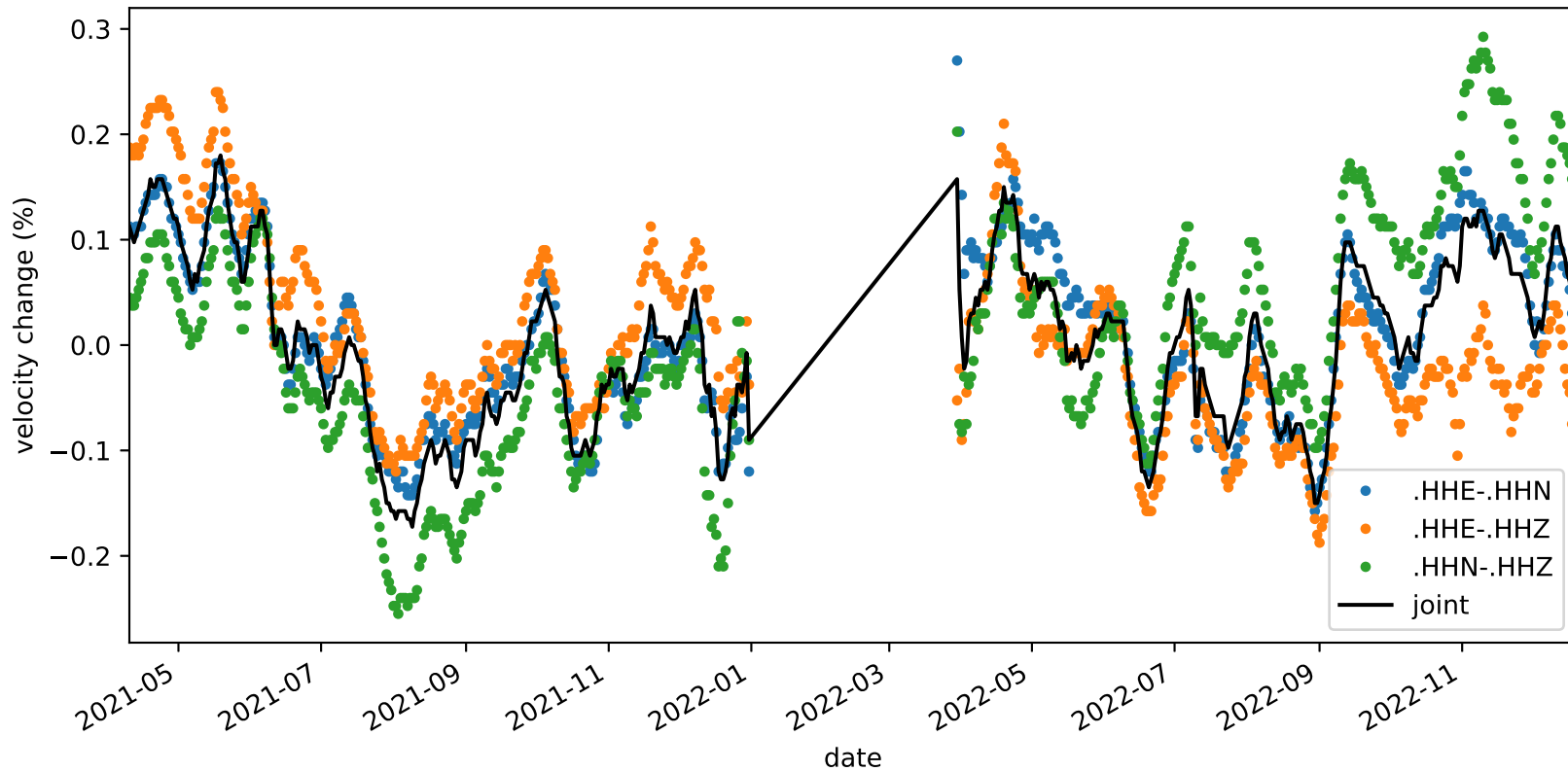
velocity_change_c1c_s3_t1a_tw_005.0s-010.0s_NC.KMPB-NC.KMPB
