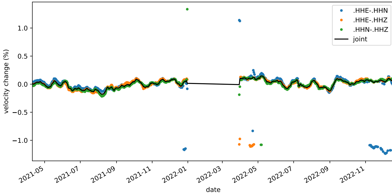
velocity_change_c1c_s3_t1b_tw_010.0s-015.0s_NC.KMPB-NC.KMPB
