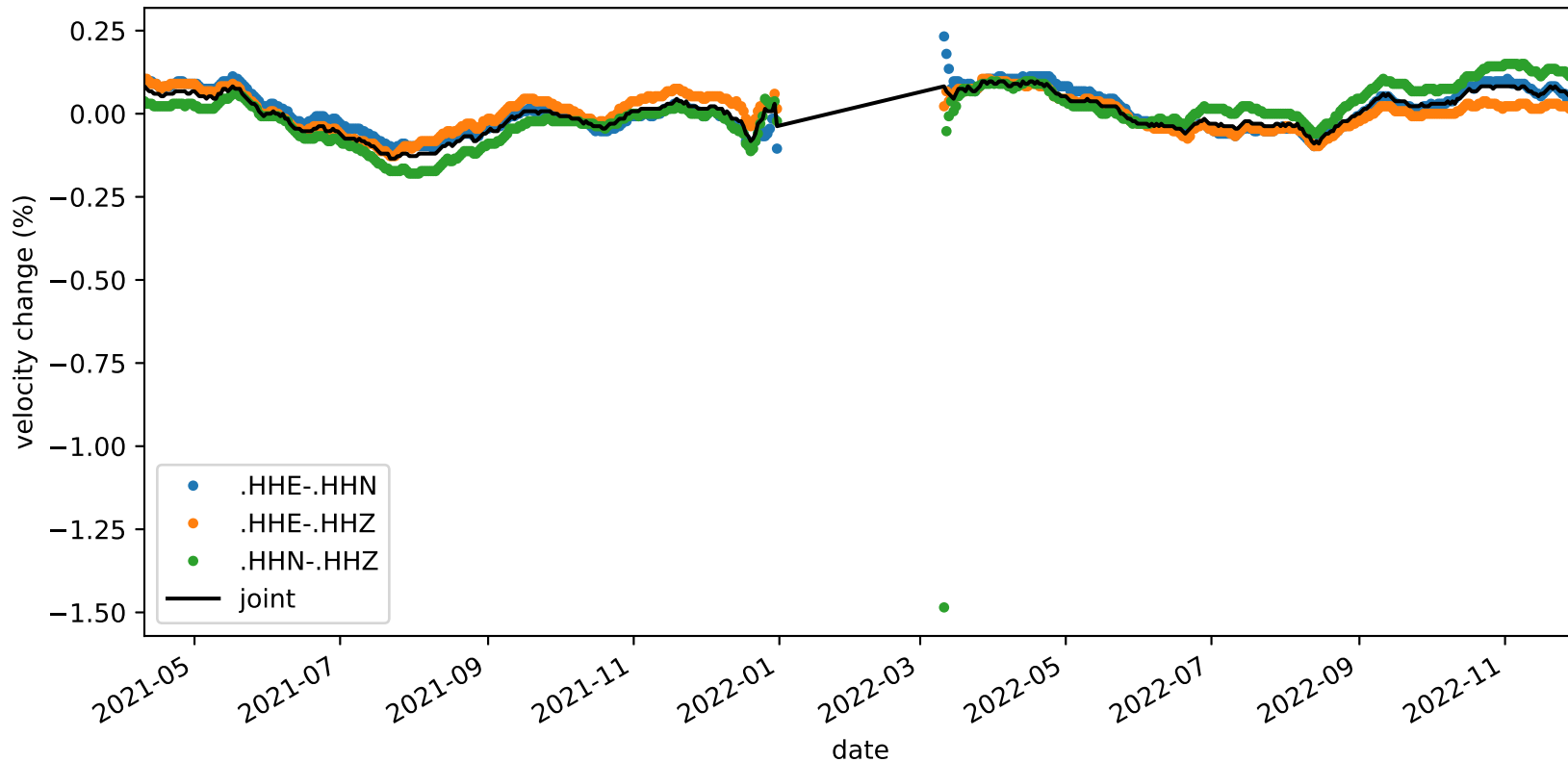
velocity_change_c1c_s2_t1c_tw_005.0s-015.0s_NC.KMPB-NC.KMPB
