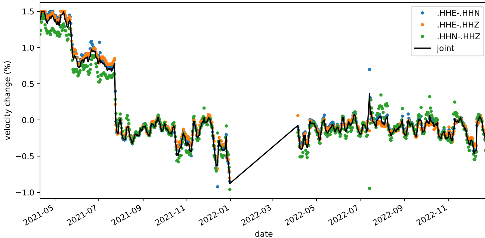
velocity_change_c1f_s4_t1c_tw_005.0s-015.0s_NC.KMPB-NC.KMPB
