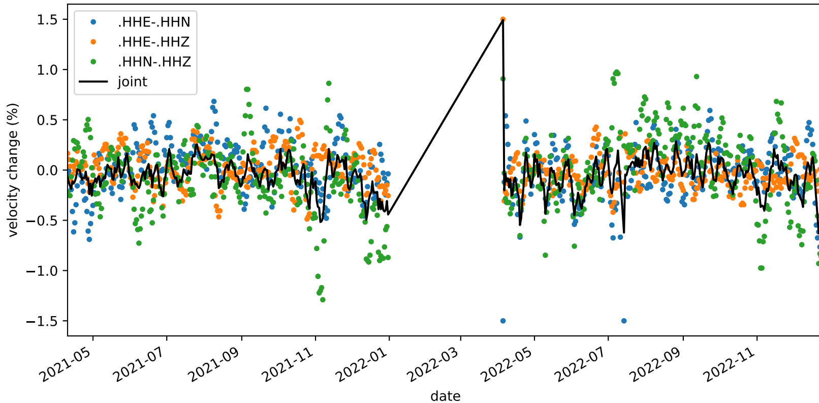
velocity_change_c1e_s4_t1a_tw_005.0s-010.0s_NC.KMPB-NC.KMPB
