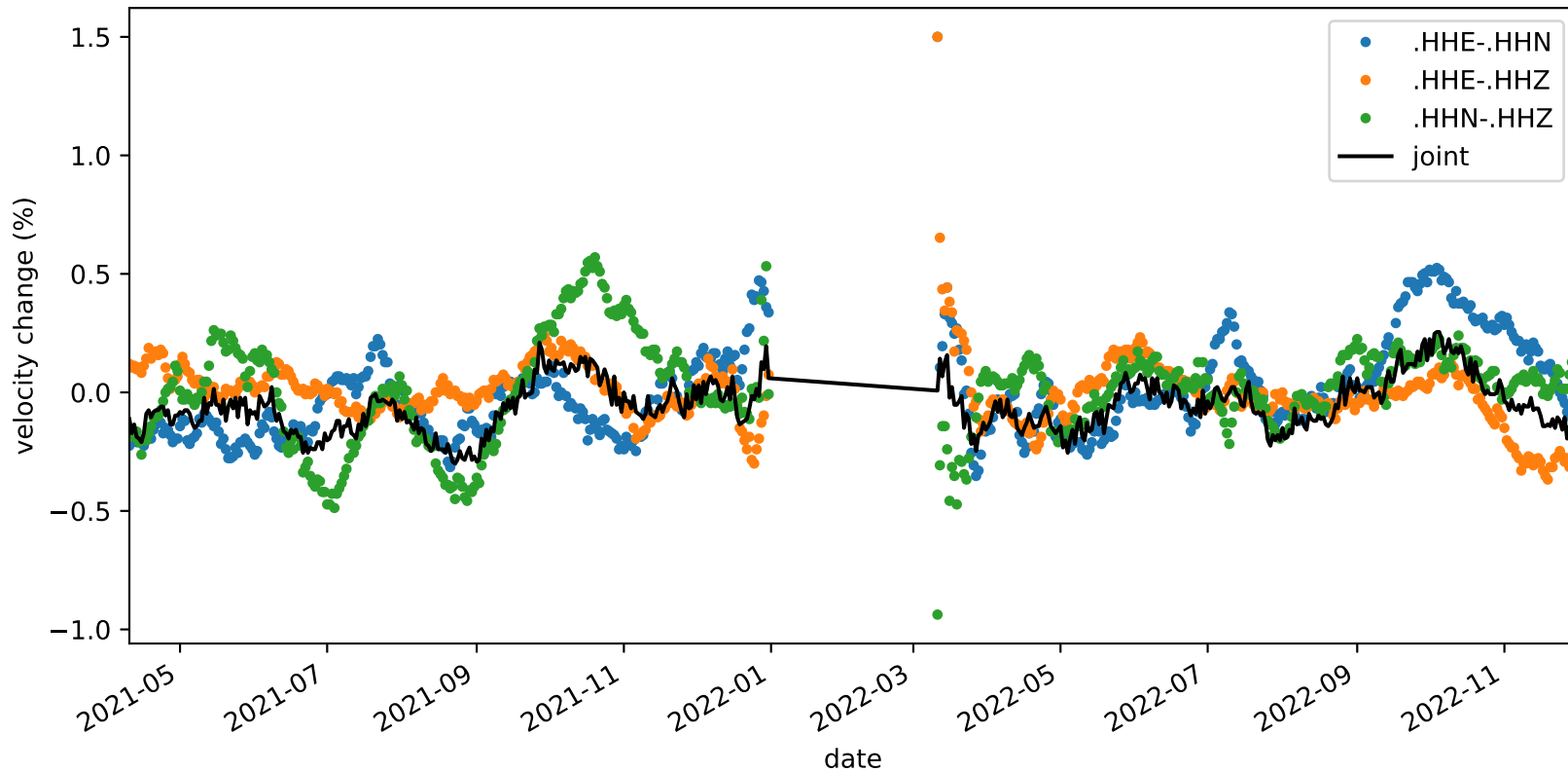
velocity_change_c1d_s2_t1c_tw_005.0s-015.0s_NC.KMPB-NC.KMPB
