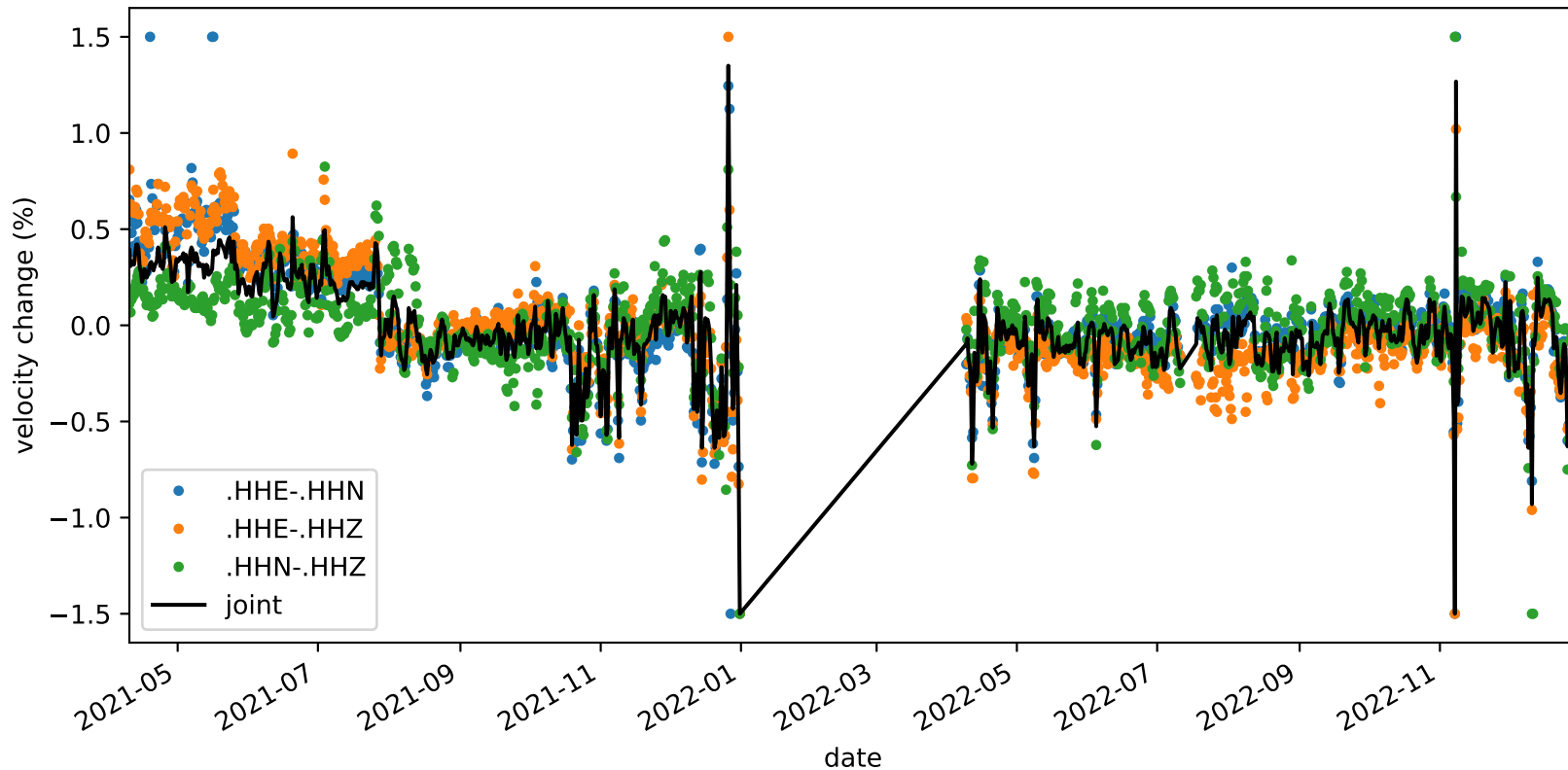
velocity_change_c1h_s1_t1a_tw_005.0s-010.0s_NC.KMPB-NC.KMPB
