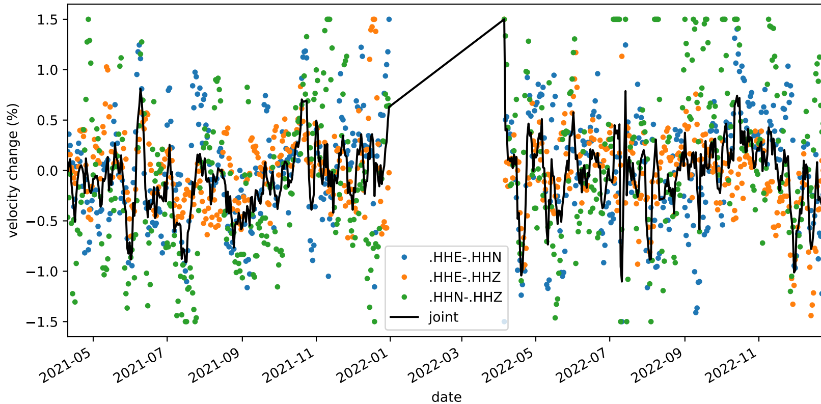
velocity_change_c1d_s4_t1a_tw_005.0s-010.0s_NC.KMPB-NC.KMPB
