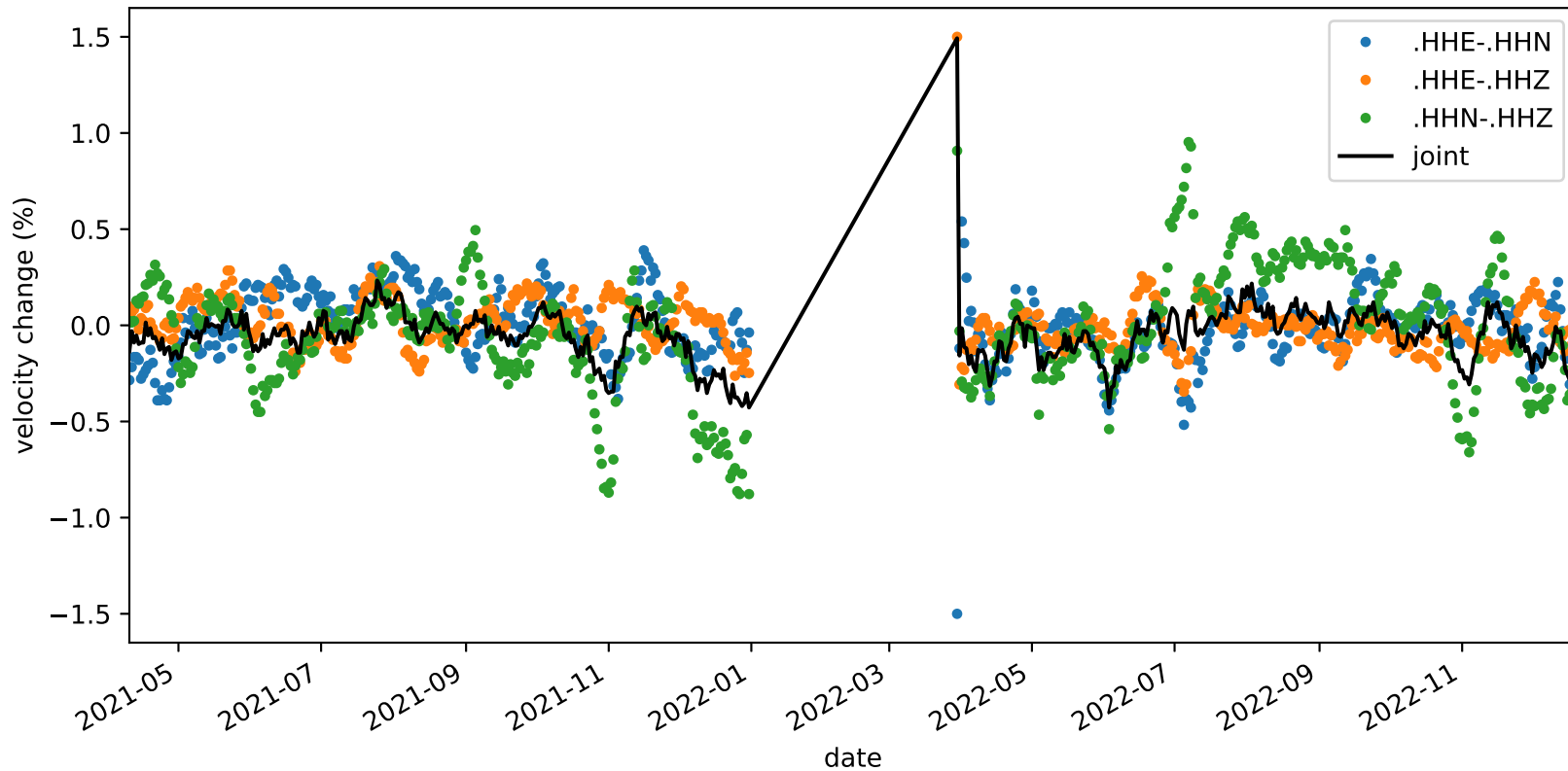
velocity_change_c1e_s3_t1a_tw_005.0s-010.0s_NC.KMPB-NC.KMPB
