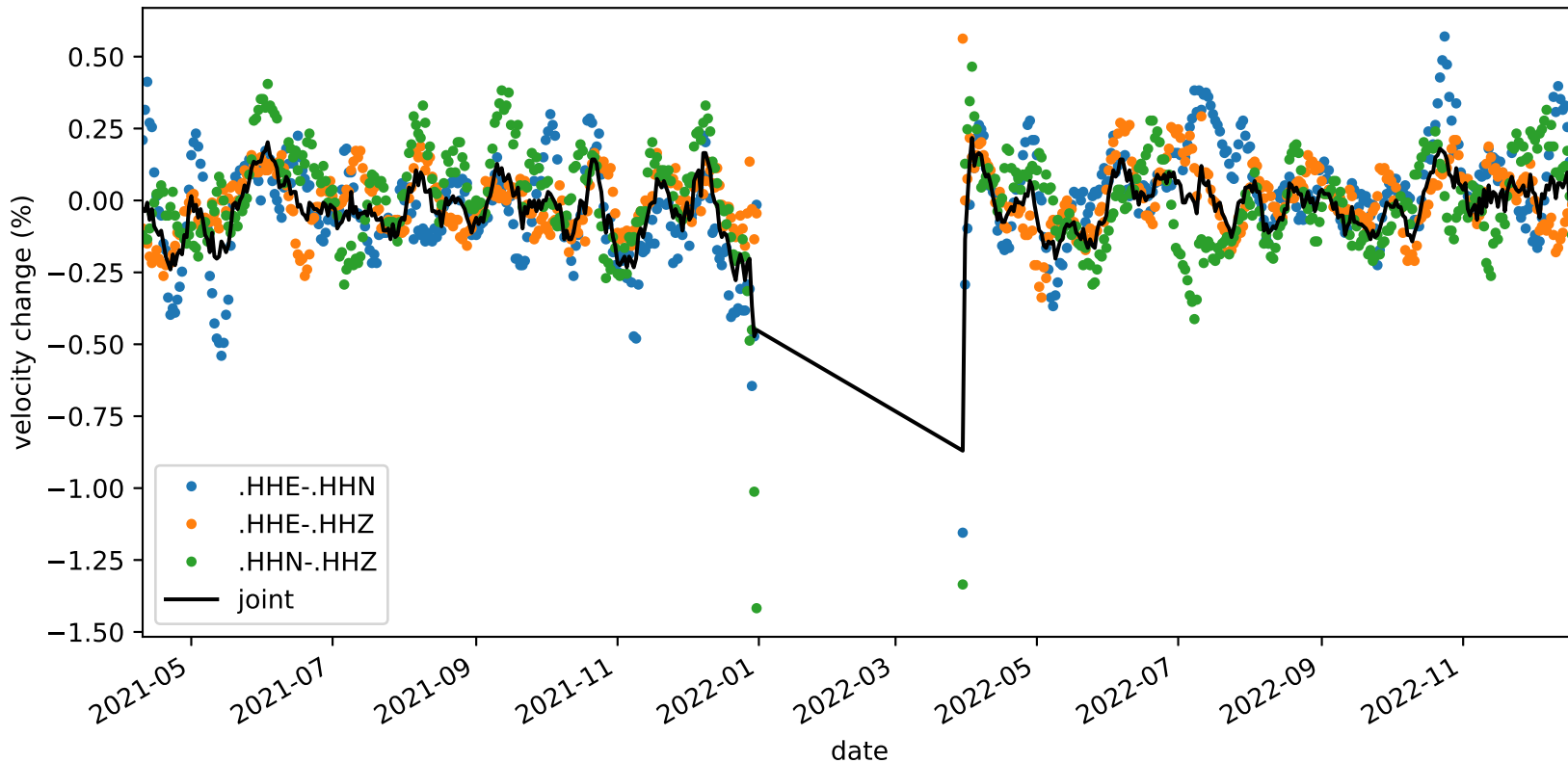
velocity_change_c1e_s3_t1b_tw_010.0s-015.0s_NC.KMPB-NC.KMPB
