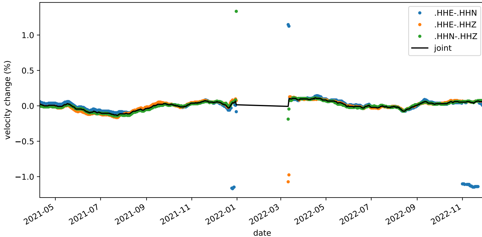
velocity_change_c1c_s2_t1b_tw_010.0s-015.0s_NC.KMPB-NC.KMPB
