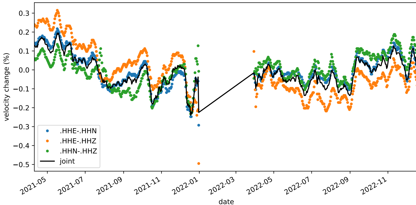
velocity_change_c1i_s3_t1a_tw_005.0s-010.0s_NC.KMPB-NC.KMPB
