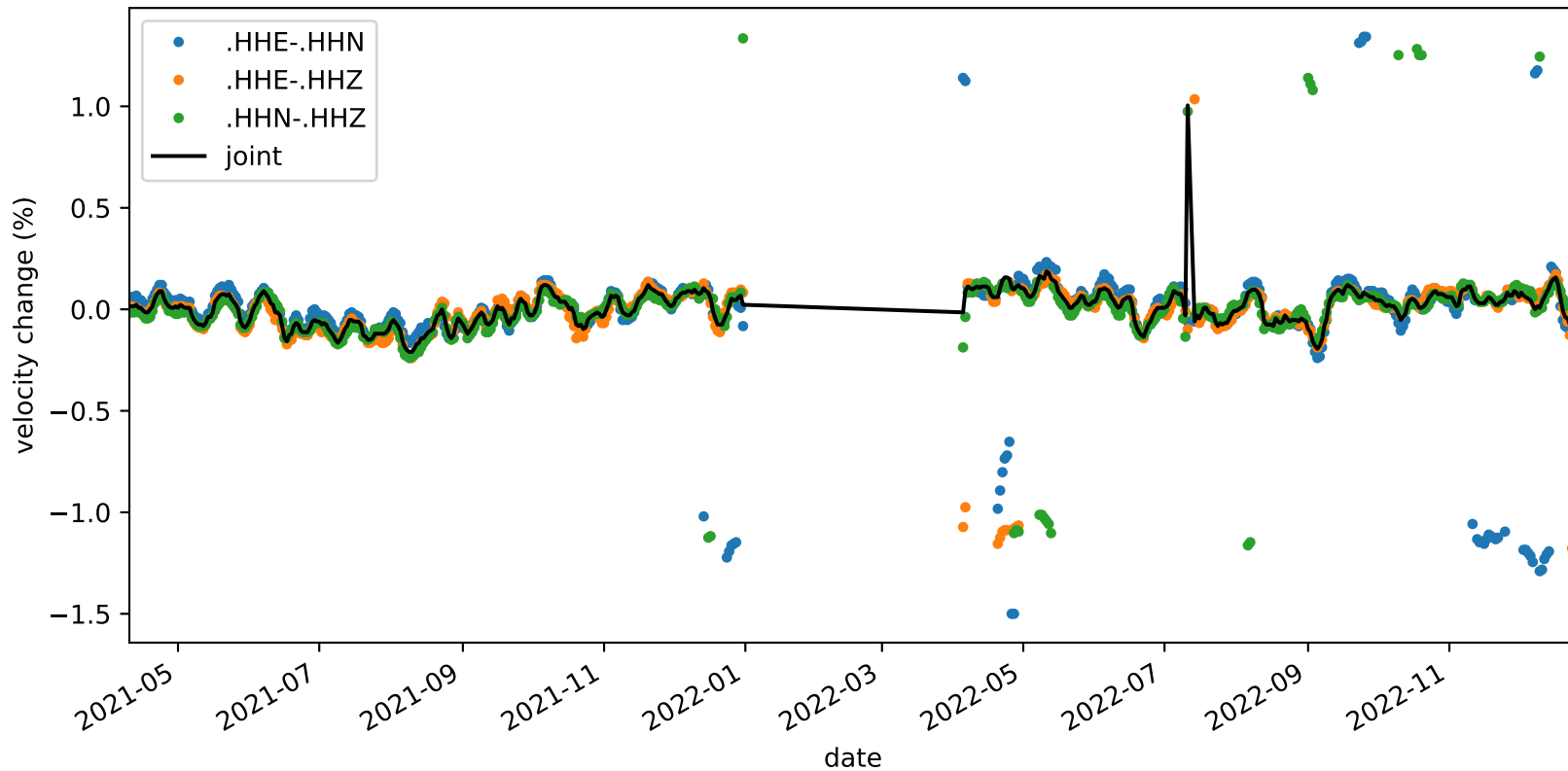
velocity_change_c1c_s4_t1b_tw_010.0s-015.0s_NC.KMPB-NC.KMPB
