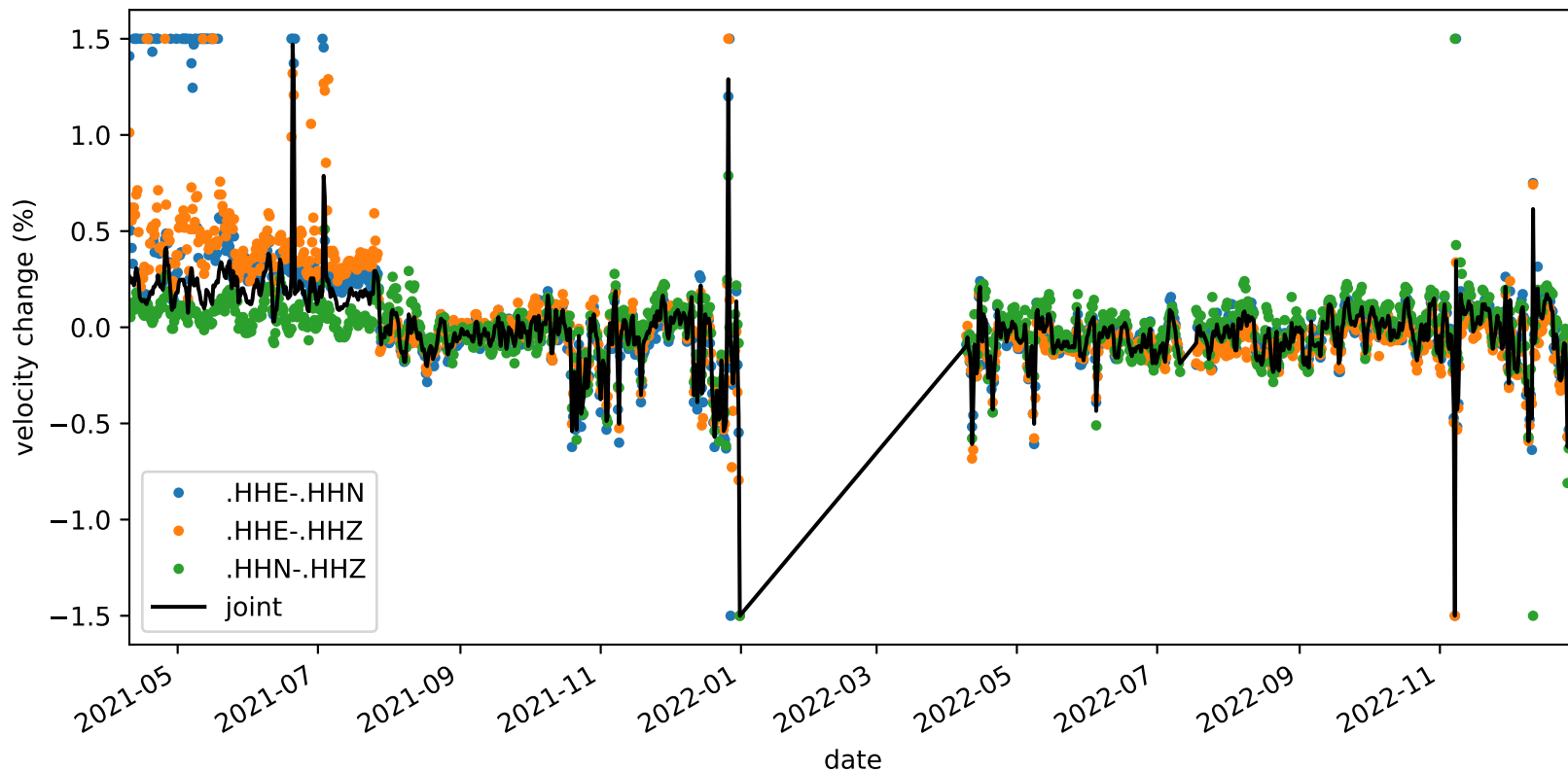
velocity_change_c1h_s1_t1c_tw_005.0s-015.0s_NC.KMPB-NC.KMPB
