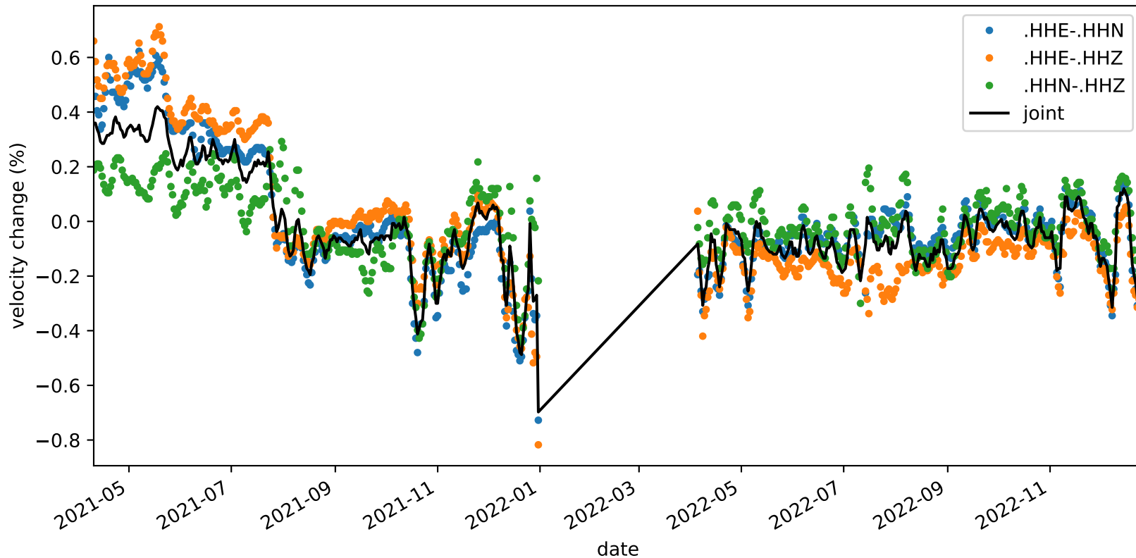
velocity_change_c1h_s4_t1a_tw_005.0s-010.0s_NC.KMPB-NC.KMPB
