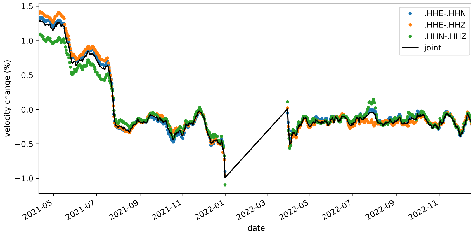
velocity_change_c1g_s3_t1a_tw_005.0s-010.0s_NC.KMPB-NC.KMPB
