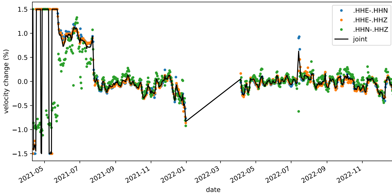
velocity_change_c1f_s4_t1b_tw_010.0s-015.0s_NC.KMPB-NC.KMPB
