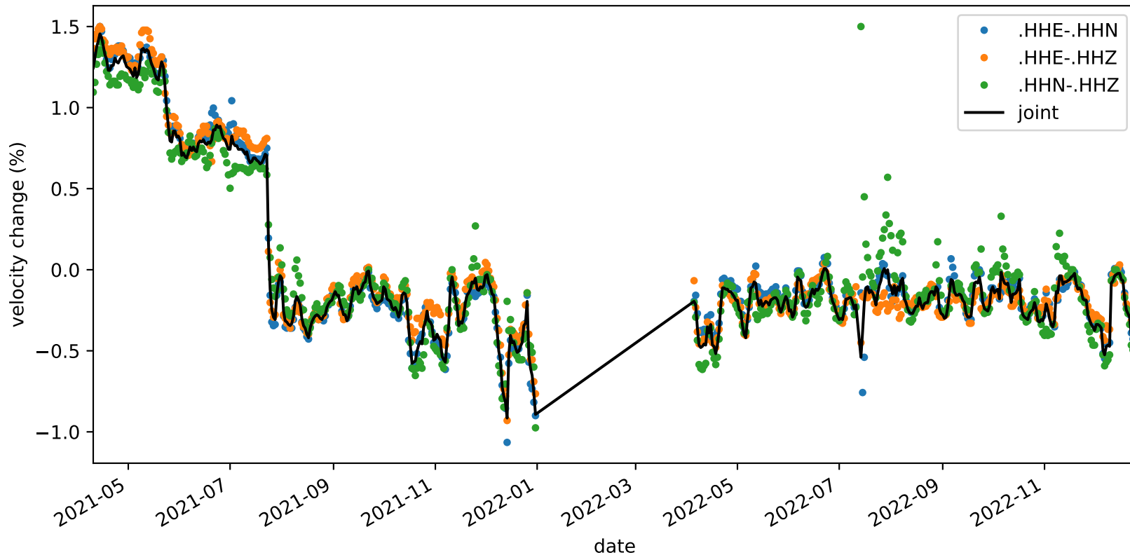
velocity_change_c1f_s4_t1a_tw_005.0s-010.0s_NC.KMPB-NC.KMPB
