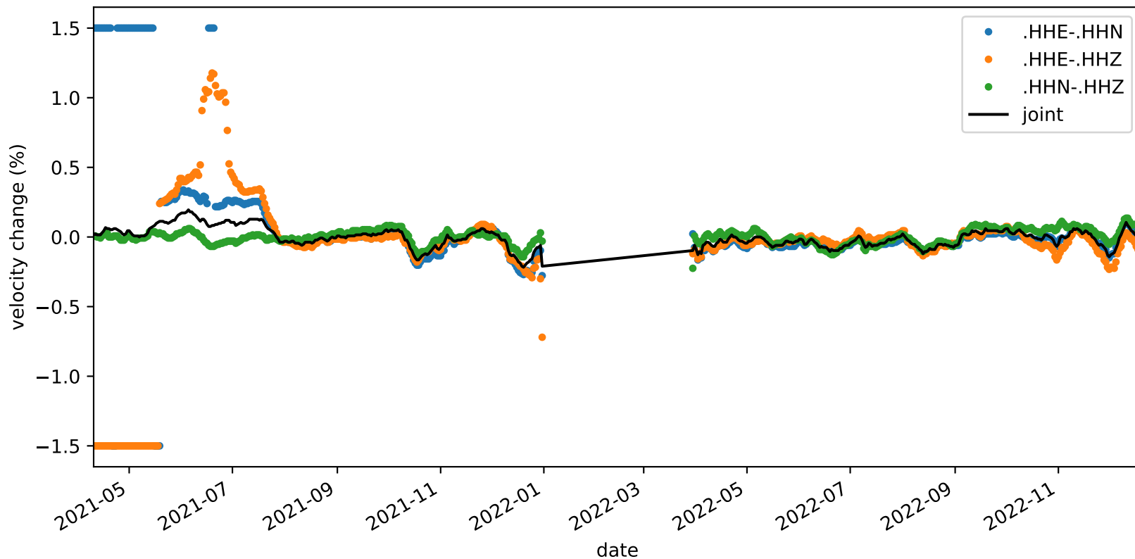
velocity_change_c1h_s3_t1b_tw_010.0s-015.0s_NC.KMPB-NC.KMPB
