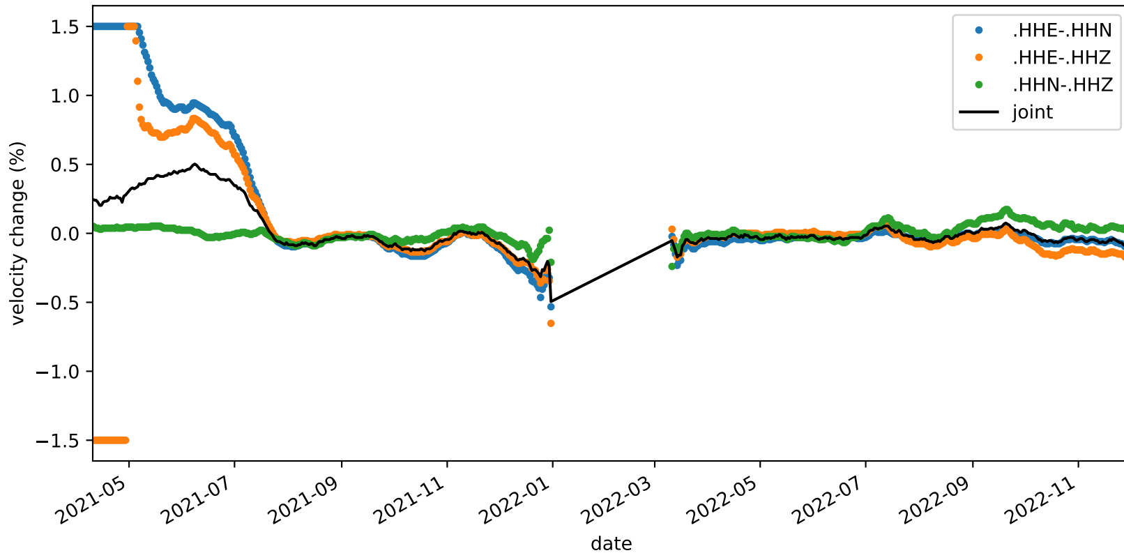
velocity_change_c1b_s2_t1b_tw_010.0s-015.0s_NC.KMPB-NC.KMPB
