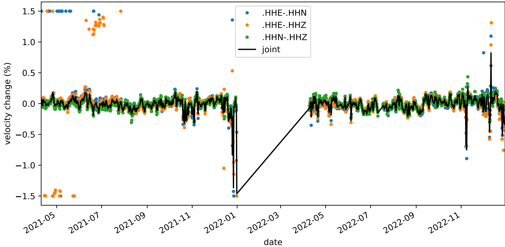
velocity_change_cli_s1_t1b_tw_010.0s-015.0s_NC.KMPB-NC.KMPB
