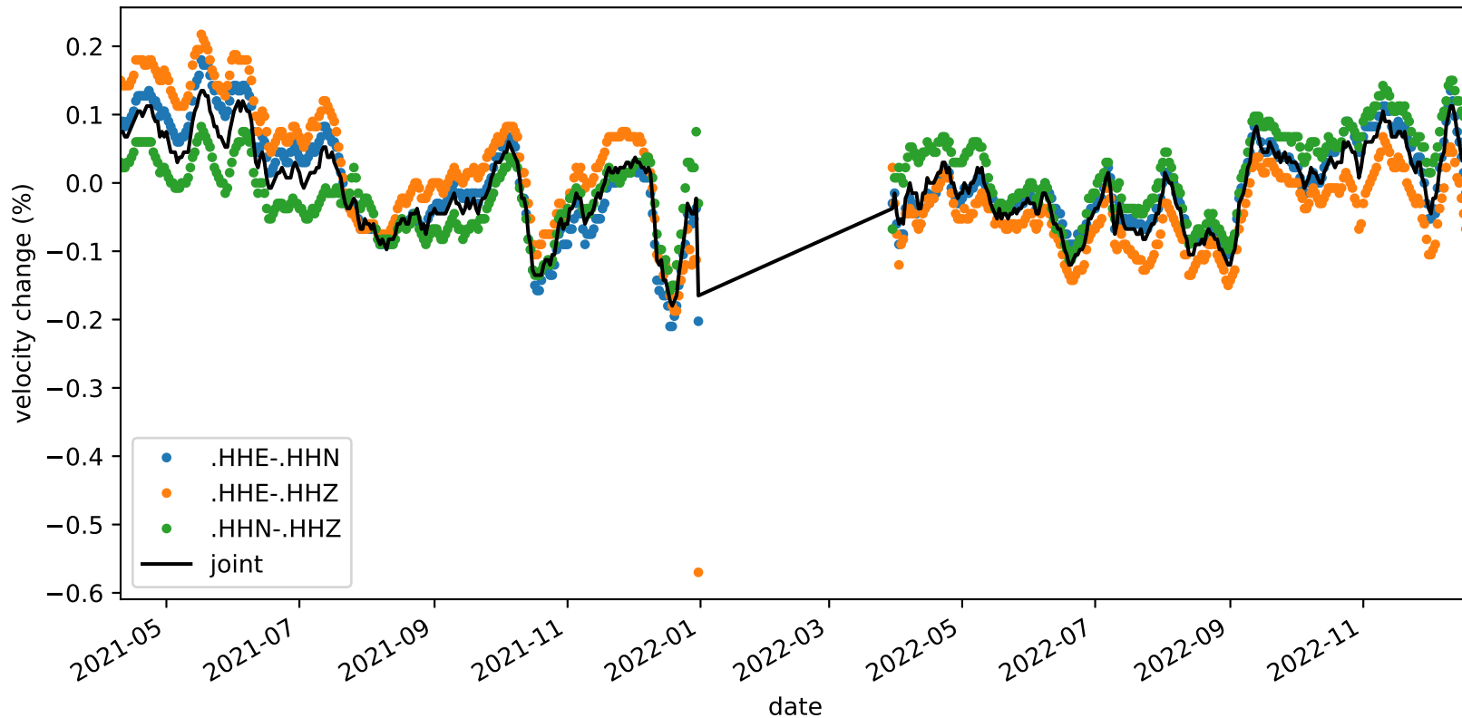
velocity_change_c1i_s3_t1c_tw_005.0s-015.0s_NC.KMPB-NC.KMPB
