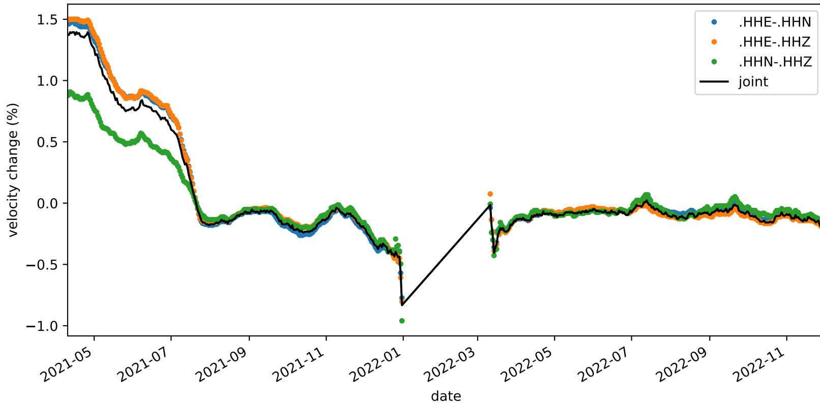
velocity_change_c1g_s2_t1c_tw_005.0s-015.0s_NC.KMPB-NC.KMPB
