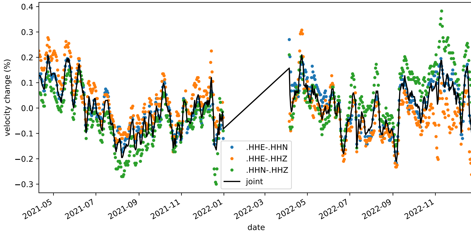
velocity_change_c1c_s4_t1a_tw_005.0s-010.0s_NC.KMPB-NC.KMPB
