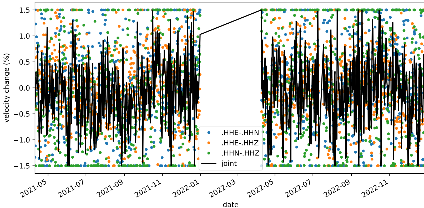
velocity_change_c1d_s1_t1a_tw_005.0s-010.0s_NC.KMPB-NC.KMPB
