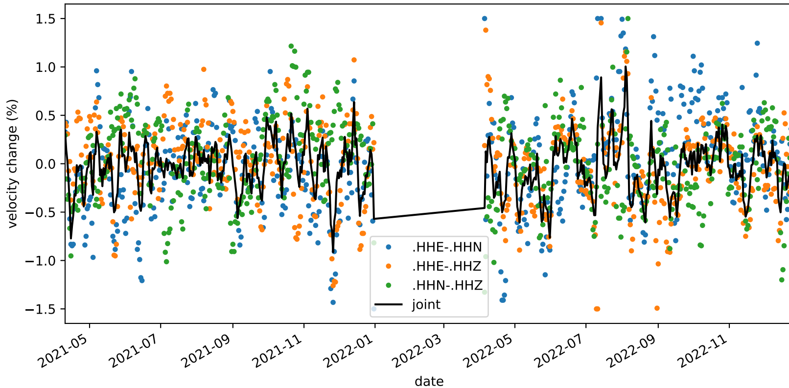
velocity_change_c1d_s4_t1b_tw_010.0s-015.0s_NC.KMPB-NC.KMPB
