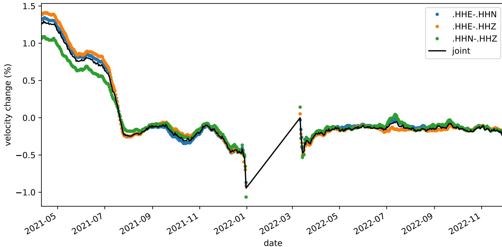
velocity_change_c1g_s2_t1a_tw_005.0s-010.0s_NC.KMPB-NC.KMPB
