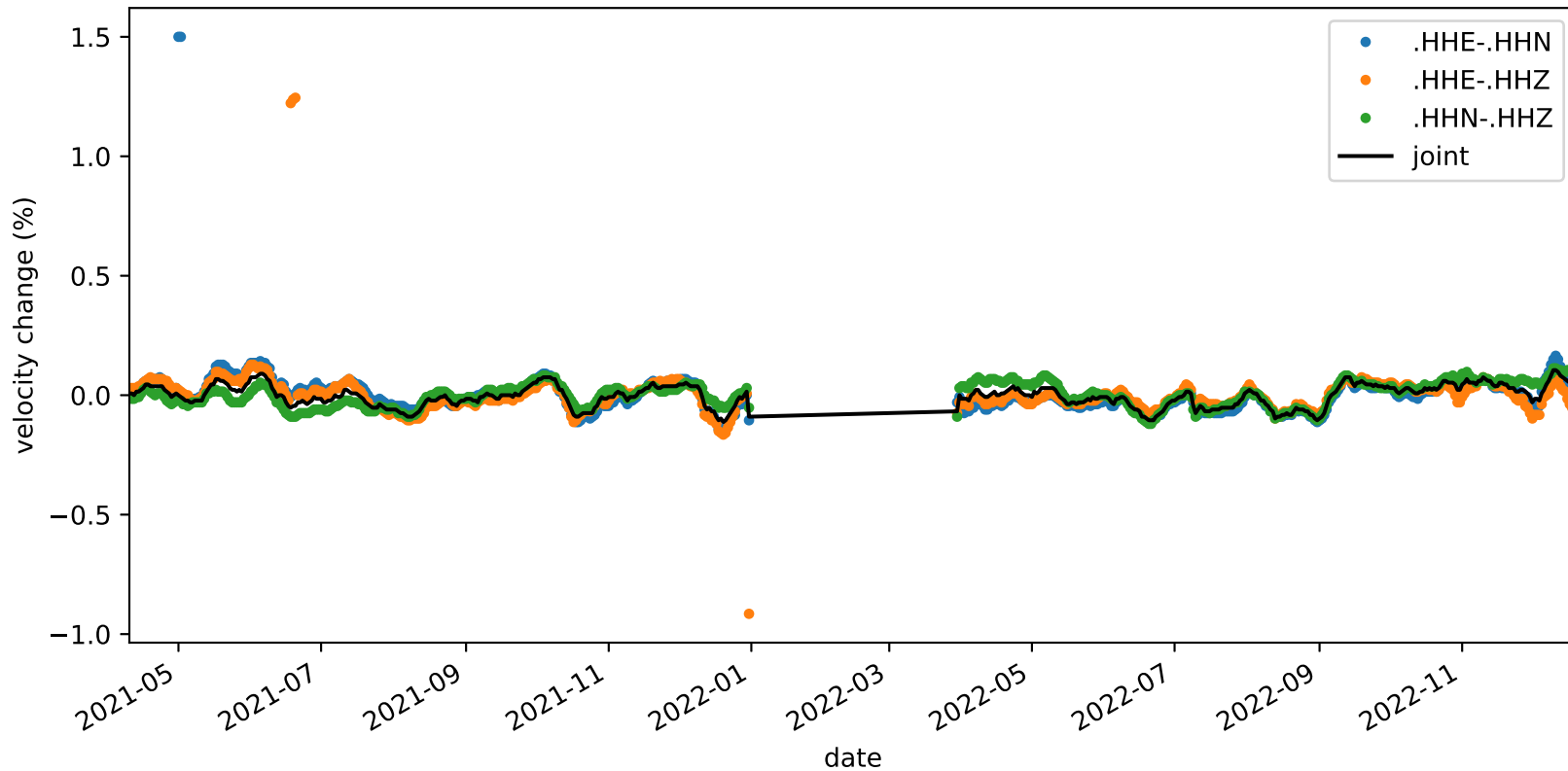
velocity_change_c1i_s3_t1b_tw_010.0s-015.0s_NC.KMPB-NC.KMPB
