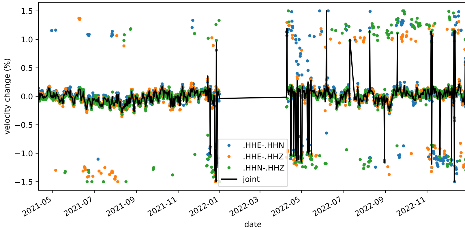
velocity_change_c1c_s1_t1b_tw_010.0s-015.0s_NC.KMPB-NC.KMPB
