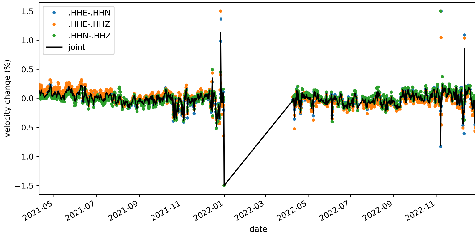
velocity_change_cli_s1_t1c_tw_005.0s-015.0s_NC.KMPB-NC.KMPB
