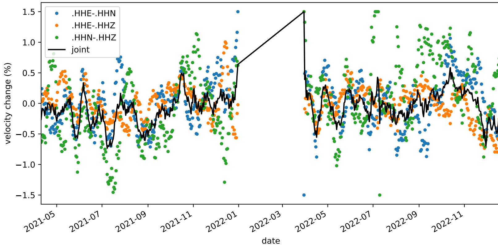
velocity_change_c1d_s3_t1a_tw_005.0s-010.0s_NC.KMPB-NC.KMPB
