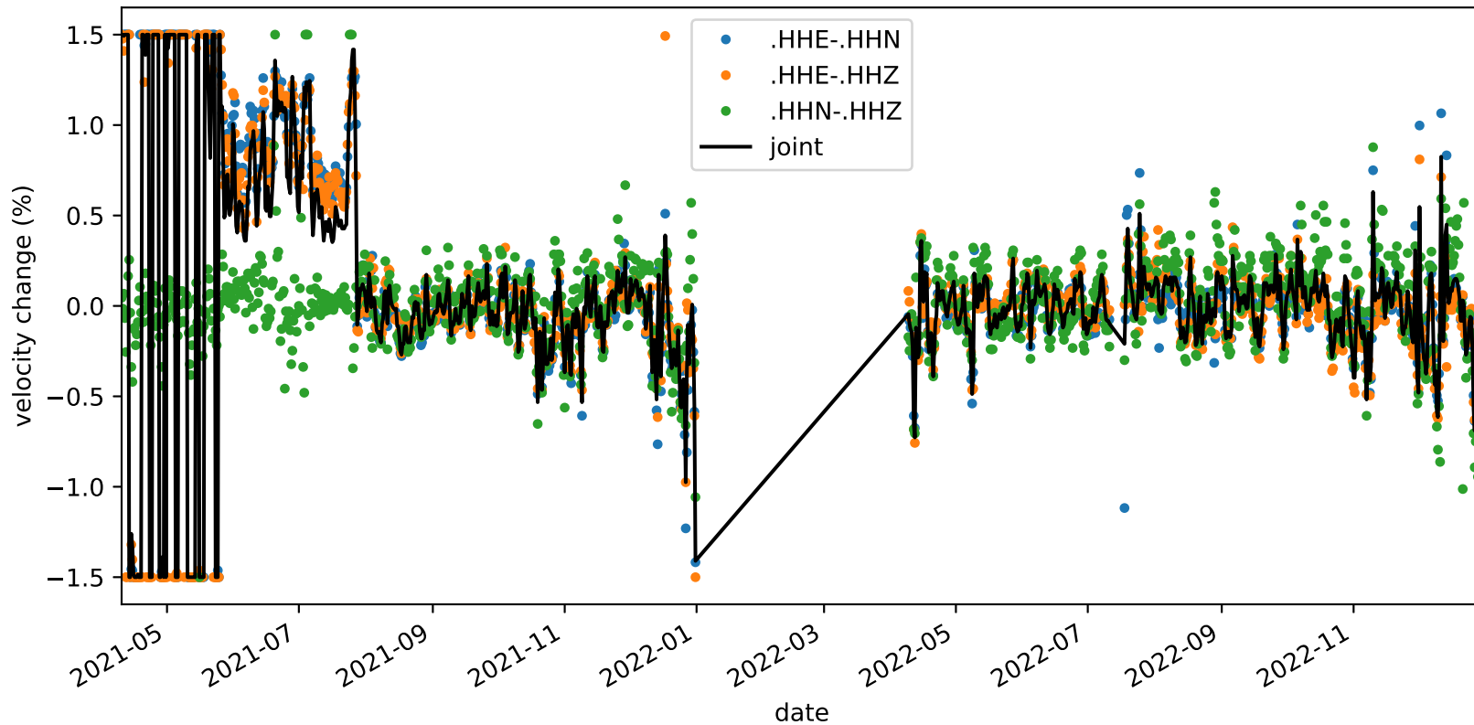
velocity_change_c1g_s1_t1b_tw_010.0s-015.0s_NC.KMPB-NC.KMPB
