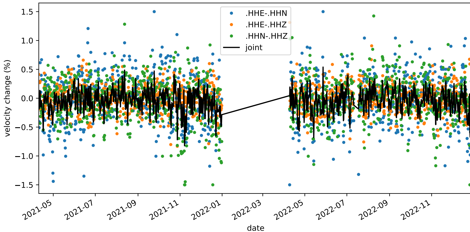
velocity_change_c1e_s1_t1c_tw_005.0s-015.0s_NC.KMPB-NC.KMPB
