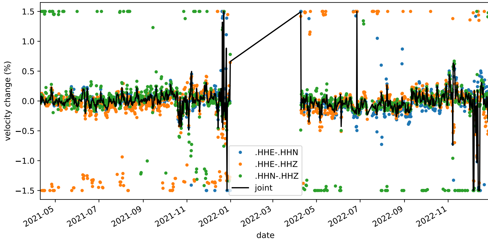
velocity_change_c1_s1_t1b_tw_010.0s-015.0s_NC.KMPB-NC.KMPB
