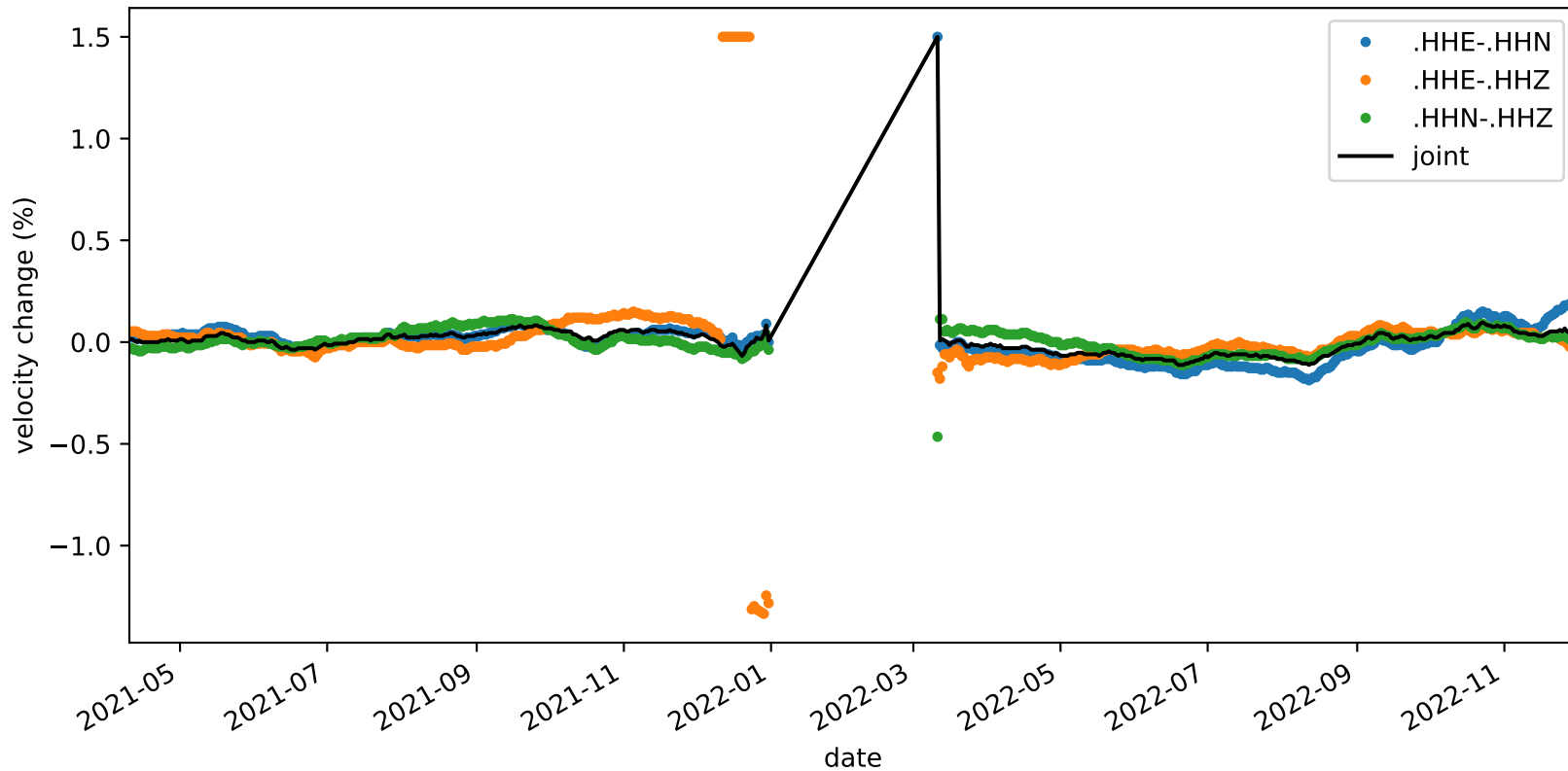
velocity_change_c1_s2_t1b_tw_010.0s-015.0s_NC.KMPB-NC.KMPB
