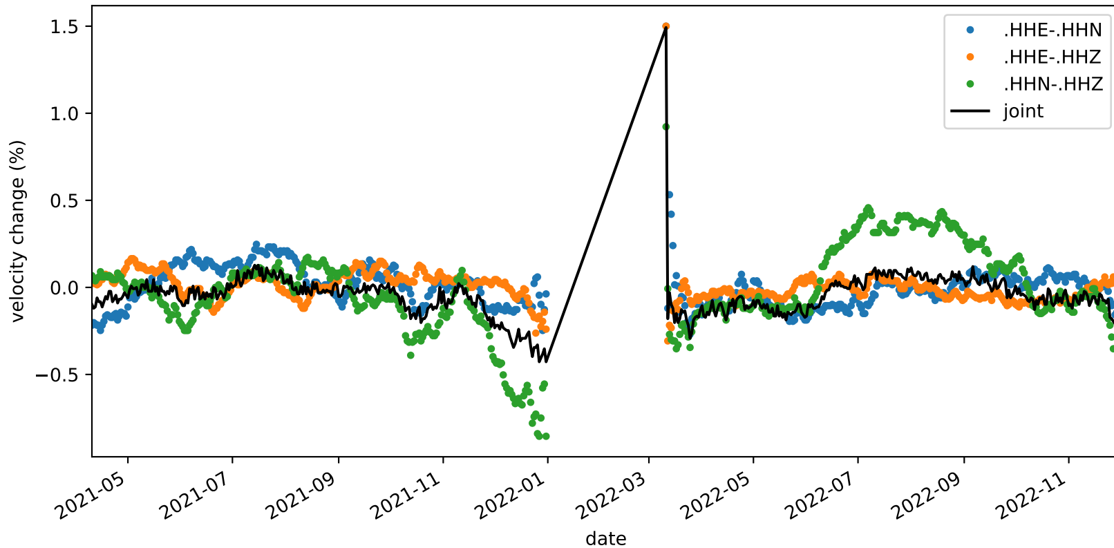
velocity_change_c1e_s2_t1a_tw_005.0s-010.0s_NC.KMPB-NC.KMPB
