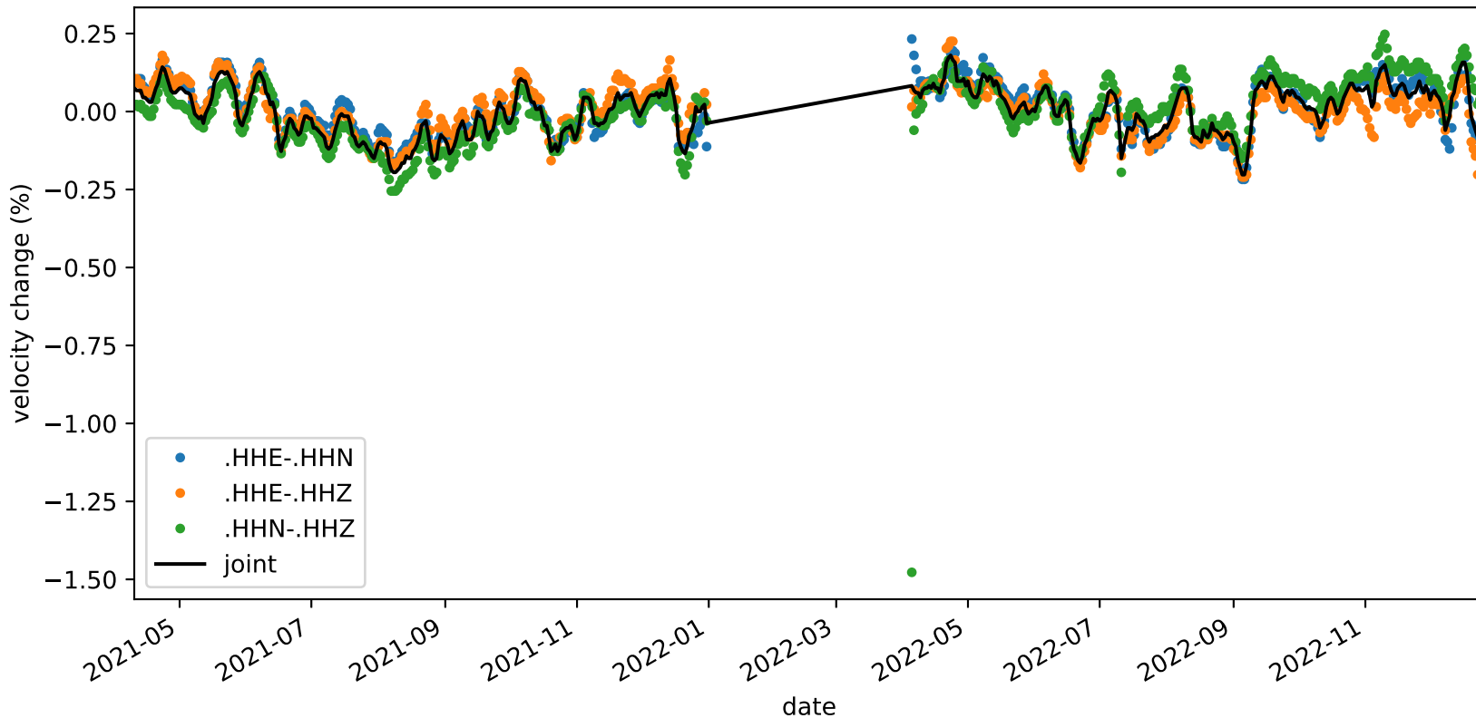
velocity_change_c1c_s4_t1c_tw_005.0s-015.0s_NC.KMPB-NC.KMPB
