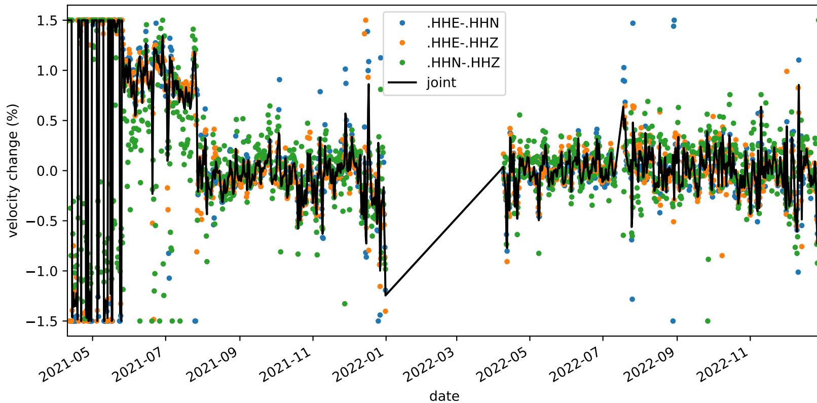
velocity_change_c1f_s1_t1b_tw_010.0s-015.0s_NC.KMPB-NC.KMPB
