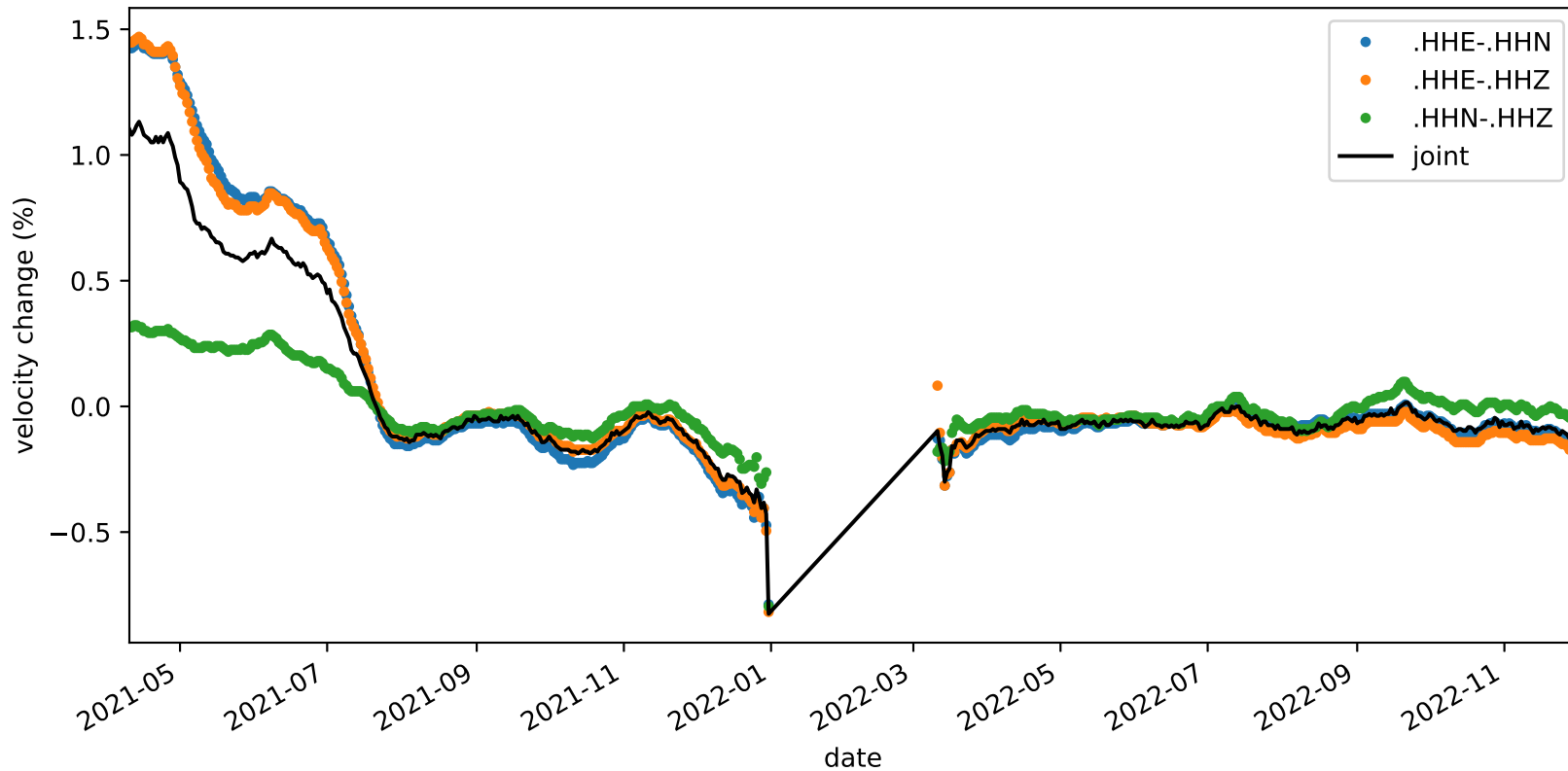
velocity_change_c1b_s2_t1c_tw_005.0s-015.0s_NC.KMPB-NC.KMPB
