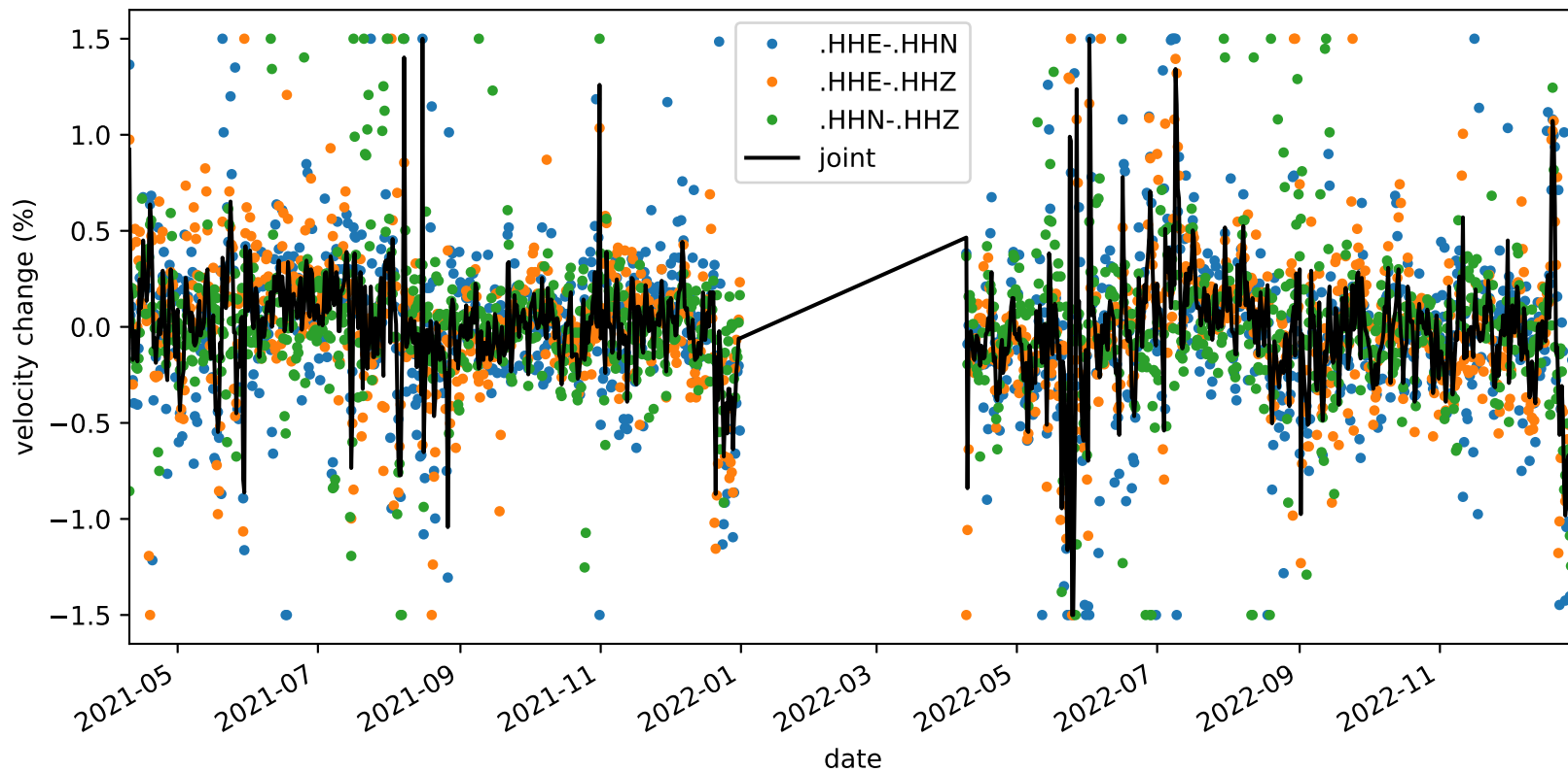
velocity_change_cli_s1_t1a_tw_005.0s-010.0s_NC.KCT-NC.KCT
