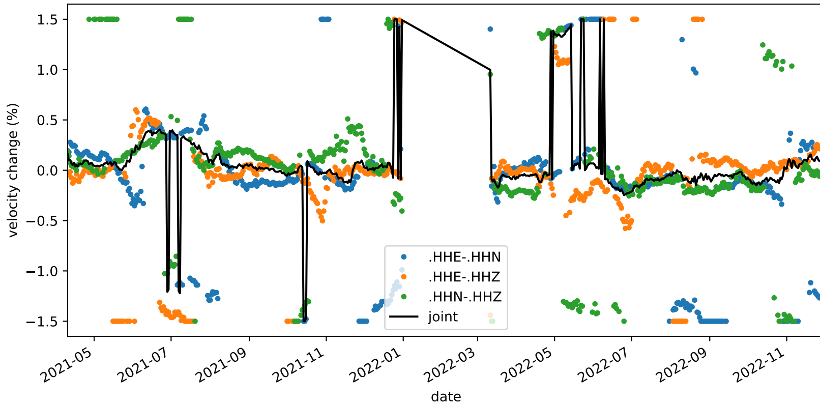
velocity_change_c1_s2_t1b_tw_010.0s-015.0s_NC.KCT-NC.KCT
