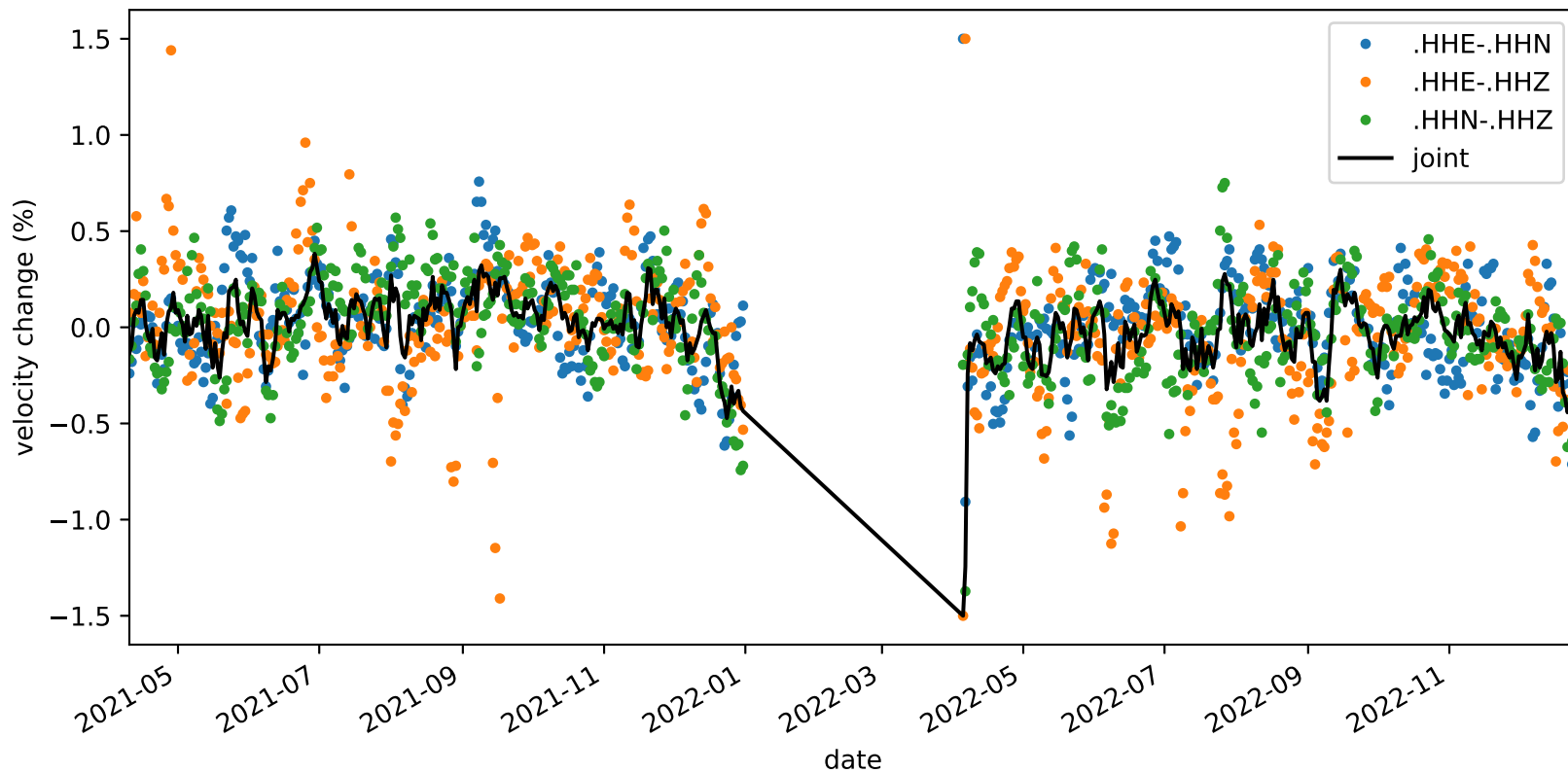
velocity_change_c1g_s4_t1b_tw_010.0s-015.0s_NC.KCT-NC.KCT
