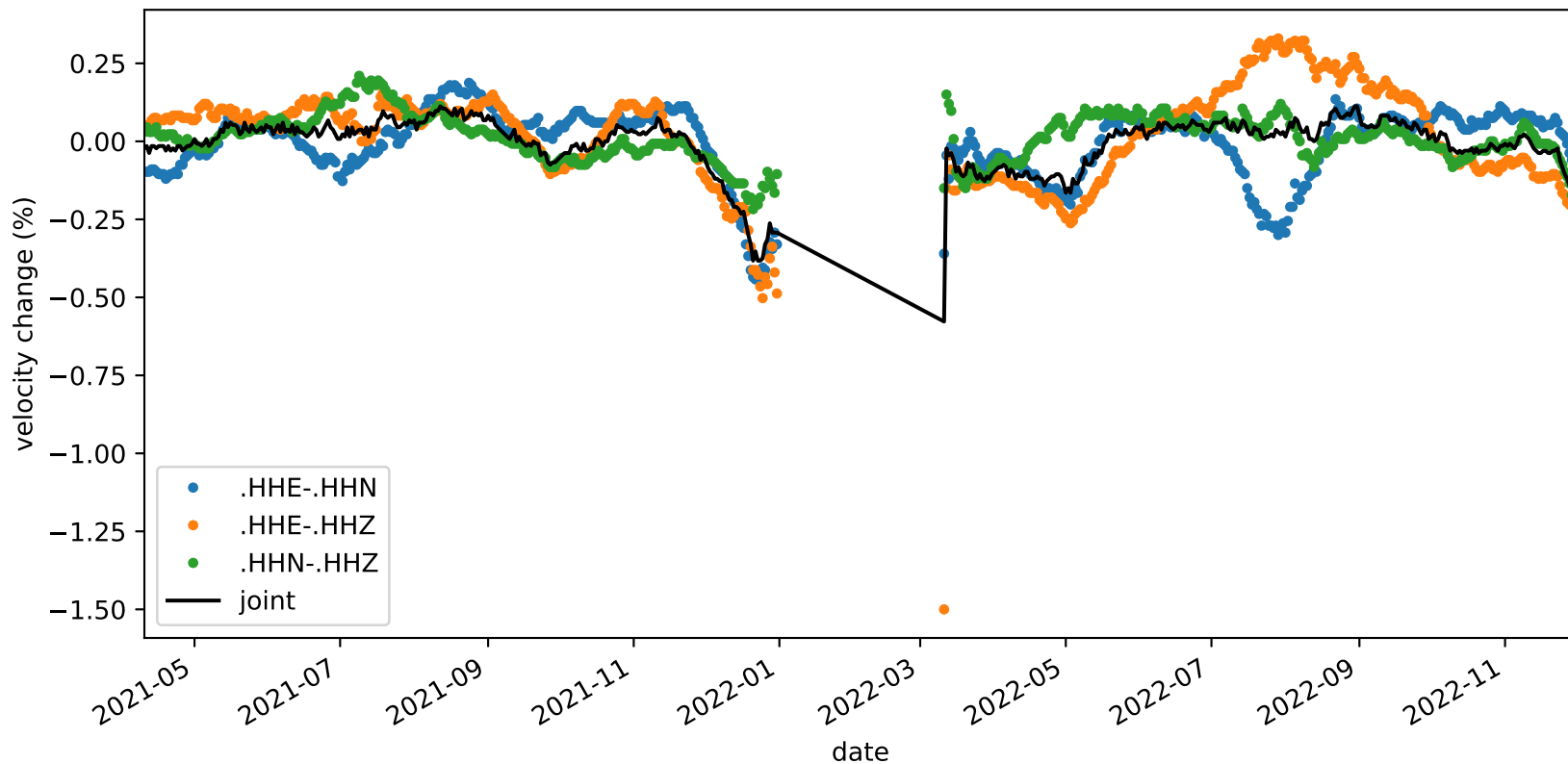
velocity_change_c1b_s2_t1c_tw_005.0s-015.0s_NC.KCT-NC.KCT
