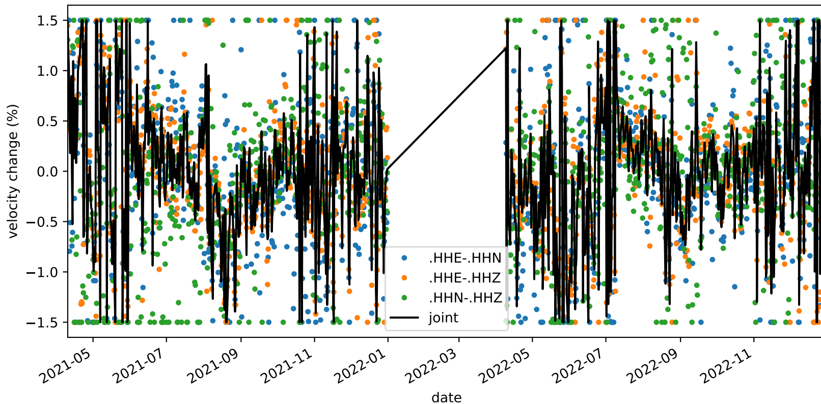
velocity_change_c1_s1_t1a_tw_005.0s-010.0s_NC.KCT-NC.KCT
