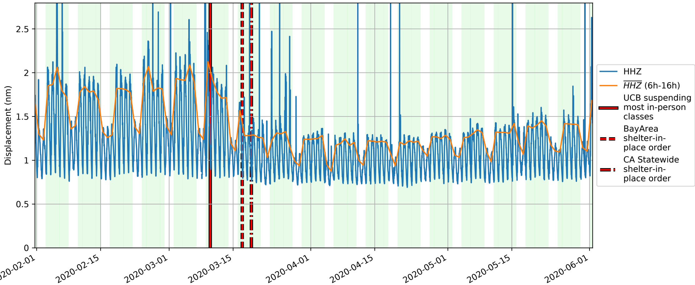
Seismic Noise for BK.BRK.00.HHZ - Filter: [4.0-14.0] Hz
